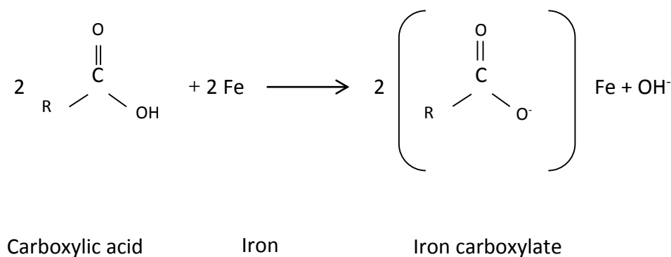
Figure 2.8: Chemical reaction that describes mechanism of Fe (II) adsorption by IDS and CB.
