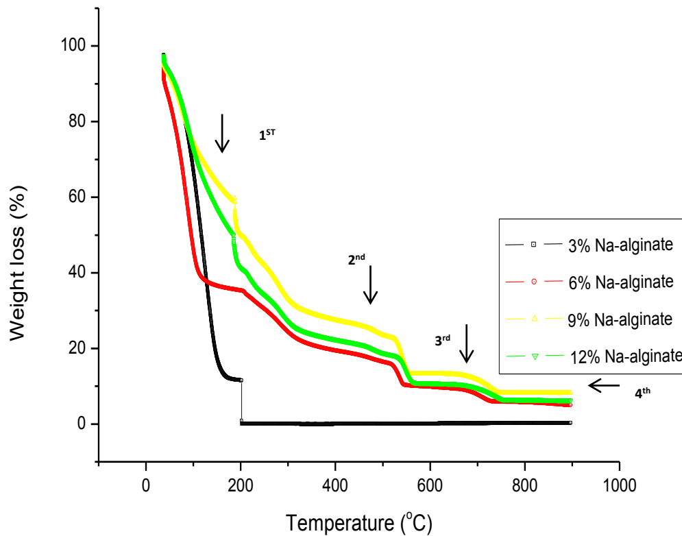
Figure 3.5: Shows TGA curves of CB when various concentrations of Na-alginate were used.
