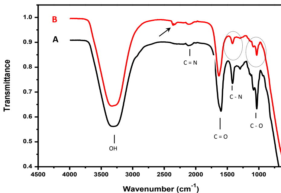
Figure 3.1: The FTIR spectra of (A) IDS before Fe (II) adsorption and (B) after Fe (II) adsorption.
