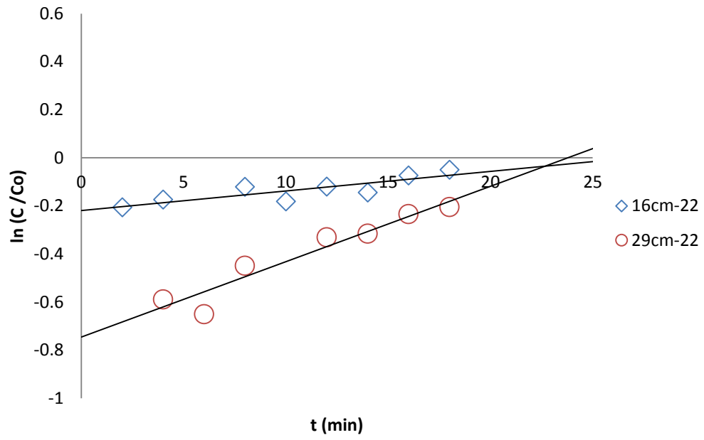
Figure 5.11: Linear plot of Adam-Bohart model with experimental data at different heights of CB. Z = 16 and 29 cm; C_o = 120 mg/L and Q = 22 mL/min.
