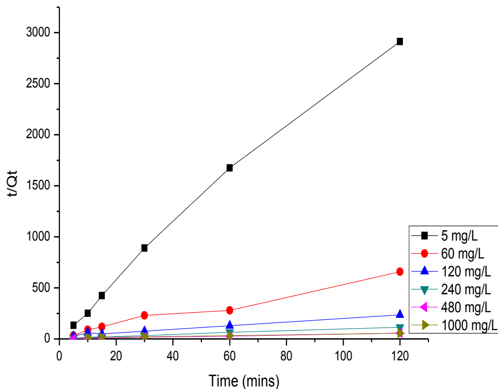
Figure 4.9: Sorption of Fe (II) by immobilized algal beads on pseudo-second-order kinetic model
