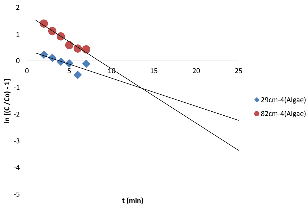
Figure 5.10: Linear plot of Thomas model with experimental data at different heights of IDS. Z = 29 cm and 82 cm; C_0 = 120 mg/L and Q = 4 mL/min.
