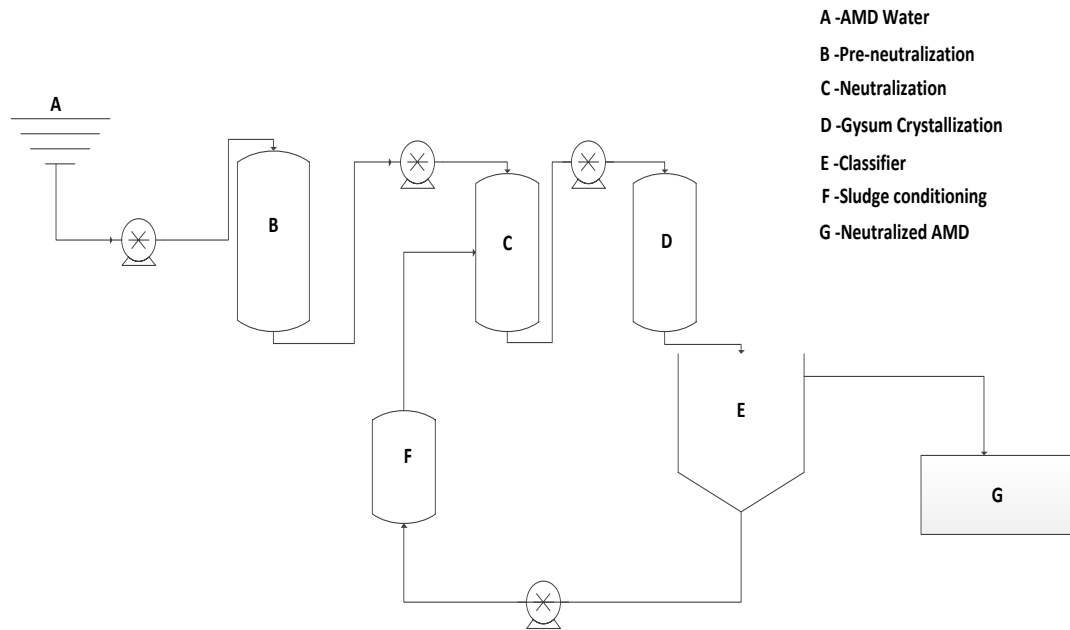
Figure 1.2: The proposed HDS process for the treatment of AMD for the immediate and short term interventions.
