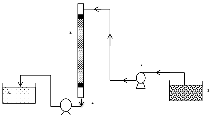
Figure 5.1: Schematic diagram of the experimental column, (1). Feed storage (2); Peristaltic pump (3); Adsorption column and adsorption bed; (4). Outlet liquid; (5) Sample collection
