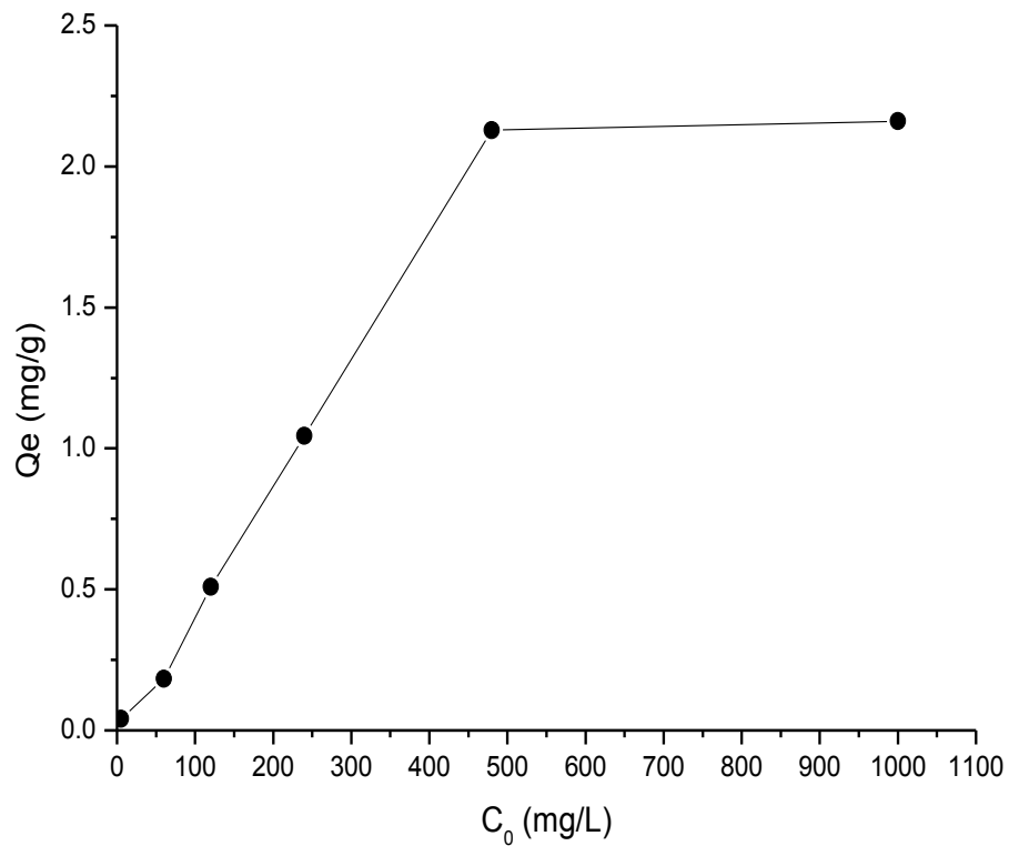
Figure 4.3: Maximum amount of Fe (II) adsorbed per unit amount of adsorbent at various initial concentrations
