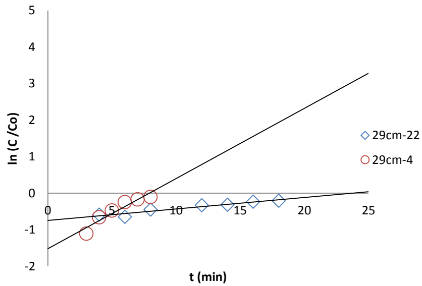
Figure 5.12: Linear plot of Adam-Bohart model with experimental data at different flow rates of CB. Z = 29 cm; C_o = 120 mg/L and Q = 4 and 22 mL/min.
