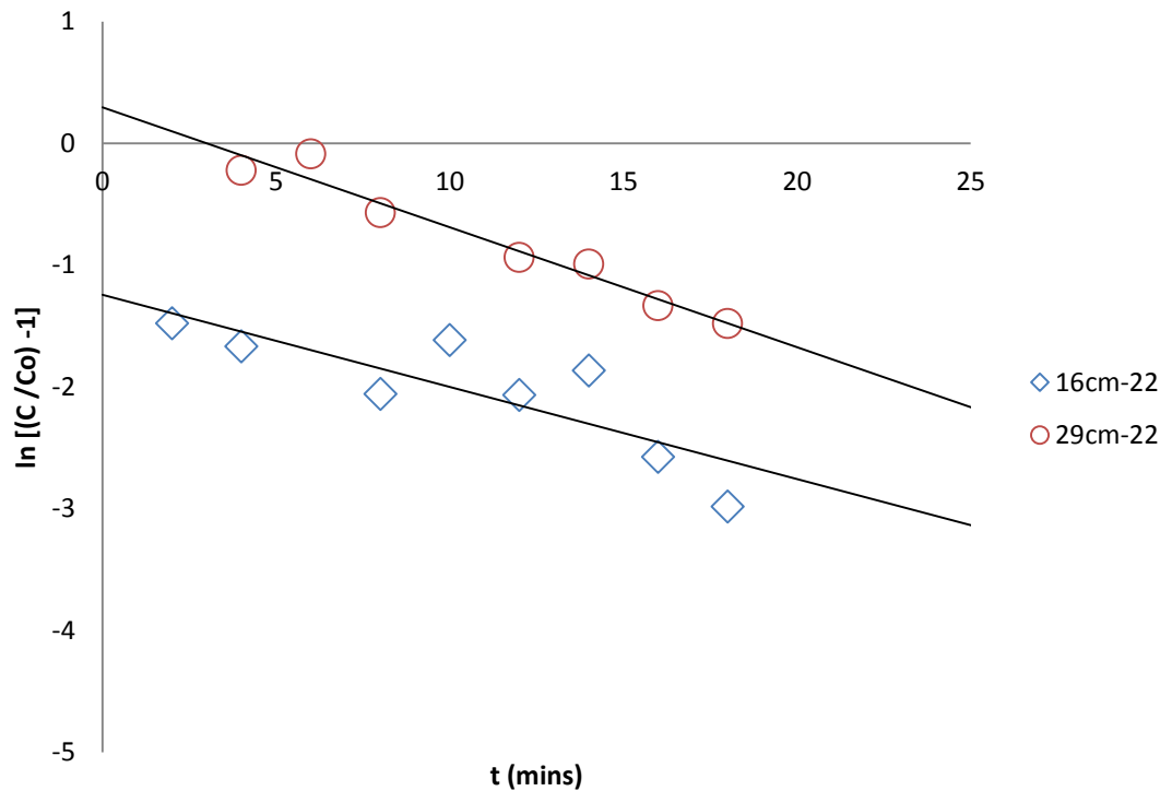
Figure 5.8: Linear plot of Thomas model with experimental data at different bed heights of CB. Z = 16 and 29 cm; C_0 = 120 mg/L and Q = 22 mL/min.
