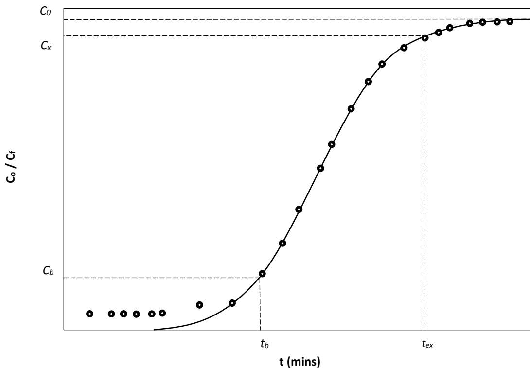
Figure 5.2: A typical S-shaped breakthrough curve
