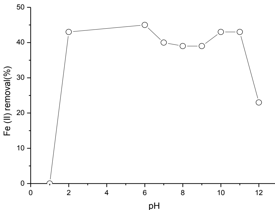
Figure 3.7: The Fe (II) ion uptake at different surface pH of CB.
