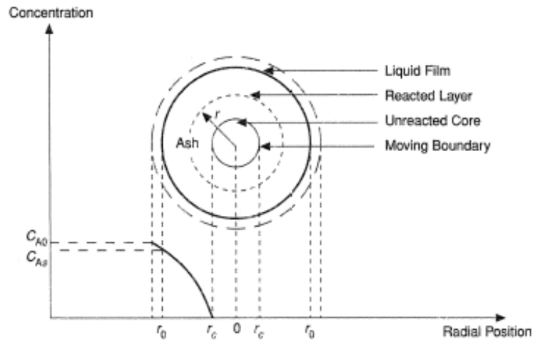
Figure 4.1: Schematic representation of shrinking core model of a spherical particle (Naiya et al., 2009).
