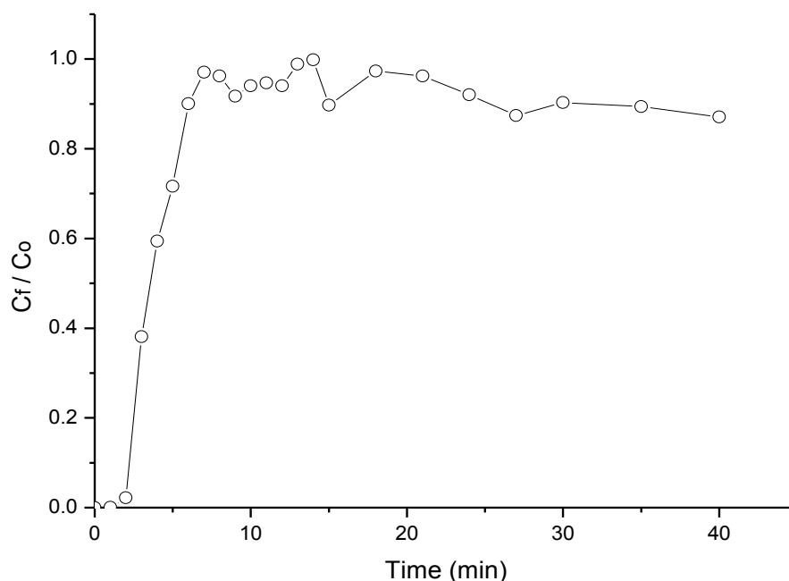
Figure 5.5: Breakthrough curves for Fe (II) adsorption by CB biomass at, Z = 29 cm; C_0 = 120 mg/L and Q = 4 mL/min.
