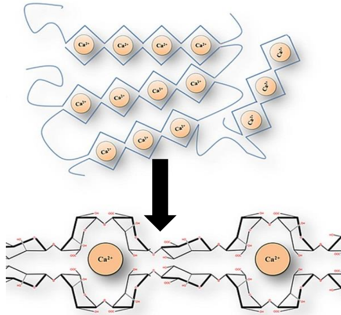
Figure 1.9: Linear block polymers of \beta -d-mannuronate (M) and -l-guluronate (G) with a variation in composition and sequential arrangements being cross-linked by \text{Ca}^{2+} ions to form calcium alginate matrix.
