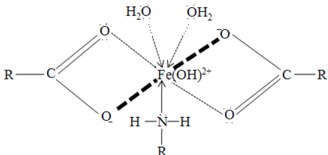
Figure 4.5: Scheme of octahedral coordination formed by Fe (II) adsorption on the function groups found in IDS (Aryal & Liakopoulou-Kryiakides, 2013)
