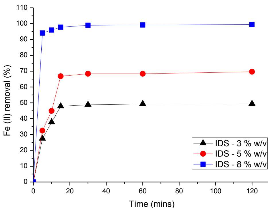
Figure 3.10: Removal of Fe (II) ion concentration in the presence of beads with various biomass concentrations.
