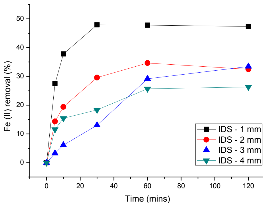
Figure 3.9: Removal of Fe (II) ion concentration with time when 1; 2; 3 and 4 mm IDS are used.
