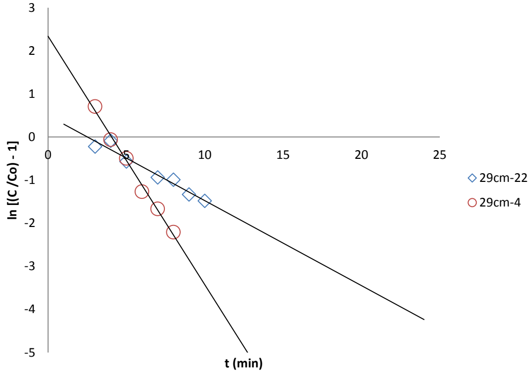
Figure 5.9: Linear plot of Thomas model with experimental data at flow rates of CB. Z = 29 cm; C_0 = 120 mg/L and Q = 4 and 22 mL/min.
