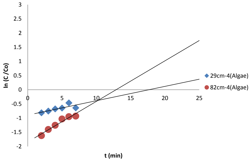
Figure 5.13: Linear plot of Adam-Bohart model with experimental data at different heights of IDS. Z = 29 and 82 cm; C_o = 120 mg/L and Q = 4 mL/min.
