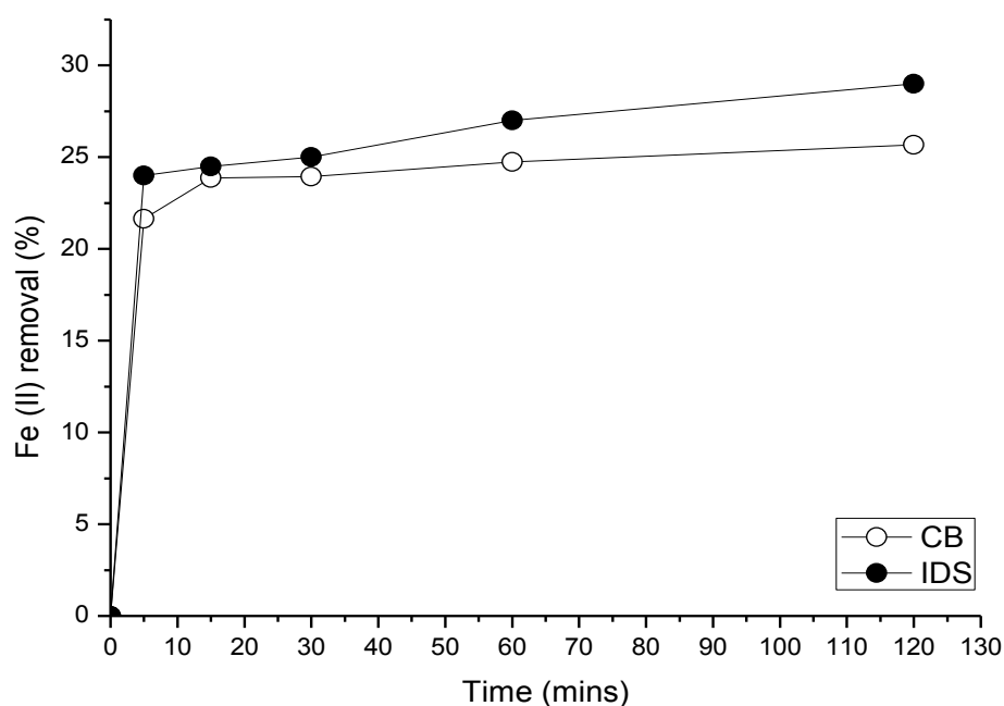
Figure 2.7: The study of loading capacity of CB and IDS in the presence of Fe (II) at 120 mg/L and pH 2.5. Three mm bead diameter of beads was used.
