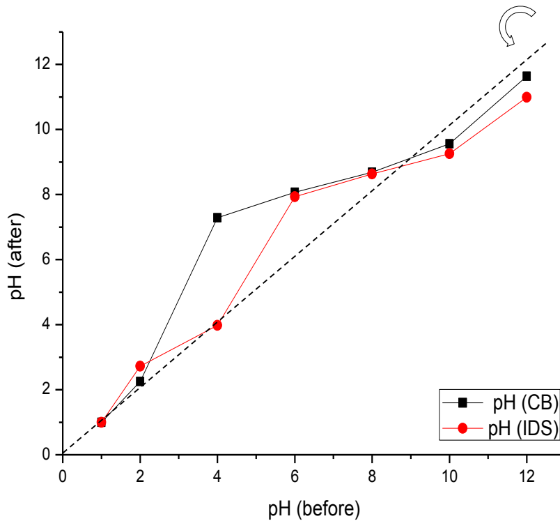
Figure 3.6: The point of zero charge ( \text{pH}_{\text{pzc}} ) for biosorbents IDS at pH 8.8 and CB obtained at pH 9.2.
