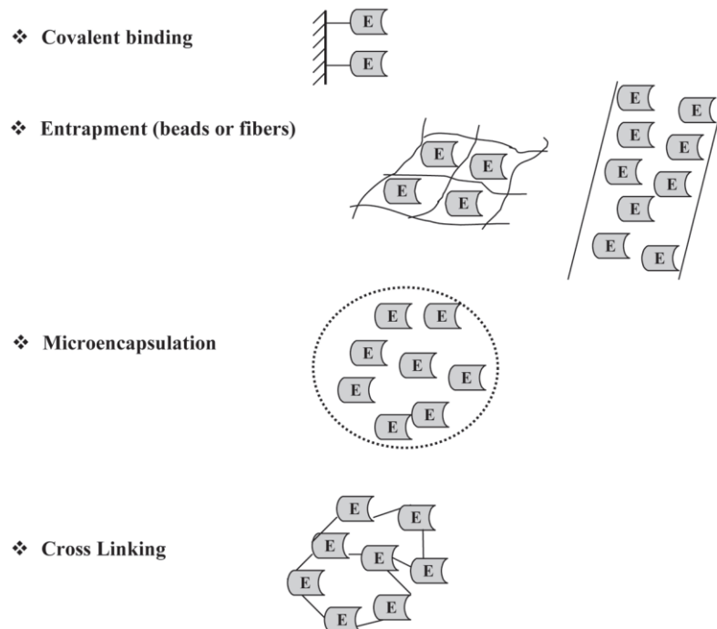
Figure 1.8: Immobilization systems: covalent attachment to an insoluble particle; entrapment within an insoluble particle by a cross-linked polymer; confinement within a semipermeable membrane; and cross-linkage (Guisán, 2006).
