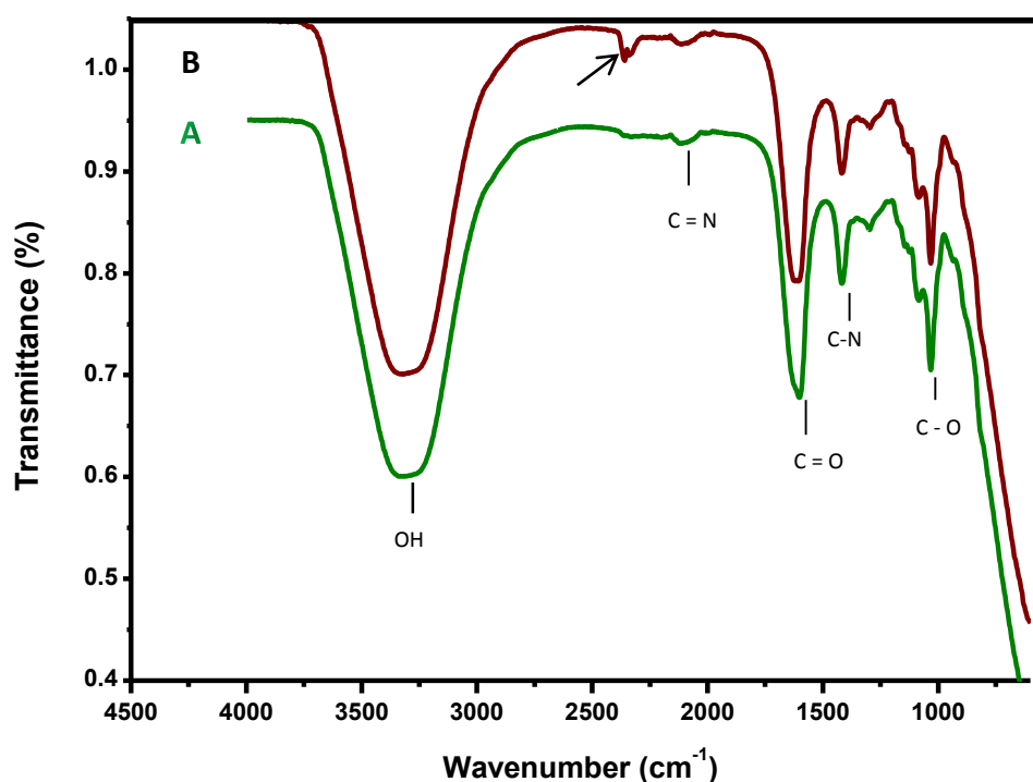
Figure 3.2: FTIR spectra of CB (A) before Fe (II) adsorption and (B) after Fe (II) adsorption
