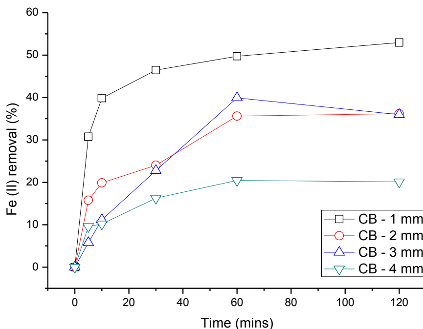
Figure 3.8: Removal Fe (II) ion concentration with time when 1; 2; 3 and 4 mm CB are used.
