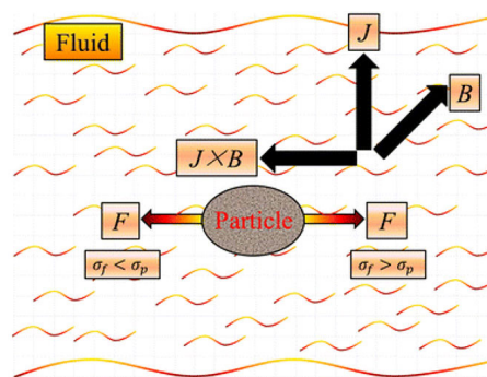
Figure 5—Electromagnetic forces on a spherical particle associated with a single particle in crossed electric and magnetic fields (Zhang et al., 2014). The direction of movement of the particle depends on the electrical conductivity difference between the fluid and the particle
