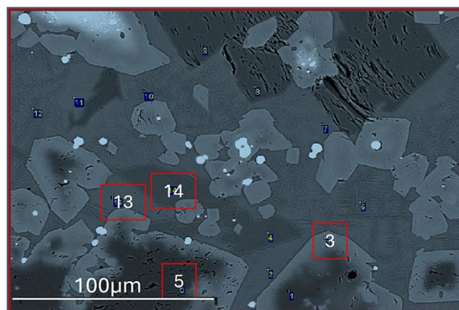
Figure 4a—Microstructure of Cr-bearing spinel particles in air-cooled FeCr slag, showing the typical phases of interest: 13-glass, 5-Mg-Al spinel, 3-Mg-Al-Cr spinel, 14-pyroxene (Tanskanen and Makonnen, 2007)
