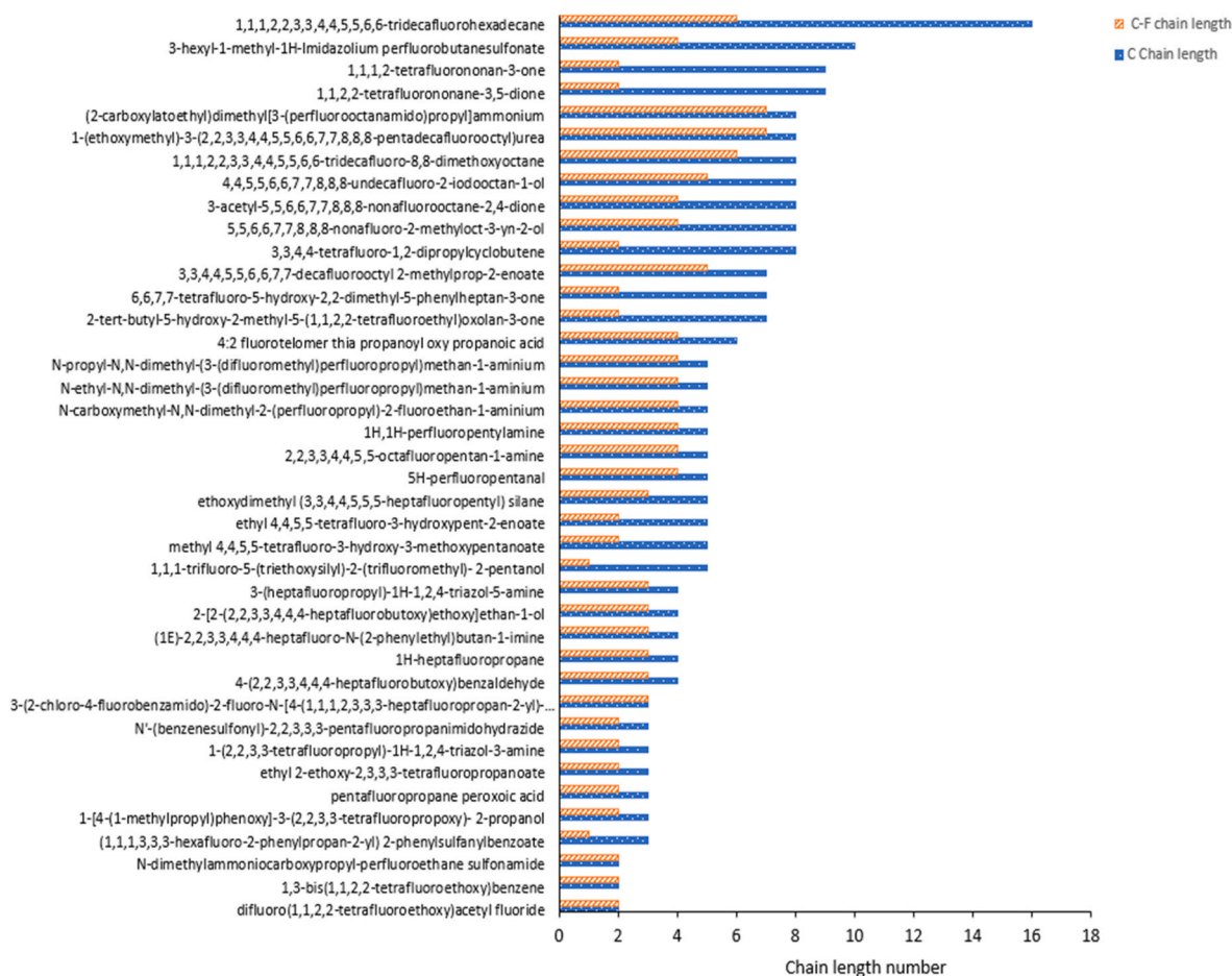
Fig. 4. Carbon chain lengths of identified PFAS.
