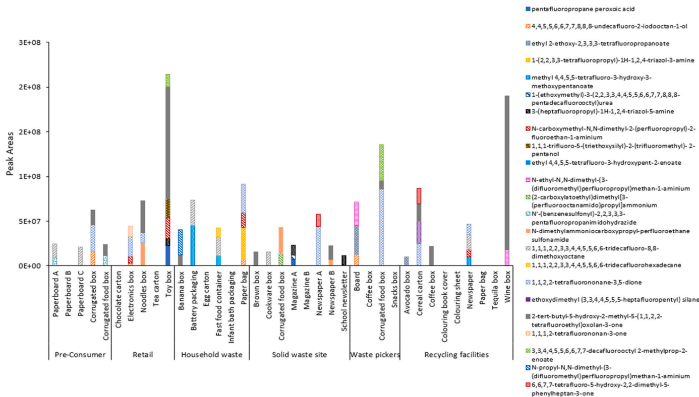
Fig. 6. Average peak areas of identified PFAS from UAE sample pre-treatment.
