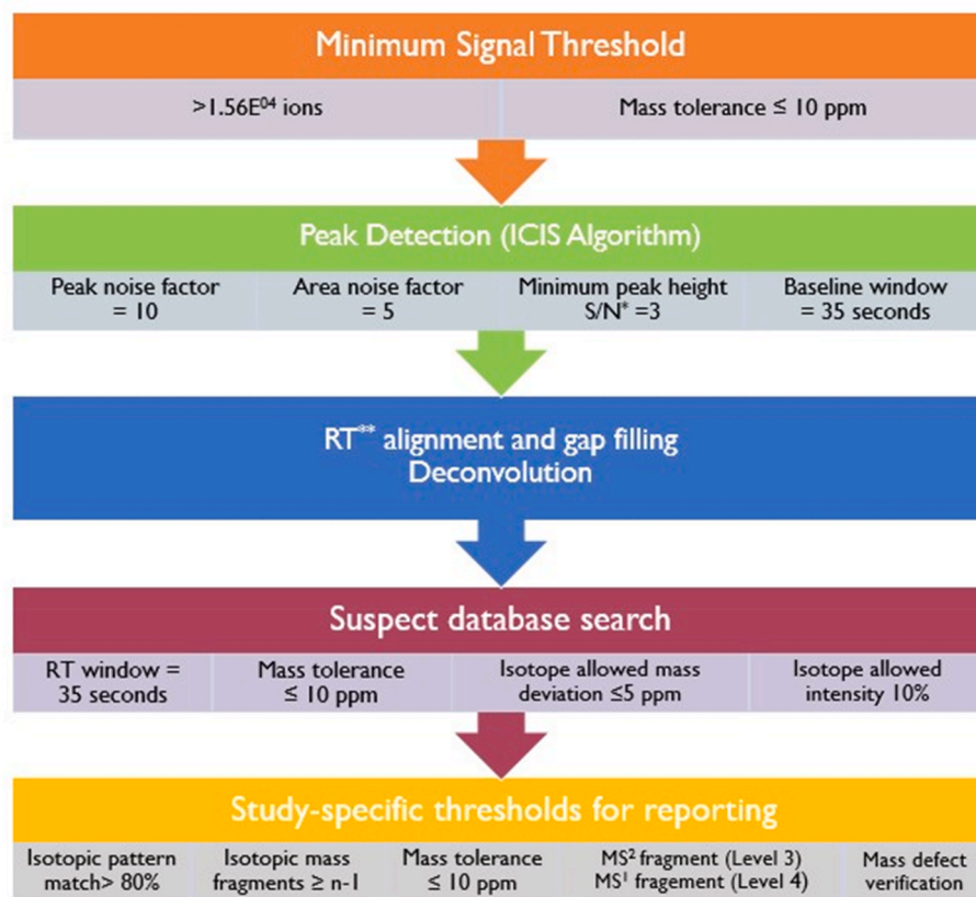
Fig. 1. Suspect screening protocol.
