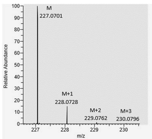
Fig. 3. Isotopic pattern for [M – H] 227.0701 m/z
