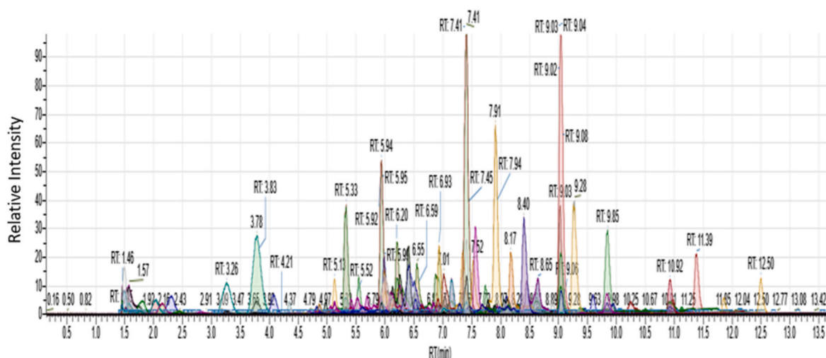
Fig. 2. XIC for magazine sample.
