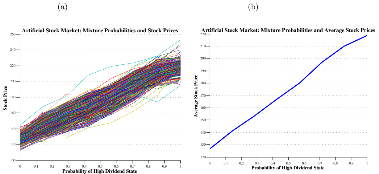
Figure 19: Multiple Stock Mixed Gaussian Multiple Stock Mixed Gaussian Artificial Stock Market: Relationship Between Stock Prices and Underlying Variables (Stock Market) - Panel C.
