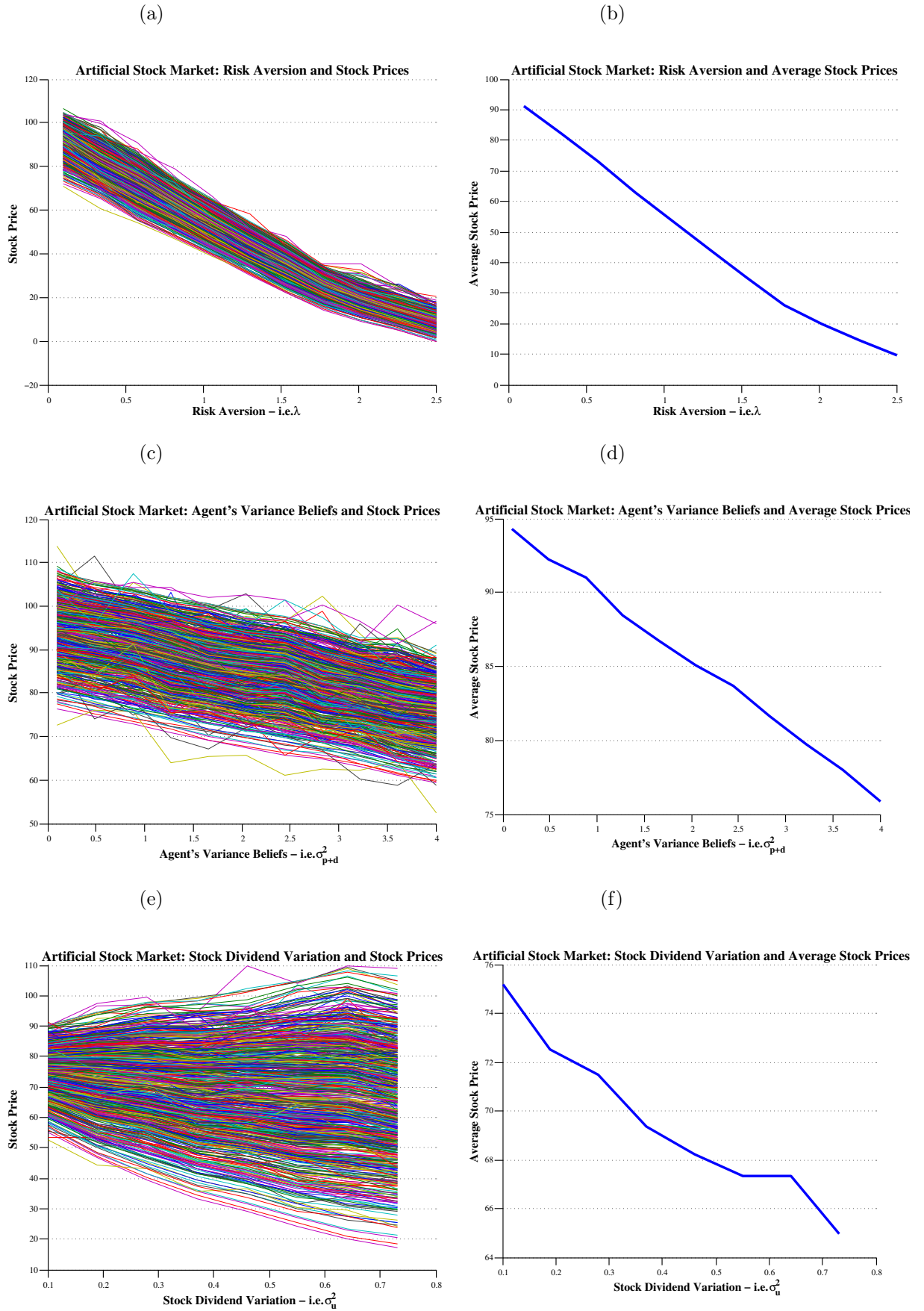
Figure 1: Impact of Parameters on the agent-based SFASM: Parameters impact the model in a plausible manner (Panel A)
