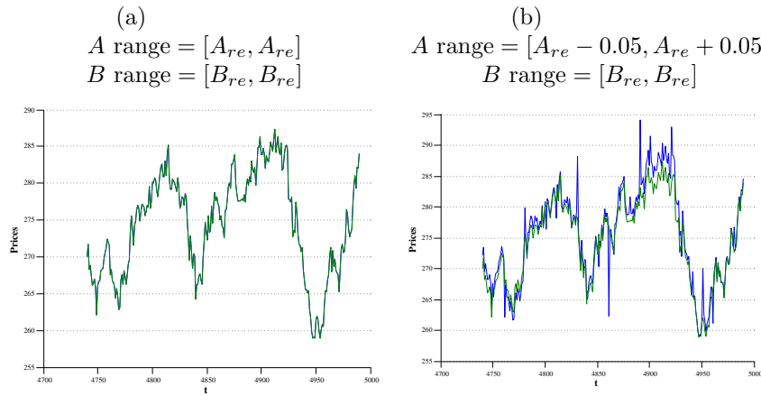
Figure 8: Single-Stock Mixed Gaussian Agent-Based Model Stock Prices and Theoretical Stock Prices.
