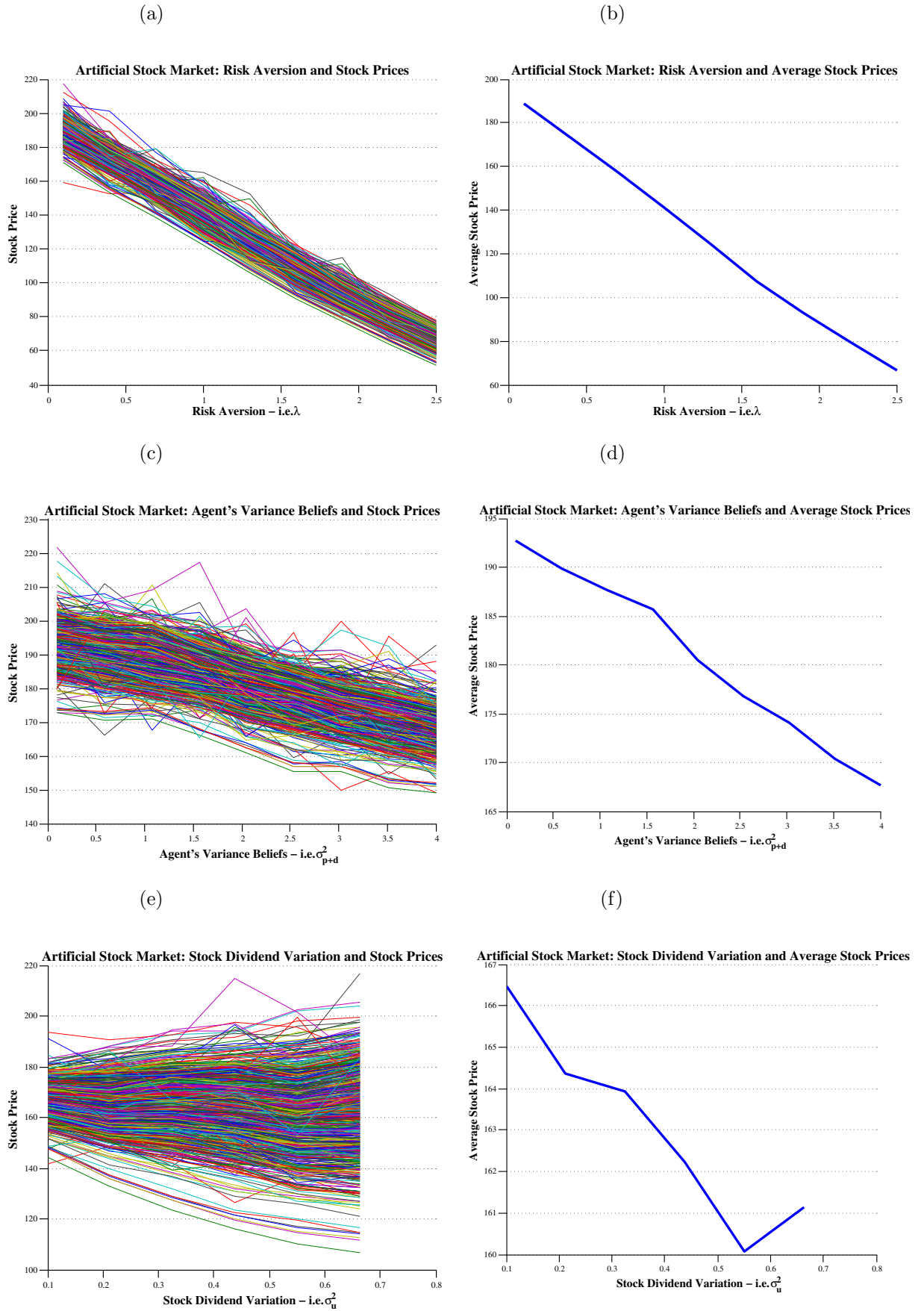
Figure 3: Multivariate Artificial Stock Market: Relationship Between Stock Prices and Underlying Variables (Asset 2) - Panel A.
