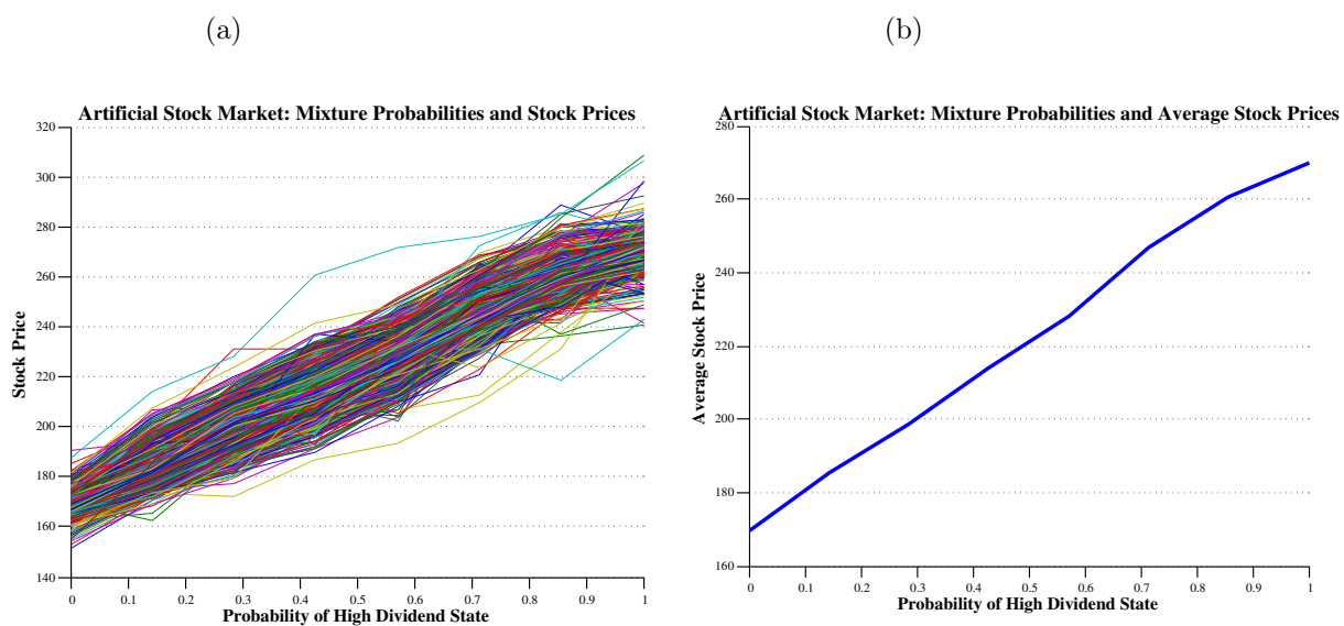
Figure 13: Multiple Stock Mixed Gaussian Multiple Stock Mixed Gaussian Artificial Stock Market: Relationship Between Stock Prices and Underlying Variables (Asset 1) - Panel C.
