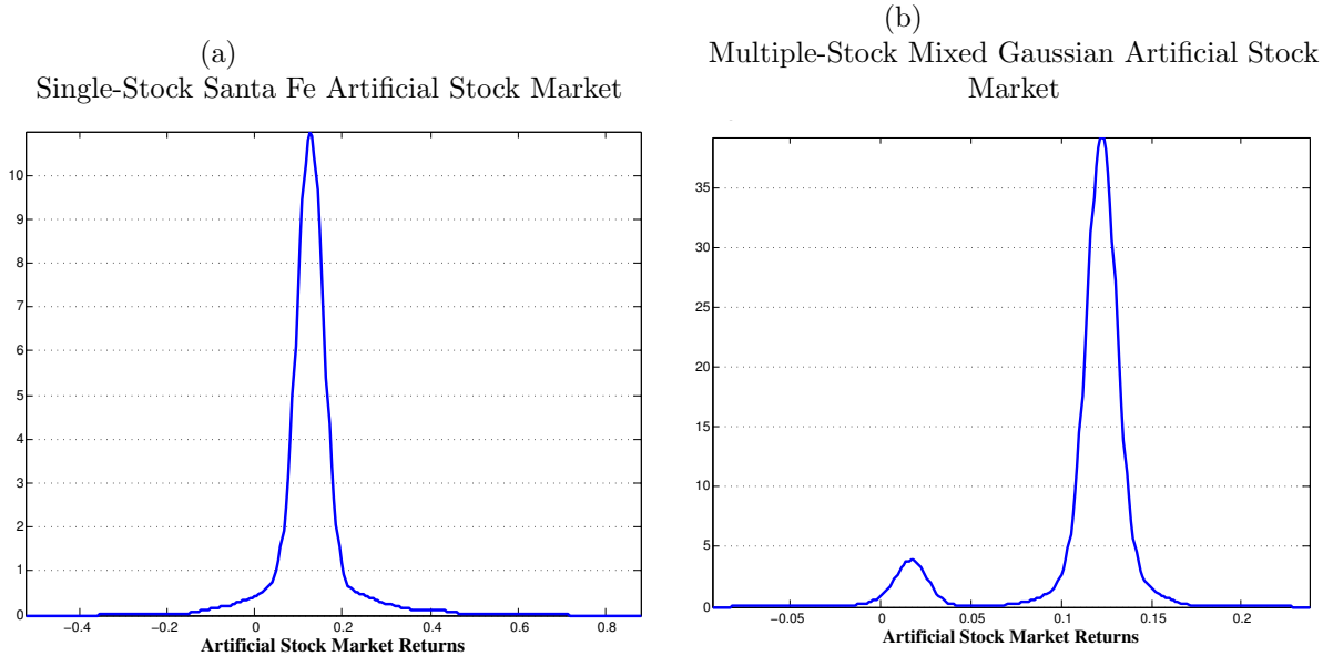
Figure 10: Density Estimate of Artificial Stock Market Returns (Multiple-Stock Mixed Gaussian Artificial Stock Market)
