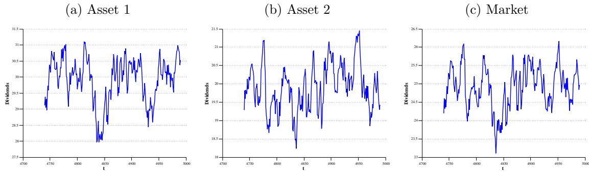
Figure 20: Multiple Stock Mixed Gaussian Artificial Stock Market Agent-Based Model Stock Dividend Process.
