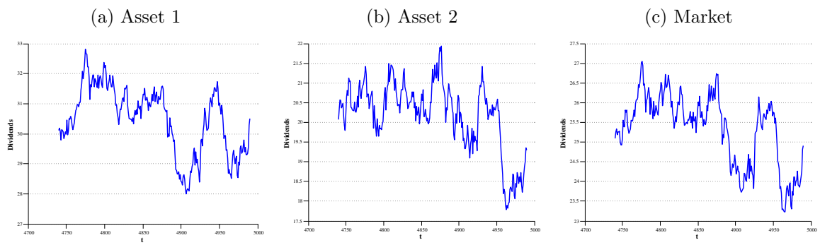
Figure 7: Agent-Based Model Stock Dividend Process (Multivariate model).
