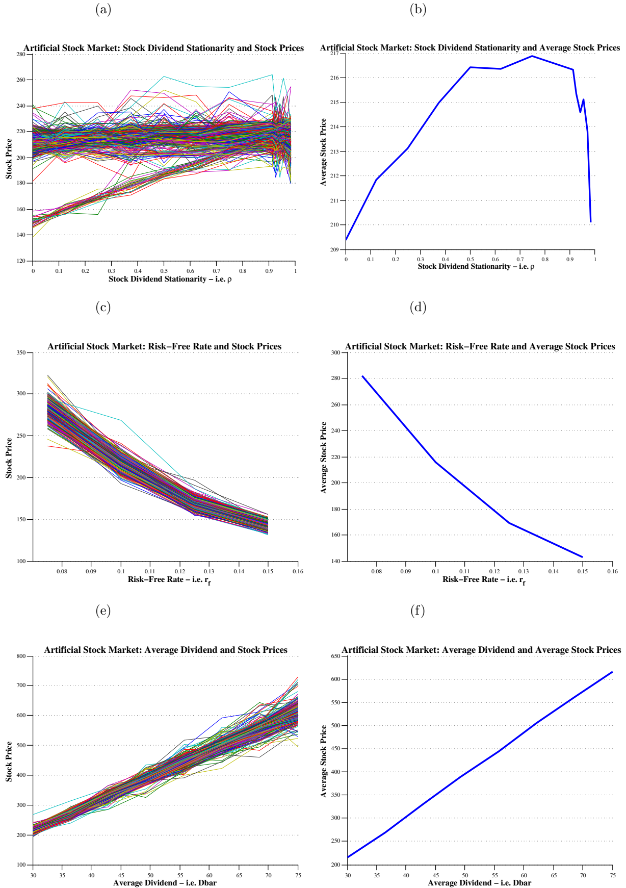
Figure 18: Multiple Stock Mixed Gaussian Artificial Stock Market: Relationship Between Stock Prices and Underlying Variables (Stock Market) - Panel B.
