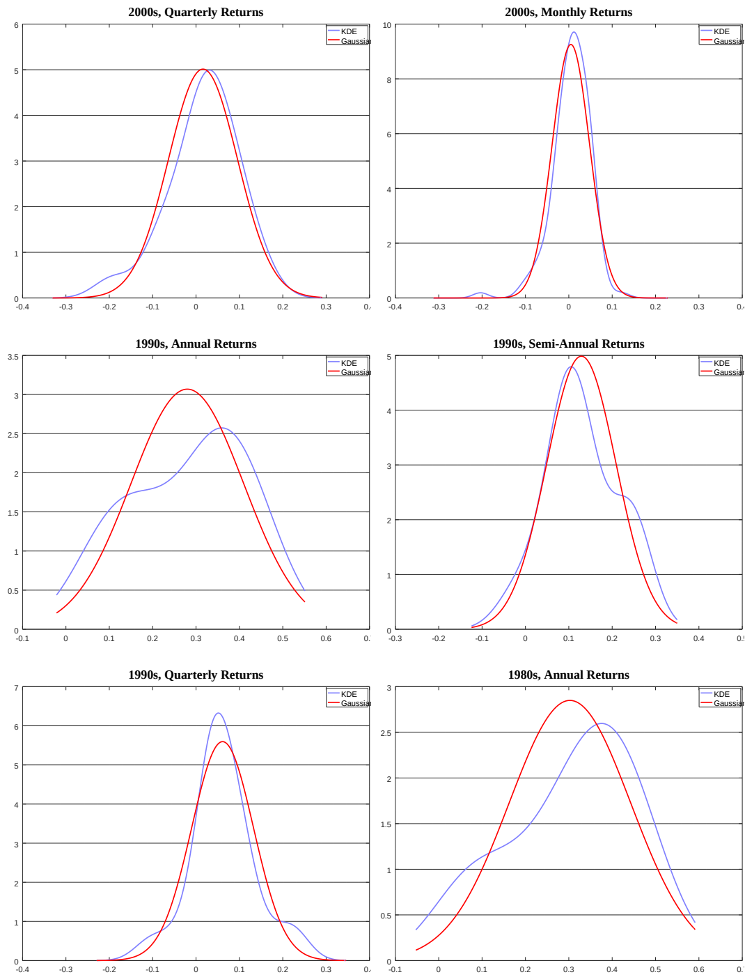
Figure 7: Kernel Density Estimates of S&P 500 Stock Market Returns (Multivariate Mixed Model) - Panel F
