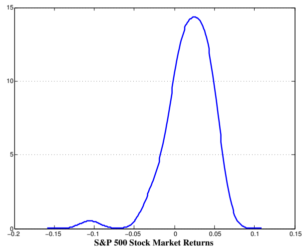
Figure 1: Density Estimate of Monthly S&P 500 Stock Market Returns (June 2010 - June 2015) - Multivariate Mixed Model
