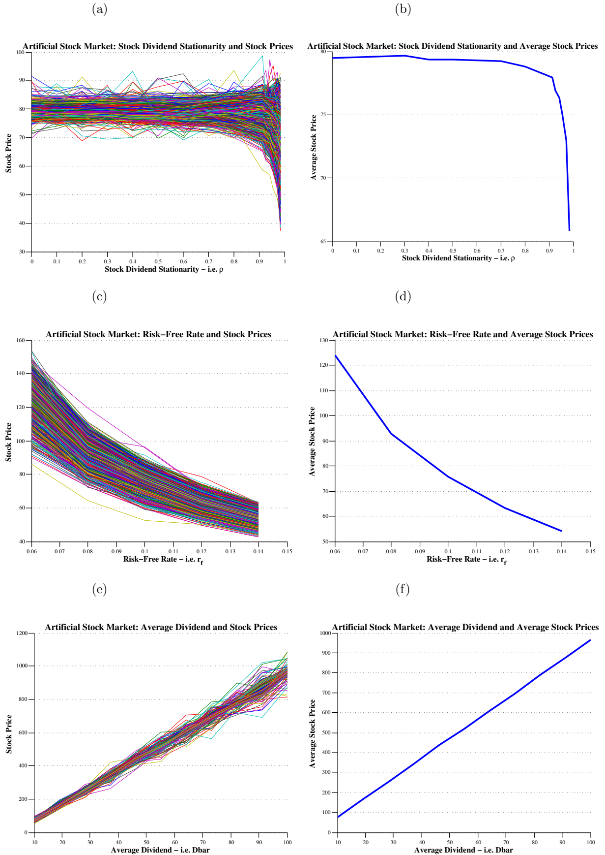
Figure 2: Impact of Parameters on the agent-based SFASM: Parameters impact the model in a plausible manner (Panel B)
