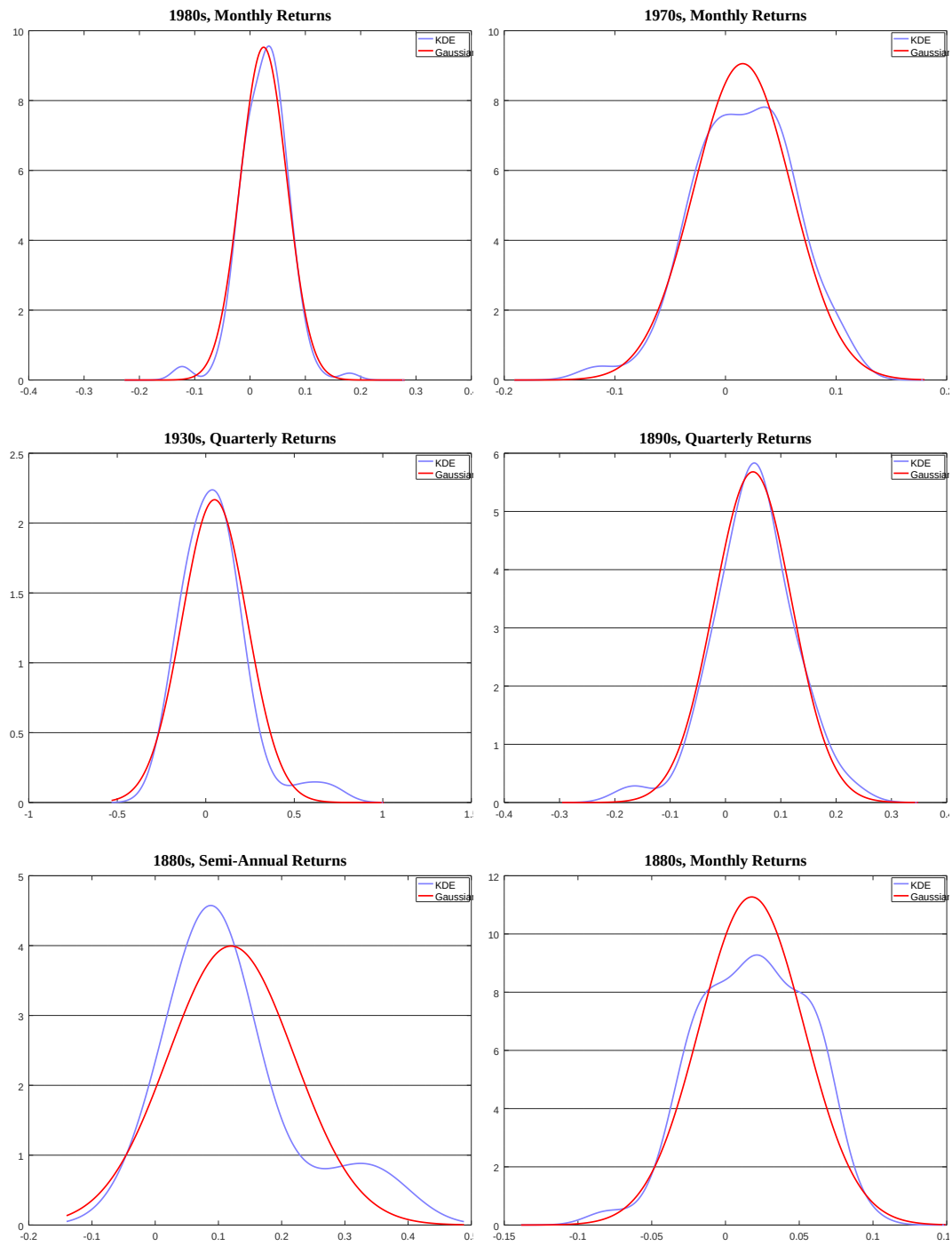
Figure 8: Kernel Density Estimates of S&P 500 Stock Market Returns (Multivariate Mixed Model) - Panel G
