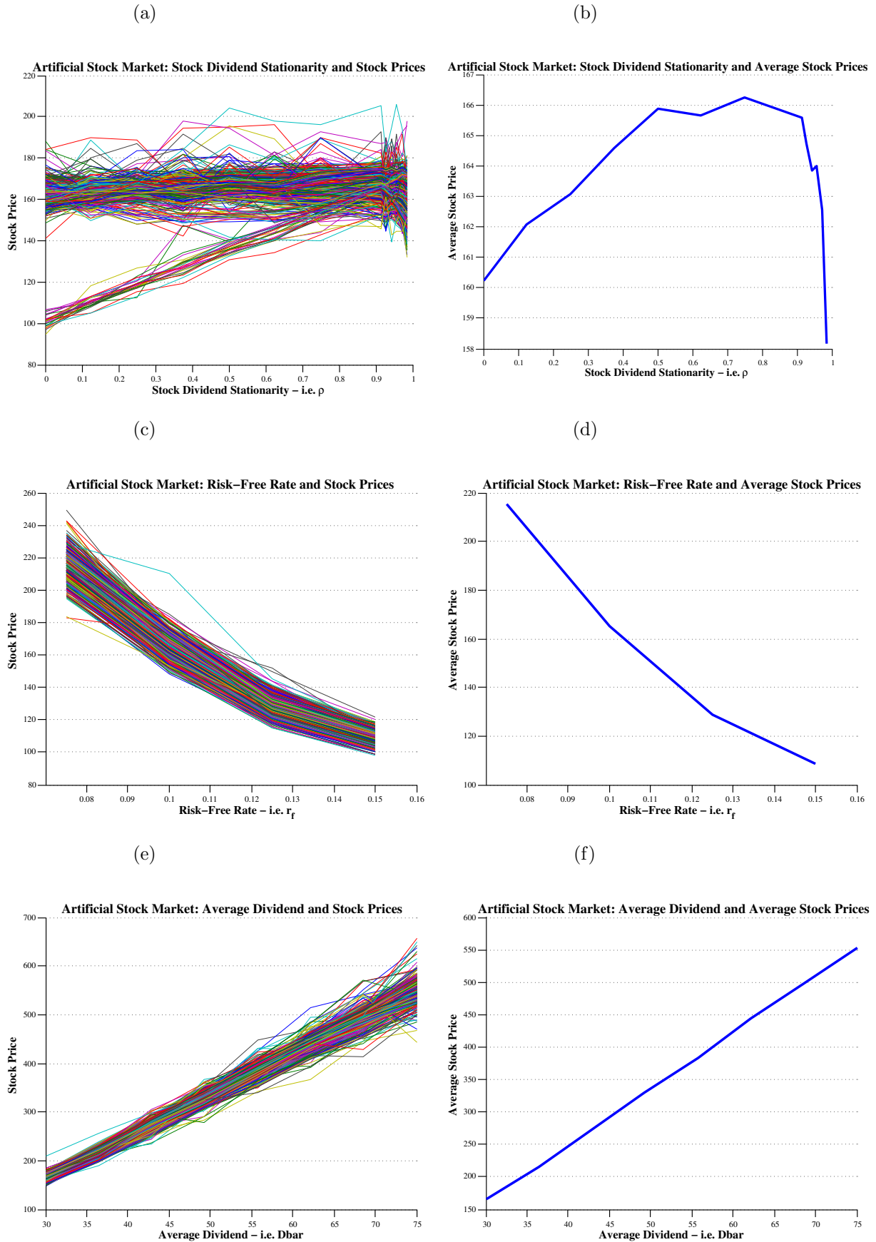
Figure 15: Multiple Stock Mixed Gaussian Artificial Stock Market: Relationship Between Stock Prices and Underlying Variables (Asset 2) - Panel B.
