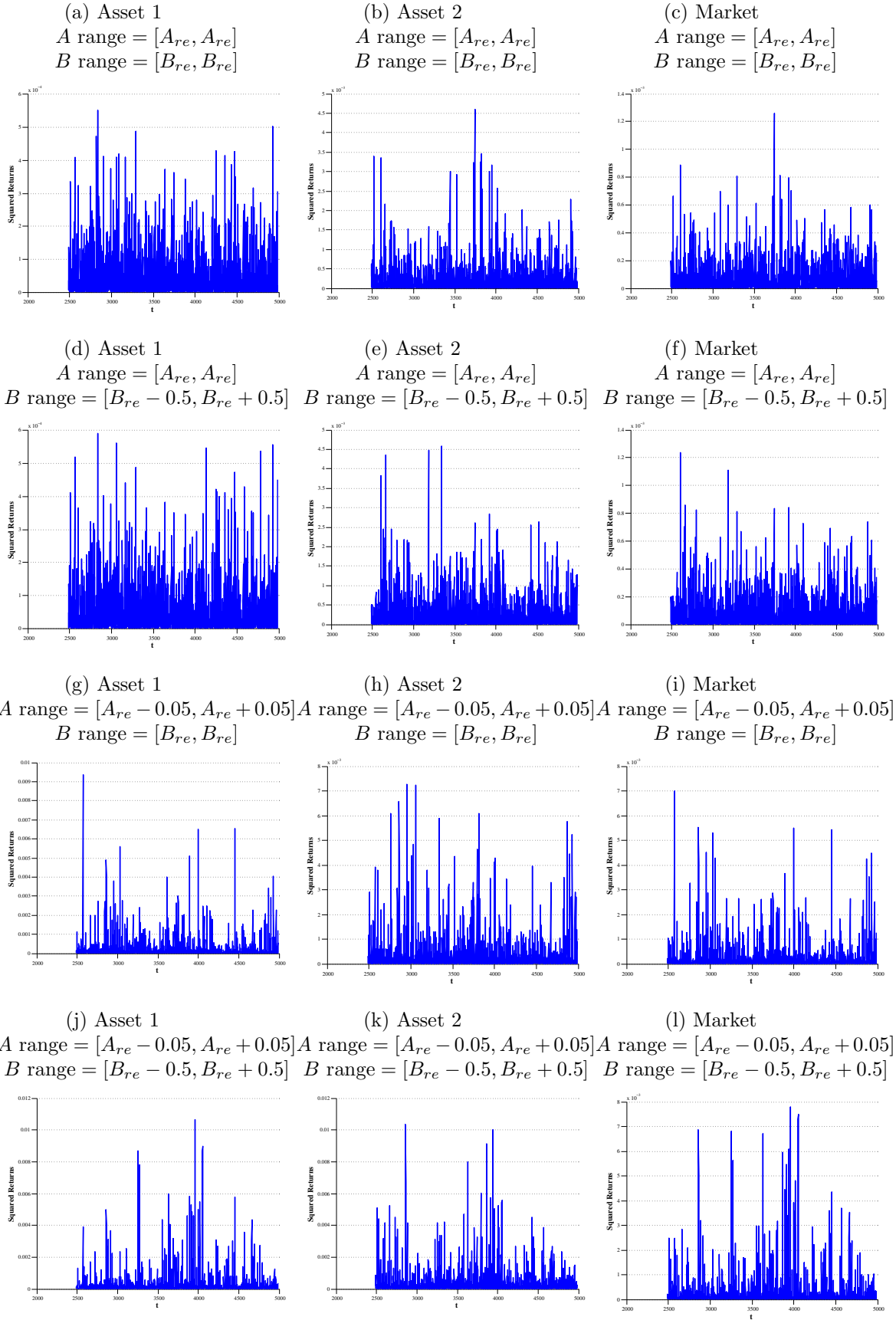
Figure 9: Multivariate Agent-Based Model Squared Stock Returns.
