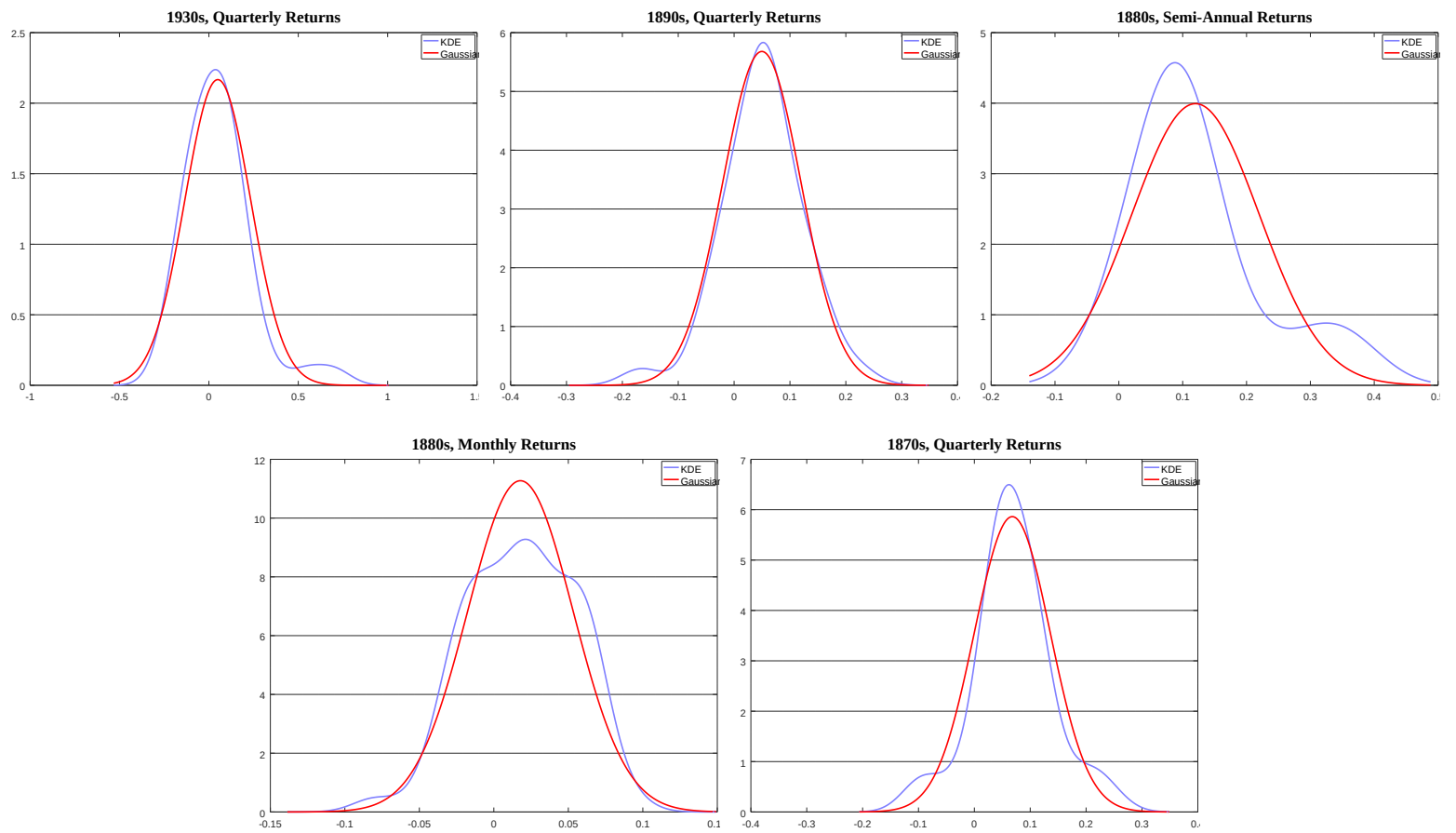
Figure 3: Kernel Density Estimates of S&P 500 Stock Market Returns (Single-Stock Santa Fe Artificial Stock Market) - Panel B.
