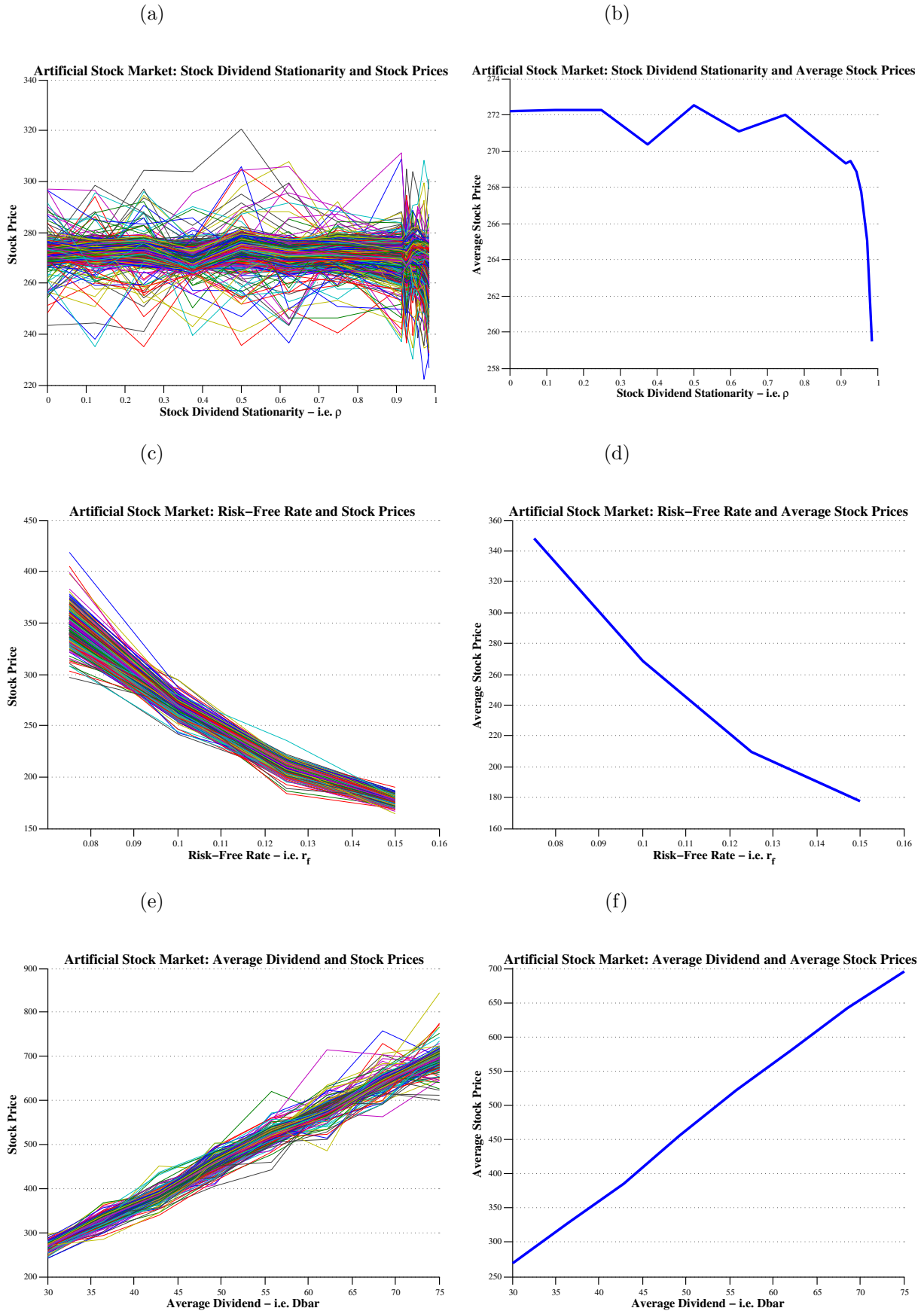
Figure 2: Multivariate Artificial Stock Market: Relationship Between Stock Prices and Underlying Variables (Asset 1) - Panel B.
