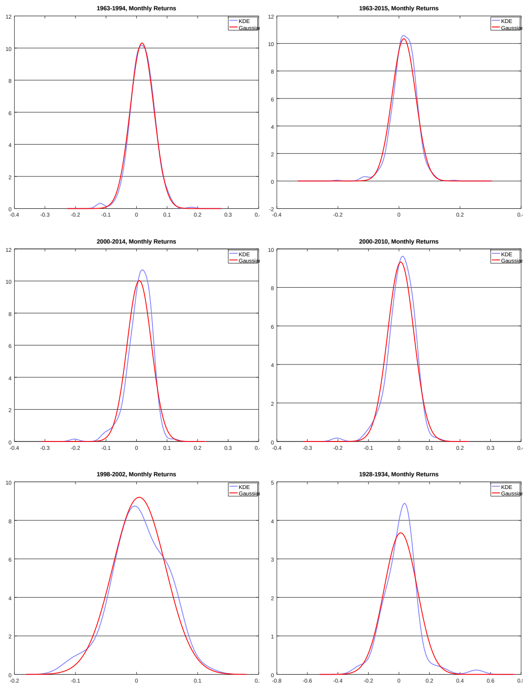
Figure 2: Kernel Density Estimates of S&P 500 Stock Market Returns (Multivariate Mixed Model) - Panel A
