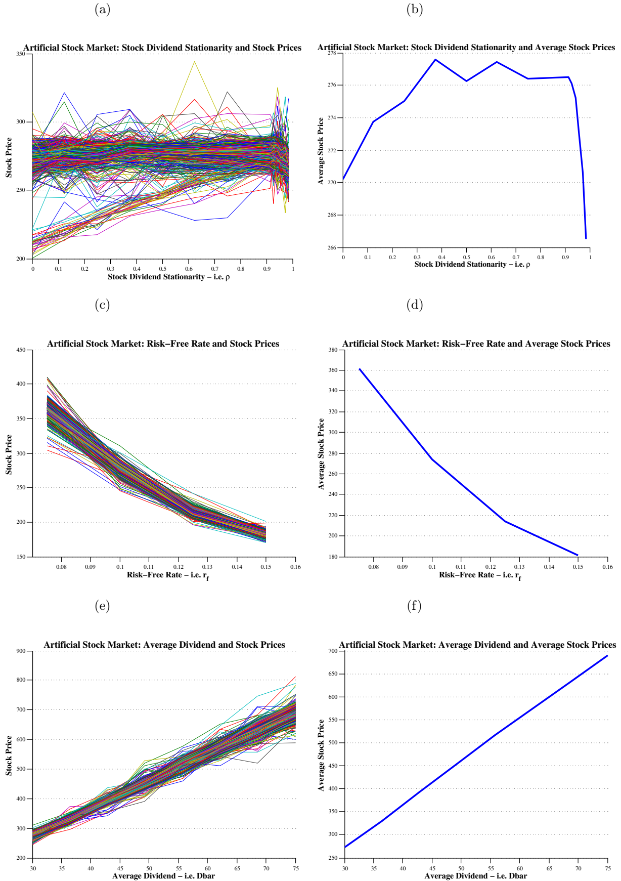
Figure 6: Single Stock Mixed Gaussian artificial stock market: Relationship Between Stock Prices and Underlying Variables - Panel B.
