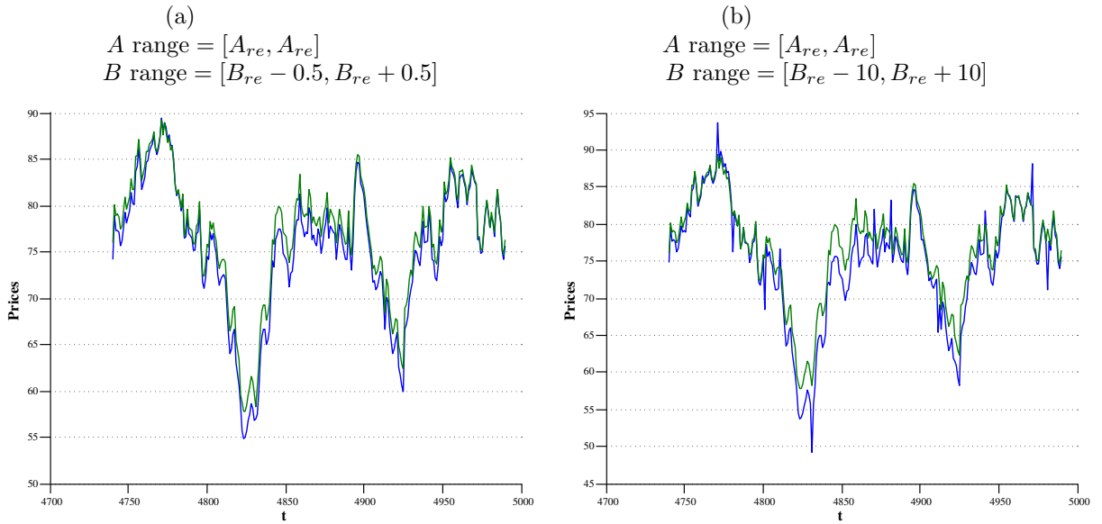
Figure 3: Agent-Based Model Stock Prices and Theoretical Stock Prices: mispricing is higher if agents have more uncertain beliefs regarding the stock market (Santa Fe model).
