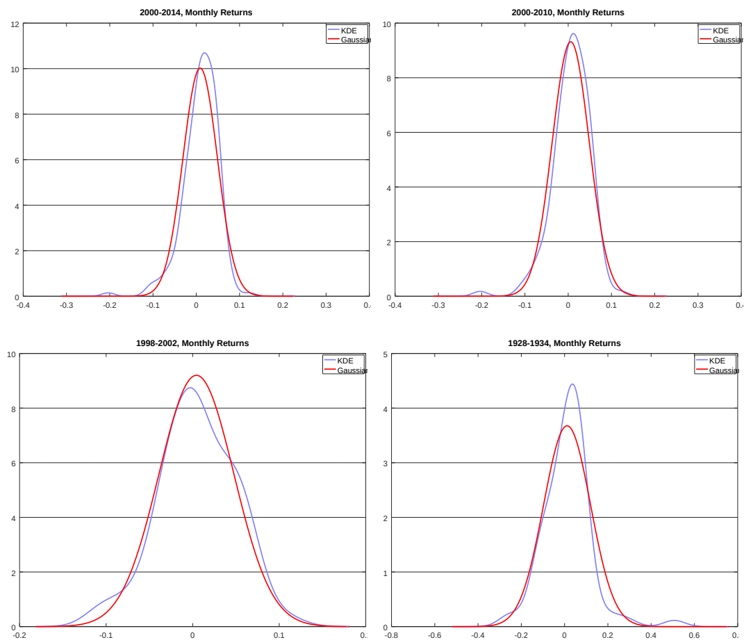
Figure 3: Kernel Density Estimates of S&P 500 Stock Market Returns (Multivariate Mixed Model) - Panel B
