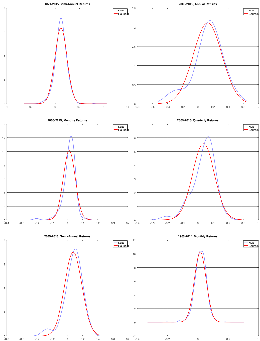
Figure 4: Kernel Density Estimates of S&P 500 Stock Market Returns (Multivariate Mixed Model) - Panel C
