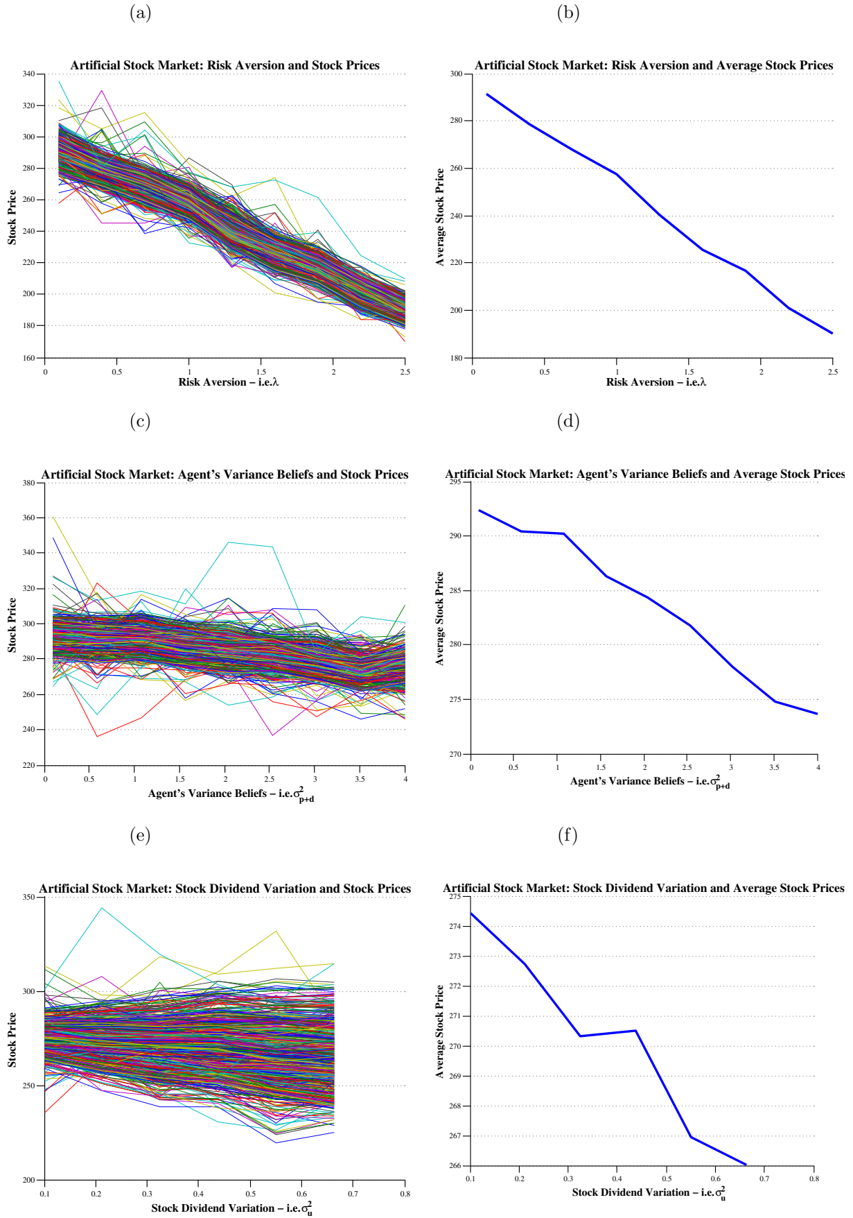
Figure 5: Single Stock Mixed Gaussian artificial stock market: Relationship Between Stock Prices and Underlying Variables - Panel A.
