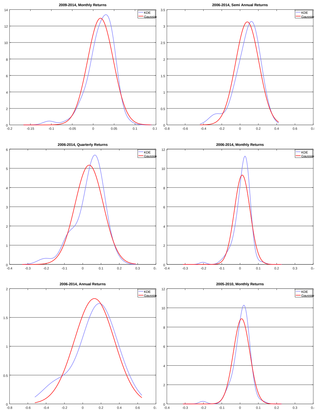
Figure 6: Kernel Density Estimates of S&P 500 Stock Market Returns (Multivariate Mixed Model) - Panel E
