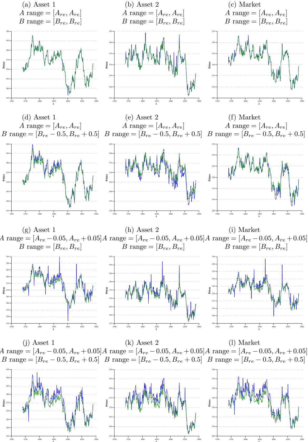
Figure 8: Agent-Based Model Stock Prices and Theoretical Stock Prices (Multivariate model).
