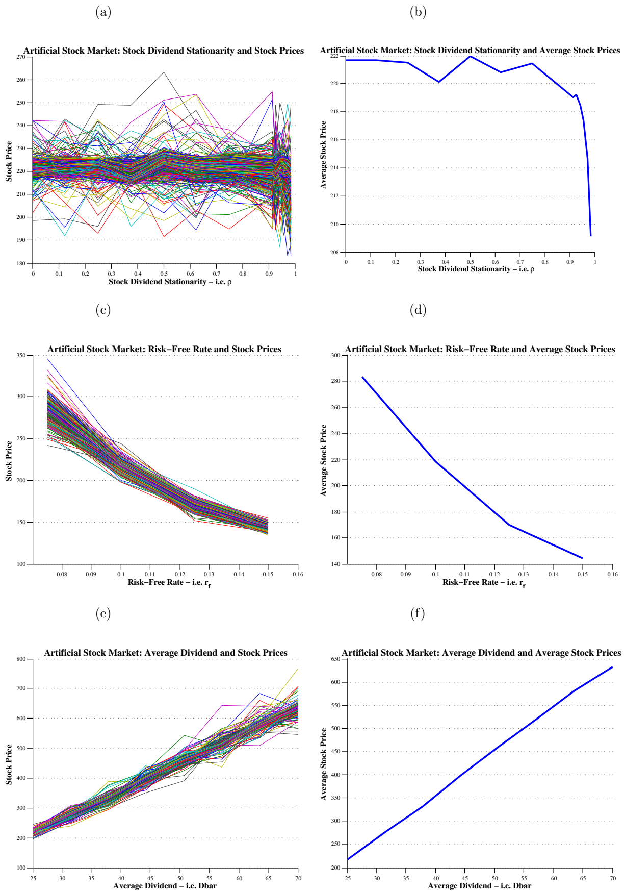
Figure 6: Multivariate Artificial Stock Market: Relationship Between Stock Prices and Underlying Variables (Stock Market) - Panel B.
