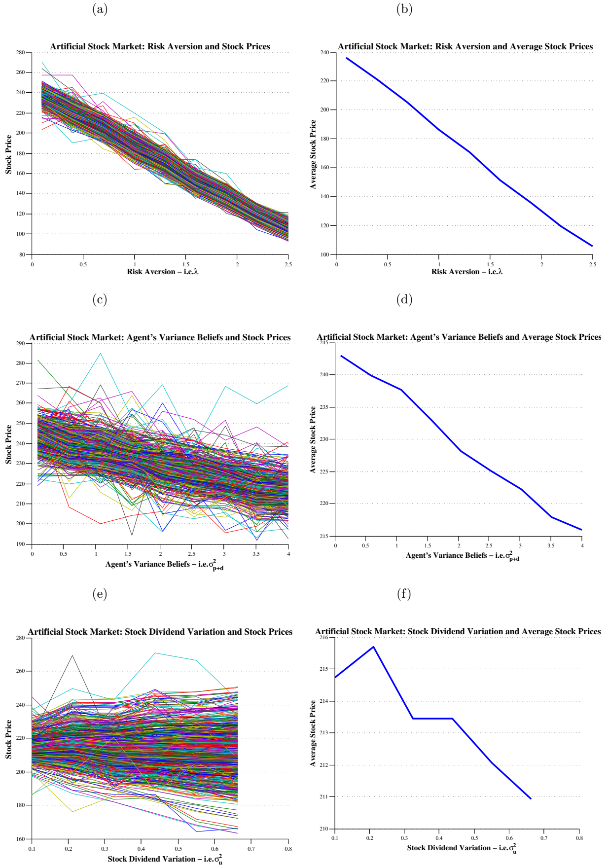
Figure 17: Multiple Stock Mixed Gaussian Artificial Stock Market: Relationship Between Stock Prices and Underlying Variables (Stock Market) - Panel A.
