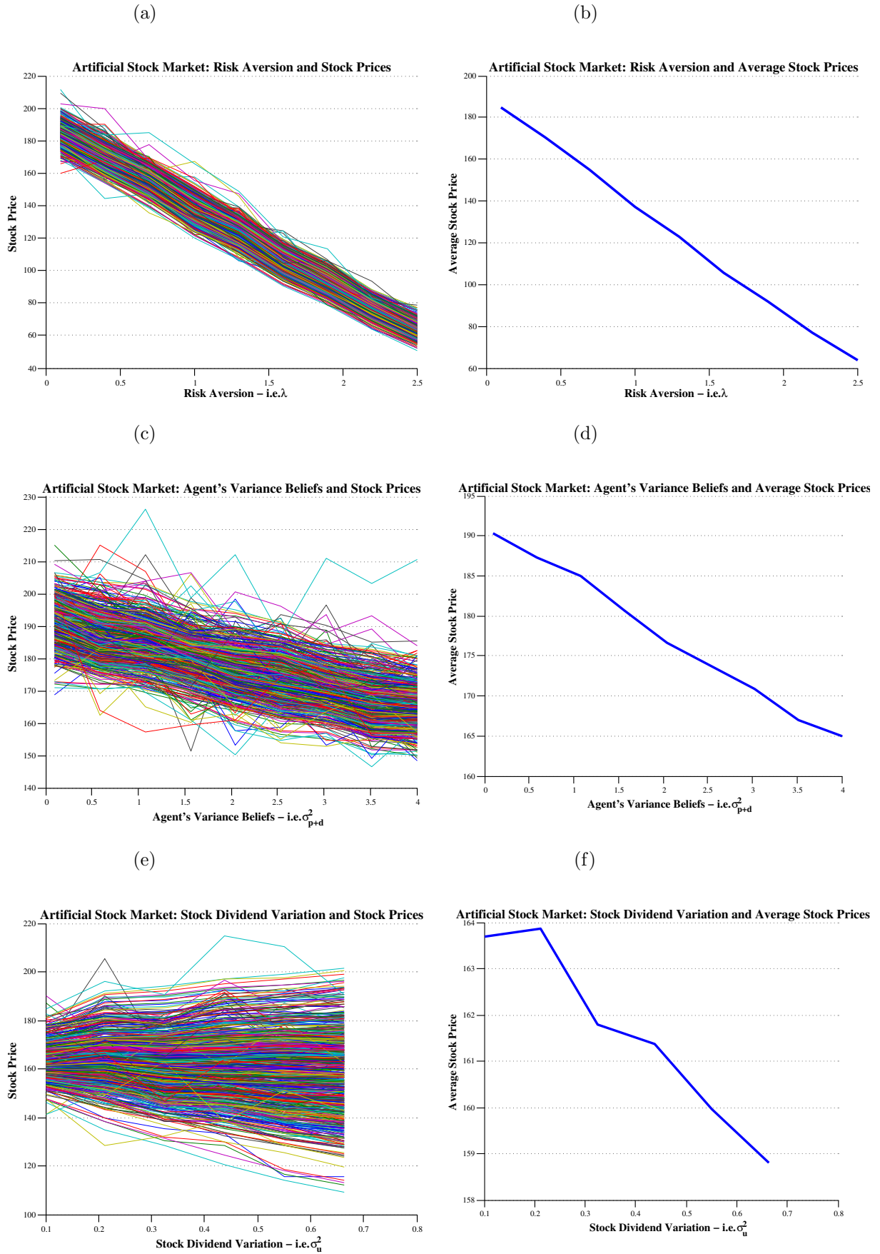
Figure 14: Multiple Stock Mixed Gaussian Artificial Stock Market: Relationship Between Stock Prices and Underlying Variables (Asset 2) - Panel A.
