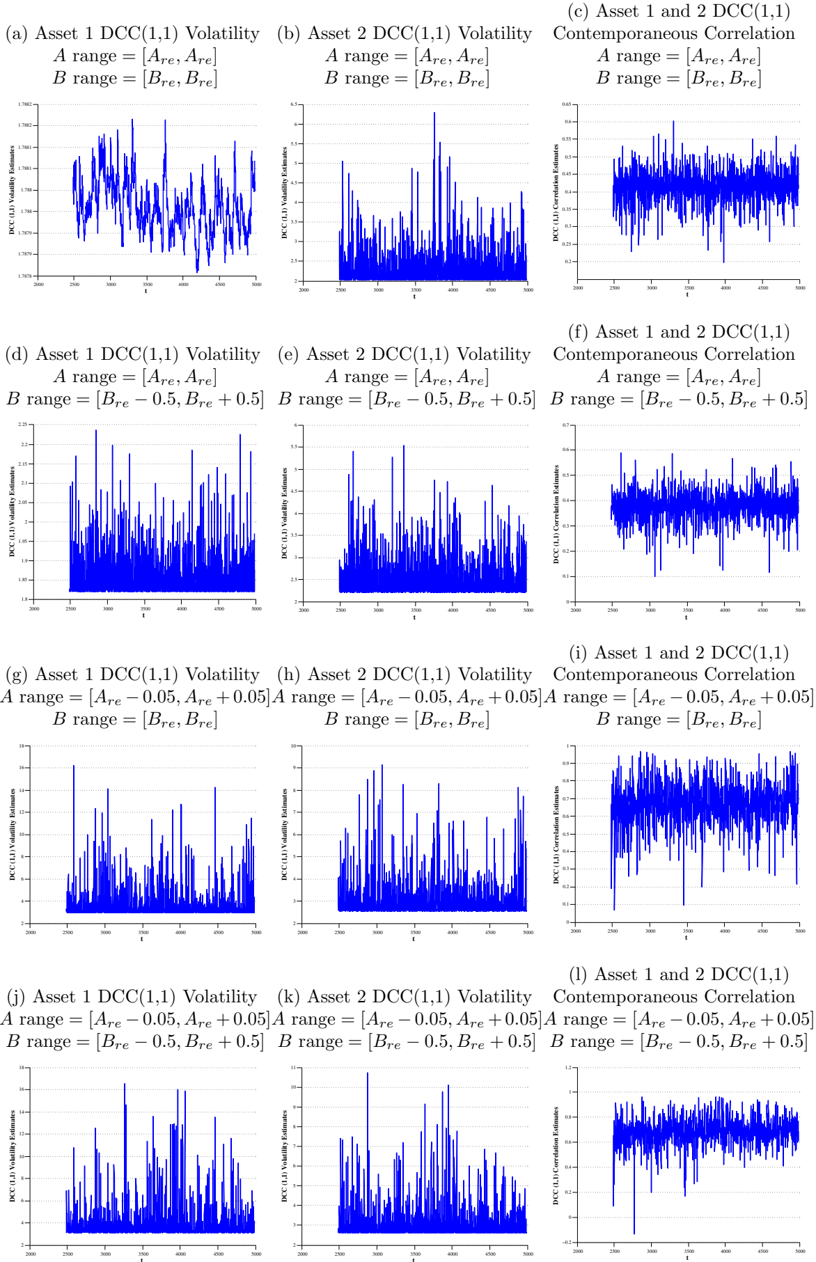
Figure 10: Multivariate Agent-Based Model Volatility and Covariation.
