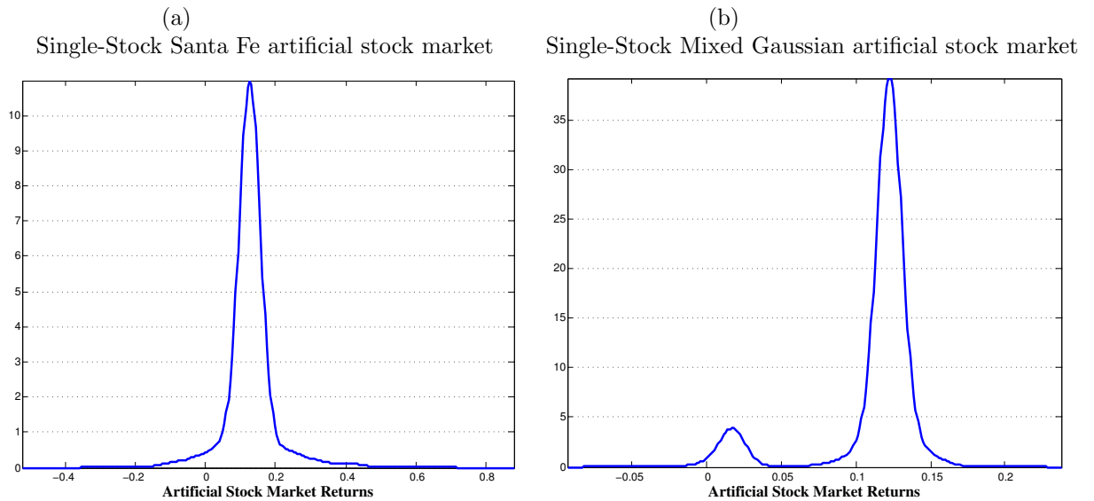
Figure 4: Density Estimate of Artificial Stock Market returns (Single-Stock Mixed Gaussian Artificial Stock Market)
