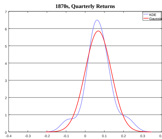
Figure 9: Kernel Density Estimates of S&P 500 Stock Market Returns (Multivariate Mixed Model) - Panel H
