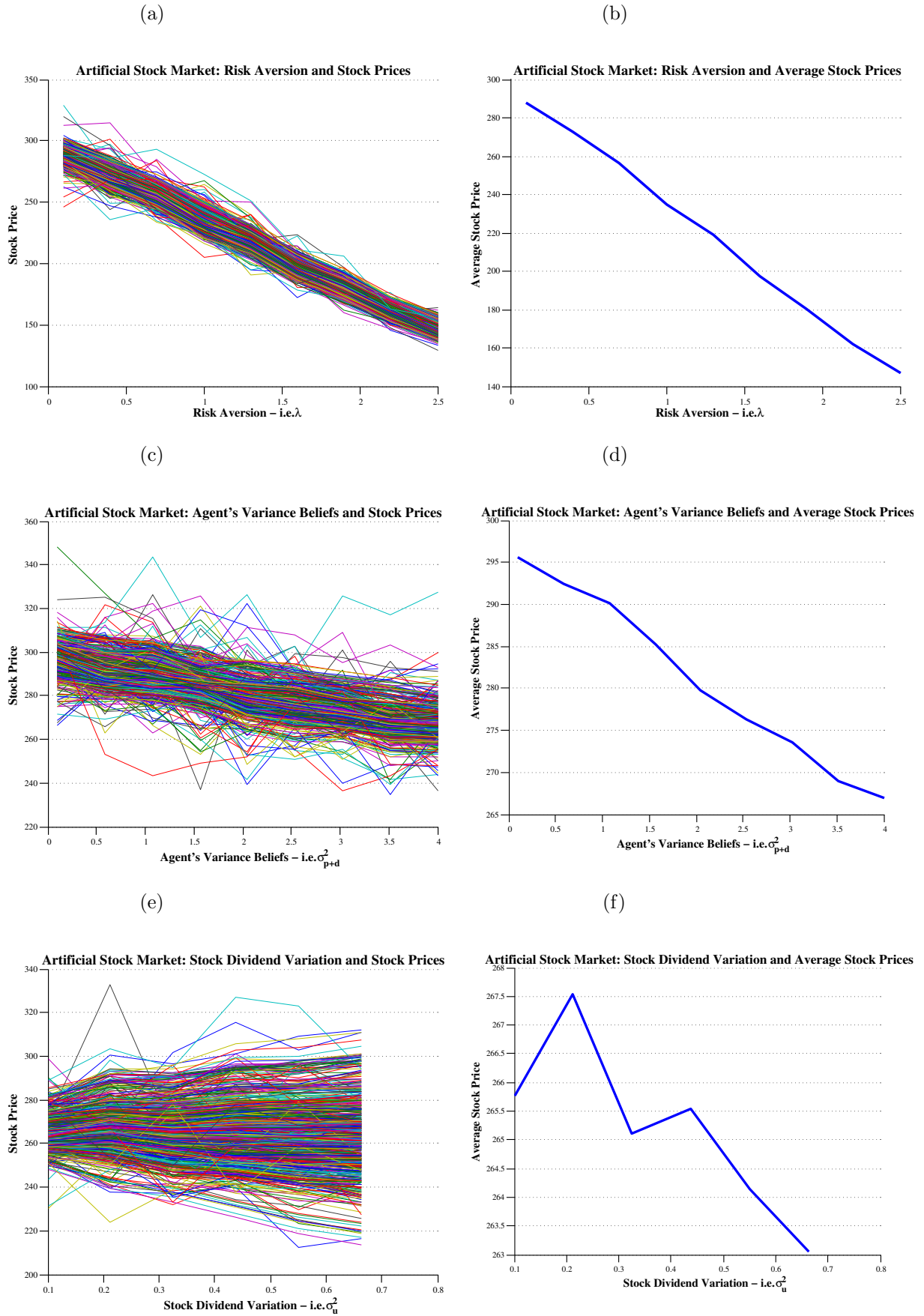
Figure 11: Multiple Stock Mixed Gaussian Artificial Stock Market: Relationship Between Stock Prices and Underlying Variables (Asset 1) - Panel A.
