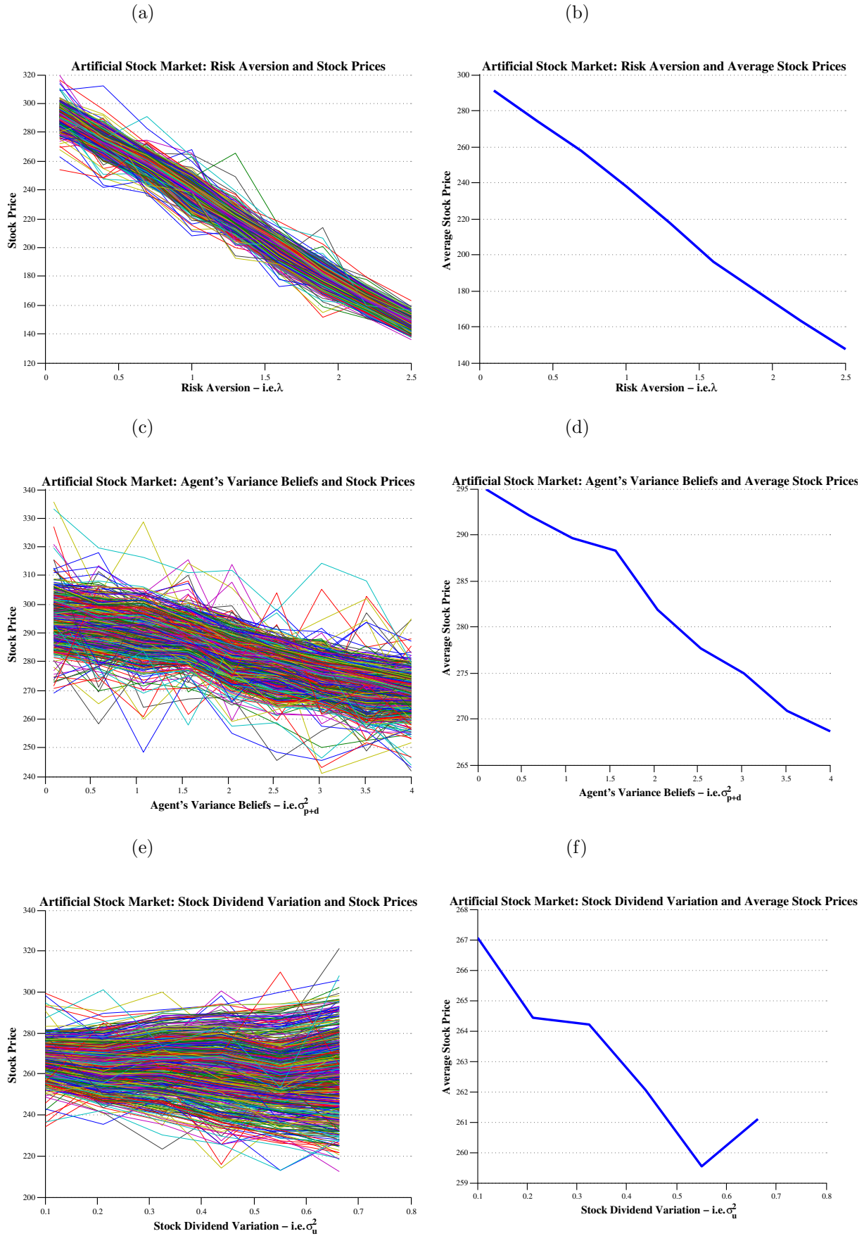
Figure 1: Multivariate Artificial Stock Market: Relationship Between Stock Prices and Underlying Variables (Asset 1) - Panel A.
