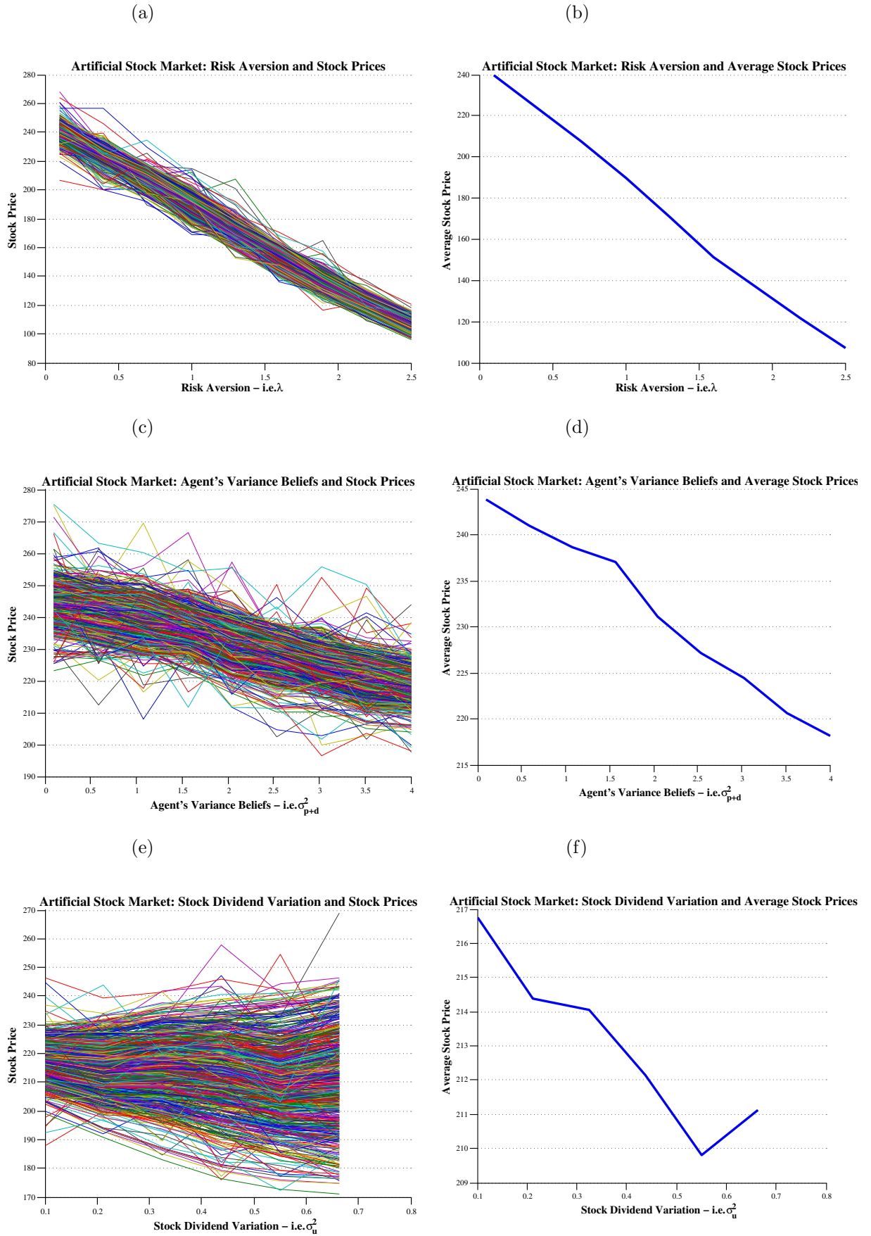
Figure 5: Multivariate Artificial Stock Market: Relationship Between Stock Prices and Underlying Variables (Stock Market) - Panel A.
