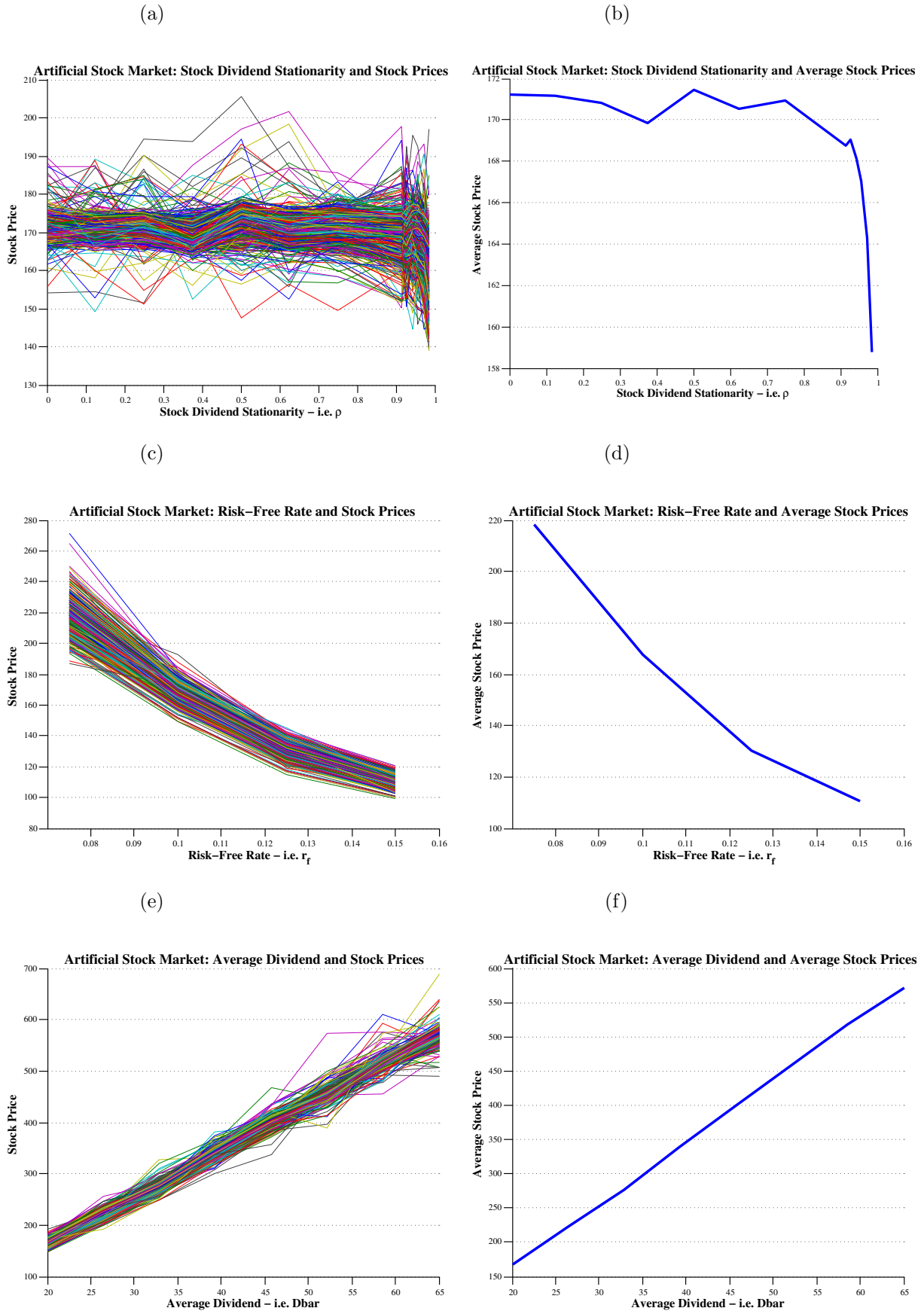
Figure 4: Multivariate Artificial Stock Market: Relationship Between Stock Prices and Underlying Variables (Asset 2) - Panel B.
