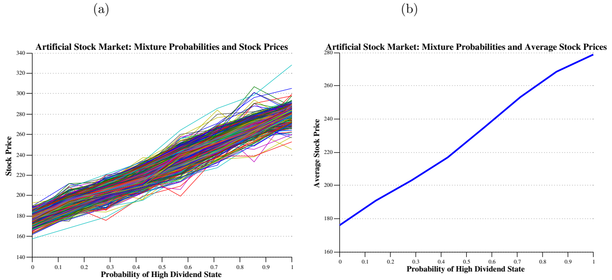
Figure 7: Single Stock Mixed Gaussian artificial stock market: Relationship Between Stock Prices and Underlying Variables - Panel C.
