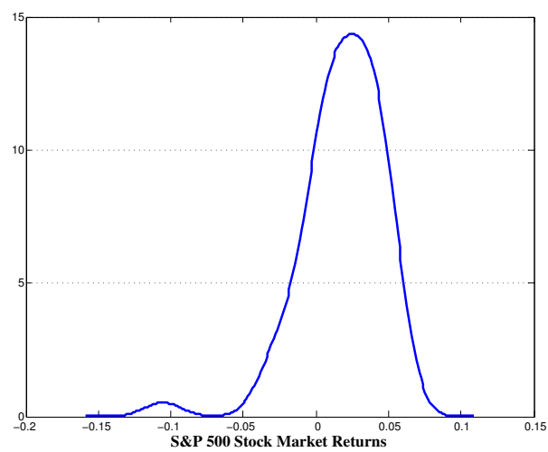
Figure 1: Density Estimate of S&P 500 Stock Market Returns (June 2010 - June 2015) - Single-Stock Santa Fe Artificial Stock Market
