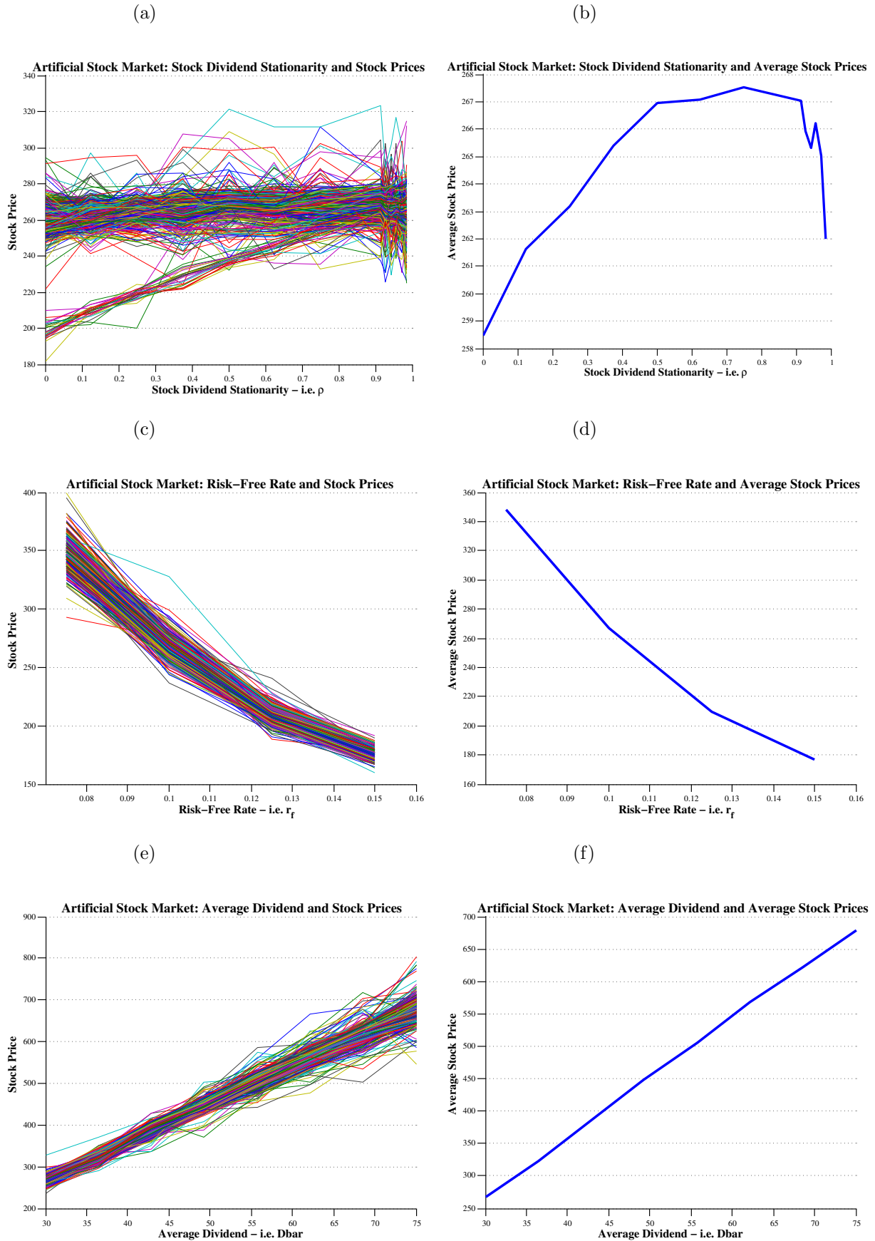
Figure 12: Multiple Stock Mixed Gaussian Artificial Stock Market: Relationship Between Stock Prices and Underlying Variables (Asset 1) - Panel B.
