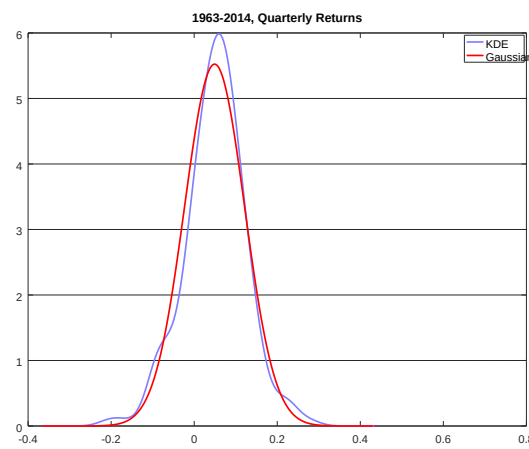
Figure 5: Kernel Density Estimates of S&P 500 Stock Market Returns (Multivariate Mixed Model) - Panel D
