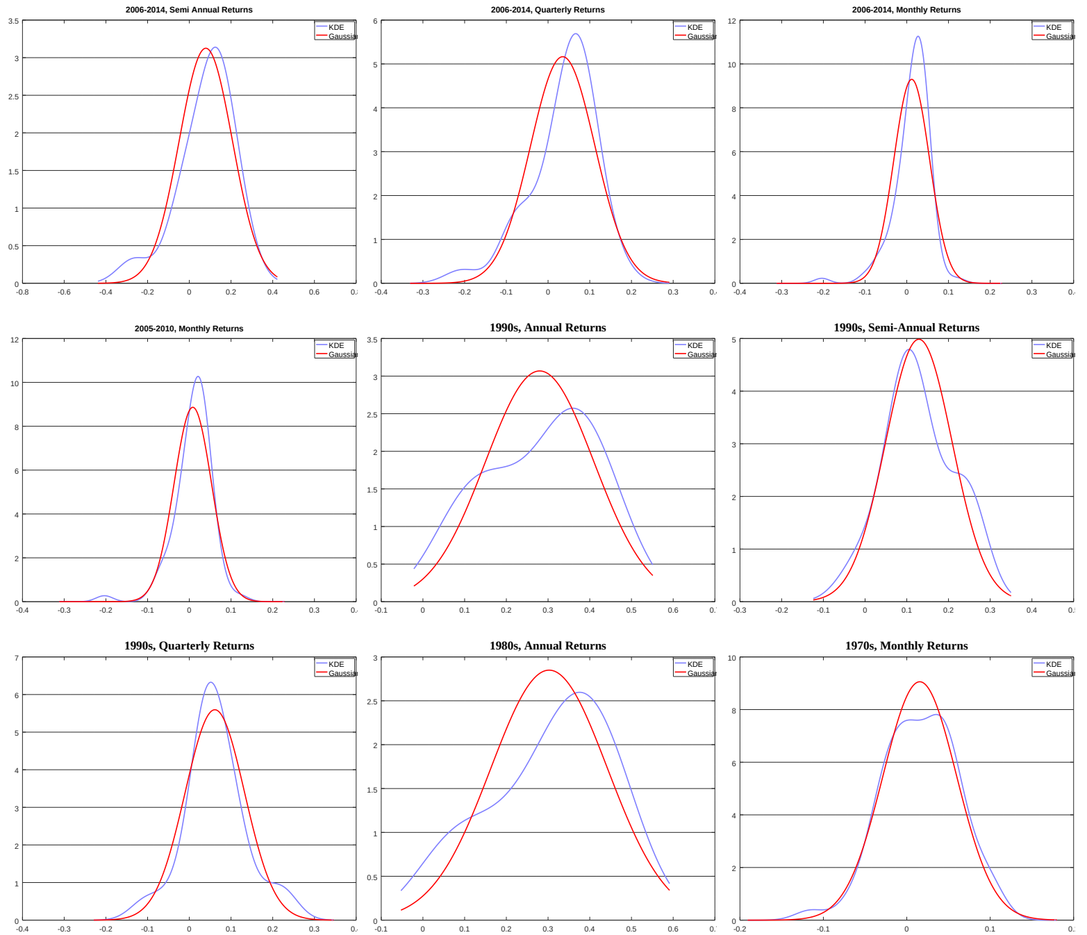
Figure 2: Kernel Density Estimates of S&P 500 Stock Market Returns (Single-Stock Santa Fe Artificial Stock Market) - Panel A.
