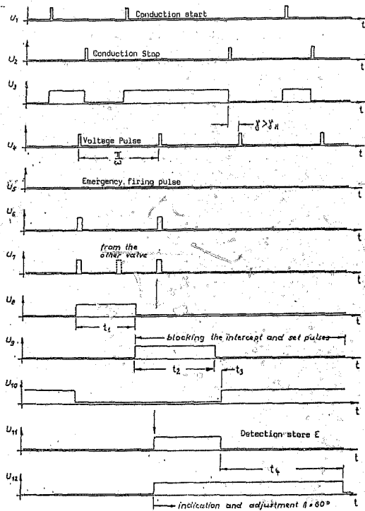
Fig. 5.1.7 Response by commutation failure (without negative valve voltage no emergency firing pulse)
