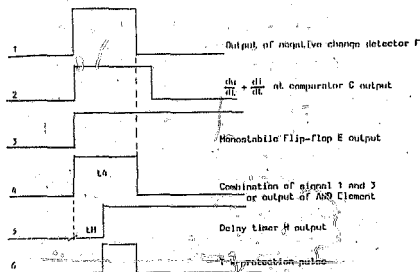
Fig. 5.2.2 When t_4 > t_H the protection pulse is generated.
