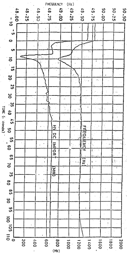
Fig. 5.5-2. AC frequency and input power at the inverter end.
