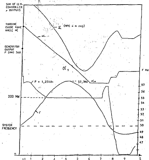
Fig. 5.5.1 Generating plant response for 50% load rejection.
