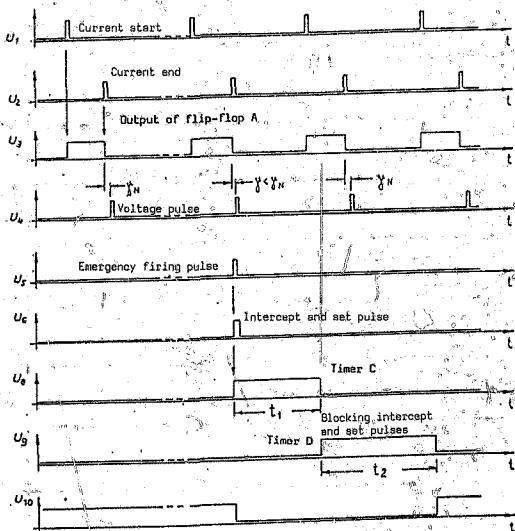
Fig. 9.1.6 Responses by a single dip below the rated extinction angle \gamma and forming an emergency firing pulse from the valve (Zemco TSE, 1979).
