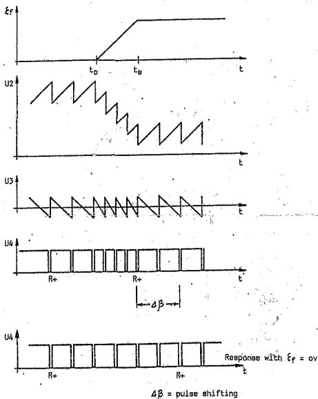
Fig. 4.13 Response of the pulse generator by input control voltage \xi_f = f(t) . (Zamco TSE, 1979).
