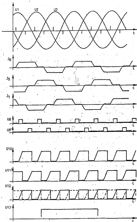
Fig. 4.16 Forming \gamma actual value by collecting the extinction angles
