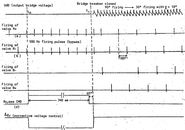
Fig. 4.21 Valve firing during bridge switch-on (SON).
