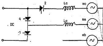
Fig. 5.1.4 DC and AC short-circuit due to bridge valve commutation.
