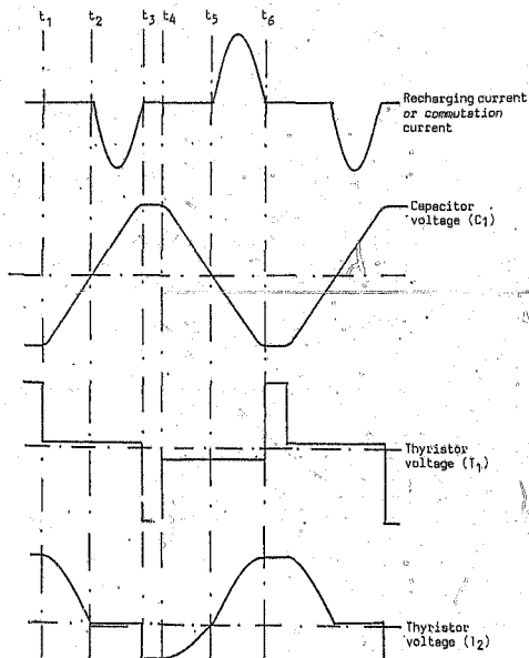
Fig. 4.24 Voltage and current diagrams on the parallel-resonant circuit inverter of the gate pulse amplifier.
