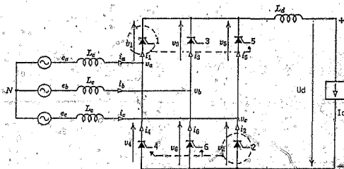
Fig. 5.1.8 Valve 1 and 2 in the conducting condition.
