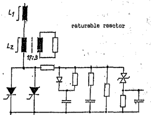
Fig. 5.1.3 Voltage grading network of Apollo valves.
