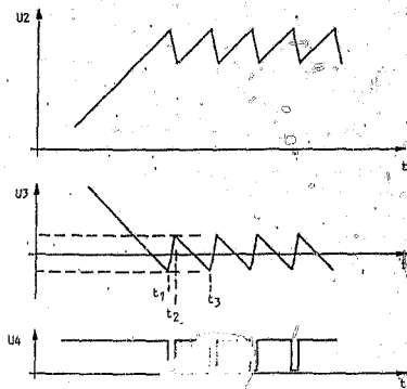
Fig. 4.11 Time diagram of the pulse generator with \xi f = 0 (Zemco TSE, 1979).
