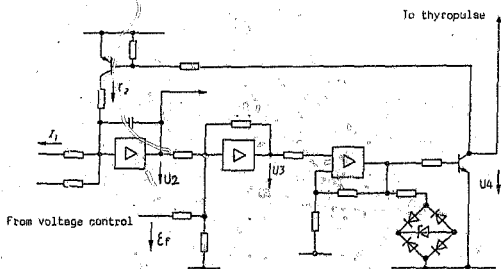
Fig. 4.10 Basic circuit diagram of the pulse generator.
