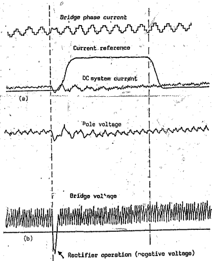
Fig. 5.1.10 False commutation failure due to a spurious emergency firing pulse. (Recorded at Appilo station).
