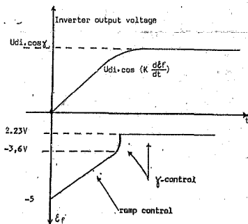
Fig. 4.20 Voltage control and inverter output voltage during transient (bridge switching on).
