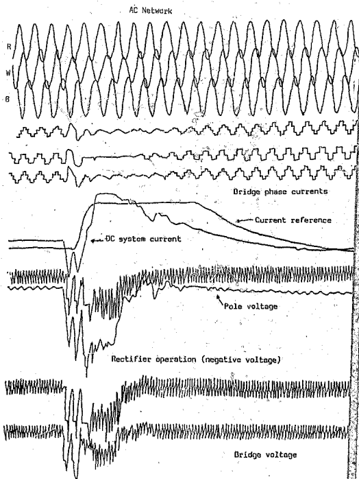
Fig. 5.1.13 AC system fault: all pole bridges are affected by commutation failure (recorded at Apollo station).
