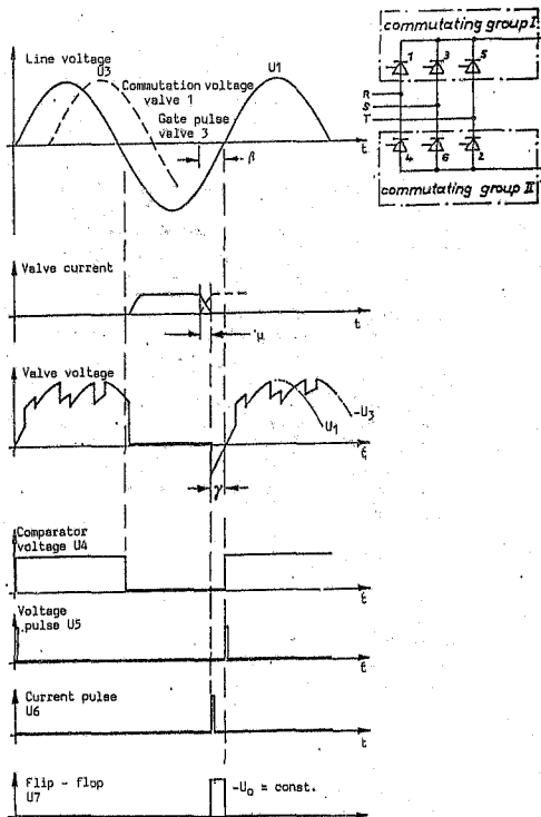
Fig. 4.17 Forming \gamma actual value for one valve.
