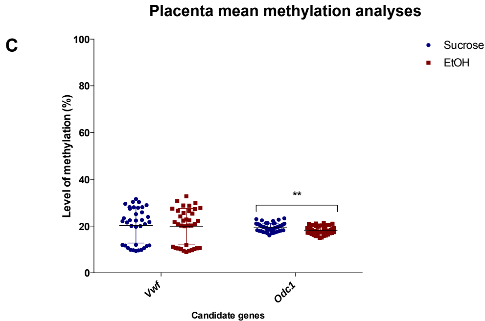
Figure 3.11: Column scatter plots of mean methylation levels of the candidates gene in different embryonic tissues. Embryos were sired by male mice exposed to EtOH or sucrose for ten weeks. Statistically significant ** ( P \leq 0.01 ) * ( 0.01 < P \leq 0.05 ) Trending significance ^ ( 0.05 \leq P < 0.1 ) Error bars indicate the standard deviation.
