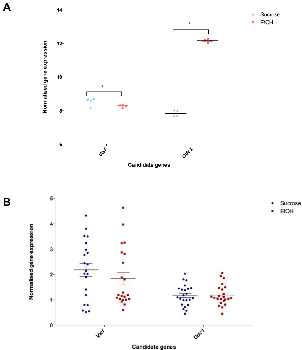
Figure 3.9: Real-time PCR validation of placental microarray results. A Microarray analysis of the effects of preconception paternal alcohol or sucrose exposure on gene expression in the embryonic placenta. B Real-time analysis of the effects of preconception paternal alcohol or sucrose exposure on candidate gene expression in the embryonic brain. SYBR green quantitative PCR was used to analyse the gene expression levels relative to the housekeeping gene Actb . Statistically significant ** ( P \leq 0.01 ) * ( 0.01 < P \leq 0.05 ) Trending significance ^ ( 0.05 \leq P < 0.1 ) Error bars indicate the standard deviation.
