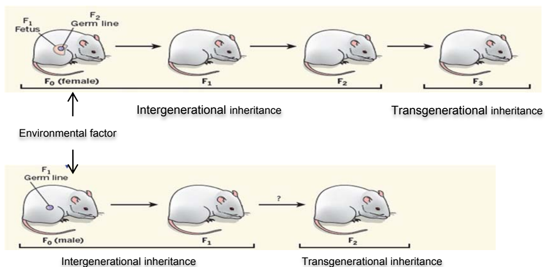
Figure 1.4: Intergenerational and transgenerational epigenetic inheritance. Epigenetic changes in mammals can arise sporadically or can be induced by the environment (toxins, nutrition, and stress). In the case of an exposed female mouse, if she is pregnant, the foetus can be affected in utero (F1), as can the germline of the foetus (the future F2). These are considered to be parental effects, leading to intergenerational epigenetic inheritance. Only F3 individuals can be considered as true transgenerational inheritance in the absence of exposure. In the case of males in which an epigenetic change is induced, the individual (F0) and his germline (future F1) are exposed; the F1 is thus considered as intergenerational. Only F2 and subsequent generations can be considered for evidence of transgenerational inheritance (Skinner, 2010).
