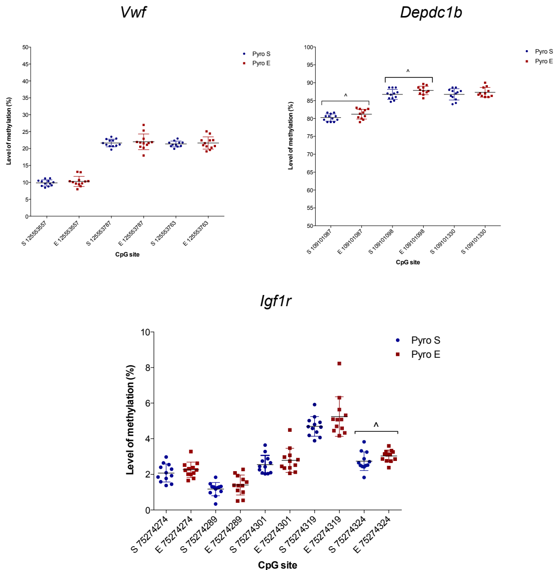
Figure 3.13: Column scatter plots of DNA methylation at individual CpG sites of the embryonic liver. Embryos were sired by male mice exposed to EtOH or sucrose for ten weeks. Statistically significant ** ( P \leq 0.01 ) * ( 0.01 < P \leq 0.05 ) Trending significance ^ ( 0.05 \leq P < 0.1 ) Error bars indicate the standard deviation.
