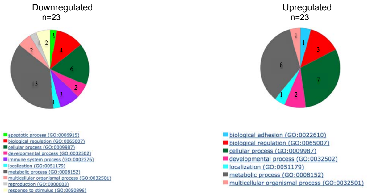
Figure 3.17: Pie charts of the biological processes of genes significantly ( p < 0.001 & FC > 1.2 ) downregulated and upregulated in the brain and liver of embryos sired by males treated with EtOH. The genes were grouped into these categories by the PANTHER classification system. n indicates the number of genes that were either up or downregulated. The number in each portion of the pie chart indicates the number of candidate genes dysregulated per biological process.
