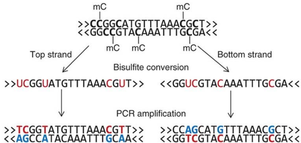
Figure 2.3: Schematic of the bisulphite conversion for the analysis of DNA methylation. Methylated cytosines (mC) remain as Cs, while unmethylated Cs are converted to uracil (U) and subsequently to thymine (T) during the PCR amplification reaction (Krueger et al., 2012).
