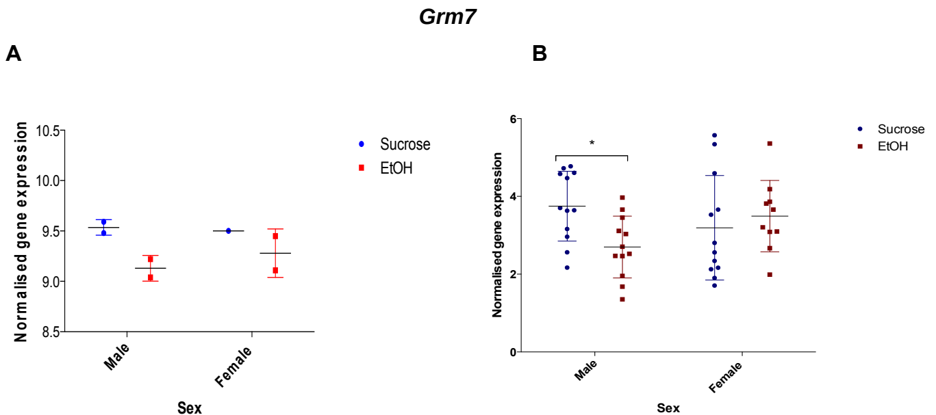
Figure 3.10: Differential Grm7 expression in male and female embryos sired by male mice exposed to EtOH or sucrose. A. Microarray expression results. B Expression analysed by quantitative real-time PCR. Statistically significant * ( P \leq 0.05 ). Error bars indicate the standard deviation.
