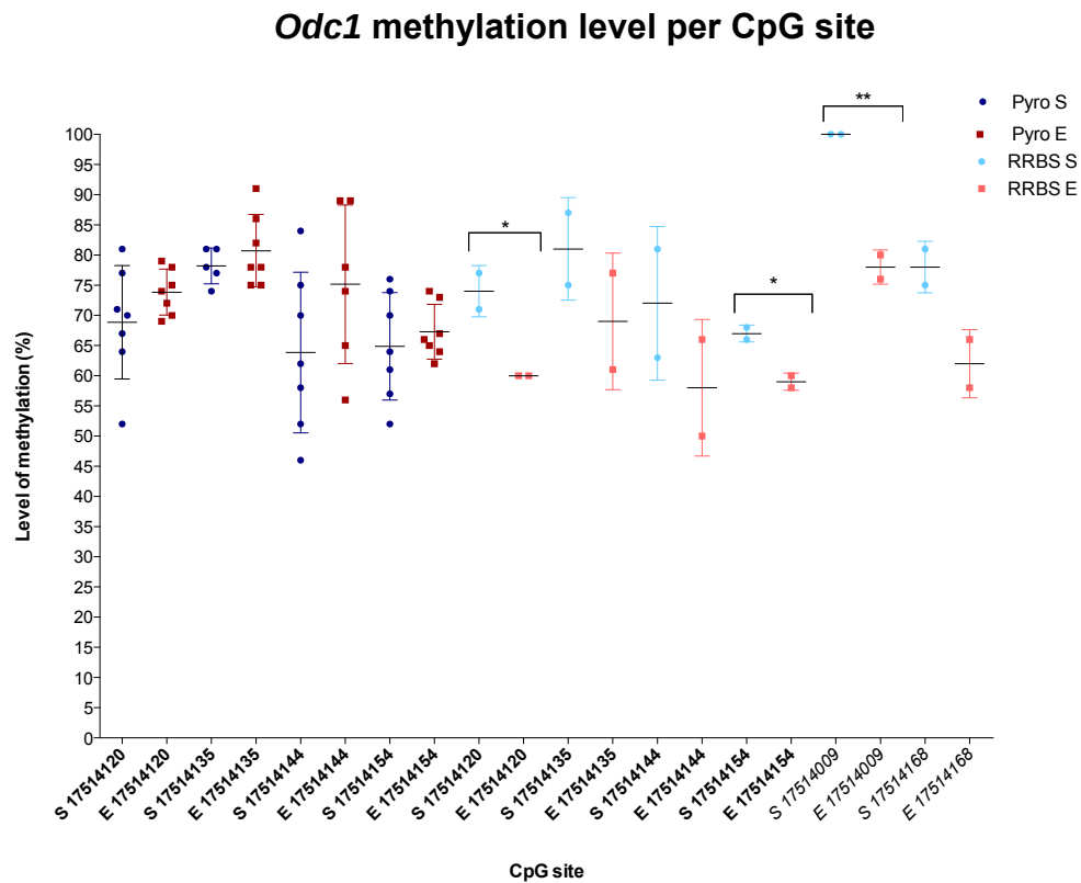
Figure 3.5: Validation of Odc1 RRBS CpG site-specific sperm DNA methylation data of male mice exposed to EtOH or sucrose using pyrosequencing. CpG sites 17514120, 17514135, 17514144 and 17514154 were analysed for validation. Statistically significant ** ( P \leq 0.01 ) * ( 0.01 < P \leq 0.05 ) Trending significance ^ ( 0.05 \leq P < 0.1 ) Error bars indicate the standard deviation.
