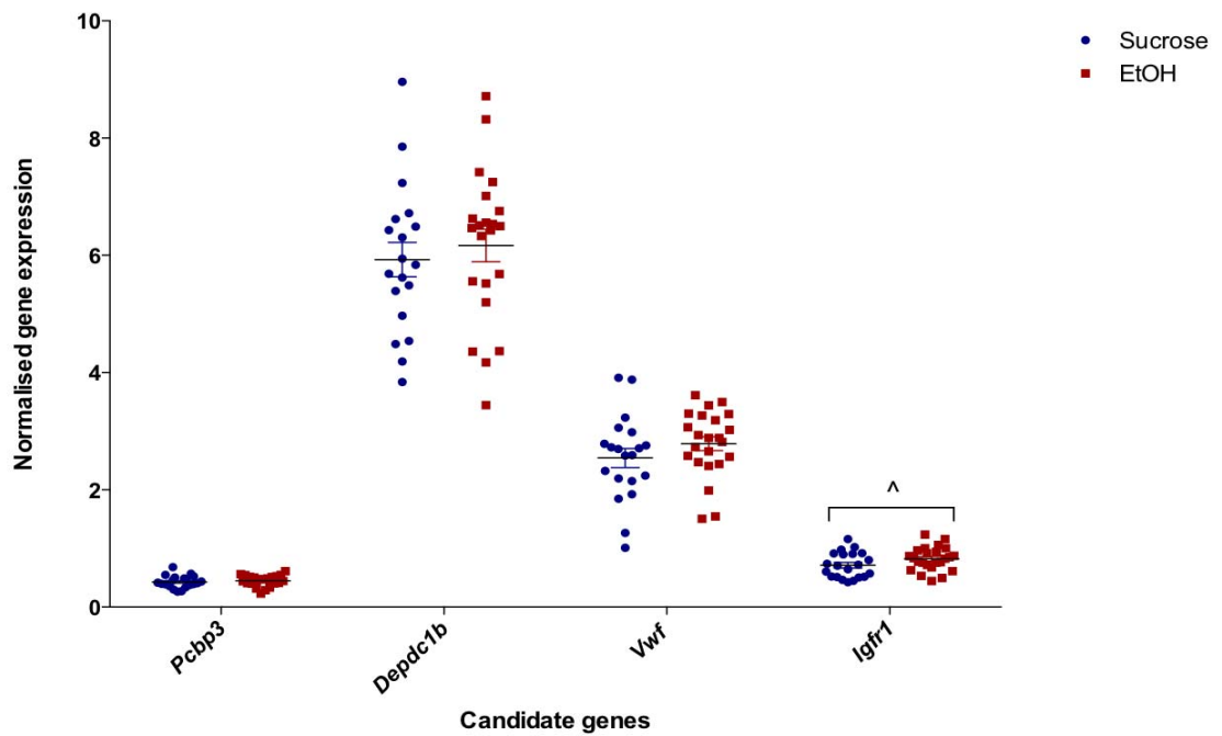
Figure 3.8: Real-time PCR validation of embryonic liver microarray results. A Microarray analysis of the effects of preconception paternal alcohol or sucrose exposure on gene expression in the embryonic liver. B Real-time analysis of the effects of preconception paternal alcohol or sucrose exposure on candidate gene expression in the embryonic brain. SYBR green quantitative PCR was used to analyse the gene expression levels relative to the housekeeping gene Actb . Statistically significant ** ( P \leq 0.01 ) * ( 0.01 < P \leq 0.05 ) Trending significance ^ ( 0.05 \leq P < 0.1 ) Error bars indicate the standard deviation.
