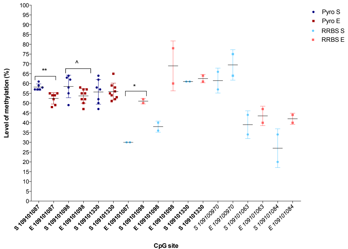
Figure 3.6: Validation of Depdc1b RRBS CpG site-specific sperm DNA methylation data of male mice exposed to EtOH or sucrose using pyrosequencing. CpG sites 109101087, 109101098, 109101330 were analysed for validation. Statistically significant ** ( P \leq 0.01 ) * ( 0.01 < P \leq 0.05 ) Trending significance ^ ( 0.05 \leq P < 0.1 ) Error bars indicate the standard deviation.
