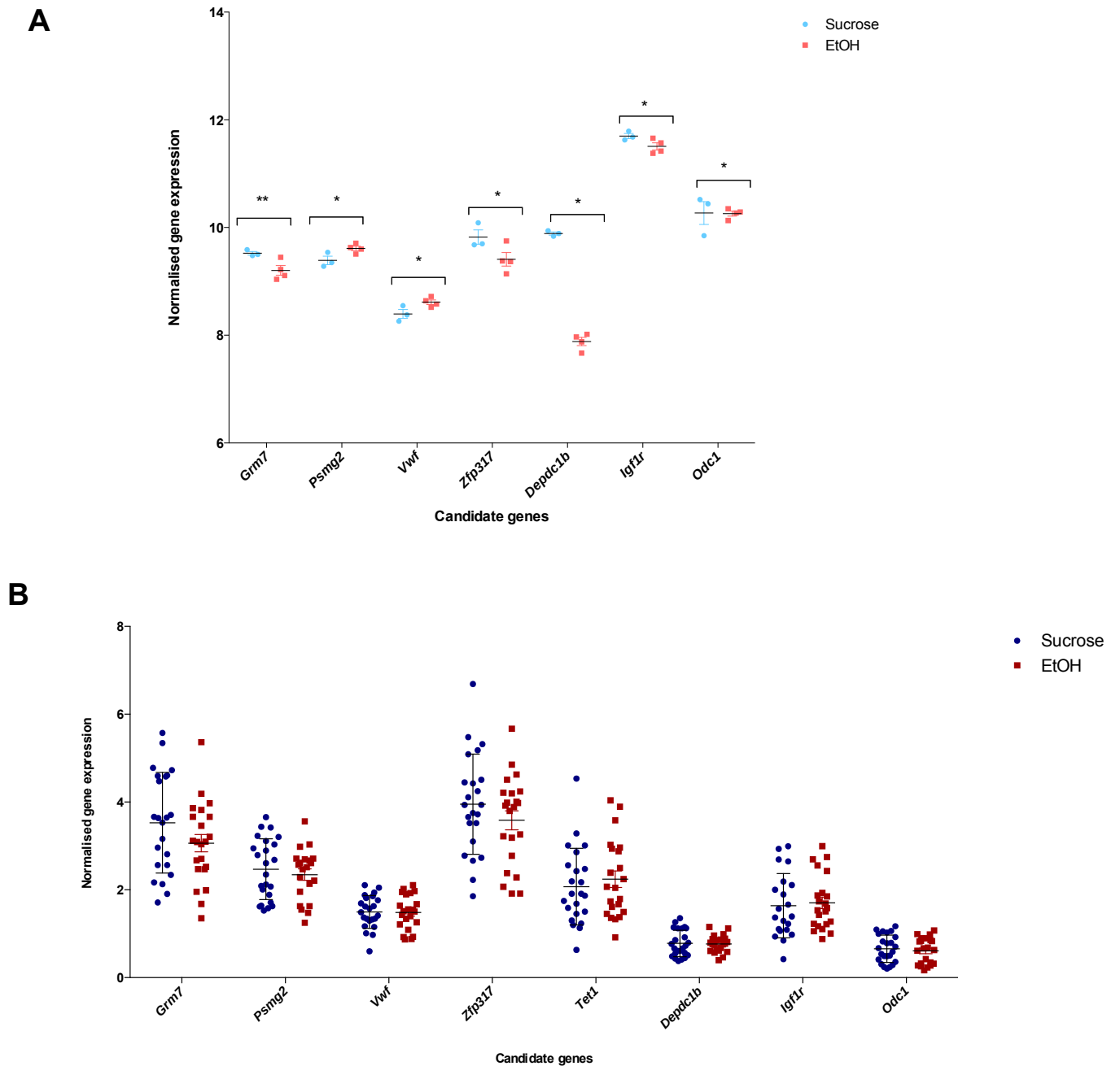
Figure 3.7: Real-time PCR validation of embryonic brain microarray results. A Microarray analysis of the effects of preconception paternal alcohol or sucrose exposure on gene expression in the embryonic brain. B Real-time analysis of the effects of preconception paternal alcohol or sucrose exposure on candidate gene expression in the embryonic brain. SYBR green quantitative PCR was used to analyse the gene expression levels relative to the housekeeping gene Actb . Statistically significant ** ( P \leq 0.01 ) * ( 0.01 < P \leq 0.05 ) Trending significance ^ ( 0.05 \leq P < 0.1 ) Error bars indicate the standard deviation.
