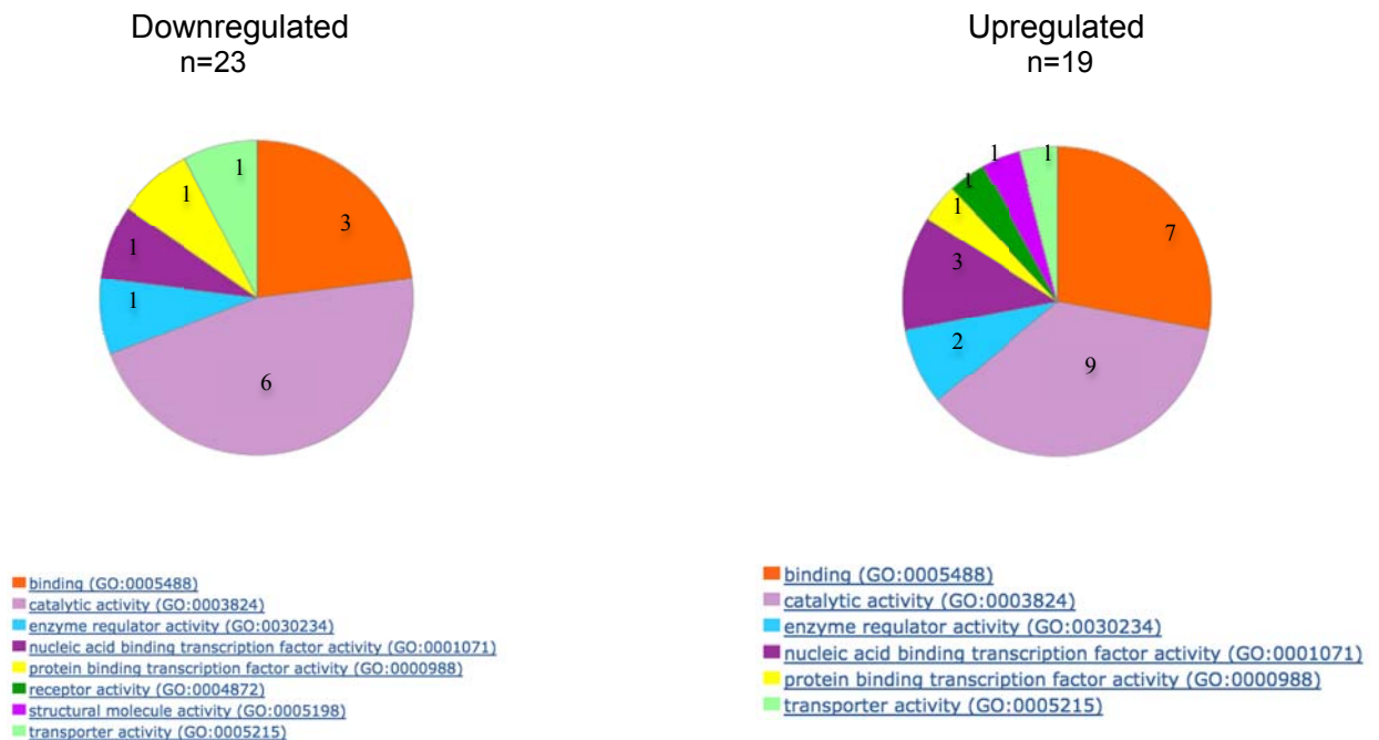
Figure 3.16: Pie charts of the molecular function of genes significantly ( p < 0.001 & FC > 1.2 ) downregulated and upregulated in the brain and liver of embryos sired by males treated with EtOH. The genes were grouped into these categories by the PANTHER classification system. n indicates the number of genes that were either up or downregulated. The number in each portion of the pie chart indicates the number of candidate genes dysregulated per molecular function.
