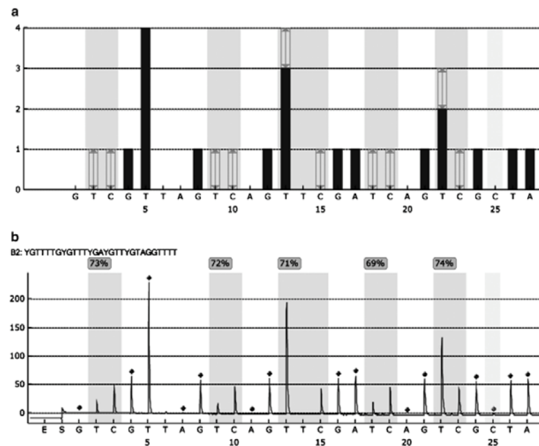
Figure 2.7: Results of a bisulphite pyrosequencing assay to determine the DNA methylation status within a region of interest. (a) The theoretical histogram based on the nucleotide input sequence showing the expected peak pattern for the region of interest. (b) The pyrogram obtained for the bisulphite sequencing describing the methylation levels at the CpG sites within the region (Tollefsbol, 2011).
