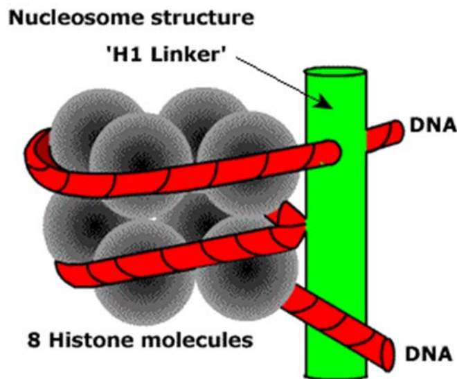
Figure 1.1: Nucleosome structure. Chromatin is comprised of histones and DNA: a 147bp chain of DNA wrapped around 8 core histone proteins forms the basic chromatic unit, the nucleosome (Sarkar, 2012).
