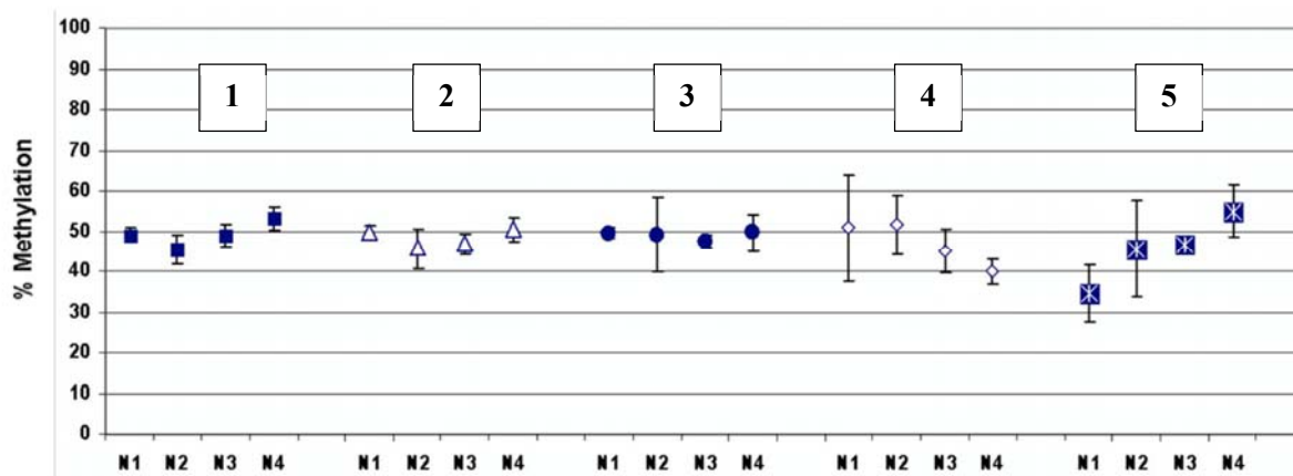
Figure 4.1: The effect of bisulfite treatment and DNA concentration on the quantification of DNA methylation, as determined by pyrosequencing. Analysis of four control samples (N1 to N4) in which 50ng [1], 20ng [2], 10ng [3], 5ng [4], and 2.5ng [5] of template DNA was added to the PCR reaction. The values for percentage of methylation were corrected for methylation bias. The error bars indicate the standard deviations for triplicate analyses (White, 2006).
