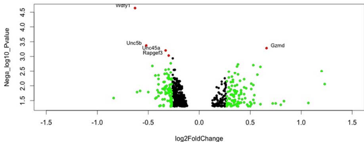
Figure 3.15: Volcano plots of significance against fold change of embryonic brain (A), liver (B) and placental (C) gene expression. Each dot represents a single gene. Highly significant values are toward the top and small expression changes are near the centre. Genes with decreased expression levels will lie on the negative x-axis, while genes that display an increase in expression are located on the positive side. The red dots represent the genes that are highly significant ( p < 0.001 ) and have a high FC > 1.2 , the green dots represent genes that have a significance of p < 0.05 and a FC > 1.2 and the black dots represent genes that have a significance of p < 0.05 and a FC < 1.2 . The log fold change is plotted on the x-axis and the negative log10 p-value is plotted on the y-axis.
