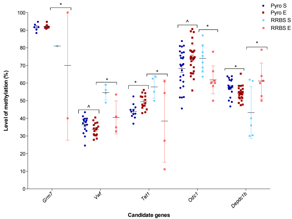
Figure 3.1: Validation of RRBS mean methylation data for five candidate genes using pyrosequencing. Comparison of the mean methylation levels and the techniques used to detect the methylation changes between sires exposed to EtOH or sucrose for ten weeks. Statistically significant ** ( p \leq 0.01 ) * ( 0.01 < P \leq 0.05 ) Trending significance ^ ( 0.05 \leq P < 0.1 ) Error bars indicate the standard deviation.
