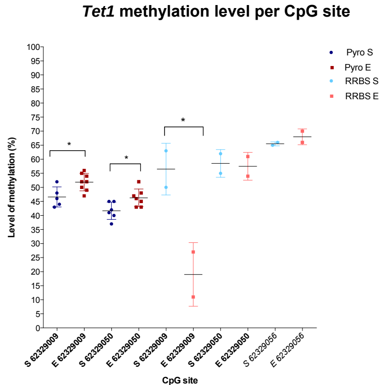
Figure 3.3: Validation of Tet1 RRBS CpG site-specific sperm DNA methylation data of male mice exposed to EtOH or sucrose using pyrosequencing. CpG site 62329009 and 62329050 were analysed for validation. Statistically significant ** ( P \leq 0.01 ) * ( 0.01 < P \leq 0.05 ) Trending significance ^ ( 0.05 \leq P < 0.1 ) Error bars indicate the standard deviation
