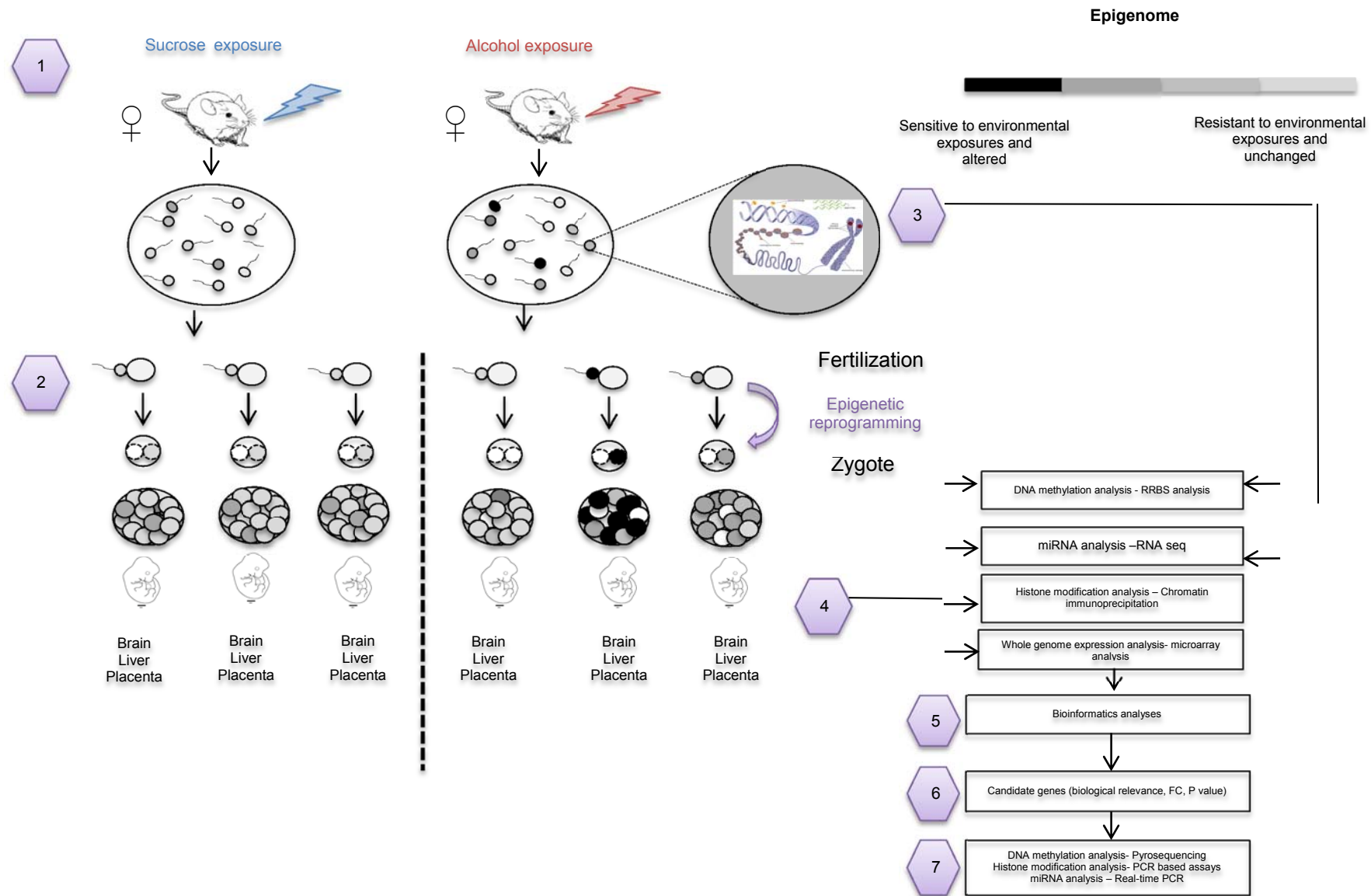
Figure 4.2: A simplistic future model to investigate the effect of preconception paternal alcohol exposure on epigenetic mechanisms in mouse offspring. (1) Expose C57BL/6 male mice to alcohol (3g/kg) (test) by gavage for ten weeks and to sucrose (control). (2) Mate male mice with unexposed
