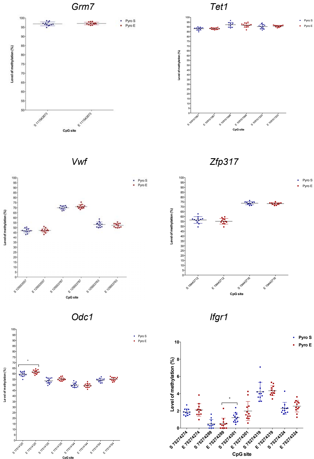
Figure 3.12: Column scatter plots of DNA methylation at individual CpG sites of the embryonic brain. Embryos were sired by male mice exposed to EtOH or sucrose for ten weeks. Statistically significant ** ( P \leq 0.01 ) * ( 0.01 < P \leq 0.05 ) Trending significance ^ ( 0.05 \leq P < 0.1 ) Error bars indicate the standard deviation.
