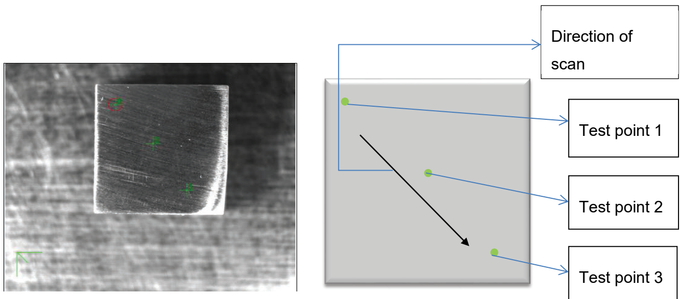
Figure 3-28: An illustration of how the tester measured the hardness of the sample.
