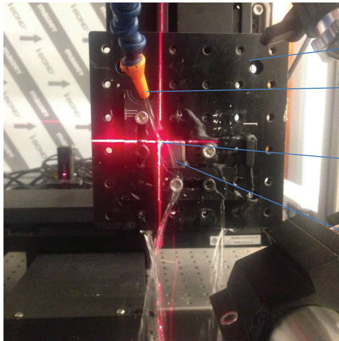
Figure 3-17: A turbine sample being treated with LSPwC
