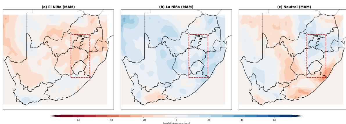
Figure 5.11: Rainfall anomaly maps (mm) for MAM, associated with the ENSO cycle based on ENSO events between 1981 and 2023, for (a) El Niño, (b) La Niña and (c) Neural phases. Anomalies are calculated from the 1981-2023 average.
