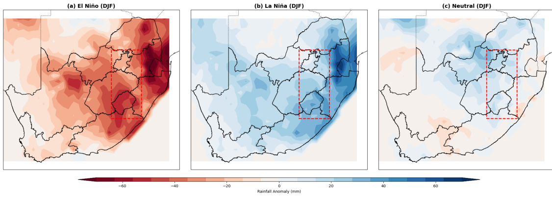
Figure 4.6: Rainfall anomaly maps (mm) for DJF, associated with the ENSO cycle based on ENSO events between 1981 and 2023, for (a) El Niño, (b) La Niña and (c) Neural phases. Anomalies are calculated from the 1981-2023 average.
