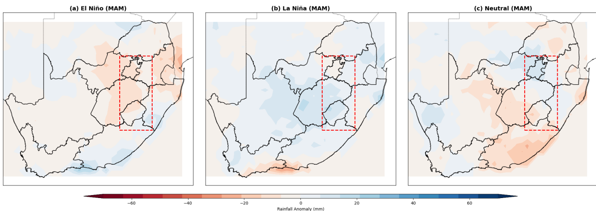
Figure 4.7: Rainfall anomaly maps (mm) for MAM, associated with the ENSO cycle based on ENSO events between 1981 and 2023, for (a) El Niño, (b) La Niña and (c) Neural phases. Anomalies are calculated from the 1981-2023 average.
