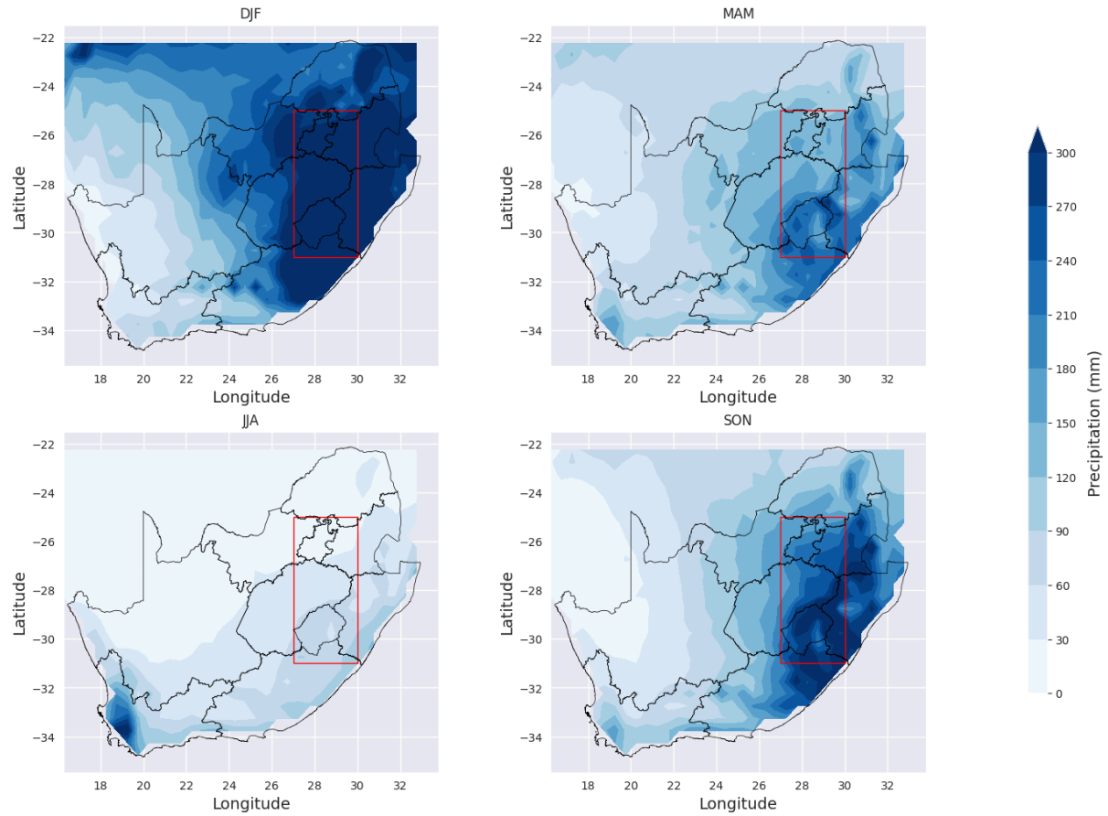
Figure 5.2: Mean seasonal ERA5 rainfall totals (mm) across South Africa for 1981-2023, with the rectangular (red) box highlighting the study site.
