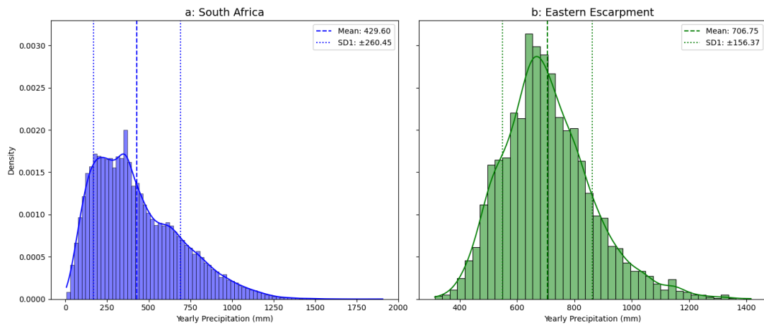
Figure 4.3: Mean annual rainfall distribution across (a) South Africa and (b) the eastern escarpment study site for CRU, with mean (thicker dotted line) and standard deviations (thinner dotted lines).
