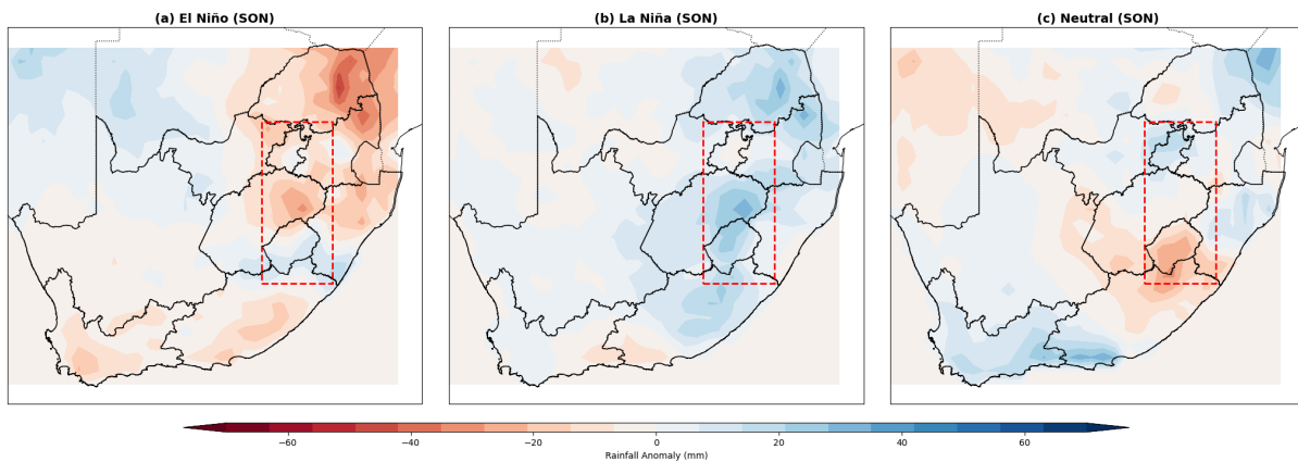
Figure 5.13: Rainfall anomaly maps (mm) for SON, associated with the ENSO cycle based on ENSO events between 1981 and 2023, for (a) El Niño, (b) La Niña and (c) Neutral phases. Anomalies are calculated from the 1981-2023 average.
