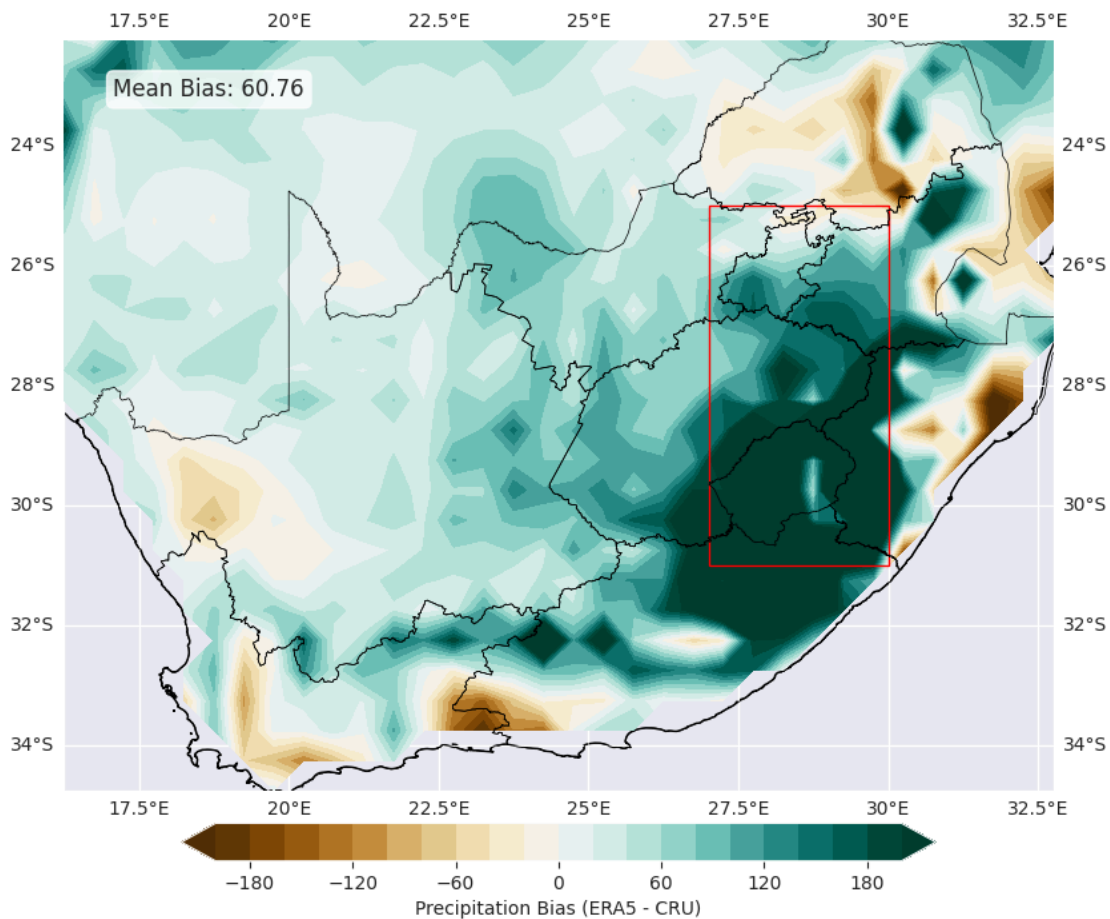
Figure 5.6: Mean annual rainfall bias (mm) in the ERA5 data relative to CRU.
