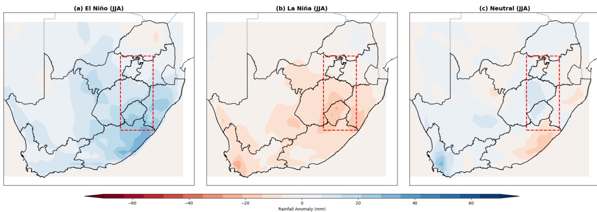
Figure 5.12: Rainfall anomaly maps (mm) for JJA, associated with the ENSO cycle based on ENSO events between 1981 and 2023, for (a) El Niño, (b) La Niña and (c) Neutral phases. Anomalies are calculated from the 1981-2023 average.
