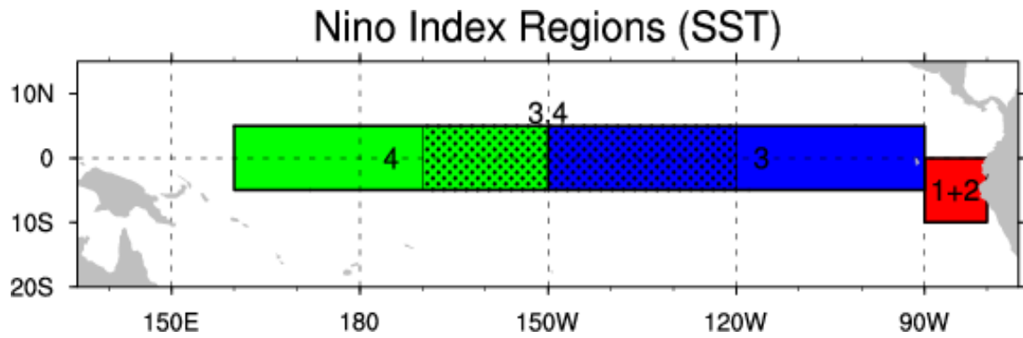
Figure 3.2: A map of the regions used for various Niño indices (UCAR, 2024).
