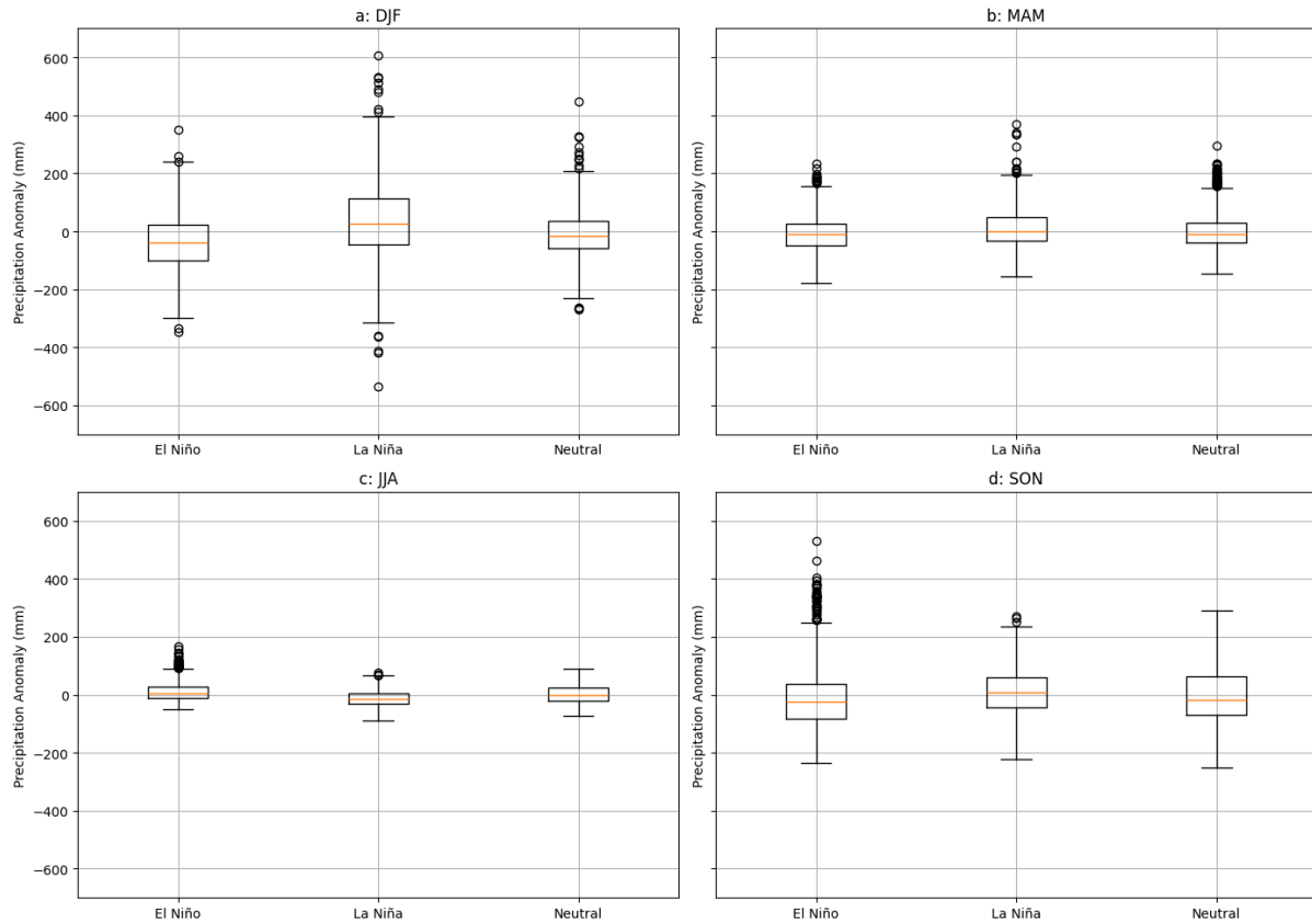
Figure 5.9: Spread in the seasonal rainfall anomalies according to specific ENSO phases, across the eastern escarpment study site, for (a) DJF, (b) MAM, (c) JJA and (d) SON. Boxplots show the 25 th , 50 th and 75 th percentiles; whiskers extend to the most extreme values within 1.5 \times \text{IQR} from the lower and upper quartiles; circles represent outliers beyond this range.
