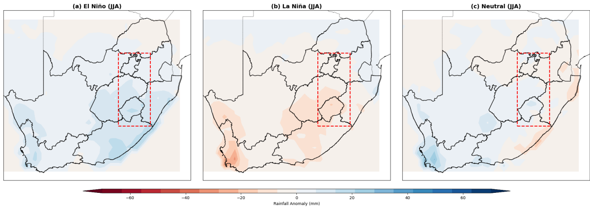
Figure 4.8: Rainfall anomaly maps (mm) for JJA, associated with the ENSO cycle based on ENSO events between 1981 and 2023, for (a) El Niño, (b) La Niña and (c) Neural phases. Anomalies are calculated from the 1981-2023 average.
