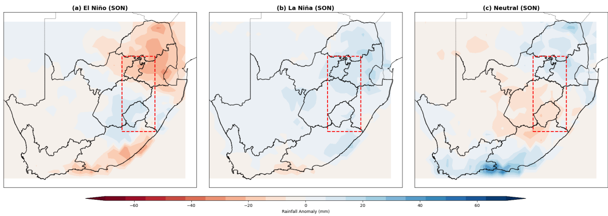
Figure 4.9: Rainfall anomaly maps (mm) for SON, associated with the ENSO cycle based on ENSO events between 1981 and 2023, for (a) El Niño, (b) La Niña and (c) Neural phases. Anomalies are calculated from the 1981-2023 average.
