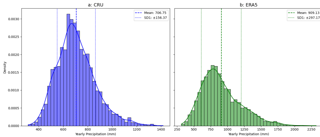
Figure 5.3: Mean annual rainfall distribution across the eastern escarpment study site for (a) CRU and (b) ERA5, with mean (thicker dotted line) and standard deviations (thinner dotted lines).
