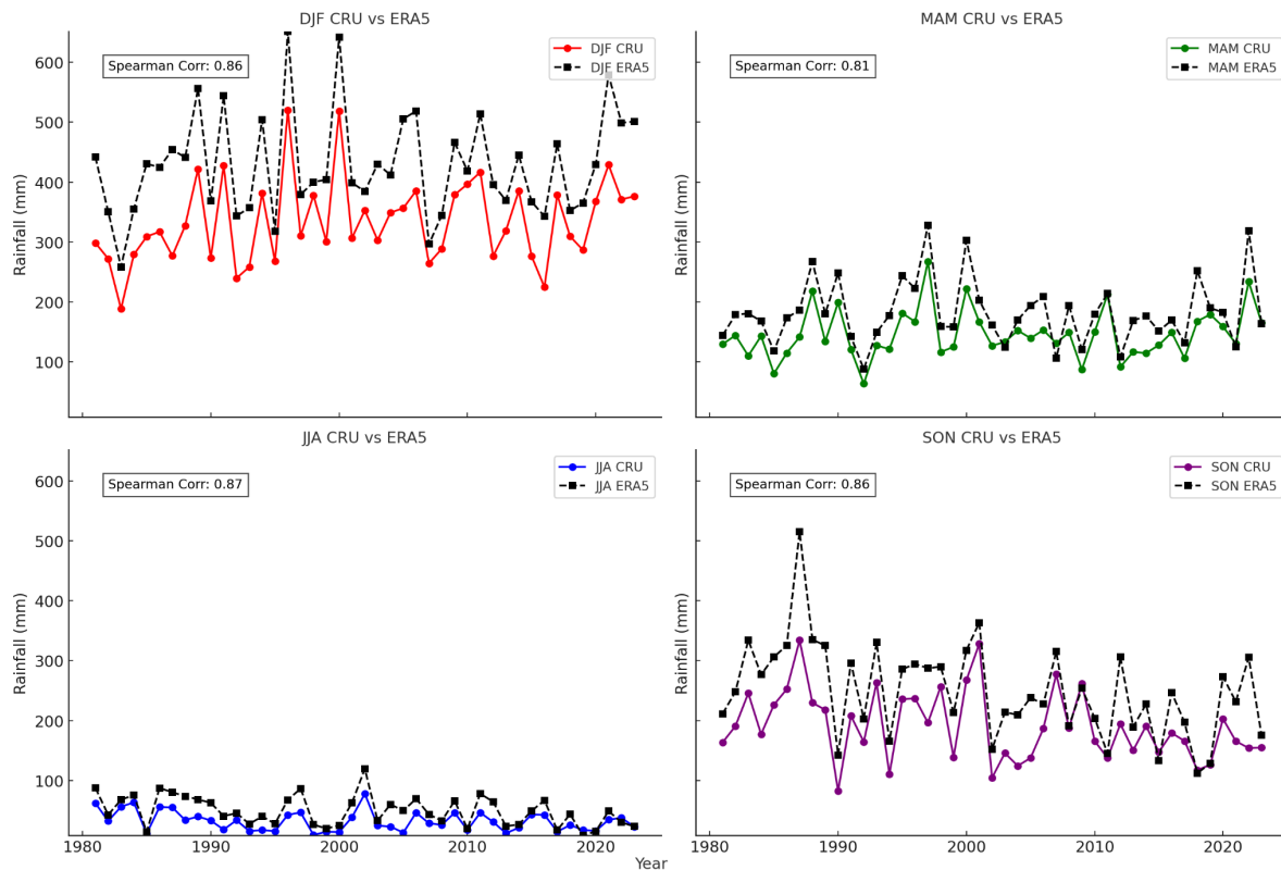
Figure 5.5: Interannual seasonal rainfall variability for CRU (solid coloured lines) and ERA5 (black dotted lines) across the eastern escarpment study site. Each subplot represents a different season (DJF, MAM, JJA, SON), and Spearman correlation coefficients indicate the similarity in rainfall variability between the two datasets for each season.
