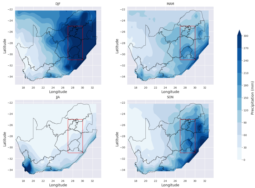
Figure 4.2: Mean seasonal CRU rainfall totals (mm) across South Africa for 1981-2023, with the rectangular (red) box highlighting the study site.
