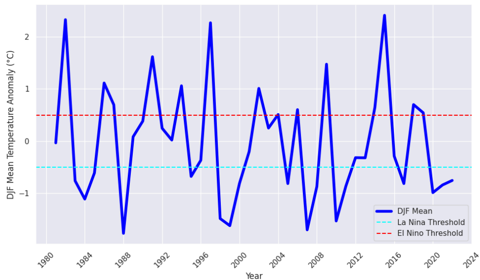
Figure 4.4: Niño 3.4 Index for the DJF season for the period 1981 to 2023.
