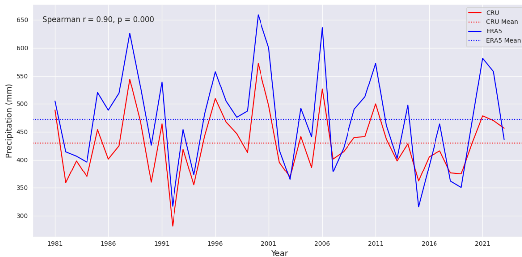
Figure 5.4: Interannual rainfall variability in the CRU (red line) and ERA5 (blue line) data sets, across the eastern escarpment study site, for the period 1981 to 2023.
