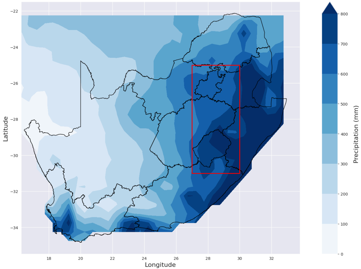
Figure 4.1: Spatial distribution of CRU total annual rainfall (mm) across South Africa, for the period 1981-2023, with the rectangular (red) box highlighting the study site.
