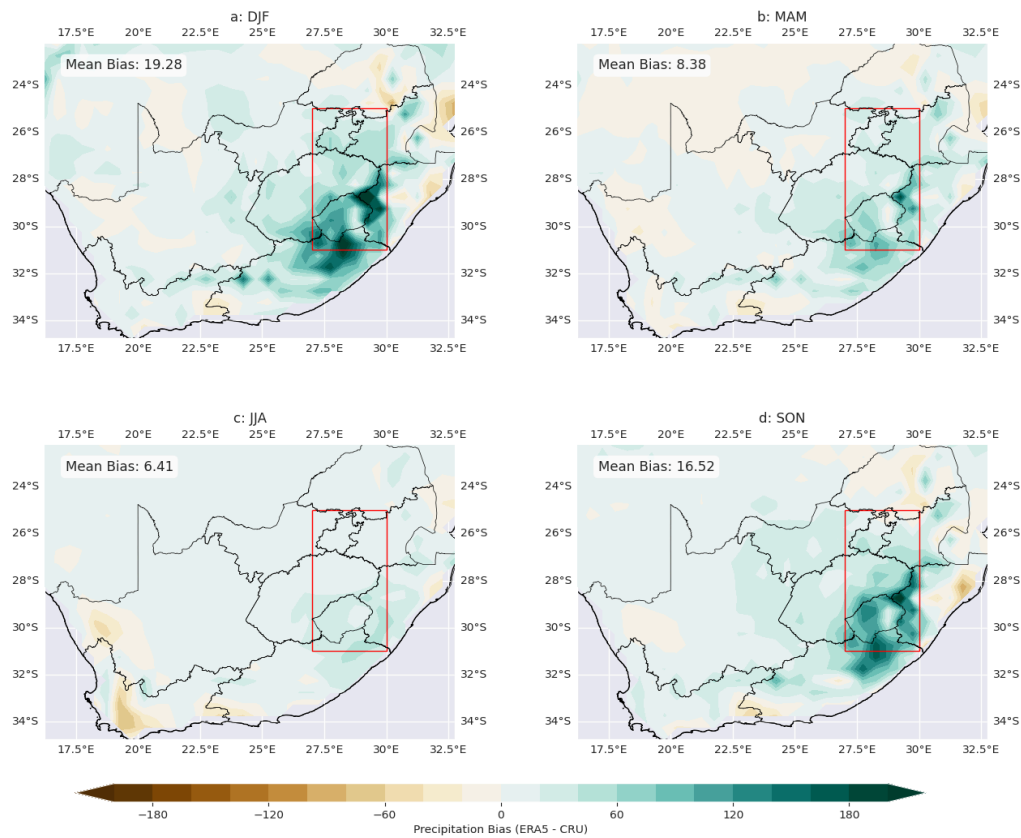
Figure 5.7: Seasonal bias in the ERA5 data relative to CRU for (a) DJF, (b) MAM, (c) JJA and (d) SON seasons.
