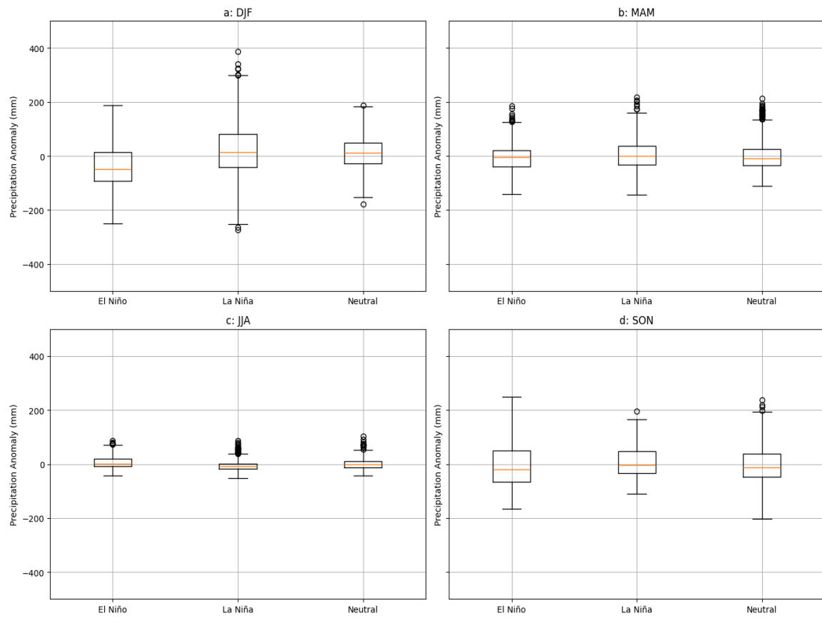
Figure 4.5: Spread in the seasonal rainfall anomalies, according to specific ENSO phases, across the eastern escarpment study site, for (a) DJF, (b) MAM, (c) JJA and (d) SON. Boxplots show the 25 th , 50 th and 75 th percentiles; whiskers extend to the most extreme values within 1.5 X IQR from the lower and upper quartiles; circles represent outliers beyond this range.
