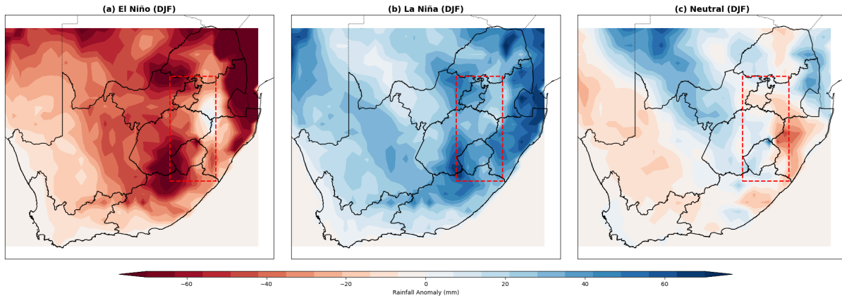
Figure 5.10: Rainfall anomaly maps (mm) for DJF, associated with the ENSO cycle based on ENSO events between 1981 and 2023, for (a) El Niño, (b) La Niña and (c) Neutral phases. Anomalies are calculated from the 1981-2023 average.
