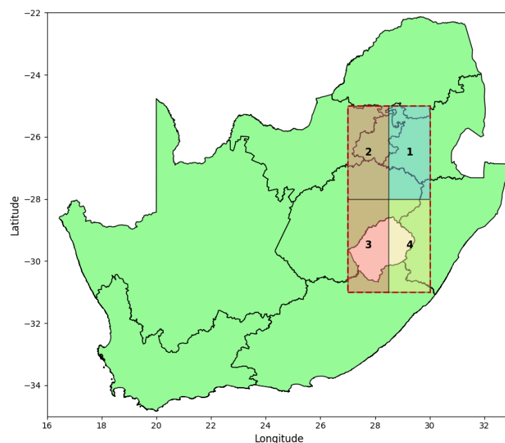
Figure 5.8: The four quadrants investigated within the eastern escarpment study site.
