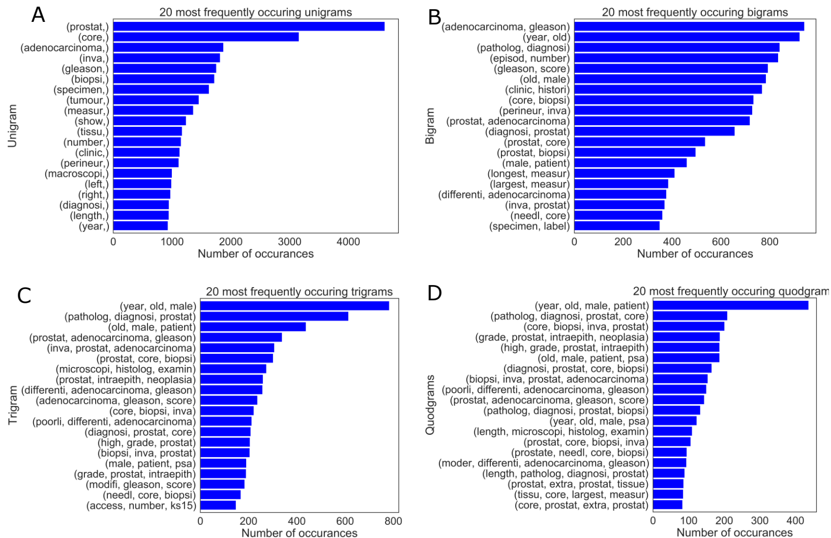
Figure 3.3: Horizontal bar graph depicting the top twenty occurring unigrams (A), bigrams (B), trigrams (C) and quadgrams (D). The number of occurrences is displayed on the x-axis.
