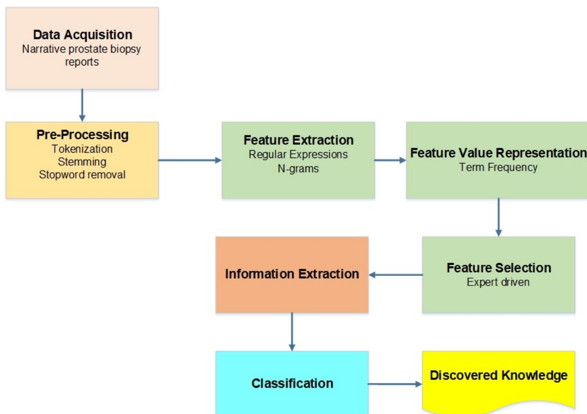
Figure 3.1: Diagram describing the logical processes used to analyse the raw narrative prostate biopsy report to generate the discovered knowledge. The steps were as follows: (i) data acquisition (ii) pre-processing and (iii) feature extraction, (iv) feature value representation, (v) feature selection, (vi) information extraction (vii) classification and (viii) discovered knowledge.
