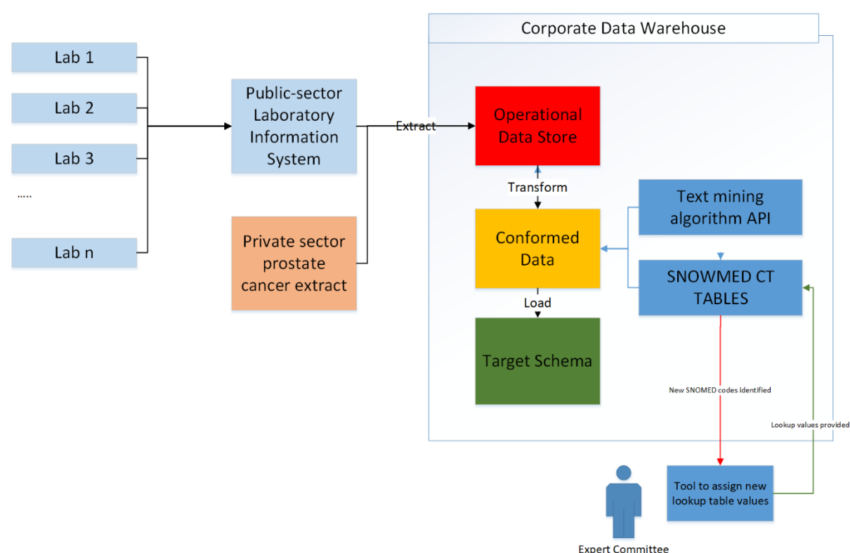
Figure 6.3: Database diagram showing how the SNOMED CT lookup tables and text mining application programming interface (API) could automate the generation of a PCa diagnosis. The private sector prostate cancer data extract could also be accommodated through the CDW process. The Expert Committee would code all new SNOMED CT M and T code combinations to update the CDW lookup tables.
