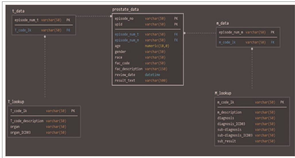
FIGURE 3: Relational database diagram describes how the various tables were joined (left outer). For each table, the primary and foreign keys are provided. The lookup tables contain only the unique Systemized Nomenclature of Medicine code combinations. The lines indicate a relationship join between tables. Once the table joins are implemented, variables from any table can be reported. Structured query language could be used to combine the required data for analysis.
