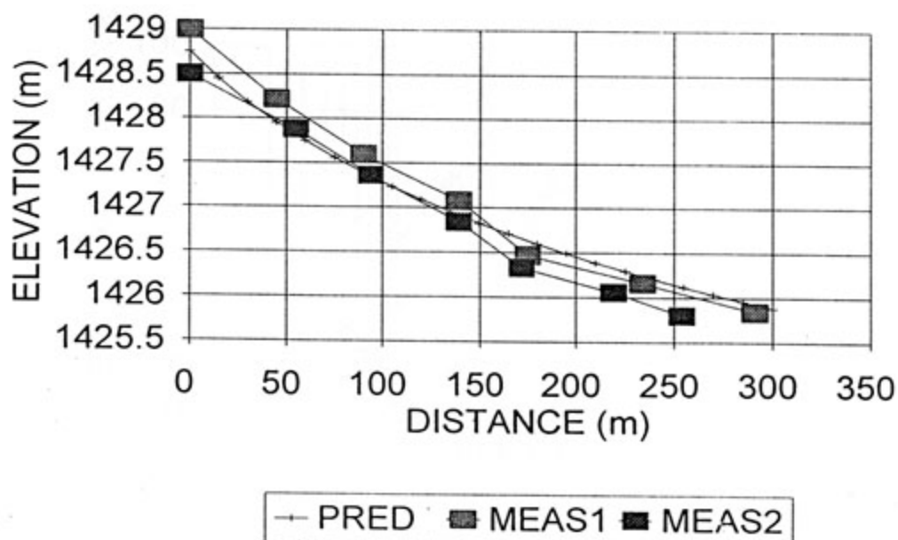
FIGURE 8.51 : CALIBRATED BEACH PROFILE - COARSER PRODUCT
