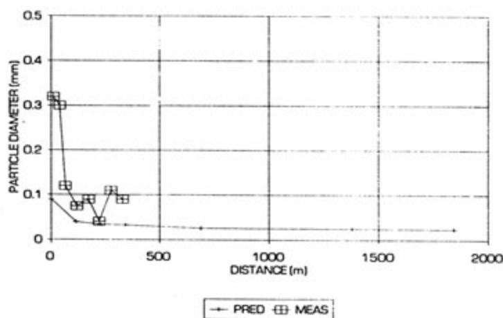
FIGURE 7.26 : COMPARISON OF d_{50} SIZE WITH DISTANCE
