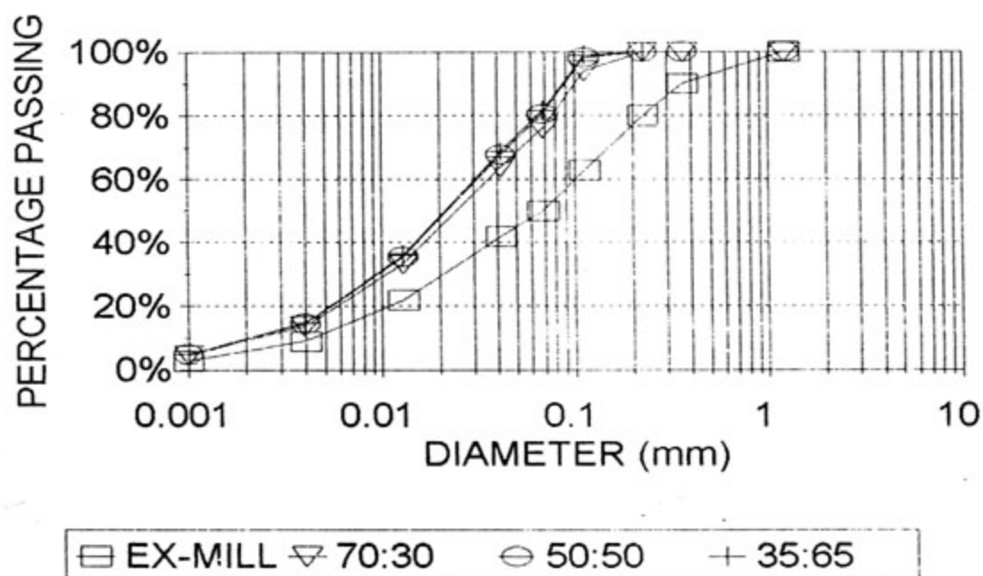
FIGURE 5.18 : PREDICTED PARTICLE SIZE DISTRIBUTIONS FOR VARIATIONS IN WATER:SOLIDS RATIO - AT 125 m
