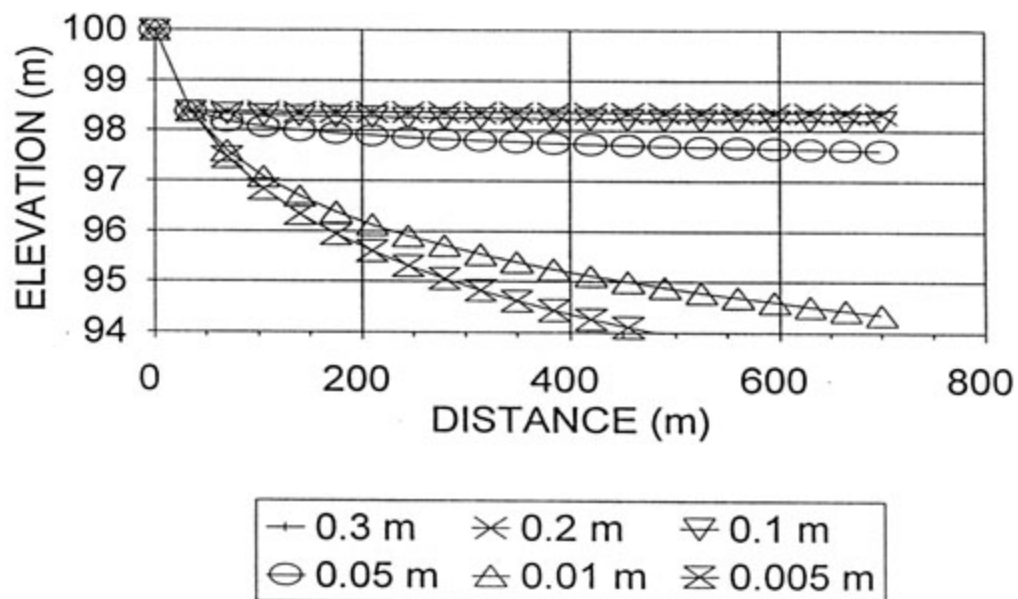
FIGURE 8.18 : 700 m BEACH, COARSE PRODUCT, DENSITY 1,75 t/m 3
