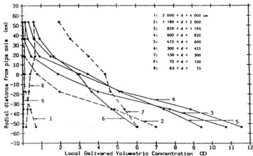
FIGURE 2.6 VARIATION OF LOCAL CONCENTRATION OF DIFFERENT SIZE FRACTIONS (After Cooke and Lazarus (1988))
