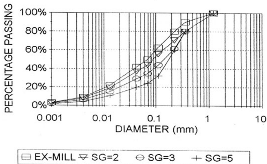
FIGURE 5.7 : PREDICTED PARTICLE SIZE DISTRIBUTIONS FOR VARIATIONS IN PARTICLE SPECIFIC GRAVITY - AT DISCHARGE
