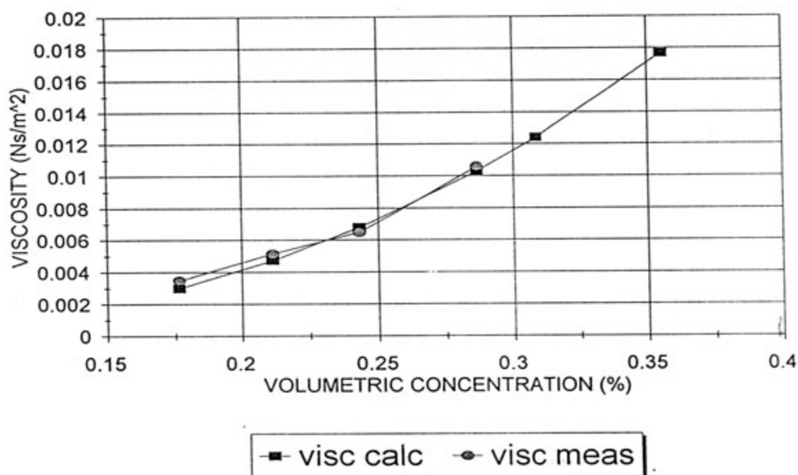
FIGURE 8.12 : CONCENTRATION vs VISCOSITY
