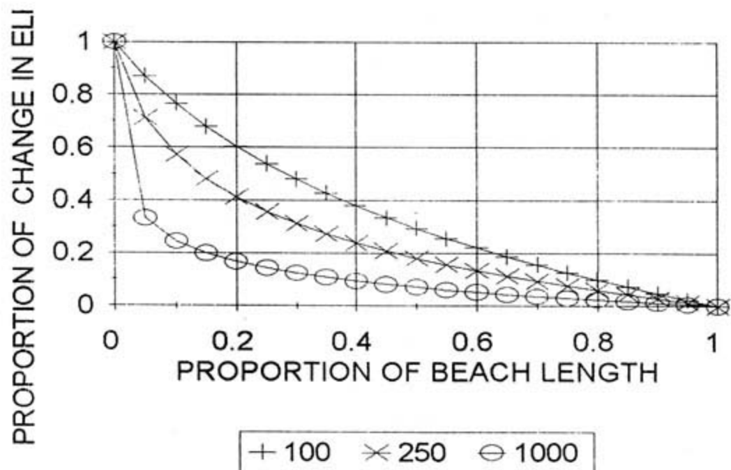
FIGURE 5.21 : PREDICTED NORMALISED BEACH PROFILES FOR VARIATION IN BEACH LENGTH
