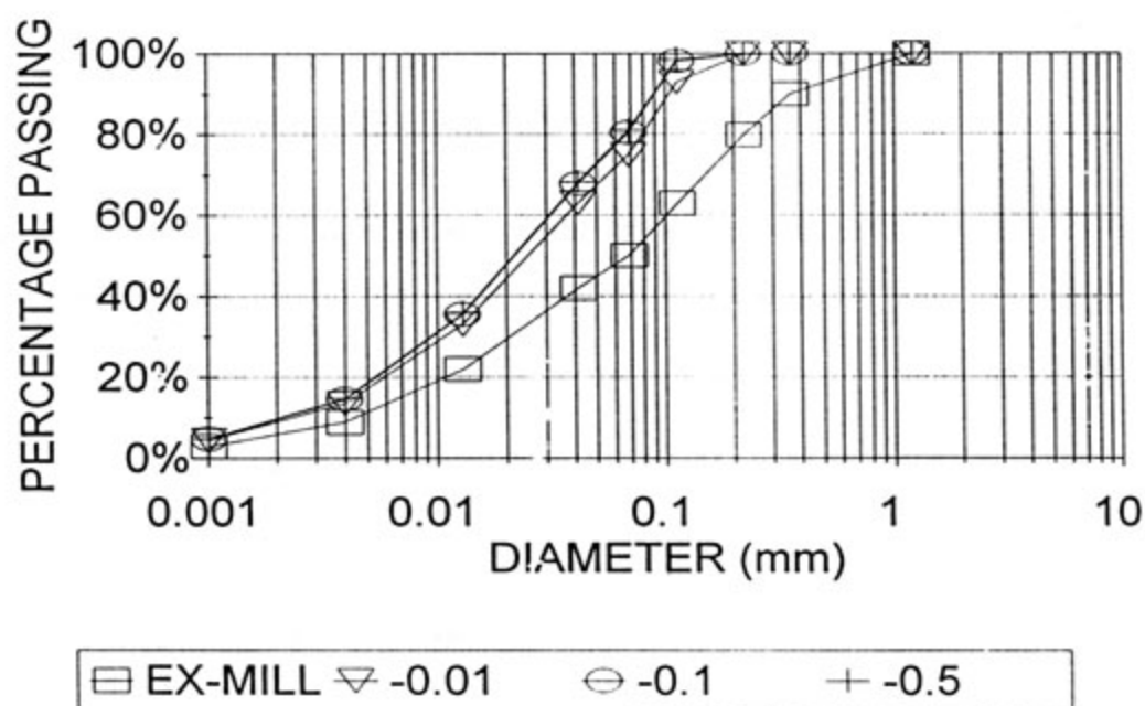
FIGURE 5.32 : PREDICTED PARTICLE SIZE DISTRIBUTION FOR VARIATION IN FRICTIONAL RESISTANCE (initial beach slope) - AT 125 m
