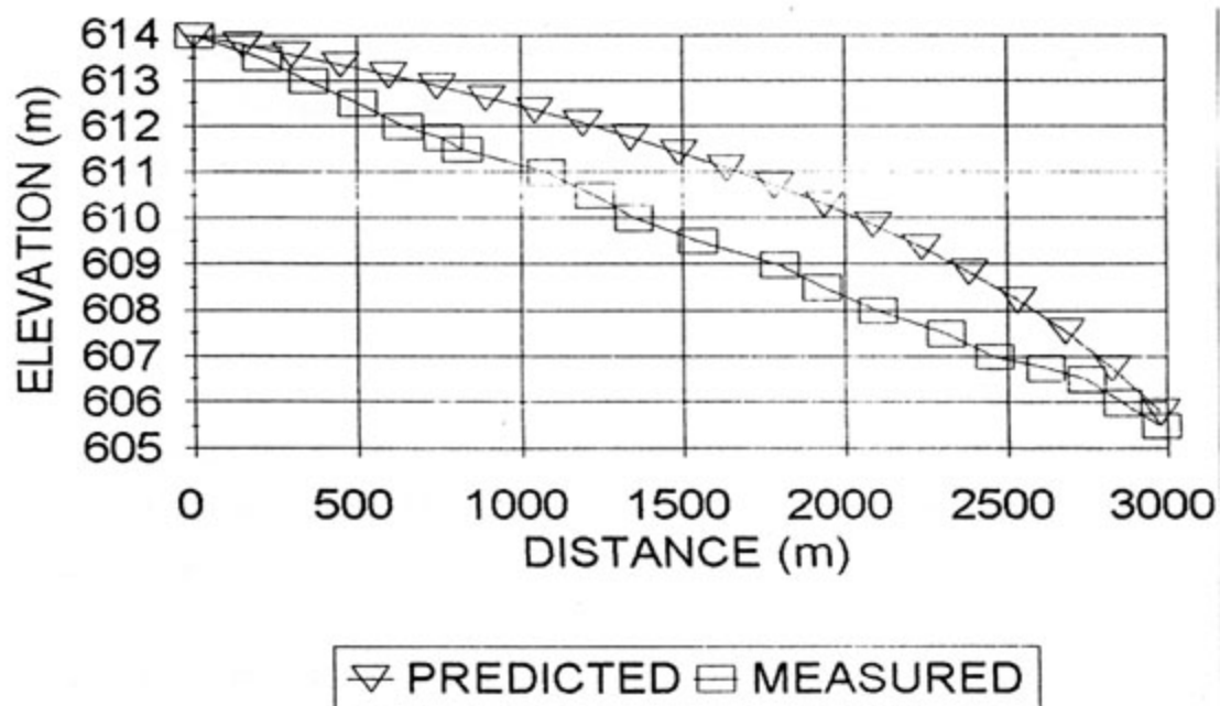
FIGURE 6.14 : PREDICTED BEACH PROFILE USING DATA FROM THE FLUME TEST FOR A FLOW RATE OF 2,6 l/s
