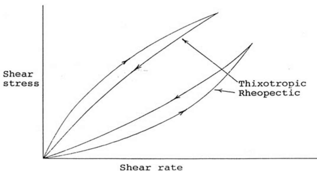
FIGURE 2.11 : TYPICAL RHEOGRAMS FOR TIME-DEPENDENT FLUIDS
