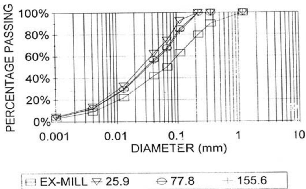
FIGURE 5.13 : PREDICTED PARTICLE SIZE DISTRIBUTIONS FOR VARIATIONS IN FLOW RATE - AT 25 m
