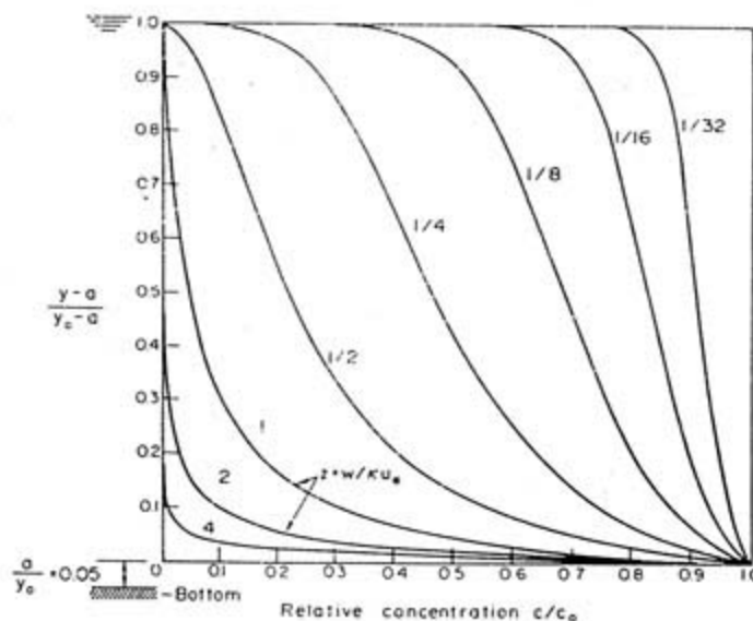
FIGURE 2.1 DISTRIBUTION OF SUSPENDED LOAD IN A FLOW ACCORDING TO THE EQUATION OF ROUSE - Equation 12. (After Raudkivi (1991))
