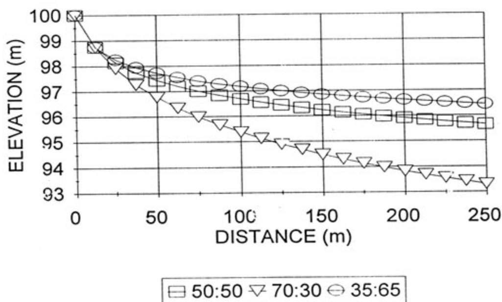
FIGURE 5.16 : PREDICTED BEACH PROFILE FOR VARIATIONS IN WATER:SOLIDS RATIO
