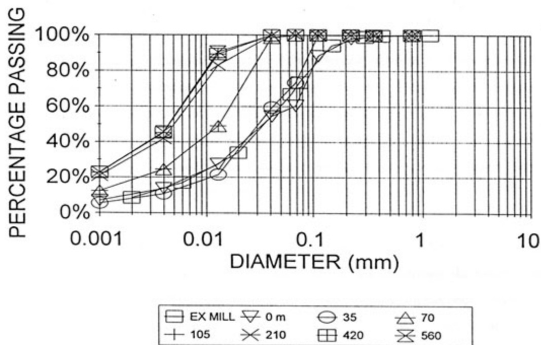
FIGURE 8.27 : 700 m BEACH, FINE PRODUCT, DISCHARGE HEIGHT 0,2 m, DENSITY 1,75 t/m 3
