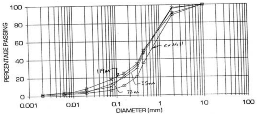
FIGURE 7.6: MEASURED PARTICLE SIZE DISTRIBUTIONS
