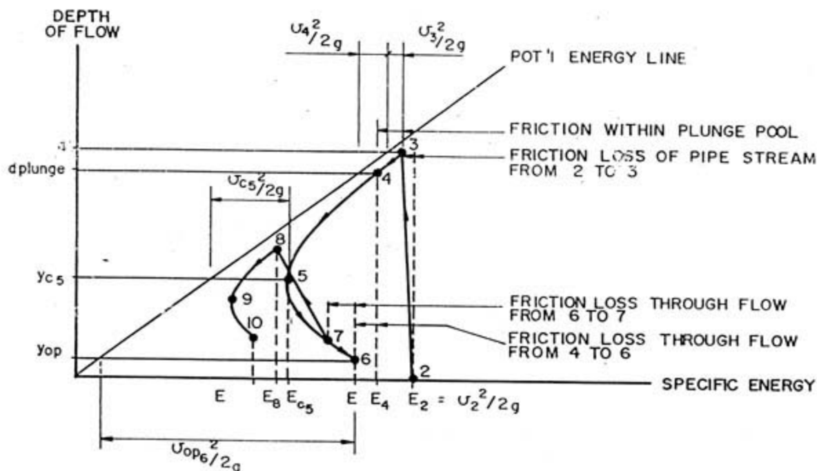
FIGURE 3.7 : TYPICAL SPECIFIC ENERGY DIAGRAM FOR THE PLUNGE POOL AND DISCHARGE CHANNEL
