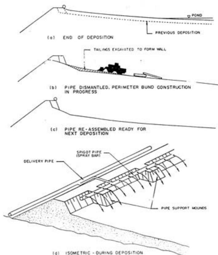
FIGURE 1.18 : SECTIONS ILLUSTRATING THE SEQUENCE OF OPERATION OF A TYPICAL SOUTH AFRICAN TAILINGS DAM CONSTRUCTED USING SPIGOTS ON A SPRAY-BAR
