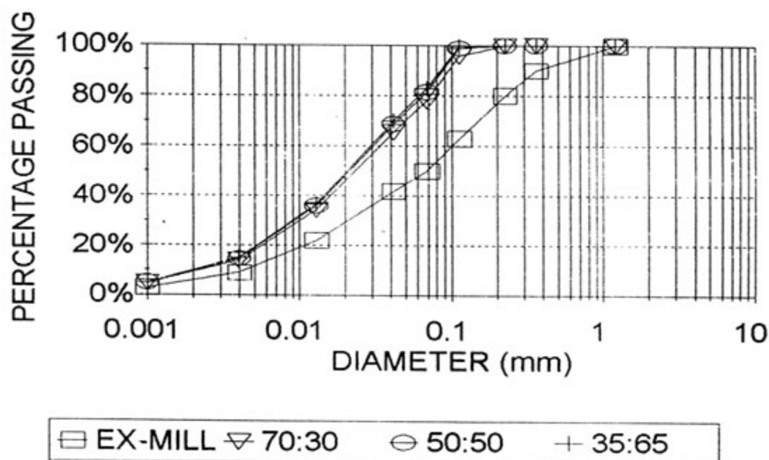
FIGURE 5.19 : PREDICTED PARTICLE SIZE DISTRIBUTIONS FOR VARIATIONS IN WATER:SOLIDS RATIO - AT 225 m
