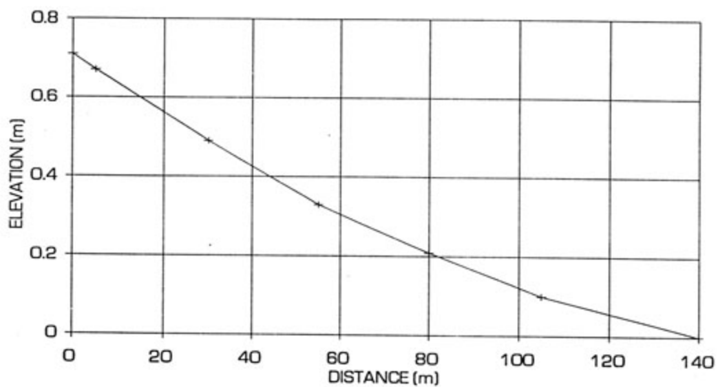
FIGURE 4.9 : THOMSON GOLD DATA - MEASURED BEACH PROFILE
