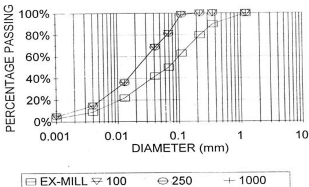
FIGURE 5.24 : PREDICTED PARTICLE SIZE DISTRIBUTION FOR VARIATION IN BEACH LENGTH - AT 225 m
