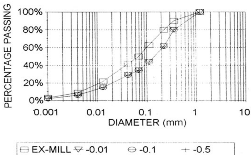
FIGURE 5.31 : PREDICTED PARTICLE SIZE DISTRIBUTION FOR VARIATION IN FRICTIONAL RESISTANCE (initial beach slope) - AT DISCHARGE
