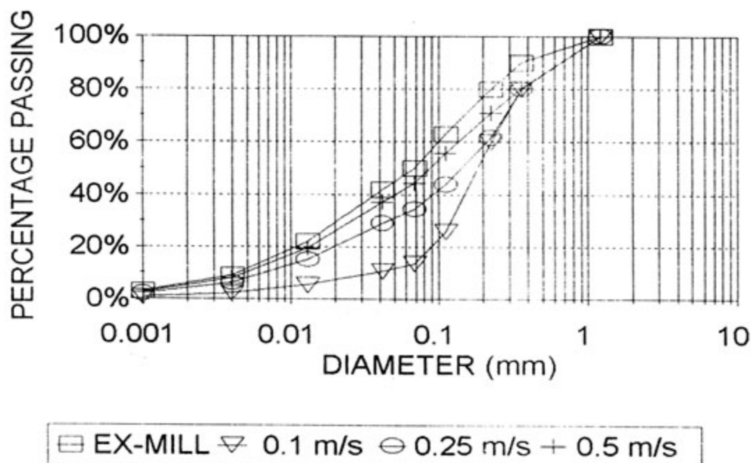
FIGURE 5.27 : PREDICTED PARTICLE SIZE DISTRIBUTION FOR VARIATION IN VELOCITY EX-PLUNGE POOL - AT DISCHARGE
