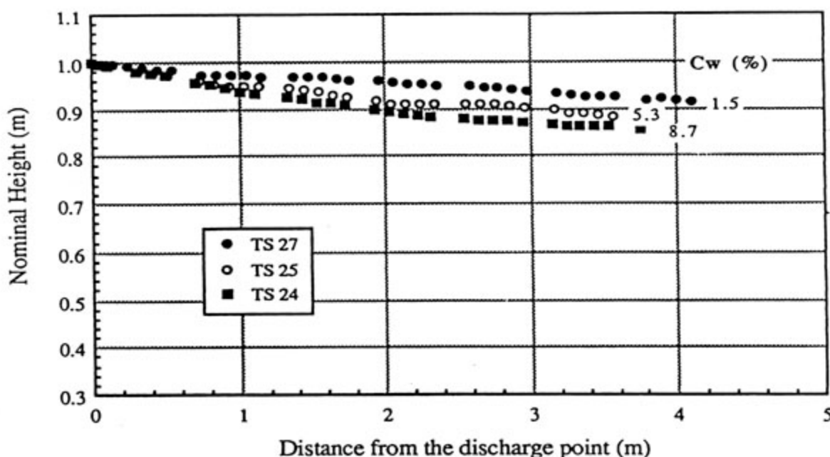
FIGURE 6.4 : PROFILES OF TS TESTS WITH Q_t = 20 l/min AND VARIOUS C_w (After Kùpper (1991))
