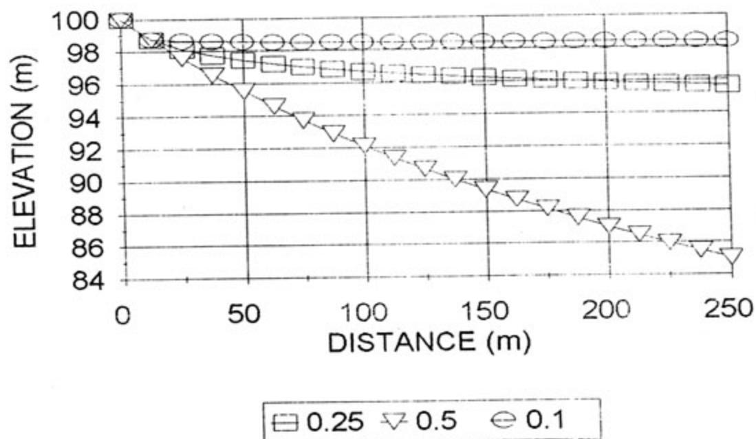
FIGURE 5.26 : PREDICTED BEACH PROFILES FOR VARIATION IN VELOCITY EX-PLUNGE POOL
