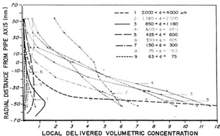
FIGURE 3.1: VARIATION OF LOCAL CONCENTRATION OF DIFFERENT SIZE FRACTIONS (After Cooke and Lazarus (1988)) WITH CONCENTRATIONS PREDICTED USING HUNT'S EQUATIONS (HUNT (1967))
