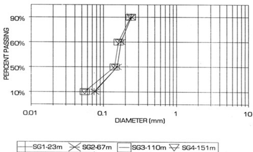
FIGURE 4.6 : KÜPPER:TEST 4 SECTION 1 - MEASURED PARTICLE SIZE DISTRIBUTIONS
