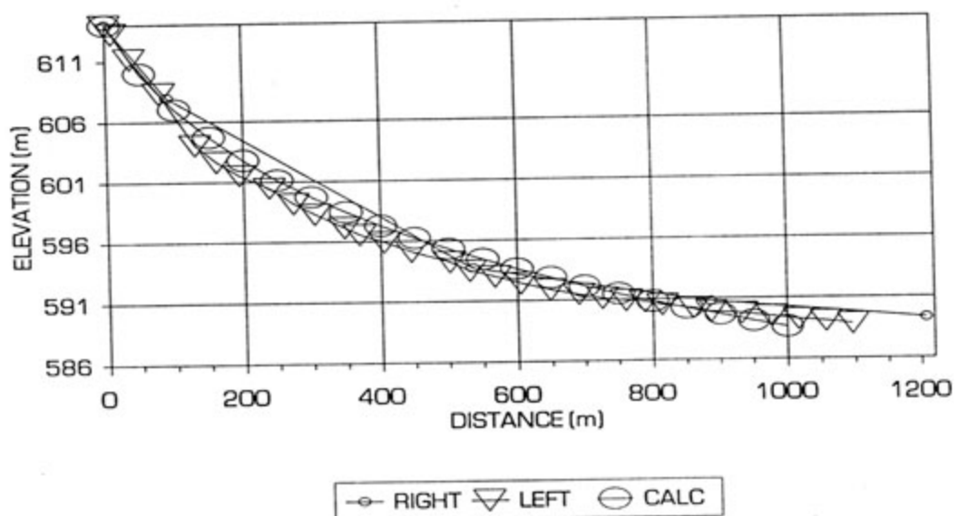
FIGURE 7.9 : PREDICTED BEACH PROFILES FOR RÖSSING OLD BEACH
