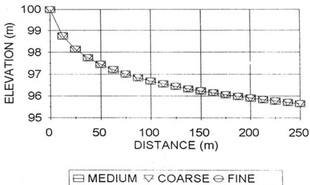
FIGURE 5.2 : PREDICTED BEACH PROFILES - COARSE, MEDIUM AND FINE PRODUCTS
