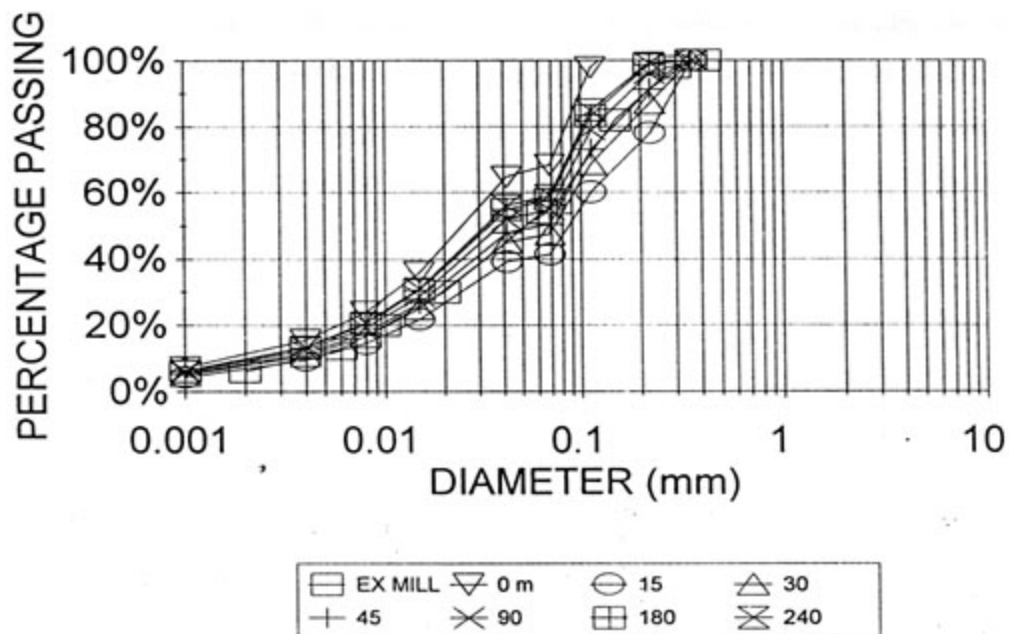
FIGURE 8.52 : PREDICTED PARTICLE SIZE DISTRIBUTIONS - COARSER PRODUCT WITH INDIVIDUAL DISCHARGES COMBINING DOWN THE BEACH
