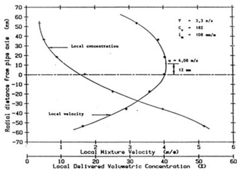
FIGURE 2.4 MEASURED VELOCITY AND CONCENTRATION PROFILES (After Cooke and Lazarus (1988))
