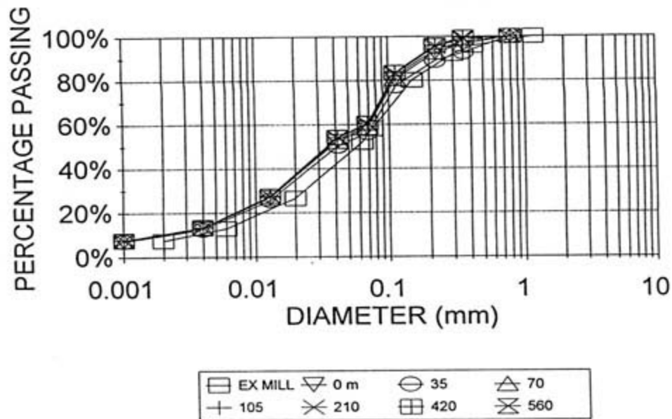
FIGURE 8.22 : 700 m BEACH, COARSE PRODUCT, DISCHARGE HEIGHT 0,01 m, DENSITY 1,45 t/m 3
