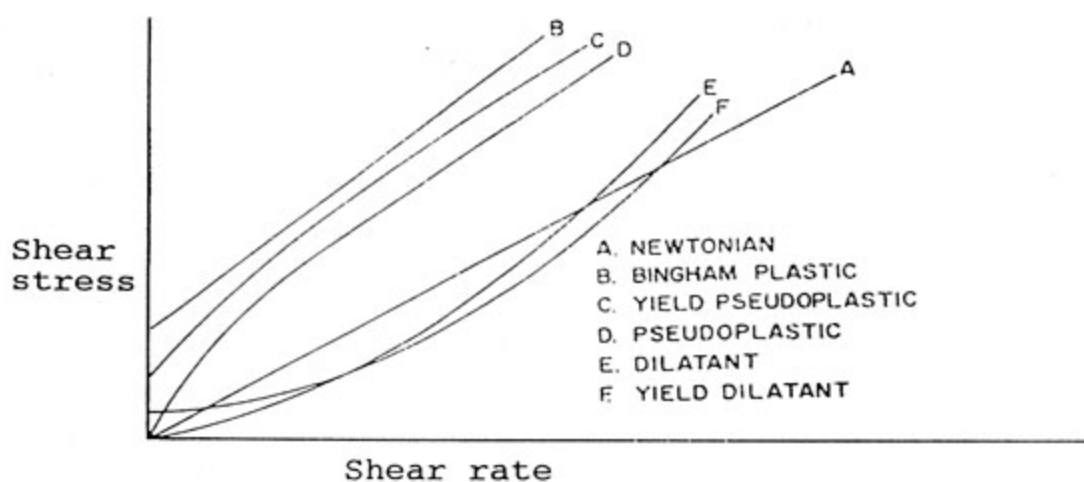
FIGURE 2.10 : TYPICAL RHEOGRAMS FOR TIME-INDEPENDENT FLUIDS
