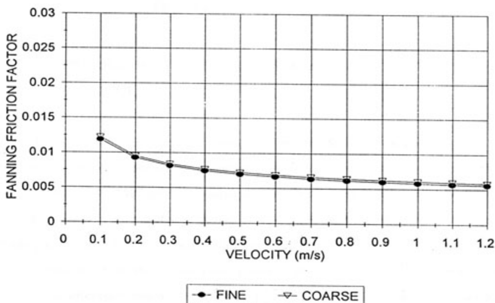
FIGURE 8.44 : FANNING FRICTION FACTORS FROM VERKERK RUNS
