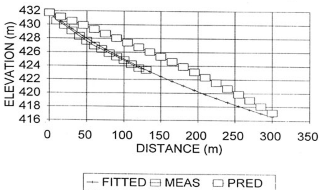
FIGURE 7.30 : CALIBRATED, MEASURED AND PREDICTED BEACH PROFILES
