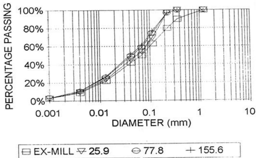
FIGURE 5.12 : PREDICTED PARTICLE SIZE DISTRIBUTIONS FOR VARIATIONS IN FLOW RATE - AT 12,5 m
