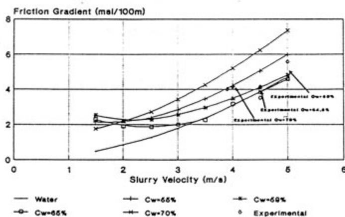
Figure 11 332mm Friction Gradients
