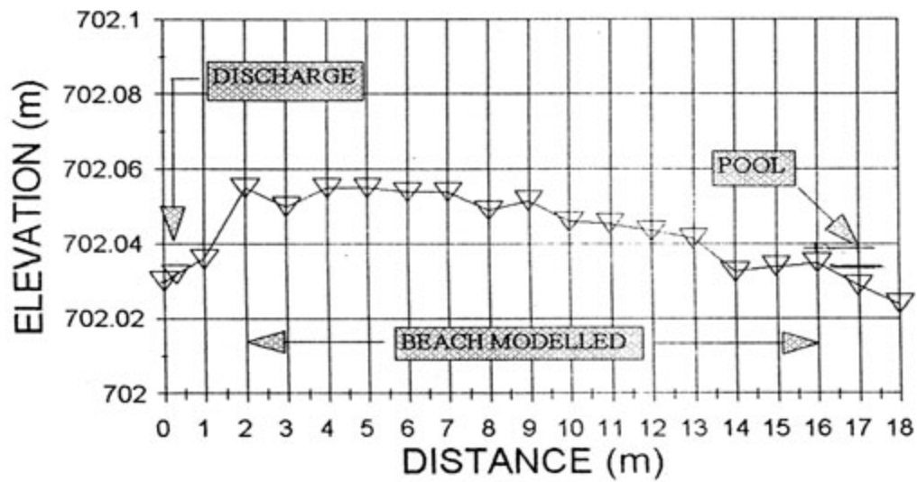
FIGURE 6.10 : MEASURED BEACH PROFILE FOR FLOW RATE OF 2,6 l/s
