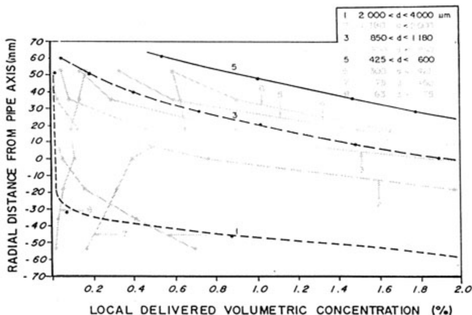
FIGURE 3.1: VARIATION OF LOCAL CONCENTRATION OF DIFFERENT SIZE FRACTIONS (After Cooke and Lazarus (1988)) WITH CONCENTRATIONS PREDICTED USING HUNT'S EQUATIONS (HUNT (1967))
