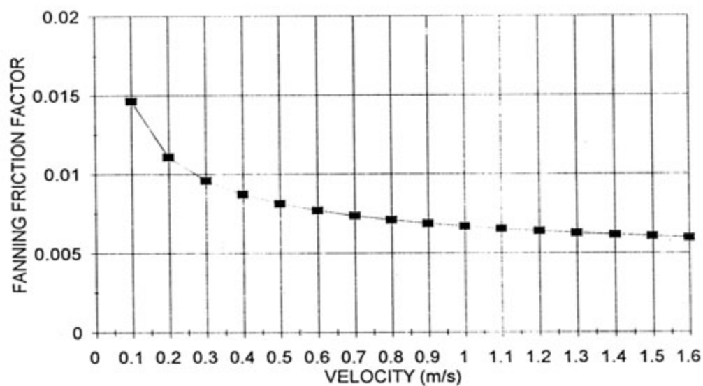
FIGURE 7.20 : FANNING FRICTION PARAMETERS
