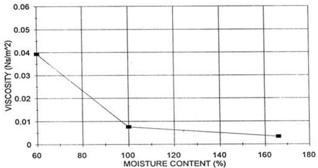
FIGURE 7.18 : BINGHAM VISCOSITY vs MOISTURE CONTENT
