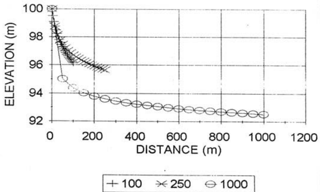
FIGURE 5.20 : PREDICTED BEACH PROFILES FOR VARIATION IN BEACH LENGTH
