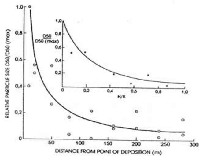
FIGURE 1.4 : FRACTIONATION OF TAILINGS (After Bentel (1981) and Blight and Bentel (1983))
