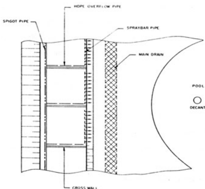
FIGURE 8.33 : SECTION THROUGH HYBRID DEPOSITION SYSTEM ILLUSTRATING COVERING OF THE MAIN DRAIN
