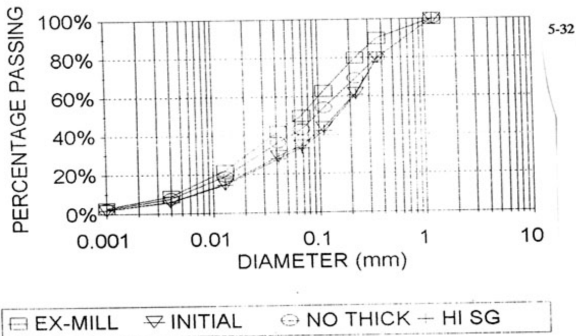
FIGURE 5.35 : PREDICTED PARTICLE SIZE DISTRIBUTIONS FOR VARIATION OF THICKENER OPERATION AND ORE TYPE - AT DISCHARGE
