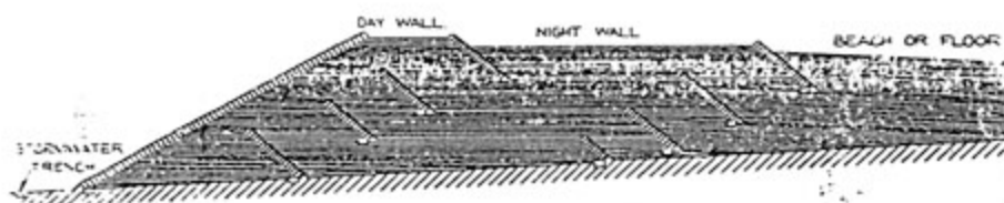
SECTION THROUGH WALL SHOWING SUCCESSIVE STEPPINGS BACK OF INNER BOUNDARIES OF DAY AND NIGHT WALLS.
