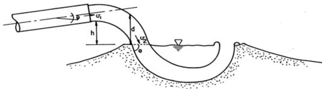
(a) SECTION A-A THROUGH PLUNGE POOL
