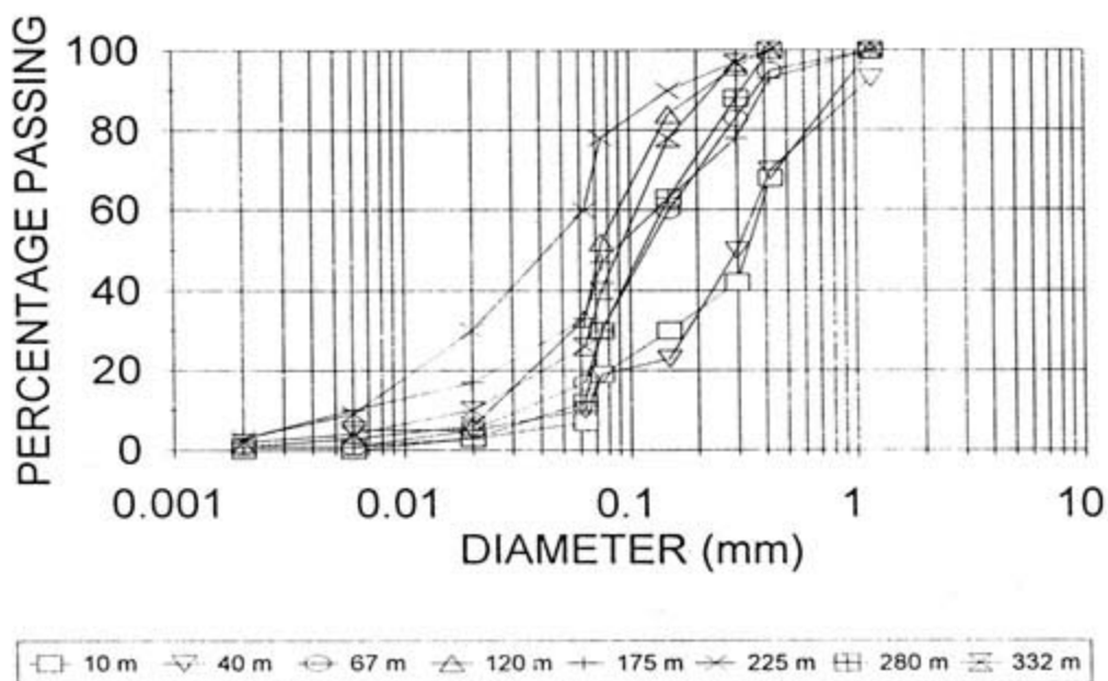
FIGURE 7.24 : MEASURED PARTICLE SIZE DISTRIBUTIONS
