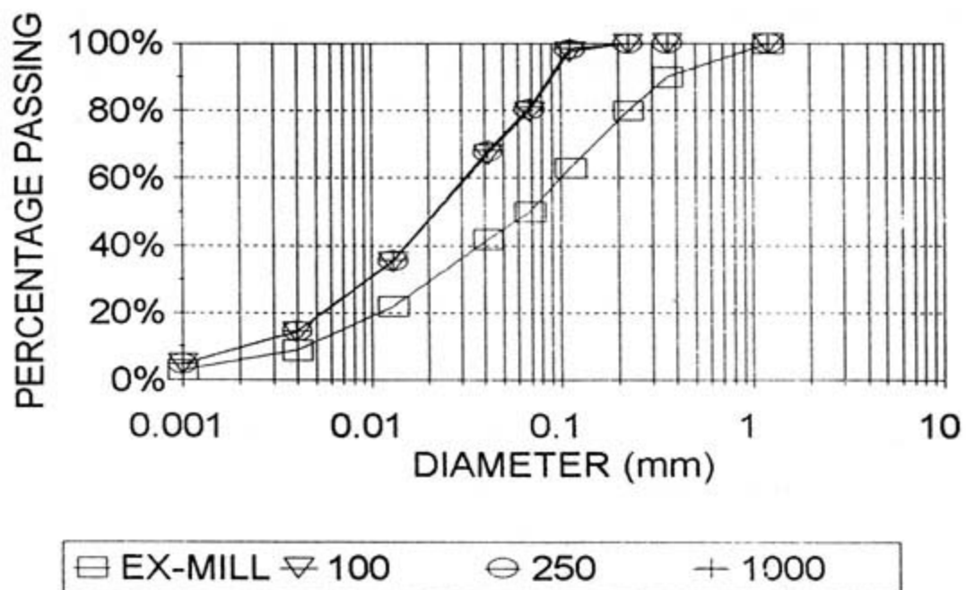
FIGURE 5.23 : PREDICTED PARTICLE SIZE DISTRIBUTIONS FOR VARIATION IN BEACH LENGTH - AT 125 m
