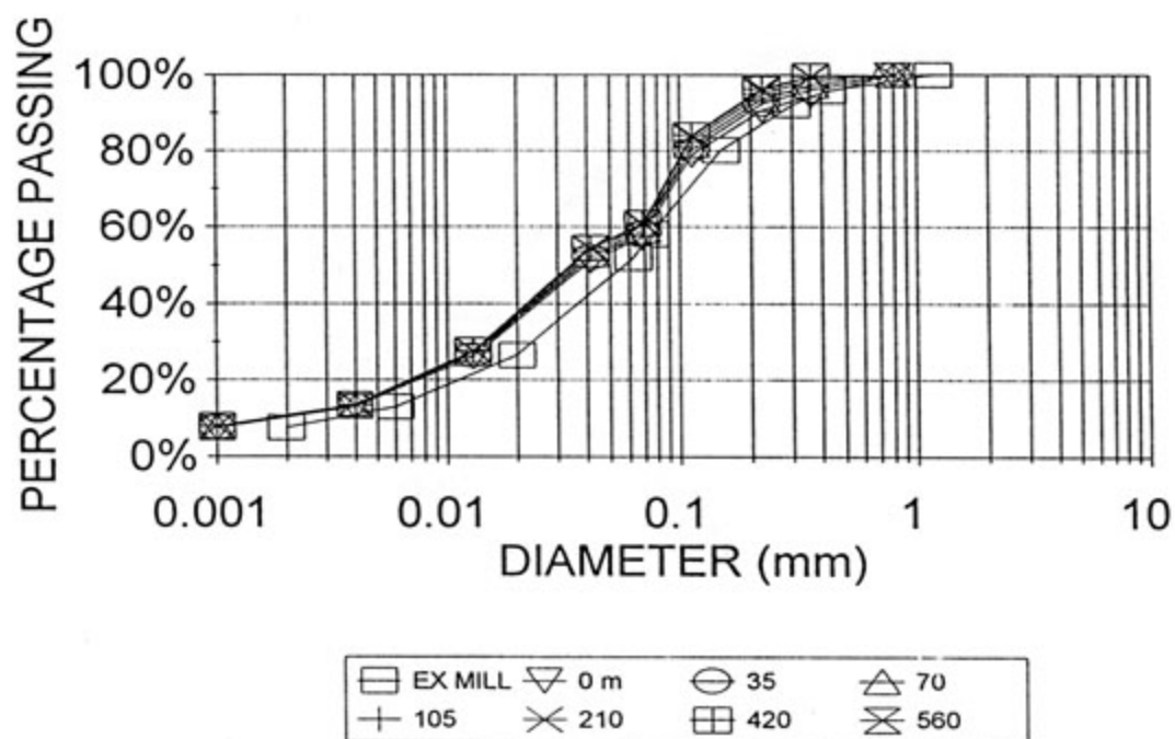
FIGURE 8.26 : 700 m BEACH, COARSE PRODUCT, DISCHARGE HEIGHT 0,01 m, DENSITY 1,75 t/m 3
