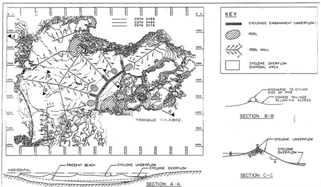
FIGURE 8.10 : LAYOUT OF PADDOCKS ON A LARGE TAILINGS DAM
