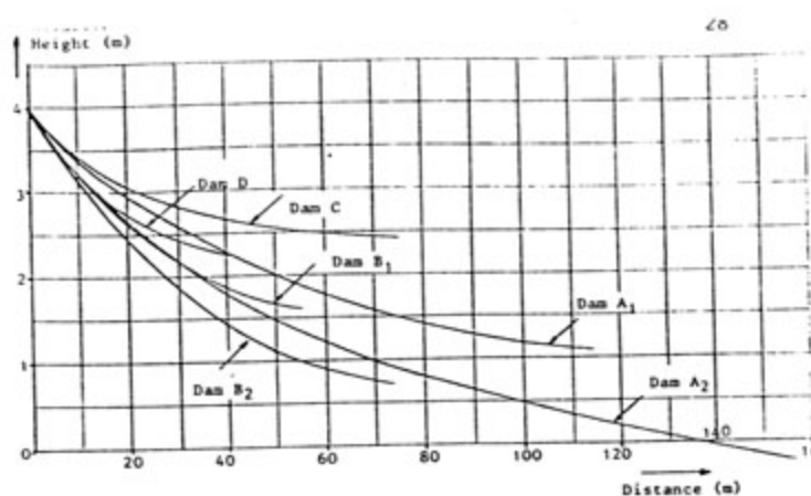
Figure 2.6: Measured Beach Profiles (Platinum)
