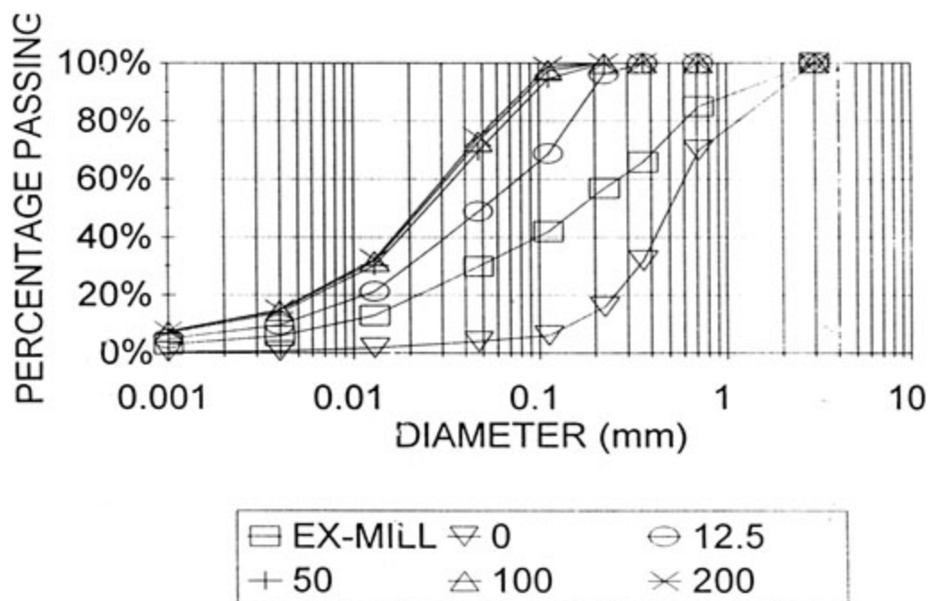
FIGURE 5.3 : PREDICTED PARTICLE SIZE DISTRIBUTIONS - COARSE PRODUCT
