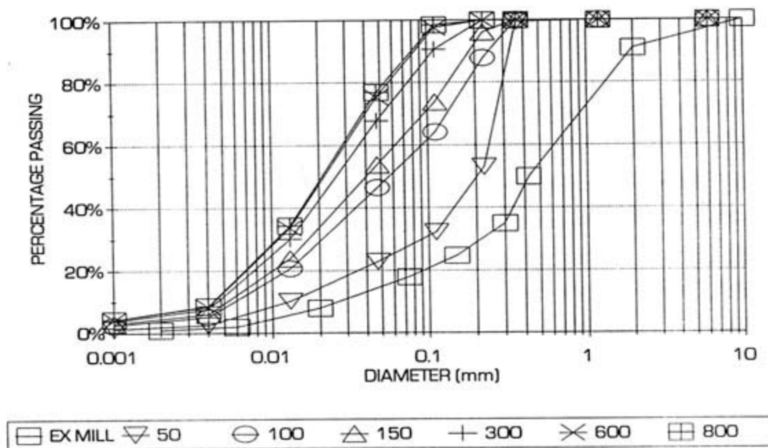
FIGURE 7.11 : PREDICTED PARTICLE SIZE DISTRIBUTIONS FOR RÖSSING OLD BEACH
