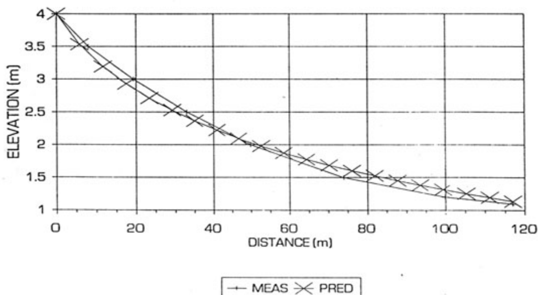
FIGURE 4.15 : BENTEL PLATINUM DATA - PREDICTED BEACH PROFILE
