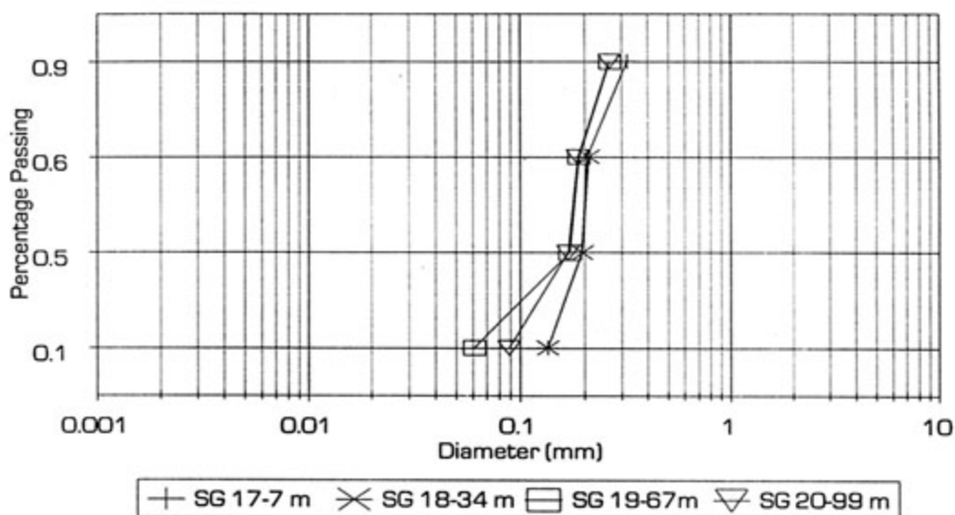
FIGURE 4.5 : KÜPPER:TEST 1 SECTION 3 - MEASURED PARTICLE SIZE DISTRIBUTIONS
