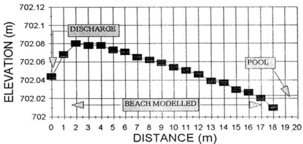
FIGURE 6.11 : MEASURED BEACH PROFILE FOR FLOW OF 0,44 l/s
