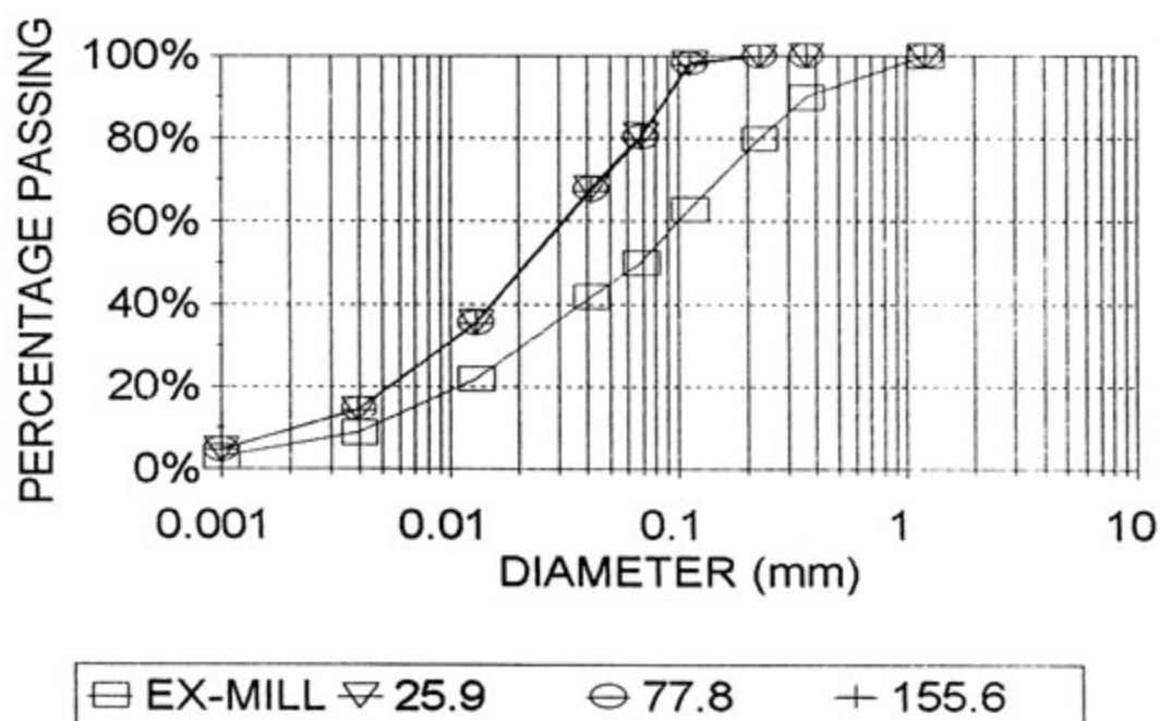
FIGURE 5.14 : PREDICTED PARTICLE SIZE DISTRIBUTIONS FOR VARIATIONS IN FLOW RATE - AT 125 m
