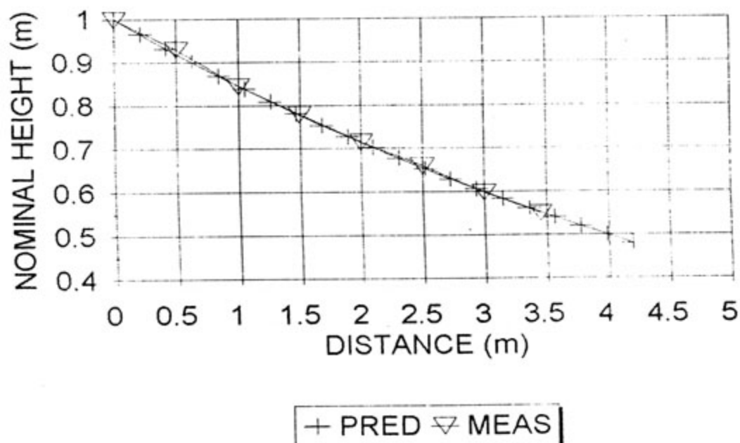
FIGURE 6.5 : MEASURED AND CALIBRATED BEACH PROFILES FOR FLUME TEST TS 19
