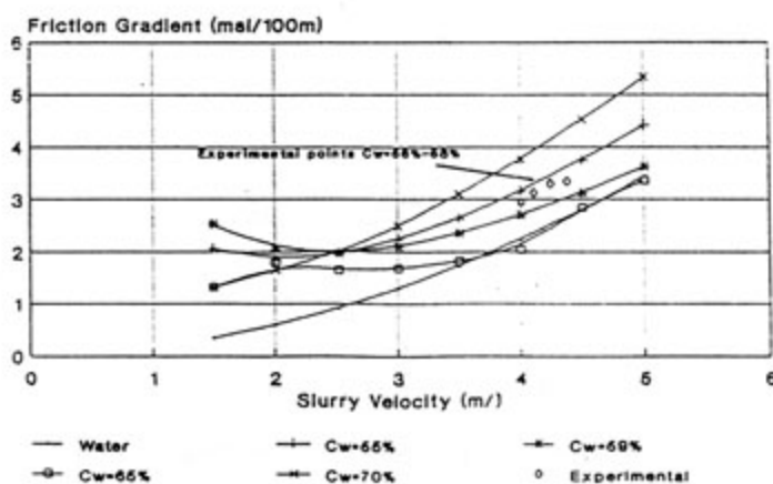
Figure 12 432mm Friction Gradients
