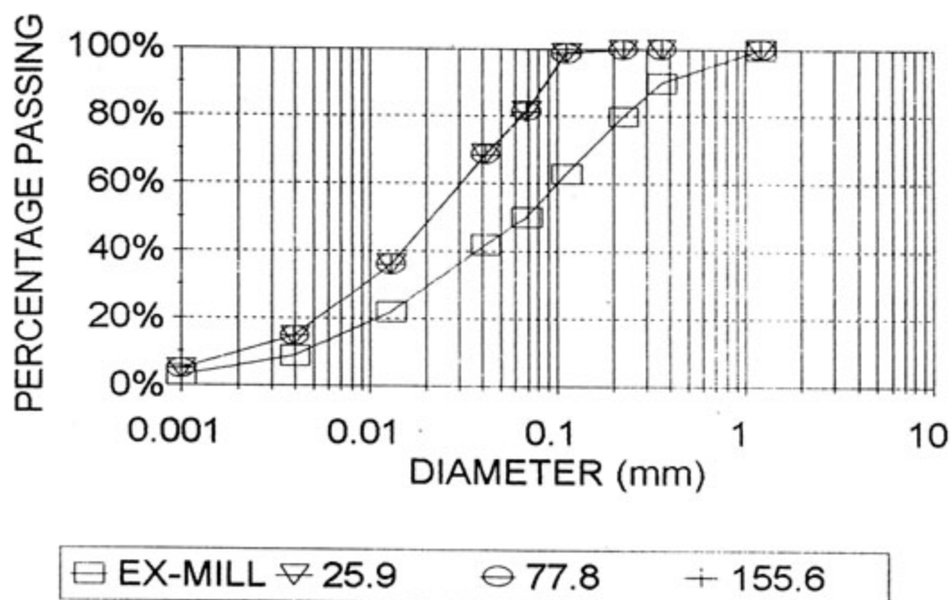
FIGURE 5.15 : PREDICTED PARTICLE SIZE DISTRIBUTIONS FOR VARIATIONS IN FLOW RATE - AT 225 m
