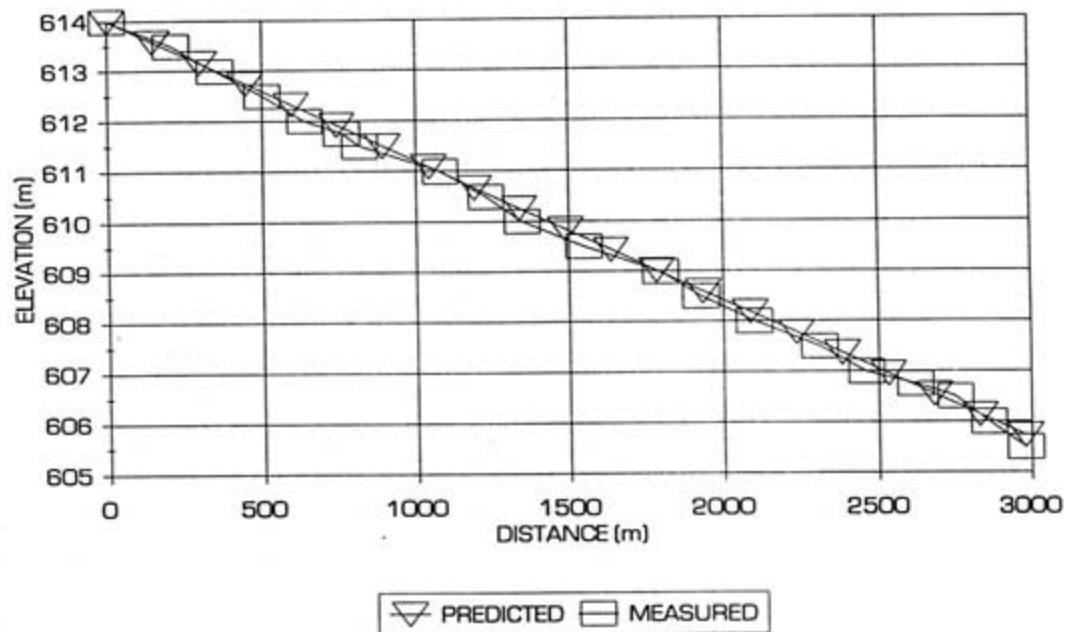
FIGURE 7.15 : CALIBRATED AND MEASURED BEACH PROFILES
