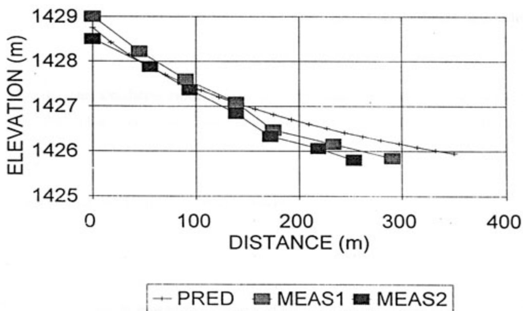
FIGURE 8.56 : PREDICTED BEACH PROFILE - FINER PRODUCT COMBINED SPIGOT FLOWS
