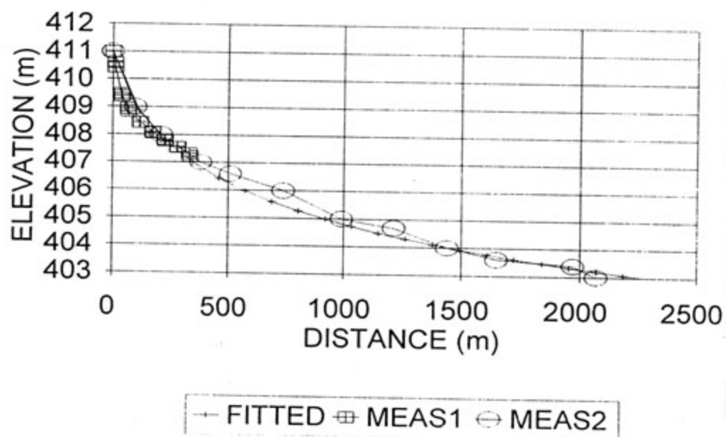
FIGURE 7.21 : MEASURED AND CALIBRATED PROFILES
