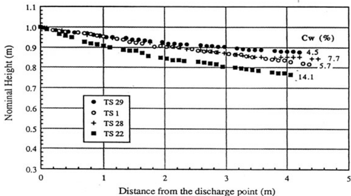
FIGURE 6.3 : PROFILES OF TS TESTS WITH Q_t = 15 l/min AND VARIOUS C_w (After Kùpper (1991))
