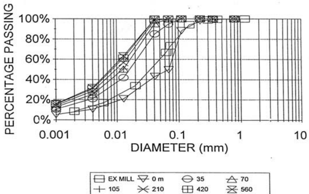
FIGURE 8.23 : 700 m BEACH, FINE PRODUCT, DISCHARGE HEIGHT 0,2 m, DENSITY 1,45 t/m 3
