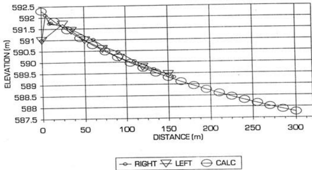
FIGURE 7.5: MEASURED AND PREDICTED BEACH PROFILES
