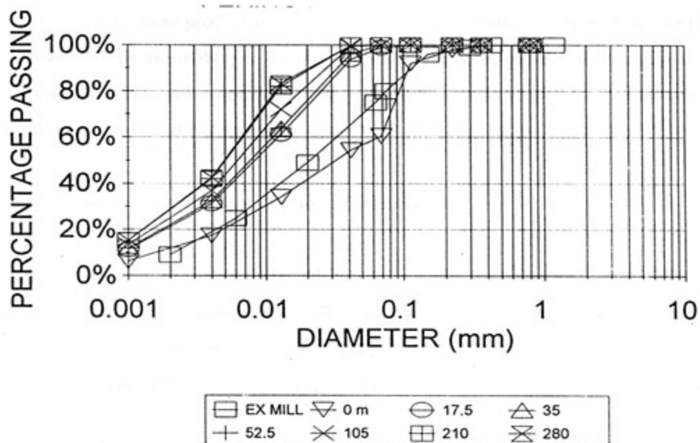
FIGURE 8.48: PREDICTED PARTICLE SIZE DISTRIBUTIONS - FINE PRODUCT : POINT DISCHARGE
