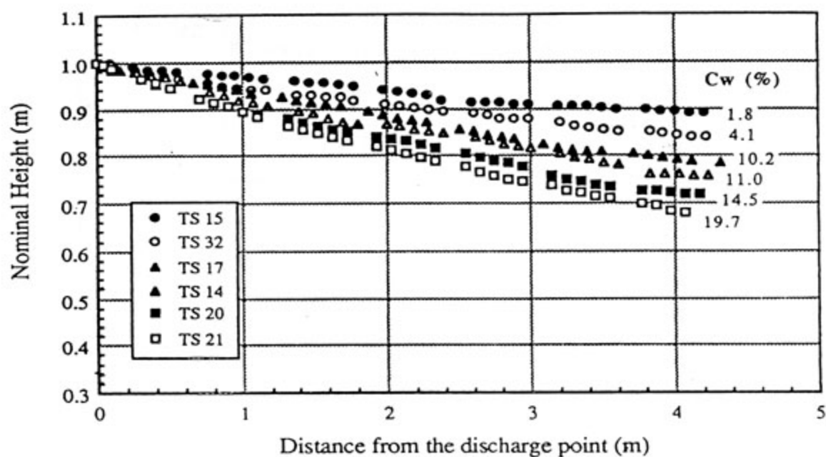
FIGURE 6.2 : PROFILES OF TS TESTS WITH Q_t = 10 l/min AND VARIOUS C_w (After Kùpper (1991))
