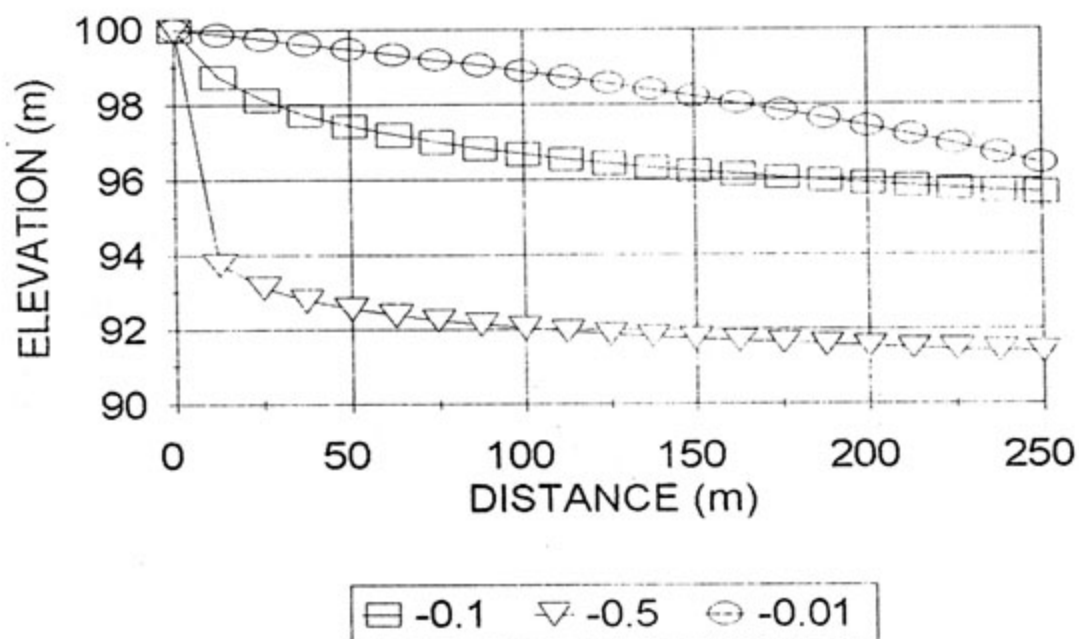
FIGURE 5.30 : PREDICTED BEACH PROFILES FOR VARIATION IN FRICTIONAL RESISTANCE (initial beach slope)
