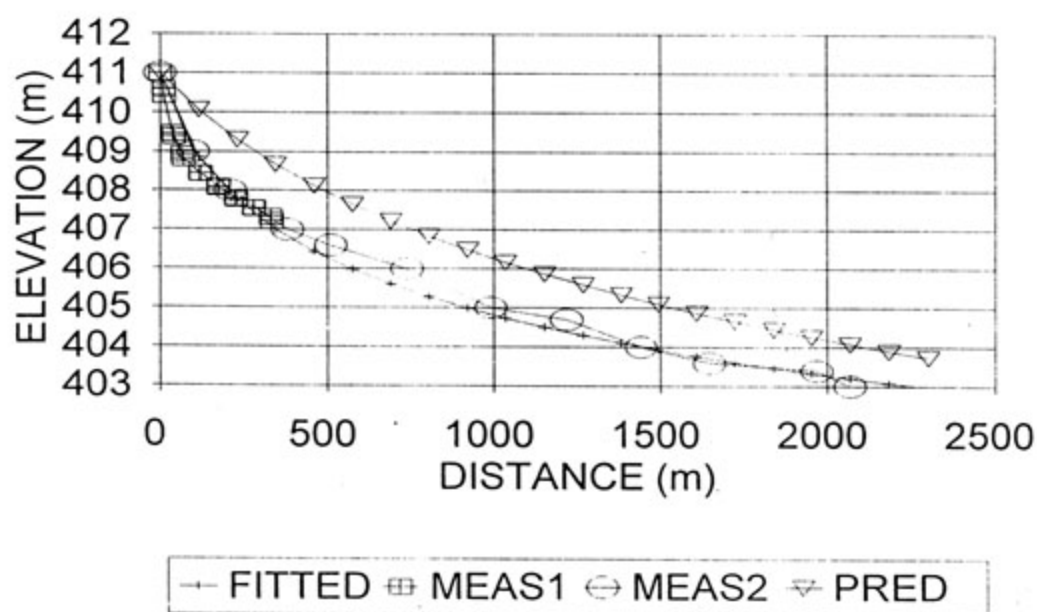
FIGURE 7.22 : MEASURED, CALIBRATED AND PREDICTED PROFILES
