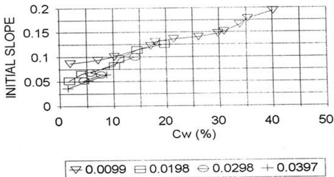
FIGURE 6.16 : CONCENTRATION VS INITIAL SLOPE FOR THE RANGE OF TS TESTS DOCUMENTED BY KÜPPER (1991)
