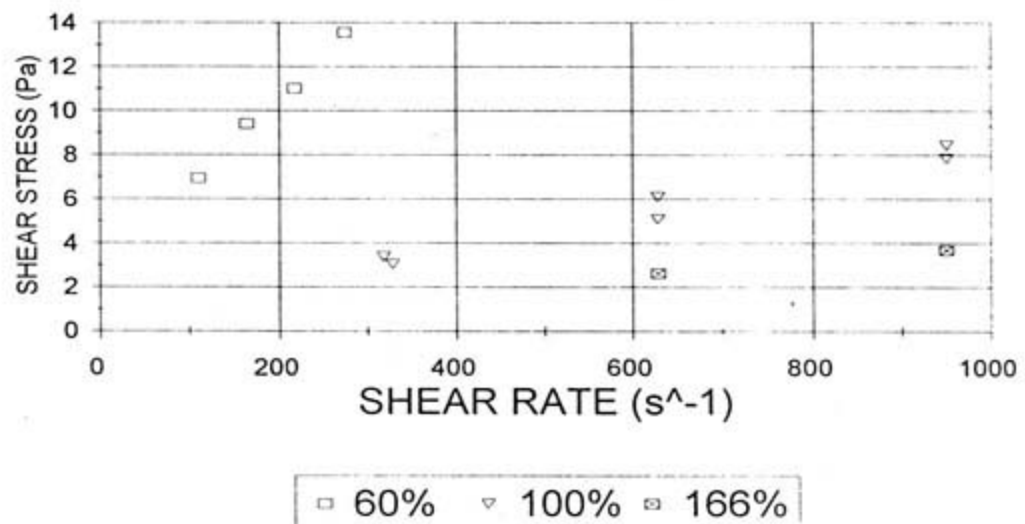
FIGURE 7.17 : COPPER TAILINGS RHEOGRAMS
