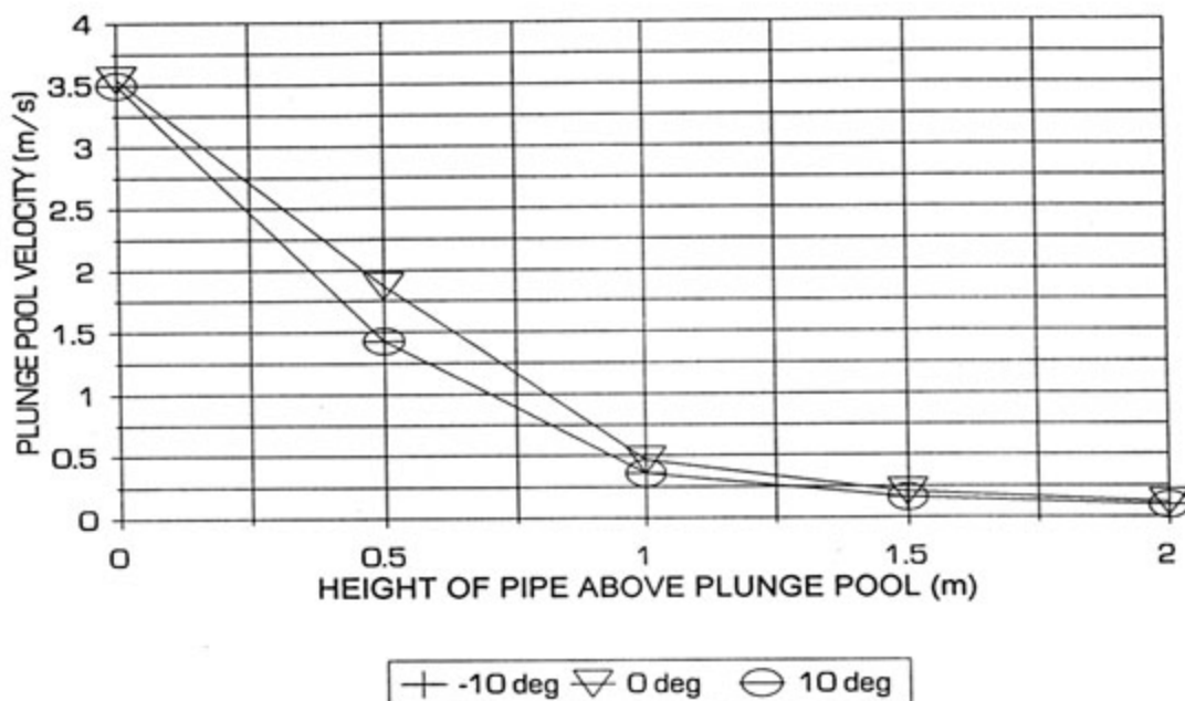
FIGURE 7.12 : PLUNGE POOL VELOCITY VERSUS PIPE HEIGHT ABOVE PLUNGE POOL FOR RÖSSING OLD BEACH
