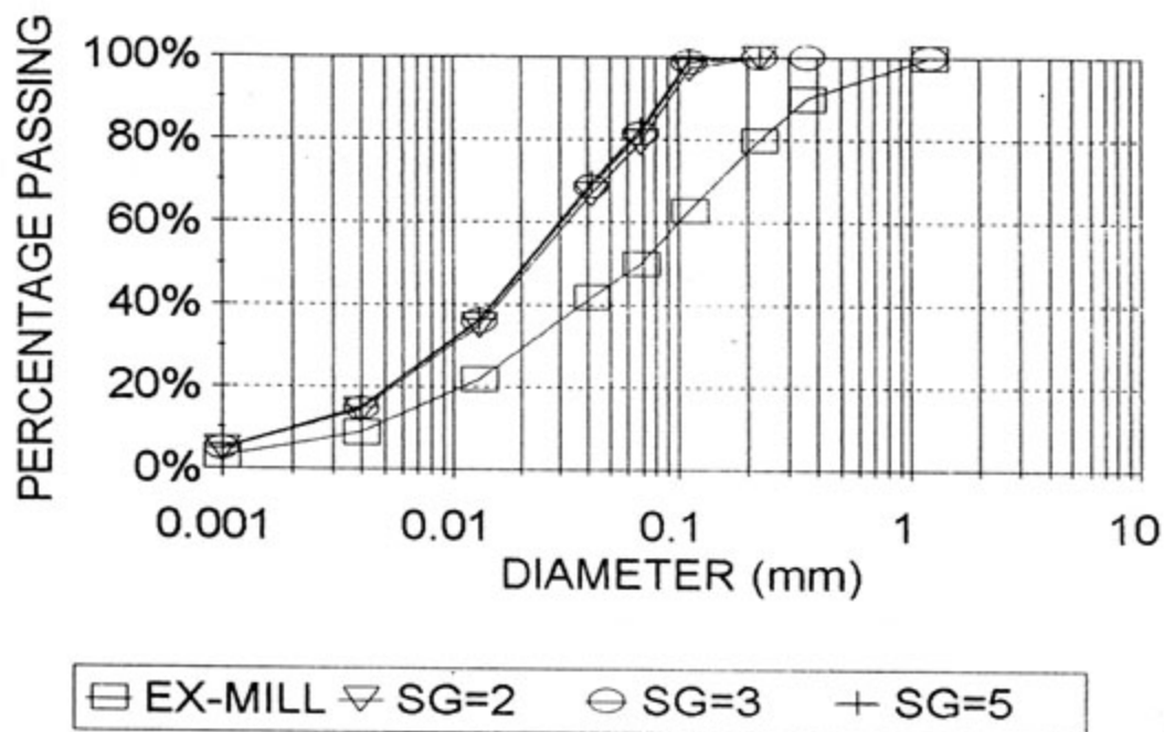
FIGURE 5.9 : PREDICTED PARTICLE SIZE DISTRIBUTIONS FOR VARIATIONS IN PARTICLE SPECIFIC GRAVITY - AT 225 m
