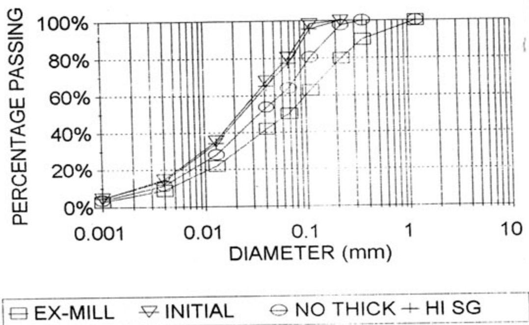
FIGURE 5.36 : PREDICTED PARTICLE SIZE DISTRIBUTION FOR VARIATION IN THICKENER OPERATION AND ORE TYPE - AT 125 m
