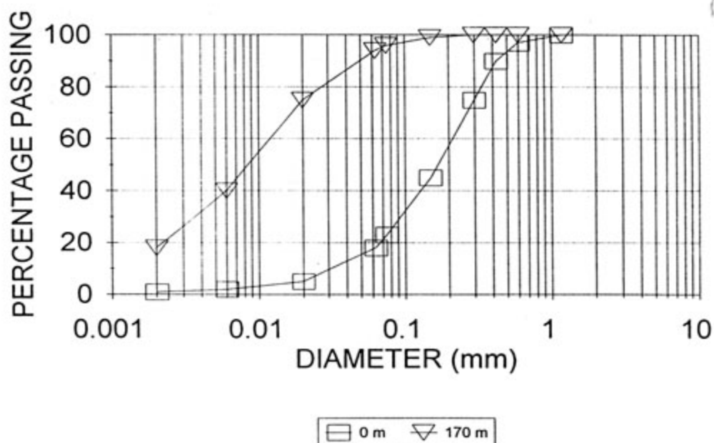
FIGURE 8.47: MEASURED PARTICLE SIZE DISTRIBUTIONS IN 1987 : COARSE GRIND
