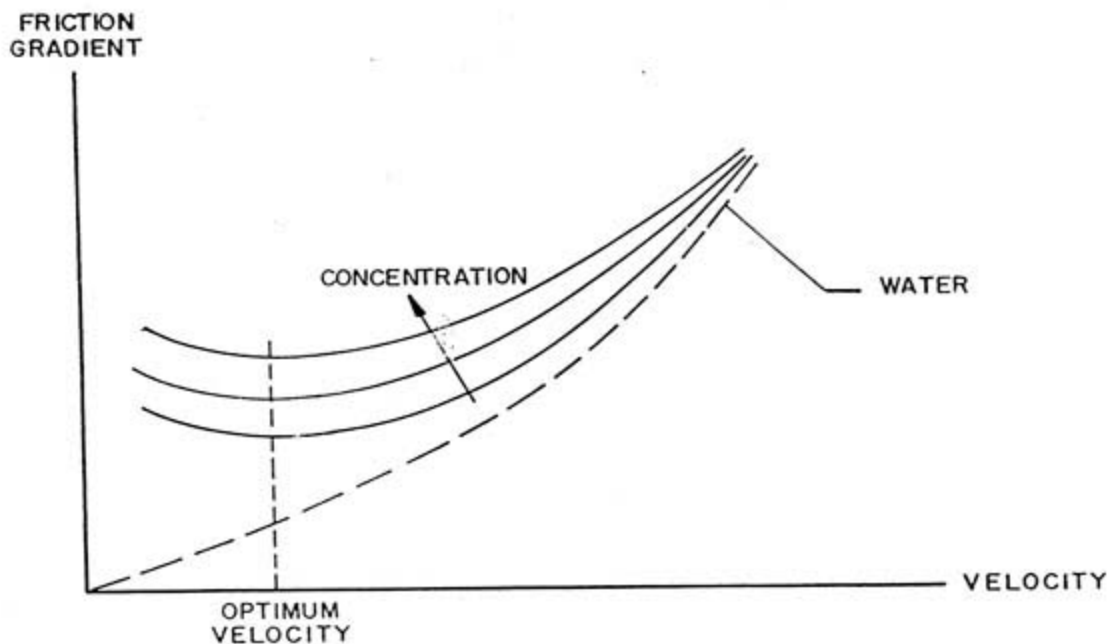
FIGURE 3.4 : INFLUENCE OF INCREASING CONCENTRATION AND VELOCITY ON THE FRICTIONAL RESISTANCE OF A TYPICAL TAILINGS SLURRY
