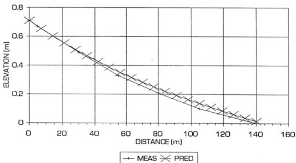
FIGURE 4.11 : THOMSON GOLD DATA - PREDICTED BEACH PROFILE
