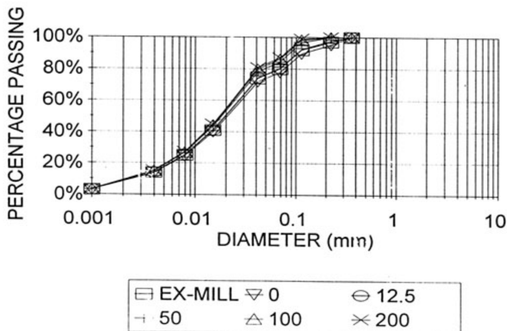
FIGURE 5.5 : PREDICTED PARTICLE SIZE DISTRIBUTIONS - FINE PRODUCT
