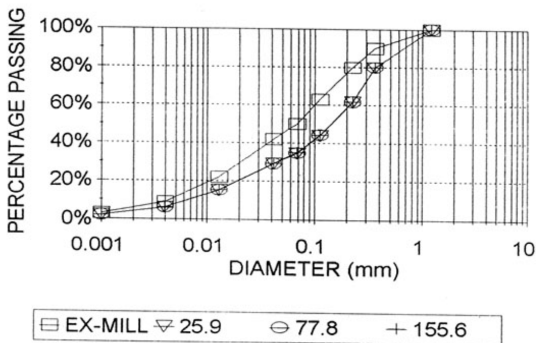
FIGURE 5.11 : PREDICTED PARTICLE SIZE DISTRIBUTION FOR VARIATIONS IN FLOW RATE - AT DISCHARGE
