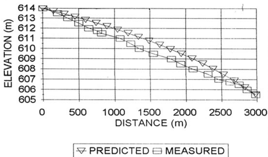
FIGURE 6.15 : PREDICTED BEACH PROFILE USING DATA FROM THE FLUME TEST FOR A FLOW RATE OF 0,44 l/s
