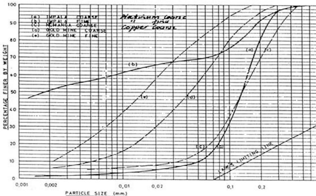
FIGURE 1.17 : TYPICAL TAILINGS PARTICLE SIZE DISTRIBUTIONS (After Jennings (1978))
