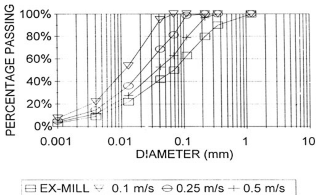
FIGURE 5.29 : PREDICTED PARTICLE SIZE DISTRIBUTION FOR VARIATION IN VELOCITY EX-PLUNGE POOL - AT 225 m
