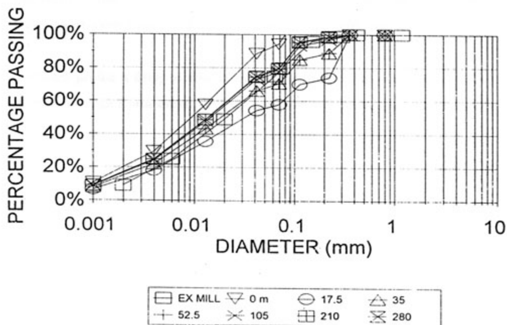
FIGURE 8.57 : PREDICTED PARTICLE SIZE DISTRIBUTIONS - FINER PRODUCT COMBINED SPIGOT FLOWS
