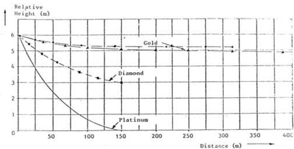
Figure 2.8 (a): Comparison of Typical Measured Beach Profiles
