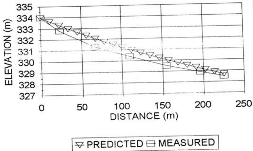
FIGURE 6.6 : MEASURED AND PREDICTED BEACH PROFILES FOR TEST 4 , SECTION 1 BASED ON FLUME DATA
