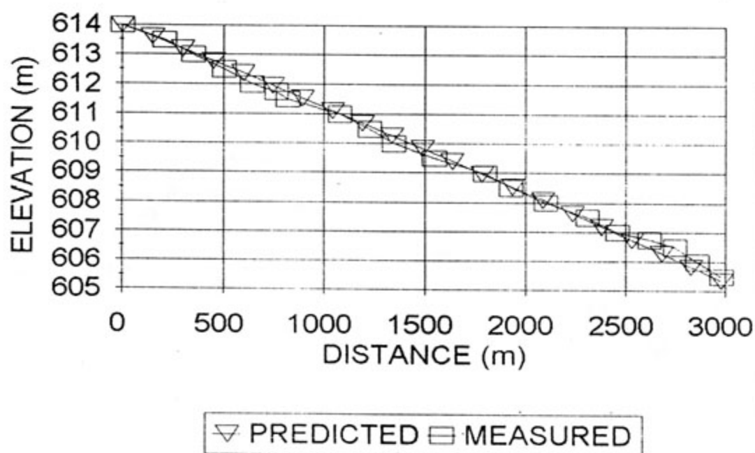
FIGURE 6.9 : MEASURED BEACH PROFILE ON THE TAILINGS DAM
