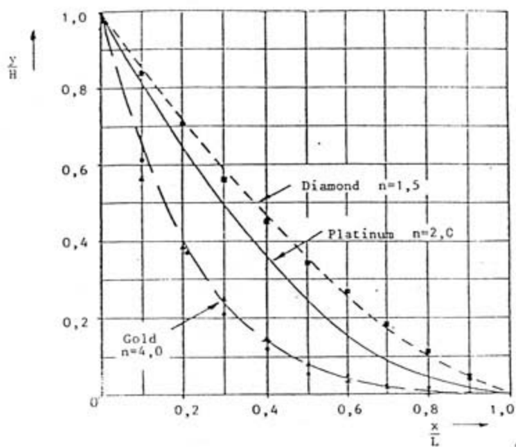
(b): Dimensionless Beach Profiles for the Various Types of Tailings
