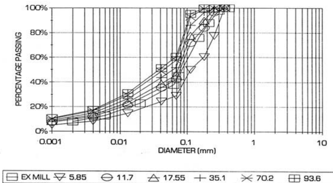
FIGURE 4.16 : BENTEL PLATINUM DATA - PREDICTED PARTICLE SIZE DISTRIBUTION
