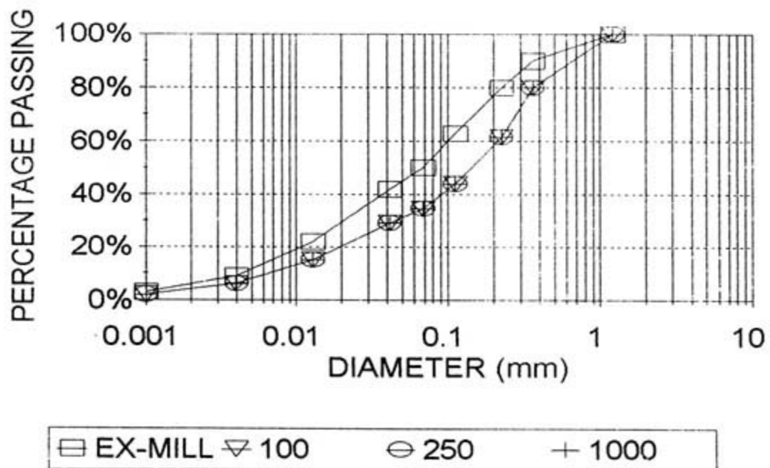
FIGURE 5.22 : PREDICTED PARTICLE SIZE DISTRIBUTIONS FOR VARIATIONS IN BEACH LENGTH - AT DISCHARGE
