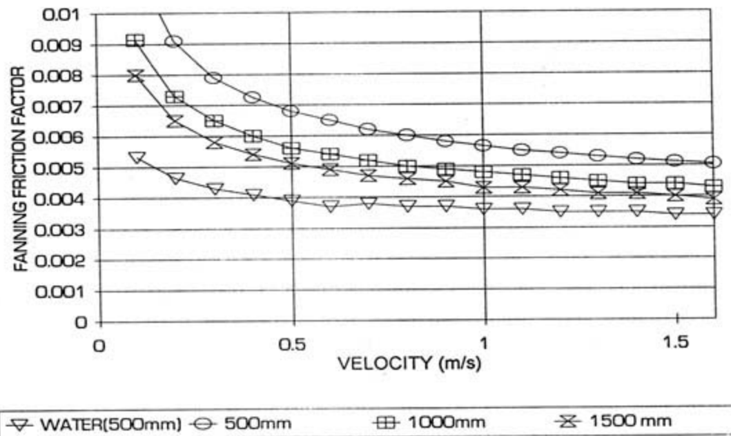
FIGURE 7.14 : FANNING FRICTION FACTORS
