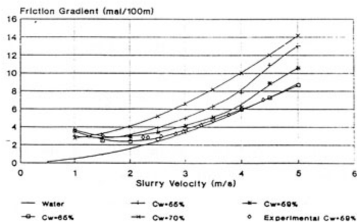
Figure 10 194mm Friction Gradients
