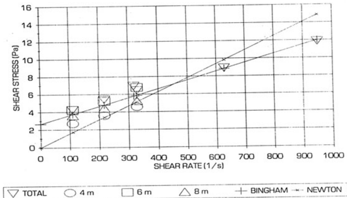
FIGURE 7.13 : RHEOGRAMS FOR THE BRAZILIAN GOLD TAILINGS
