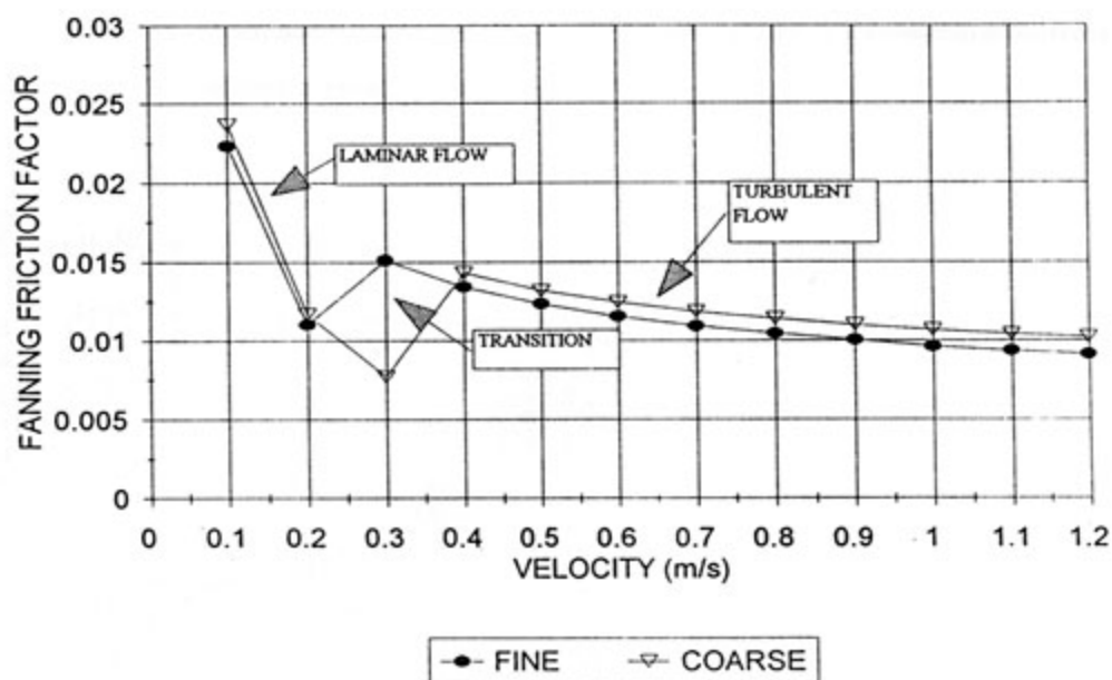
FIGURE 8.50 : FANNING FRICTION FACTORS FROM VERKERK RUNS
