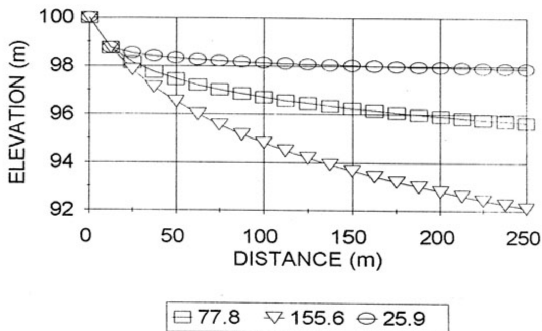
FIGURE 5.10 : PREDICTED BEACH PROFILES FOR VARIATIONS IN FLOW RATE
