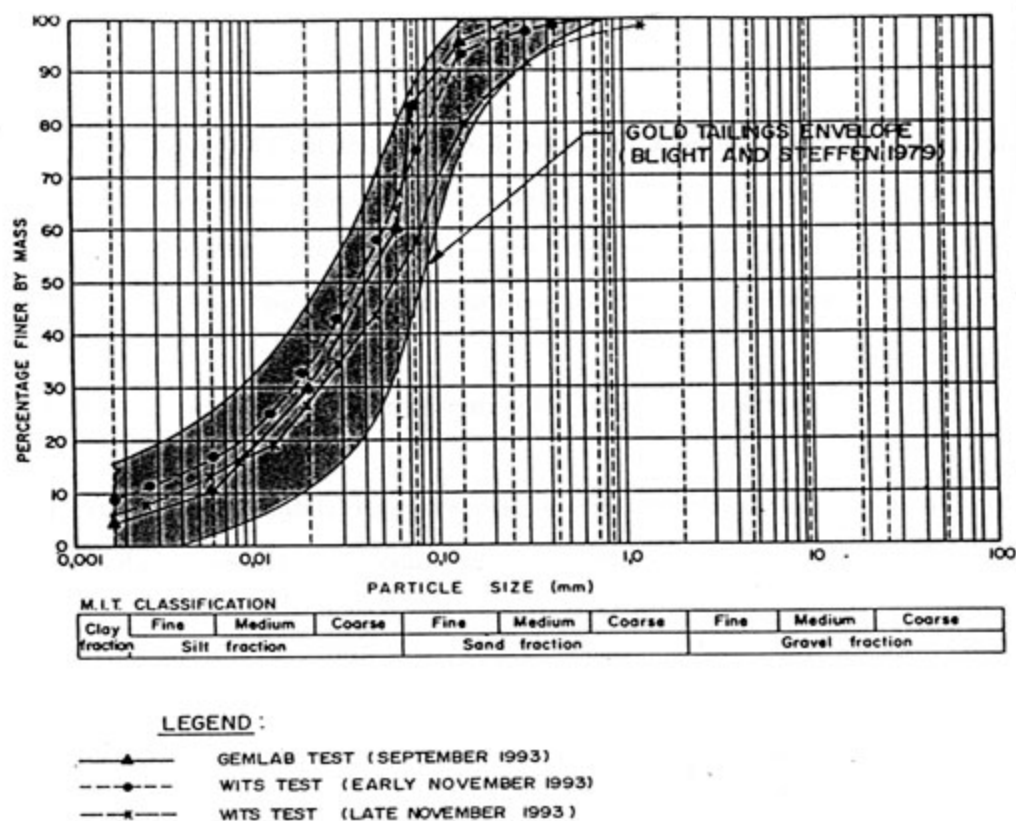
FIGURE 8.11 PARTICLE SIZE DISTRIBUTIONS OF THE COARSE AND FINE PRODUCTS
