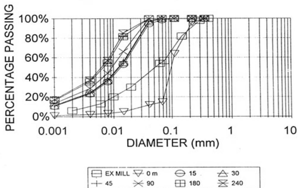
FIGURE 8.46: PREDICTED PARTICLE SIZE DISTRIBUTIONS - COARSER PRODUCT : POINT DISCHARGE
