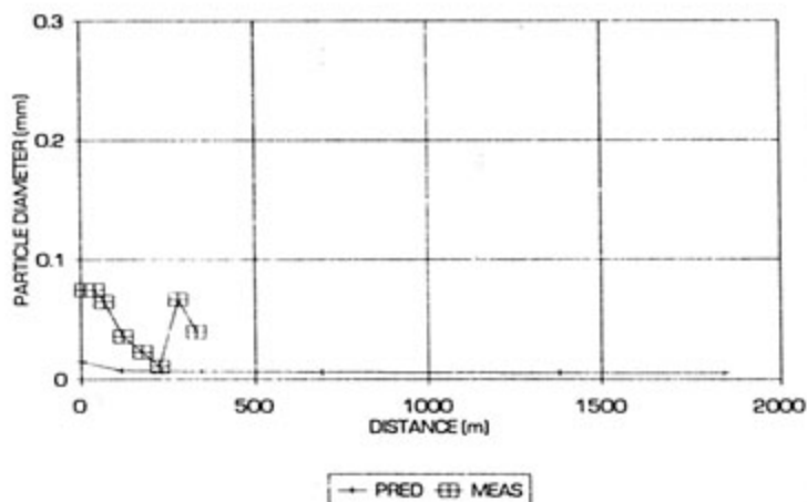
FIGURE 7.27 : COMPARISON OF d_{20} SIZE WITH DISTANCE
