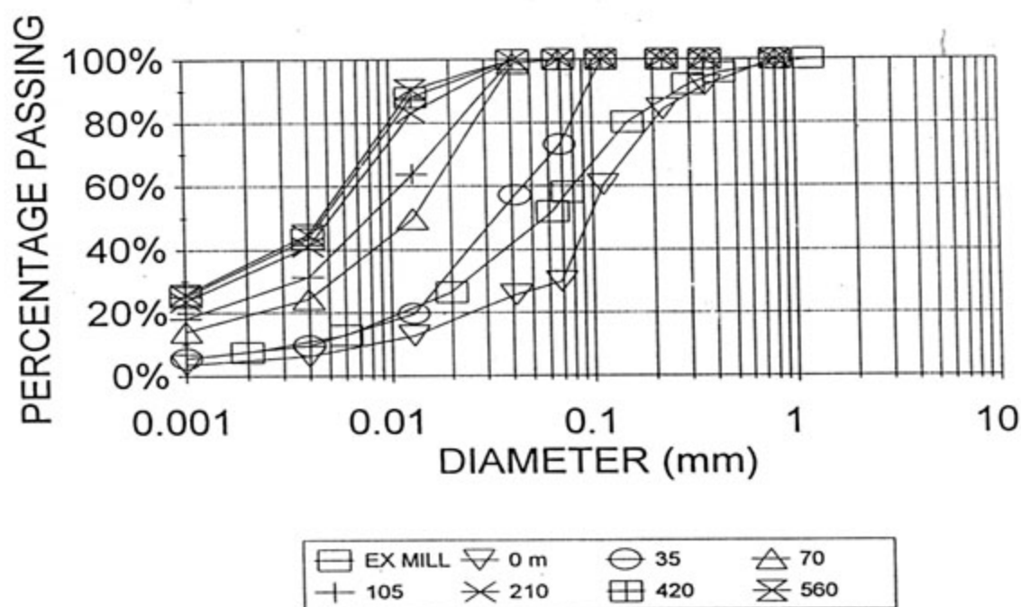
FIGURE 8.25 : 700 m BEACH, COARSE PRODUCT, DISCHARGE HEIGHT 0,2 m 1,75 t/m 3
