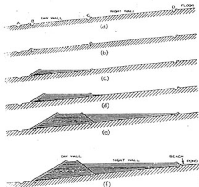
INITIAL STAGES IN THE BUILDING OF A SLUICE DAM
