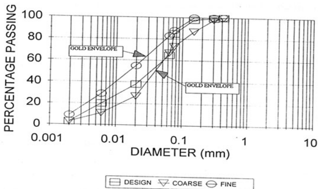
FIGURE 8.38 : DESIGN PARTICLE SIZE DISTRIBUTION OF PERING TAILINGS RELATIVE TO THE BLIGHT AND STEFFEN GOLD TAILINGS ENVELOPE (Blight and Steffen (1979))
