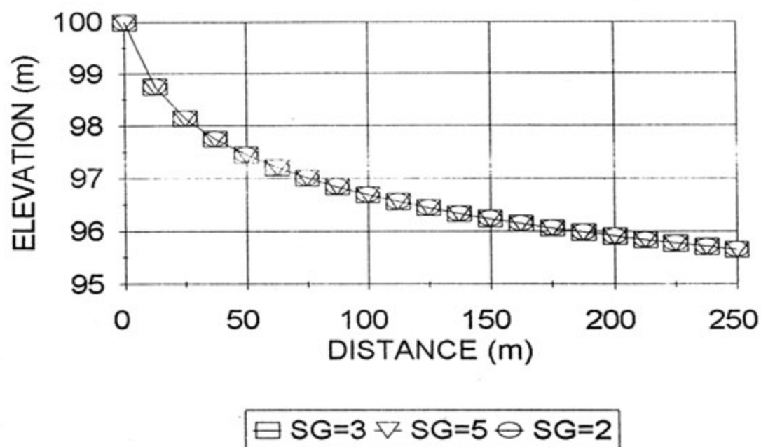
FIGURE 5.6 : PREDICTED BEACH PROFILES FOR VARIATIONS IN PARTICLE SPECIFIC GRAVITY
