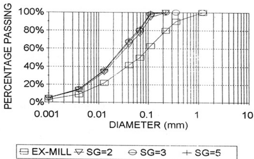
FIGURE 5.8 : PREDICTED PARTICLE SIZE DISTRIBUTIONS FOR VARIATIONS IN PARTICLE SPECIFIC GRAVITY - AT 125 m
