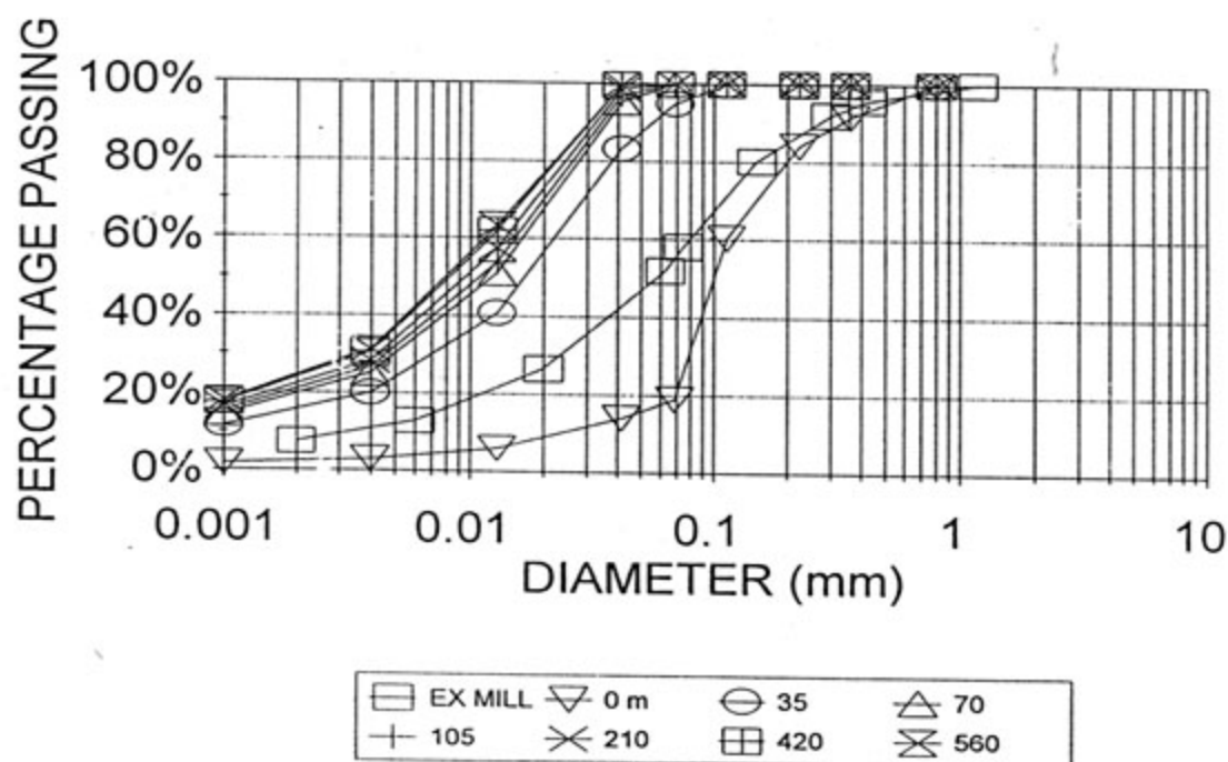
FIGURE 8.21 : 700 m BEACH, COARSE PRODUCT, DISCHARGE HEIGHT 0,2 m, DENSITY 1,45 t/m 3
