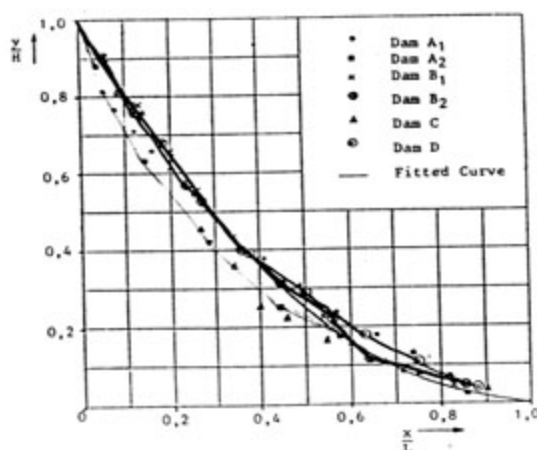
Figure 2.6: Measured Beach Profiles (Platinum)
