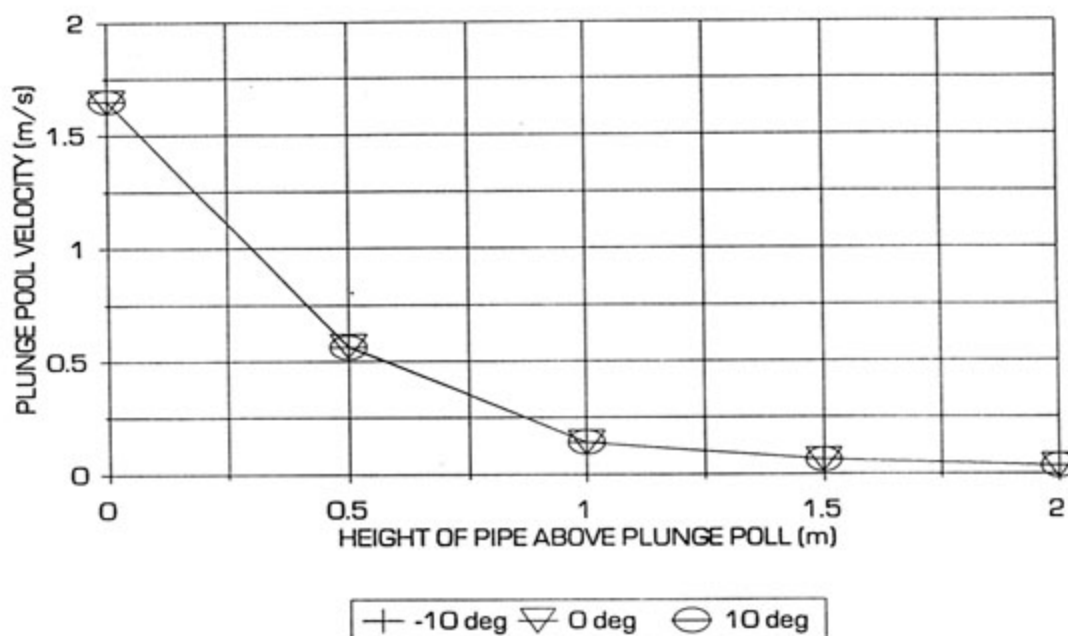
FIGURE 7.8 : VARIATION OF PLUNGE POOL VELOCITY WITH HEIGHT OF DISCHARGE PIPE
