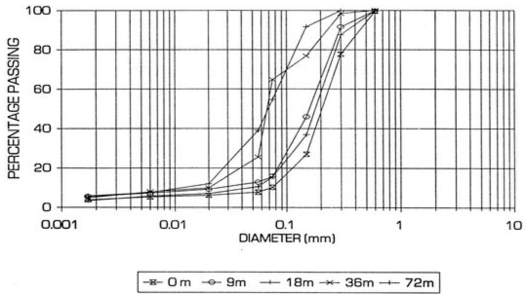
FIGURE 4.13 : BENTEL PLATINUM DATA - MEASURED PARTICLE SIZE DISTRIBUTIONS
