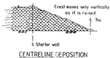
FIGURE 1.8 : UPSTREAM, DOWNSTREAM AND CENTRELINE METHODS OF TAILINGS DAM FORMATION (After ICOLD (1982))
