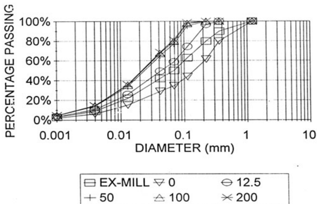
FIGURE 5.4 : PREDICTED PARTICLE SIZE DISTRIBUTIONS - MEDIUM PRODUCT
