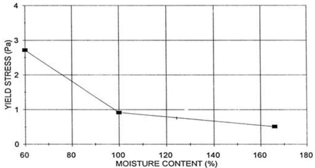
FIGURE 7.19 : YIELD STRESS vs MOISTURE CONTENT
