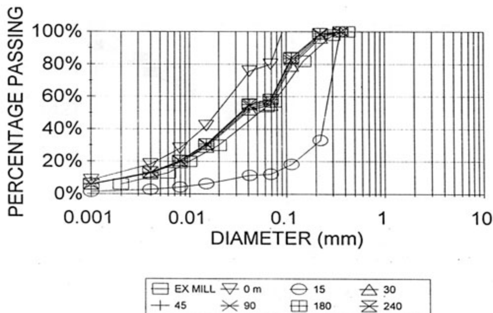
FIGURE 8.55: PREDICTED PARTICLE SIZE DISTRIBUTION FROM A SINGLE OPENING
