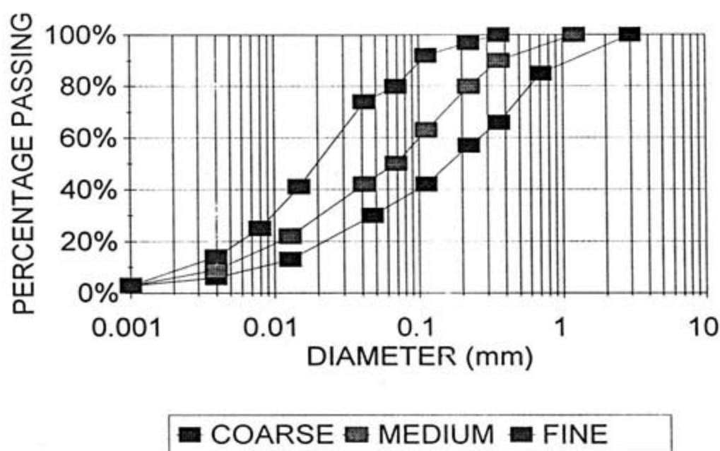
FIGURE 5.1 : COARSE , MEDIUM AND FINE PRODUCTS USED IN SENSITIVITY ANALYSIS
