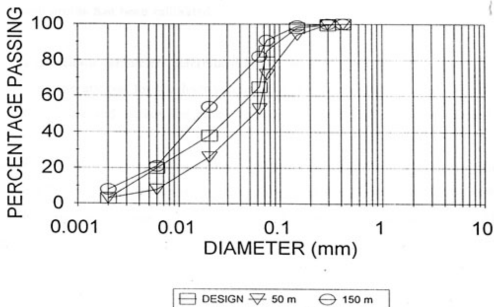
FIGURE 8.49: MEASURED PARTICLE SIZE DISTRIBUTIONS IN 1987 - FINE PRODUCT : POINT DISCHARGE
