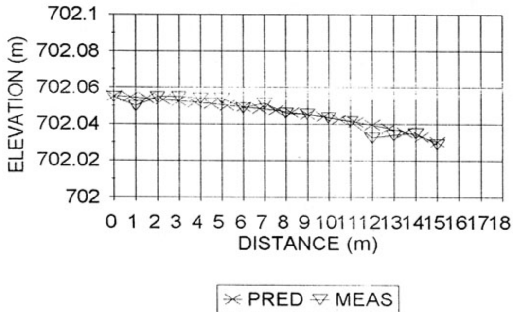
FIGURE 6.12 : CALIBRATED BEACH PROFILE FOR FLUME TEST AT FLOW OF 2,6 l/s
