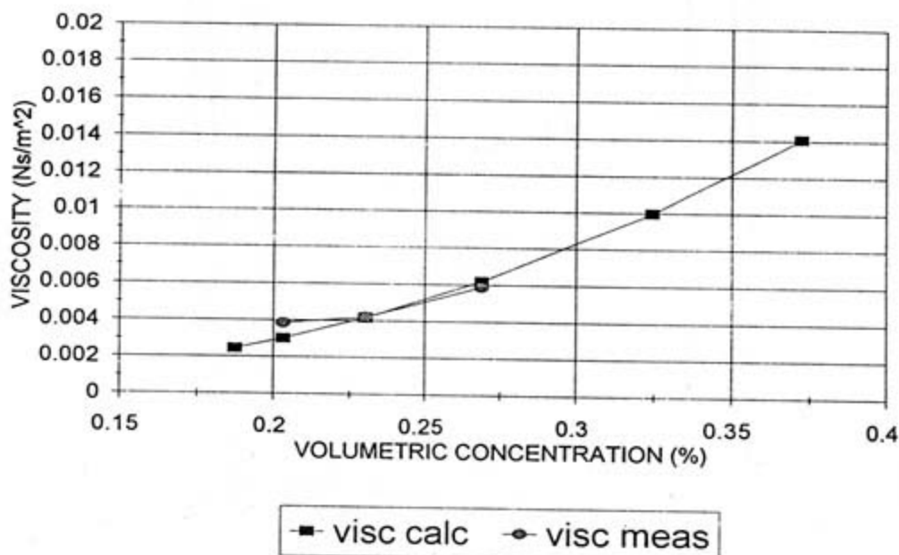
FIGURE 8.41 : CONCENTRATION vs VISCOSITY
