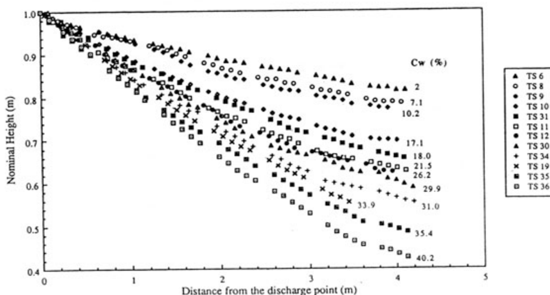
FIGURE 6.1 : PROFILES OF TS TESTS WITH Q_t = 5 l/min AND VARIOUS C_w (After Küpper (1991))
