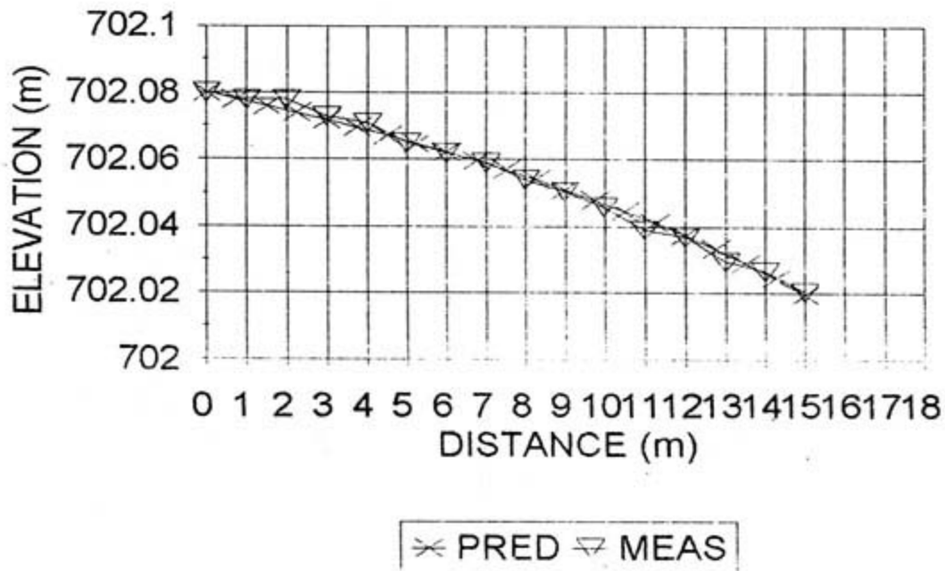
FIGURE 6.13 : CALIBRATED BEACH PROFILE FOR FLUME TEST AT FLOW OF 0,44 l/s
