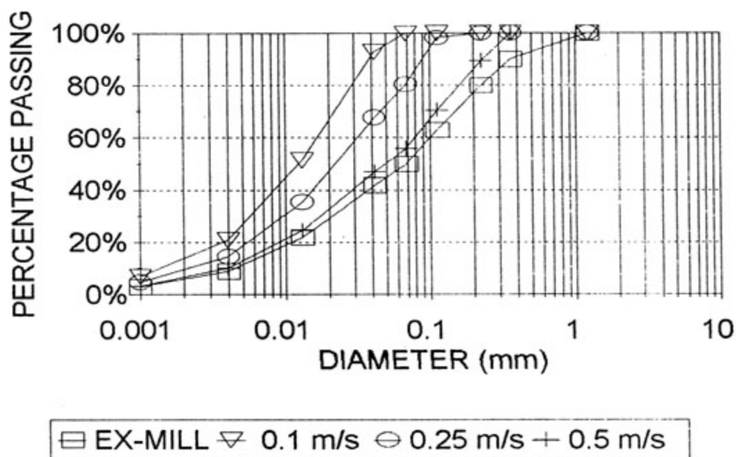
FIGURE 5.28 : PREDICTED PARTICLE SIZE DISTRIBUTIONS FOR VARIATION IN VELOCITY EX-PLUNGE POOL - AT 125 m
