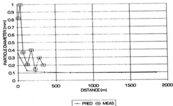
FIGURE 7.25 : COMPARISON OF d_{90} SIZE WITH DISTANCE
