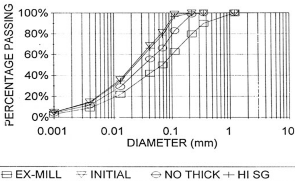
FIGURE 5.37 : PREDICTED PARTICLE SIZE DISTRIBUTION FOR VARIATION IN THICKENER OPERATION AND ORE TYPE - AT 225 m
