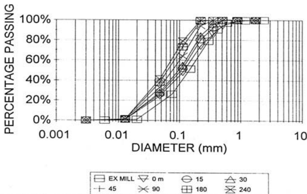
FIGURE 7.32 : PREDICTED PARTICLE SIZE DISTRIBUTIONS DOWN THE BEACH BASED ON CALIBRATED PARAMETERS
