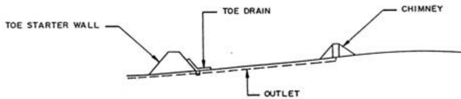
(a) INITIAL CONSTRUCTION
