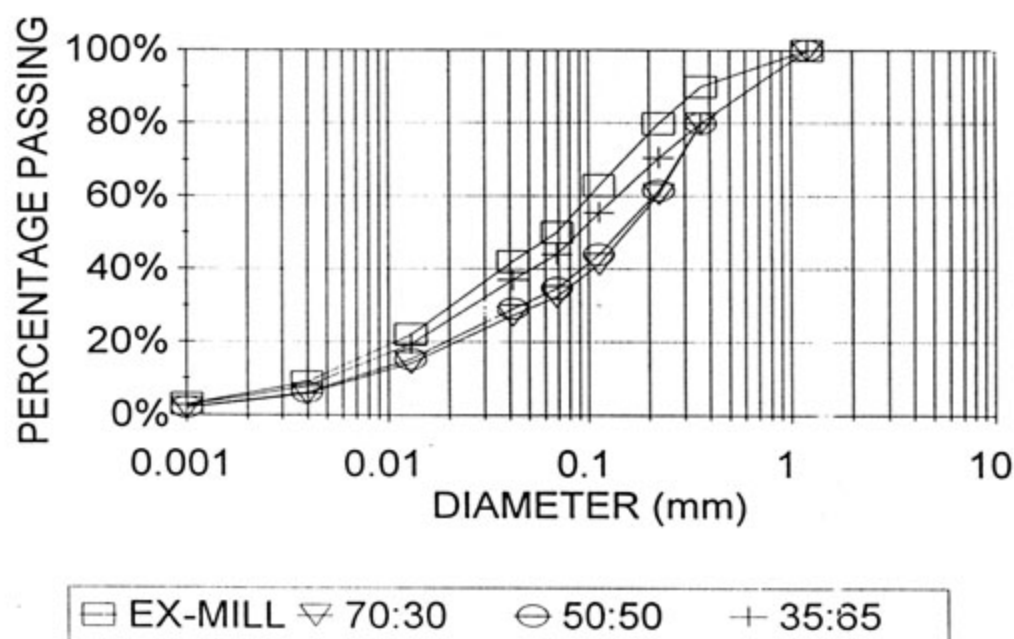
FIGURE 5.17 : PREDICTED PARTICLE SIZE DISTRIBUTIONS FOR VARIATIONS IN WATER:SOLIDS RATIO - AT DISCHARGE
