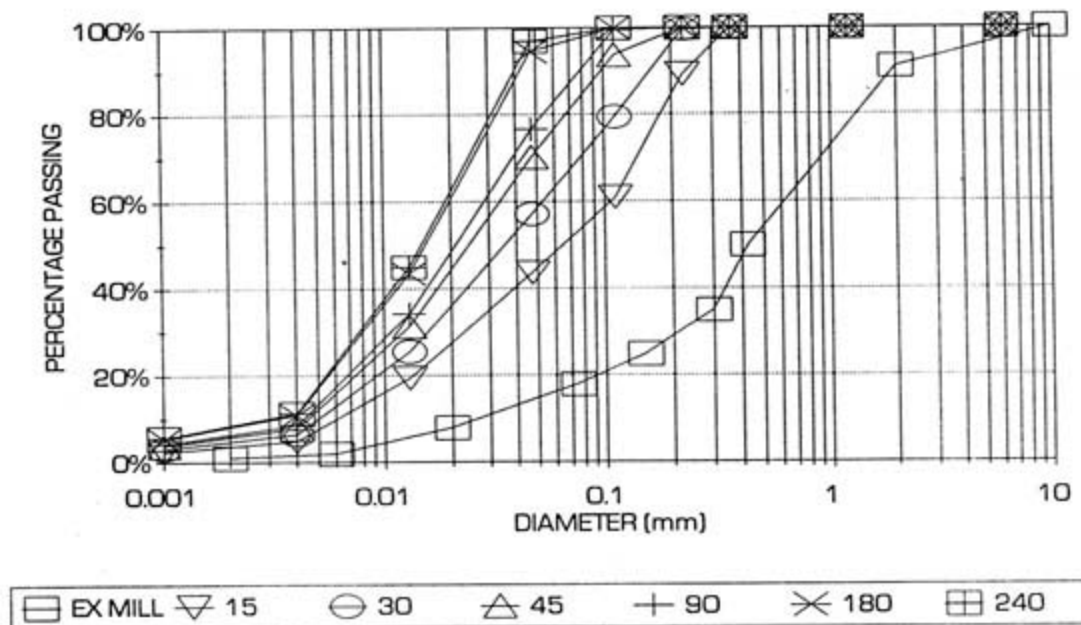
FIGURE 7.7 : PREDICTED PARTICLE SIZE DISTRIBUTIONS
