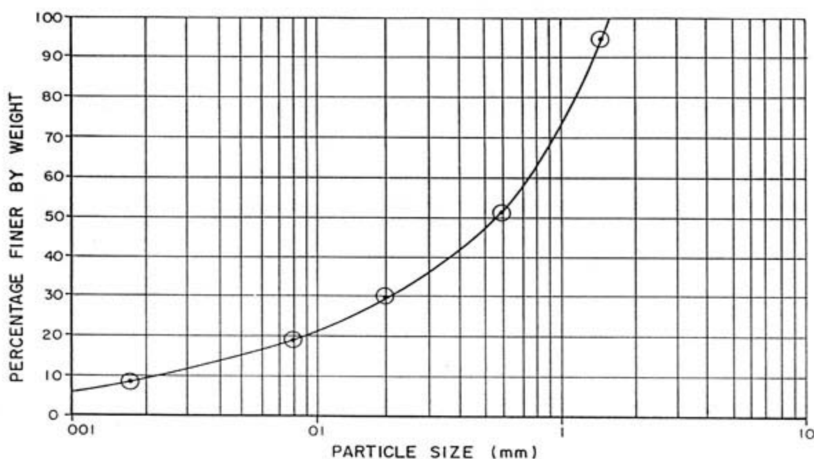
FIGURE 1.14 : PARTICLE SIZE DISTRIBUTION FOR SOUTH AFRICAN GOLD TAILINGS DURING THE 1950's (After National Building Research Institute (1959))
