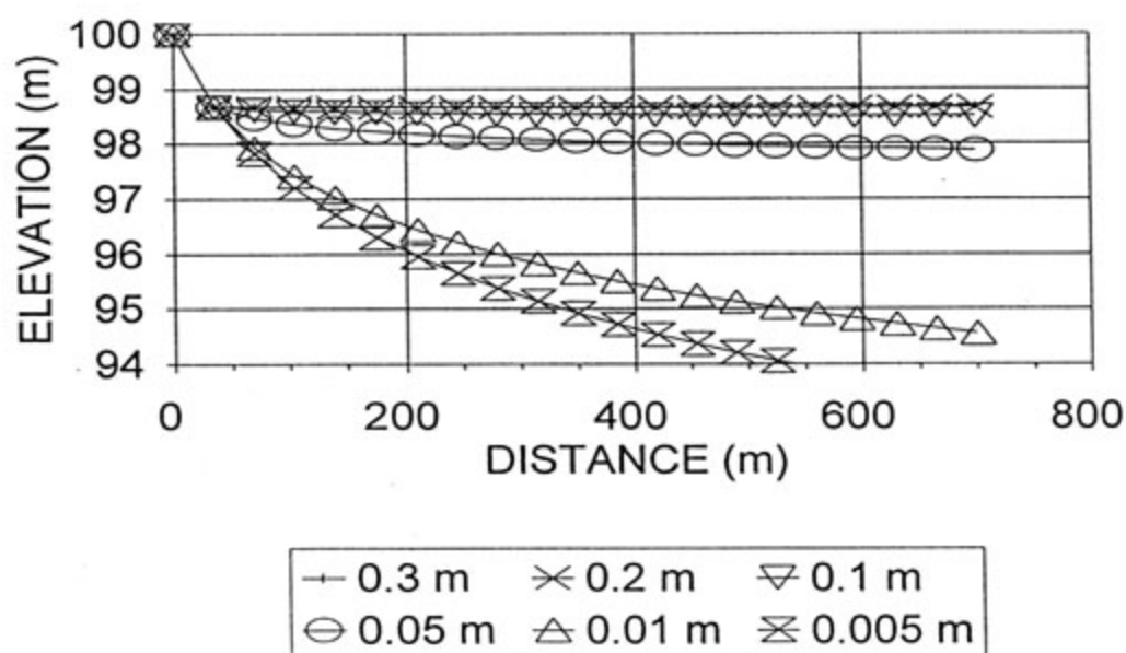
FIGURE 8.20 : 700 m BEACH, FINE PRODUCT, DENSITY 1,75 t/m 3
