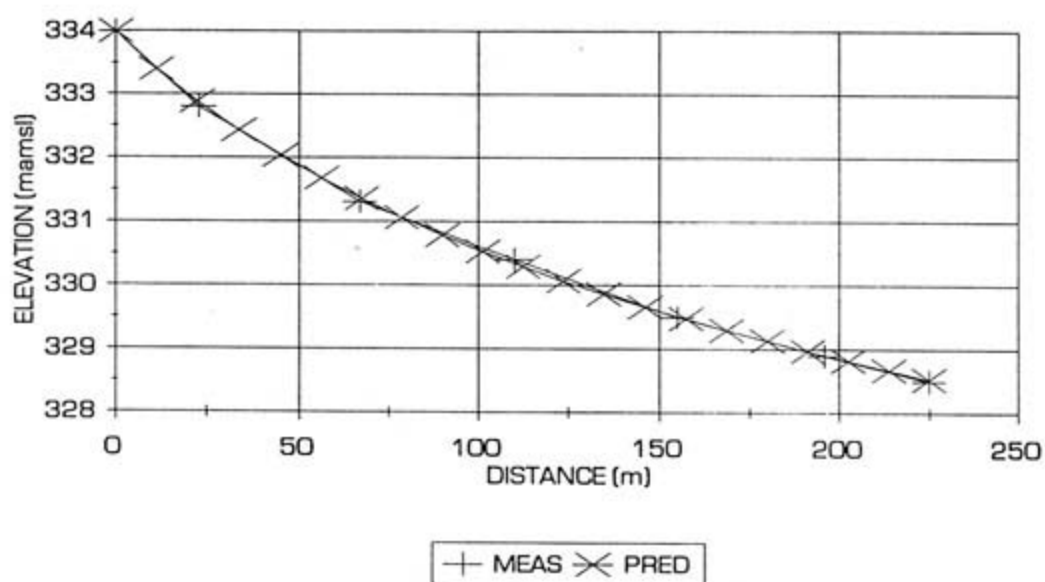
FIGURE 4.4 : KÜPPER:TEST 4 SECTION 1 - PREDICTED BEACH PROFILE
