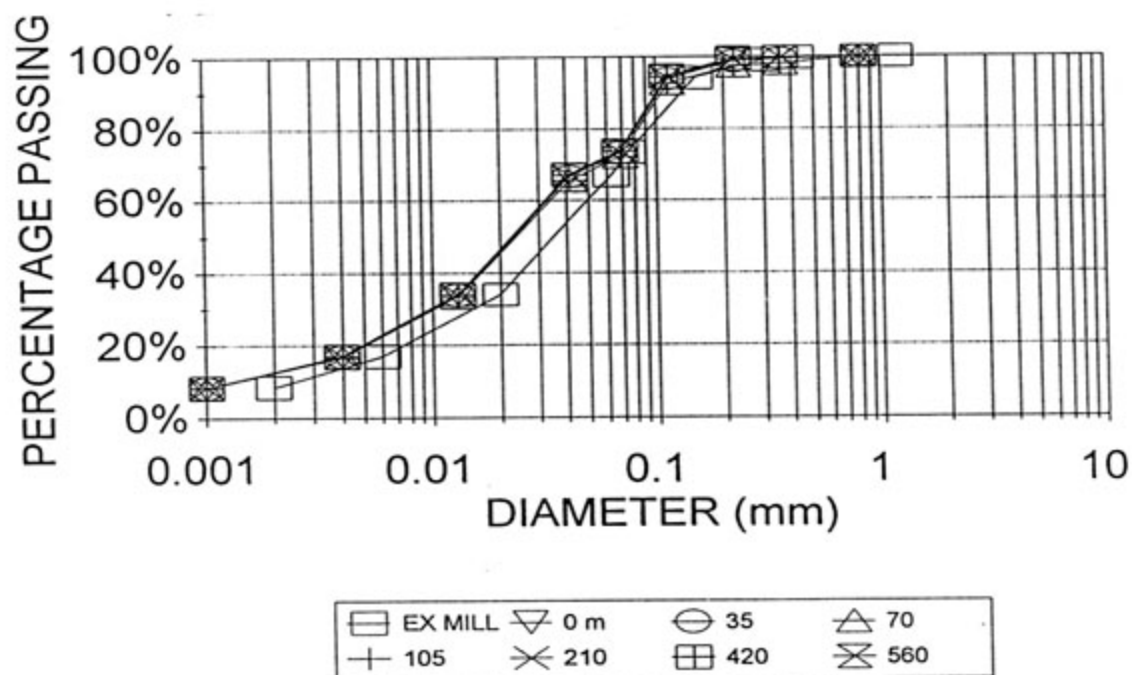
FIGURE 8.24 : 700 m BEACH, FINE PRODUCT, DISCHARGE HEIGHT 0,01 m, DENSITY 1,45 t/m 3
