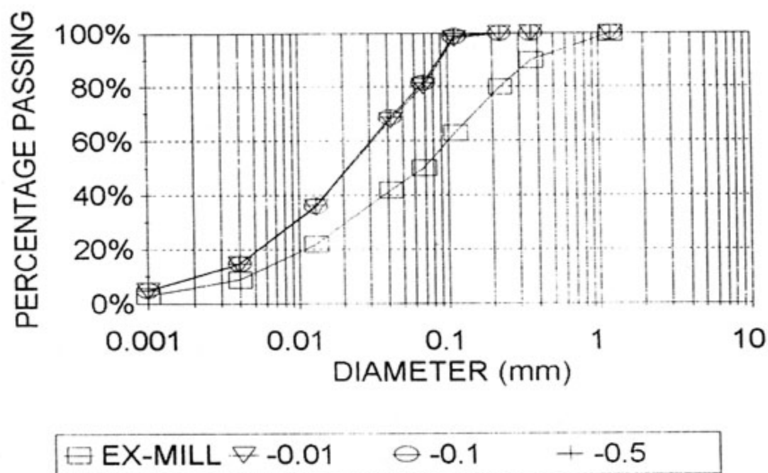
FIGURE 5.33 : PREDICTED PARTICLE SIZE DISTRIBUTION FOR VARIATION IN FRICTIONAL RESISTANCE (initial beach slope) - AT 225 m
