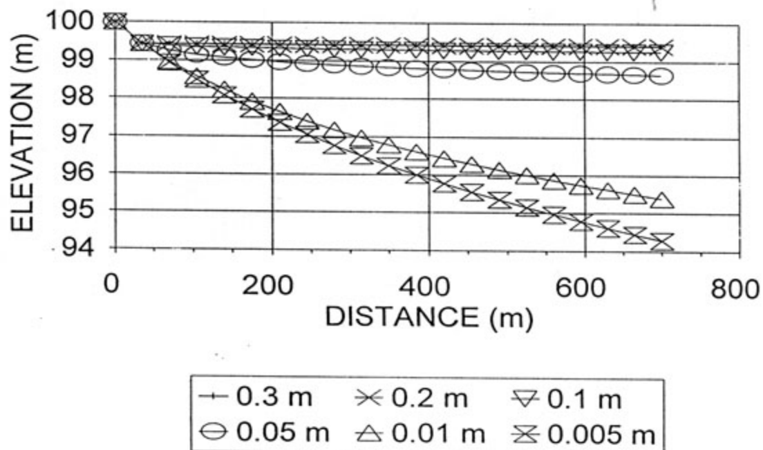
FIGURE 8.19 : 700 m BEACH, FINE PRODUCT, DENSITY 1,45 t/m 3
