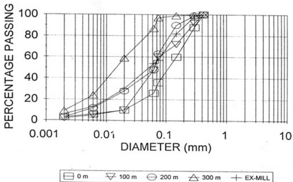
FIGURE 8.53 : MEASURED PARTICLE SIZE DISTRIBUTIONS
