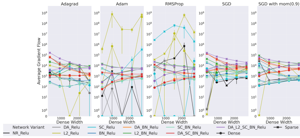
Figure A.8: Gradient Flow in CIFAR-100 using \|g\|_2 , with high learning rate (0.1)
