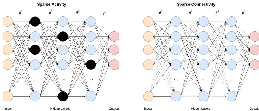
Figure 2.6: Sparse Activity (left) and Sparse Connectivity (right). In sparse activity, we have sparse activations (left), while in sparse connectivity, we have sparse weights (right).
