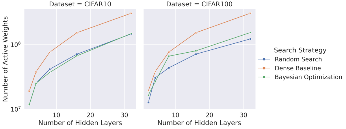
Figure 4.5: Number of Active Weights in SNAS MLPs. We compare the number of active weights in the best performing learned MLPs to their dense counterparts. We see that SNAS consistently finds much smaller architectures, especially for deeper networks.
