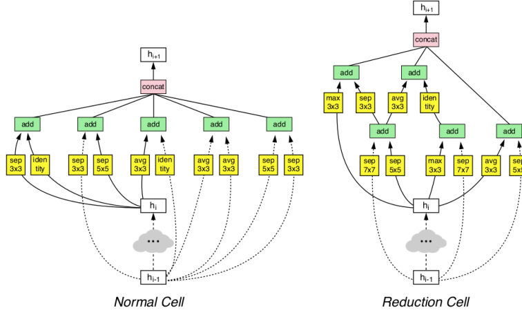
Figure 2.9: Best NAS Cells Learned by NASNet [Zoph et al., 2018] . We show the best performing convolutional cells, that were learned by NASNet-a on CIFAR-10.
