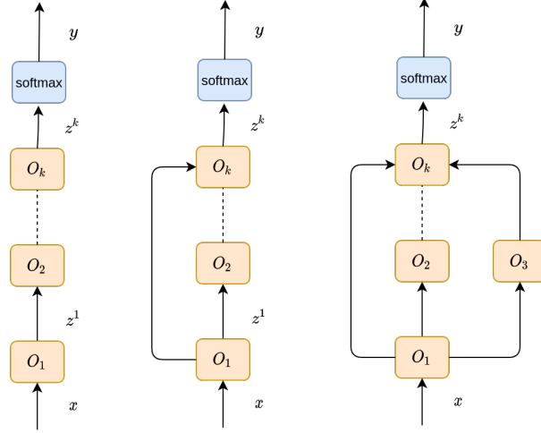
Figure 2.8: An Illustration of the Different Kinds of NAS Chain-structured Search Spaces. We show a simple chain only dependent on its parent node (left), a chain with skip connections (middle), and a more complex chain with branching and skip connections (right).
