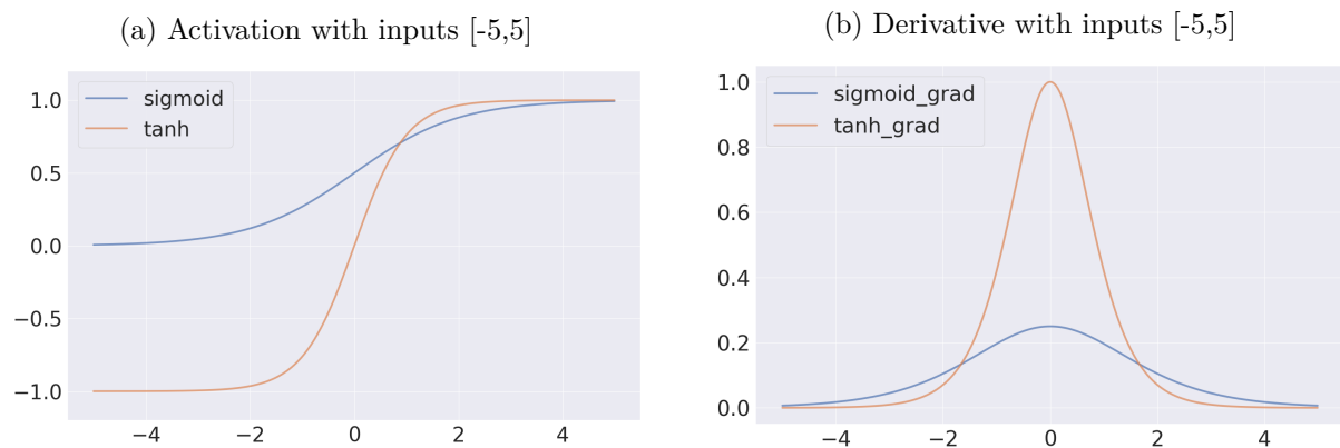
Figure 2.3: Plot of Sigmoid and Tanh Activation Functions. We plot the Sigmoid and tanh activation functions and their derivatives using an input range of [-5,5] .
