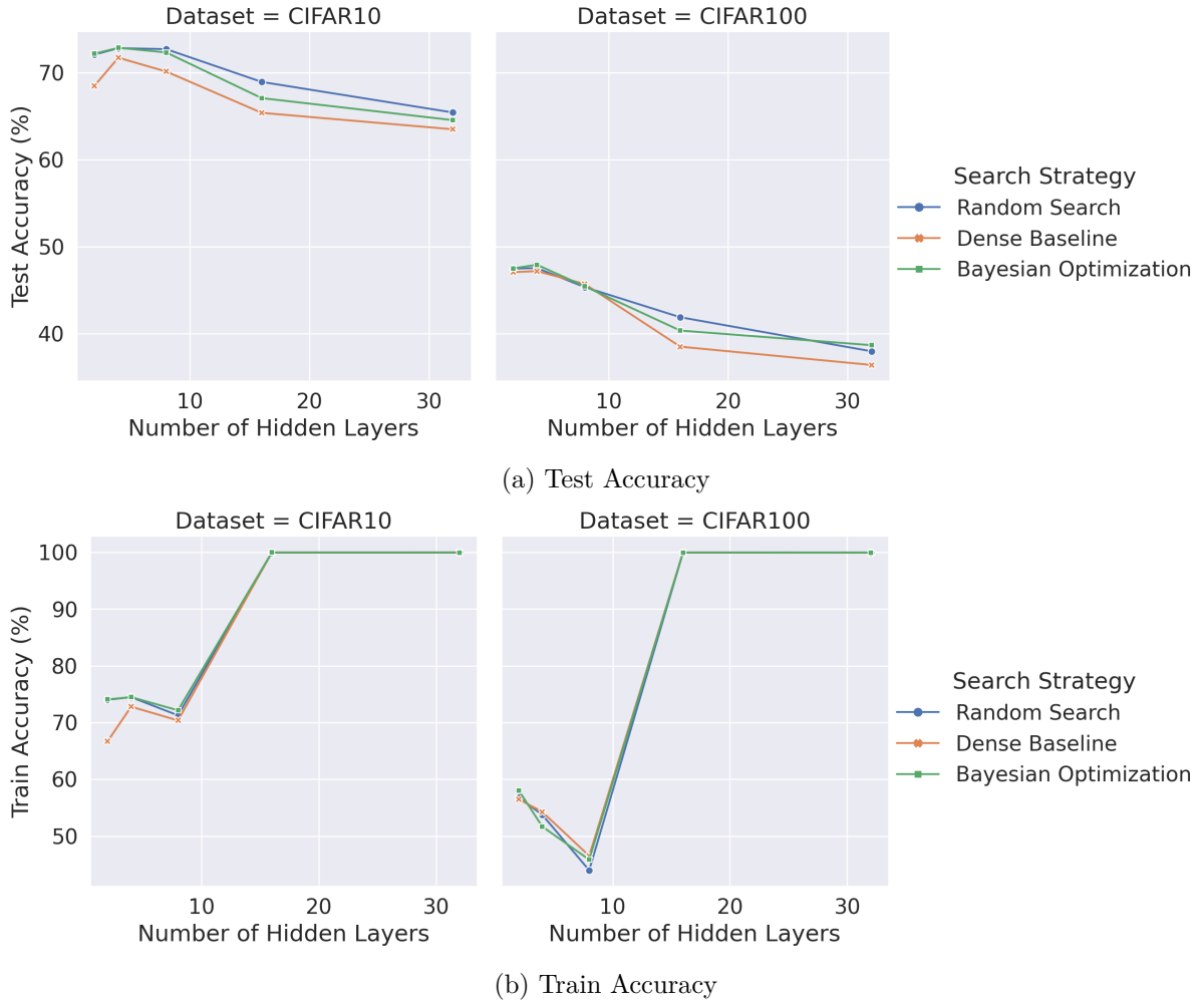
Figure 4.4: Test and Train Accuracy of SNAS MLPs Across Various Depths. We show the test and train accuracy of the best MLPs learned at different depths, compared to the dense baselines. We see that across all depths, SNAS consistently finds better performing MLP architectures than the dense baselines.
