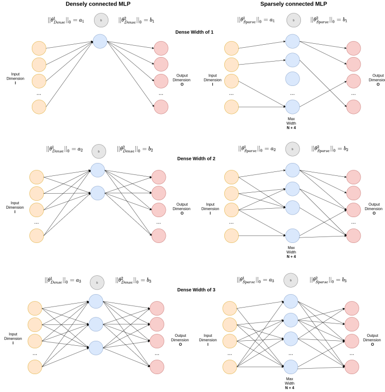
Figure A.2: Fairly Comparing Sparse and Dense Networks at Different Widths. We show how we ensure that sparse and dense networks have the same parameter count, at different widths.
