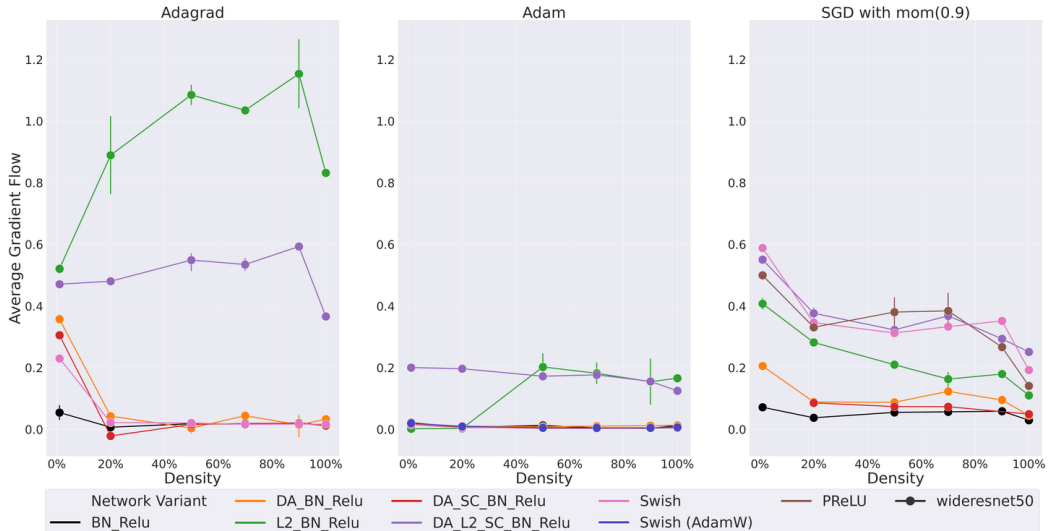
Figure A.19: Wide ResNet-50 Gradient Flow on CIFAR-100. We illustrate the gradient flow of Wide ResNet-50 on CIFAR-100, with the density ranging from 1% to 100%. The accuracy results can be found in Figure 3.5.
