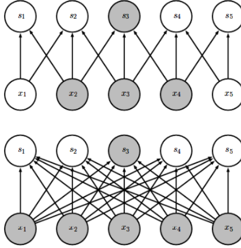
Figure 2.2: Sparse Connectivity in CNNs [Goodfellow et al., 2016]. We show sparse connectivity in convolutional layers of CNNs (top), compared to dense connectivity found in dense layers (below).
