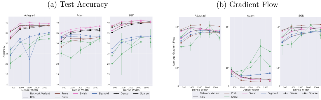
Figure 3.4: Effect of Activation Functions on Accuracy and Gradient Flow on CIFAR-100, With a Low Learning Rate (0.001). We see that Swish is the most promising activation function across most optimizers. The results across all optimizers and learning rates are shown in Figure A.15 and A.17.
