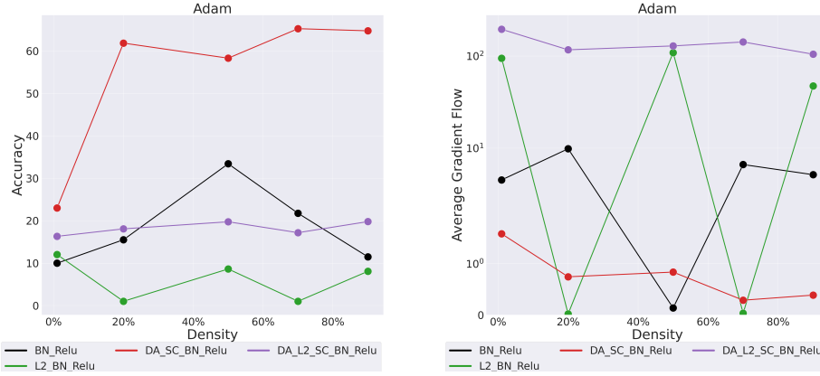
Figure 3.6: Accuracy and Gradient Flow for Magnitude Pruning. We see that similarly to randomly pruned networks, magnitude pruned networks trained with Adam and L2 lead to high EGF and poor performance.
