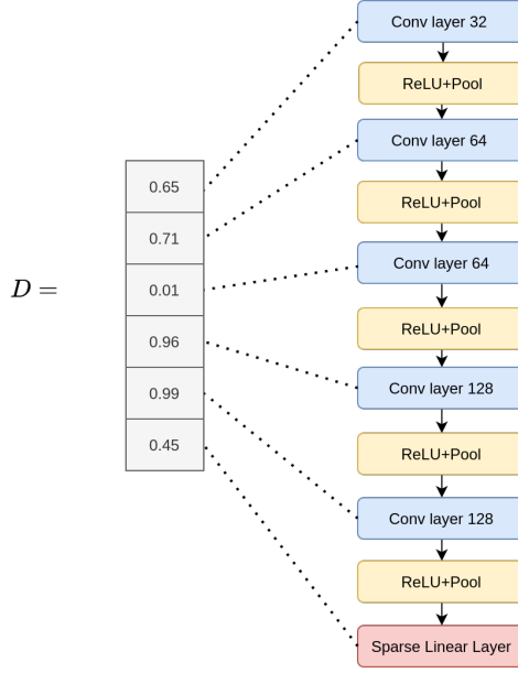
Figure 4.3: CNN Sparse Search Space. We show how we can use an existing CNN architecture and learn the densities for each convolutional and linear layer. D represents our learned density vector, where d_i is the density of weight layer i (convolutional or linear layer).
