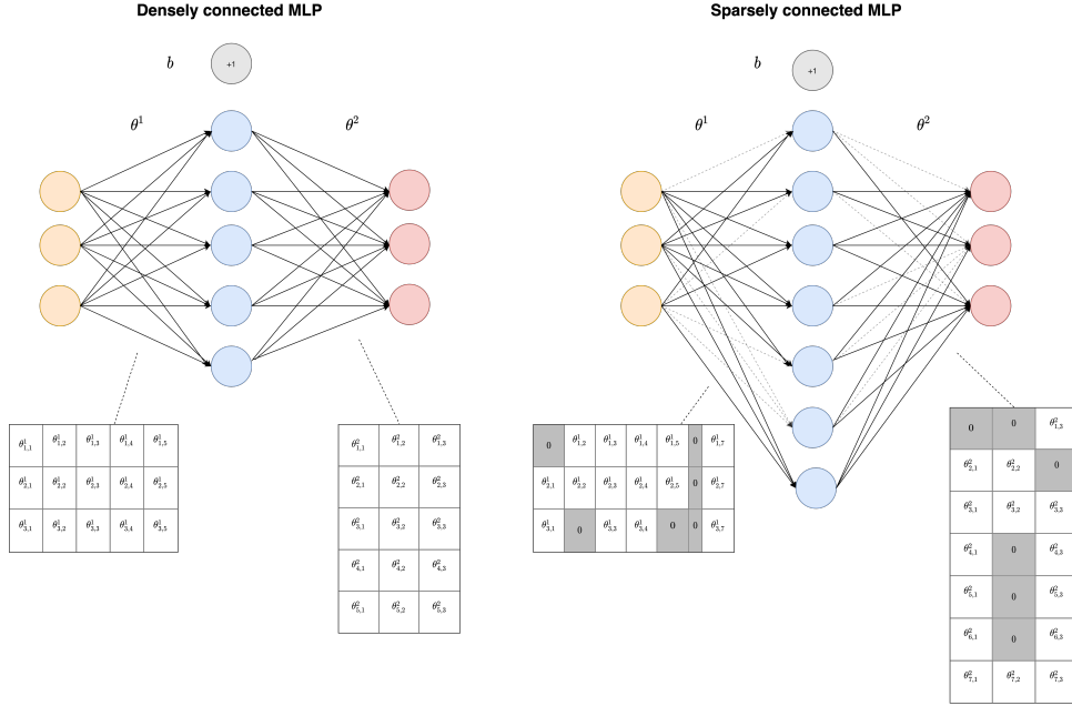
Figure A.1: Fair Comparison of Sparse and Dense Networks. We fairly compare sparse and dense networks, by ensuring they have the same number of connections per layer and turning off the bias unit.
