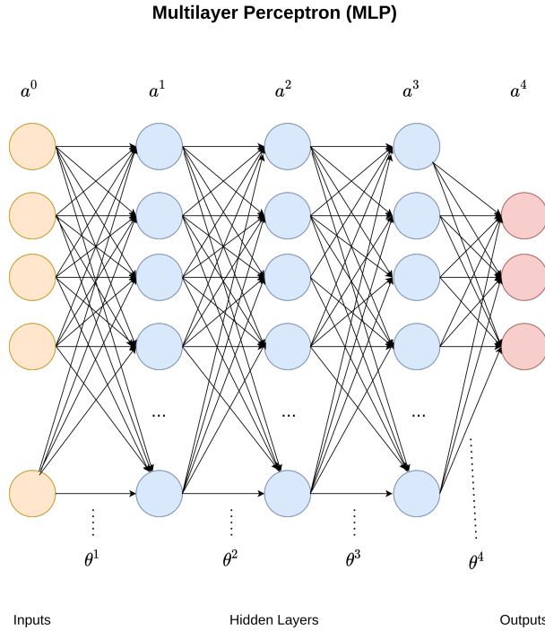
Figure 2.1: An Illustration of an MLP. We provide an illustration of an MLP showing input, hidden and output layers. Bias nodes are not included in the figure.
