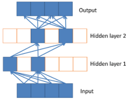
Figure 2.4: Sparse Propagation of Activations and Gradients of ReLU [Glorot et al., 2011]. ReLU’s sparse formulation results in sparse activations, where some activations are inactive (shown in white).
