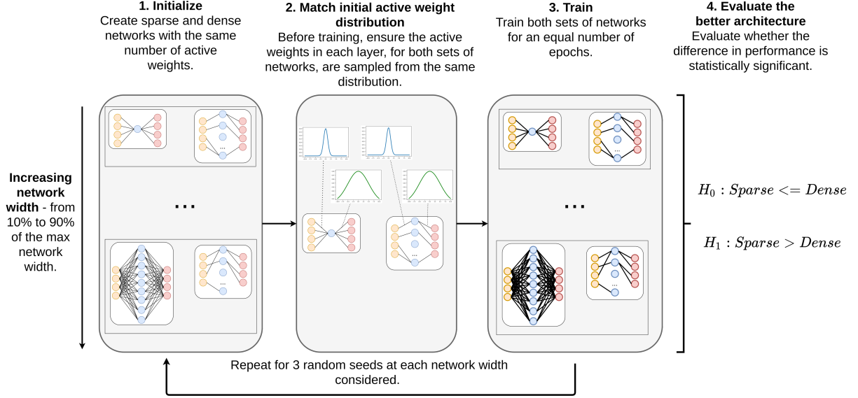
Figure 3.1: Same Capacity Sparse vs Dense Comparison (SC-SDC) . SC-SDC is a simple framework that fairly compares sparse and dense networks. This is done by ensuring that the compared sparse and dense networks have the same number of active (nonzero) weights in each layer, and that these active weights are initially sampled from the same distribution.
