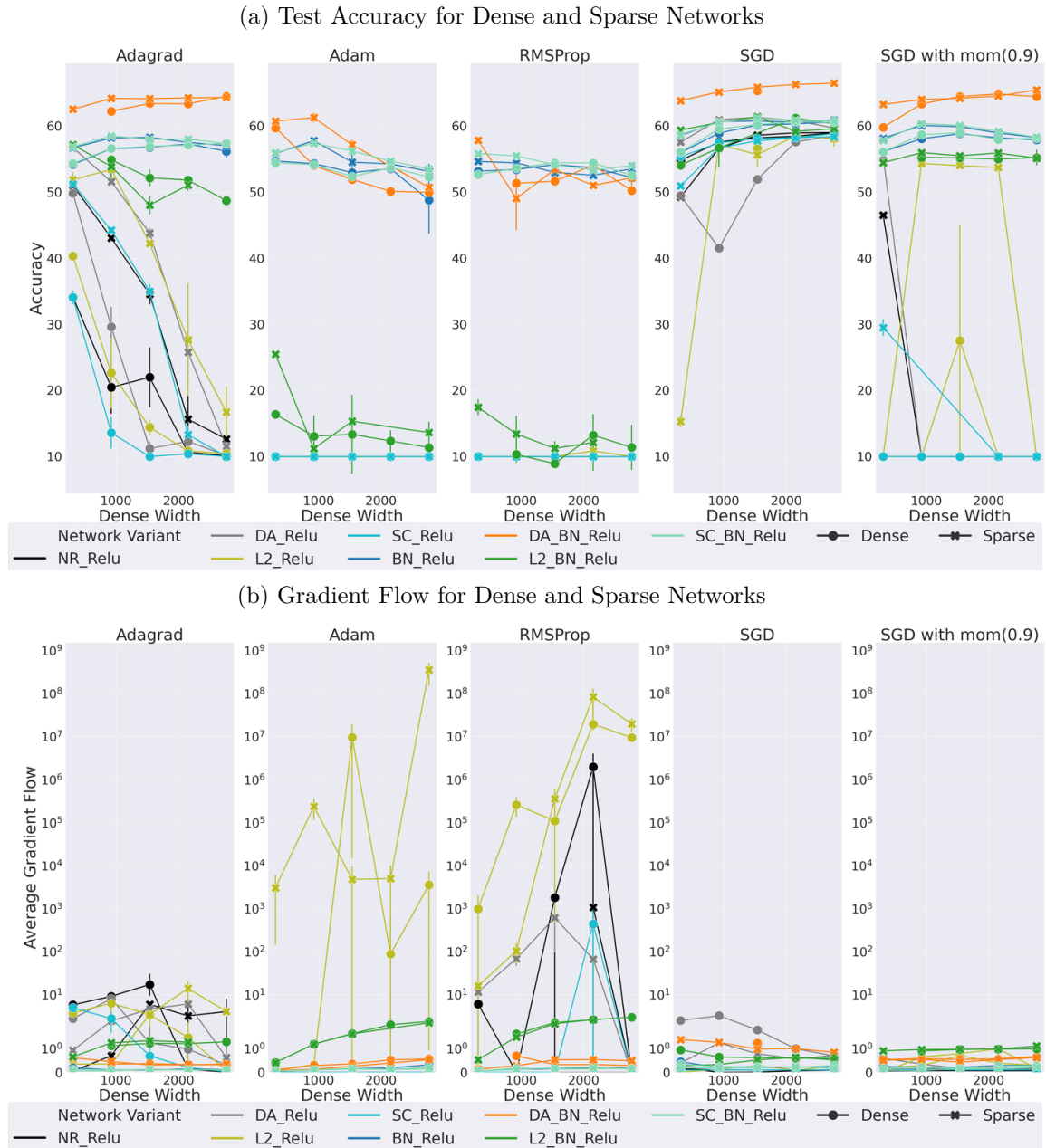
Figure A.13: Effect of Activation Functions on Accuracy and Gradient Flow for Dense and Sparse Networks with Four Hidden Layers on CIFAR-10, with low learning rate (0.001)
