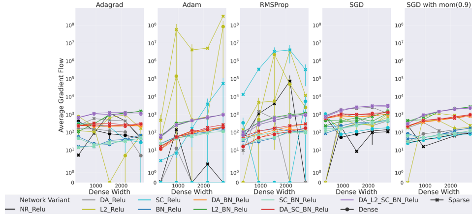
Figure A.6: Gradient Flow in CIFAR-100 using EGF_1 , with high learning rate (0.1)
