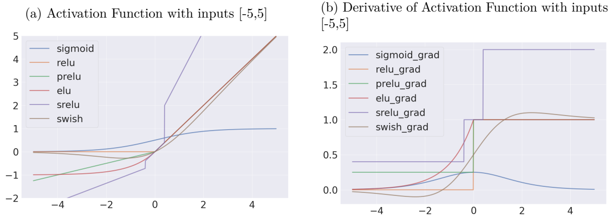
Figure A.9: Plot of Activation Functions. We plot the activation functions we used and their derivatives. We see that Swish is the only activation function that allows for the flow of negative gradients, due its non-monotonicity.
