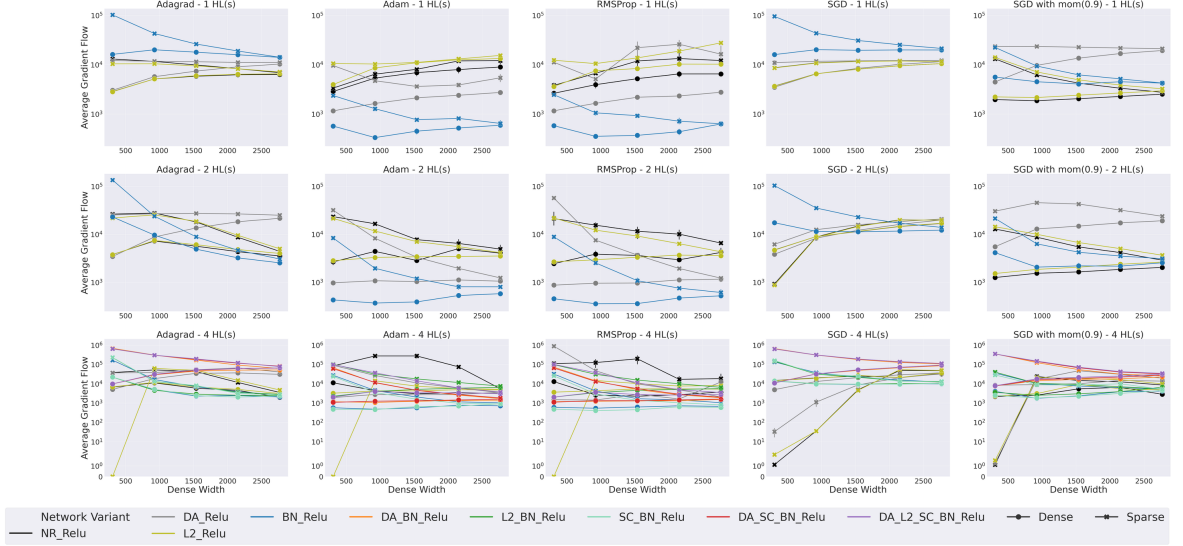
Figure A.4: Gradient Flow in CIFAR-100 using \|g\|_1 , with low learning rate (0.001)
