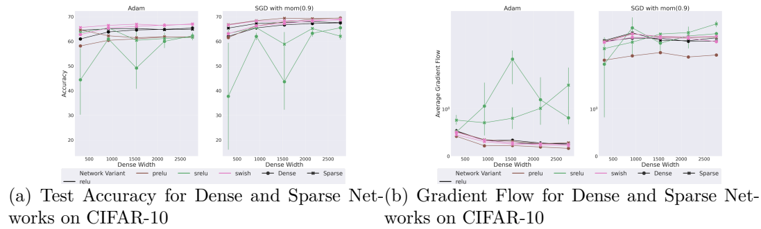
Figure A.13: Effect of Activation Functions on Accuracy and Gradient Flow for Dense and Sparse Networks with Four Hidden Layers on CIFAR-10, with low learning rate (0.001)
