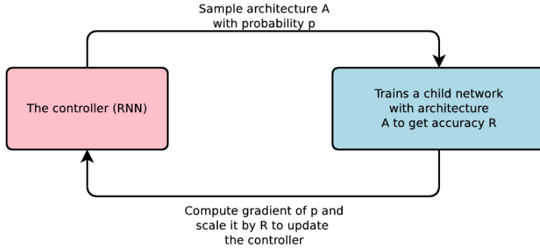
Figure 2.10: NAS Using Reinforcement Learning [Zoph and Le, 2016] . We illustrate how reinforcement learning can be used as a NAS search algorithm.
