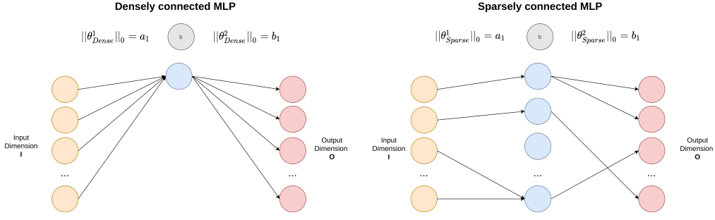
Figure 3.2: Simple Comparison of Sparse and Dense Networks We show a simple illustration of how we ensure sparse and dense networks have the same parameter count (the sparse network has more hidden nodes than the dense network, but it has the same number of active connections/weights).
