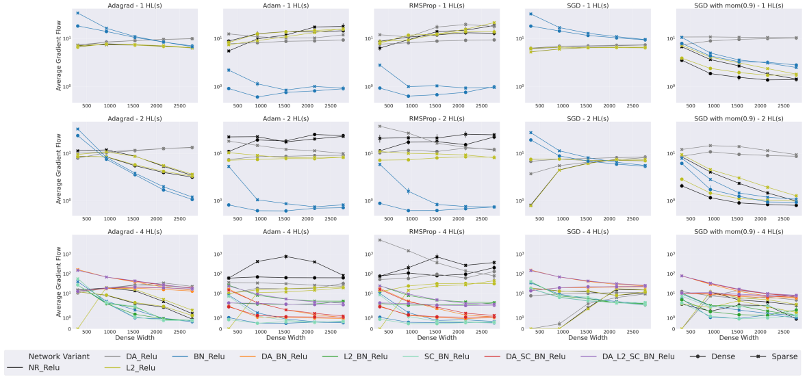
Figure A.6: Gradient Flow in CIFAR-100 using EGF_1 , with high learning rate (0.1)
