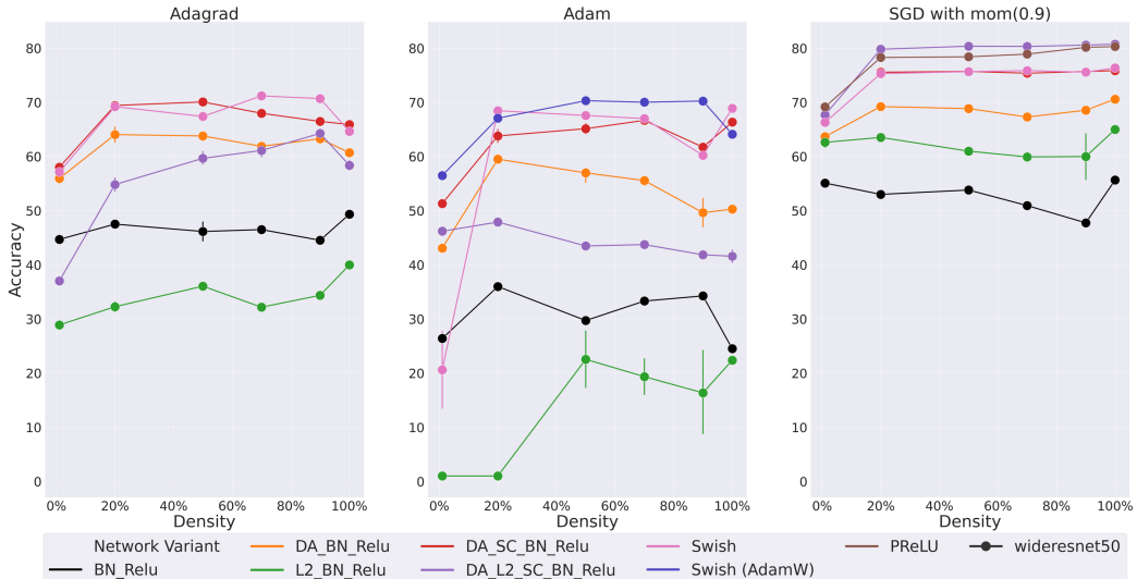
Figure 3.5: Wide ResNet-50 Test Accuracy on CIFAR-100. We see that the results achieved on MLPs, using SC-SDC, are also consistent in CNNs. The densities range from 1% to 100% (fully dense) and the gradient flow results can be found in Figure A.19.
