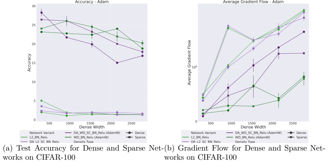
Figure A.18: Comparison of Adam and AdamW for Dense and Sparse Networks. We compare the performance of Adam and AdamW for dense and sparse Networks with four hidden layers on CIFAR-100, with a high learning rate (0.1). We see that AdamW’s weight decay formulation has a lower EGF than the standard L2 formulation used in Adam and this correlates to better network performance in AdamW
