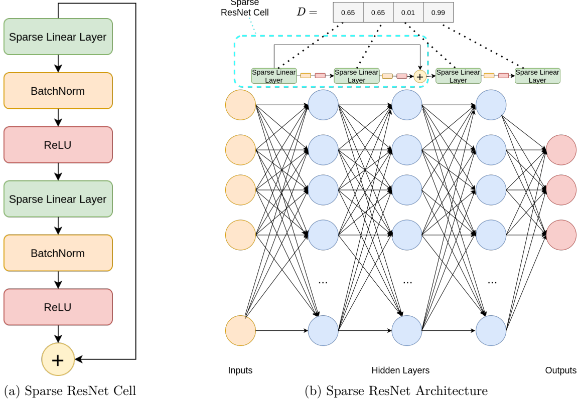
Figure 4.2: MLP Sparse Search Space. We show our sparse ResNet-like cells and how they can be chained to form Sparse ResNet Architectures. In our Sparse ResNet Architecture diagram, we omit the BatchNorm and ReLU cells for conciseness, and D represents our learned density vector, where d_i is the density of weight layer i .
