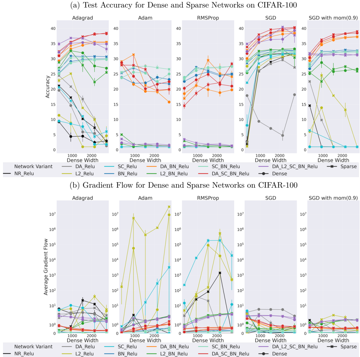
Figure A.16: Effect of Regularization ( with BatchNorm ) on Accuracy and Gradient Flow for Dense and Sparse Networks, with Four Hidden Layers on CIFAR-100, with high learning rate (0.1)
