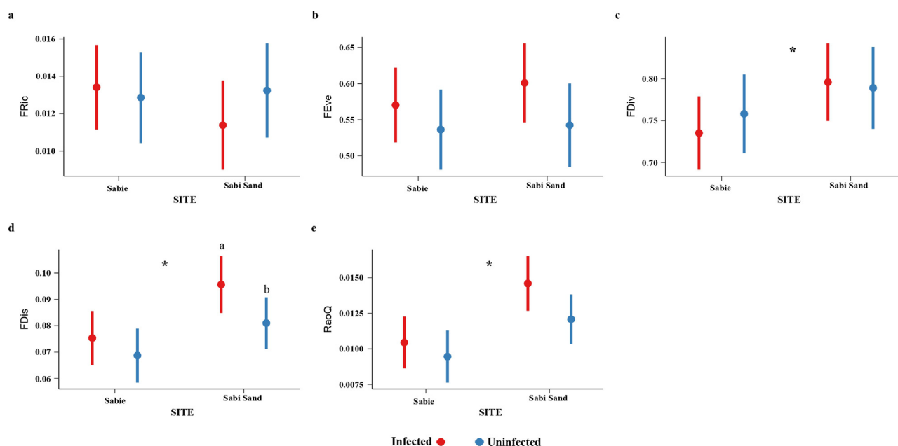
Fig. 3. The effects of site (Sabi Game Reserve, 500 mm MAR, Sabi Sand Game Reserves, 610 mm MAR) and mistletoe infection on functional richness (FRic), functional evenness (FEve), functional divergence (FDiv), functional dissimilarity and RaoQ. Asterisks show differences between sites.
