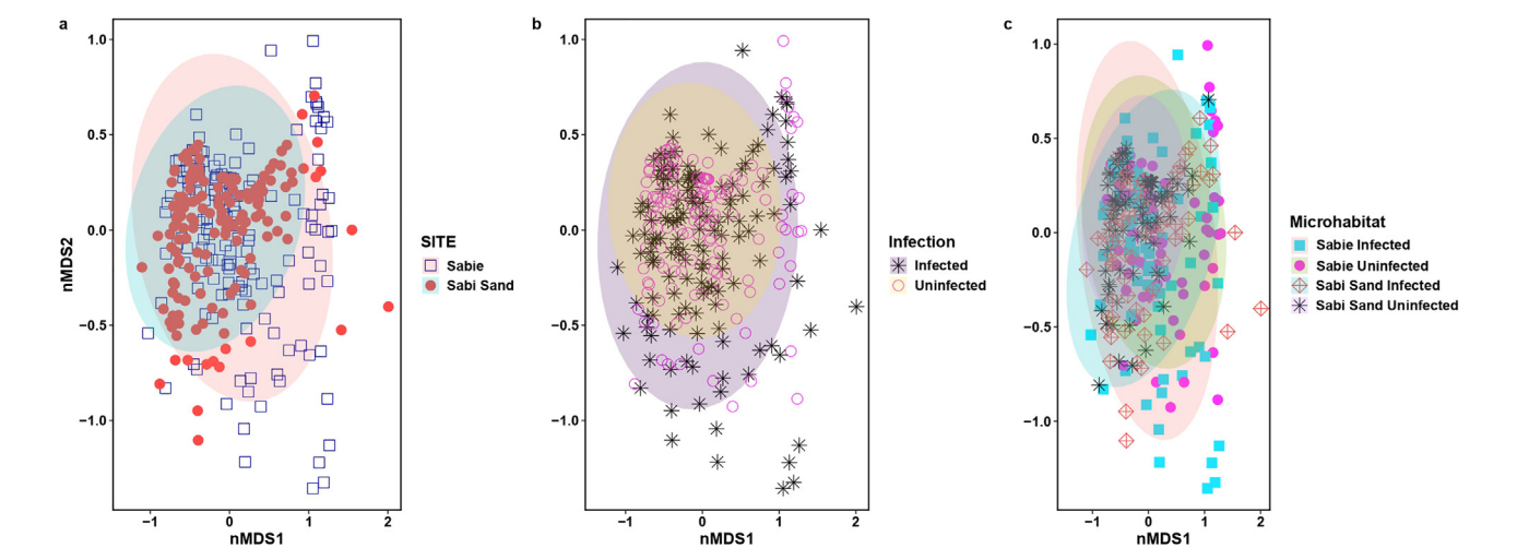
Fig 2. Non-metric multidimensional scale (nMDS) plots of total understorey plants (a) between Sabie (drier site) and Sabi Sand (wetter site) Game Reserves (stress value -0.21), (b) infected and uninfected microhabitats (stress value -0.21), and (c) microhabitats from the interaction of site and infection (stress value -0.21). The symbols represent the quadrats (1 m × 1 m) sampled underneath each tree.
