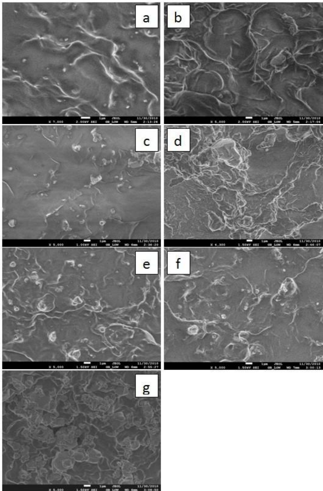
Figure 4-17 SEM images of PDMS composites containing (a)50 wt %, (b) 56wt %, (c) 60wt %, (d) 65wt%, (e) 70wt%, (f) 74wt% and (f) 77 wt % Silver loadings
