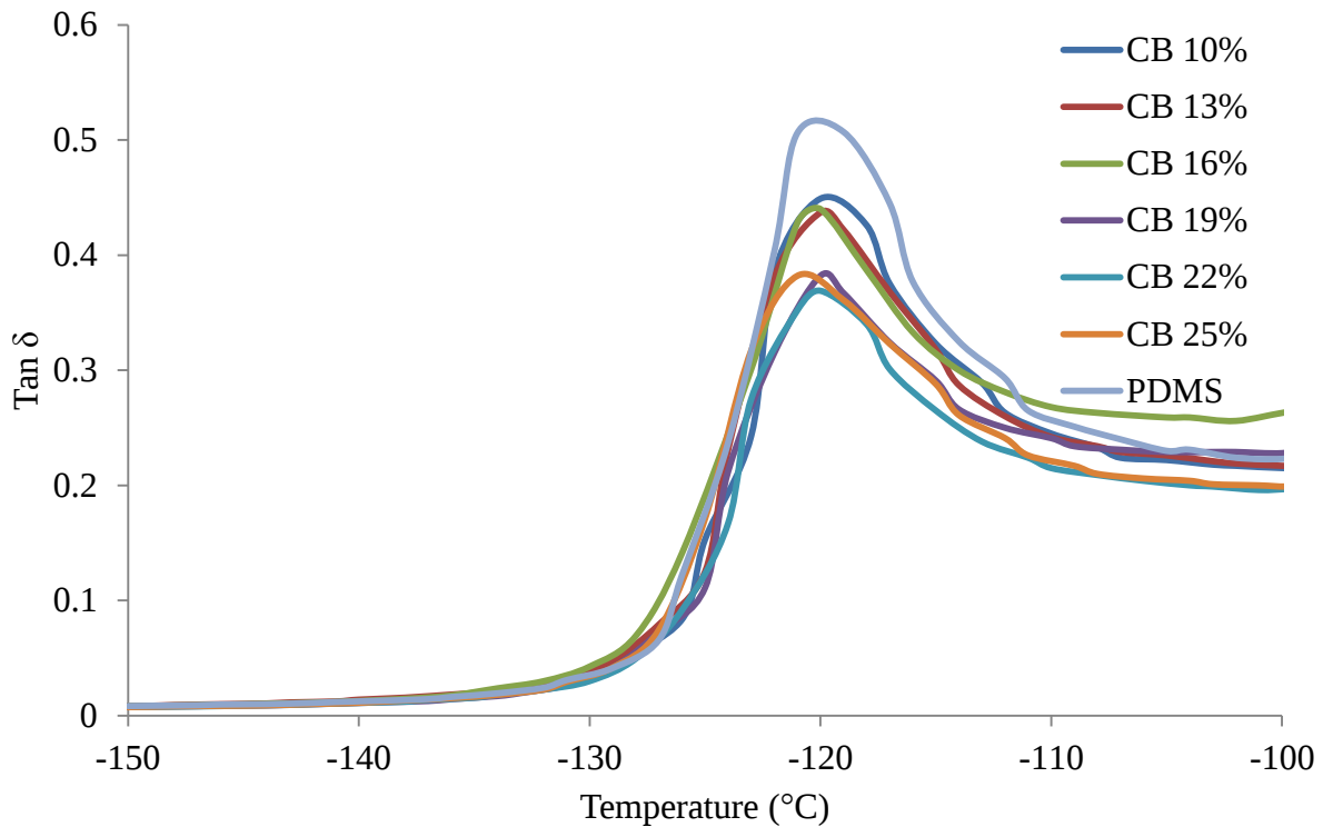
Figure 4-13 Temperature dependence of the \tan \delta of pure PDMS and the PDMS-CB composite
