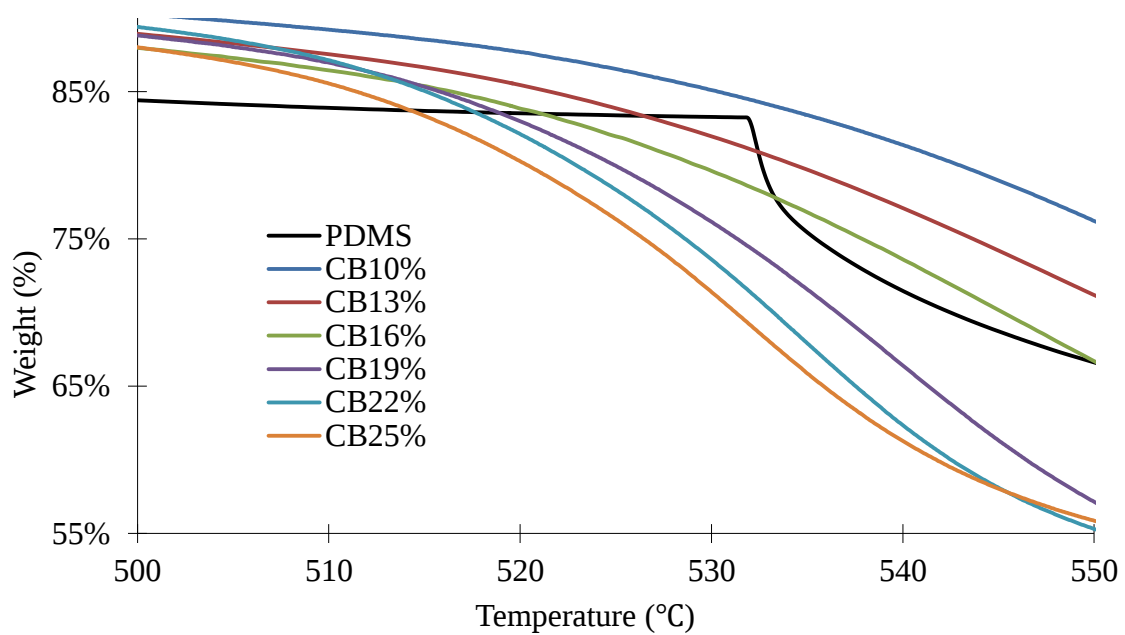
Figure 4-6 A zoom between 500 and 550 °C of figure 4-2
