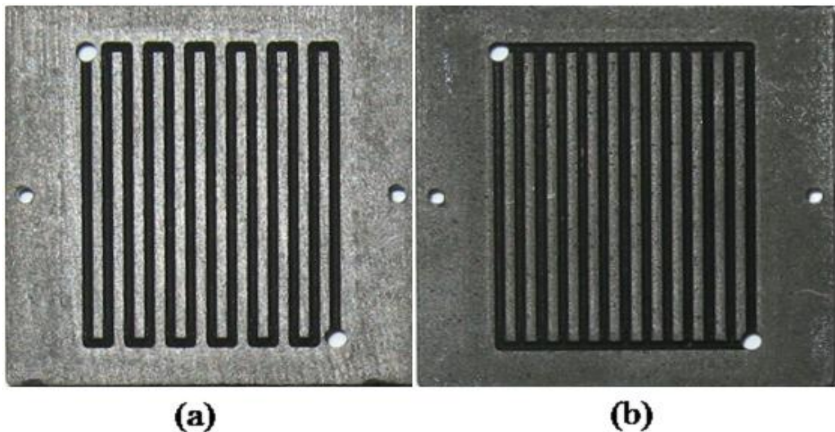
Figure 2-2 Photograph of graphite two bipolar plates (a) Serpentine (b) Interdigital
