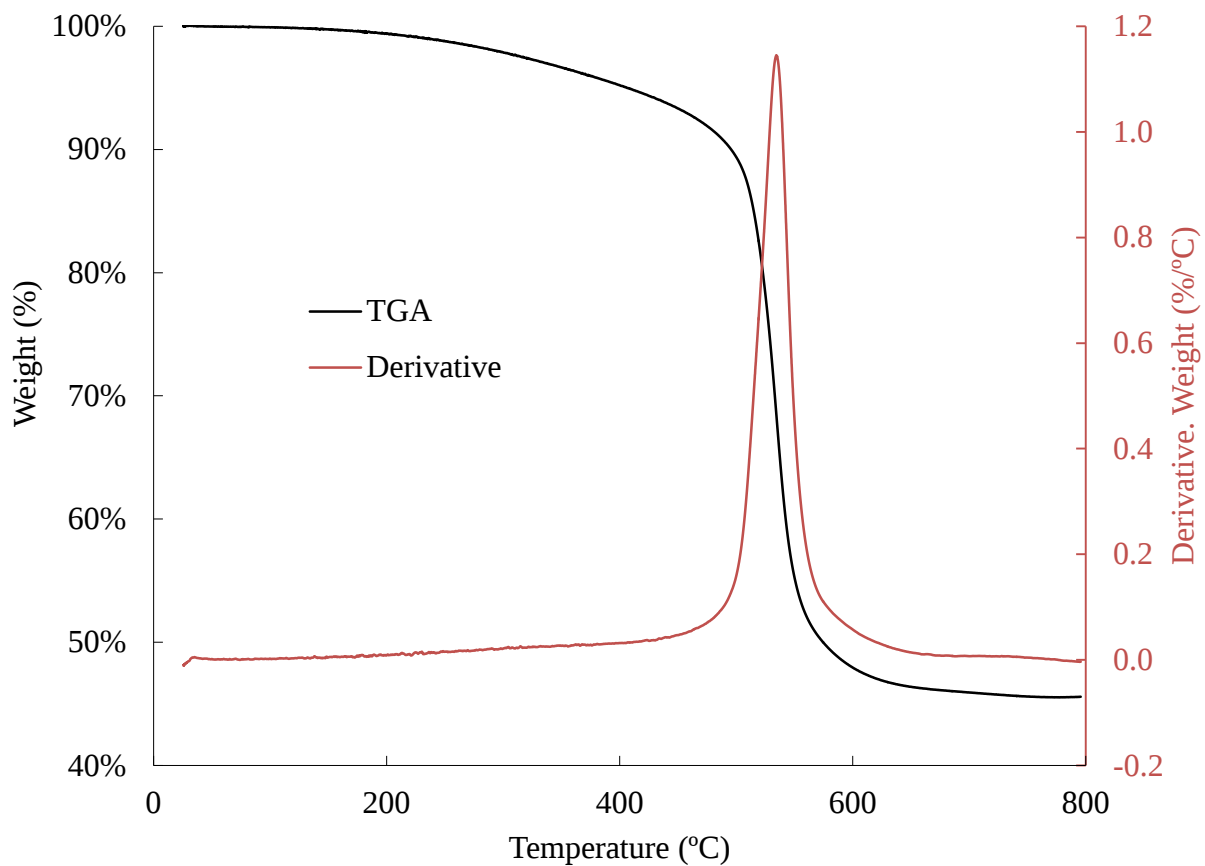
Figure 4-7 TGA and its derivative plot for our 22% PDMS-CB sample in Nitrogen
