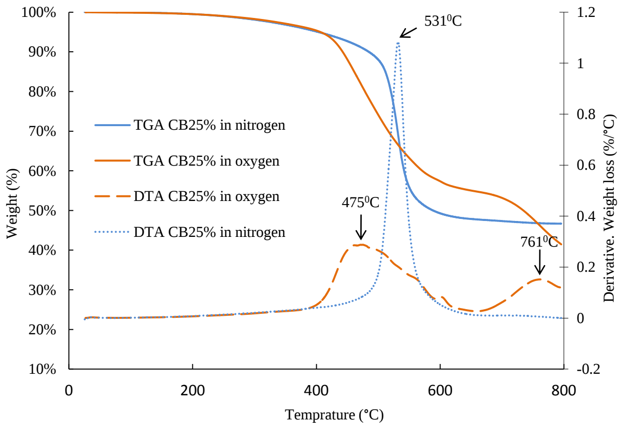
Figure 4-9 Weight loss and its derivative as a function of temperature for 25wt% carbon black filled PDMS composite under oxygen and nitrogen atmosphere
