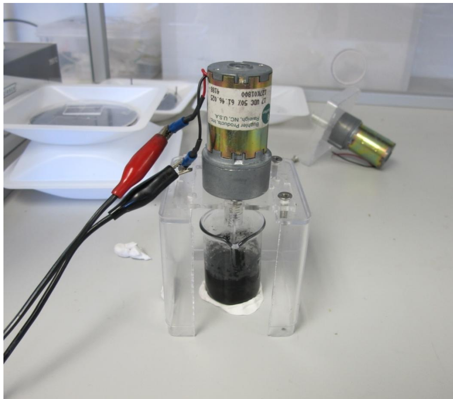
Figure 0-1 Polymer blends mixer
