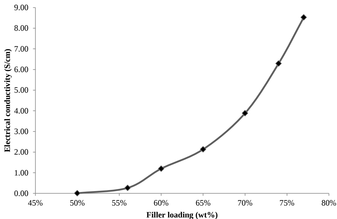
Figure 4-2 Conductivity versus silver filler weight concentration
