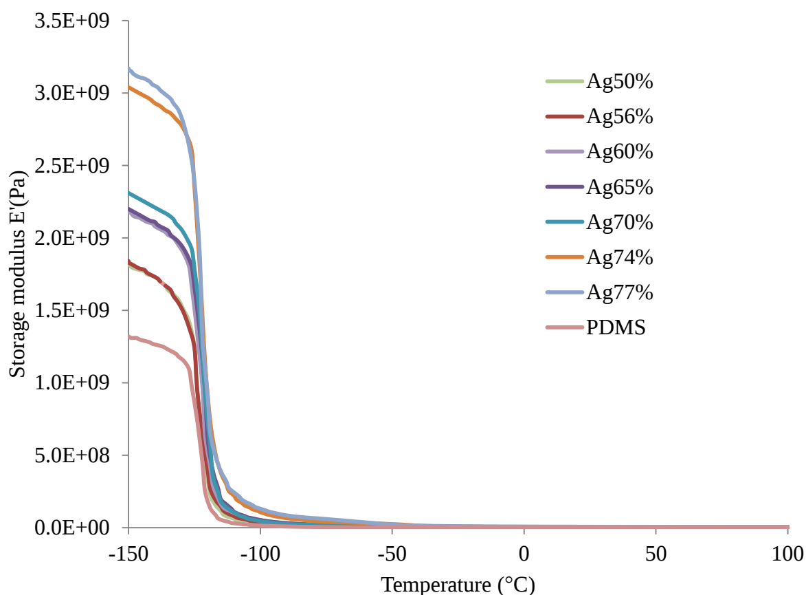
Figure 4-14 Temperature dependence of the storage modulus of pure PDMS and the PDMS-Ag composite
