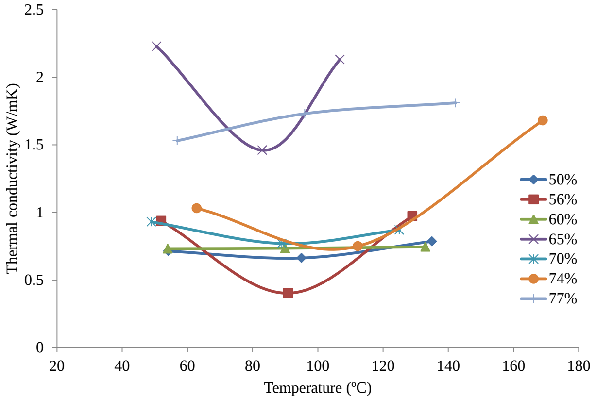
Figure 4-4 Thermal conductivity vs temperature for Silver-filled PDMS composites with different filler loadings (50–77 wt %)
