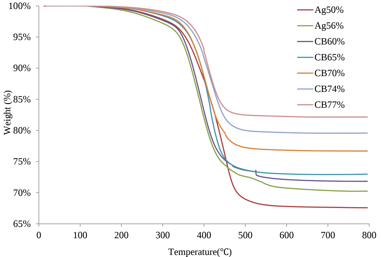
Figure 4-11 TGA analysis of pure PDMS and PDMS-Ag composites with filler loadings range 50wt%-77wt% under oxygen atmosphere.
