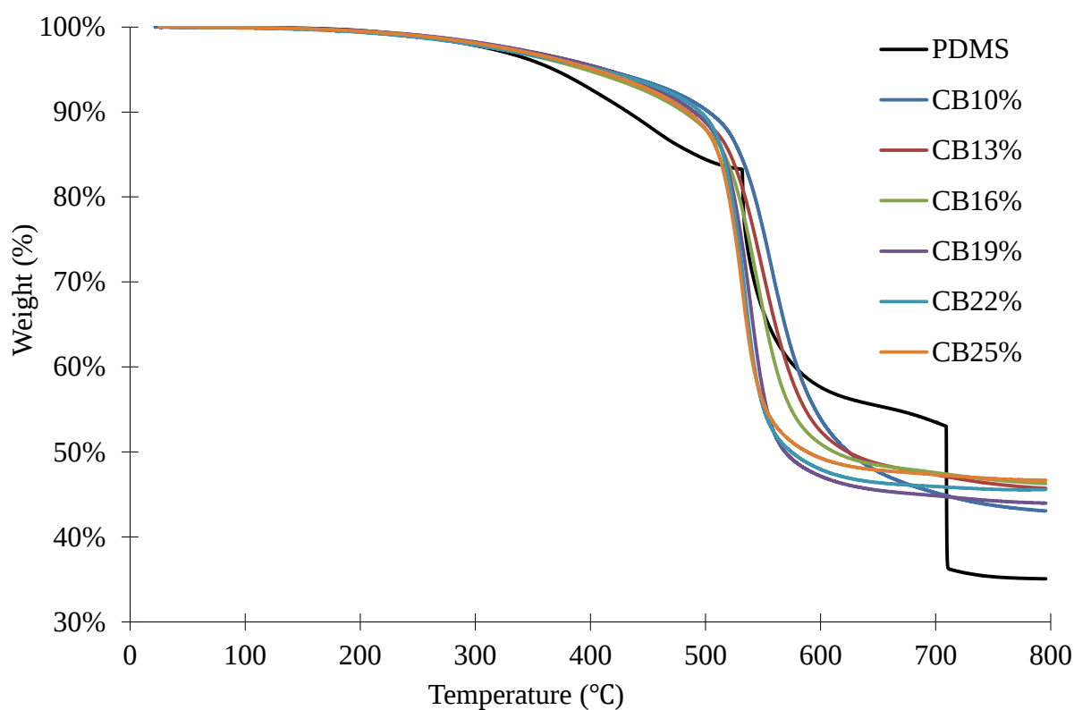
Figure 4-5 TGA analysis of pure PDMS and PDMS-CB composites in Nitrogen
