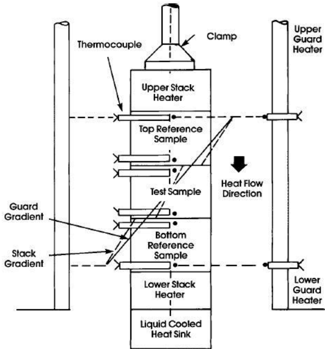
Figure 3-3 Schematic configuration of the setup
