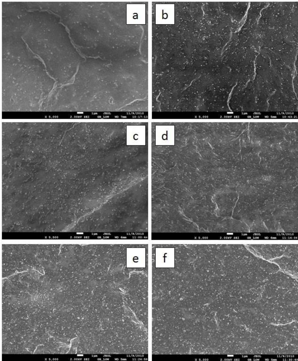
Figure 4-16 SEM images of PDMS composites containing (a) 10 wt %, (b) 13 wt %, (c) 16 wt %, (d) 19 wt%, (e) 22 wt% and (f) 25 wt % Carbon black loadings
