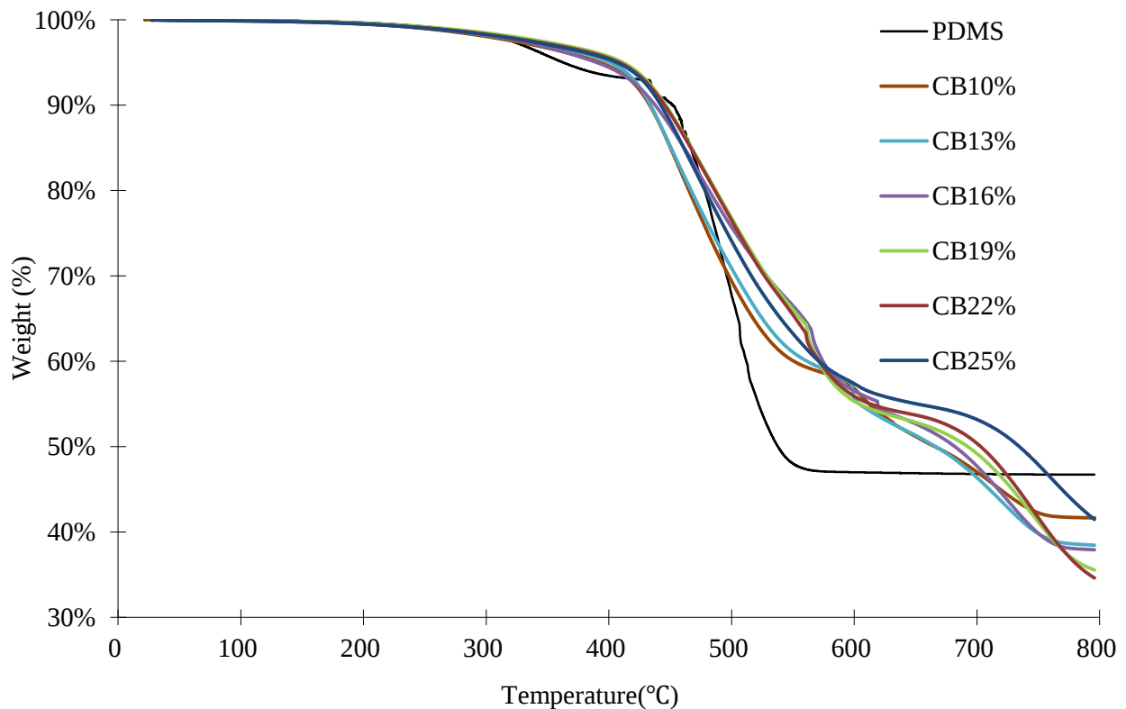
Figure 4-8 TGA analysis of pure PDMS and PDMS-CB composites with filler loadings range 10wt%-25wt% under oxygen atmosphere
