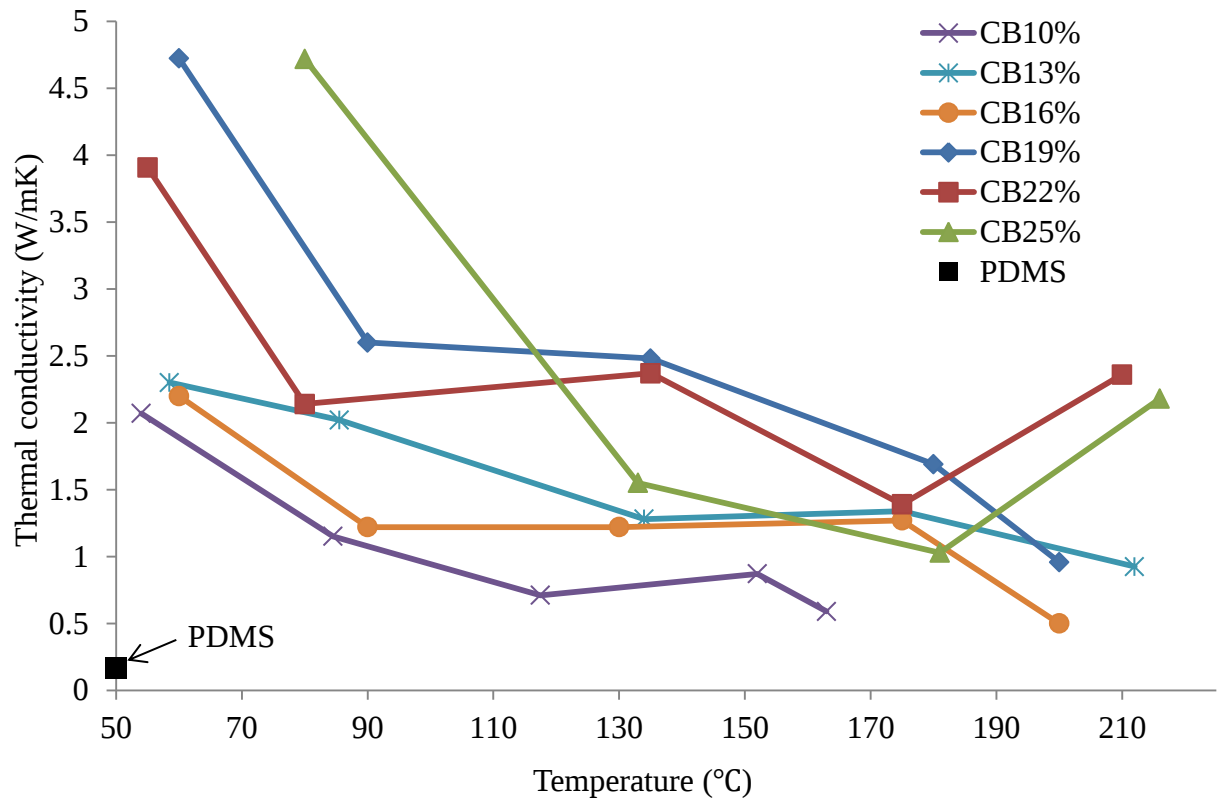
Figure 4-3 Thermal conductivity vs temperature for carbon black-filled PDMS composites with different filler loadings (10–25 wt %) The solid dot represents pure PDMS thermal conductivity value
