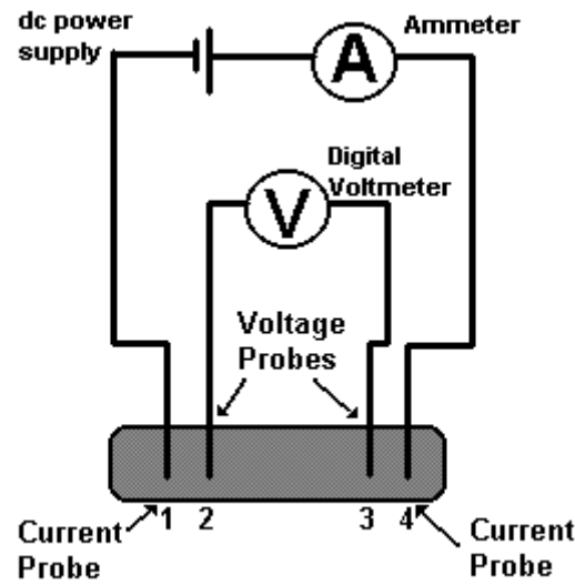
Figure 3-2 Four point probe schematic (Scientific instruments, 2010)
