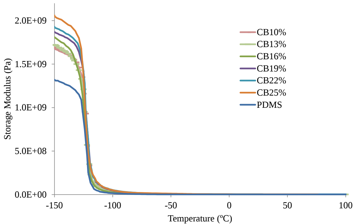
Figure 4-12 Temperature dependence of the storage modulus of pure PDMS and the PDMS-CB composite
