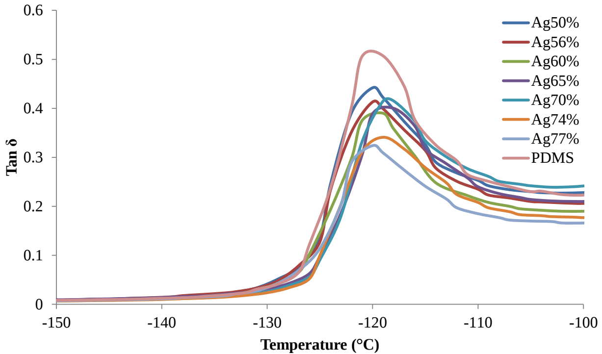
Figure 4-15 Temperature dependence of the \text{Tan } \delta of pure PDMS and the PDMS-Ag composite
