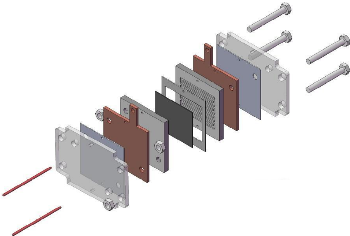
Figure 2-1 Schematic of DMFC structure and components (from side to the centre: end plate, gasket, copper current collector, graphite flow field plate, MEA and gasket)
