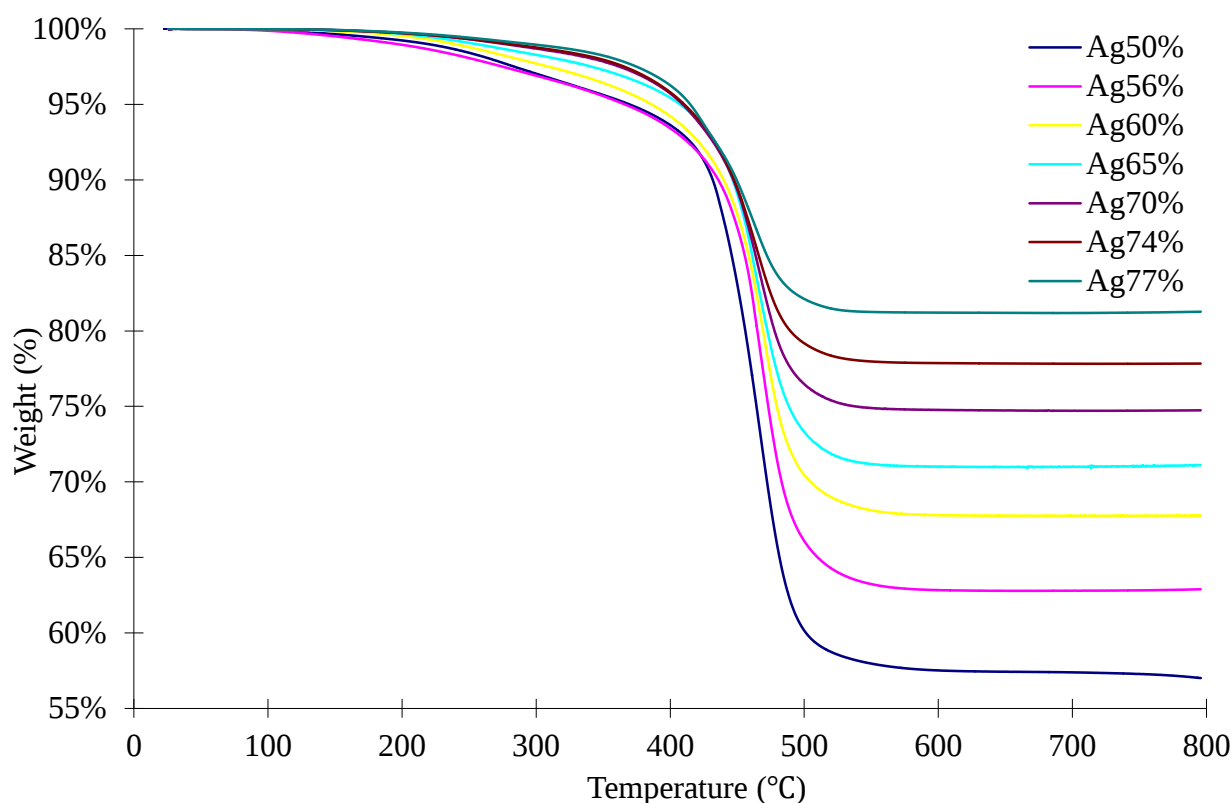
Figure 4-10 TGA analysis of pure PDMS and PDMS-Ag composites with filler loadings range 50wt%-77wt% under nitrogen atmosphere
