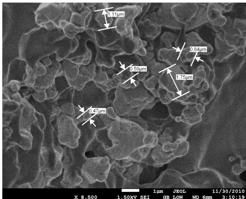
Figure 4-18 Particle size measurement with SEM
