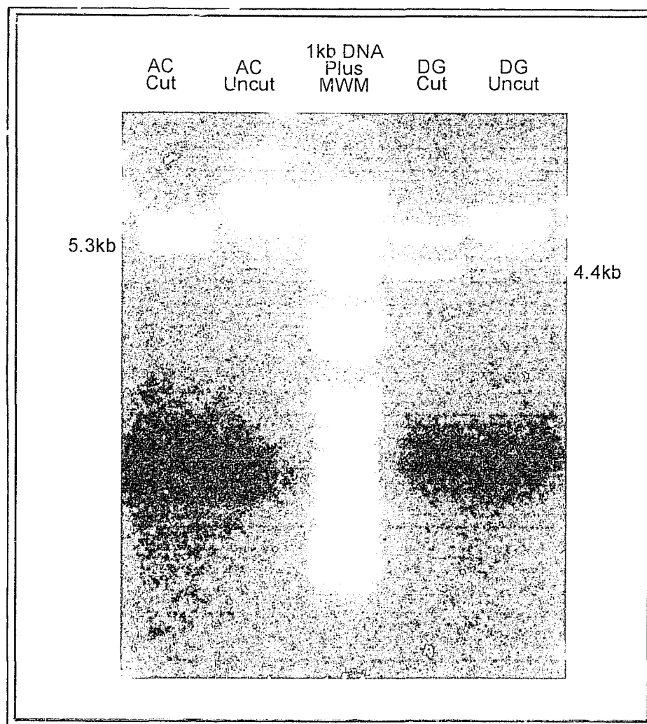
Figure 9: Visualisation of pUC18 vector (with modified polylinker) containing two partial BRCA2 cDNA clones (S. Tavtigian - Myriad Genetics), termed "AC" and "DG"; restricted with endonucleases; and electrophoresed on a 0.8% agarose gel. These clones were later used for hybridisation after Southern blotting. Lanes 1 & 2: pUC18 vector containing "AC" clone - lane 1: restricted with endonucleases SalI and EcoRV , "AC" clone 5.3 kilobases (kb) - lane 2: unrestricted; lane 3: 1kb "DNA Plus" molecular weight marker (MWM); lanes 4 & 5: pUC18 vector containing "DG" clone - lane 4: restricted with SacI and SalI endonucleases, "DG" clone 4.4kb - lane 5:unrestricted.
