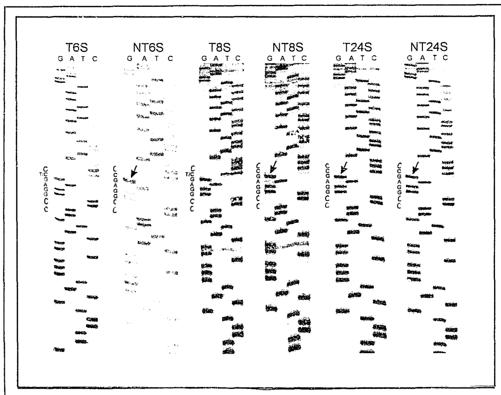
Figure 13: Autoradiograph of polyacrylamide gels showing sequencing profile of the codon 249 region of the p53 gene. Panels left to right: sequence of the sense (S) strand of tumour (T) and non-tumorous (NT) tissue DNA. The AGG→AGT mutation at codon 249 is visible in the tumour tissue of individuals 6 and 8 (T6S; T8S). These individuals are heterozygous for the mutation and thus the wild-type AGG sequence is also visible. The two G bands have, however, been compressed into one as a result of a gel artefact (section 4.1.3.1). The compression results in the uneven spacing of the bands (CCC) directly ahead causing the T band to lie adjacent to the C band. (Composite photograph).
