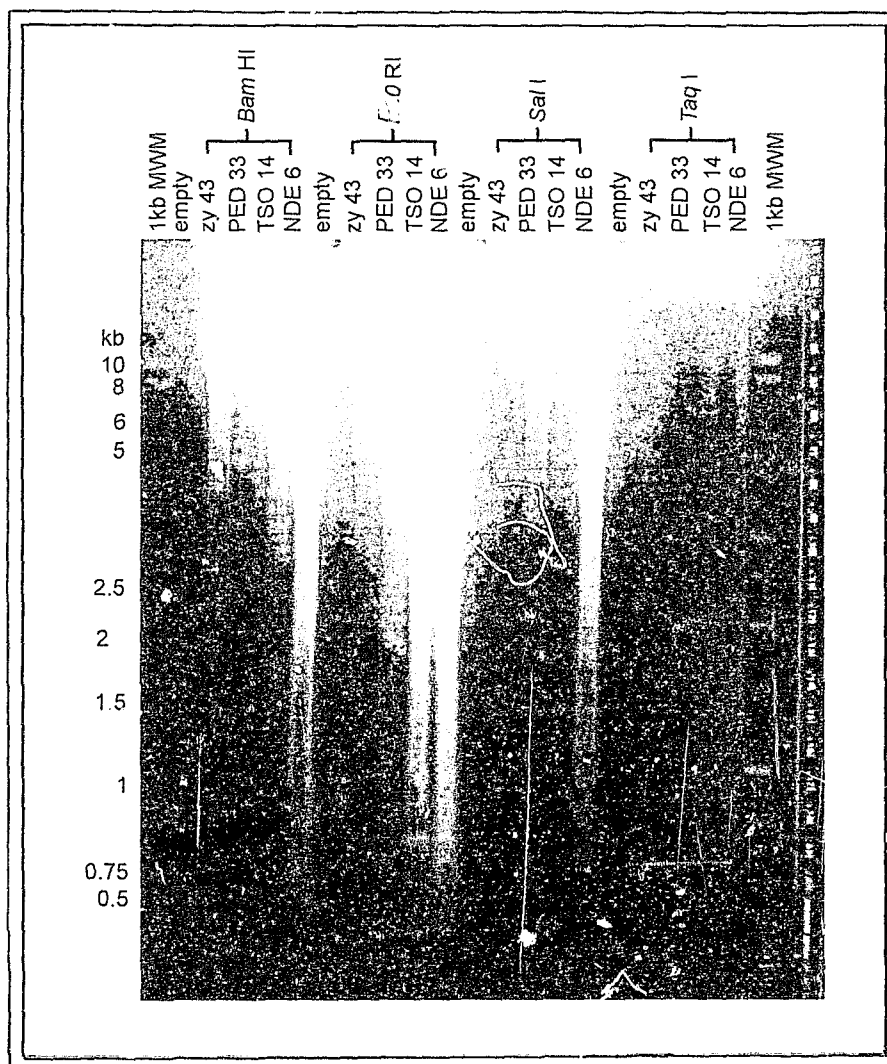
Figure 10: DNA from a random black population restricted with endonucleases, and visualised on a 0.8% agarose gel, later used in Southern blotting. Lanes 1 & 22: 1 kilobase (kb) molecular weight marker (MWM); lanes 3-6, 8-11, 13-16, 18-21: DNA of individuals ZY 43, PED33, TSO14, and NDE6 restricted with the endonucleases Bam HI, Eco RI, Sal I, and Taq I respectively.
