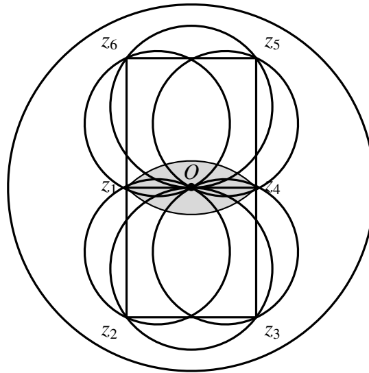
Figure 4.3: n = 6
