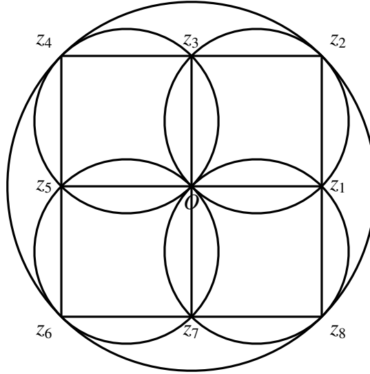
Figure 4.2: n = 8
