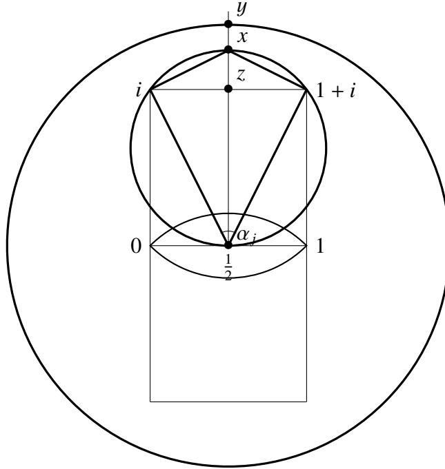
Figure 4.8: Case (ii)
