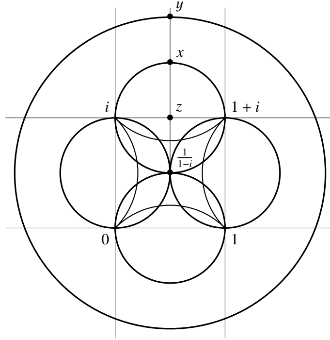
Figure 4.9: Case (iii)
