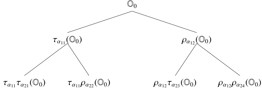
Figure 6.2: Graph \mathcal{G}_0
