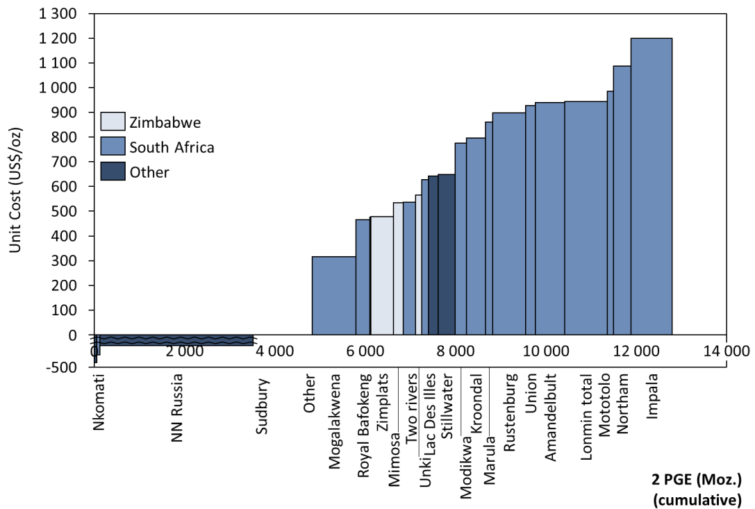
Figure 4.4 :2017 PGM Cost Curve per 2PGE. After Appendix 8.14
