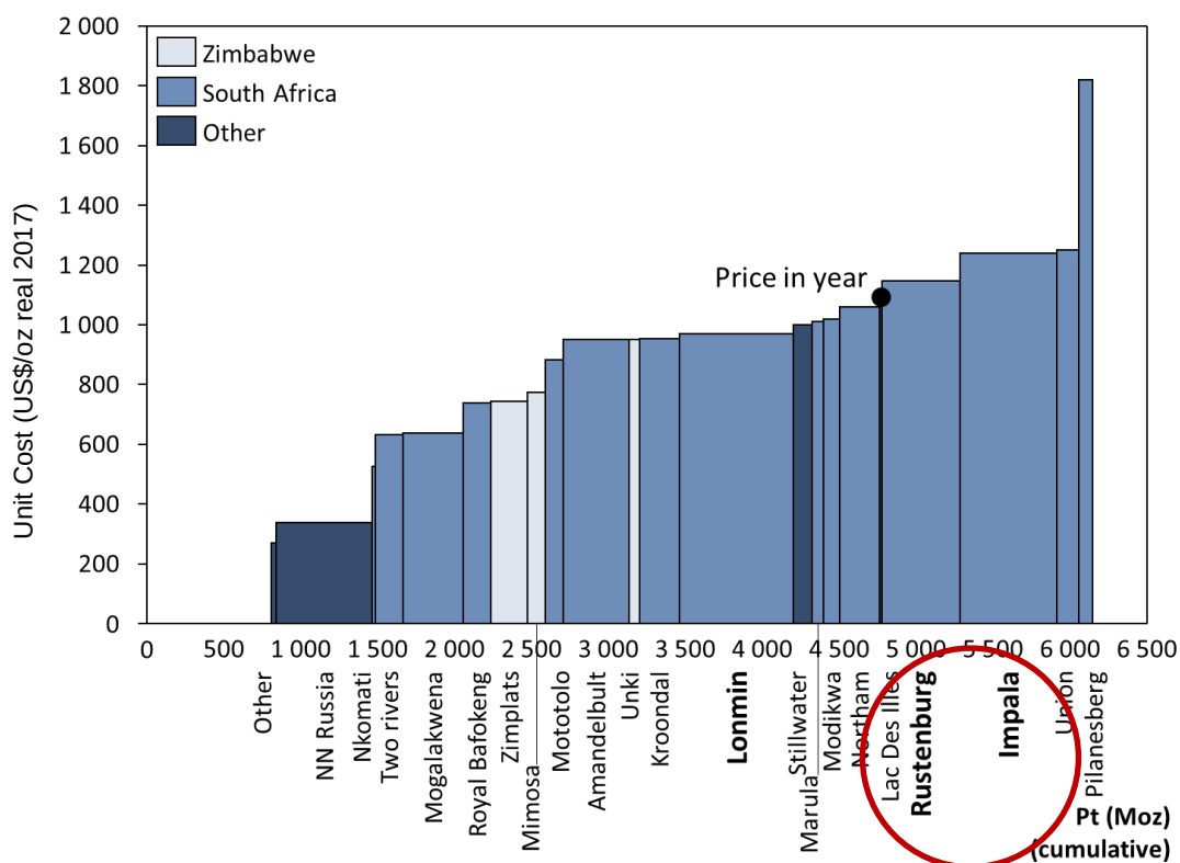
Figure 4.15 : 2015 PGM Cost Curve per ounce Platinum (co-product). After Appendix 8.8
