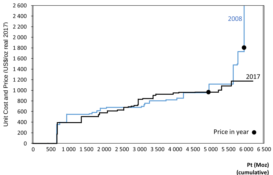
Figure 4.7 : 2017 and 2008 PGM Cost Curve per ounce Platinum (US$/oz Pt, real 2017, co-product). After Appendix 8.1 and 8.10
