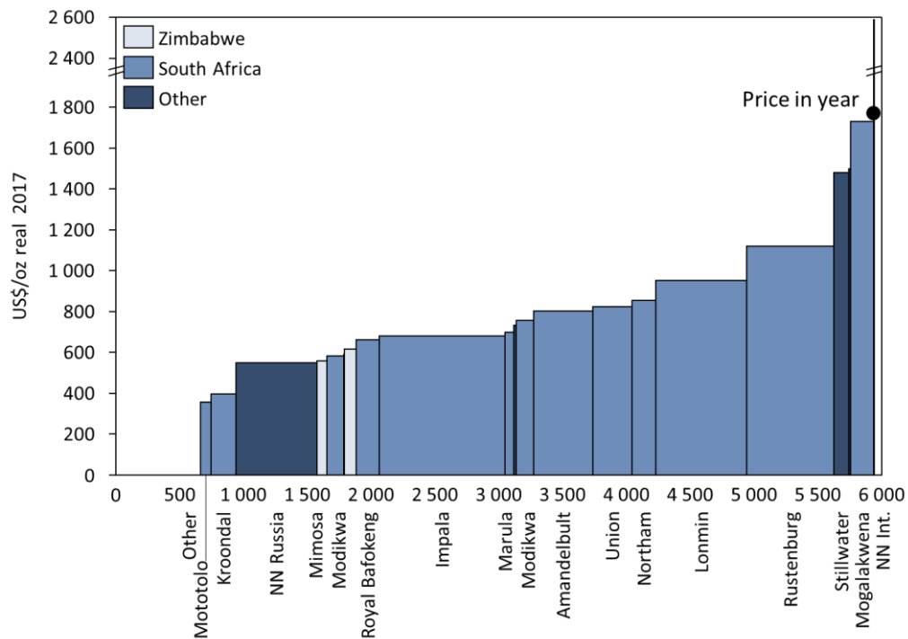
Figure 8.1 : 2008 PGM Cost Curve per ounce Platinum (co-product)
