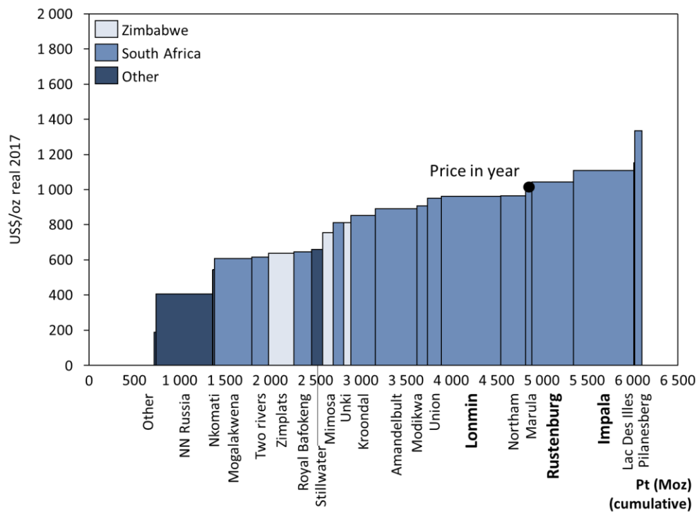
Figure 8.9 : 2016 PGM Cost Curve per ounce Platinum (co-product)
