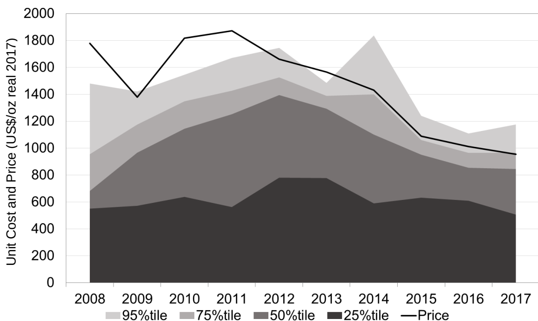
Figure 4.12 : Summary PGM cost curves 2008 – 2017 (cost percentile). After Appendix 8.1 to 8.10
