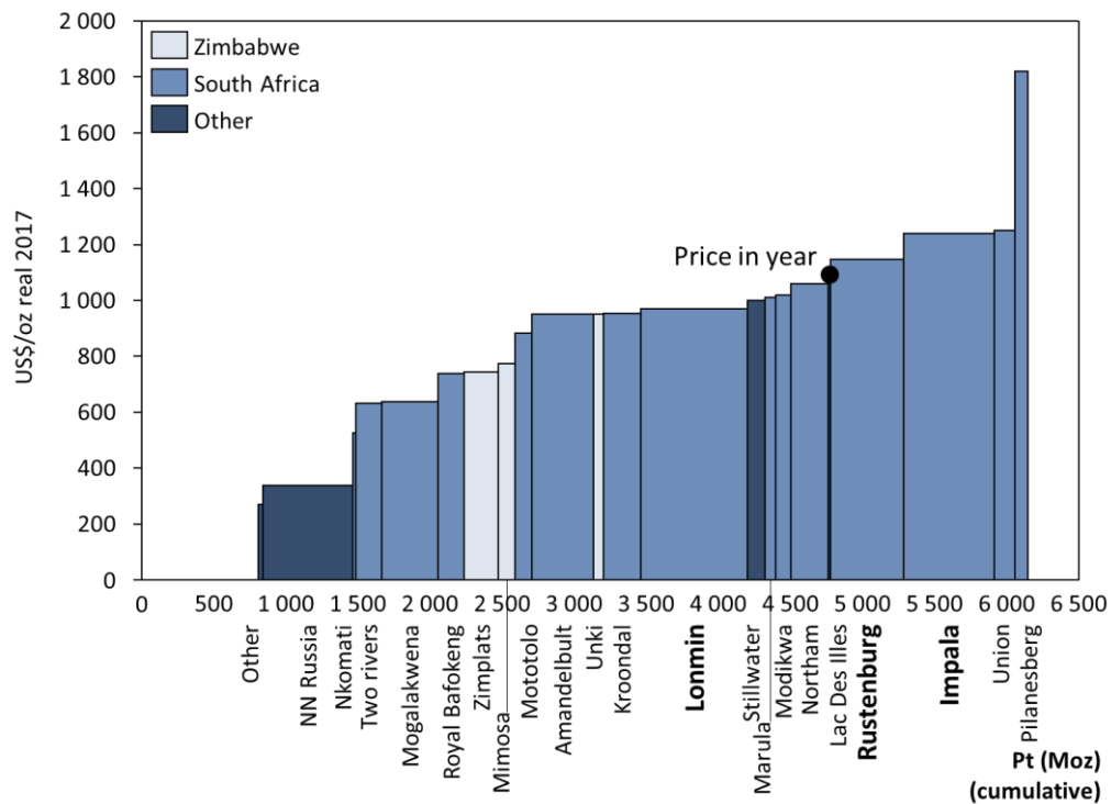
Figure 8.8 : 2015 PGM Cost Curve per ounce Platinum (co-product)
