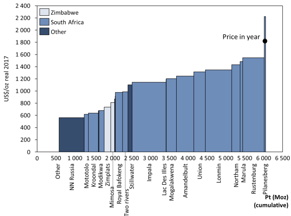
Figure 8.3 : 2010 PGM Cost Curve per ounce Platinum (co-product)
