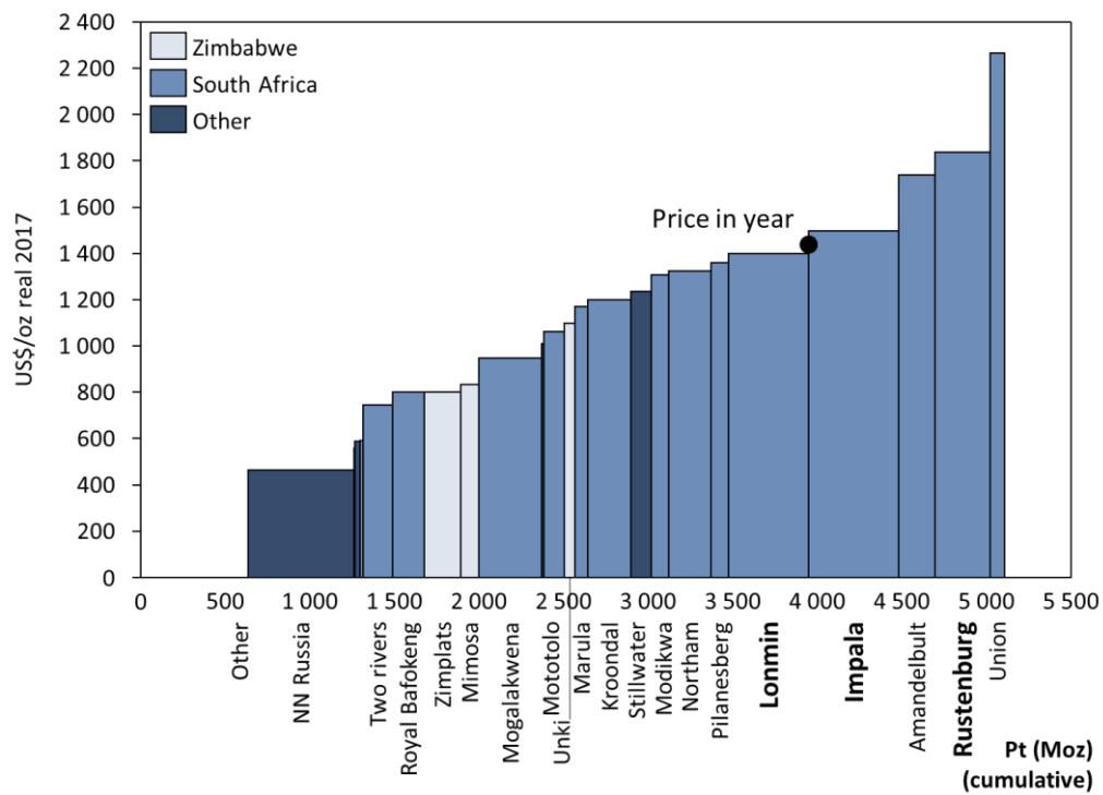
Figure 8.7 : 2014 PGM Cost Curve per ounce Platinum (co-product)
