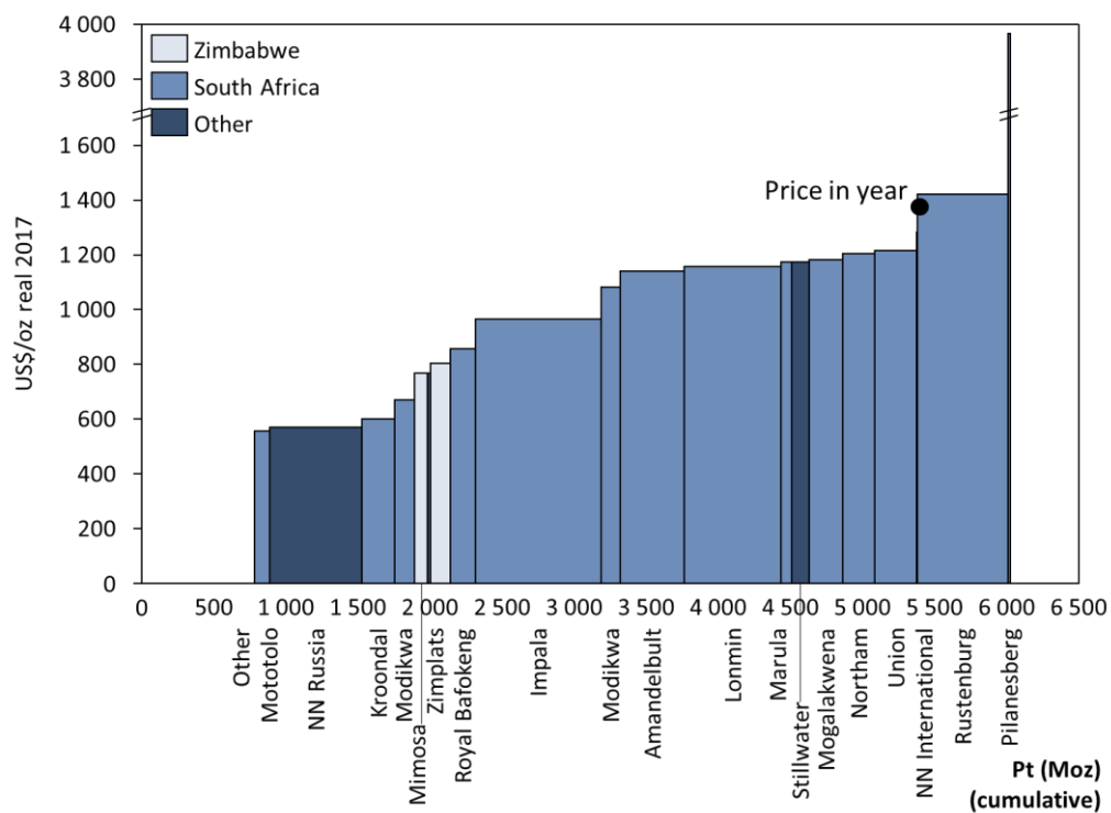
Figure 8.2 : 2009 PGM Cost Curve per ounce Platinum (co-product)
