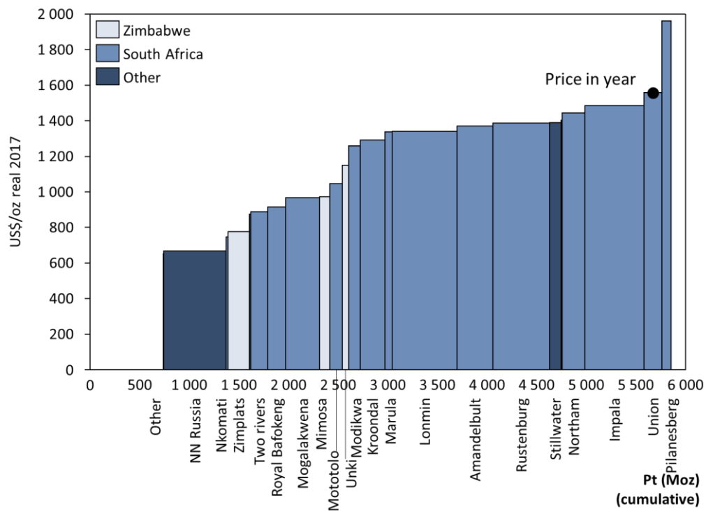
Figure 8.6 : 2013 PGM Cost Curve per ounce Platinum (co-product)
