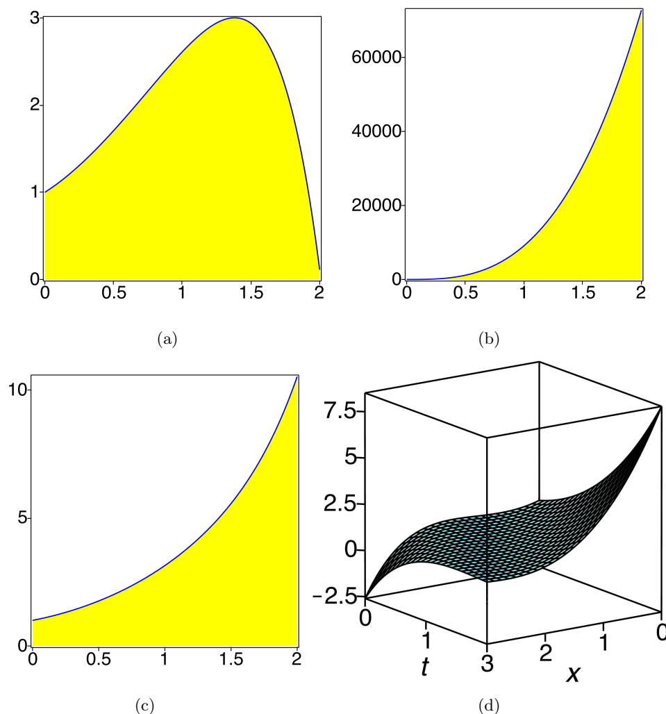
Fig. 2 We select the parameter values \alpha = a_k = 1 : Plots of (a) Eq. (37); (b) Eq. (39); (c) Eq. (41); (d) Eq. (28).
