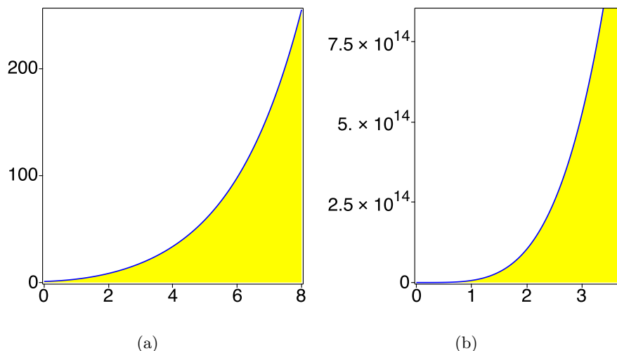
Fig. 1 We select the parameter values \alpha = a_k = 1 : Plots of (a) Eq. (28); (b) Eq. (31).
