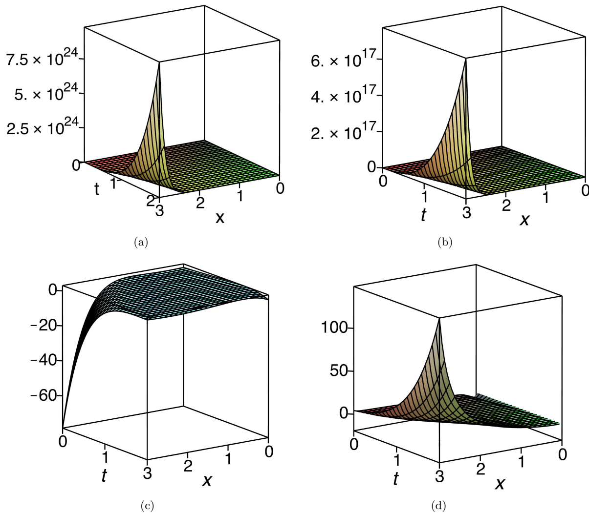
Fig. 3 Parameter values \alpha = a_k = 1 : 3D plots of (a) Eq. (31); (b) Eq. (39); (c) Eq. (37); (d) Eq. (41).
