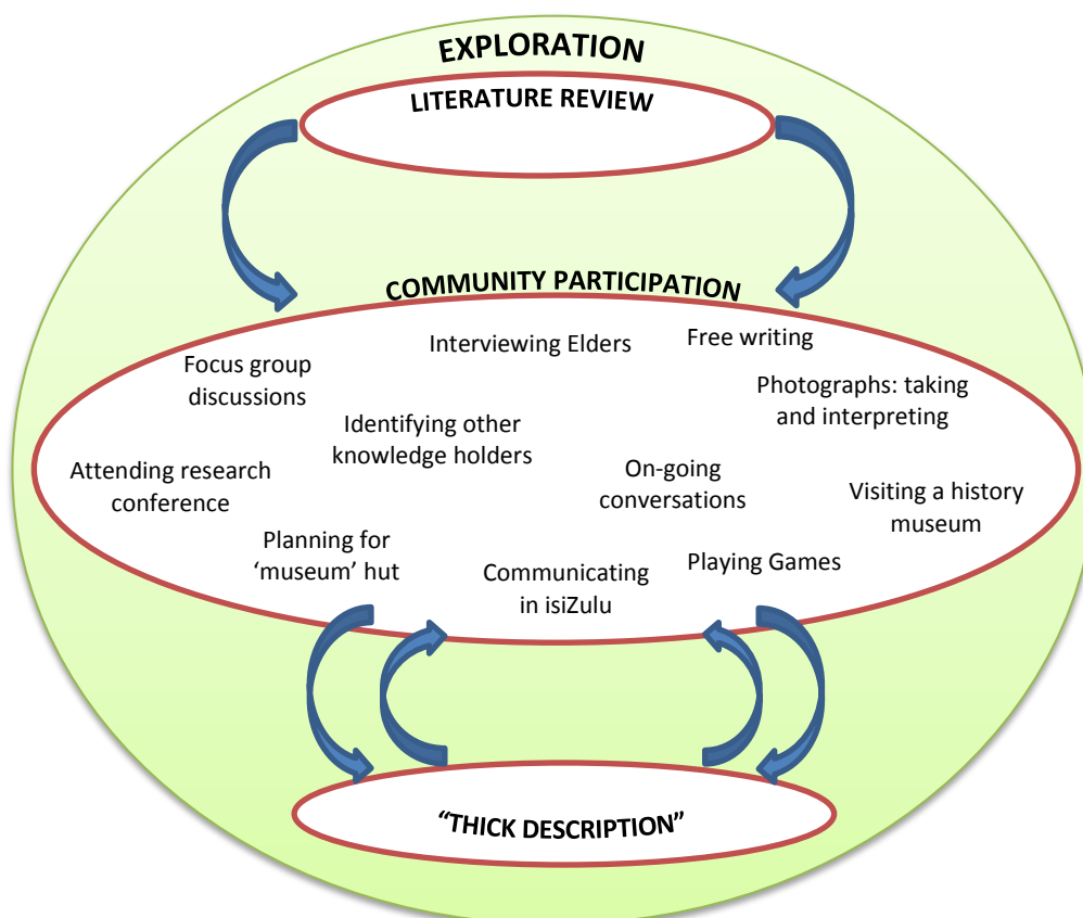
Figure 5.1: Research Design
