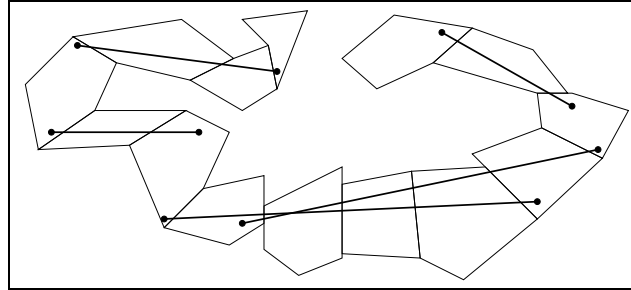
Figure 8.6: Set of lines that cross the greatest number of adjacencies
