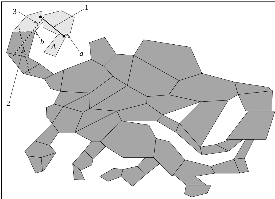
Figure 6.11: A configuration of convex polygons with algorithm 11 applied once. Line 1 is now in the solution set and lines 2 and 3 are in the data structure.
