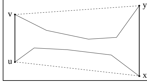
Figure 2.19: Illustration of inner convex hulls. The inner convex hulls are formed by finding the convex hulls of the reduced chains from figure 2.18.
