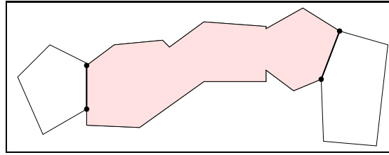
Figure 2.13: The adjacency polygon has been found and is indicated by the shaded region.
