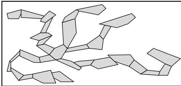
Figure 1.3: A star of convex polygons
