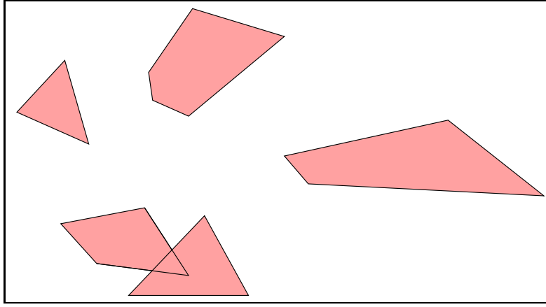
Figure 2.24: Illustration of stabbing in 2-space
