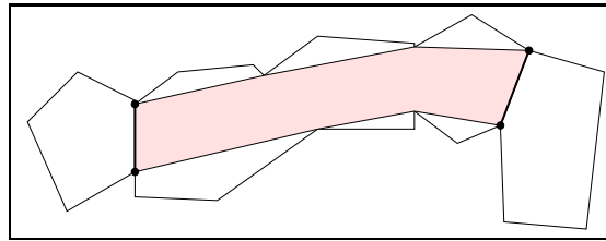
Figure 2.14: The reduced adjacency polygon is indicated by the shaded region. It is found by reducing the adjacency polygon shown in figure 2.13.
