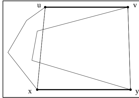
Figure 2.16: An example of C(v, y) cutting through Q(u, v, y, x) indicating that uv is not partially visible to xy .
