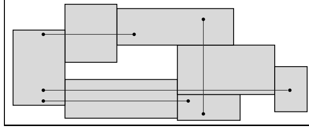
Figure 2.2: Example of axial line placement with orthogonal lines in orthogonal rectangles (ALP-OLOR).
