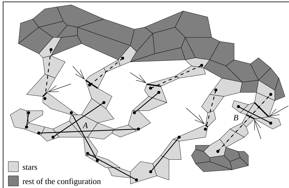
Figure 8.14: A general configuration with stars A and B
