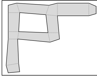
Figure 2.6: Example of a deformed urban grid.
