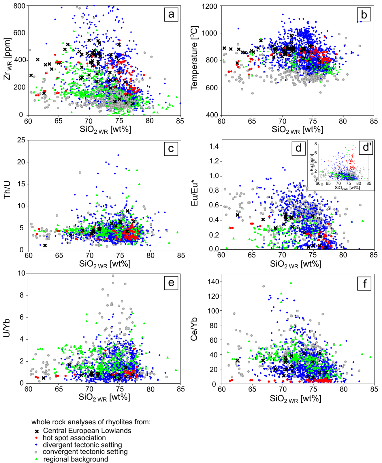
Fig. 2 Rhyolite whole rock data (a) \text{SiO}_2 (wt%) vs [Zr] (ppm) concentration. The CEL as indicated by the xs, are located close to the investigated sites of Fehmarn, Salzwedel, Penkun and Wysoka Kamieńska (data from: Protas et al. 1995; Benek et al. 1996; Paulick
