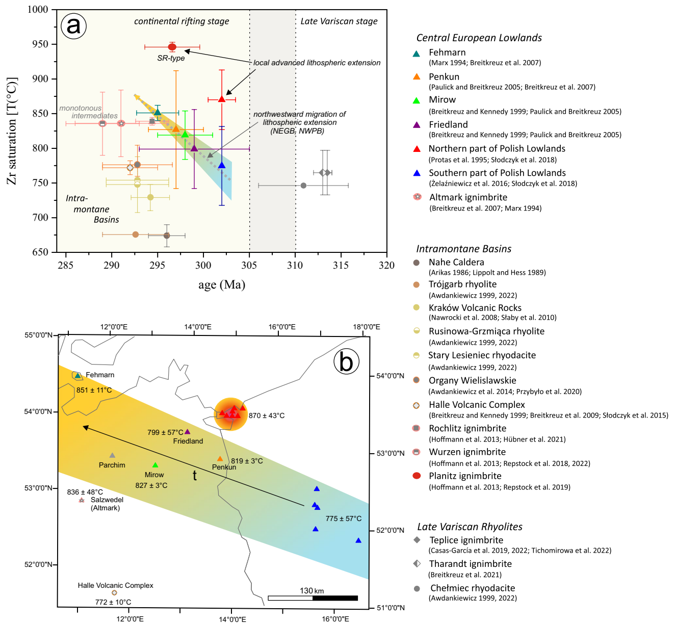
Fig. 4 (a) Zircon saturation temperatures of presented rhyolitic units of the Central European Lowlands with respect to their ages; (b) schematic illustration of alignment of regional change in zircon saturation temperature
