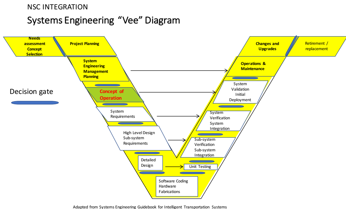
Figure 5.9: CONOPS place in the Systems Engineering V-Model (SE Guidebook for ITS (2015))
