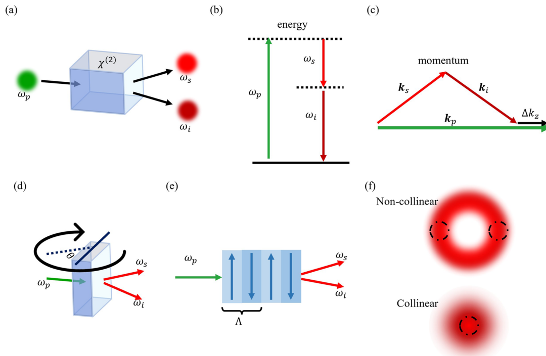
FIG. 5. Spontaneous parametric down-conversion. (a) Generation of SPDC photons from nonlinear crystals (NC) that are characterized by a second order nonlinear susceptibility tensor, \chi^{(2)} . In this process, a single photon with a frequency, \omega_p , is absorbed by the crystal, and twin photons with frequencies, \omega_s and \omega_i , are produced. (b) Energy diagram for the three photons involved in SPDC, showing energy conservation. (c) Momentum conservation in the SPDC process. The momentum vectors of the emitted s and i photons must add up to those of the pump photon. The phase mismatch occurs in the longitudinal direction. The emission cones can be altered by changing the phase matching conditions. This can be achieved via (d) angle tuning in bulk crystals and (e) temperature tuning in periodically poled (PP-) crystals. (f) Far-field intensity profiles of SPDC photons showing non-collinear and collinear geometries where the entangled photons are found in the regions highlighted with dashed lines.
