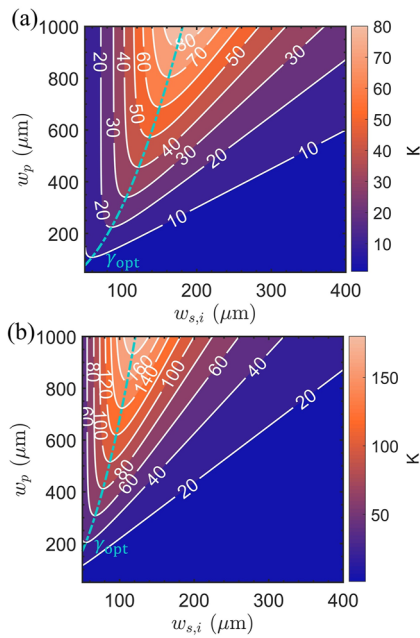
FIG. 11. SPDC measurable OAM bandwidth. Example of measurable bandwidth ( K \equiv K_{\text{eff}} ) as a function of the pump and detection beam sizes for a (a) L = 5 mm crystal and a (b) L = 1 mm crystal. The dotted line indicates the optimal ratio for maximum bandwidth between the detection and signal beam waists.
