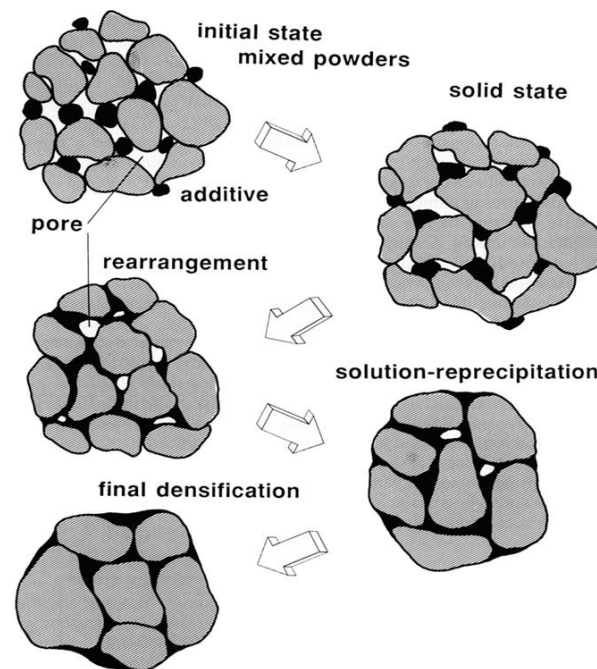
Figure 25: Microstructure changes during conventional sintering, starting from mixed powders to fully dense sintered compact [31].
