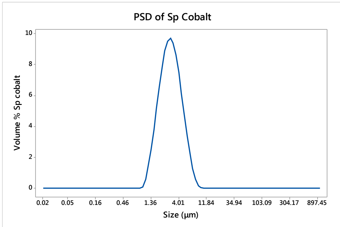
Figure 44: Particle size distribution of spherical cobalt.
