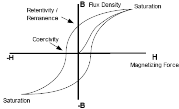
Figure 32: The area contained within the hysteresis loop has energy units and denotes the energy consumed during one complete reversal of the magnetization and back. A large hysteresis loop is desirable in hard permanent magnets, while the opposite applies to electrical transformer cores [60].
