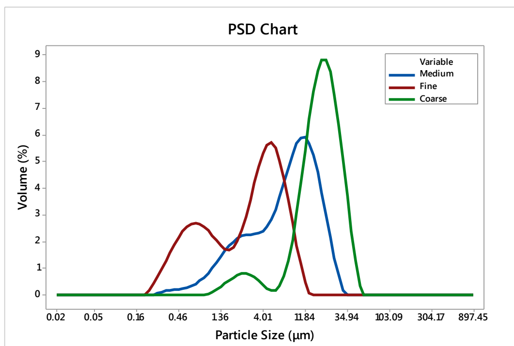
Figure 46: PSD of 3 different mixed diamond powders.
