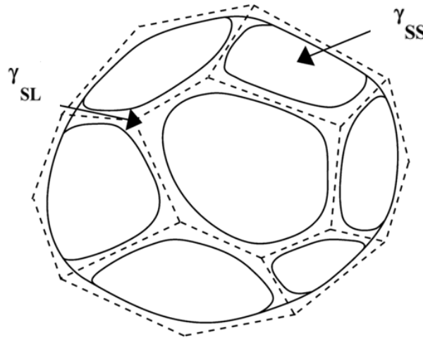
Figure 23: Grain shape change as fully density is reached during LPS [31].
