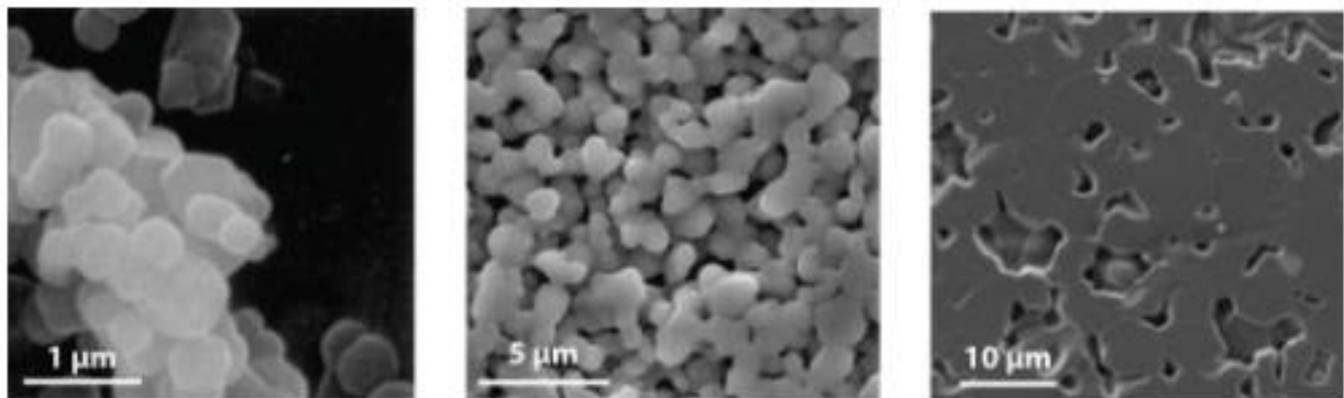
Figure 19: Micrograph of ceramic material sintering stages process when temperature increases. Left: Initial stage sintering, middle: Microstructure after sintering for two hours at 1250 °C (Less porosity than initial stage), and right: the microstructure after sintering for two hours at 1450 °C [32].
