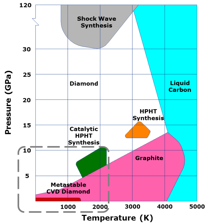
Figure 3: Phase diagram of carbon and graphite [18].
