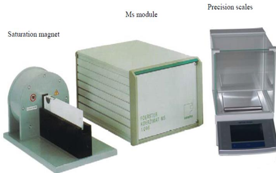
Figure 40: Magnetic Saturation Measuring Equipment Components.
