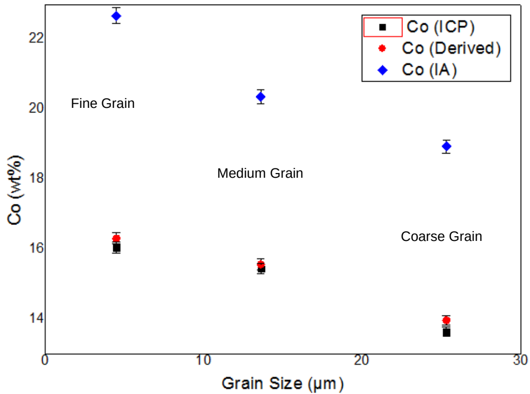
Figure 59: Relationship between ICP, IA and derived cobalt content and diamond grain size after sintering. The derived value was calculated using Archimedes immersion density values.
