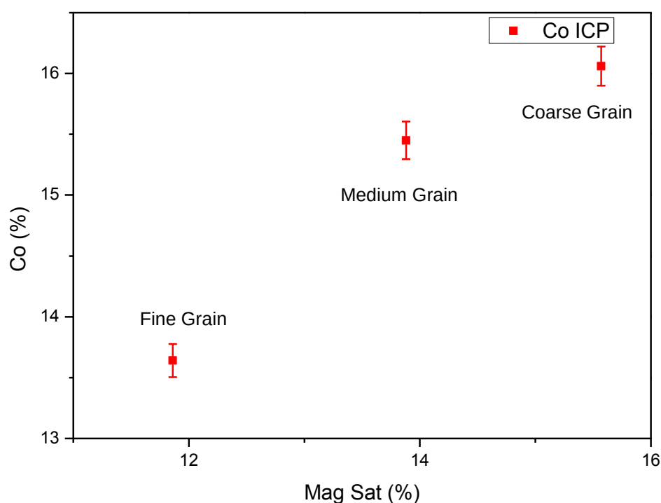
Figure 63: Relationship between magnetic saturation and ICP cobalt content after sintering.
