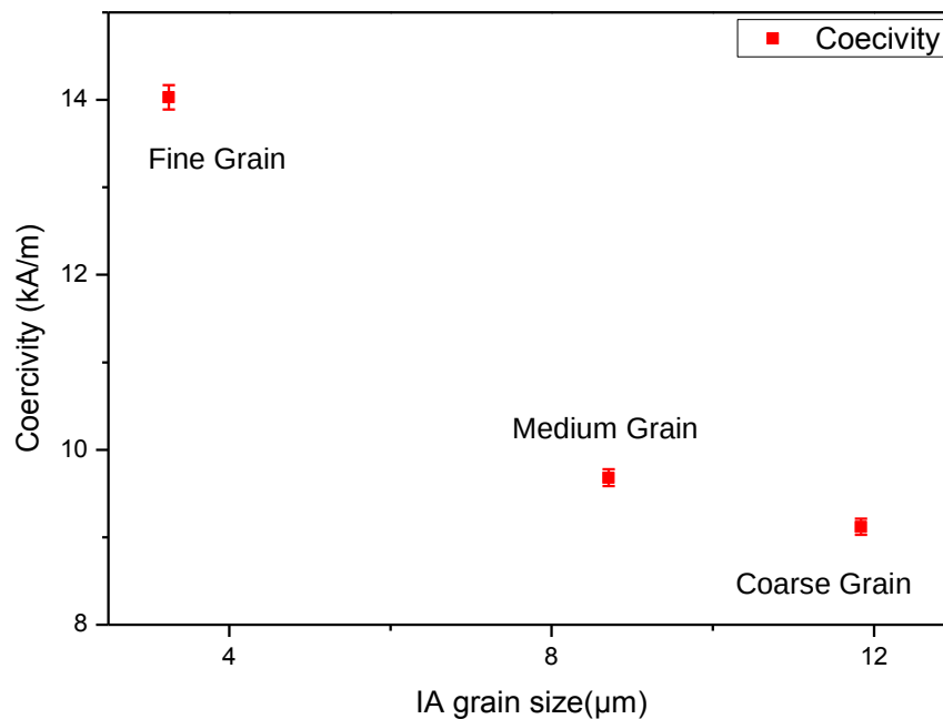
Figure 65: Relationship between coercivity and image analysis diamond grain size after sintering.
