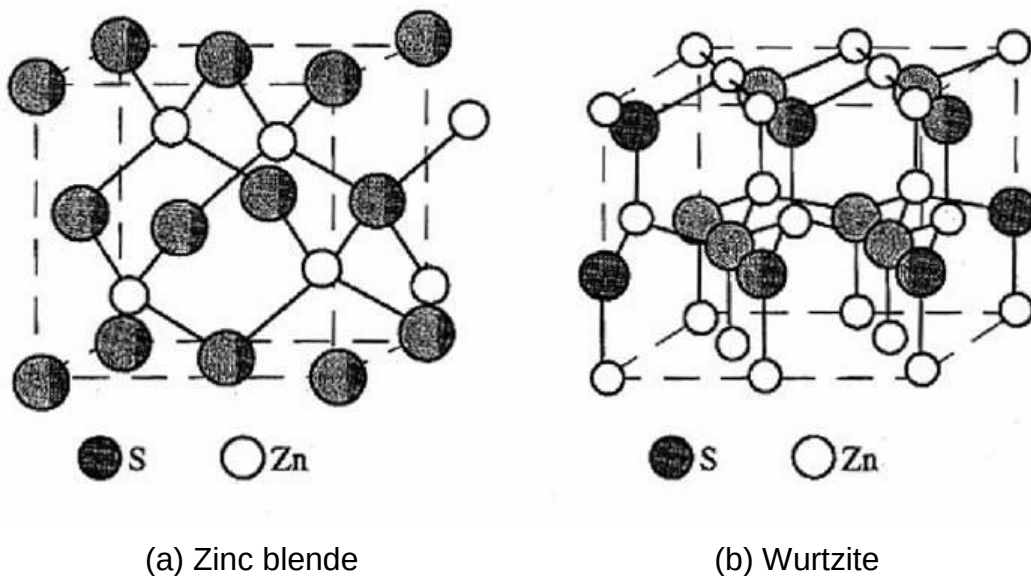
Figure 2: Correlation of the crystal structures of zinc blende with wurtzite [15].
