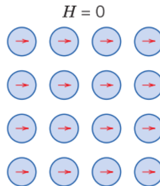
Figure 31: Schematic diagram of the mutual configuration of atomic dipoles for a ferromagnetic material [51].
