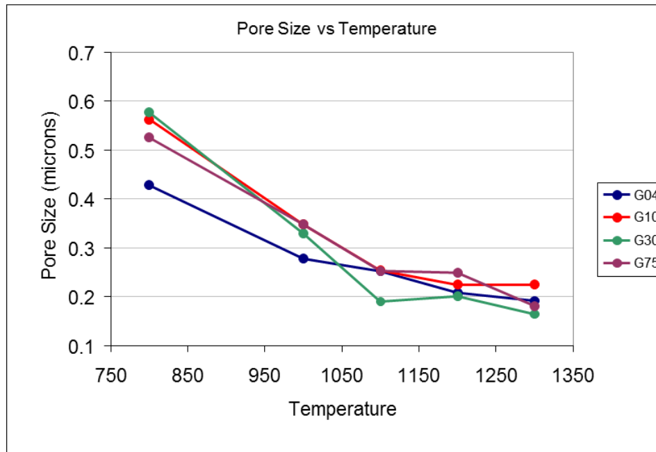
Figure 17: Pore size change during hot compaction as temperature is increased which maintain pressure at 5.5 GPa [29].
