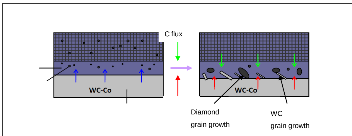
Figure 10: Diagram of the sintering of PDC materials [30].
