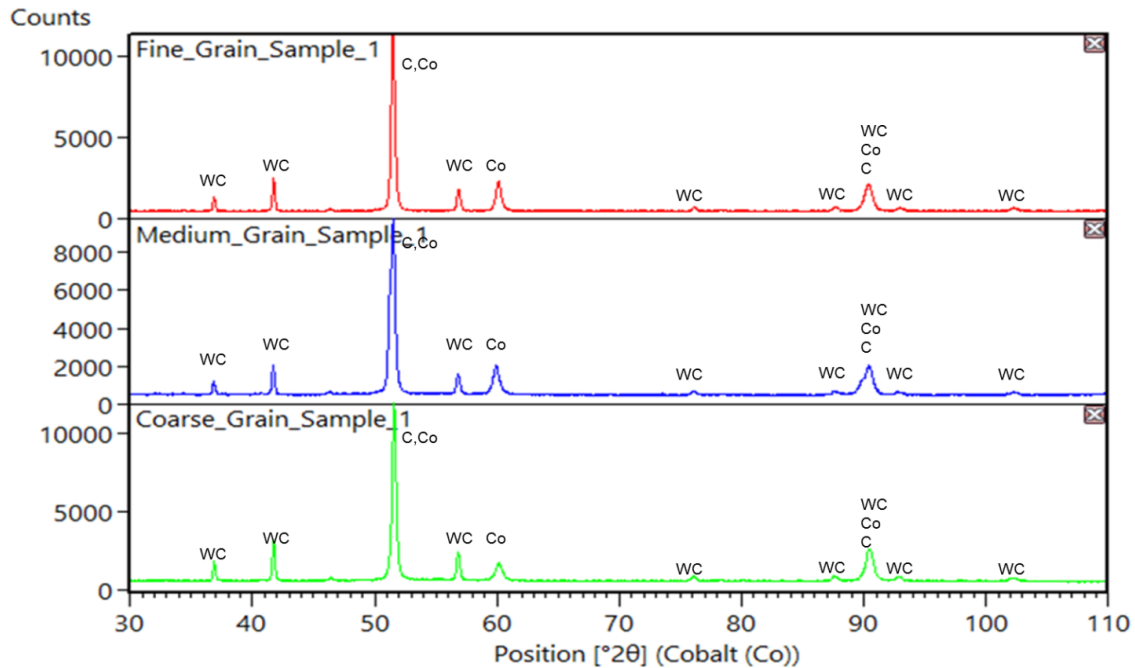
Figure 49: XRD spectra of fine, medium, and coarse grain diamond tables.
