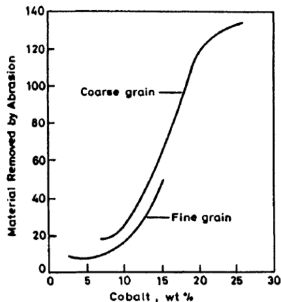
Figure 35: Influence of grain size and Co content on the abrasion resistance of WC-Co [69].
