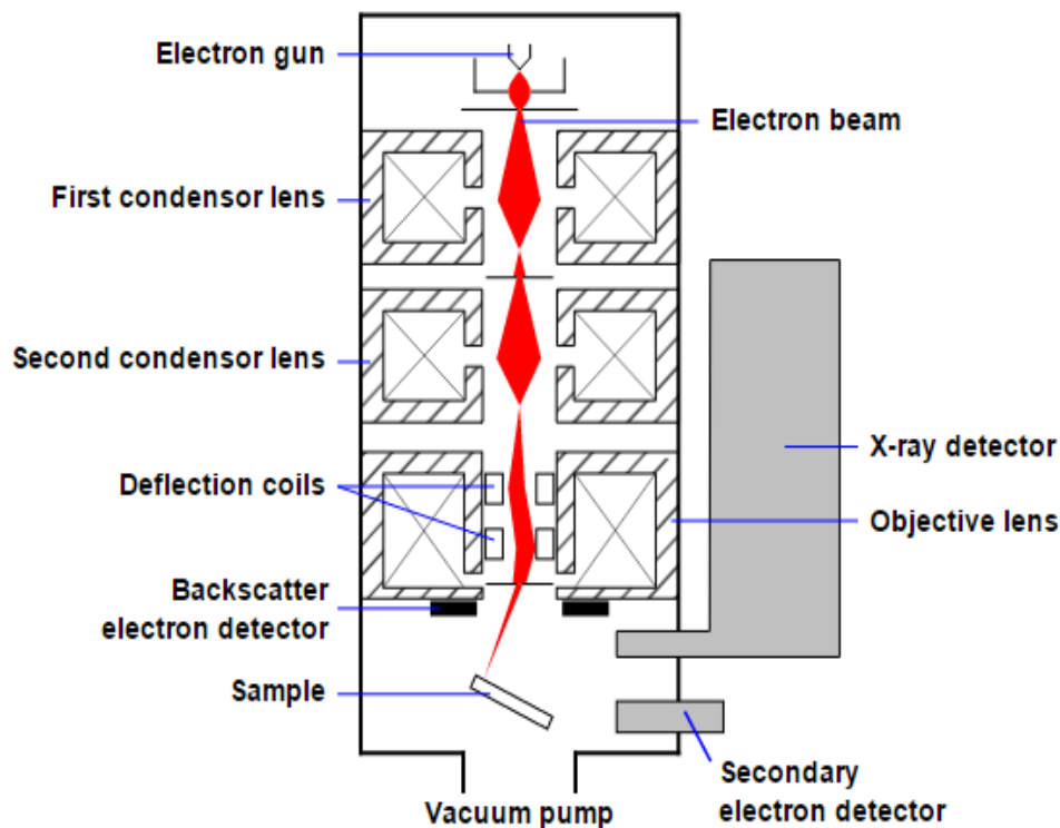
Figure 36: Schematic representation of an SEM [79].
