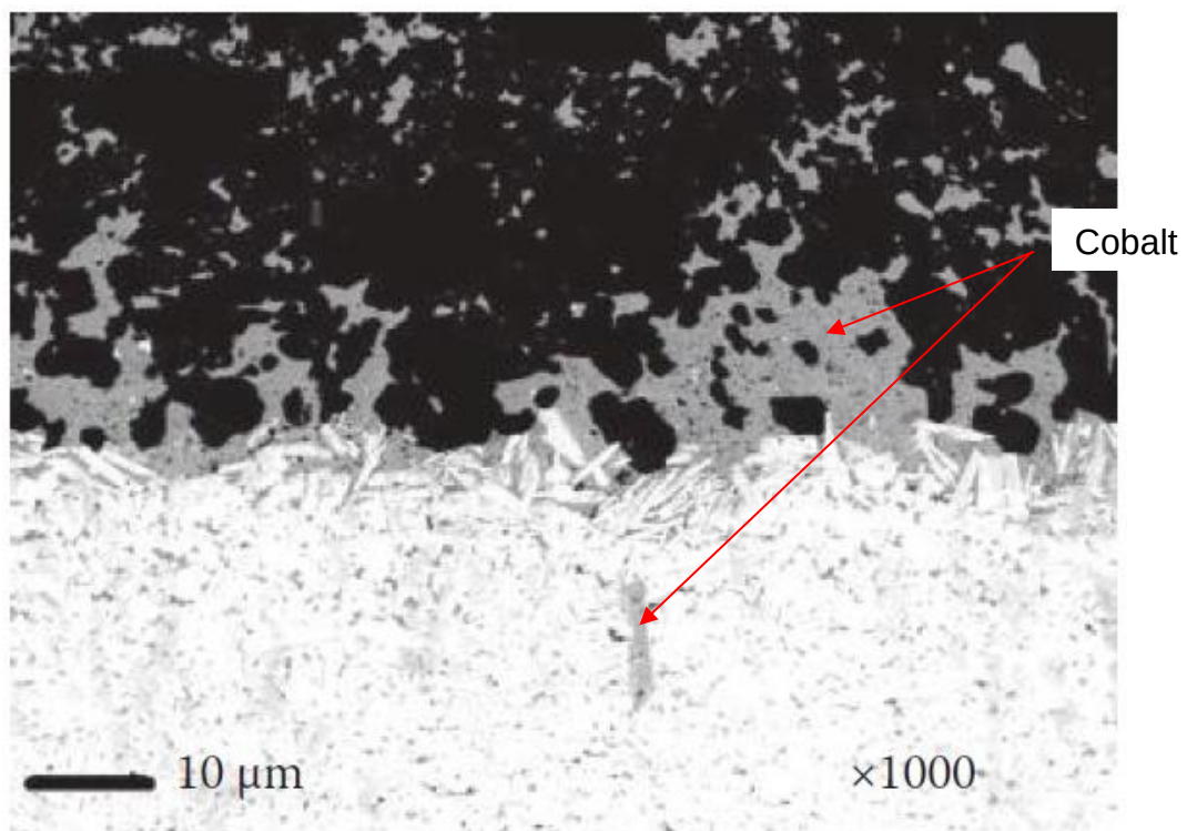
Figure 55: Micrograph of fully sintered PCD compact [10].
