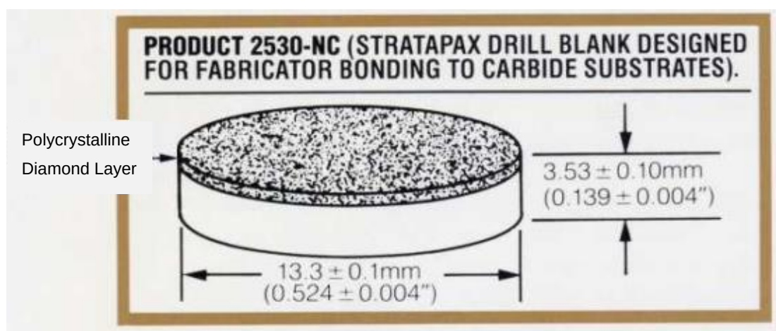
Figure 6: Early PDC diamond layer and substrate [26].
