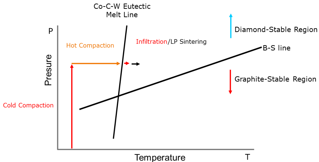
Figure 8: PDC sintering schematic trajectory [29].
