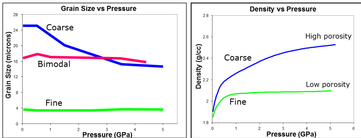
Figure 13: Graph representation of densification taking place during cold compaction [29].
