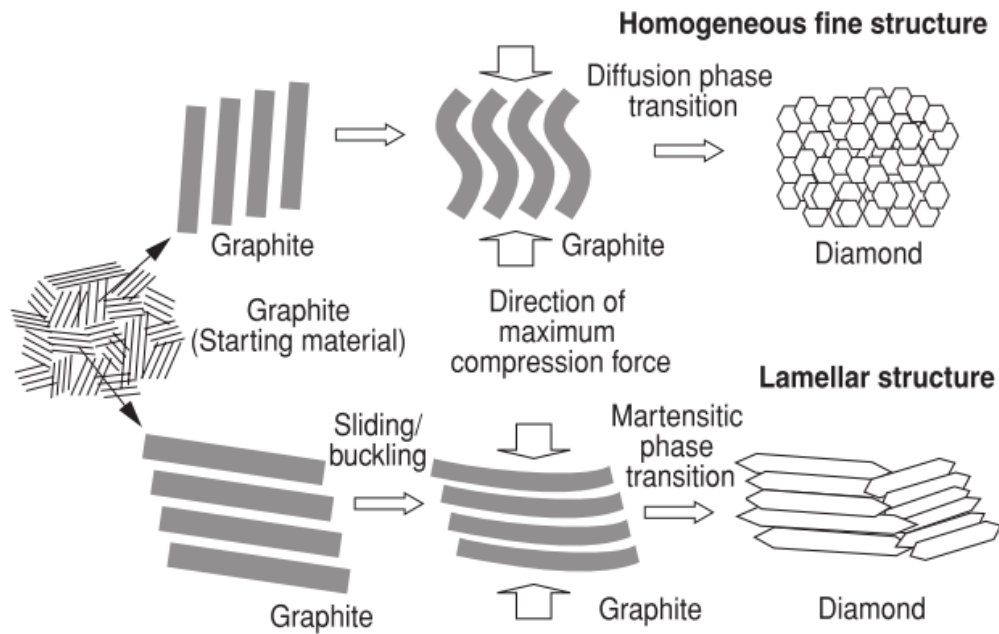
Figure 4: Schematic diagram of the direct conversion of graphite to diamond [19].
