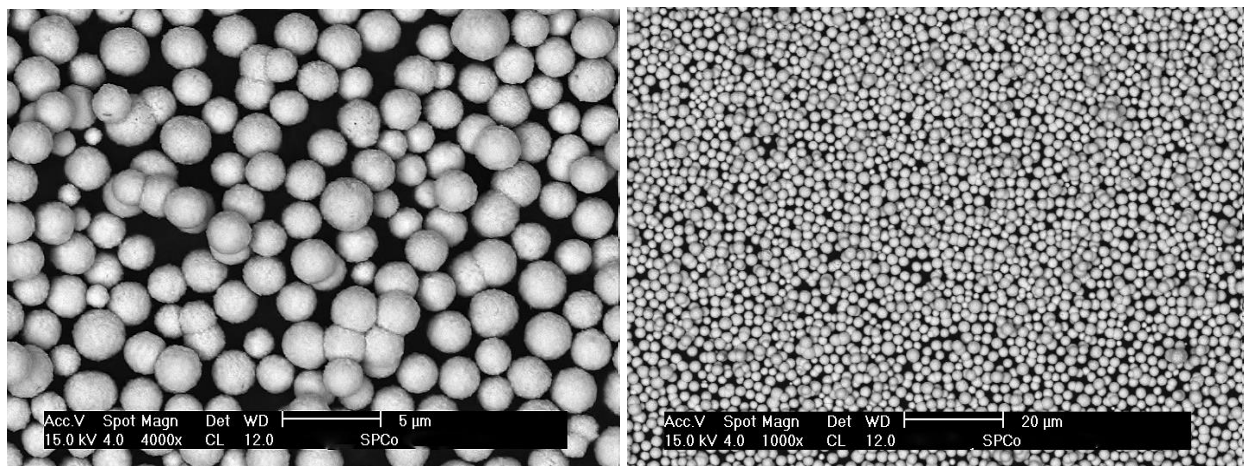
Figure 45: Micrographs of spherical cobalt.
