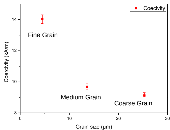
Figure 53: Coercivity results versus grain size of each variant.
