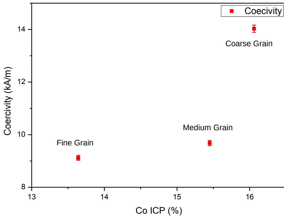
Figure 68: Relationship between coercivity and cobalt content from ICP after sintering.
