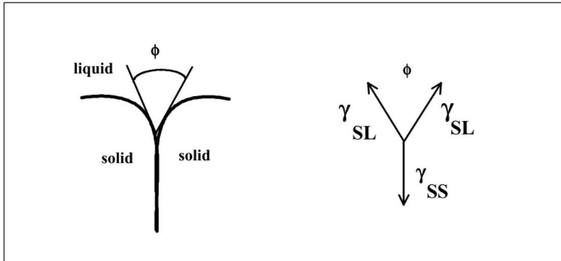
Figure 22: Figure of dihedral angle in a solid/liquid system [42].
