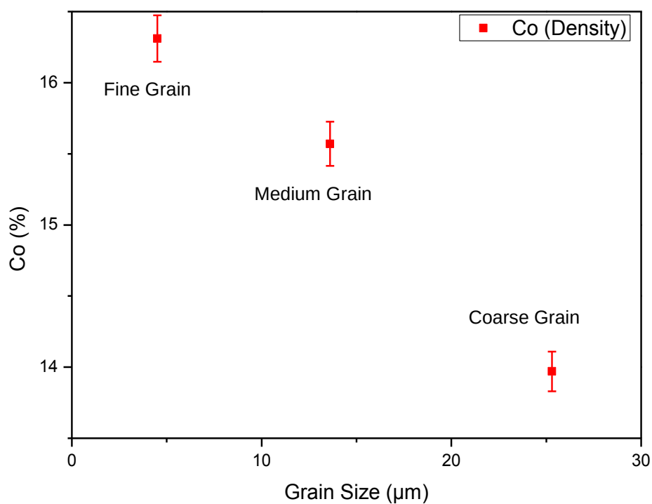
Figure 54: Grain size versus Co content from derived densities. This includes the effect of heavy WC in the PCD table as were clearly shown by XRD analysis.
