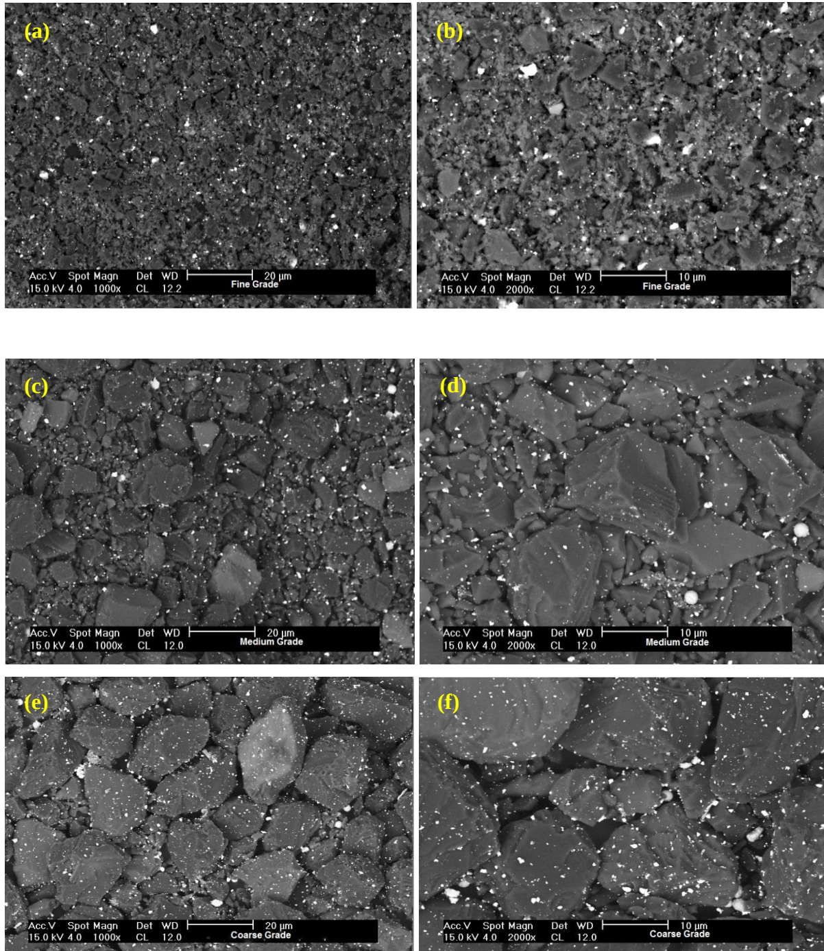
Figure 47: Micrographs of fine ((a) and (b)), medium ((c) and (d)) and coarse ((e) and (f)) diamond powders. These micrographs were captured at 1000x and 2000x magnification respectively for each size.
