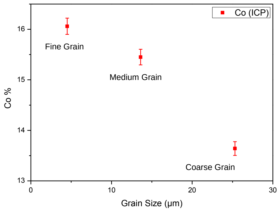
Figure 50: Cobalt content given by ICP in Wt% versus diamond grain size.
