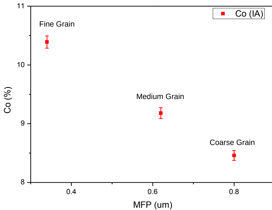
Figure 62: Relationship between MFP and Co (IA) content after sintering.
