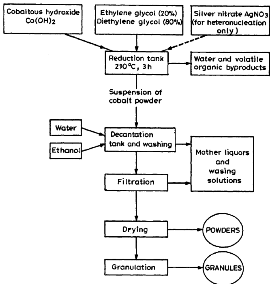
Figure 34: Flow diagram of the production of cobalt powders and granules [69].
