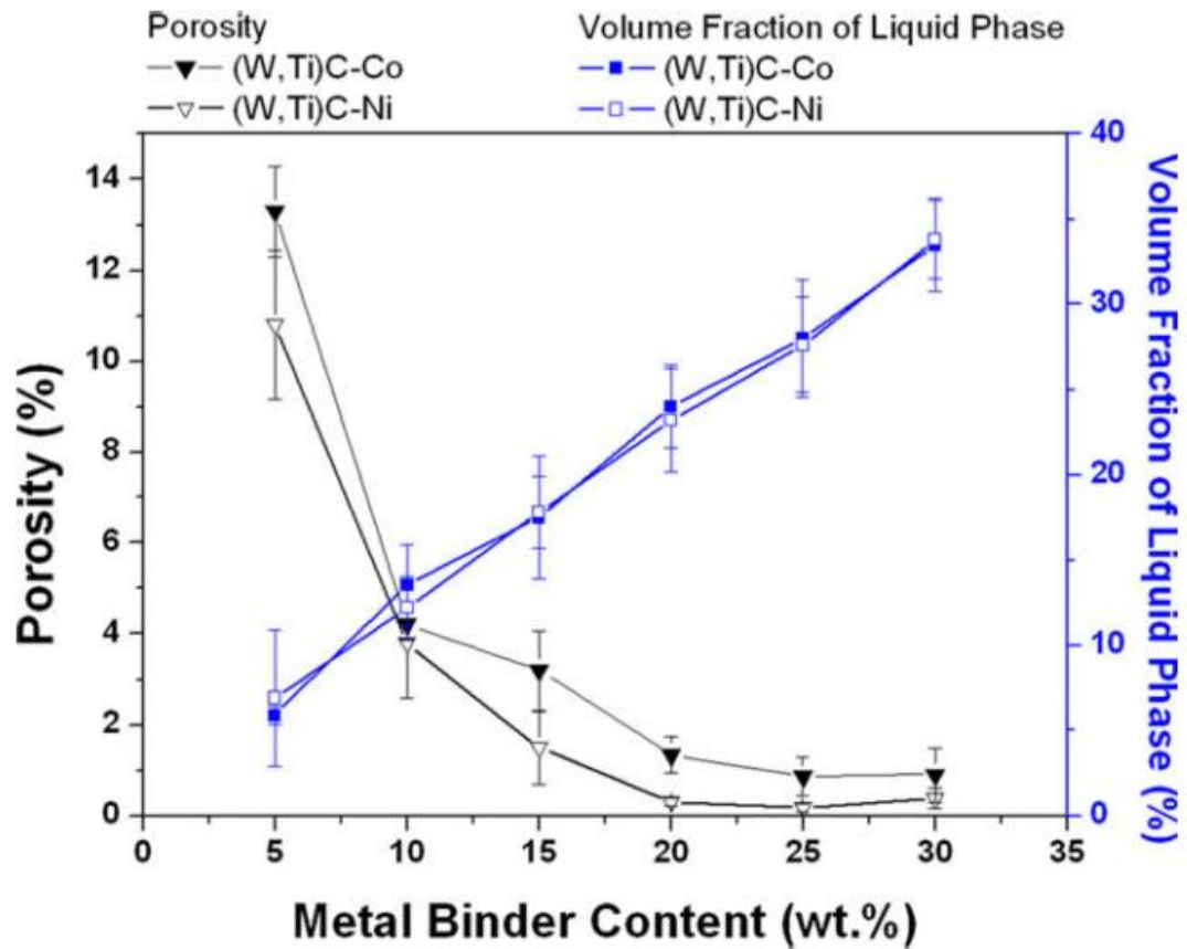
Figure 67: Influence of the composition of the metal binder on the porosity and the volume fraction of the binder of the (W,Ti)C–Co and (W,Ti)C–Ni cemented carbides [86].
