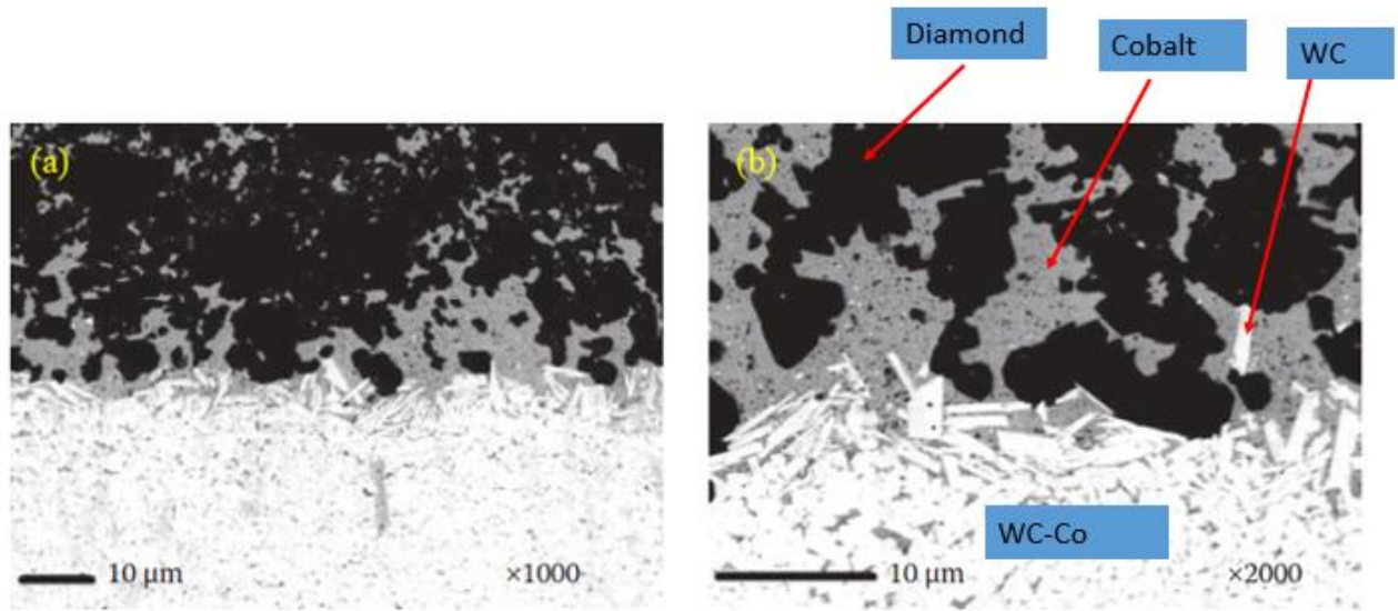
Figure 11: SEM micrographs of a polished section showing interface and bulk of PCD [10].
