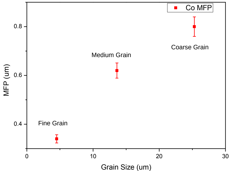
Figure 61: Relationship between MFP and diamond grain size.
