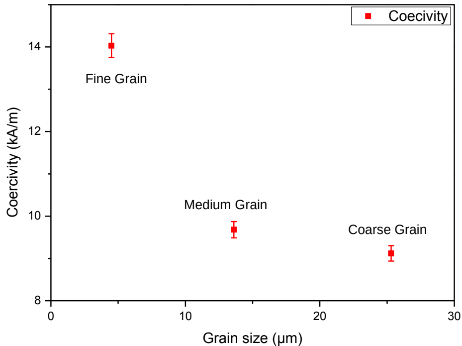
Figure 64: Relationship between coercivity and diamond grain size after sintering.
