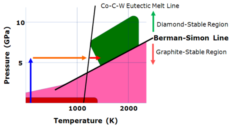
Figure 5: Catalytic HPHT Synthesis [18].
