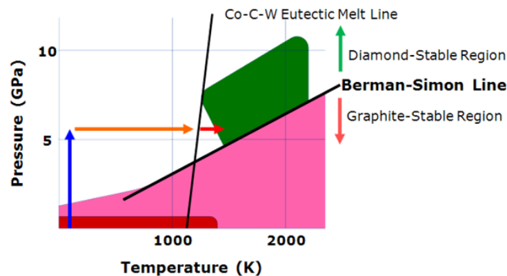
Figure 24: Phase diagram showing cobalt melt line and LPS of PCD sintered Structures [18].
