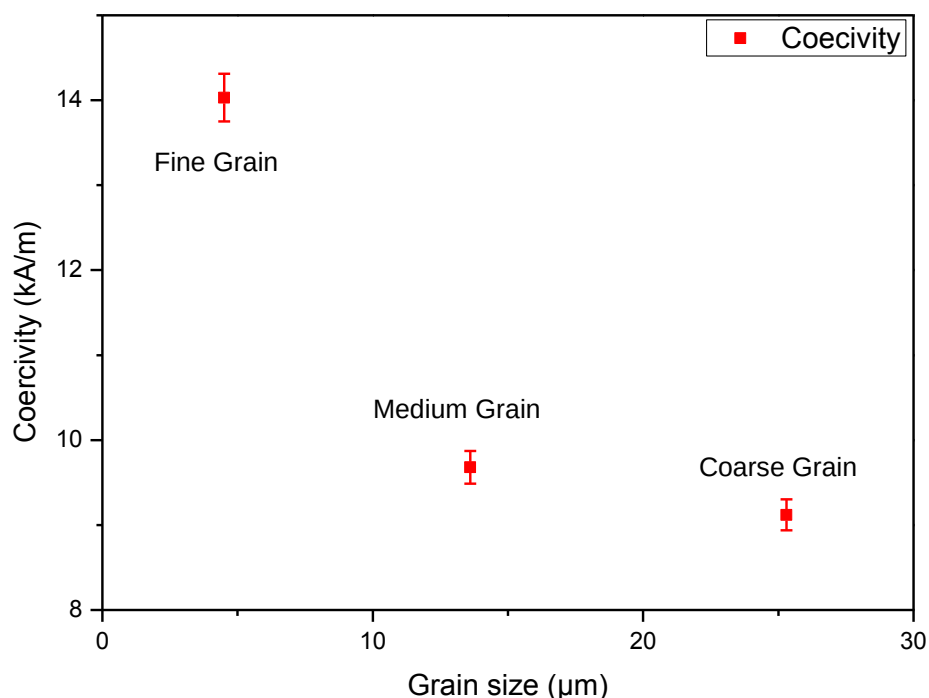
Figure 58: Relationship between coercivity and diamond grain size after sintering.
