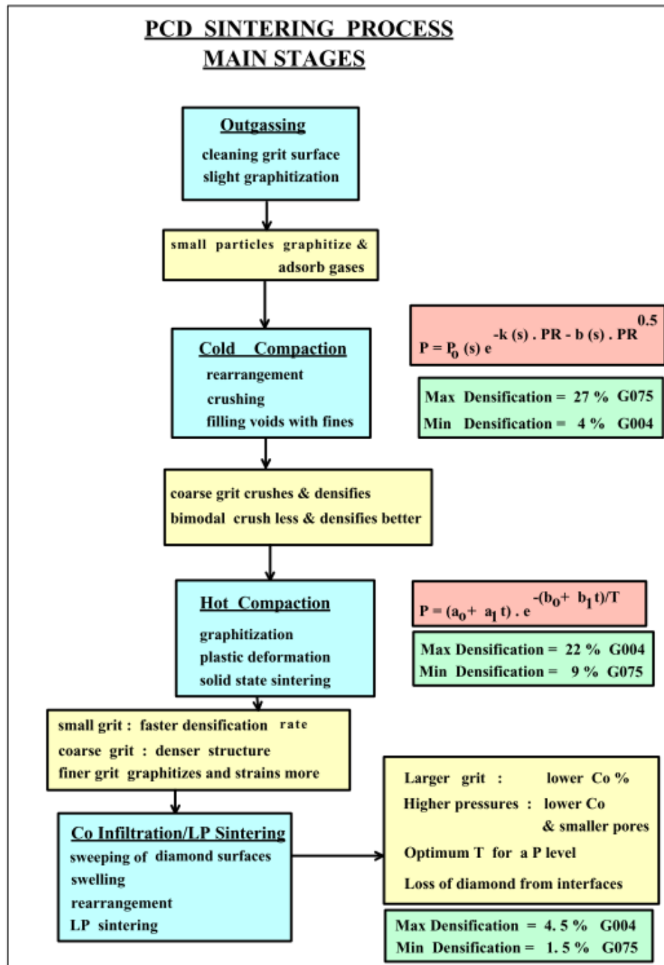
Figure 38: Process steps during sintering [47].
