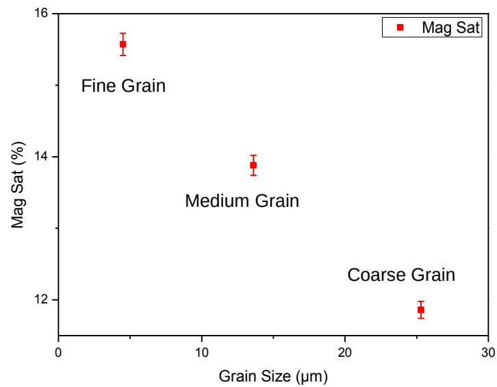
Figure 52: Saturation magnet versus grain size of each variant.
