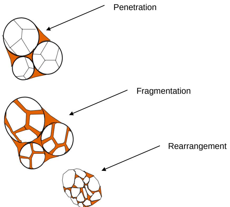
Figure 14: Illustration of rearrangement and fragmentation of polycrystalline particles leading to secondary rearrangement [29].
