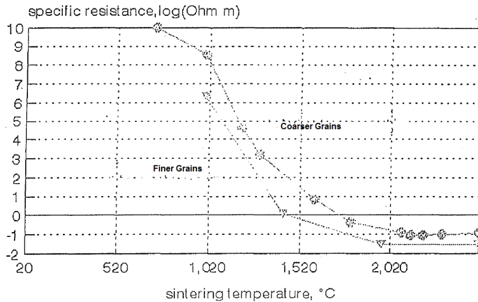
Figure 18: Change in specific resistance of diamond compacts with sintering temperature [29].
