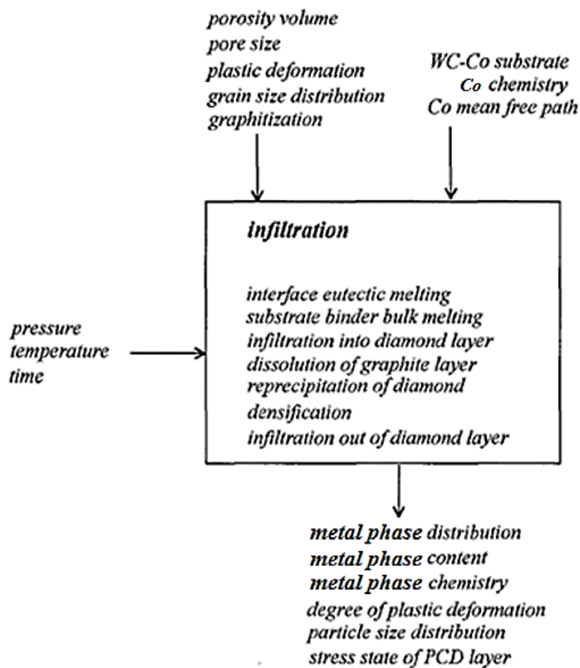
Figure 20: Critical Parameters and Processes in Liquid Phase Sintering [29].
