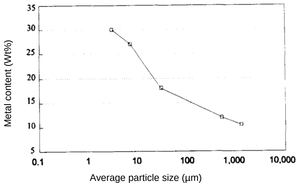
Figure 26: Cobalt content in PCD layers as a function of grain size [35].
