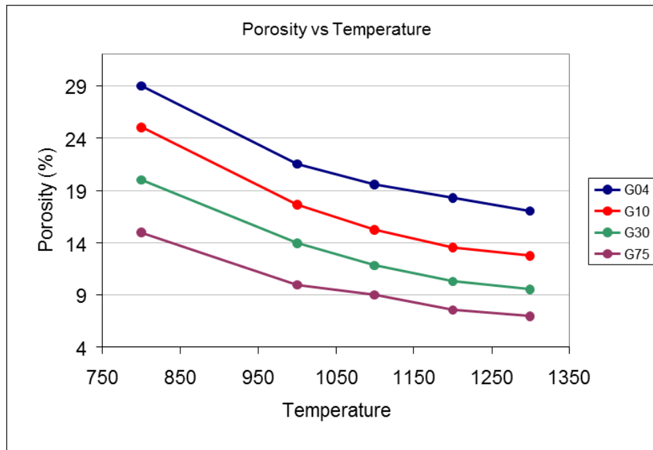
Figure 16: Porosity versus temperature during hot compaction at 5.5 GPa [29].
