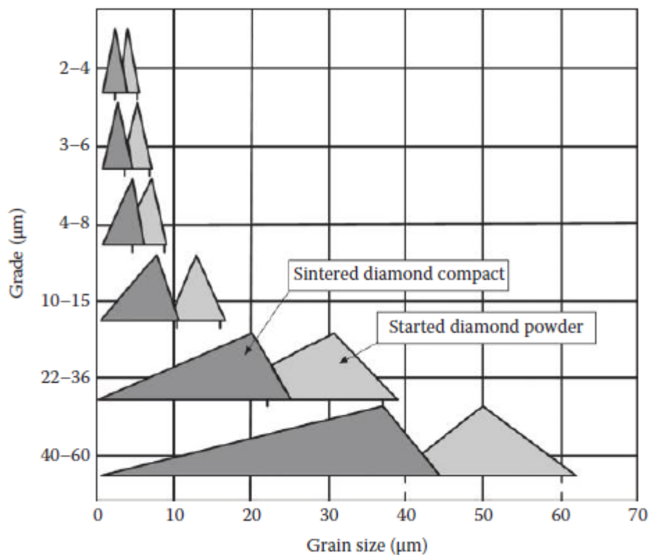
Figure 7: Schematic diagram showing the relationship between the grain size of diamond before and after sintering [10].
