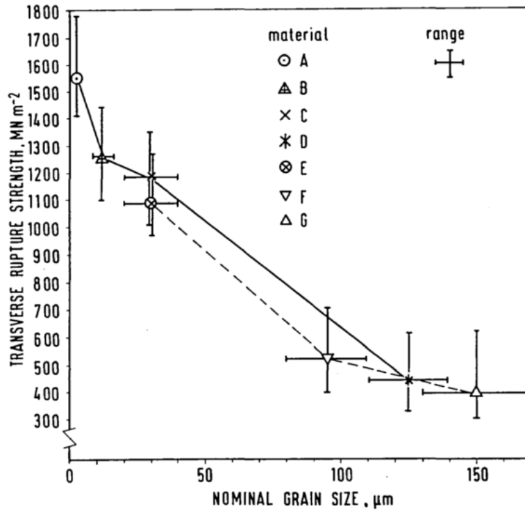
Figure 27: TRS of Polycrystalline Diamond layers as a function of grain size [25].
