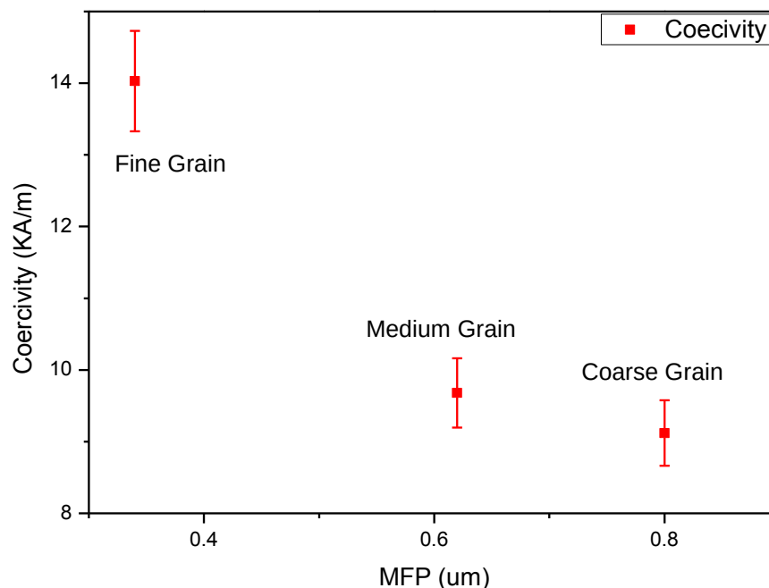
Figure 60: Correlation of coercivity and Co mean free path (MFP) (μm).
