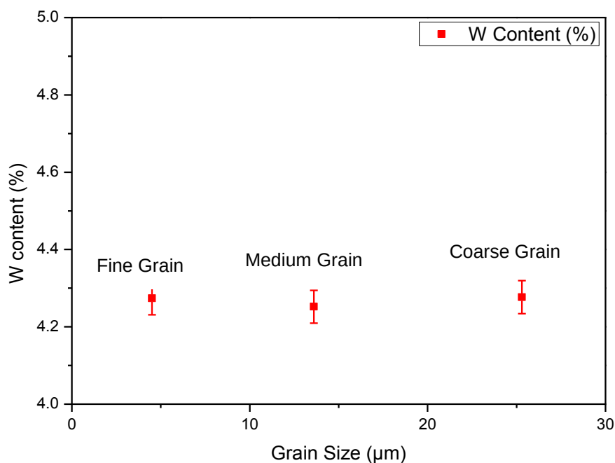
Figure 51: Dissolved Tungsten content in PCD of each variant given by ICP in wt%.
