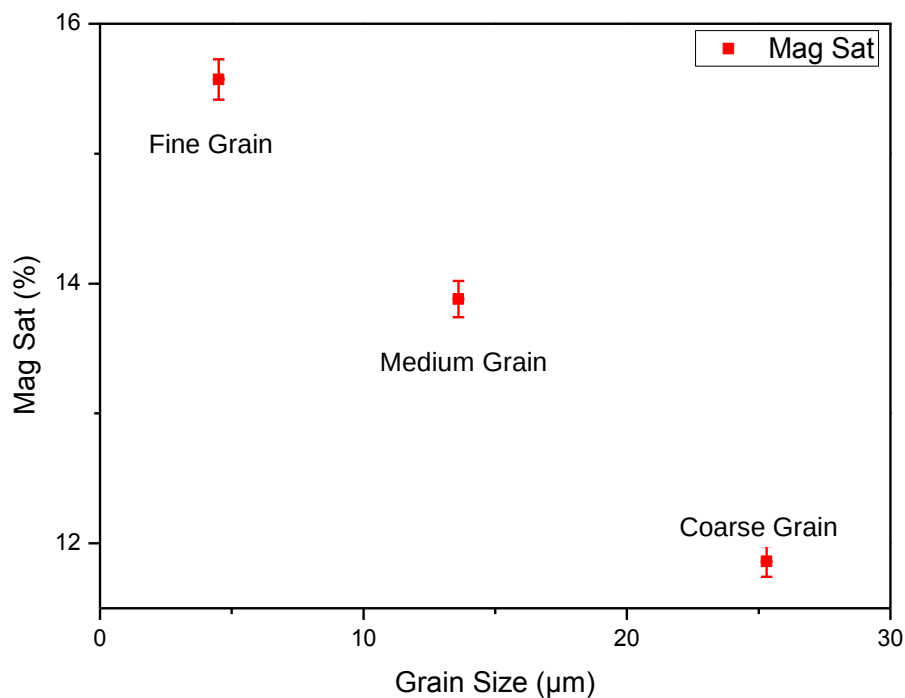
Figure 57: Relationship between magnetic saturation and diamond grain size after sintering.
