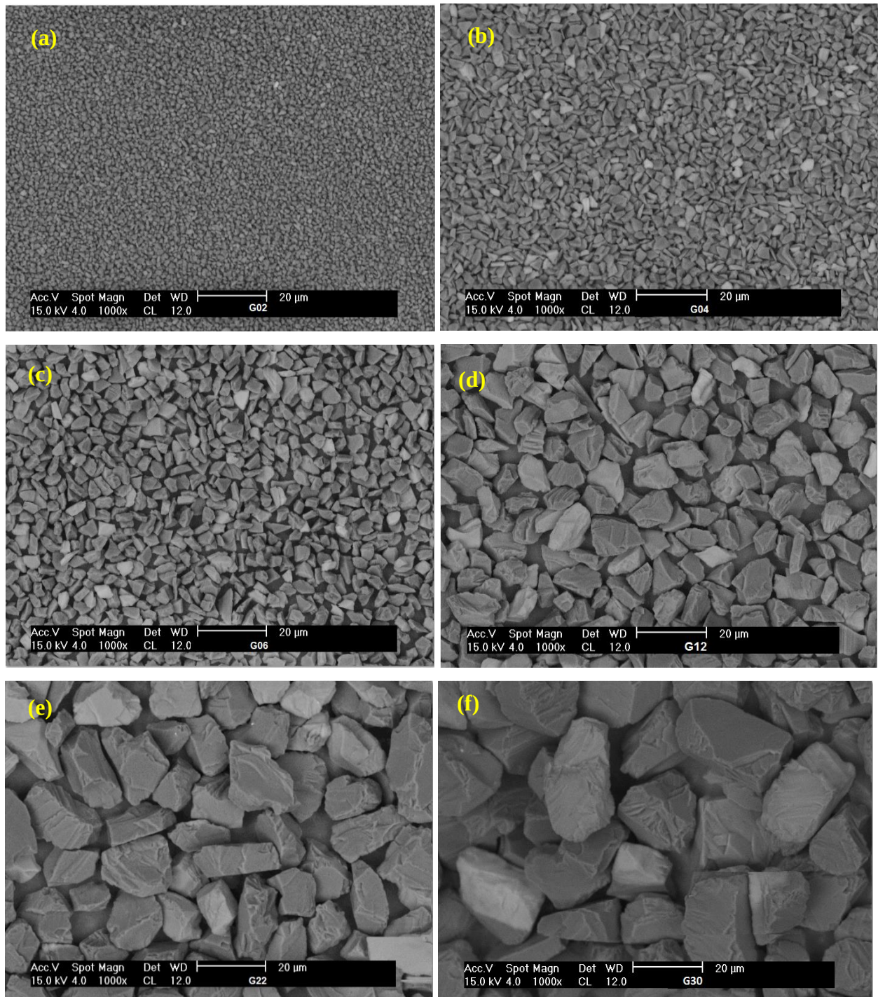
Figure 43: Micrographs of (a) G02, (b) G04, (c) G06, (d) G12, (e) G22, and (f) G30 constituent grades.
