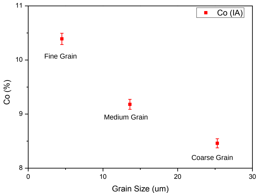
Figure 66: The relationship between cobalt calculated by IA and diamond grain size after sintering.
