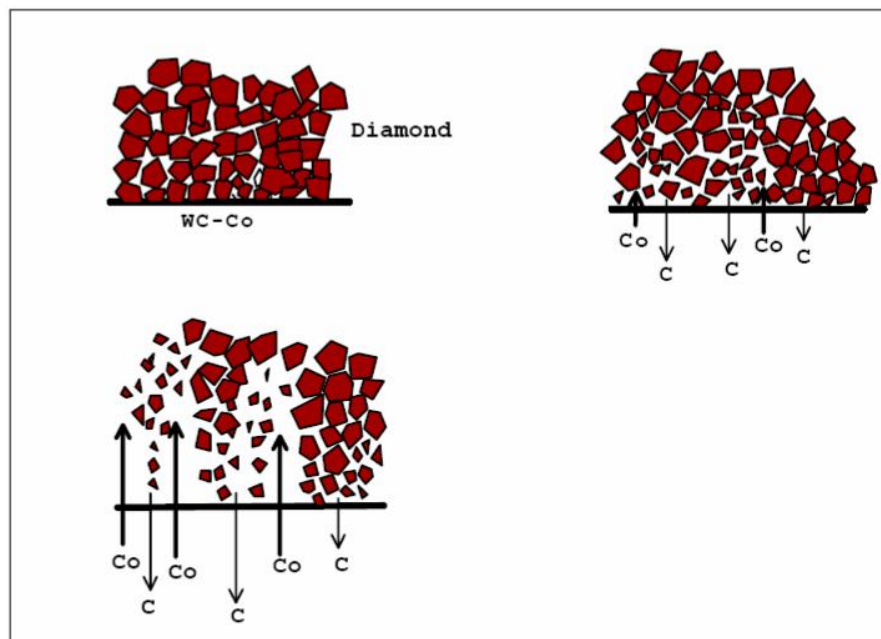
Figure 9: Selective dissolution of diamond grains in infiltrating Co causing "river marks" in the regions next to interface [29].
