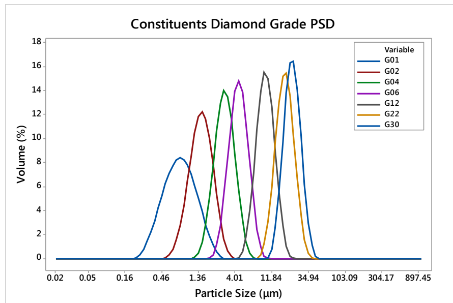
Figure 42: Constituent Diamond Grade PSD.
