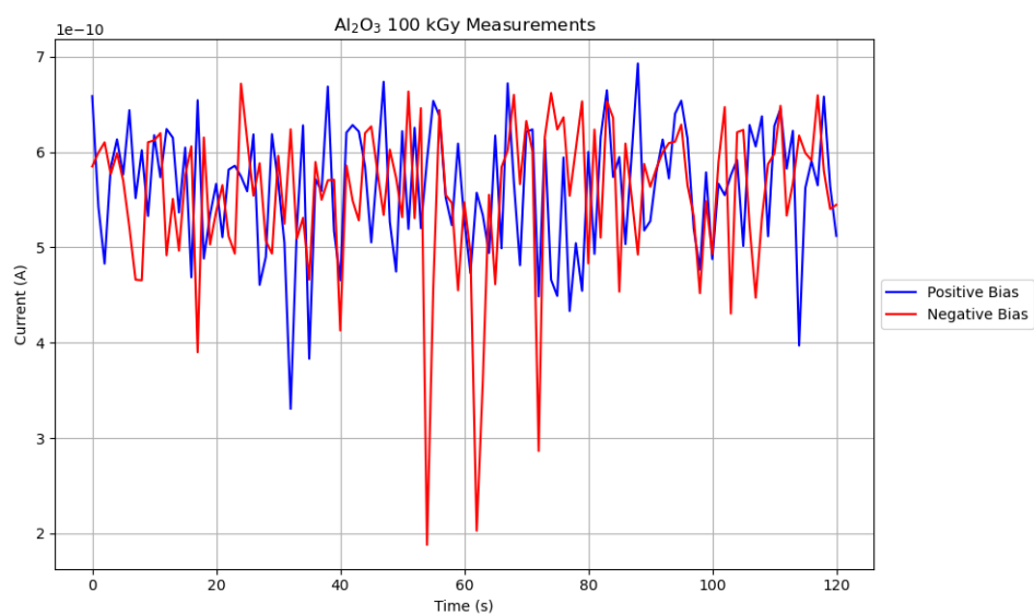
Figure 5.22: Measured current under positive and negative applied voltage bias for Aluminium Oxide samples with an absorbed gamma radiation dose of 100 kGy.
