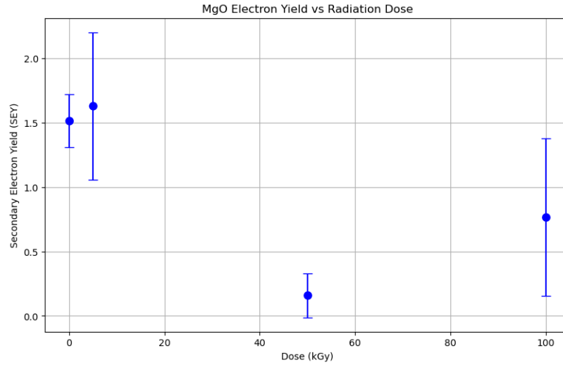
Figure 5.26: This figure presents the variation in electron emission yield of Magnesium Oxide as a function of radiation dose, illustrating how the material's electron emission yield responds to increasing gamma radiation exposure.
