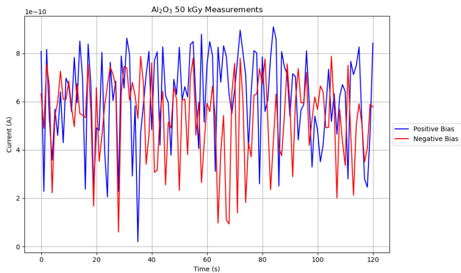
Figure 5.21: Measured current under positive and negative applied voltage bias for Aluminium Oxide samples with an absorbed gamma radiation dose of 50 kGy.
