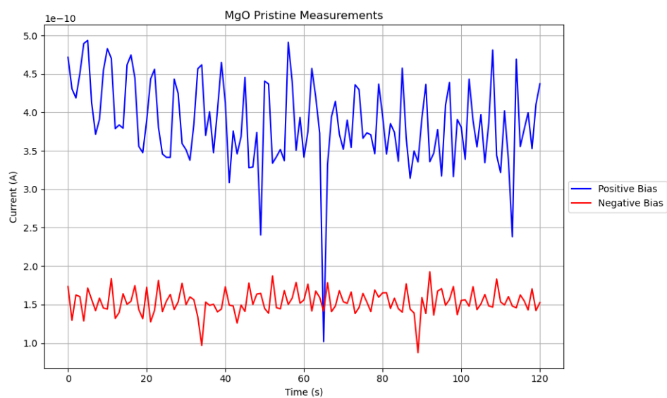
Figure 5.15: Measured current under positive and negative applied voltage bias for pristine Magnesium Oxide.
