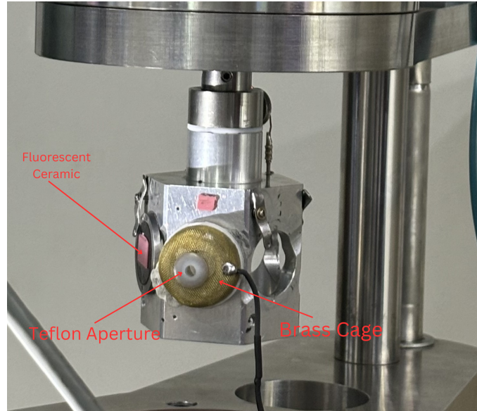
Figure 4.10: Microprobe Carousel Setup: Showing the Teflon aperture, brass cage, and a fluorescent ceramic.
