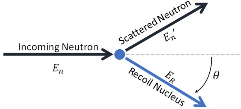
Figure 2.4: Incident neutron with energy E_n elastically scattering off of the target nucleus, the result of this interaction is the recoiling of the target nucleus with an energy E_R . deflected by angle \theta and the scattered neutron with energy E_n' [13].
