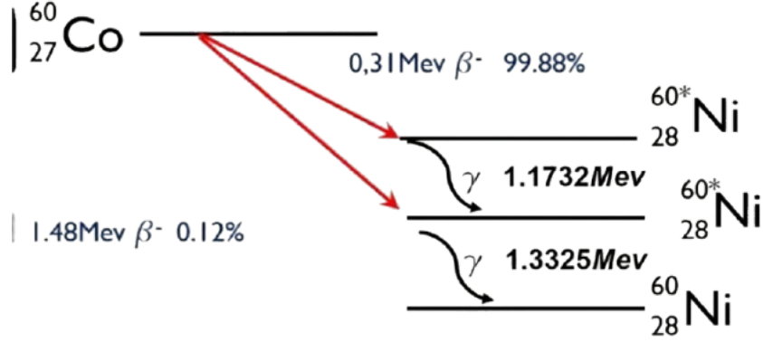
Figure 4.4: This figure illustrates the decay pathway of Cobalt-60 ( ^{60}_{27}\text{Co} ) to the ground state of Nickel-60 ( ^{60}_{28}\text{Ni} ). This image illustrates the two possible decay pathways (given by the two red lines) and the energies of the electrons emitted for both possible pathways as well as the energies of the gamma-rays emitted at each stage [39].
