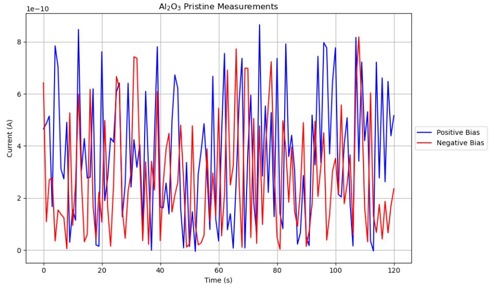
Figure 5.19: Measured current under positive and negative applied voltage bias for pristine Aluminium Oxide.
