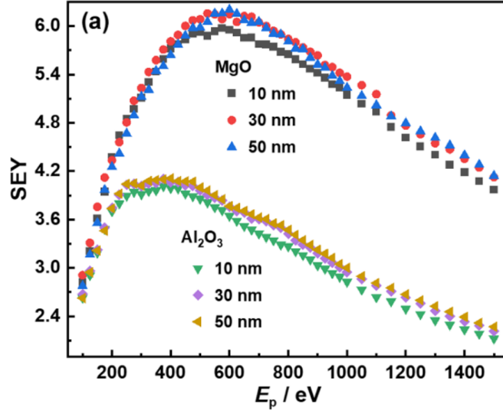
Figure 5.28: Secondary electron yield as a function of the primary electron energy for Aluminium Oxide and Magnesium Oxide thin films at varying film thickness [52].
