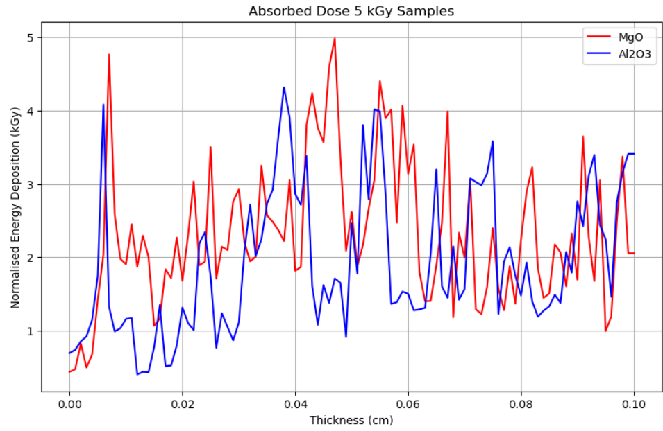
Figure 5.7: Simulated absorbed dose from a 70 TBq Co-60 source placed 88.00 \text{ cm} \pm 0.05 \text{ cm} away from the target for 6.846 \pm 0.00001 days for the two samples.
