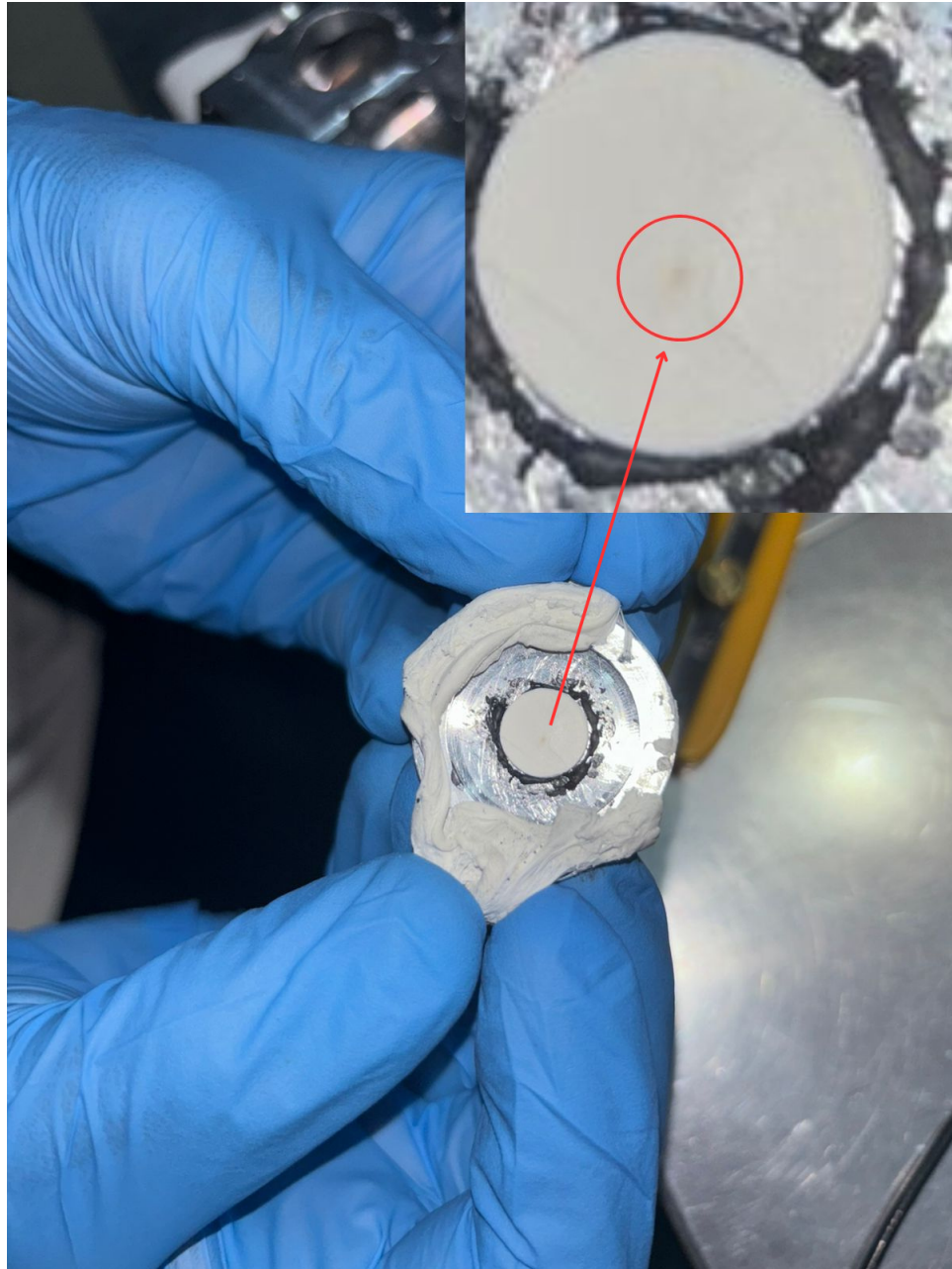
Figure 4.13: \text{Al}_2\text{O}_3 sample mounted on a metallic disc using graphite-based conductive paste, with a temporary rubber adhesive securing the brass cage over the sample.
