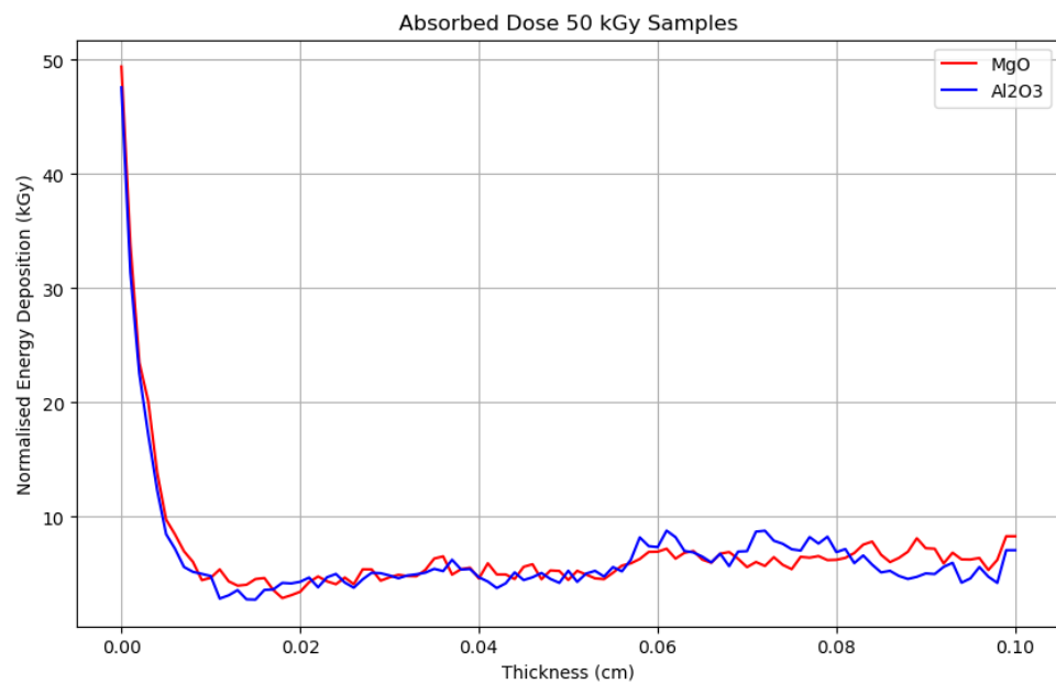
Figure 5.8: Simulated absorbed dose from a 70 TBq Co-60 source placed at a distance of 80.00 cm \pm 0.05 cm from the target for 10.825 \pm 0.00001 days and then placed at 20.00 \pm 0.05cm from the target for 3.919 \pm 0.00001 days for the two samples.
