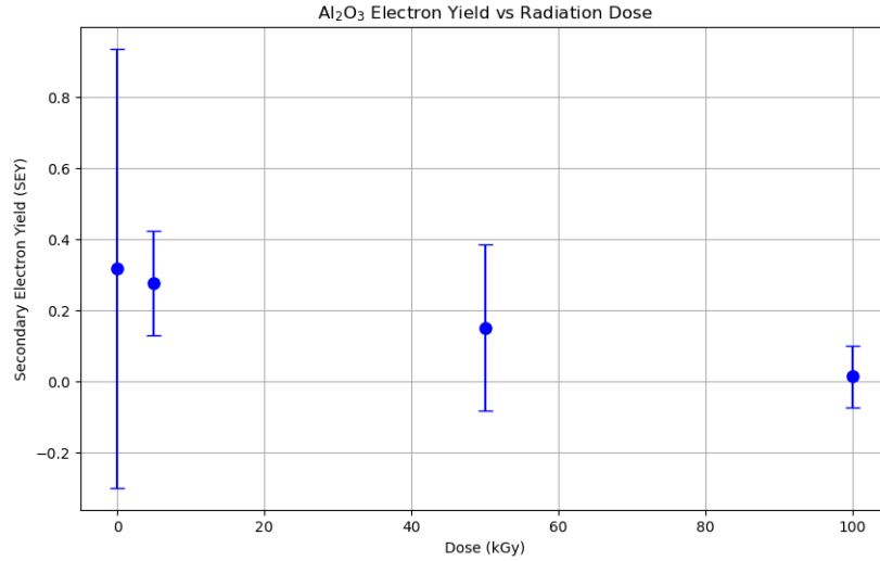
Figure 5.25: This figure presents the variation in electron emission yield of Aluminium Oxide as a function of radiation dose, illustrating how the material's electron emission yield responds to increasing gamma radiation exposure.
