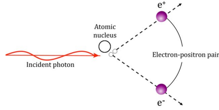
Figure 2.3: Pair production process.
