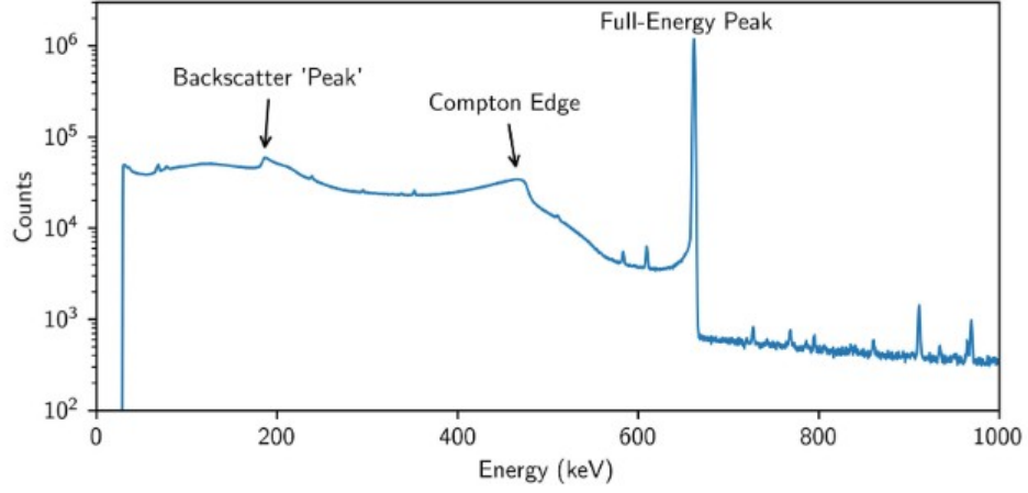
Figure 2.2: The following gamma-ray spectroscopy measurement displays a phenomenon known as the Compton Edge [18], this feature is due to the fact that the photons in this region have been scattered off of the atomic electrons of the target. This edge represents the maximum energy transfer that an incident photon can impart onto an atomic electron in a single scattering event.
