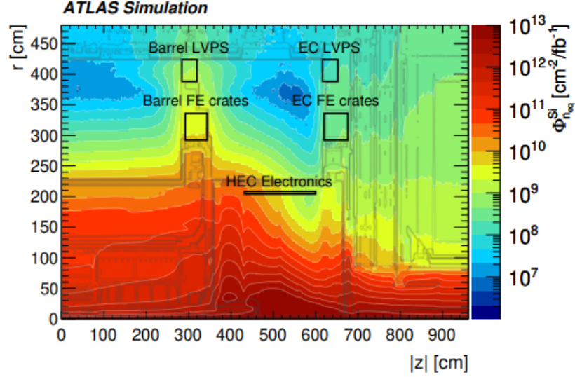
Figure 4.2: Radiation levels which the electronics found in the calorimeter systems in the ATLAS detector are subjected to [8]. Here FE crates are the "Front-End" crates which house readout electronics and LVPS refers to the "Low Voltage Power Supplies".
