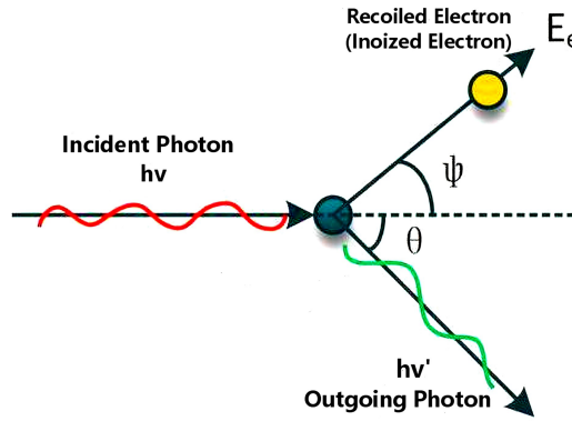
Figure 2.1: Compton Scattering process.
