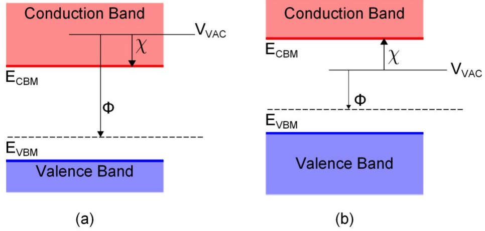
Figure 3.1: Energy band diagrams, (a) Positive EA (b) Negative EA [24].
