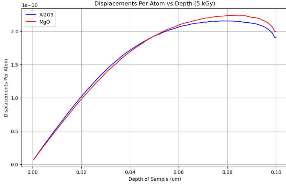
Figure 5.4: Simulated DPA from a mono-energetic photon source (1.25 MeV) placed 88.00 \text{ cm} \pm 0.05 \text{ cm} away from the target for 6.846 \pm 0.00001 days for the two samples. Please note the scaling factor shown in the top left corner of the plot, and keep this in mind throughout the remainder of this thesis.
