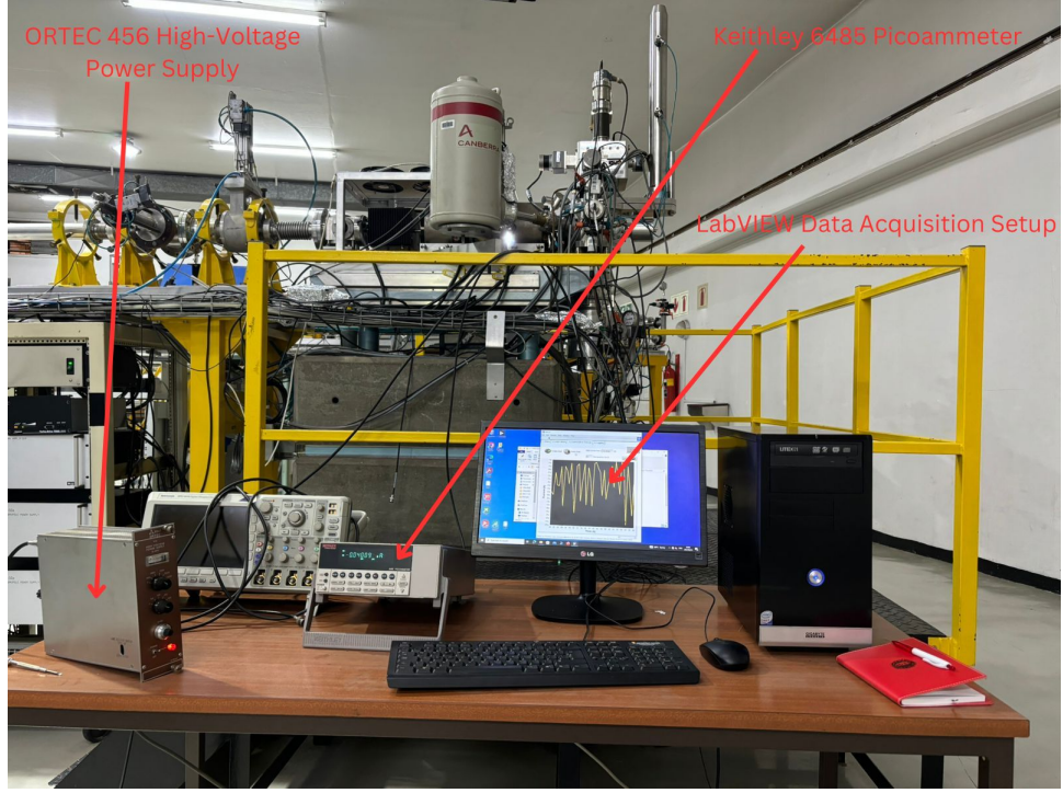
Figure 4.14: Data Acquisition Setup.
