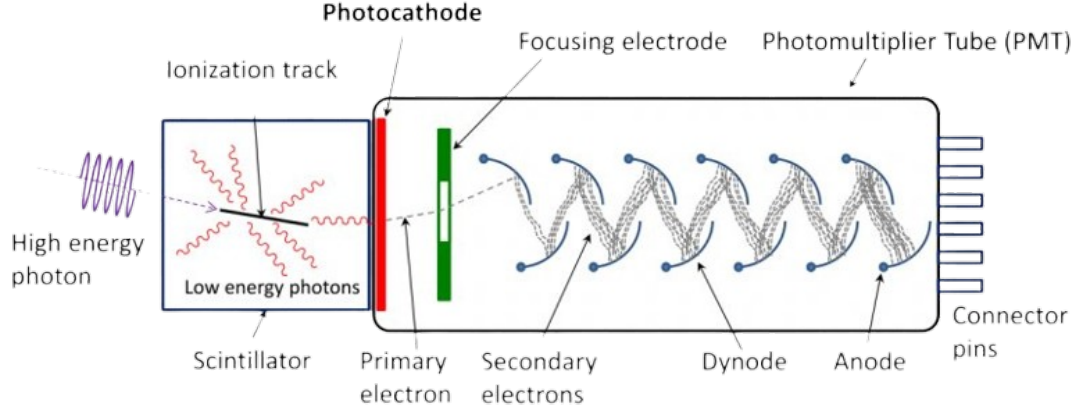
Figure 1.1: Photomultiplier tube.
