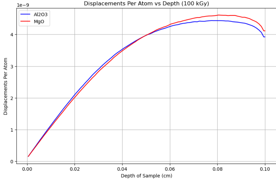
Figure 5.6: Simulated DPA from a mono-energetic photon source (1.25 MeV) placed at a distance of 20.00 \text{ cm} \pm 0.05 \text{ cm} from the target for 10.828 \pm 0.00001 days for the two samples.
