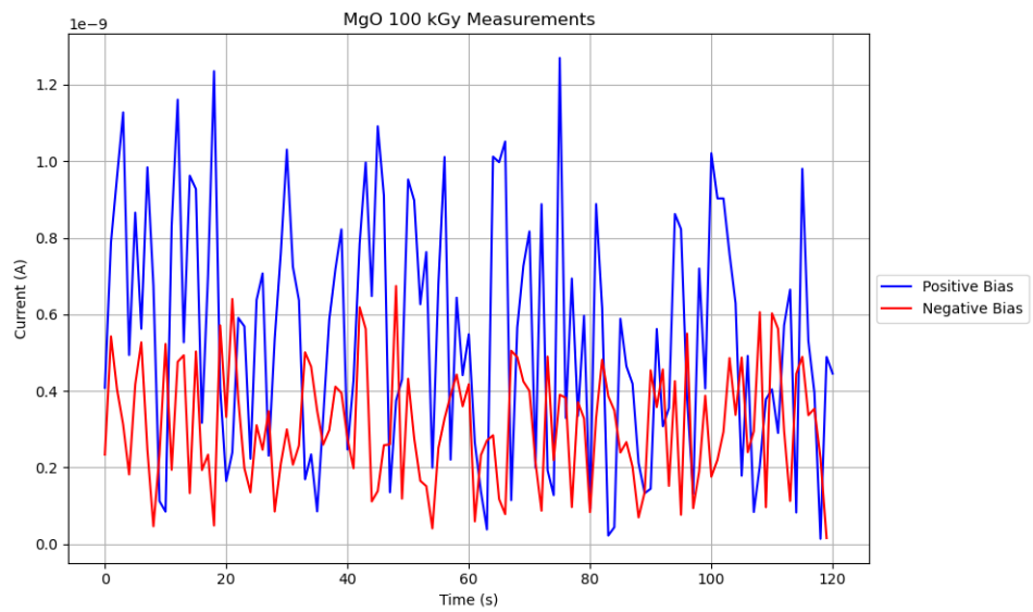
Figure 5.18: Measured current under positive and negative applied voltage bias for Magnesium Oxide samples with an absorbed gamma radiation dose of 100 kGy.
