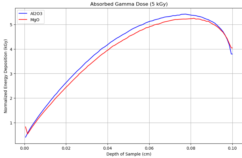
Figure 5.1: Simulated absorbed dose from a mono-energetic photon source (1.25 MeV) placed 88.00 \pm 0.05 cm away from the target for 6.846 \pm 0.00001 days for the two samples.
