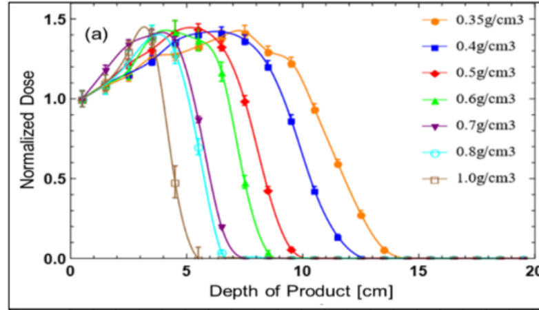
Figure 5.13: This figure serves as a reference for the normalized dose (Gy) distribution of a 10 MeV electron beam, exhibiting characteristics similar to those observed in the final simulations presented above [49]. Although the material densities used in the referenced figure are higher than those employed in this study, the figure is included to demonstrate the simulation's ability to reproduce experimental trends.
