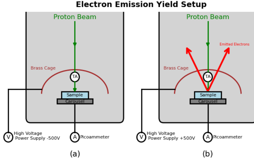
Figure 4.12: Experimental setup used to determine the EEY of the MgO and Al 2 O 3 samples.
