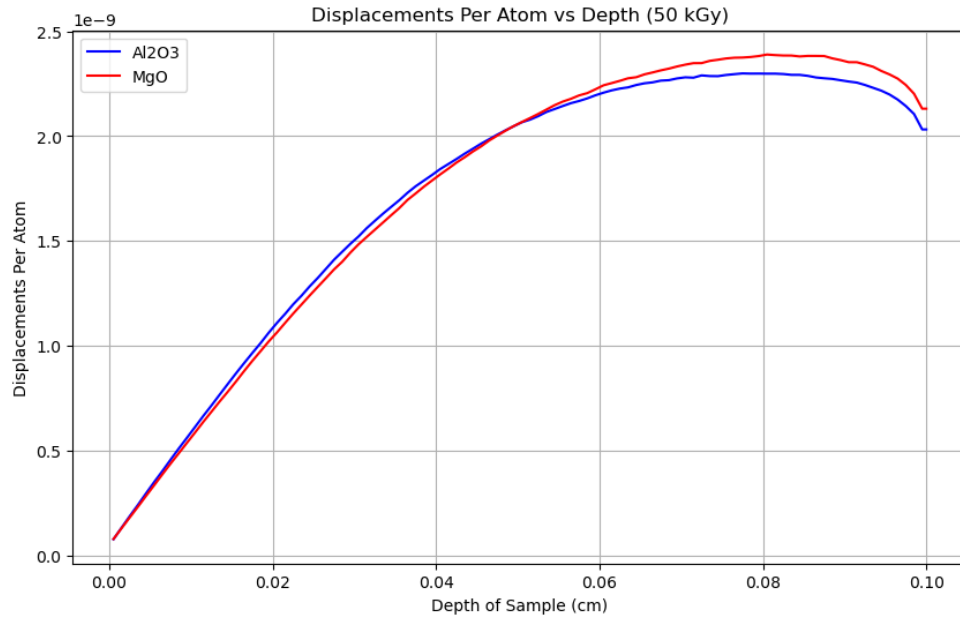
Figure 5.5: Simulated DPA from a mono-energetic photon source (1.25 MeV) placed at a distance of 80.00 \text{ cm} \pm 0.05 \text{ cm} from the target for 10.825 \pm 0.00001 days and then placed at 20.00 \pm 0.05 \text{ cm} from the target for 3.919 \pm 0.00001 days for the two samples.
