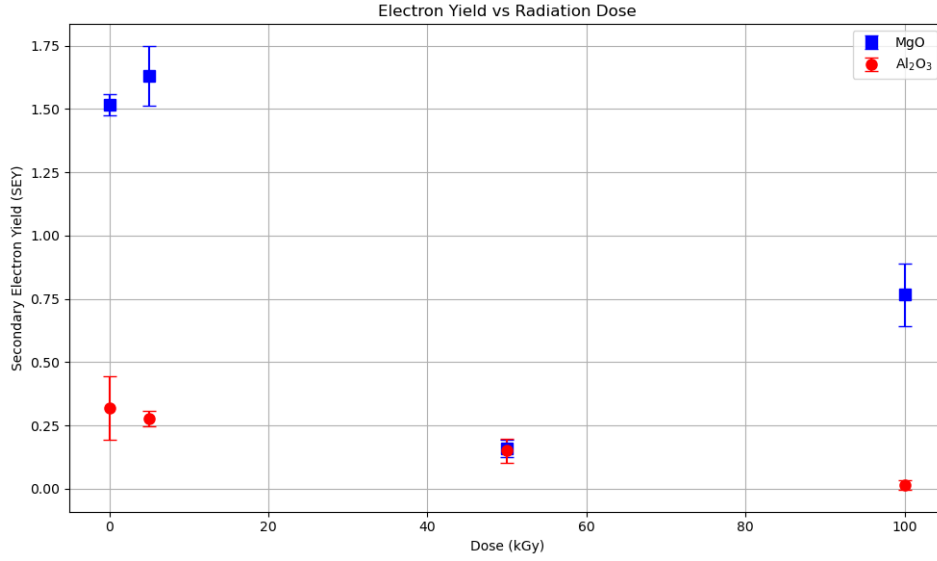
Figure 5.27: This figure presents the combined variation in electron emission yield of both Magnesium Oxide and Aluminium Oxide as a function of radiation dose, illustrating how the material's electron emission yield responds to increasing gamma radiation exposure.
