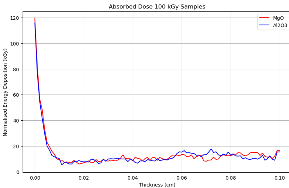
Figure 5.9: Simulated absorbed dose from a 70 TBq Co-60 source placed at a distance of 20.00 cm \pm 0.05 cm from the target for 10.828 \pm 0.00001 days for the two samples.
