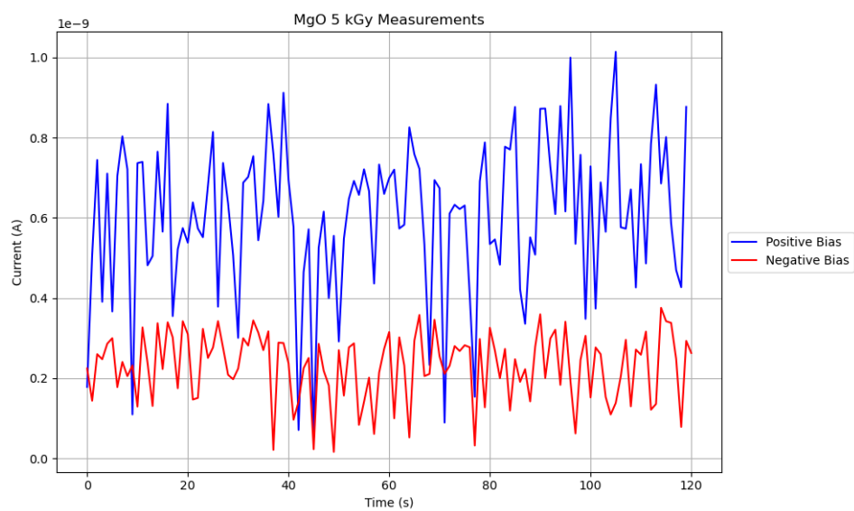
Figure 5.16: Measured current under positive and negative applied voltage bias for Magnesium Oxide samples with an absorbed gamma radiation dose of 5 kGy.
