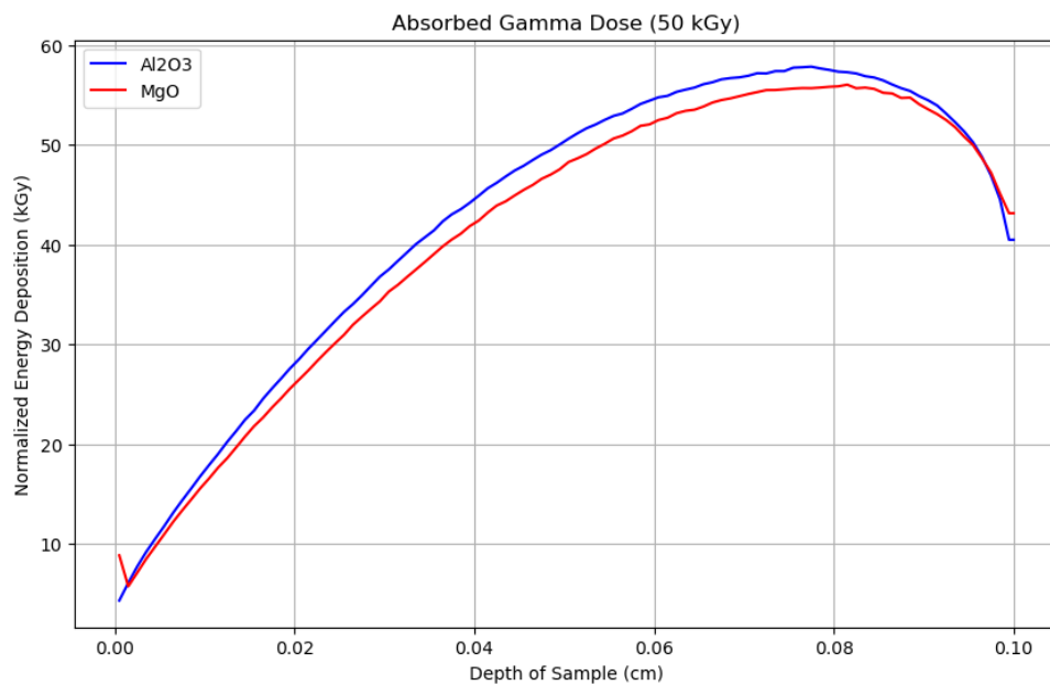
Figure 5.2: Simulated absorbed dose from a mono-energetic photon source (1.25 MeV) placed at a distance of 80.00 \text{ cm} \pm 0.05 \text{ cm} from the target for 10.825 \pm 0.00001 days and then placed at 20.00 \pm 0.05 \text{ cm} from the target for 3.919 \pm 0.00001 days for the two samples.
