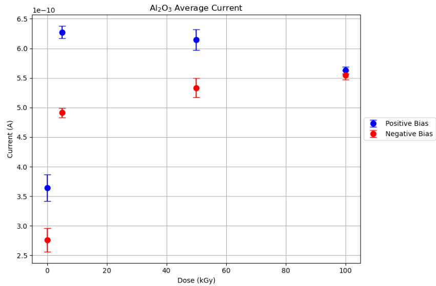
Figure 5.24: Averaged measured current under positive and negative applied bias for Aluminium Oxide samples as a function of absorbed gamma radiation dose.
