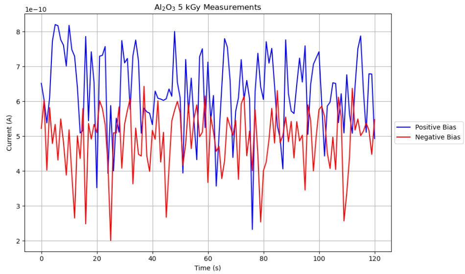
Figure 5.20: Measured current under positive and negative applied voltage bias for Aluminium Oxide samples with an absorbed gamma radiation dose of 5 kGy.
