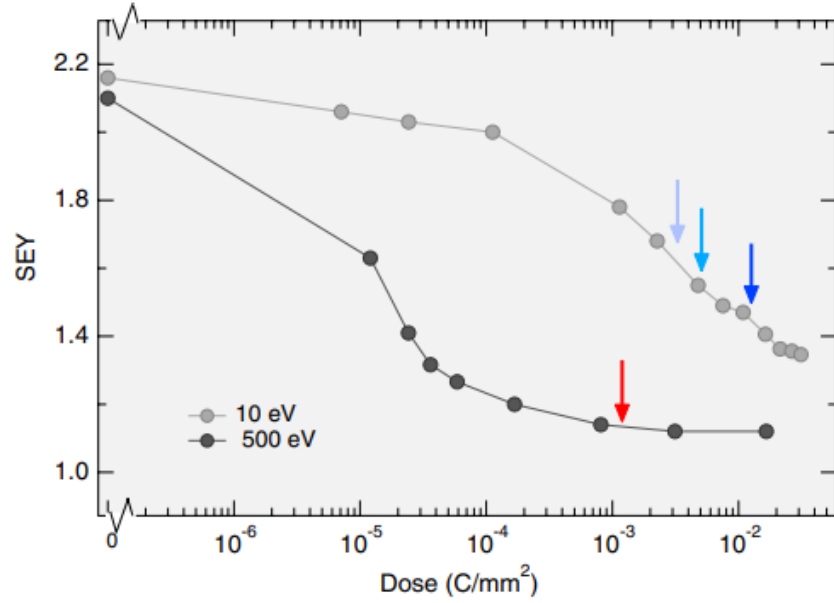
Figure 5.30: SEY as a function of the absorbed electron dose on a copper sample, based on [54], for an electron energy of 500 eV (dark gray) and 10 eV (gray).
