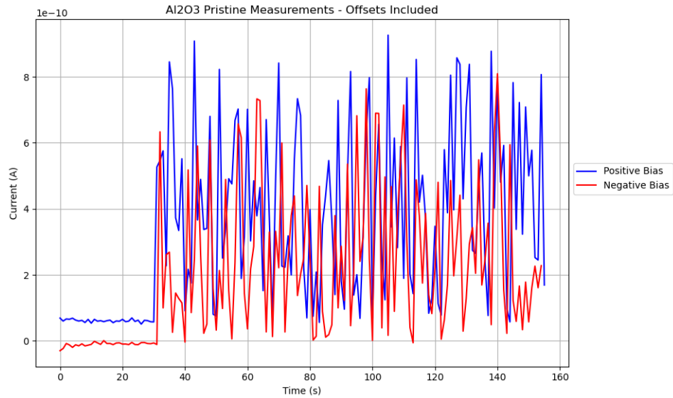
Figure 5.14: Current Vs Time measurements for the Al_2O_3 Pristine sample, including both the negative and positive bias and their respective offset measurements included.
