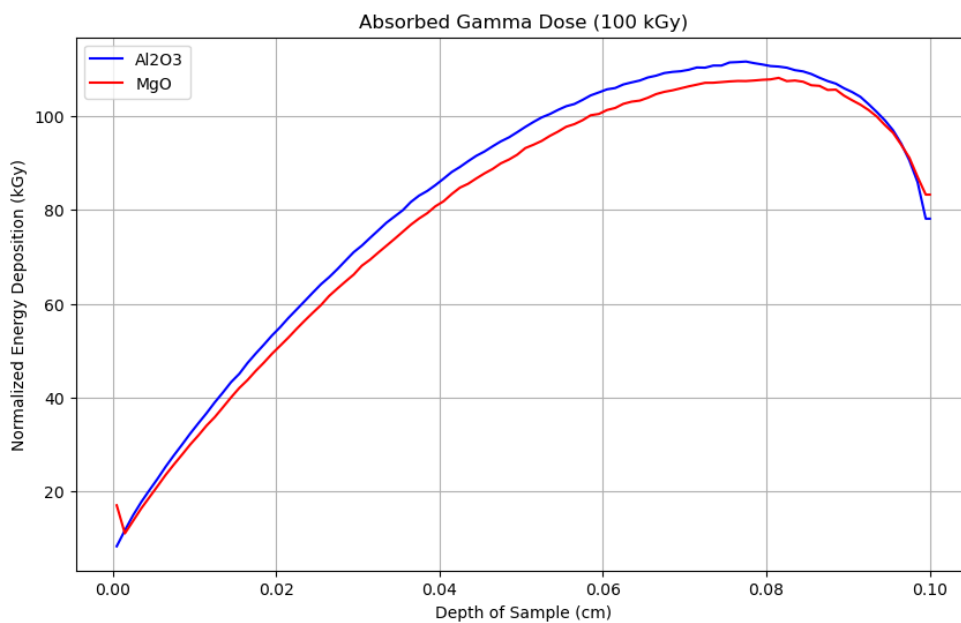
Figure 5.3: Simulated absorbed dose from a mono-energetic photon source (1.25 MeV) placed at a distance of 20.00 \text{ cm} \pm 0.05 \text{ cm} from the target for 10.828 \pm 0.00001 days for the two samples.
