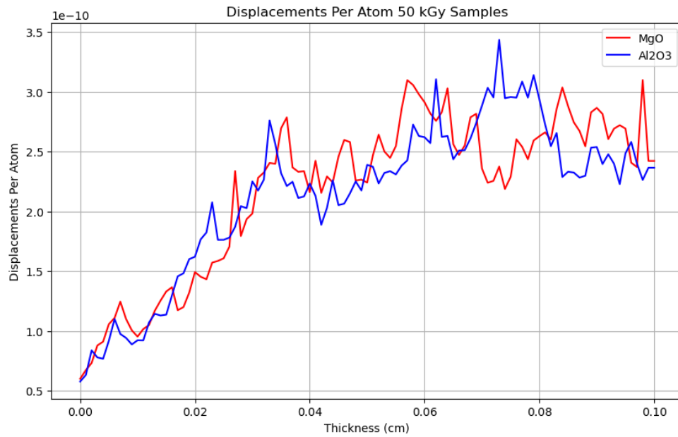
Figure 5.11: Simulated DPA from a 70 TBq Co-60 source placed at a distance of 80.00 \text{ cm} \pm 0.05 \text{ cm} from the source for 10.825 \pm 0.00001 days and then placed at 20.00 \pm 0.05 \text{ cm} from the source for 3.919 \pm 0.00001 days for the two samples.
