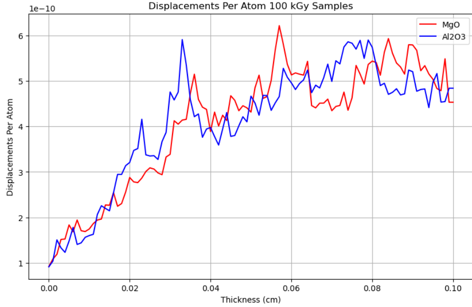
Figure 5.12: Simulated DPA from a 70 TBq Co-60 source placed at a distance of 20.00 \text{ cm} \pm 0.05 \text{ cm} for 10.828 \pm 0.00001 days for the two samples.
