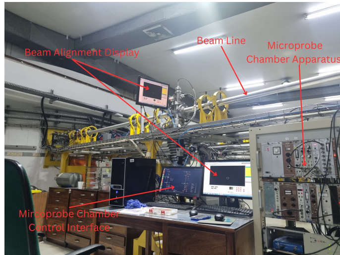
Figure 4.11: The microprobe chamber control interface is used for all microprobe chamber-related processes, such as vacuum pumping, venting, and other operational controls.
