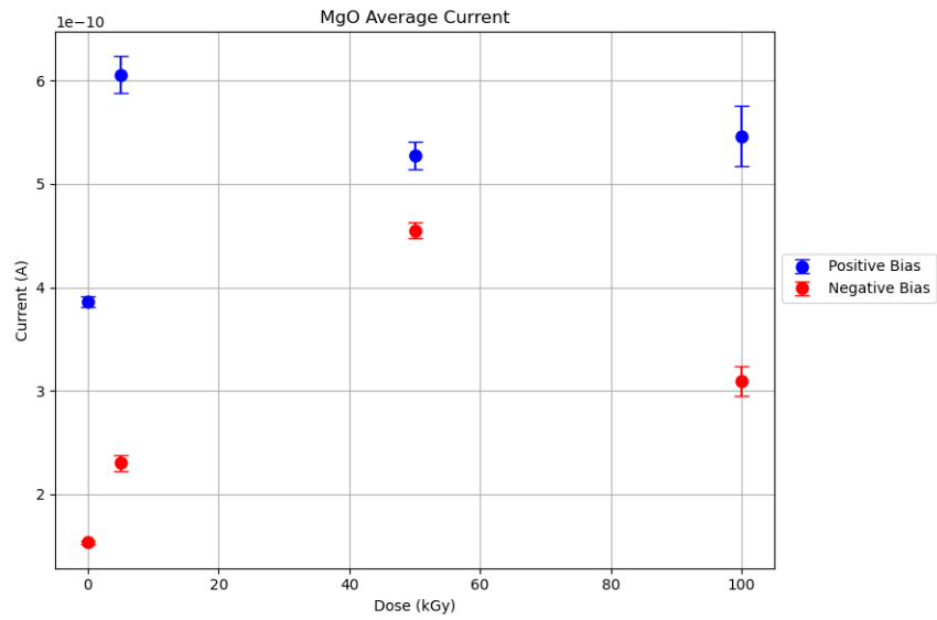
Figure 5.23: Averaged measured current under positive and negative applied bias for Magnesium Oxide samples as a function of absorbed gamma radiation dose.
