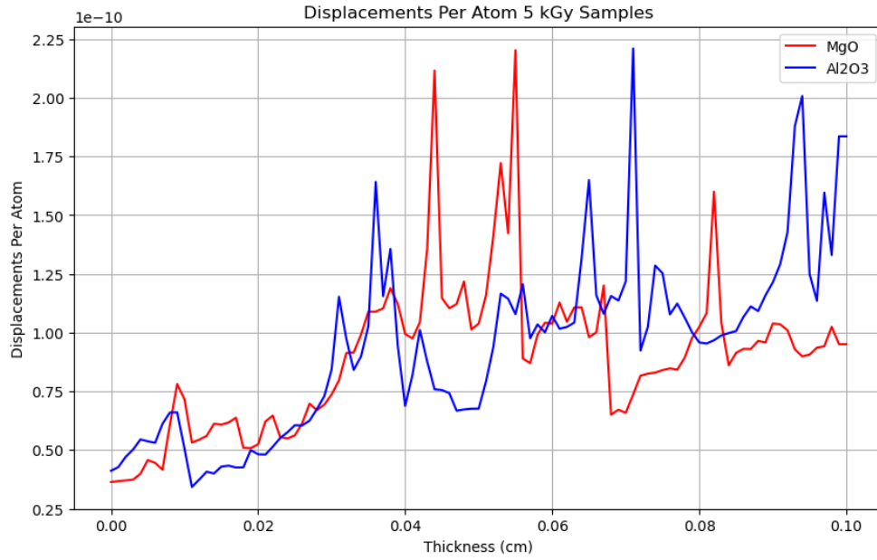
Figure 5.10: Simulated DPA from a 70 TBq Co-60 source placed 88.00 \text{ cm} \pm 0.05 \text{ cm} away from the source for 6.846 \pm 0.00001 days for the two samples.
