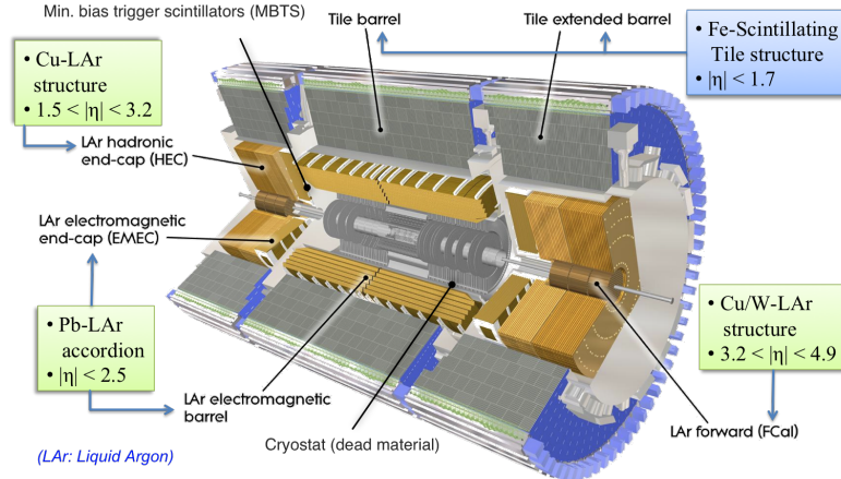
Figure 4.1: Calorimeter section of the ATLAS Detector [33]. In this figure \eta represents the pseudorapidity which expresses the range of a section of the detector with respect to the axis of colliding beams [34].
