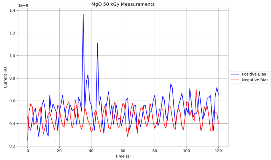
Figure 5.17: Measured current under positive and negative applied voltage bias for Magnesium Oxide samples with an absorbed gamma radiation dose of 50 kGy.
