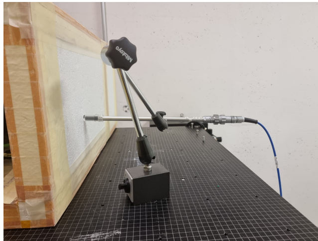
Figure 4.6: A calibrated cylindrical ionization chamber probe, Farmer-type, which measures radiation levels, is positioned at the location where the sample holder will be placed. This probe serves as the primary reference for quantifying the dose or activity arriving from the source at that specific distance. The probe is connected to a data acquisition system, as shown in Figure 4.8.
