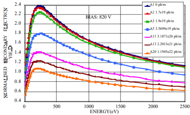
Figure 5.29: Normalized electron emission yield for a Copper sample at varying levels of absorbed radiation dose induced by photons [53].
