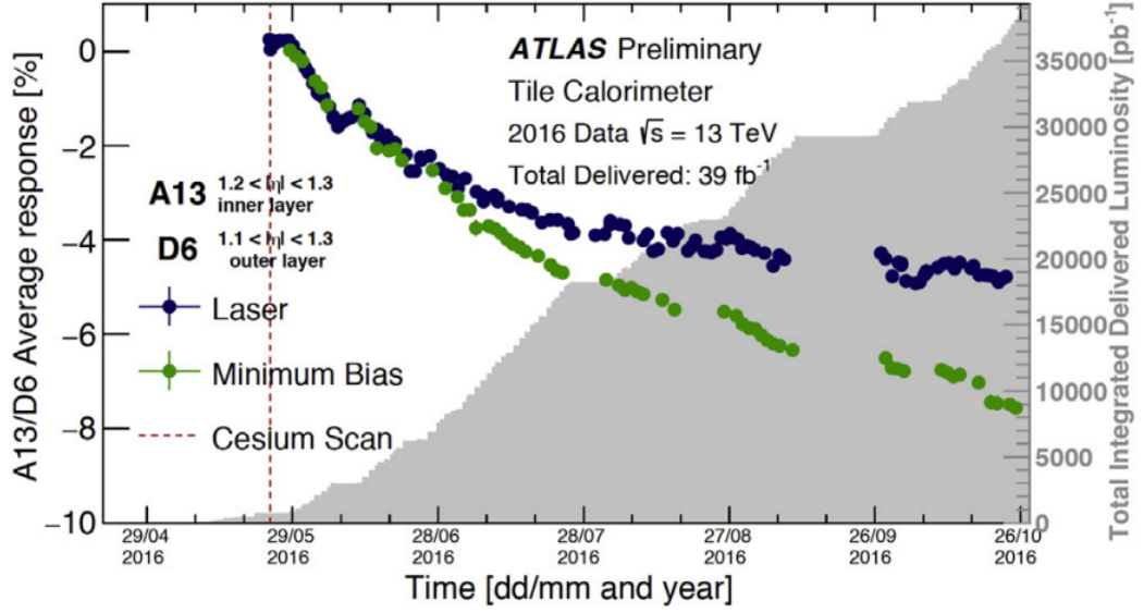
Figure 1.2: Response down-drift of innermost tiles in the ATLAS TileCal [11]. This figure shows the response of a PMT relative to the total integrated delivered luminosity. This figure demonstrates the down-drift of a PMT in a radiation-harsh environment.
