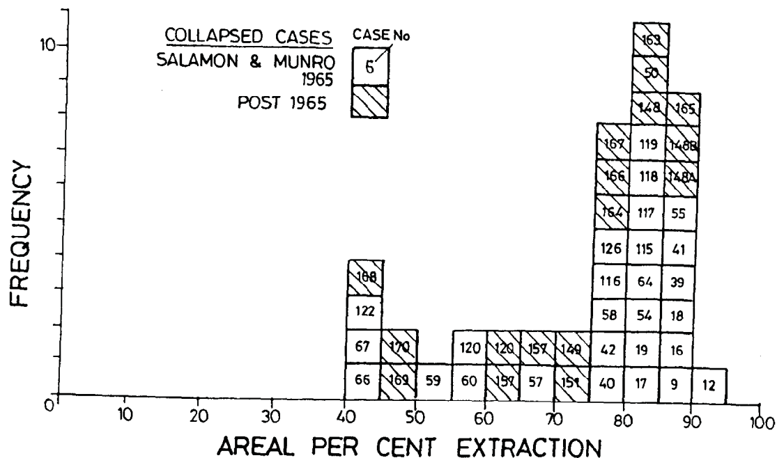
Figure 3.3 Frequency of occurrence versus the areal percentage extraction of collapsed pillar cases.
