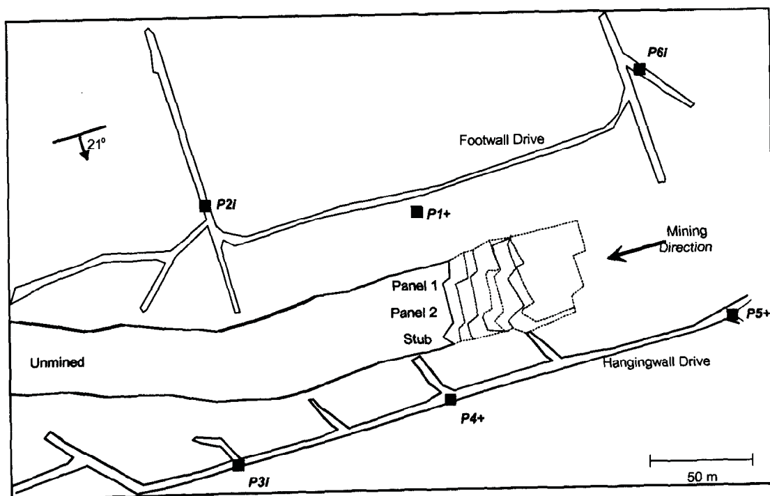
Figure 4.2.3 Plan of the preconditioning test site, showing the geophone positions for the PSS network
