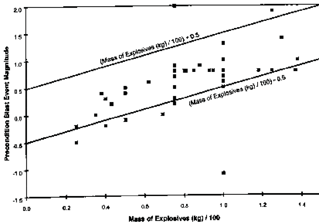
Figure 4.2.4 Comparison of the recorded preconditioning blast event magnitudes with the amount of explosive used for each blast
