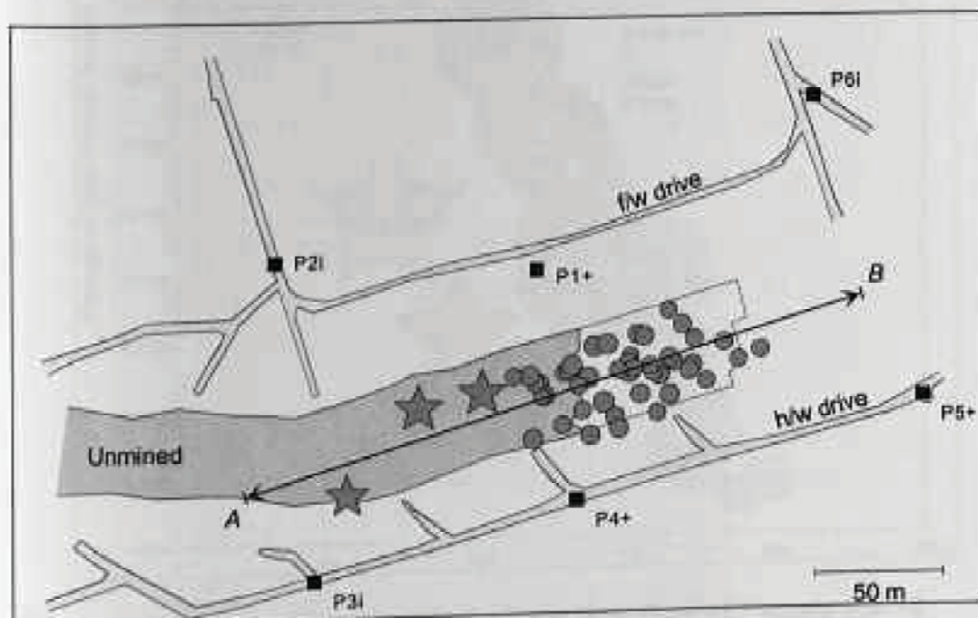
Figure 4.2.18 Plan of the locations of the larger seismic events recorded prior to seismic tomography experiment
