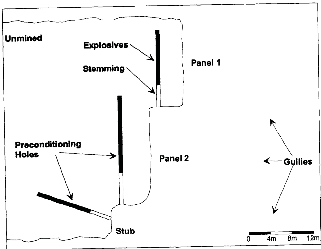
Figure 4.2.2 Preconditioning layout at the test site (17-24W stope)
