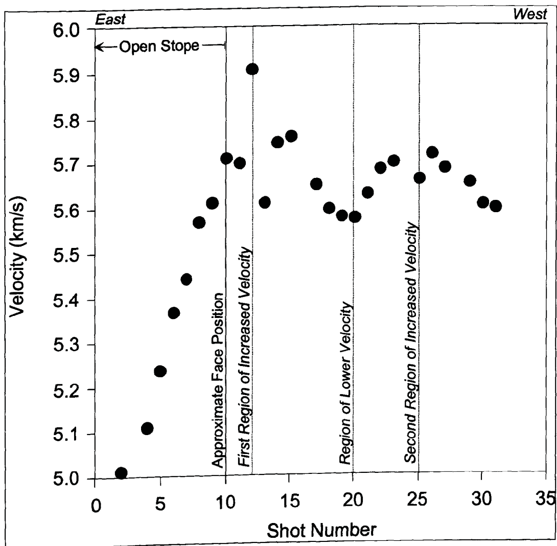
Figure 4.2.16 Plot of the straight ray apparent velocity measured between common shot and receiver hole numbers, showing the velocity variation from east to west (after Maxwell and Young, 1995)
