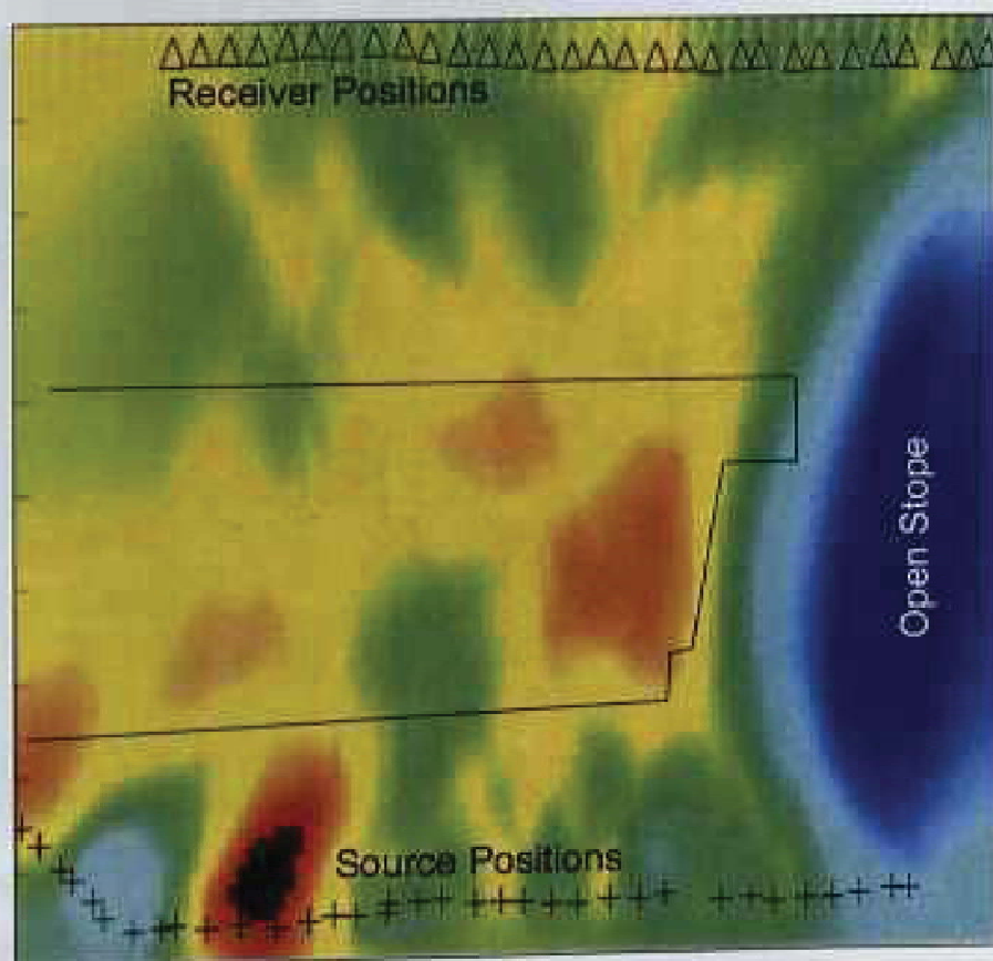
Figure 4.2.20 Velocity image of Figure 4.2.17 reconstructed through curved ray tracing (after Carneiro, 1995)
