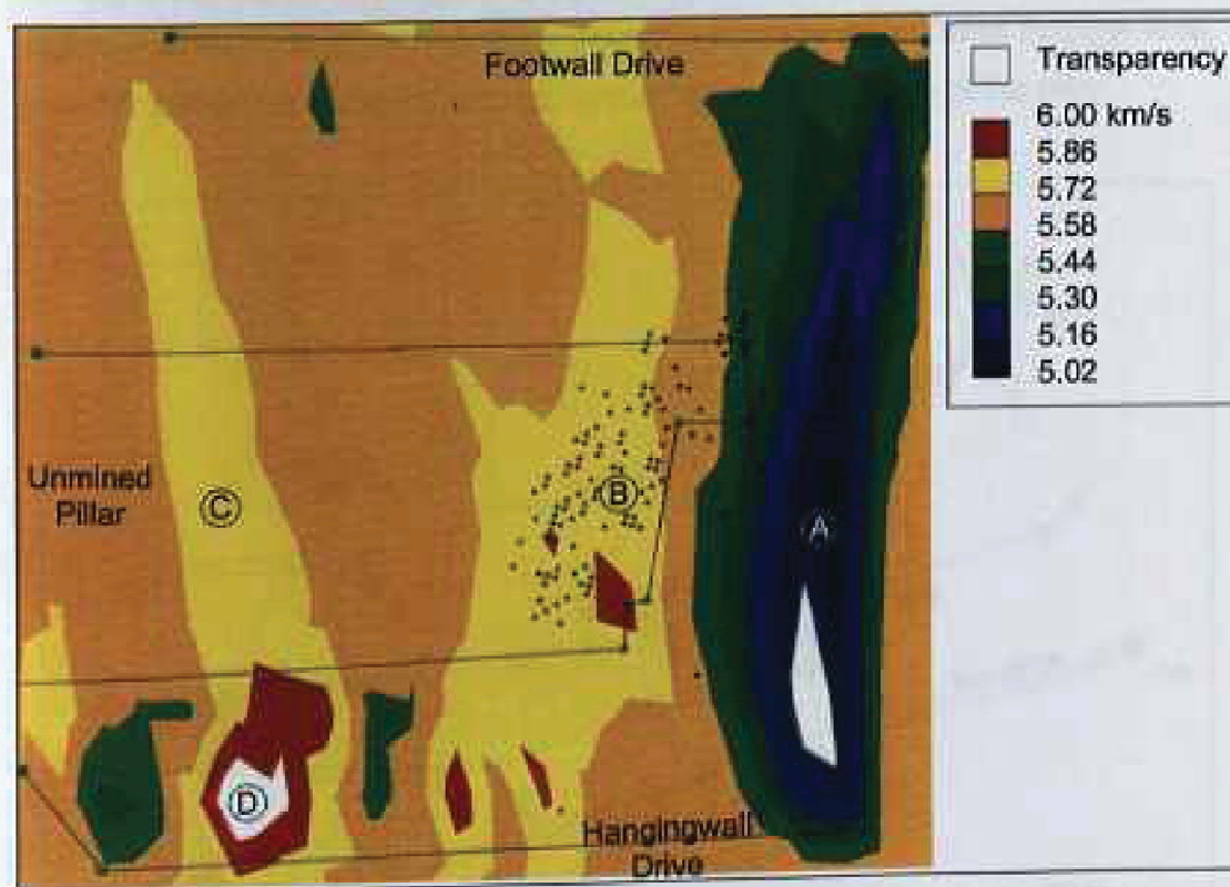
Figure 4.2.17 Straight ray velocity image produced from the seismic tomography survey (after Maxwell and Young, 1995)
