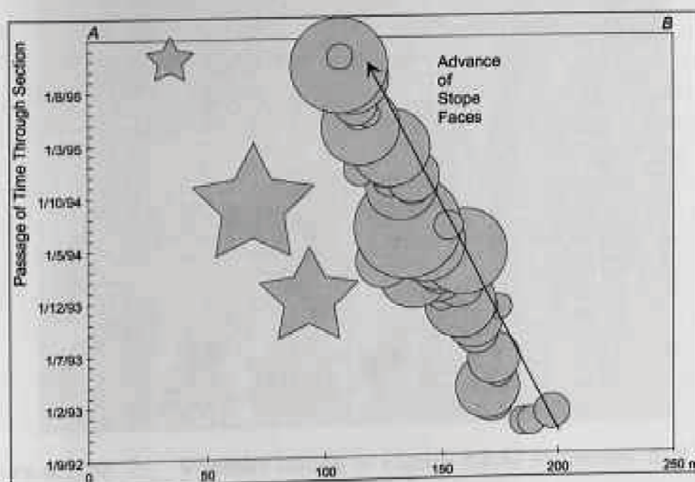
Figure 4.2.19 Time section along line A-B of Figure 4.2.18
