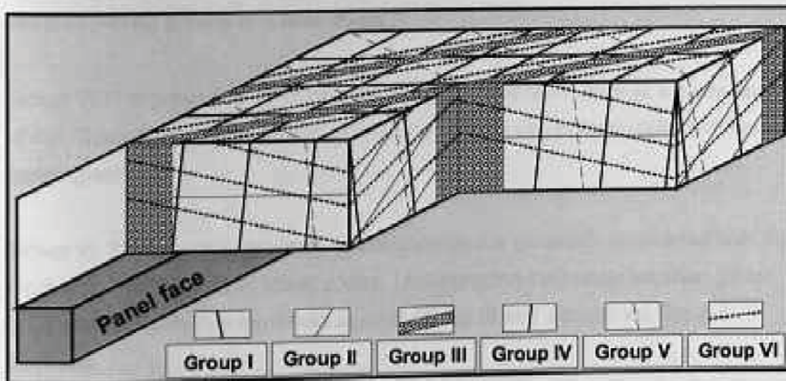
Figure 4.2.14 Schematic view of fracture groups (not to scale)
