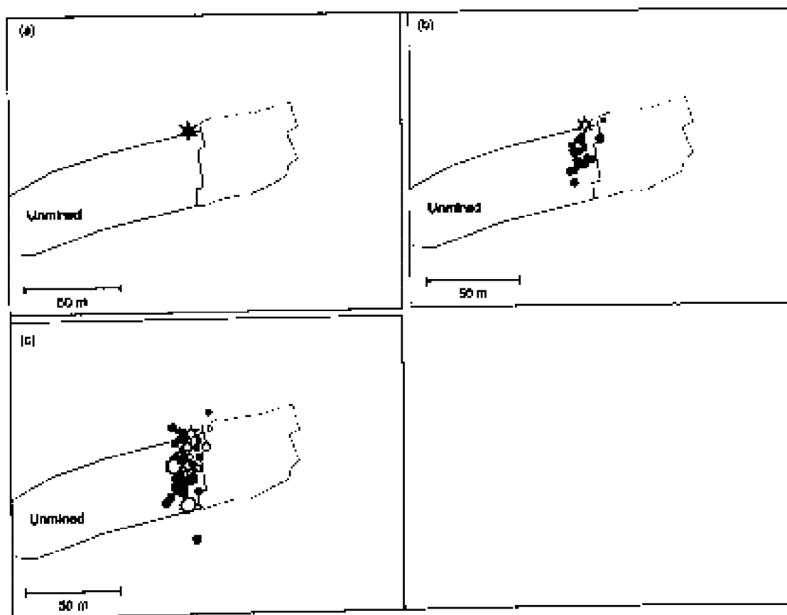
Figure 4.2.9 Seismic data recorded during and following a preconditioning blast at the test site on 10 January 1995
