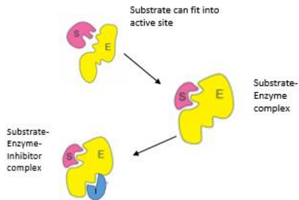
Figure 1. 12: Diagrammatical representation of the mechanistic binding of uncompetitive inhibition. Constructed using Adobe InDesign, 2017.
