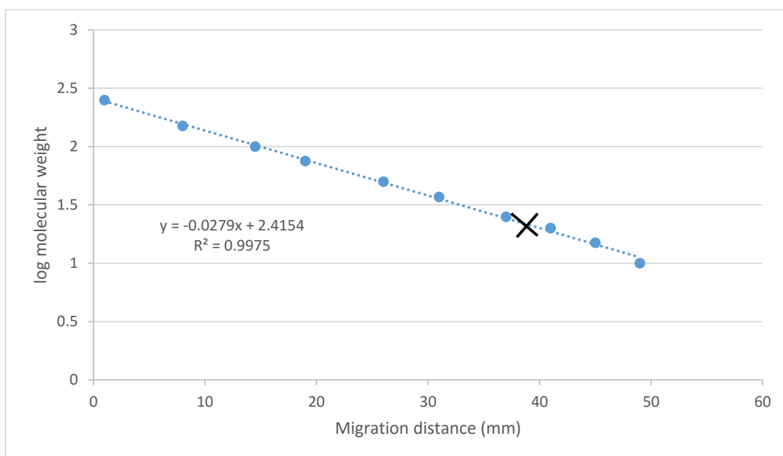
Figure 6. 6 Standard curve for the SDS PAGE gel in Figure 3.3 A of HIV-1 subtype B and C integrase before and after thrombin cleavage of the HIS tag. The X indicates the migration of the band to calculate the molecular weight
