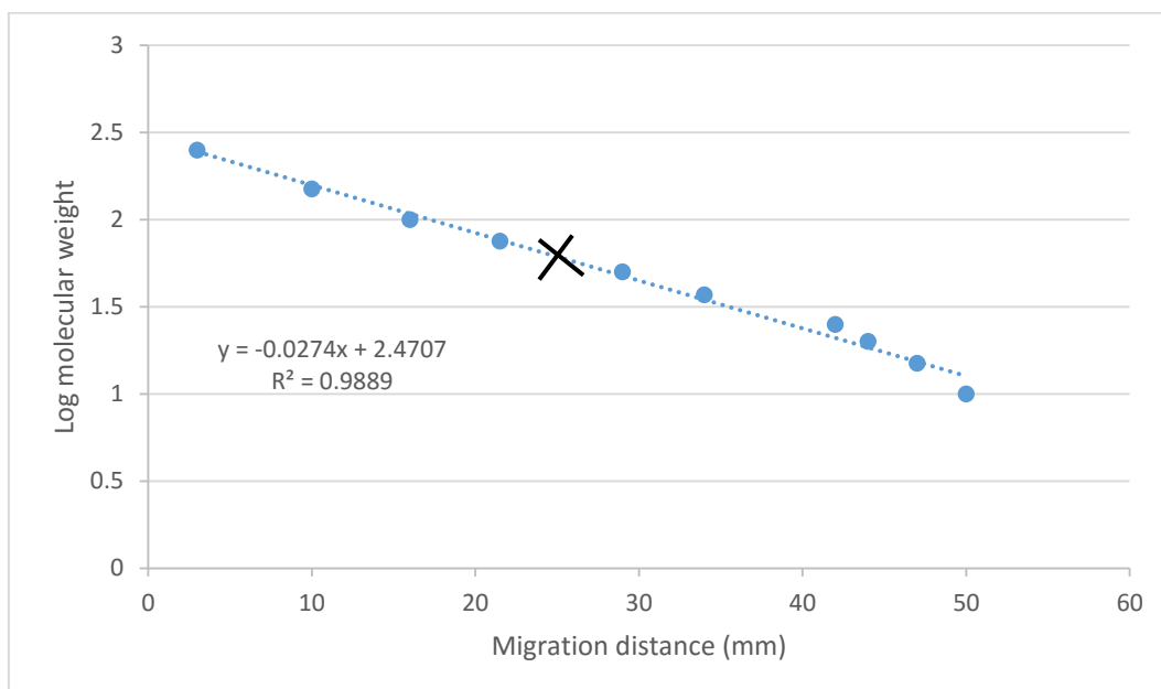
Figure 6. 4 Standard curve for SDS PAGE gel in Figure 3.2A of the purification and expression of LEDGF/p75. The X indicates the migration of the band to calculate the molecular weight
