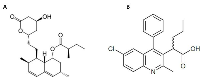
Figure 1. 25: Structure of lovastatin shown in A and CX05168 shown in B to display the similarities in compound structure. The compounds were drawn with use of Maestro 11.2, Schrodinger, 2017.
