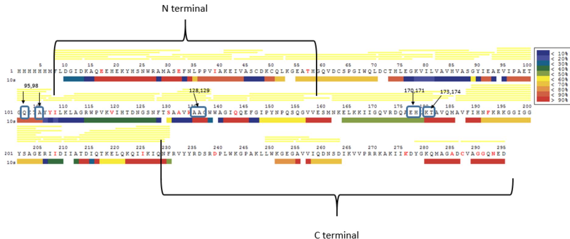
Figure 6. 14: Hydrogen exchange heat map of subtype C integrase with deuteration for 10s treated with lovastatin. The N terminal domain and C terminal domain are labelled with important amino acids of 128, 129, 170, 171, 173 and 174 highlighted for ease of analysis. Amino acids that have changed from subtype B are in red.
