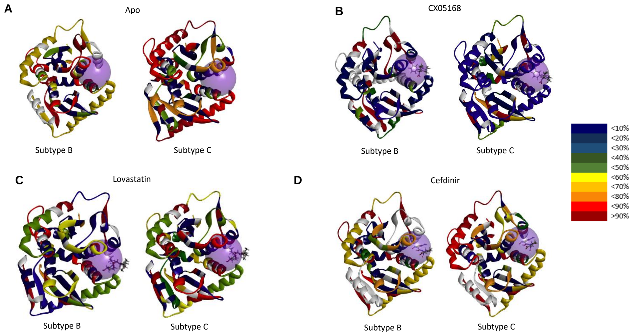
Figure 3. 18: HIV IN ribbon structure displaying the comparison of subtype B and C with the colours related to the deuterium exchange. The purple globe highlights the binding site. The ribbon structure was compiled with the use of Maestro 11.2, Schrodinger, 2017. (A) Subtype B and C HIV-1 IN with no compound bound. (B) Subtype B and C HIV-1 IN treated with CX05168. (C) Subtype B and C HIV-1 IN treated with lovastatin and Figure (D) is subtype B and C HIV-1 IN treated with cefdinir.
