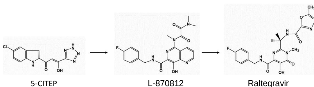
Figure 1. 14: Development of raltegravir showing the steps from 5-CITEP to L-870812 through to raltegravir. Raltegravir is a potent inhibitor of the strand transfer reaction with an IC_{50} of 2-7nM. Figure formulated with use of diagrams from Chemspider.
