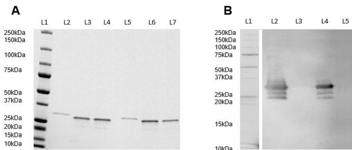
Figure 3.3: SDS-PAGE gel of HIV-1 subtype B and C IN following thrombin cleavage of the 6XHIS tag ( A ) and a western blot confirming cleavage of the HIS tag ( B ). ( A ) Shows the SDS PAGE gel with cleaved and uncleaved HIV-1 IN subtype B and C, Lane 1, precision plus protein molecular weight marker (Bio-Rad, USA); Lane 2, HIV-1 subtype B IN 6xHIS tagged protein; Lane 3, fraction 1 of cleaved HIV-1 subtype B IN; Lane 4, fraction 2 of cleaved HIV-1 subtype B IN Lane 5; HIV-1 subtype C IN 6xHIS tagged protein; Lane 6, fraction 1 cleaved HIV-1 subtype C IN Lane 7, fraction 2 of the cleaved HIV-1 subtype C. ( B ) Shows a western blot analysis of HIV-1 subtype B and C IN following thrombin cleavage of the 6XHIS tag. Lane 1, precision plus protein molecular weight marker (Bio-Rad, USA); Lane 2, HIV-1 subtype B IN 6xHIS tagged protein; Lane 3, cleaved HIV-1 subtype B IN; Lane 4, HIV-1 subtype C IN 6xHIS tagged protein; Lane 5, cleaved HIV-1 subtype C IN. Please note that image B has been split to remove a lane that was not needed on the blot. Figures 6.6 and 6.7 are the standard curves used to determine protein size marked with an X for A and B respectively.
