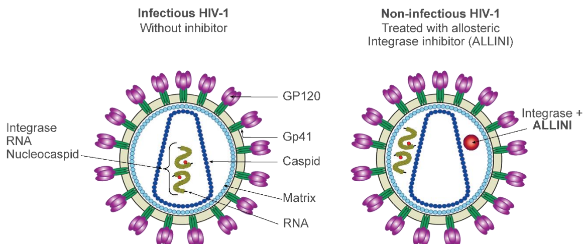
Figure 1. 19: Diagrammatical representation of a standard infectious virion and a defective immature progeny virion formed after treatment with an ALLINI. Diagram altered from Kessl et al. , 2016 (Kessl et al. , 2016a)
