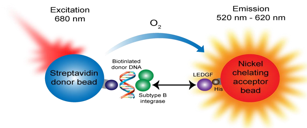
Figure 2. 1 Schematic representation of the HIV-1 IN-LEDGF/p75 interaction in an AlphaScreen assay. The streptavidin donor bead links to the biotin labelled donor DNA-IN complex which then interacts with the HIS tagged LEDGF/p75 bound to the nickel chelating acceptor bead
