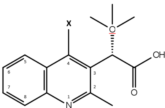
Figure 1. 20: Diagrammatic representation of a generic quinolone compound. Where X depicts an area for different functional groups. Drawn with use of Maestro 11.2, Schrodinger, 2017.
