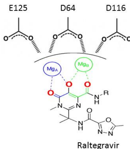
Figure 1. 15: Mechanism of action of raltegravir showing the binding to the DDE triad and the magnesium ions to the oxygen groups of raltegravir. Atoms labelled in red form part of the heteroatom donor triad which co-ordinates to the active site magnesium's chelating rings A and B where A is blue and B is green. Diagram adapted from Agrawal et al (Agrawal et al. , 2012).
