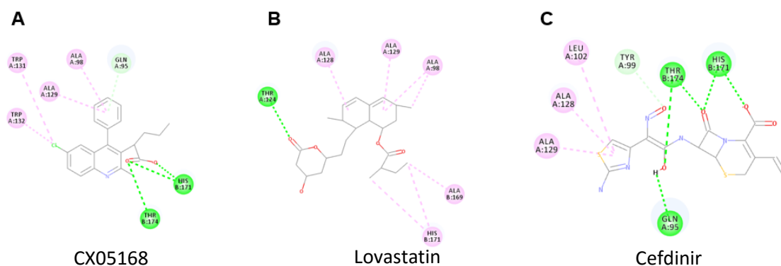
Figure 3. 11: Molecular model of the predicted binding of compounds to the HIV-1 IN dimer interface where LEDGF/p75 would dock. (A) Shows the hydrogen bond interactions between CX05168 and the LEDGF/p75 binding site were predicted to be at a relative distance less than 3Å. (B) The hydrogen bond interaction of lovastatin in the LEDGF/p75 binding site was projected to be at a relative distance of 2.88Å. (C) Shows the hydrogen bond interaction of cefdinir in the LEDGF/p75 binding site was projected to be at a relative distance of 3Å. These figures were generated using Maestro 11.2, Schrodinger, 2017.
