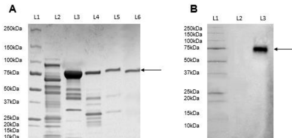
Figure 3. 2: SDS-PAGE gel showing the expression and purification steps of a protein correlating with that of LEDGF/p75 and western blot proving the successful expression of LEDGF/p75. (A) Lane 1, precision plus protein molecular weight marker (Bio-Rad, USA); Lane 2, flow-through from the nickel affinity exchange column; Lane 3, concentrated protein from the nickel affinity column; Lane 4, concentrated protein from the gradient fractions cation exchange column; Lane 5, concentrated protein from the size exclusion column; Lane 6, concentrated protein from the Amicon 50kDa cut-off; (B) Western blot analysis confirming the expression of LEDGF/p75 with primary antibody anti-PSIP1. Lane 1, precision plus protein molecular weight marker (Bio-Rad, USA); Lane 2, negative control fraction from size exclusion chromatography; Lane 3, concentrated Amicon sample after size exclusion chromatography purified LEDGF/p75. Figures 6.4 and 6.5 are the standard curves used to determine protein size marked with an X for A and B respectively.
