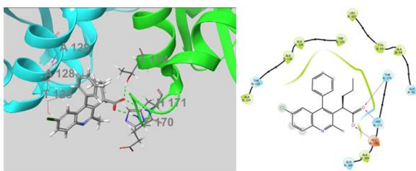
Figure 1. 21 (A) Ribbon 3D structure of the CCD of HIV IN with a known quinolone compound CX05168 docked indicating interacting amino acids. (B) 2D structure of known quinolone CX05168 docked indicating interacting amino acids.
