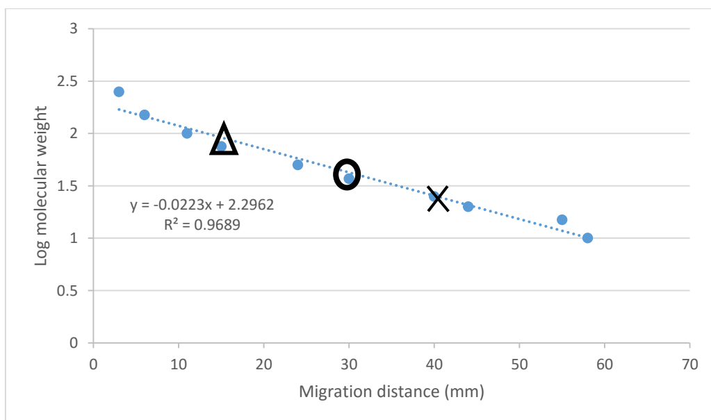
Figure 6. 8 Standard curve of the western blot in Figure 3.7A showing the dimerization studies of HIV-1 subtype B integrase and inhibitors. The X, circle and triangle indicates the migration of the bands to calculate the molecular weight
