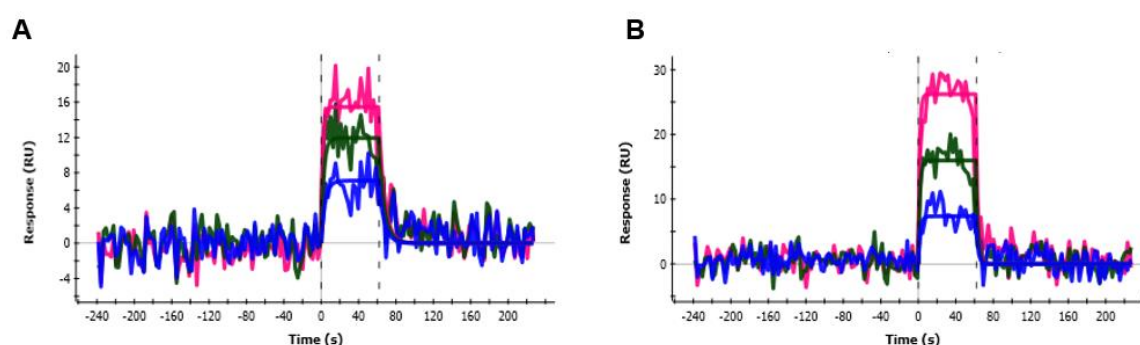
Figure 3. 20: Surface Plasmon resonance graphs for CX05168 for concentrations 10 \mu M, 5 \mu M and 2 \mu M for subtype B (A) and C (B) HIV-1 IN. The blue line represents 2 \mu M, the green line represents 5 \mu M and the pink line represents 10 \mu M.
