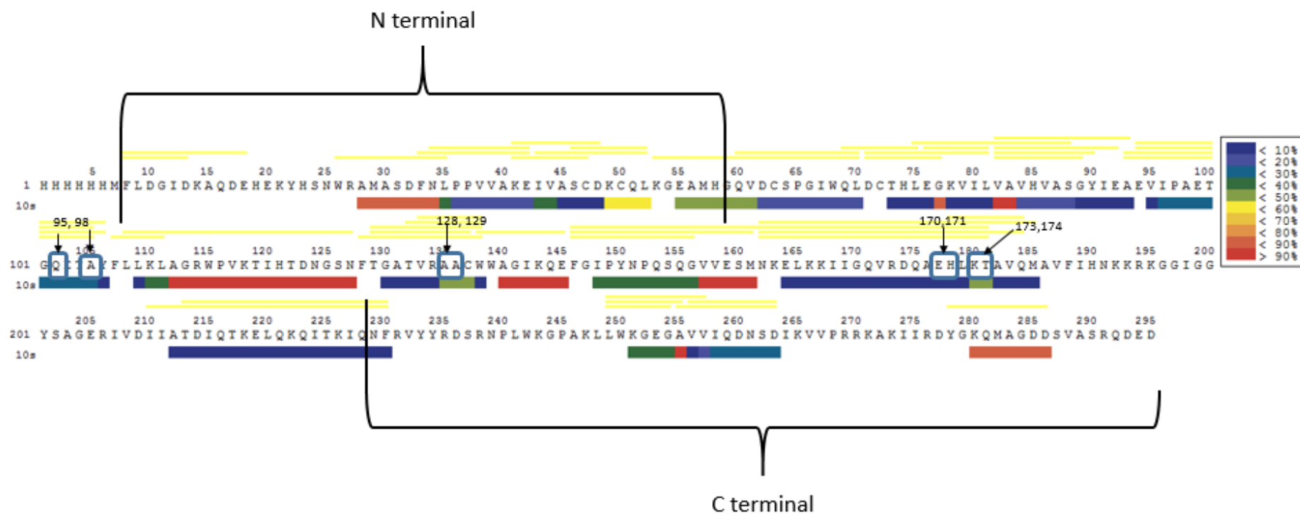
Figure 6. 10: Hydrogen exchange heat map of subtype B integrase with deuteration for 10s treated with CX05168. The N terminal domain and C terminal domain are labelled with important amino acids of 128, 129, 170, 171, 173 and 174 highlighted for ease of analysis.
