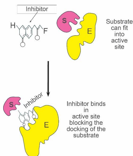
Figure 1. 11: Diagrammatical representation of the mechanistic binding of competitive inhibition. Constructed using Adobe InDesign, 2017.
