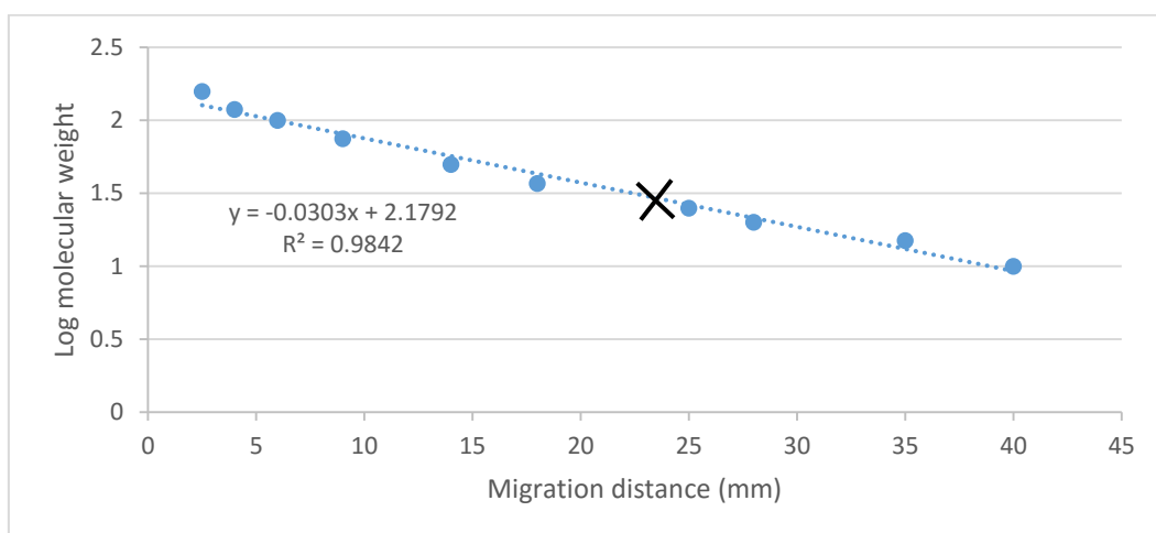
Figure 6. 2 Standard curve for SDS PAGE gel in figure 3.1 B for the purification and expression of subtype C integrase. The X indicates the migration of the band to calculate the molecular weight
