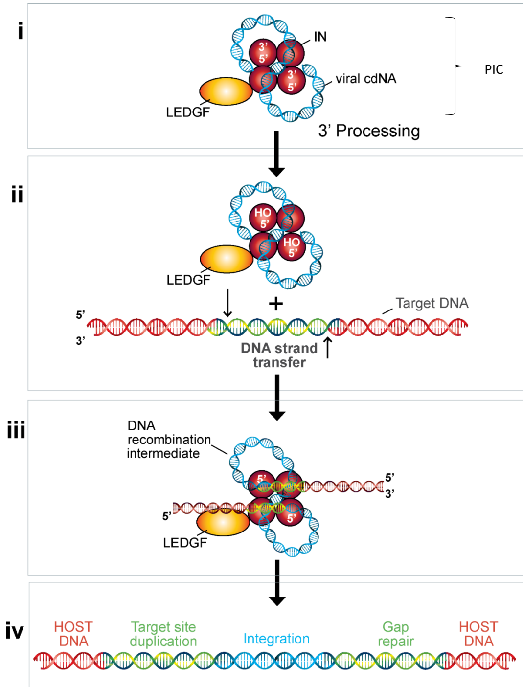
Figure 1. 7: Schematic representation of the HIV-1 integration reaction. In the first step (i) tetrameric IN is bound to viral cDNA and LEDGDF forming the PIC and produces CA overhangs during 3' processing. During step 2 (ii) the PIC is transported to the nucleus where strand transfer begins with binding to the host DNA. The penultimate phase (iii) is where binding is followed by nucleophilic attack to form phosphodiester bonds leaving a 5' DNA flap. Finally (iv) the DNA is repaired by cellular machinery resulting in integration. Diagram was drawn and altered from Bushman et al 1990 and Chen et al 2000 (Bushman et al. , 1990; Chen et al. , 2000).
