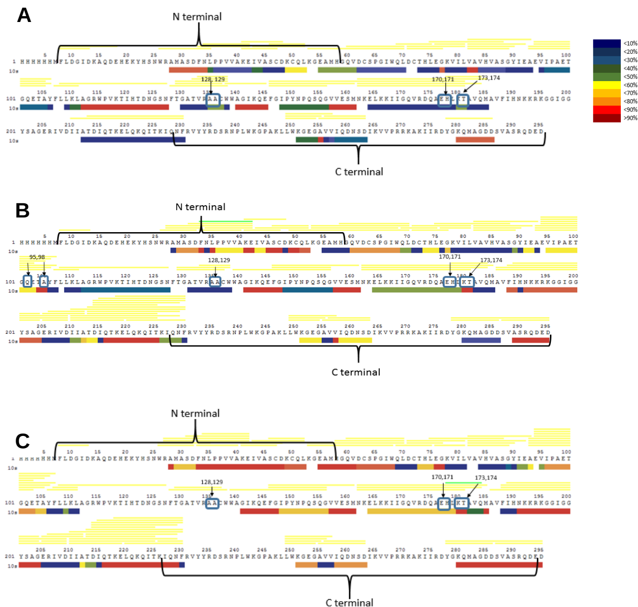
Figure 3. 13: Hydrogen exchange heat map of HIV-1 subtype B integrase with deuteration for 10s treated with CX05168 (A), lovastatin (B) and cefdinir (C). The N terminal domain and C terminal domain are labelled with important amino acids of 128, 129, 170, 171, 173 and 174 highlighted for ease of analysis. Red areas indicate areas of high exchange whereas blue areas indicate restricted hydrogen exchange. The colour key can be found on the right hand top corner.
