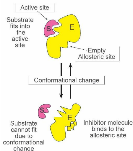
Figure 1. 13: Diagrammatical representation of the mechanistic binding of non-competitive inhibition. Constructed using Adobe InDesign, 2017
