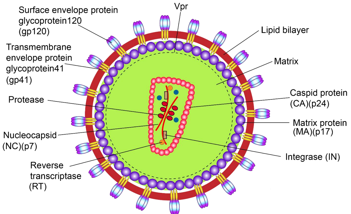
Figure 1. 2: Representative figure of an HIV virion displaying structural and functional proteins. The virion contains capsid protein (p24), matrix protein (p17), nucleocapsid (p7), reverse transcriptase, integrase and protease, as well as envelope glycoproteins, gp120 and gp41. Picture adapted Hosseini and Mac Gabhann, 2012 (Hosseini and Mac Gabhann, 2012) .
