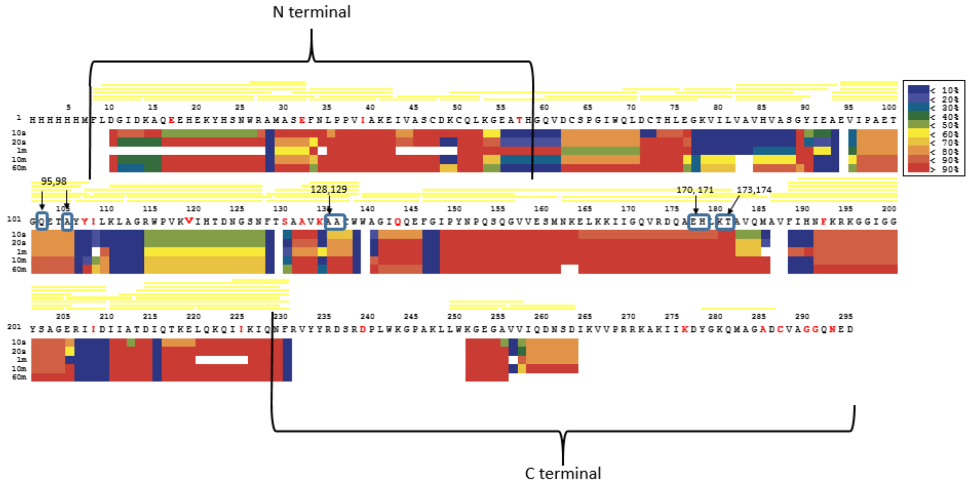
Figure 3. 15: Hydrogen exchange heat map of HIV-1 subtype C integrase with deuteration for 102, 20s, 1min, 10min and 60 min. The N terminal domain and C terminal domain are labelled with important amino acids of 128, 129, 170, 171, 173 and 174 highlighted for ease of analysis. Amino acids that differ from subtype B are in red. Areas in red are areas of high deuterium exchange whereas areas in blue are restricted from deuterium exchange
