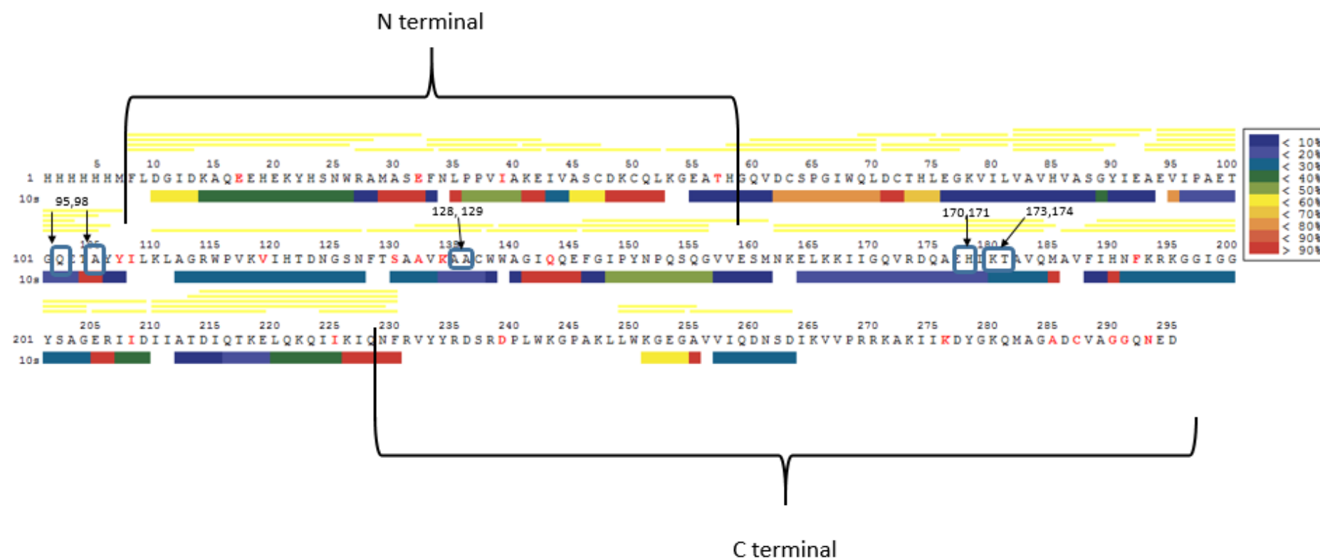
Figure 6. 13: Hydrogen exchange heat map of subtype c integrase with deuteration for 10s treated with CX05168. The N terminal domain and C terminal domain are labelled with important amino acids of 128, 129, 170, 171, 173 and 174 highlighted for ease of analysis. Amino acids that have changed from subtype B are in red.
