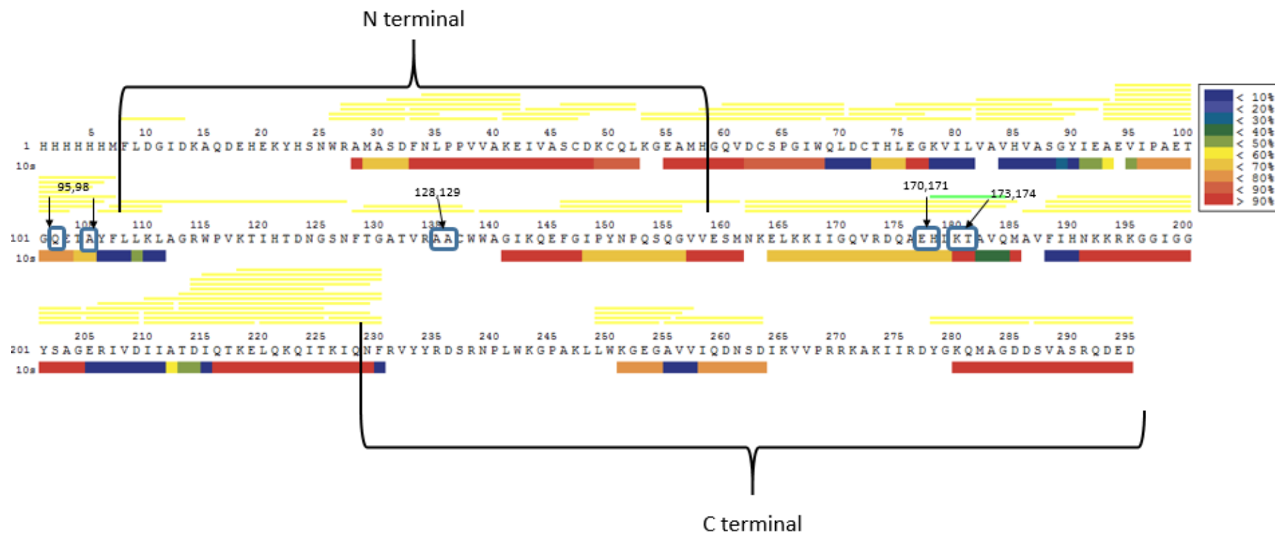
Figure 6. 12: Hydrogen exchange heat map of subtype B integrase with deuteration for 10s treated with cefdinir. The N terminal domain and C terminal domain are labelled with important amino acids of 128, 129, 170, 171, 173 and 174 highlighted for ease of analysis.
