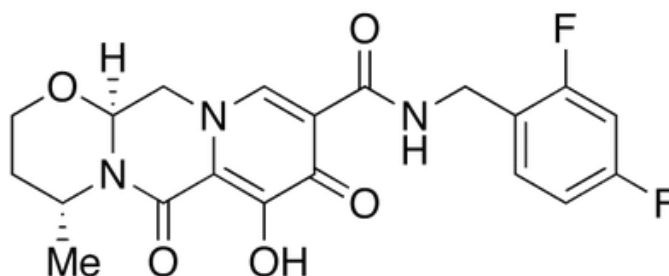
Figure 1. 18: The chemical structure of dolutegravir. DTG has strong strand transfer inhibition as well as antiviral activity with an IC_{50} of 1.07nM inhibition of strand transfer activity. Copied from Chemspider, www.chemspider.com/Chemical-Structure.25051637 , accessed on 22/03/2017.
