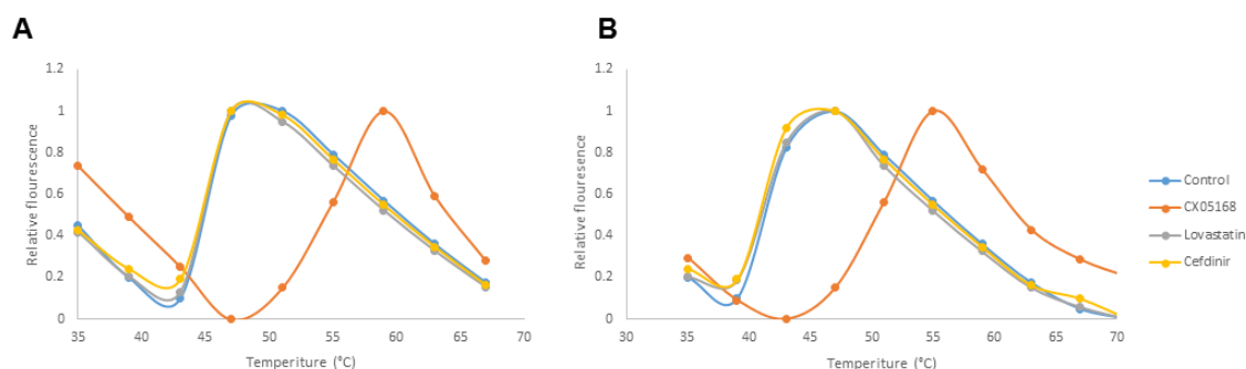
Figure 3. 10: Analysis of the melting temperature of HIV-1 subtype B ( A ) and C ( B ) IN in the absence of compound (blue), in the presence of CX05168 (red), lovastatin (grey) and cefdinir (yellow). The dotted black line represents the melting temperature for the control, lovastatin and cefdinir and the green dotted line represents the melting temperature for CX05168.
