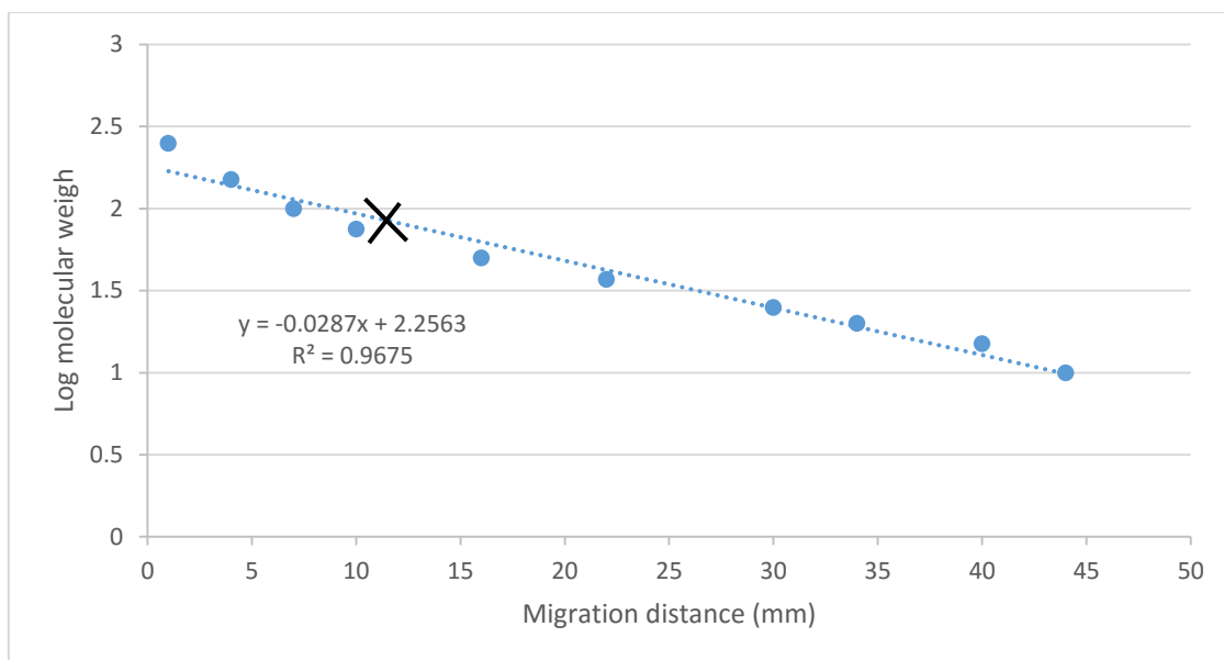
Figure 6. 5 Standard curve for the western blot in Figure 3.2 confirming the successful expression of LEDGF/p75. The X indicates the migration of the band to calculate the molecular weight
