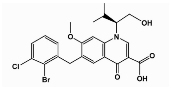
Figure 1. 17: Chemical structure of elvitegravir. Elvitegravir was co-developed by GlaxoSmithKline and Shionogi Pharmaceuticals with an IC_{50} of 16nM inhibition of strand transfer activity. Copied from Chempider, www.chemspider.com/Chemical-Structure.4441060 , date accessed 22/3/2017.
