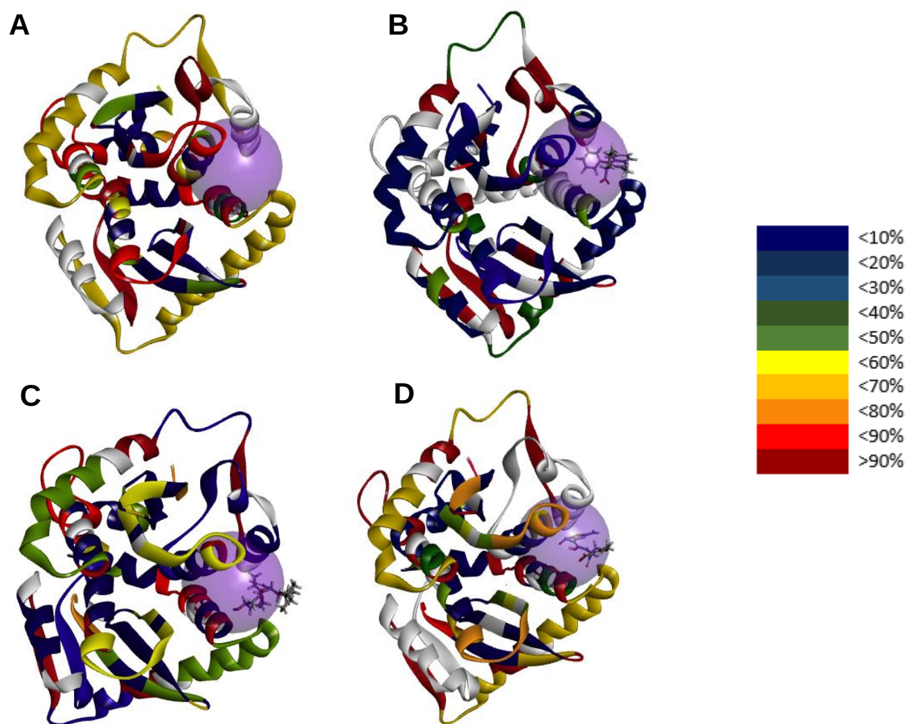
Figure 3. 14: Ribbon structure of the prepared binding site on integrase where the compounds bind to elicit their effects. The purple globe highlights the binding site. The deuterium exchange enzyme has been indicated with colour change depending on the rate of exchange for each part of the enzyme in correlation to the hydrogen exchange maps. The ribbon structure was compiled with the use of Maestro 11.2, Schrodinger, 2017. Figure A is subtype B HIV-1 IN with no compound bound. Figure B is subtype B HIV-1 IN treated with CX05168. Figure C is subtype B HIV-1 IN treated with lovastatin and Figure D is subtype B HIV-1 IN treated with cefdinir.
