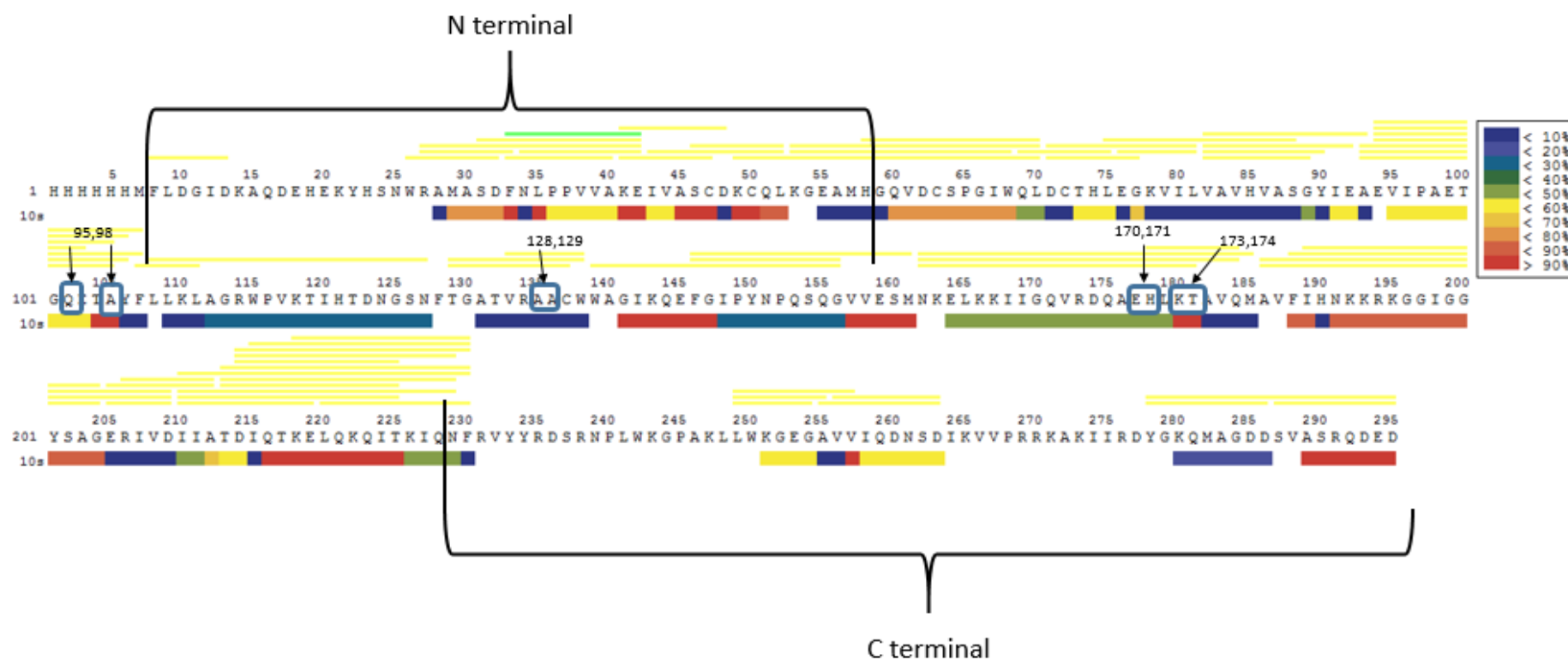
Figure 6. 11: Hydrogen exchange heat map of subtype B integrase with deuteration for 10s treated with lovastatin. The N terminal domain and C terminal domain are labelled with important amino acids of 128, 129, 170, 171, 173 and 174 highlighted for ease of analysis.
