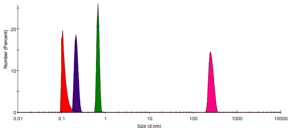
Figure 3. 9: Number distribution graph of the multimerisation effects of studied compounds for subtype B HIV-1 IN and subtype C HIV-1 IN. Differential light scattering assay was utilised to determine the number distribution of each protein treated with compound. (A) and (B) show the number distribution graph for subtype B HIV-1 IN and subtype C HIV-1 IN respectively where the red peak is HIV-1 IN incubated with DMSO, the purple peak is HIV-1 IN incubated with lovastatin, the green peak is HIV-1 IN incubated with cefdinir and the pink peak is HIV-1 IN incubated with CX05168.
