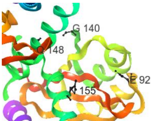
Figure 1. 16 The catalytic core domain of integrase, magnified to show the amino acids commonly associated with raltegravir resistance
