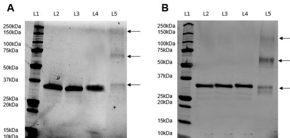
Figure 3. 8: Western blot study showing the cross-linking studies with HIV-1 subtype B IN (A) and subtype C IN (B). (A) Show the western blot of subtype B HIV-1 IN where Lane 1, precision plus protein molecular weight marker (Bio-Rad, USA); Lane 2, HIV-1 subtype B IN 6xHIS tagged protein with no compound; Lane 3, HIV-1 subtype B IN 6xHIS tagged protein with Cefdinir Lane 4, HIV-1 subtype B IN 6xHIS tagged protein with lovastatin and Lane5, HIV-1 subtype B IN 6xHIS tagged protein with CX05168. (B) Shows the western blot study showing the cross-linking studies with HIV-1 subtype C IN where Lane 1, precision plus protein molecular weight marker (Bio-Rad, USA); Lane 2, HIV-1 subtype C IN 6xHIS tagged protein with no compound; Lane 3, HIV-1 subtype C IN 6xHIS tagged protein with Cefdinir Lane 4, HIV-1 subtype C IN 6xHIS tagged protein with lovastatin and Lane5, HIV-1 subtype C IN 6xHIS tagged protein with CX05168. Figures 6.8 and 6.0 are the standard curves used to determine protein size marked with an X, circle or triangle for A and B respectively.
