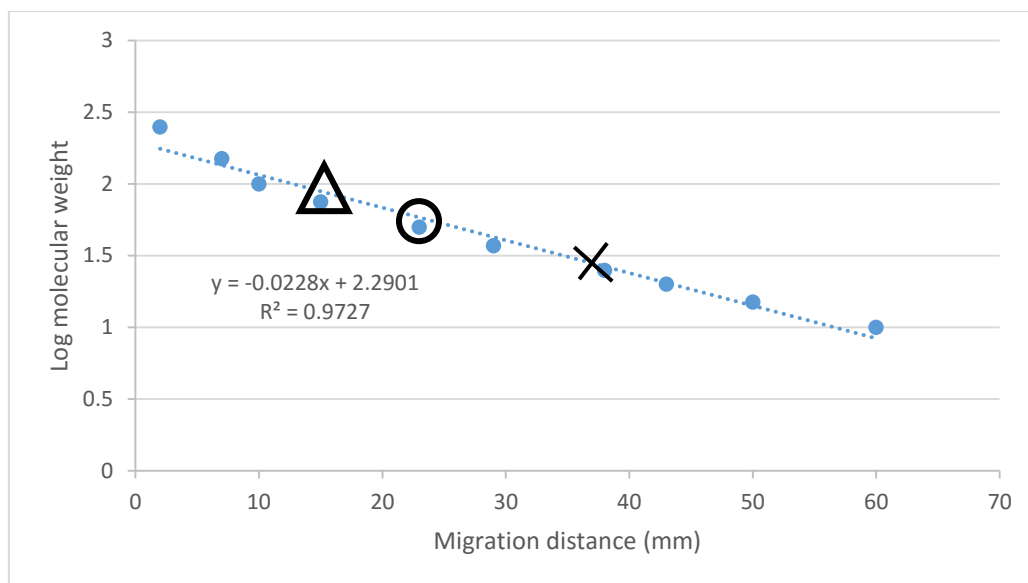
Figure 6. 9 Standard curve of the western blot in Figure 3.7B showing the dimerization studies of HIV-1 subtype C integrase and inhibitors. The X, circle and triangle indicates the migration of the bands to calculate the molecular weight
