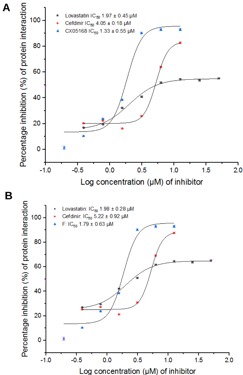
Figure 3. 5: Effects of lovastatin, cefdinir and CX05168 on the HIV-1IN-LEDGF/p75 interaction for HIV-1IN subtype B ( A ) and subtype C ( B ). The representative data of the dose response of lovastatin (square), cefdinir (circle) and CX05168 (triangle) on the HIV-1 IN-LEDGF/p75 AlphaScreen assay. The average values from 3 independent experiments are shown. The curves for each compound were plotted on the same graph for comparative purposes showing standard error bars.
