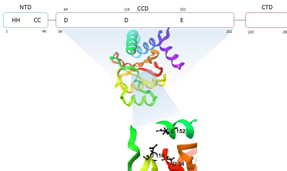
Figure 1. 4: The basic layout of HIV-1 integrase with the ribbon structure of the Catalytic Core Domain. The figure shows the formation of the DDE triad motif made up of D64, D116 and E152. Ribbon structure adapted from Protein Data bank 5KRT with use of Maestro 11.2, Schrodinger, 2017.
