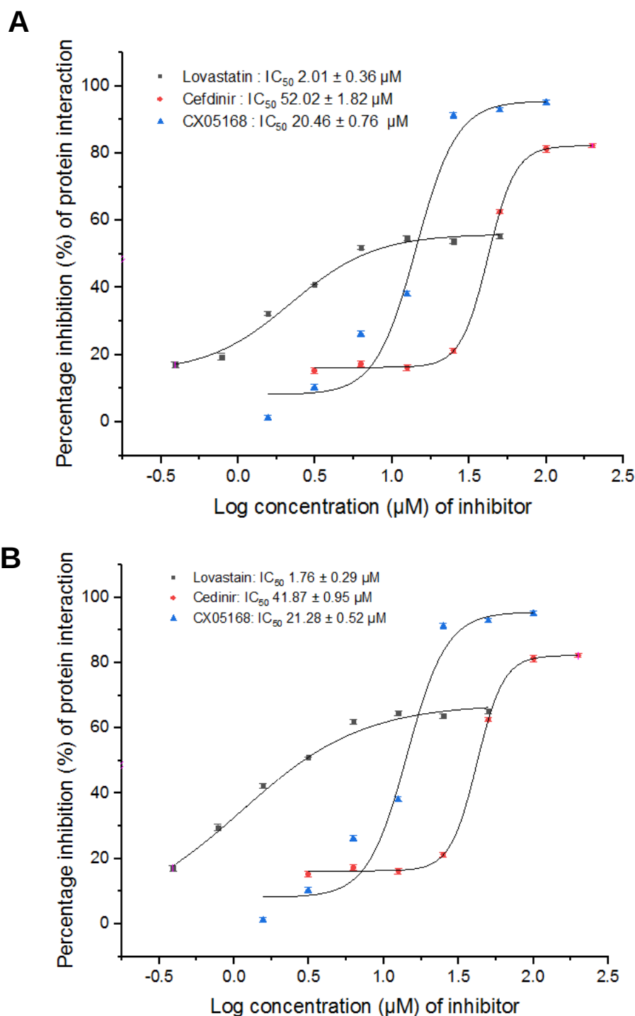
Figure 3. 6: Effects of lovastatin, cefdinir and CX05168 on the DNA-HIV-IN-LEDGF/p75 interaction of HIV-1 IN subtype B (A) and subtype C (B). Representative data of the dose response on the DNA-HIV-1IN-LEDGF/p75 interaction AlphaScreen assay. The average values for 3 independent experiments are shown. The percentage inhibition was calculated for the experiment and was plotted against the log of the concentration.
