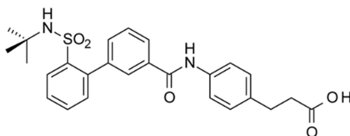
Figure 1. 23: Chemical structure of a t-butylsulfonamide discovered to have ALLINI properties. Copied from Burlein et al (Burlein et al. , 2017).
