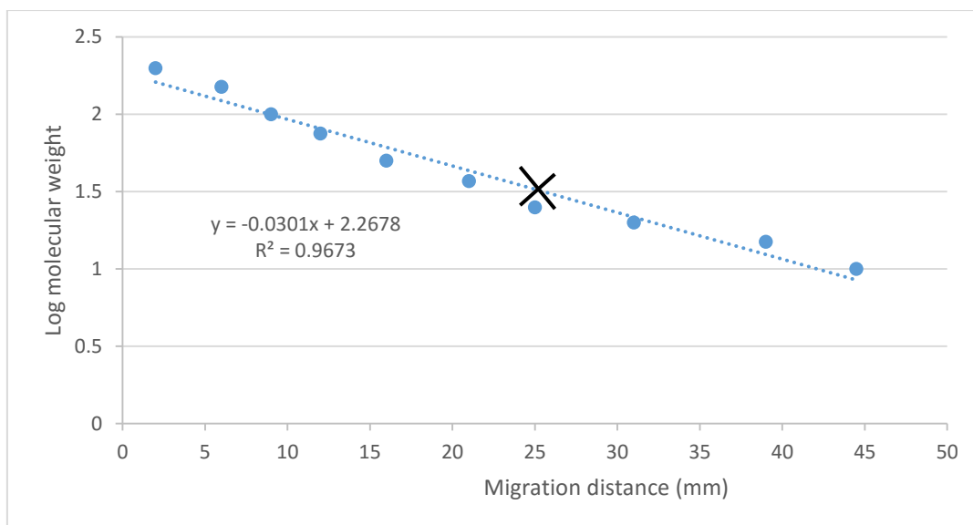
Figure 6. 3 Standard curve for western blot in Figure 3.1 C confirming the expression of subtype B and C integrase. The X indicates the migration of the band to calculate the molecular weight
