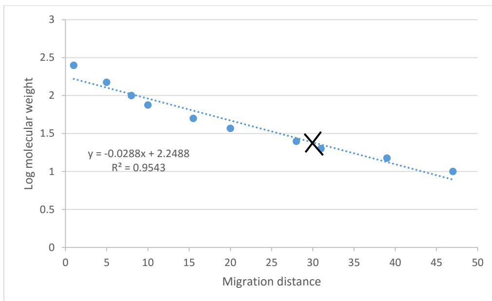
Figure 6. 7 Standard curve of the western blot in Figure 3.3 B showing the successful cleavage of the HIS tag from HIV-1 subtype B and C integrase. The X indicates the migration of the band to calculate the molecular weight.
