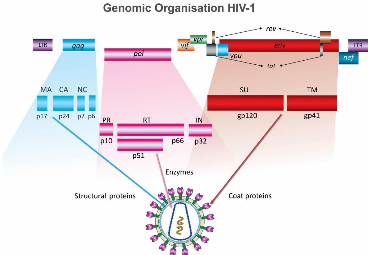
Figure 1. 1. Genomic organization of the HIV-1 genome displaying the three main structural, catalytic and envelope genes gag , pol and env flanked by two identical long terminal repeats. The gag gene codes for matrix protein, capsid proteins and nuclear cytoplasm. The pol gene codes for protease, reverse transcriptase and integrase proteins and the env gene codes for gp120 and gp41 proteins. Arrows point from the proteins towards the virion particle indicating which part of the particle they form. The figure includes regulatory genes tat and rev , and accessory genes vif , vpr , vpu and nef , needed for permanence of the virus. Picture adapted from www.stanford.edu/group/virus/retro/2005gongishmail/HIV.html .
