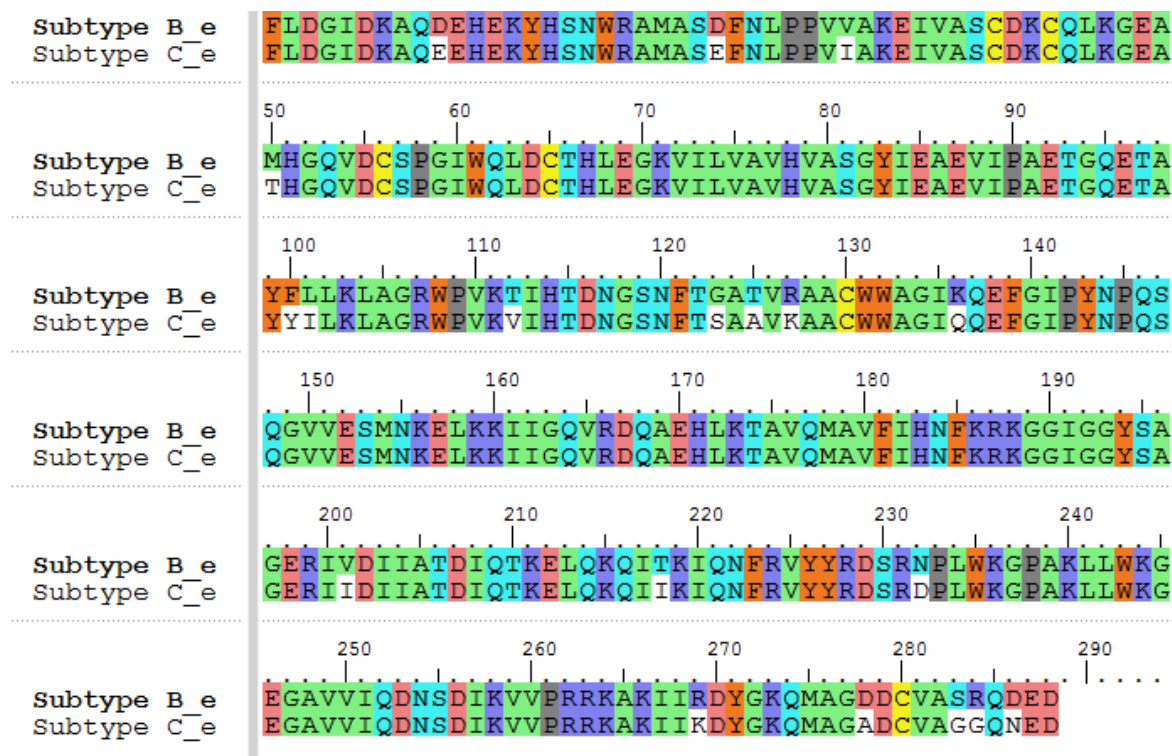
Figure 1. 6: Sequence alignment map comparing Subtype B integrase (first line) and subtype C integrase (second line). Where the difference in residues are not highlighted on the second line. The sequence alignment was done using Maestro BioLuminate 11.2, Schrodinger, 2017
