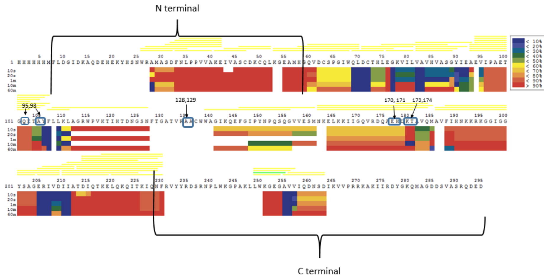
Figure 3. 12: Hydrogen exchange heat map of HIV-1 subtype B integrase in absence of compound with deuteriation for 10s, 20s, 1min, 10min and 60 min. The N terminal domain and C terminal domain are labelled with the important amino acids of 128, 129, 170, 171, 173 and 174 highlighted for ease of analysis. Red areas indicate high deuterium exchange, i.e. accessibility, whereas the blue areas indicate that the site is restricted. No shading indicates areas with no peptide coverage. The yellow lines indicate overlapping peptides.
