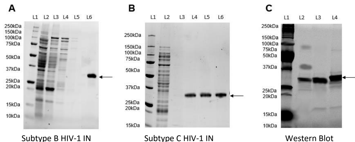
Figure 3. 1: SDS PAGE gel and western blot indicating the expression and purification of a protein at approximately 32 kDa correlating with that of recombinant subtype B HIV-1 IN. (A) SDS-PAGE indicating the expression and purification of HIV-1 IN subtype B, Lane 1, precision plus protein molecular weight marker (Bio-Rad, USA); Lane 2, flow through from the nickel affinity column; Lane 3, wash 1 from the nickel affinity column; Lane 4 wash 2 from the nickel affinity column; Lane 5, wash 3 from the nickel affinity column after which the protein was eluted via an imidazole gradient; Lane 6 lane containing concentrated fractions of a protein at approximately 32 kDa; (B) SDS-PAGE gel indicating the expression of a protein correlating with that of the recombinant subtype C HIV-1 IN. Lane 1, precision plus protein molecular weight marker (Bio-Rad, USA); Lane 2, flow-through from the nickel affinity column; Lane 3, wash 1 from the nickel affinity column; Lane 4, 5 and 6 containing at protein at 32kDa; (C) Western blot analysis confirming expression of recombinant HIV-1 IN subtype B and subtype C. Lane 1, precision plus protein molecular weight marker (Bio-Rad, USA); Lane 2, positive control recombinant HIV-1 IN obtained from the NIH AIDS Research and Reference Reagent Program; Lane 3, subtype B protein from gel A; Lane 4 concentrated nickel affinity chromatography purified subtype C HIV-1 IN from gel B. Figures 6.1,6.2 and 6.3 (found in the appendix) are the standard curves used to determine protein size marked with an X. for A, B and C respectively.
