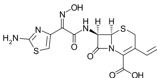
Figure 1. 26: Structure of cefdinir drawn with use of Maestro 11.2, Schrodinger, 2017.
