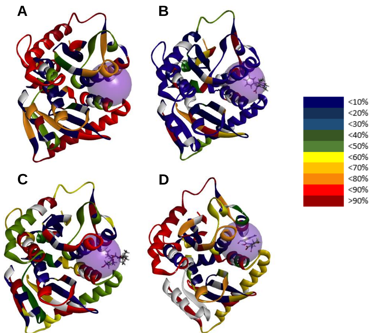
Figure 3. 17: HIV IN ribbon structure displaying the binding site for compound and the respective deuterium exchange in the absence of a bound compound on different parts of the subtype C HIV-1 IN enzyme (The ribbon structure of subtype B has been used as there is no subtype C structure). The purple globe highlights the binding site. The deuterium exchange has been indicated with colour change depending on the rate of exchange for each part of the enzyme in correlation to the hydrogen deuterium exchange heat maps. The ribbon structure was compiled with the use of Maestro 11.2, Schrodinger, 2017. (A) Subtype C HIV-1 IN with no compound bound. (B) Subtype C HIV-1 IN treated with CX05168. (C) Subtype C HIV-1 IN treated with lovastatin and Figure D is subtype C HIV-1 IN treated with cefdinir.
