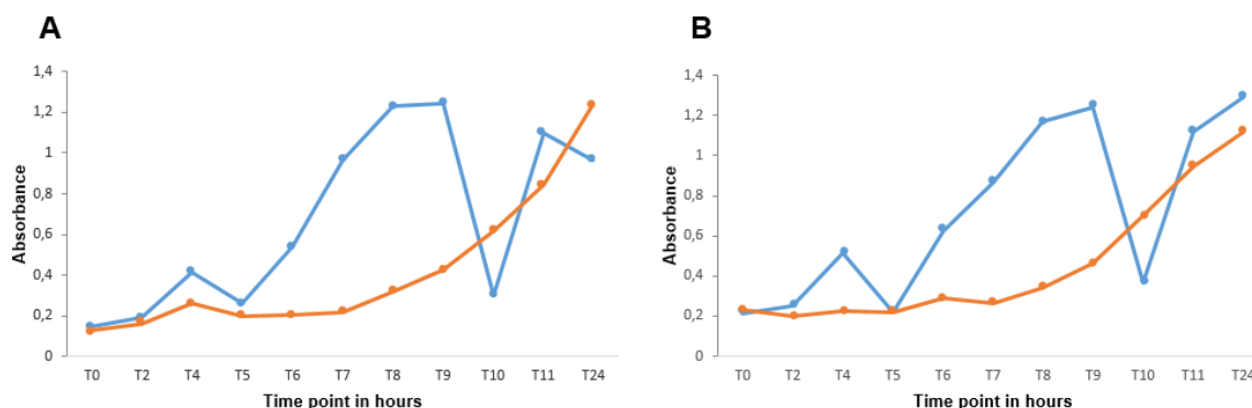
Figure 3. 21: TOA results for the antiviral effects of cefdinir and CX05168 compounds at specified time points for subtype B (A) and C (B) integrase. The blue line represents cefdinir at 100 µM and the orange trend line represent CX05168 treatment at 30 µM. The experiment for CX05168 was conducted in duplicate per experiment and 3 separate experiments were conducted. Cefdinir was tested in duplicate per experiment and 12 separate experiments were conducted.
