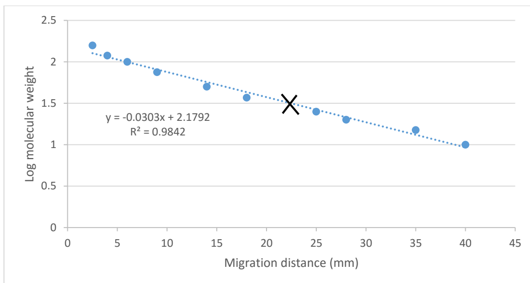
Figure 6. 1 Standard curve for SDS PAGE gel in Figure 3.1 A for the purification and expression of HIV-1 subtype B integrase. The X indicates the migration of the band to calculate the molecular weight
