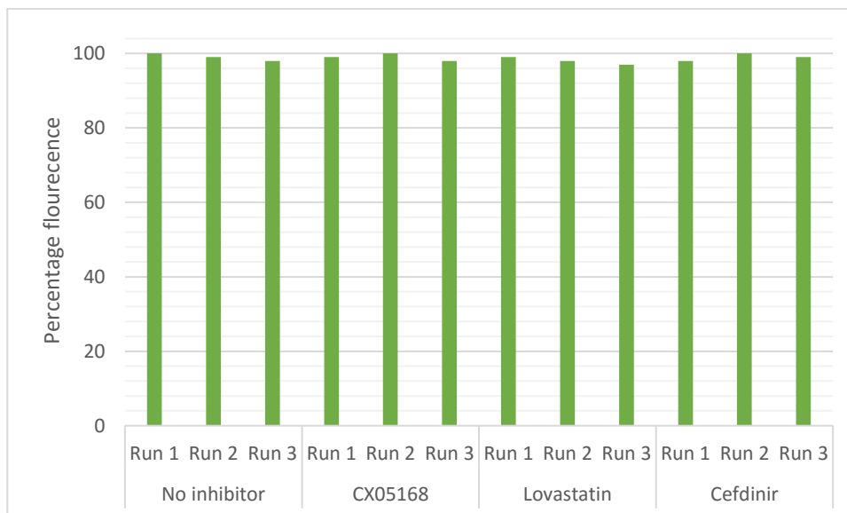
Figure 3. 7 Column graph showing the percentage fluorescence of the POGz-LEDGF/p75 interaction Alphascreen assay. Each inhibitor was run in triplicate. Full fluorescence shows a strong interaction between POGz and LEDGF/p75.
