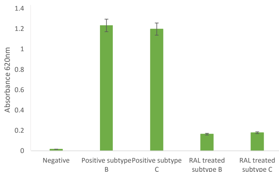
Figure 3. 4: Bar graph depicting the strand transfer activity by ELISA of both subtype B and C IN with and without addition 50nM raltegravir. The ELISA was run 3 times with duplicate samples in each run. The error bars are shown for the difference in the experimental results from each experiment. The positive samples are protein with no compound added and the negative is the absence of protein from the well.
