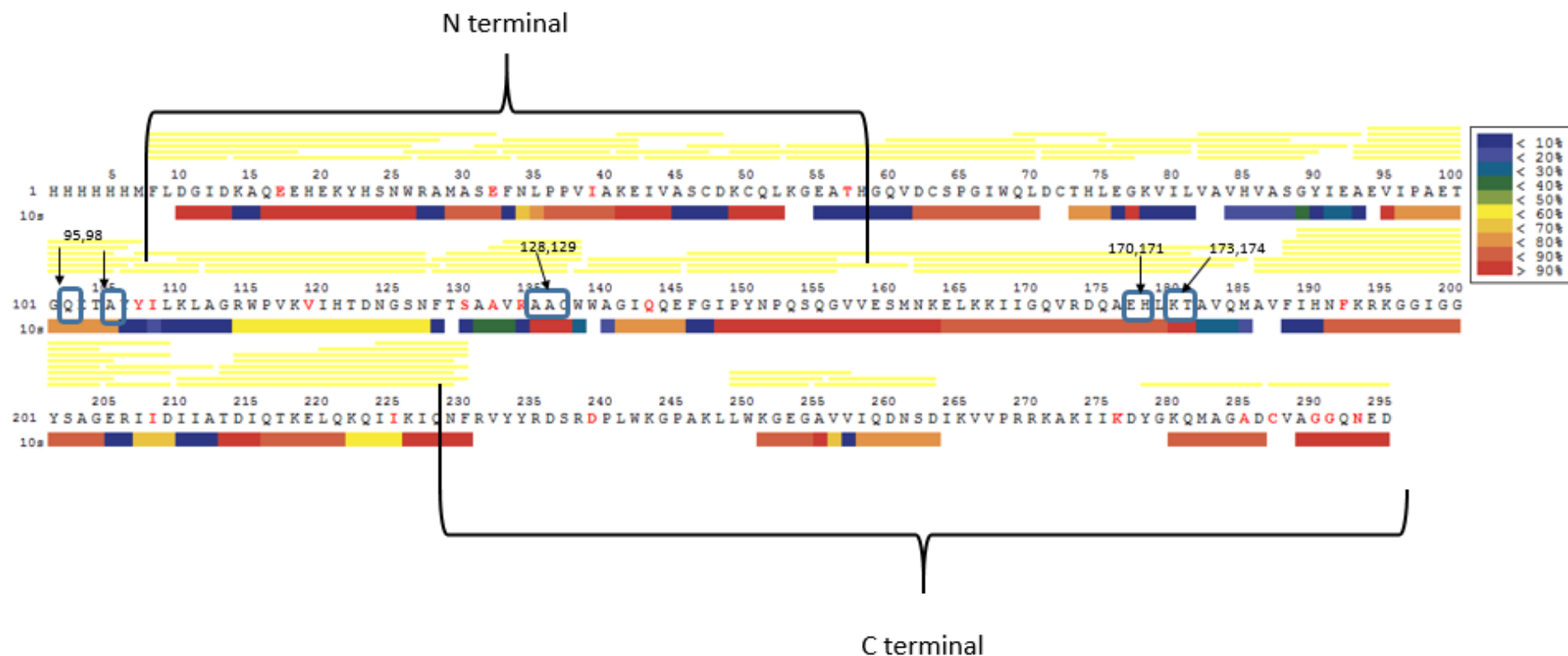
Figure 6. 15: Hydrogen exchange heat map of subtype C integrase with deuteration for 10s treated with cefdinir. The N terminal domain and C terminal domain are labelled with important amino acids of 95, 98, 128, 129, 170, 171, 173 and 174 highlighted for ease of analysis. Amino acids that have changed from subtype B are in red.
