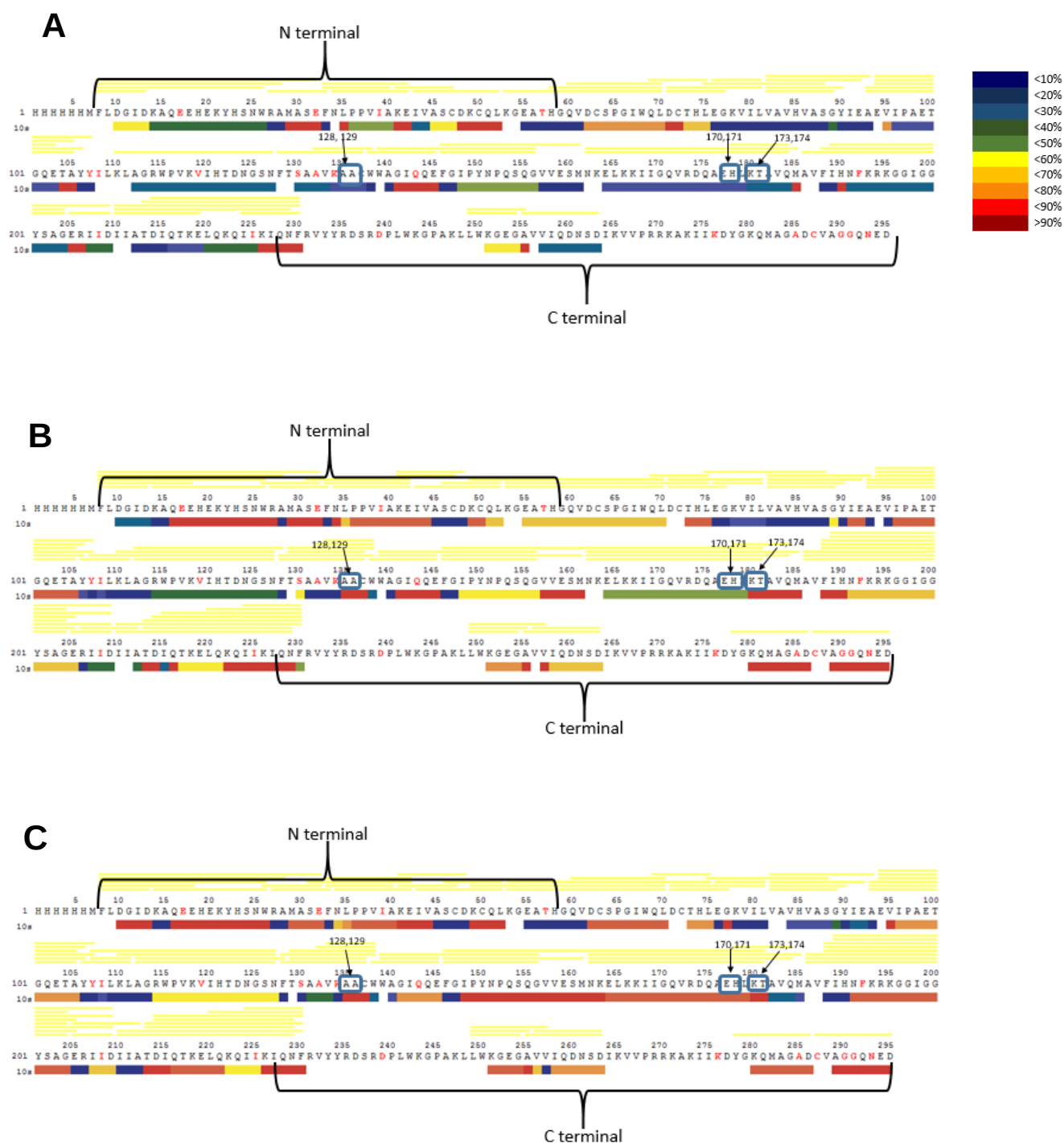
Figure 3. 16: Hydrogen exchange heat map of HIV-1 subtype C integrase with deuteration for 10s treated with CX05168 (A), lovastatin (B) and cefdinir (C). The N terminal domain and C terminal domain are labelled with important amino acids of 128, 129, 170, 171, 173 and 174 highlighted for ease of analysis. Red areas indicate areas of high exchange whereas blue areas indicate restricted hydrogen exchange. The colour key can be found on the right hand top corner.
