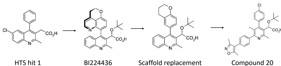
Figure 1. 22: The development progress of NCINI compounds from the original hit from library screening to the development of BI224436, through the scaffold jump to the new compound 20 with improved enteropathic recirculation. Constructed from Fenwick et al and Fader et al , (Fenwick et al. , 2014; Fader et al. , 2014a).
