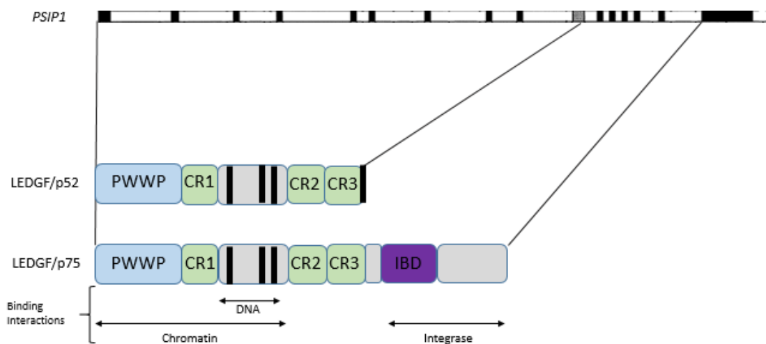
Figure 1. 8: The PSIP1 gene showing the exons and introns indicated in black and white respectively. Including the 2 splice variants LEDGF/p52 and LEDGF/p75 showing the binding interaction on the proteins where chromatin, DNA and integrase. Both proteins show the PWWP domain and LEDGF/p75 shows the integrase binding domain.
