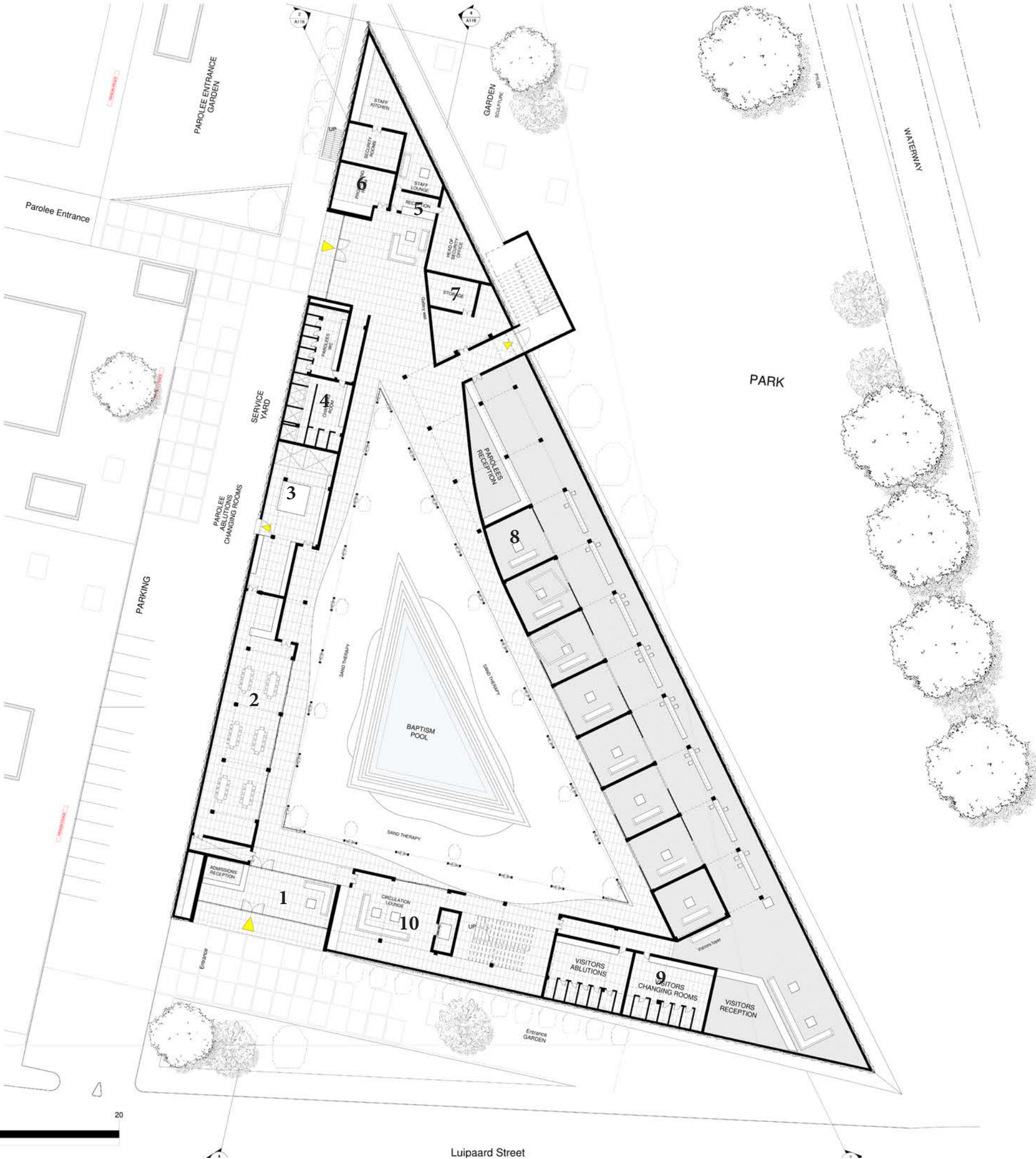
Fig.7.4 Ground Floor (Author 2021)
