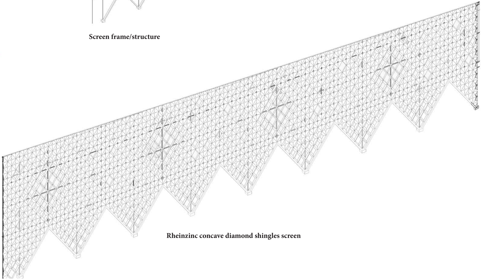
Fig.7.16 Screen drawings (Author 2021)
