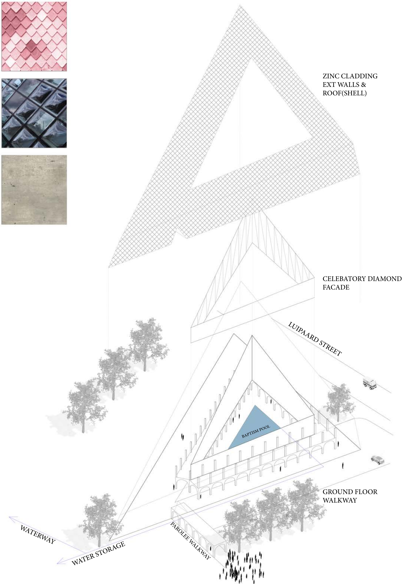
Figure 6.10 axo full exploration (Author 2021)
