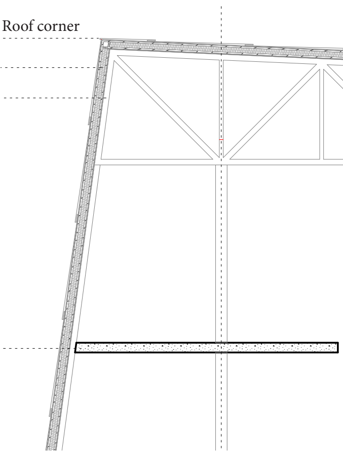
Roof detail
