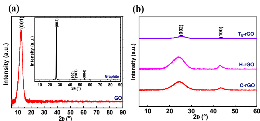
Figure 1. X-ray diffractograms for (a) GO (inset: graphite) and (b) rGO samples.
