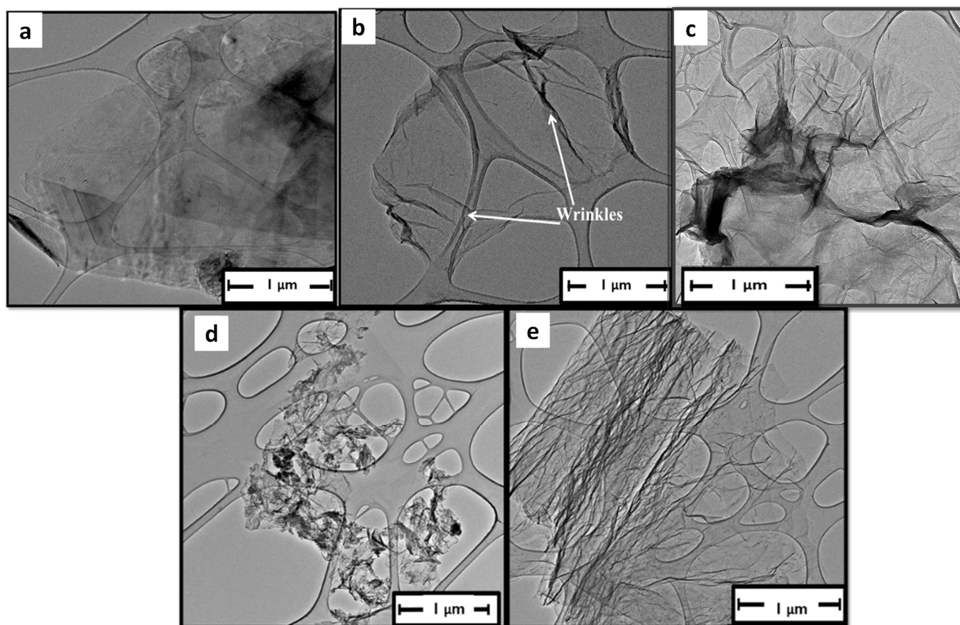
Figure 3. TEM micrographs of (a) graphite, (b) GO, (c) H-rGO, (d) C-rGO, (e) and T N -rGO.
