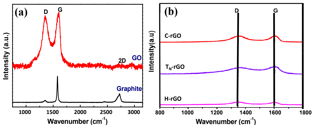
Figure 2. Raman spectra of (a) graphite and GO and (b) rGO samples.
