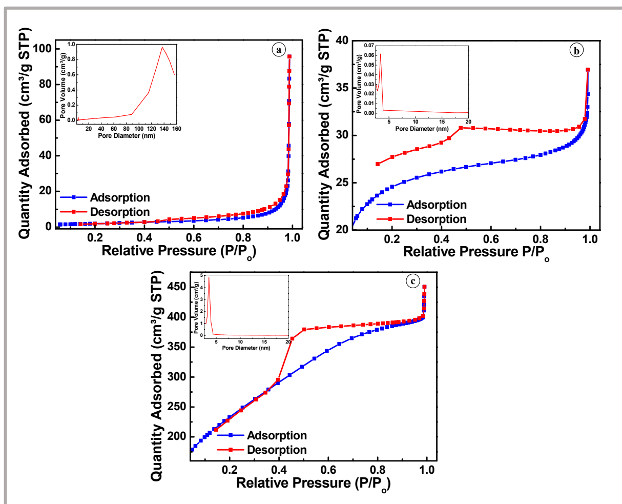
Figure 4. N 2 adsorption–desorption isotherms and their respective pore diameter distribution curves (inset) for graphite (a), GO (b), and H-rGO (c).
