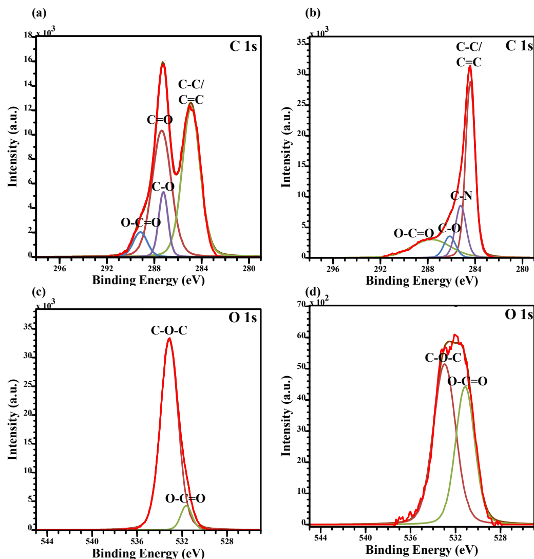
Figure 6. High-resolution XPS spectra of deconvoluted C 1s and O 1s for GO (a,c) and H-rGO (b,d).
