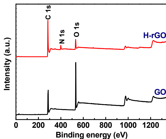
Figure 5. XPS survey spectra of GO and H-rGO.
