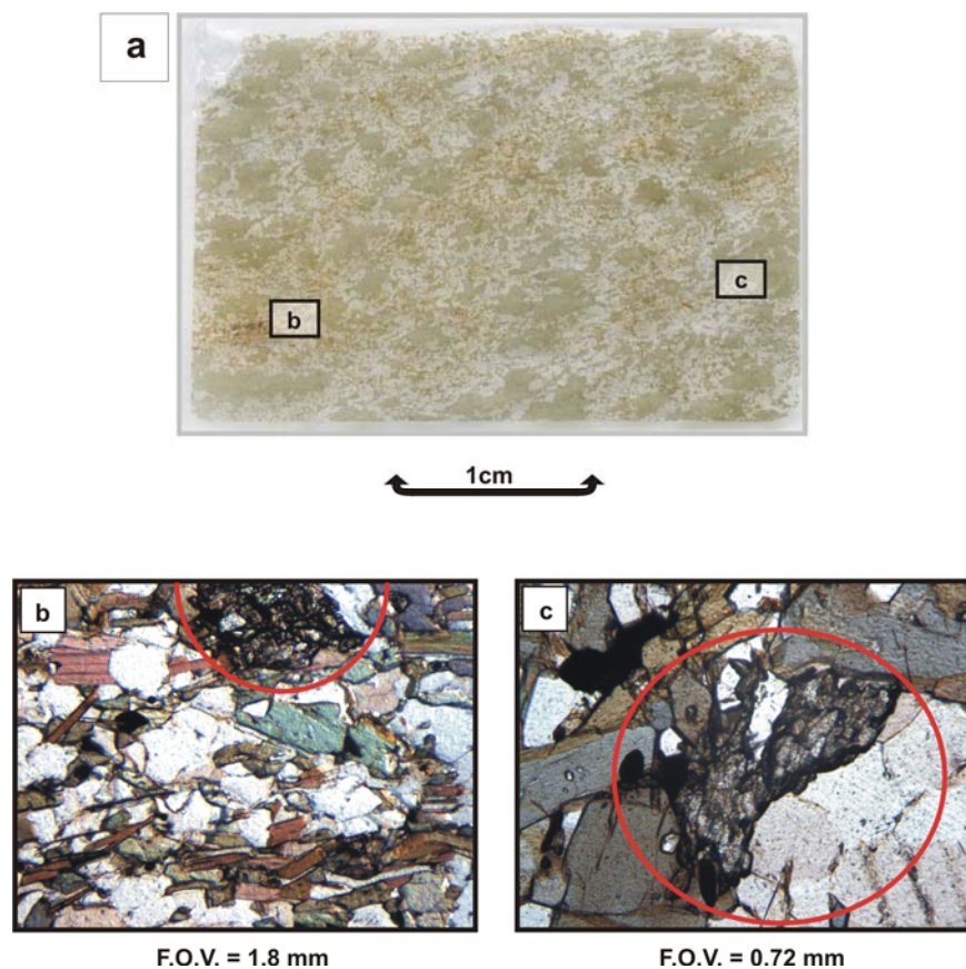
Figure 4.5 Photomicrographs of sample NMo4-3 (metagabbro, Sørøya). (a) shows the sub-parallel alignment of hornblende clusters. The orange colouring is caused by the presence of metamorphic titanite and rutile from the breakdown of hornblende. (b & c) Titanite (indicated in red circles) occurs in clusters of subhedral-anhedral crystals associated with hornblende, commonly with a crosscutting relationship.
