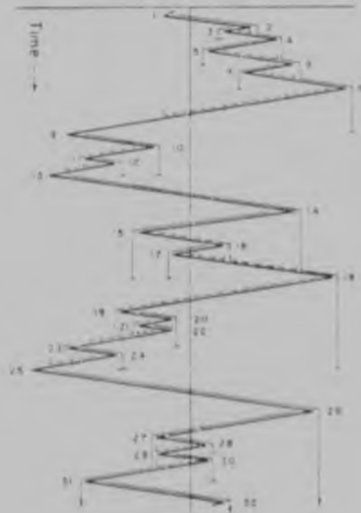
FIGURE 3.2 : Example of range-pair cycle counting method
