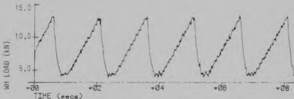
FIGURE 2.16 : Dynamic calibration at frequency of 0,7 hz and amplitude of 9 kN (Applied load fluctuates 4,5-13,5 kN)
