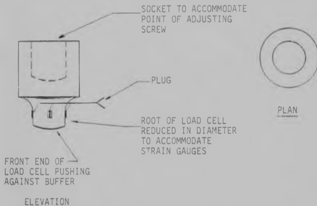
FIGURE 2.9 : SOCKET TYPE LOAD CELL
