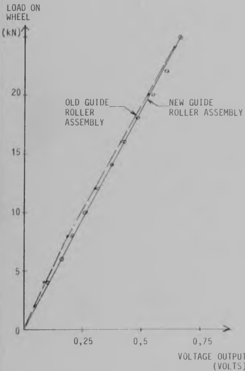
FIGURE 2.13 LOAD CELL NUMBER 3
