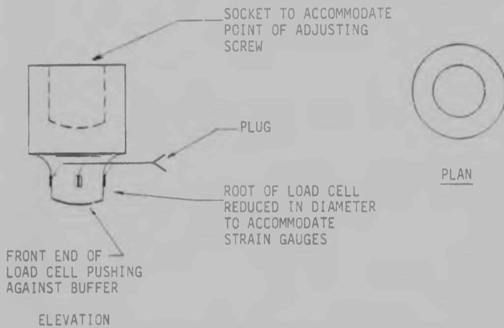
FIGURE 2.8 - SOCKET TYPE LOAD CELL
