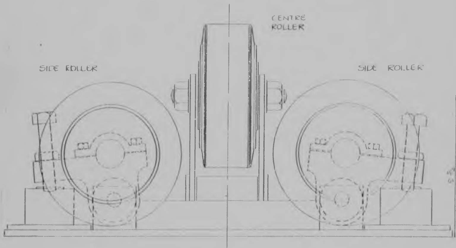
10" DIA GUIDE FRAME ASSEMBLY FRONT ELEVATION
