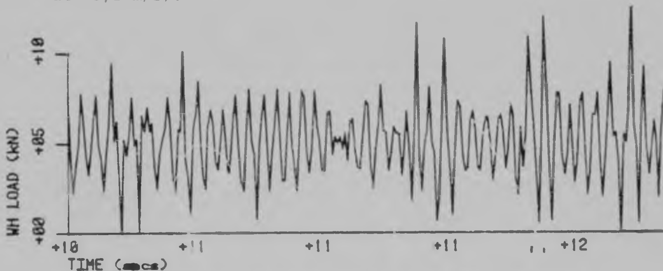
FIGURE 2.18 : Wheel load record, President Steyn No. 4 Shaft 10T skip hoisting at 15 m/s
