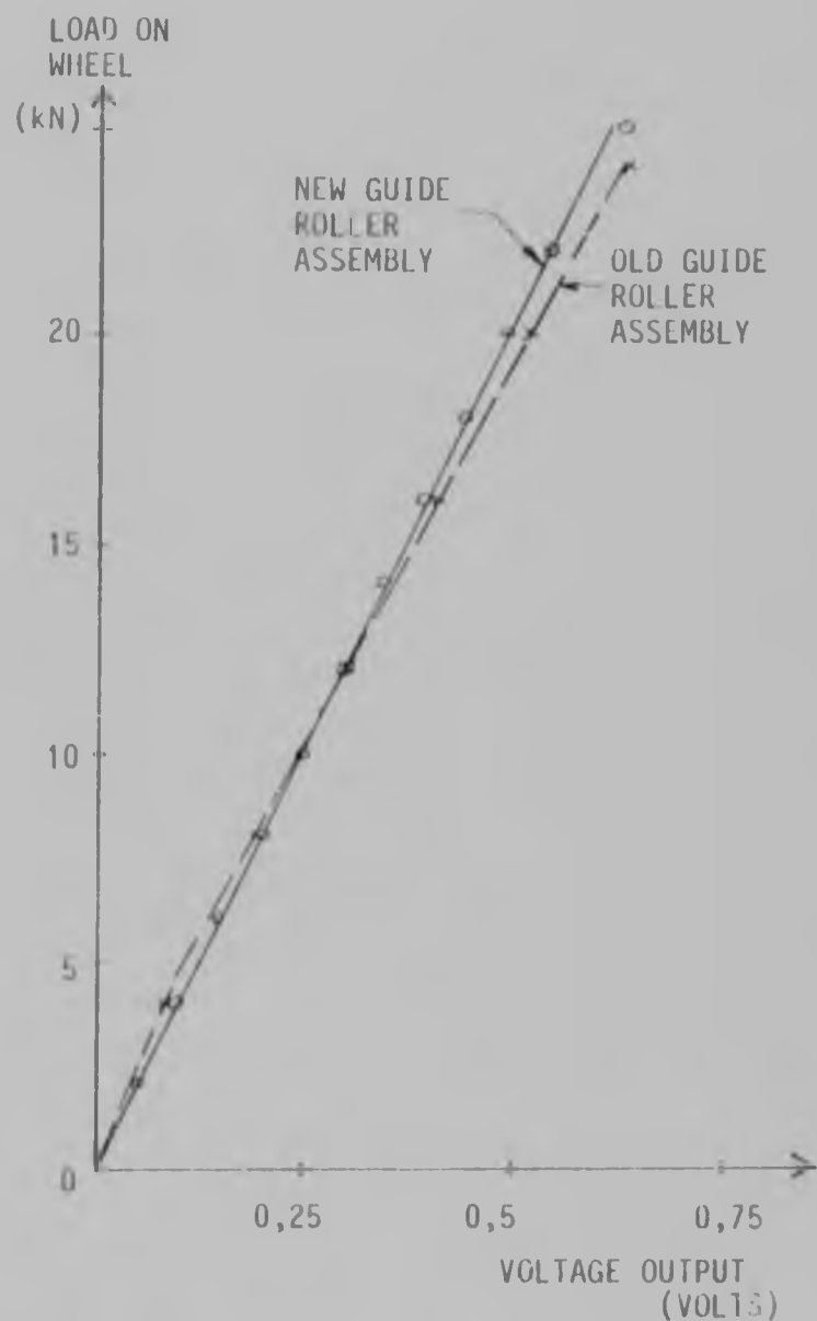
FIGURE 2.14 LOAD CELL NUMBER 4
