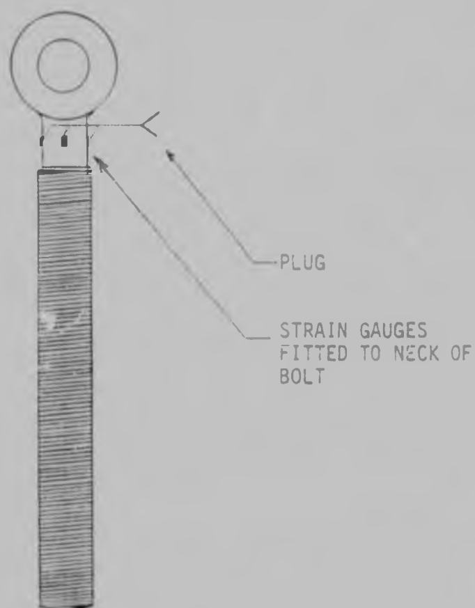
FIGURE 2.10 : LOAD CELL FOR 'SKF' GUIDE WHEELS
