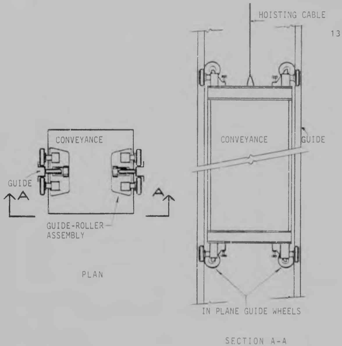
FIGURE 2.1 : CONVEYANCE ARRANGEMENT IN SHAFT
