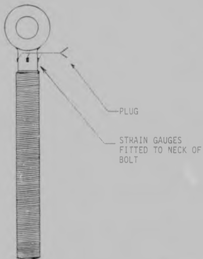
FIGURE 2.10 : LOAD CELL FOR 'SKP' GUIDE WHEELS
