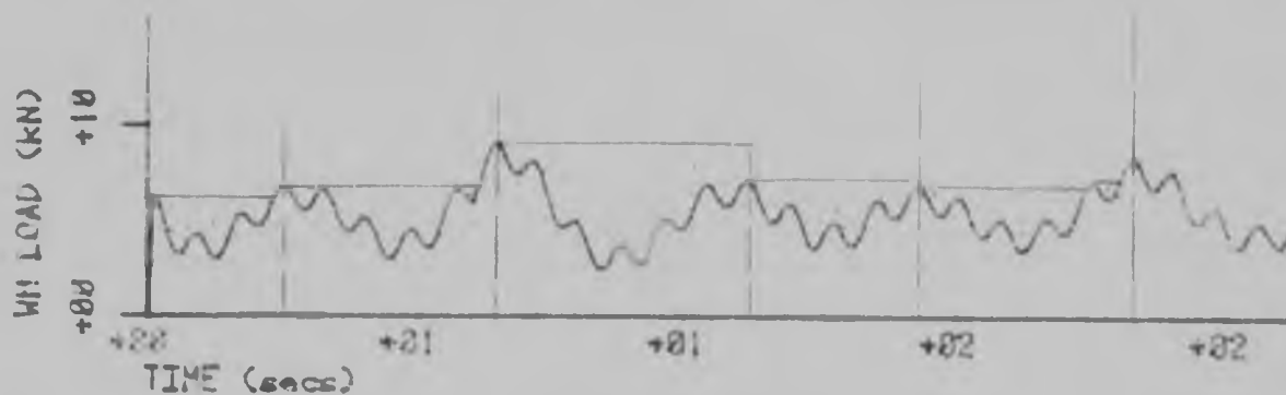
FIGURE 3.9 : Load record, ideally suited for analysis by the computer programme
