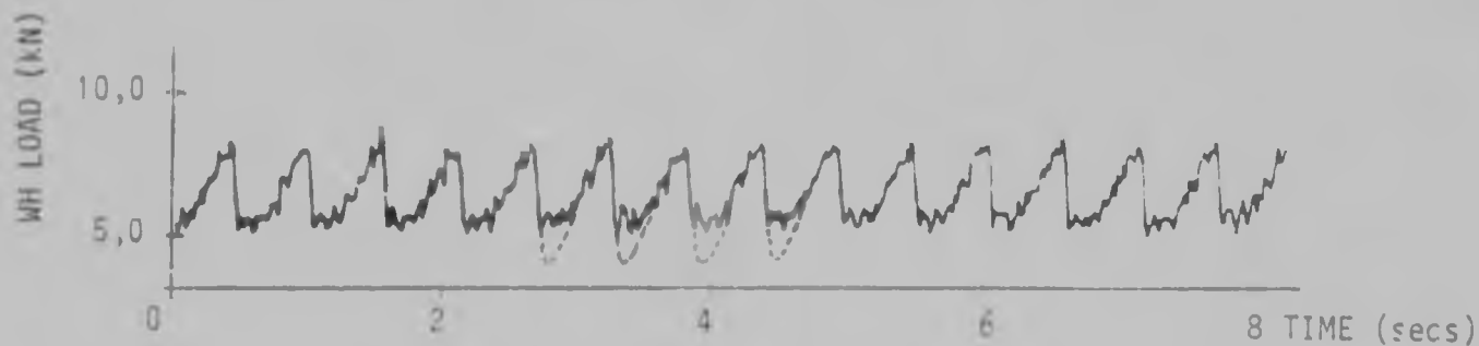
FIGURE 2.17 : Dynamic calibration at frequency of 1,85 hz and amplitude of 4 kN. (Applied load fluctuates 4,5-8,5 kN)
