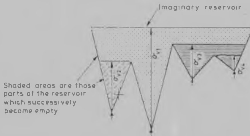
FIGURE 3.4 : Example of the reservoir method of cycle-counting
