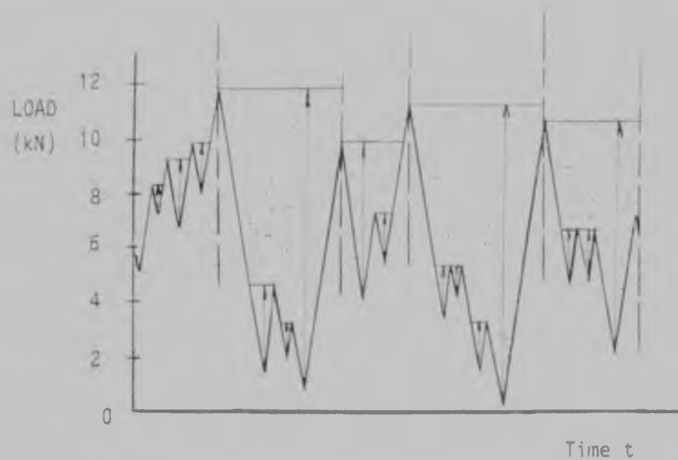
FIGURE 3.11 : Record used for comparing computer programme results to the cycle counting methods
