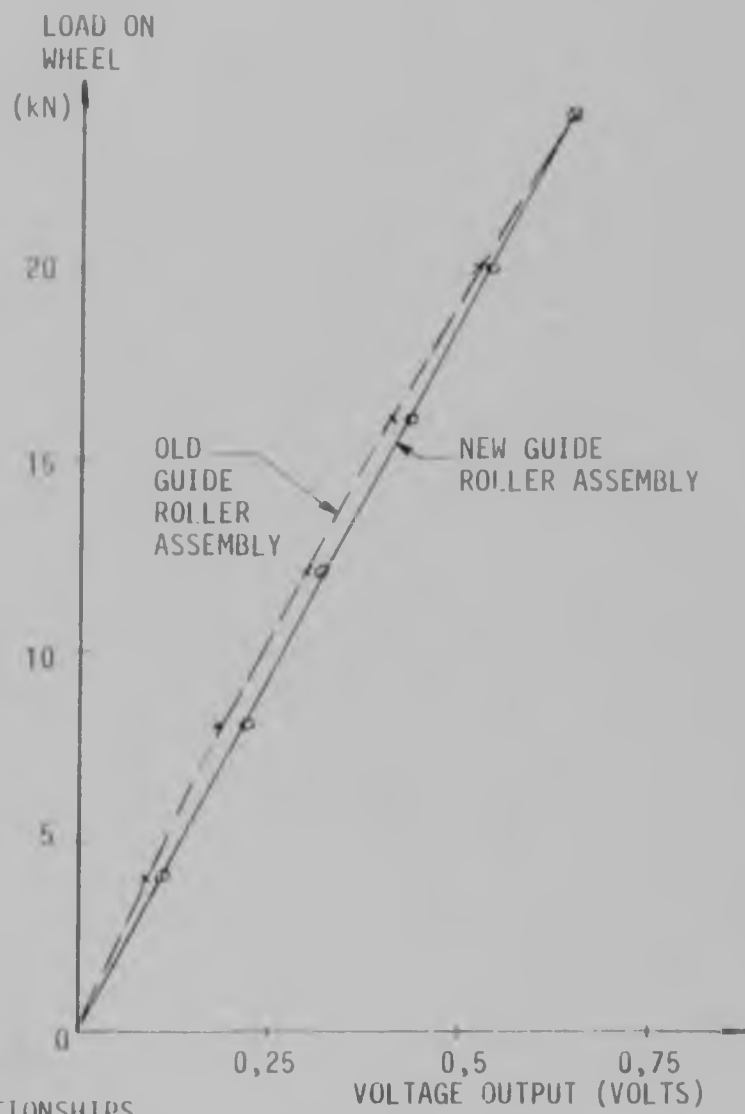
FIGURE 2.12 : LOAD CELL NUMBER 2
