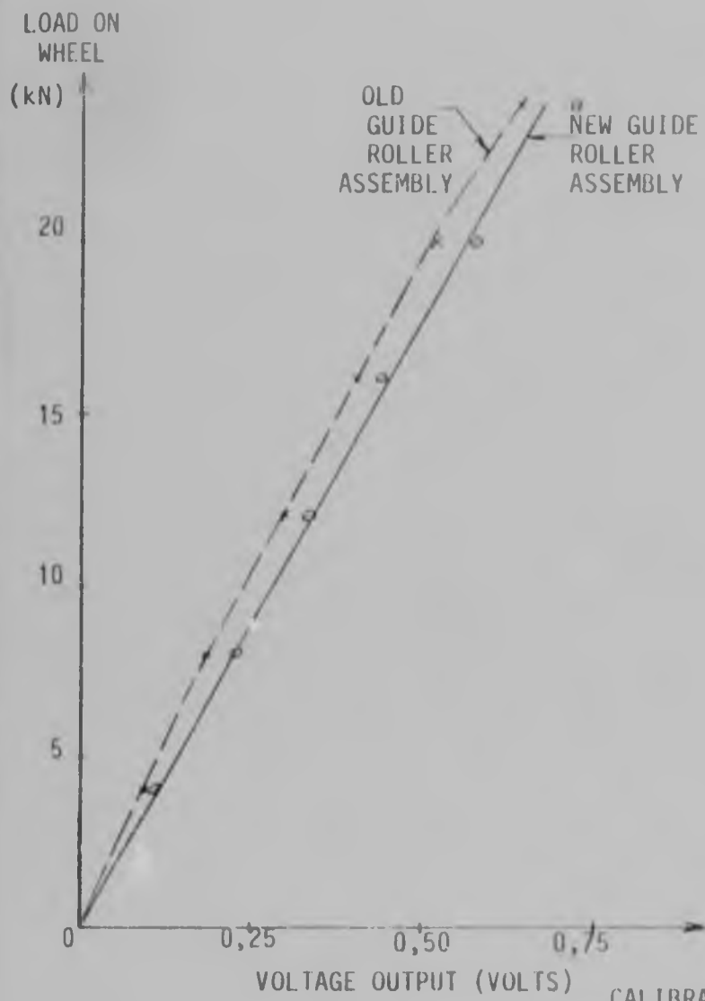
FIGURE 2.11 : LOAD CELL NUMBER 1
