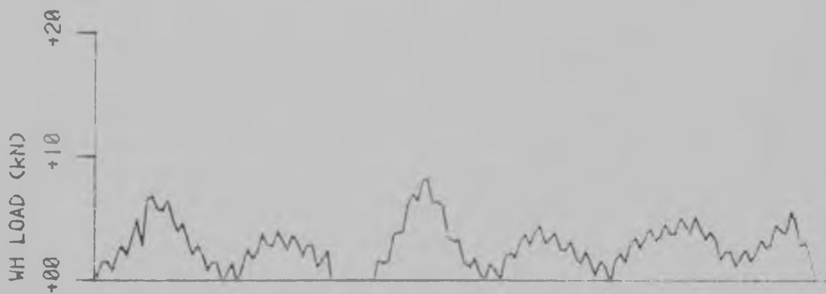
FIGURE 3.6 : Typical load record predicted by the theoretical DISCS model
