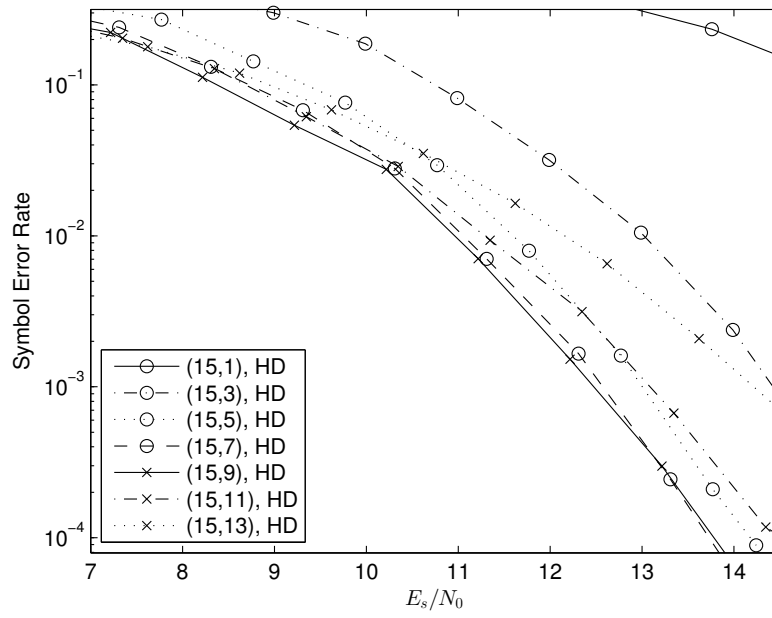
FIGURE 4.3: Comparison of code rates in an Alamouti MIMO environment
