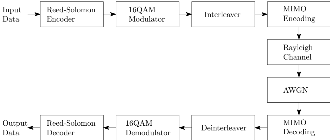
FIGURE 3.1: System Overview
