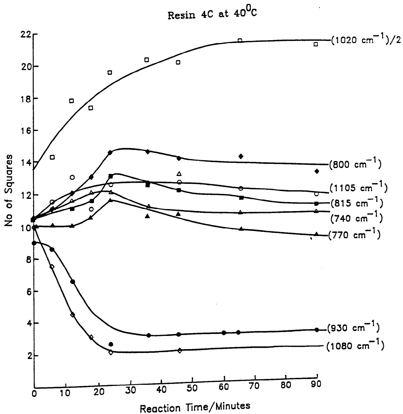
Figure 2.6 The change in concentration of the components of Resin 4C mix with reaction time at 40°C
