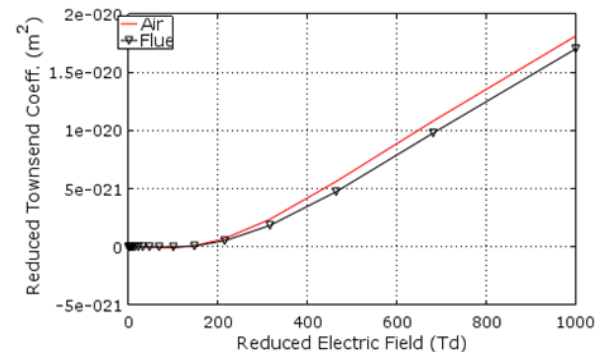
Figure 1: A comparison of Townsend's coefficients for air and engine exhaust flue gas compositions.
