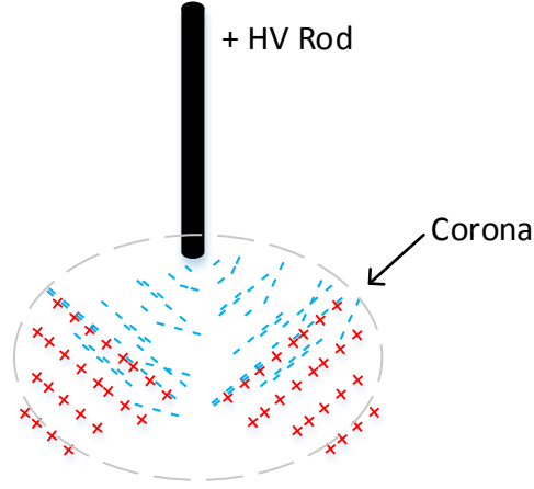
FIGURE 3.1: Schematic of the formation of corona due to localised avalanches.
