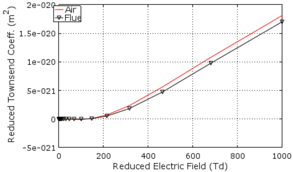
FIGURE 4.12: Effective ionisation coefficient for air and flue
