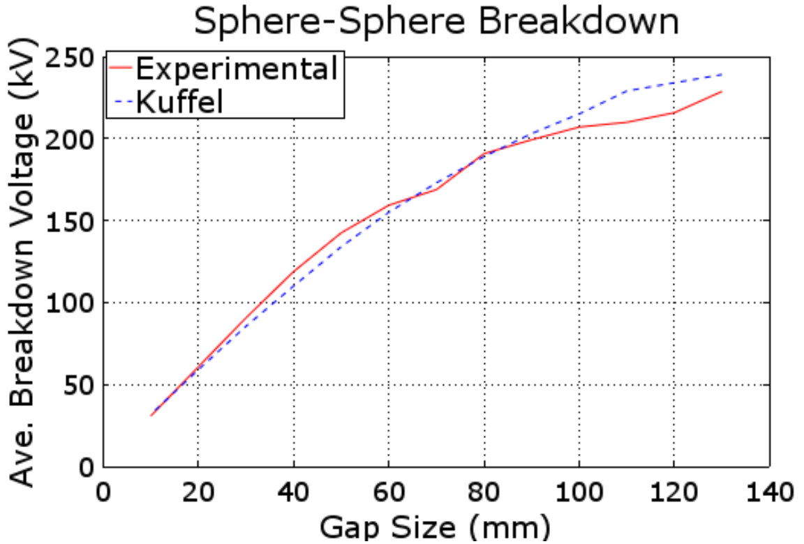
FIGURE 4.10: Sphere-Sphere breakdown calibration results compared to published data.
