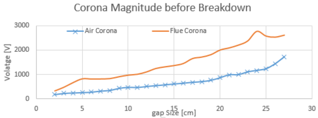
FIGURE 4.13: Pre-breakdown corona magnitude in air and in engine flue gas.
