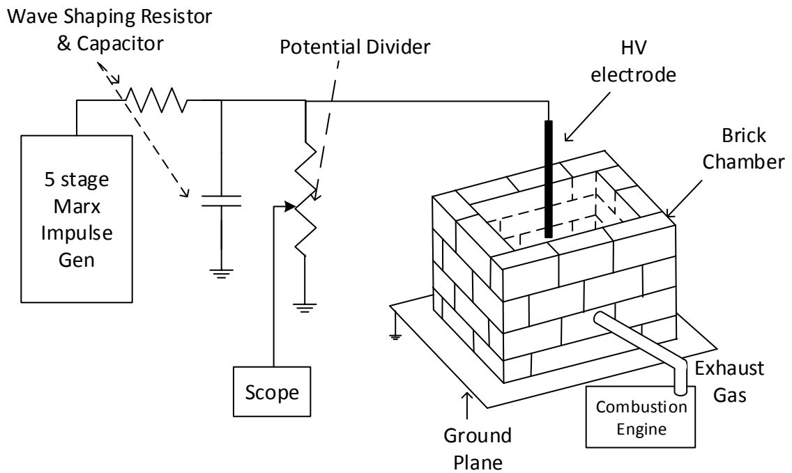
FIGURE 4.18: Impulse test setup
