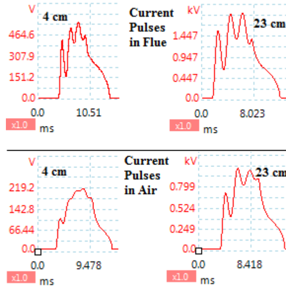
FIGURE 4.14: Comparison of pre-breakdown corona activity in air and flue at 4 cm and at 23 cm. CT output shown as voltage.
