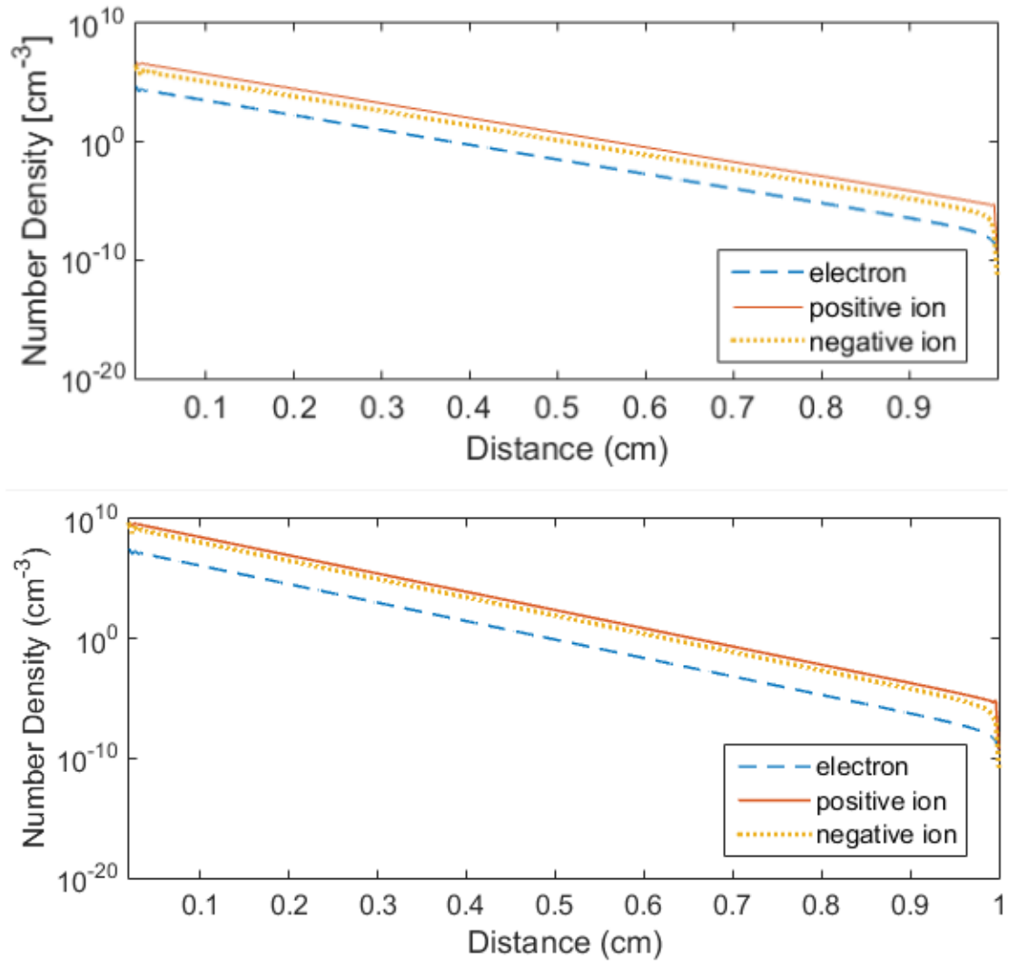
FIGURE 5.10: Space charge in air (top) and in flue (bottom) for a 1 cm gap size.
