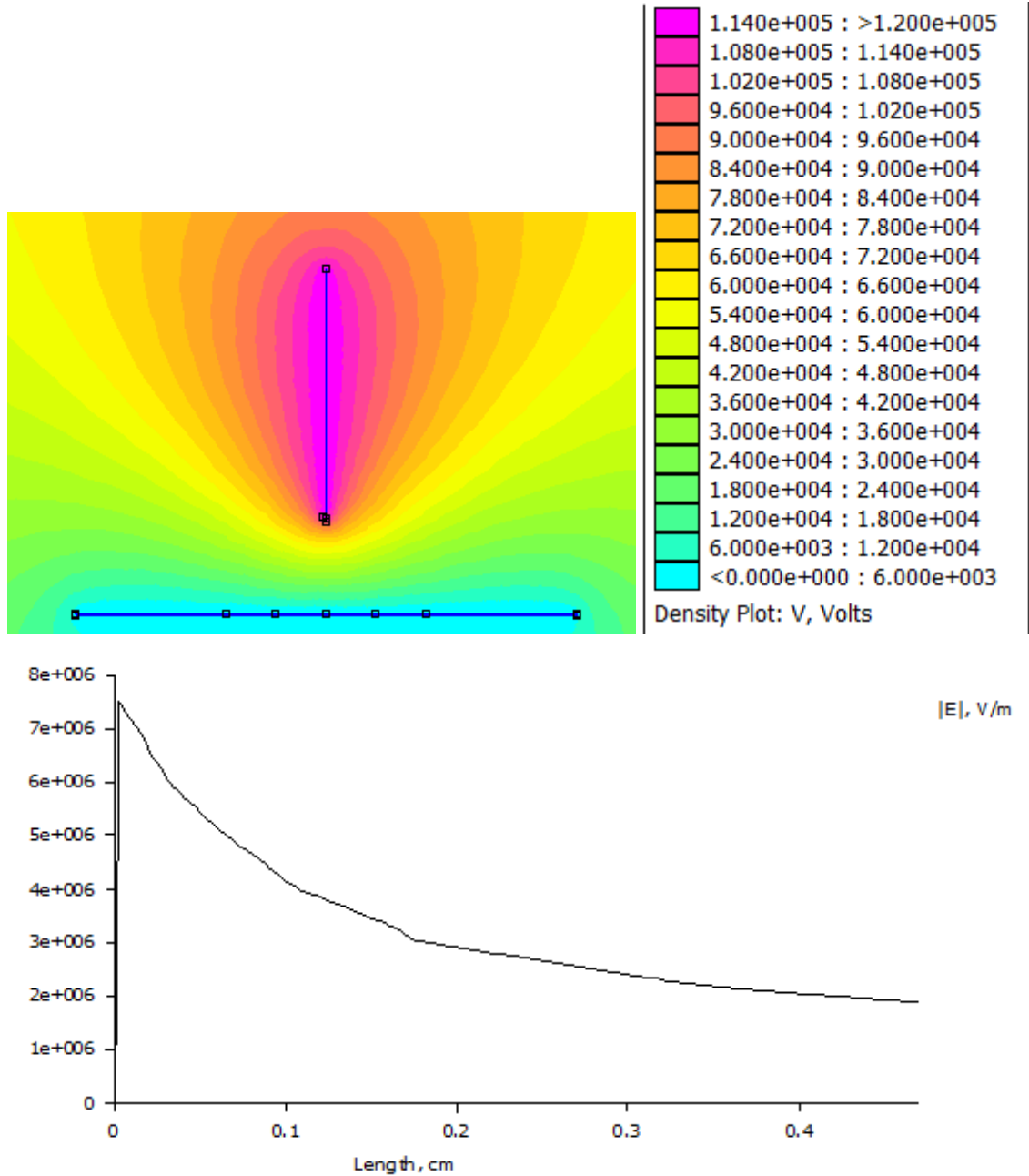
FIGURE 4.3: FEM simulation of a rod-plane geometry and its decaying field distribution within 0.4 cm of the gap from the HV electrode.
