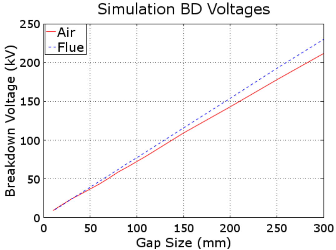
FIGURE 5.8: Simulation Results: breakdown characteristics of air and flue under standard conditions.
