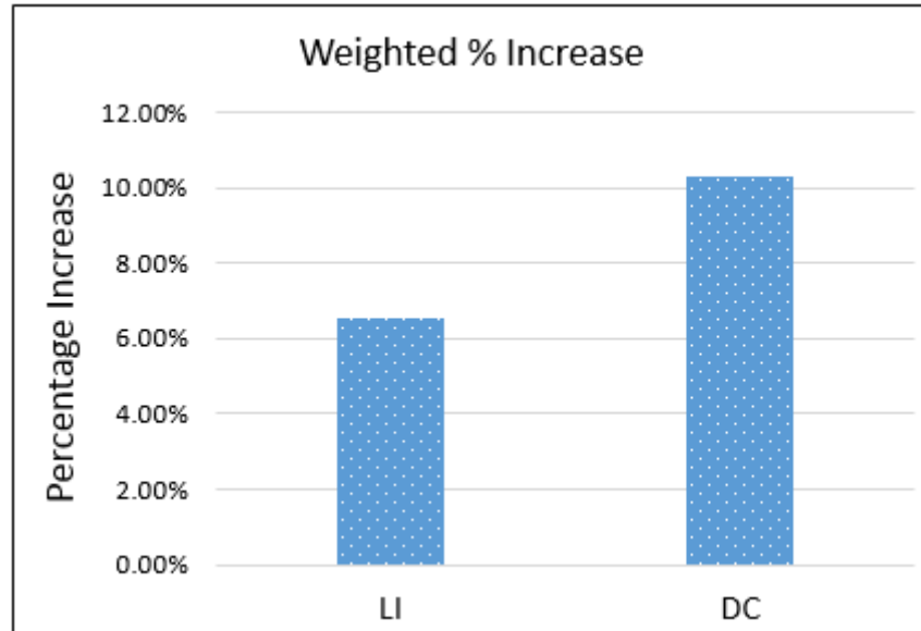
FIGURE 4.22: Weighted Mean Percentage Increase from air to flue experimental results in impulse tests and DC tests.
