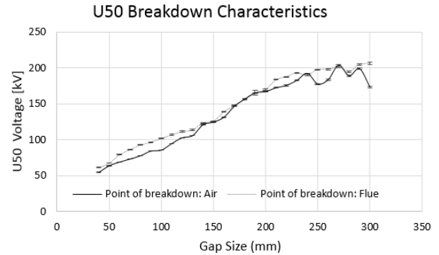
Figure 6: Experimental 1.2/50 \mu s impulse U50 breakdown characteristics for flue and air
