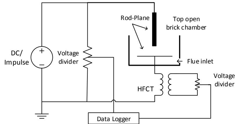
FIGURE 4.4: Experimental setup: testing DC breakdown of engine flue inside a brick chamber.
