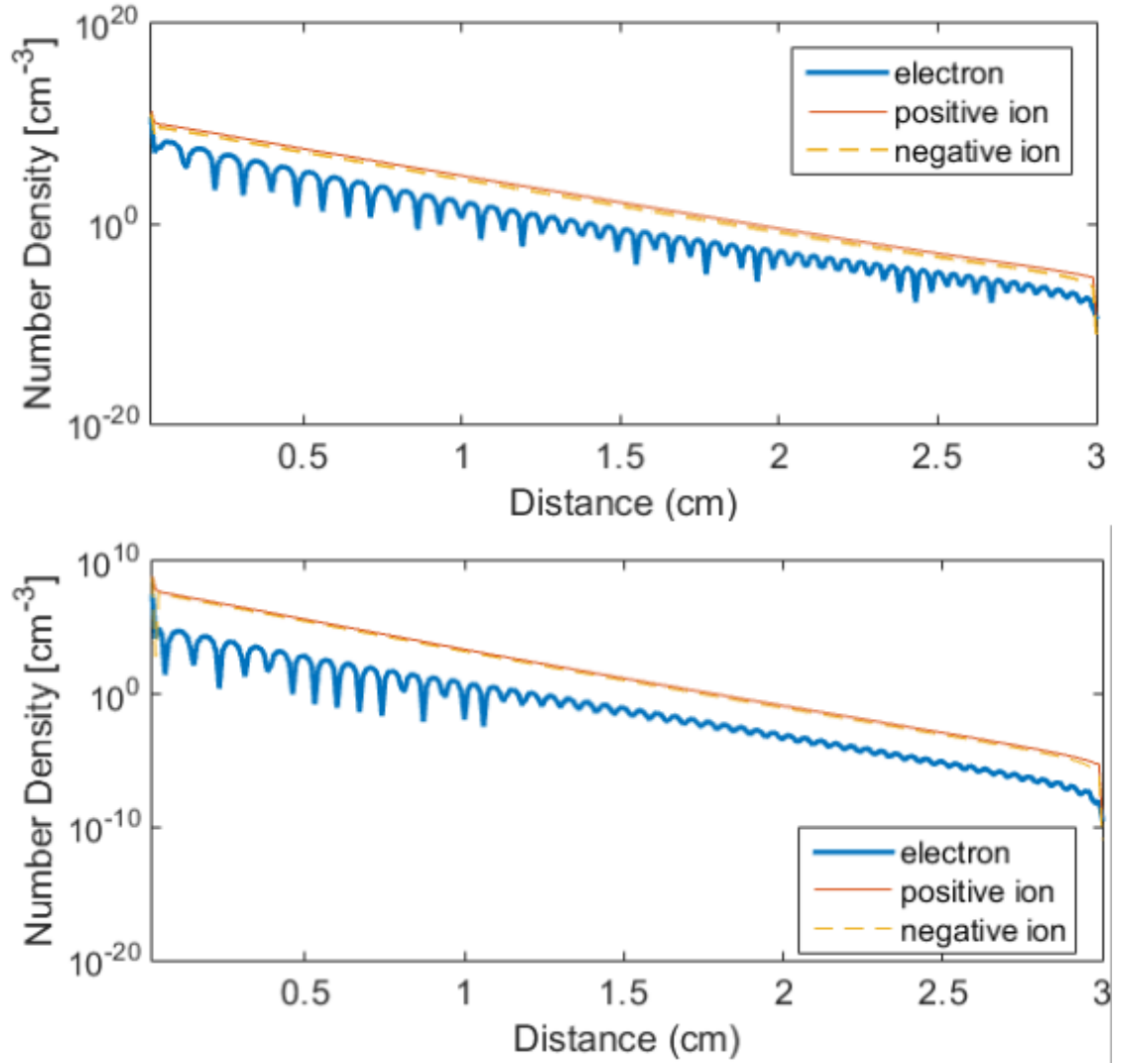
FIGURE 5.13: Space charge in air (top) and in flue (bottom) for a 3 cm gap size (the cross over).
