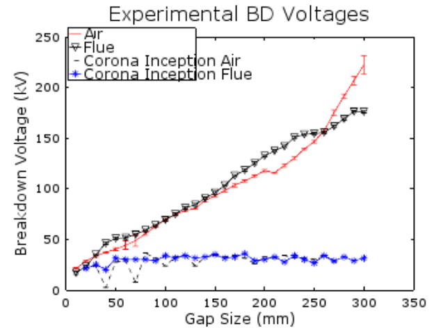
Figure 4: Corrected average DC breakdown and inception voltage curves for the rod-plane tests in air and flue.
