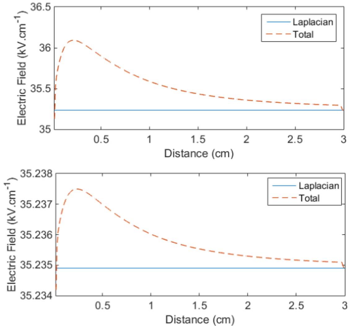
FIGURE 5.14: Electric field in air (top) and in flue (bottom) for a 3 cm gap size (the cross over).
