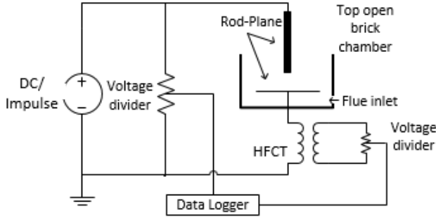
Figure 2: Experimental setup: Testing DC and impulse breakdown of engine flue and air.
