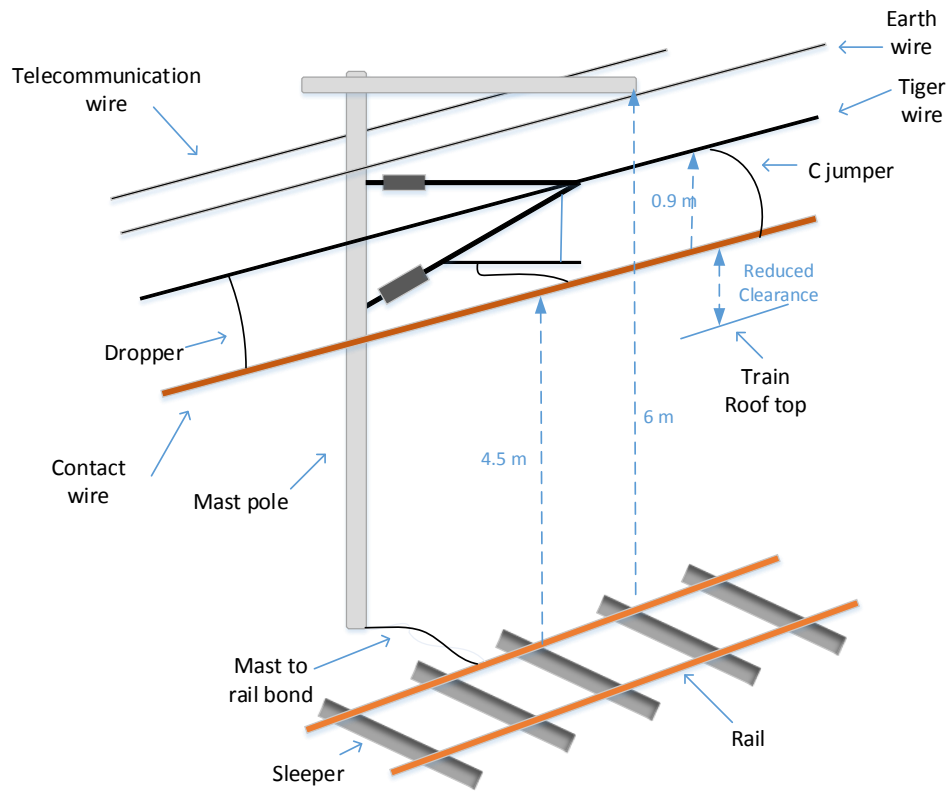
FIGURE 1.1: Illustration of RCS clearances and locomotive
