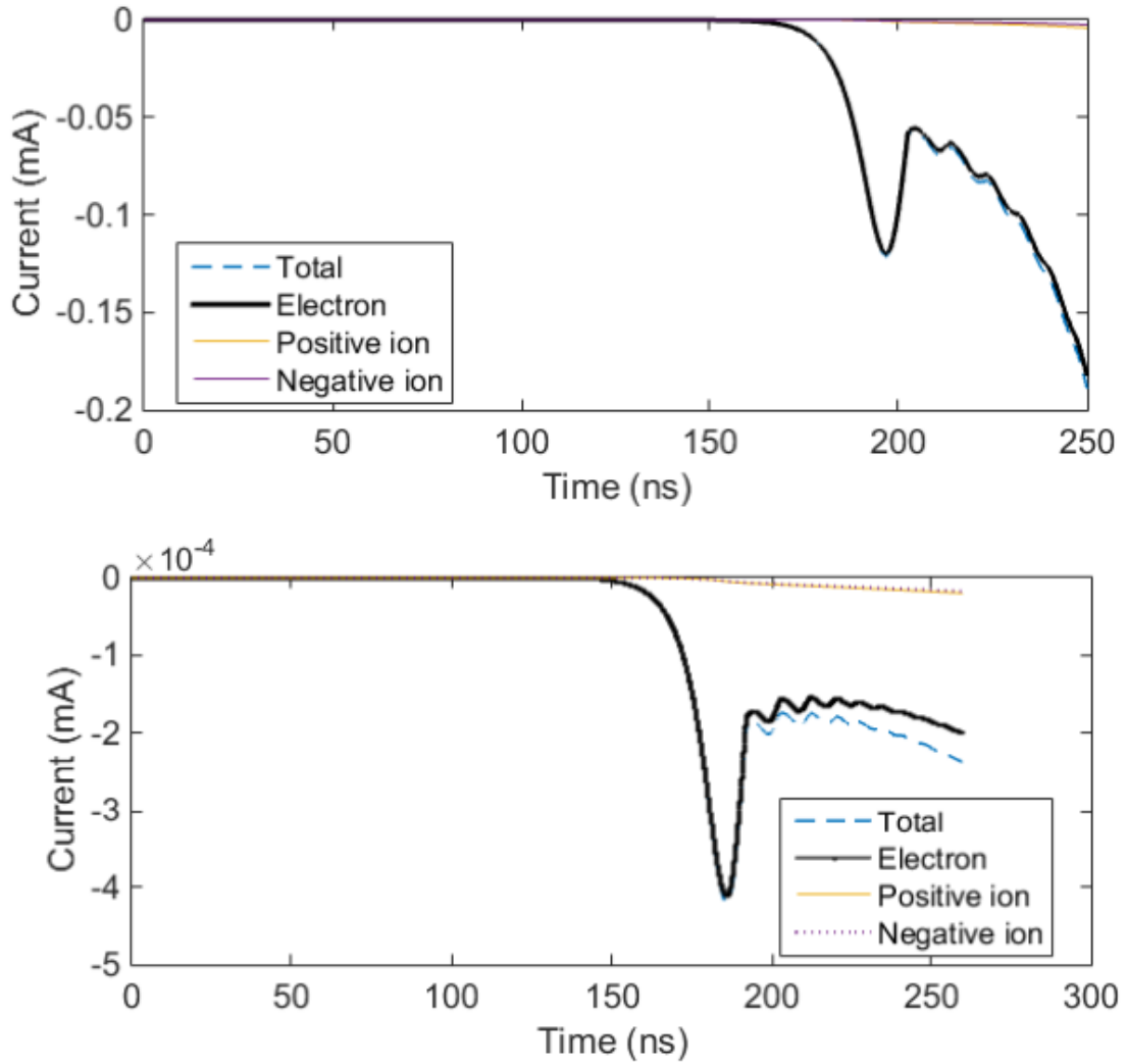
FIGURE 5.12: Current pulse in air (top) and in flue (bottom) for a 3 cm gap size (the cross over).
