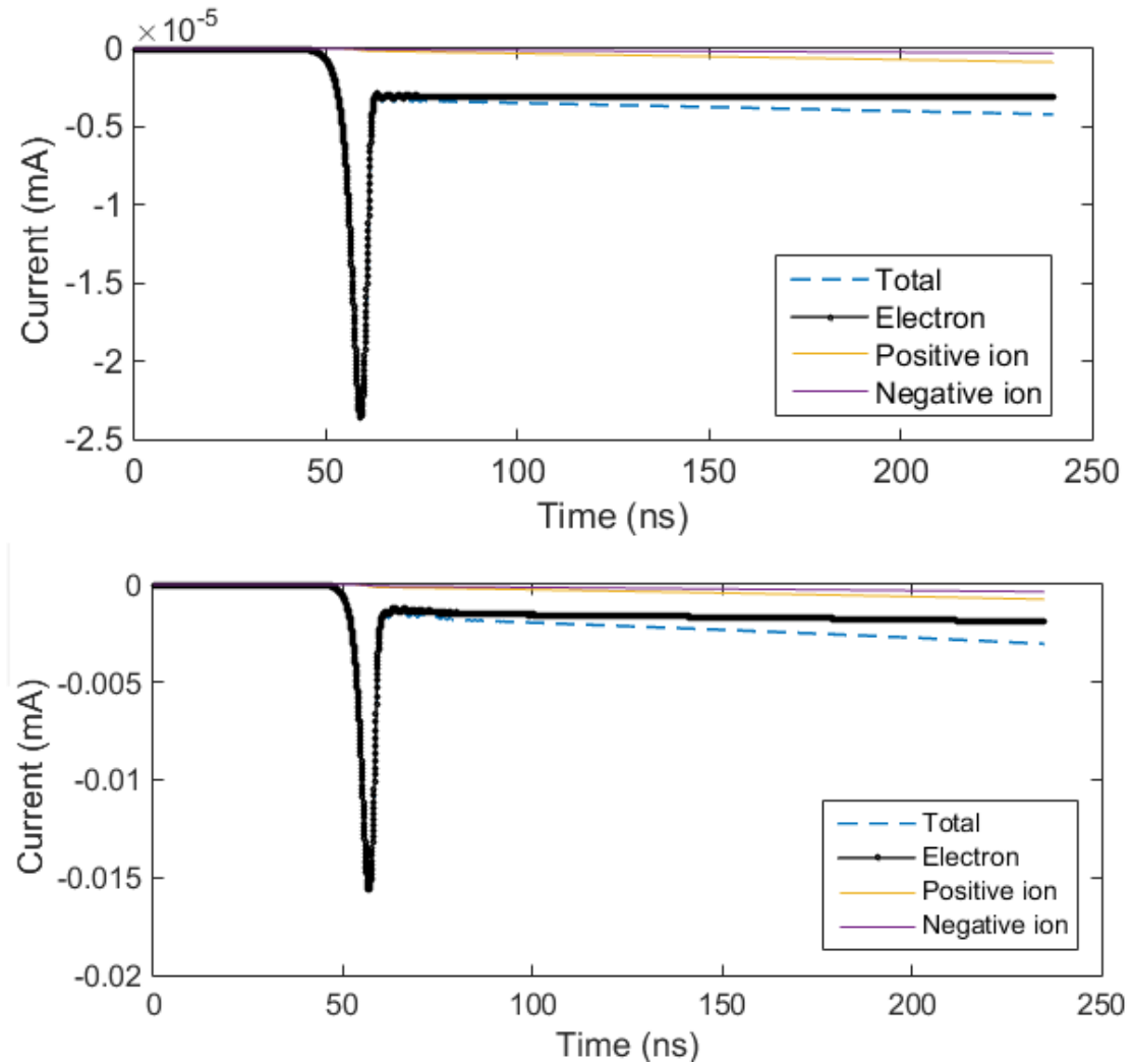
FIGURE 5.9: Current pulse in air (top) and in flue (bottom) for a 1 cm gap size.
