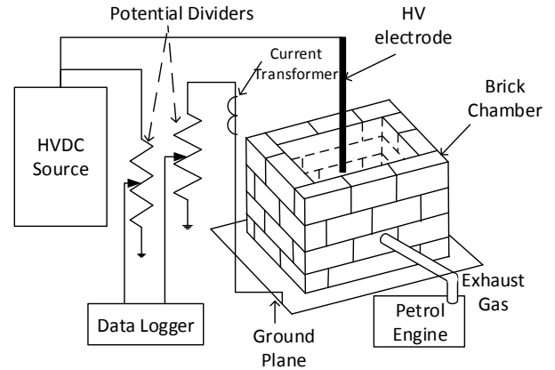
Figure 2: Experimental setup: testing breakdown of engine flue inside a brick chamber.
