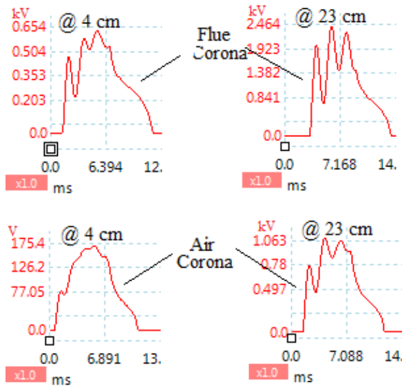
Figure 5: Comparison of corona pulsation and magnitude from small gap spacing to large gap spacing for flue and air.
