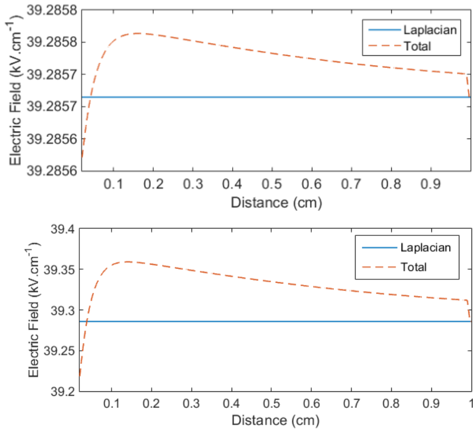
FIGURE 5.11: Electric field in air (top) and in flue (bottom) for a 1 cm gap size.
