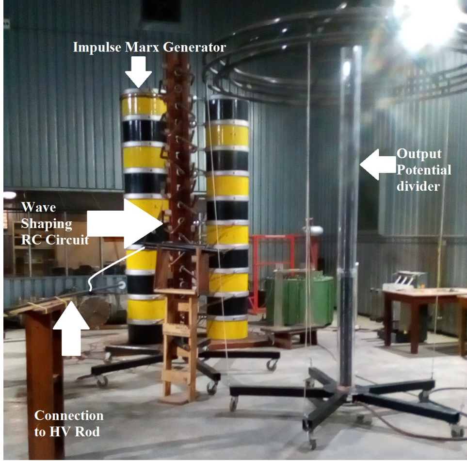
FIGURE 4.19: Image of the laboratory experiment setup for impulse tests
