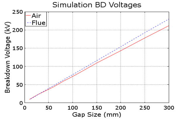
Figure 8: Simulation results: Breakdown characteristics of air and flue under standard conditions.
