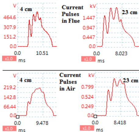
Figure 5: Comparison of pre-breakdown leakage current (represented as voltage output of the HFCT) showing discharge activity in air and flue at 4 cm and at 23 cm.
