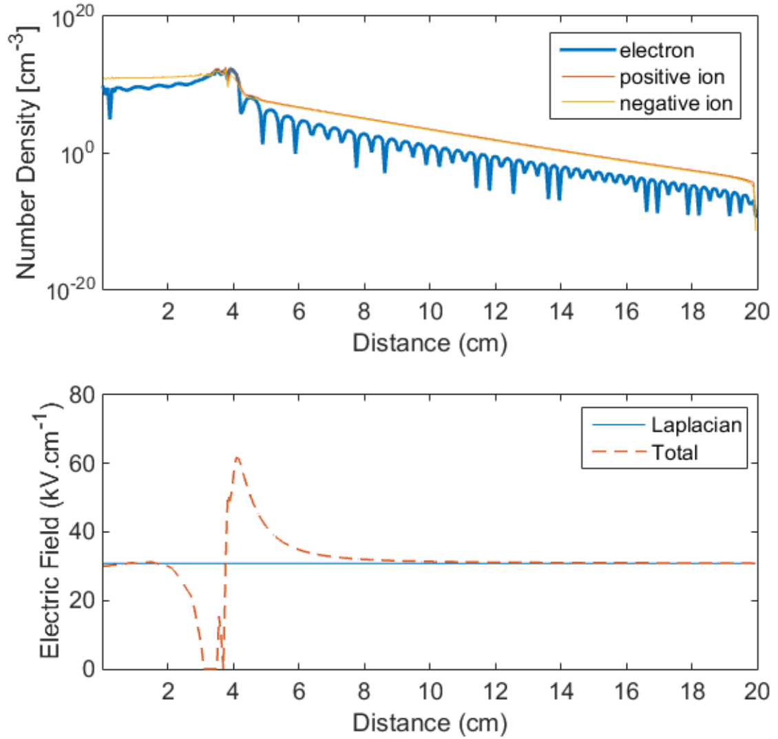
FIGURE 5.16: Space charge (top) and electric field (bottom) profile during breakdown of a 20 cm gap in air
