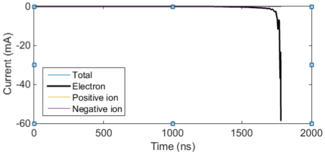
FIGURE 5.15: Current profile during breakdown of a 200 mm gap in air
