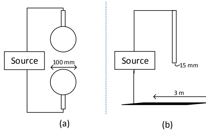
FIGURE 4.6: Test gap geometries, (a) Sphere-Sphere and (b) Rod-Plane
