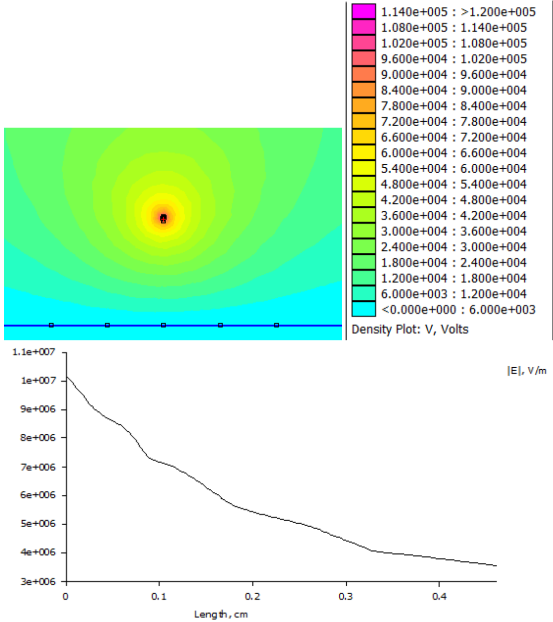
FIGURE 4.2: FEM simulation of a point-plane geometry and its decaying field distribution within 0.4 cm of the gap from the HV electrode.
