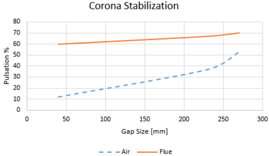
FIGURE 4.17: Corona stabilization with increasing gap size.
