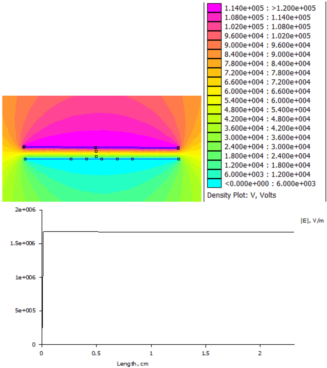
FIGURE 4.1: FEM simulation of a wire-plane geometry and its field distribution within 2 cm of the gap from HV wire to plane.
