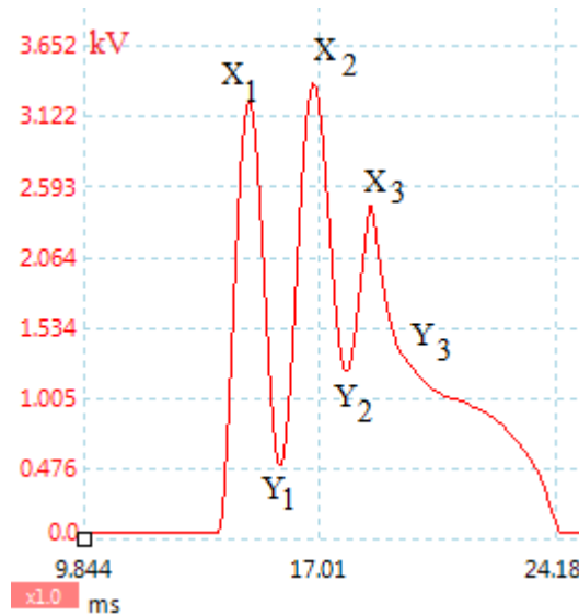
FIGURE 4.16: Illustration of points used to compute pulsation %
