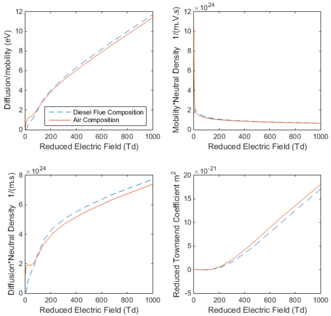
FIGURE 5.6: A comparison of transport parameters and townsend's coefficients for air and diesel flue gas compositions.
