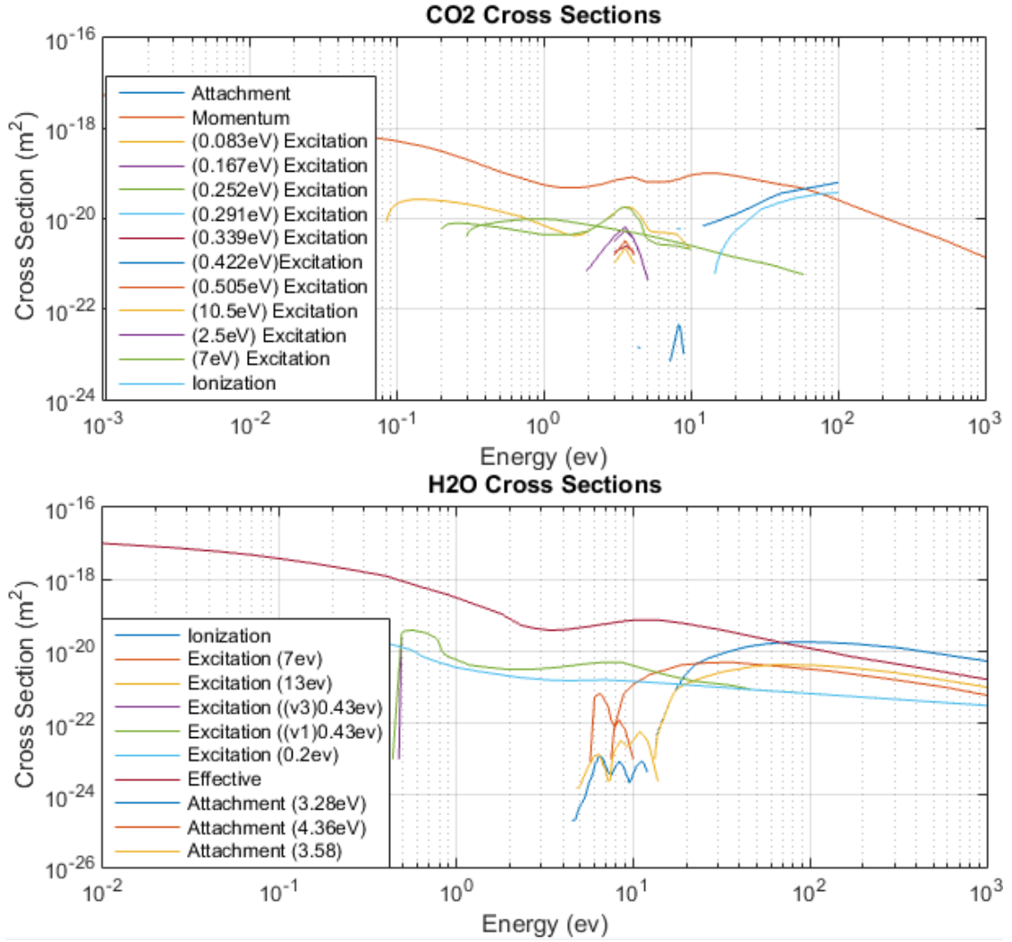
FIGURE 5.5: CO_2 and H_2O Collisional Cross Sections for the various possible reactions depending on the energy of the electrons colliding with the molecules.
