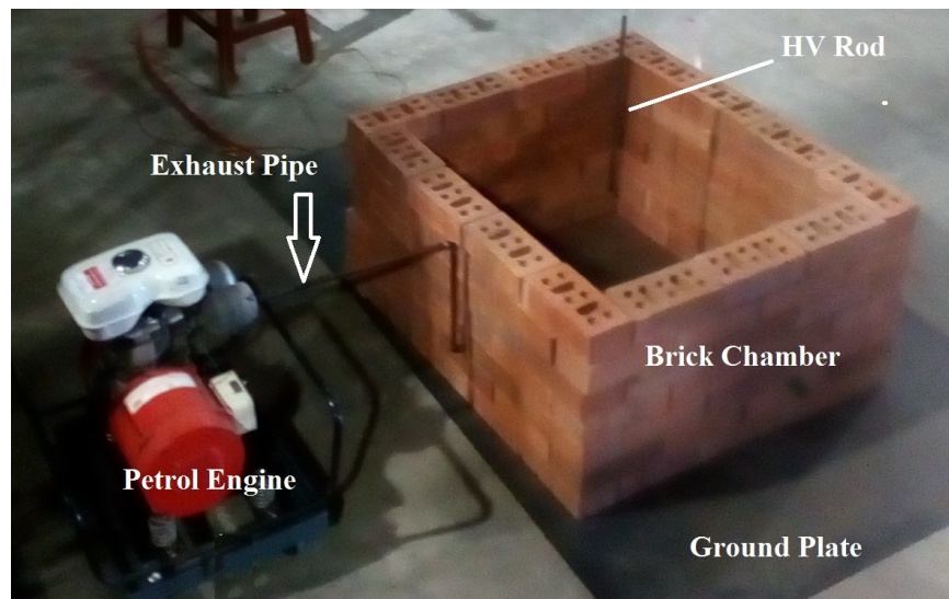
FIGURE 4.7: Image of the laboratory experiment setup with the petrol engine source.
