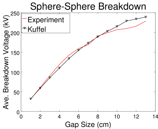
Figure 3: Breakdown characteristic for sphere-sphere electrode setup in air.
