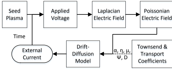
Figure 7: Flux Corrected Algorithm flow chart [24]
