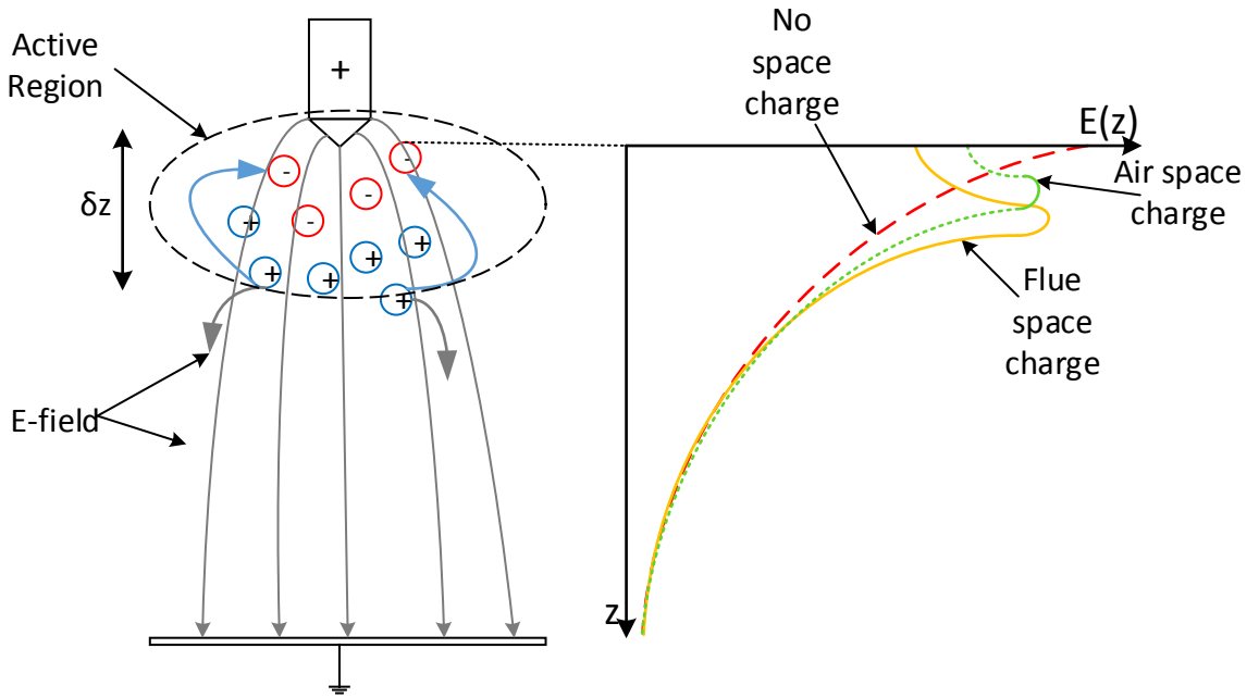
FIGURE 4.15: Illustration of electric field collapse due to corona space charge.
