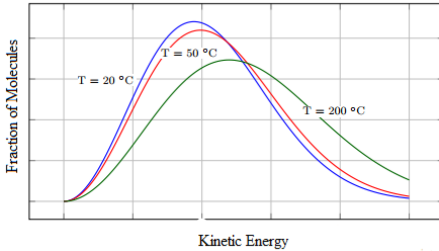
FIGURE 5.2: Maxwell-Boltzmann's distribution for number of particles with enough energy to react at temperature T. adapted from [18]
