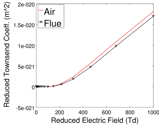
Figure 1: A comparison of Townsend's coefficients for air and engine exhaust flue gas compositions.
