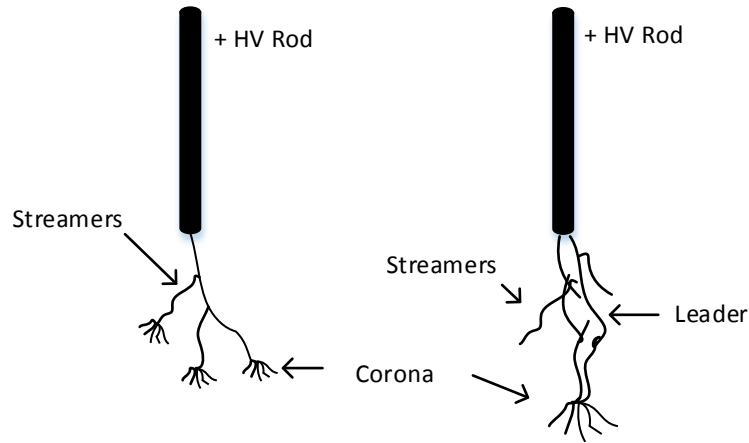
FIGURE 3.2: Schematic of streamer channel and corona at the head, developing into a leader.
