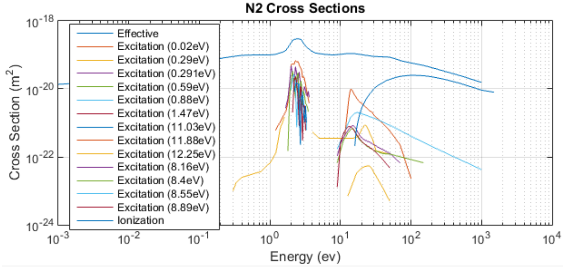
FIGURE 5.4: N_2 Collisional Cross Sections for the various possible reactions depending on the energy of the electrons colliding with the molecule.
