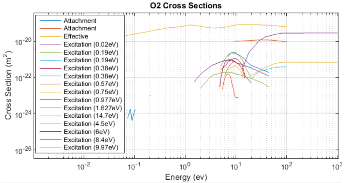
FIGURE 5.3: O_2 Collisional Cross Sections for the various possible reactions depending on the energy of the electrons colliding with the molecule.
