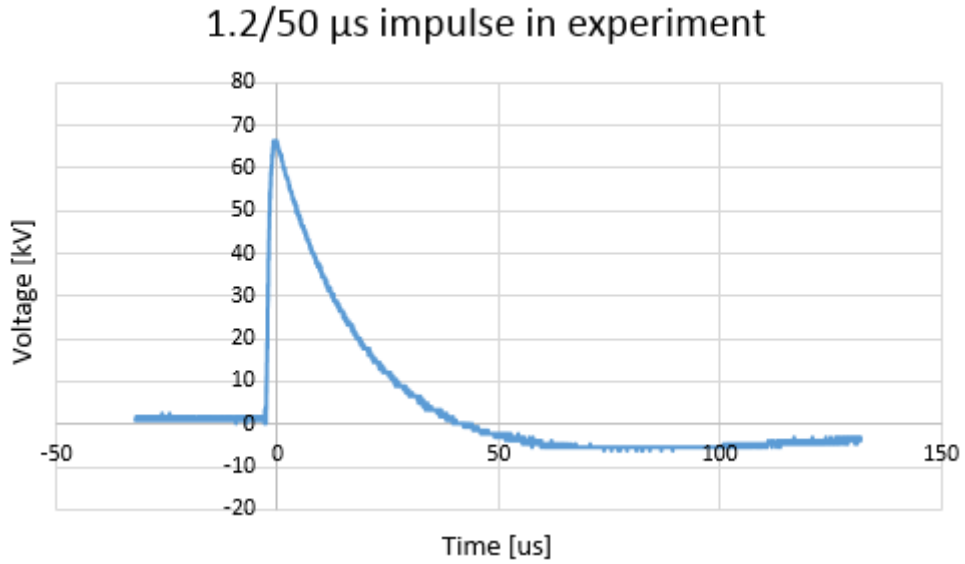
FIGURE 4.20: Laboratory generated standard 1.2/50 \mu s lightning impulse waveform
