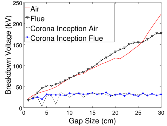
Figure 4: Breakdown and corona inception voltage comparison for air and flue.
