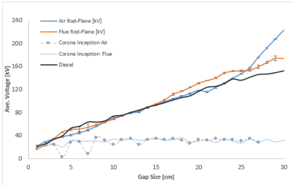
FIGURE 4.11: Breakdown voltage curves for the rod-plane tests in air, petrol and diesel flue.
