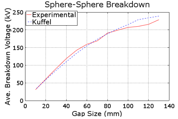
Figure 3: Sphere-Sphere average DC breakdown calibration results compared to published data in Kuffel [2].
