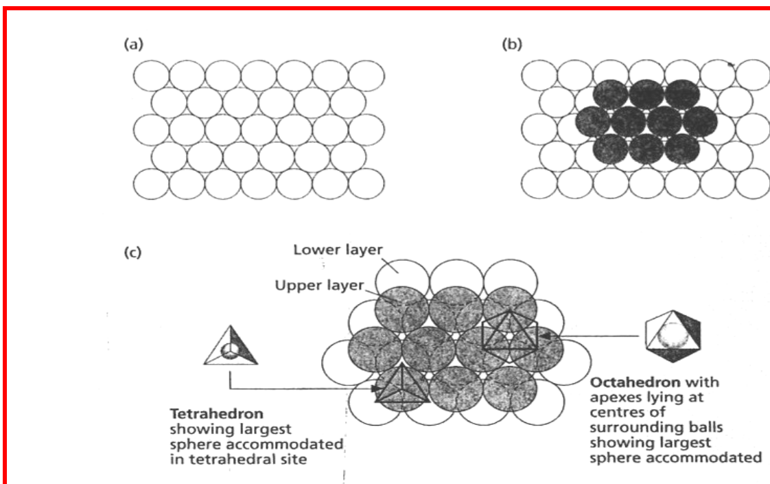
Figure 2.1 (a) Spheres in planar layers showing hexagonal symmetry. (b) An upper layer of spheres (shaded) is stacked on the layer in (a), such that each upper sphere fits into the depression between three spheres in the lower layer. (c) enlargement of (b), where heavy lines show coordination polyhedral, joining the centres of adjacent spheres, delineating two geometries, tetrahedral and octahedral.
