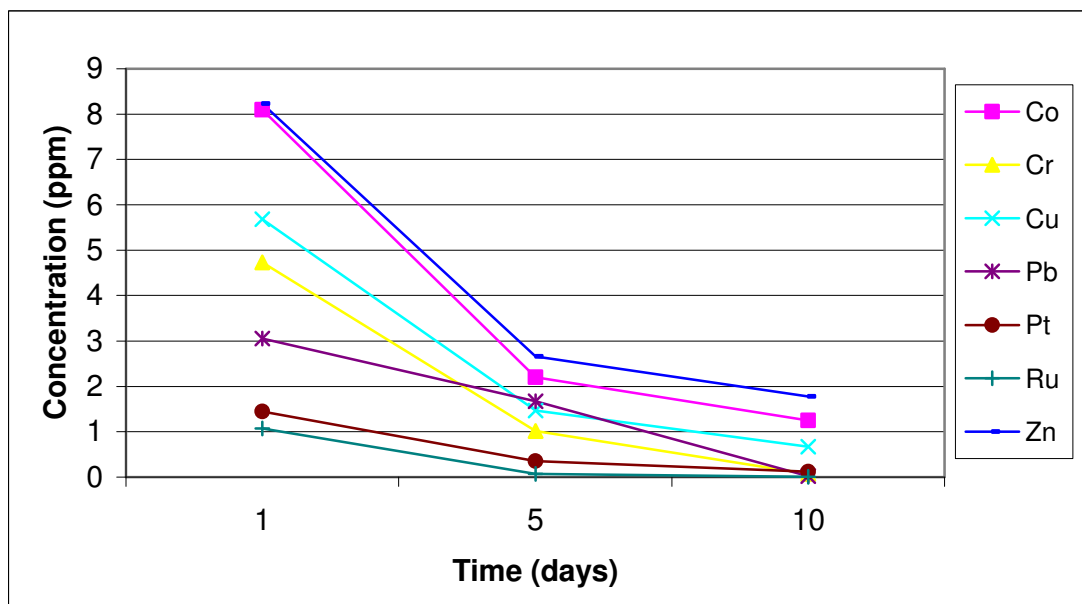
Figure 5.12 Effect of time on leachable concentration of PGMs and transition metals in sandy soil treated with (a) Chemcap TM (b) sodium silicate (pH = 2)
