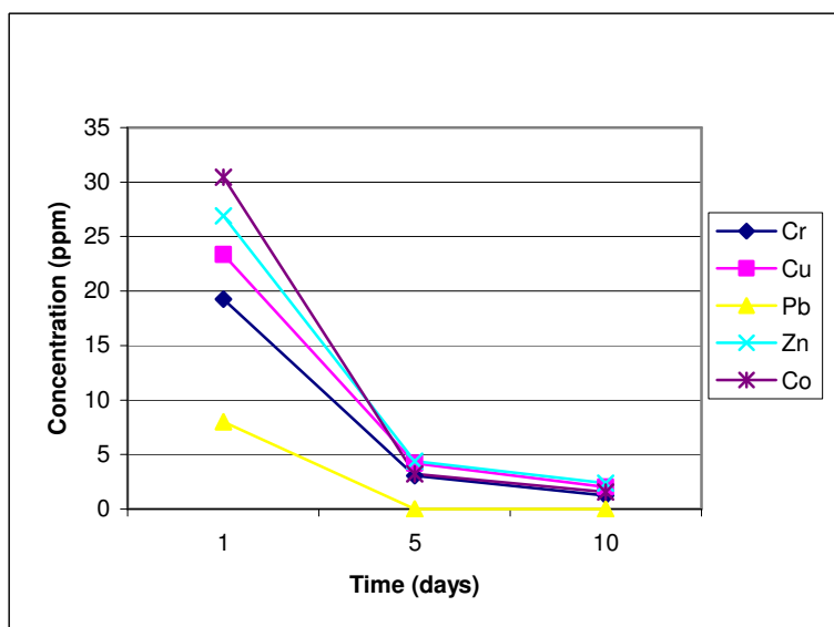
Figure 5.16 Effect of time on concentration of transition metals in water treated with (a) Chemcap TM (b) sodium silicate (pH = 2)
