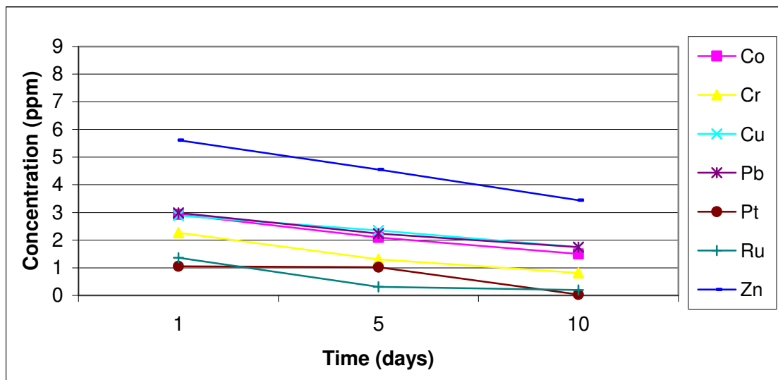
Figure 5.13 Effect of time on leachable concentration of PGMs and transition metals in clay soil treated with (a) Chemcap TM (b) sodium silicate (pH = 2)
