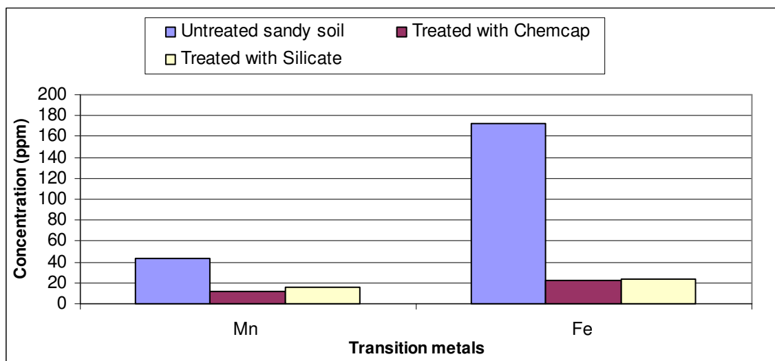
Figure 5.2 Leachable concentration of transition metals in sandy soil at (a) pH=9.3 (b) pH= 2
