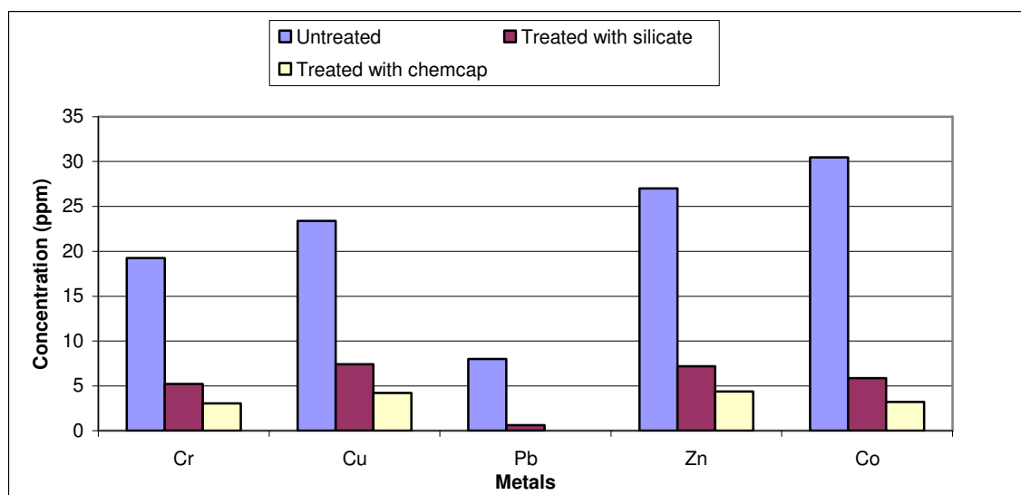
Figure 5.9 Concentration of transition metals in water at (a) pH= 9.2 (b) pH=2
