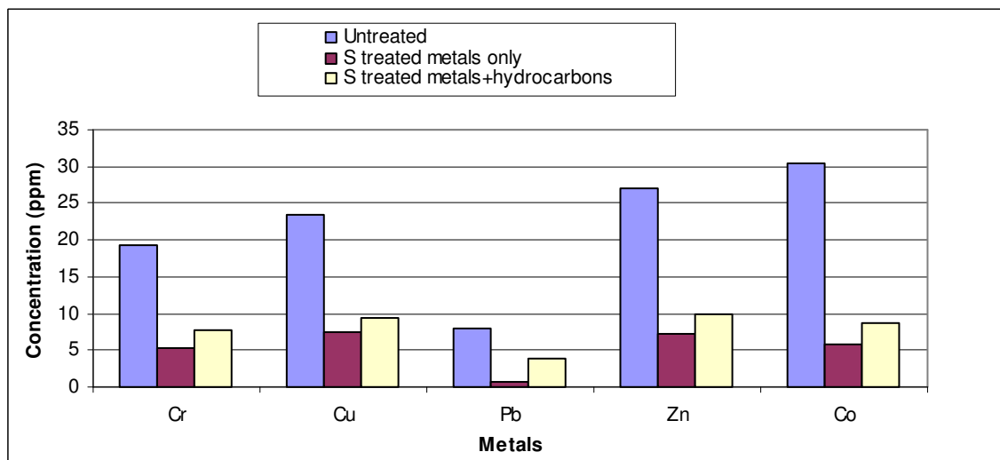
Figure 5.25 Effect of hydrocarbons on concentration of transition metals in water treated with (a) Chemcap TM (b) sodium silicate (pH = 2)
