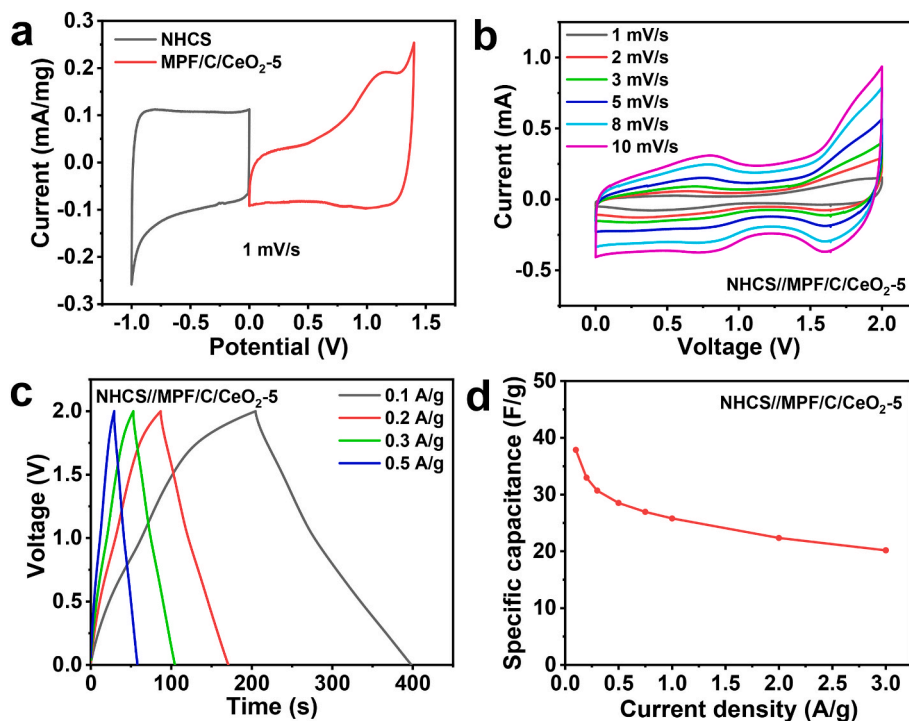
Fig. 4. a) CV curves of NHCS and MPF/C/CeO 2 -5 at 1 mV/s, b) CV curves of the NHCS//MPF/C/CeO 2 -5 device at scan rates between 1 and 10 mV/s, c) GCD curves of the NHCS//MPF/C/CeO 2 -5 device at current densities between 0.1 and 0.5 A/g, d) Specific capacitance versus current density for the NHCS//MPF/C/CeO 2 -5 devices.
