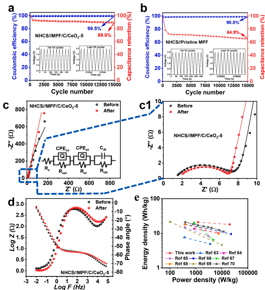
Fig. 5. a) Cycling performance of the NHCS//MPF/C/CeO 2 -5 ACS device at 1 A/g current density b) Cycling performance of the NHCS//pristine MPF ACS device at 1 A/g current density, c) Nyquist plots of the NHCS//MPF/C/CeO 2 -5 ACS device before and after 15000 cycles, c1) inset showing magnified region of the Nyquist plots for the NHCS//MPF/C/CeO 2 -5 ACS device, d) Bode plots of the NHCS//MPF/C/CeO 2 -5 ACS device before and after 15000 cycles, and e) Comparative Ragone plot illustrating the performance of the NHCS//MPF/C/CeO 2 -5 compared to other Mn-based asymmetric supercapacitors reported in recent literature.
