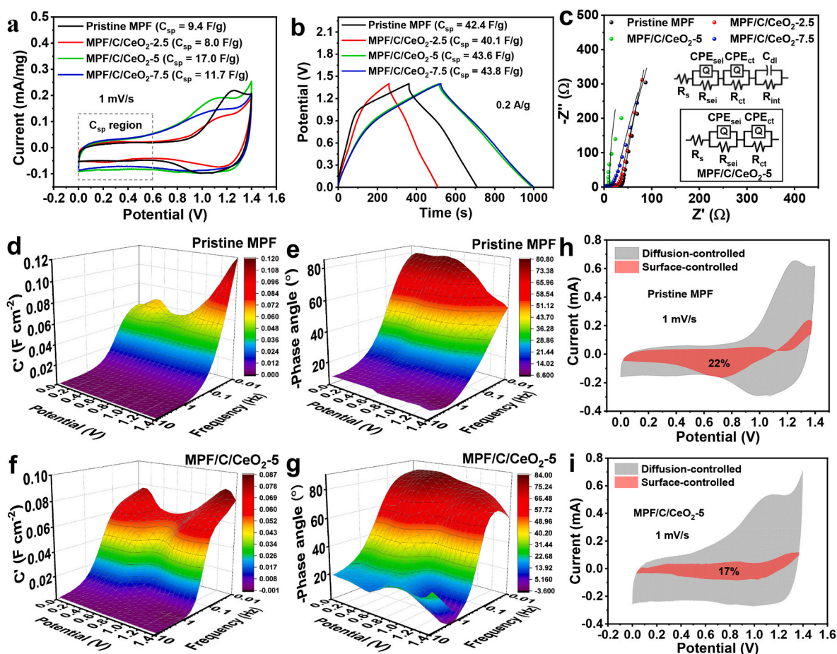
Fig. 3. a) CV curves of pristine MPF and the MPF/C/CeO 2 composites at 1 mV/s scan rates (with specific capacitance contribution in the inset region), b) GCD curves of pristine MPF and the MPF/C/CeO 2 composites at 0.2 A/g current density with calculated specific capacitances, c) Nyquist plots of pristine MPF and the MPF/C/CeO 2 composites (with insets showing the equivalent circuits for MPF/C/CeO 2 -5 and the other samples). 3D node plot representations of d) the real area-normalised capacitance ( C' ) vs frequency vs voltage and e) phase angle ( ^\circ ) vs frequency vs voltage for Pristine MPF; and c) the real area-normalised capacitance ( C' ) vs frequency vs voltage and d) phase angle ( ^\circ ) vs frequency vs voltage for MPF/C/CeO 2 -5 composite. Coloured bars correspond to the magnitude of C' and the phase angle ( ^\circ ). Comparison of the capacitive and diffusion-controlled contributions at 1 mV/s in h) pristine MPF and i) MPF/C/CeO 2 -5.
