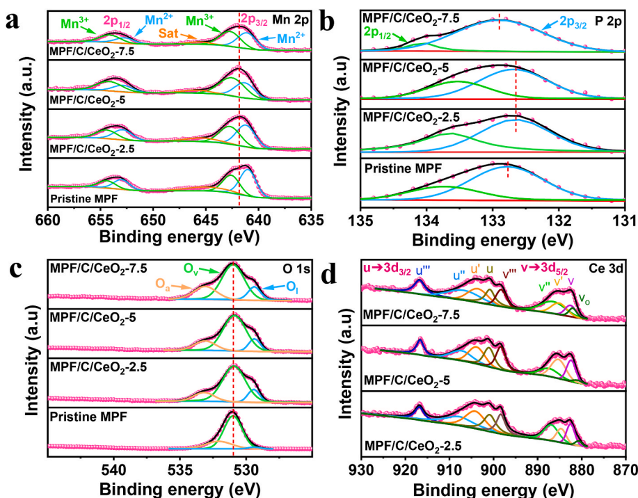
Fig. 2. XPS spectra illustrating deconvoluted a) Mn 2p, b) P 2p, and c) O 1s peaks for the pristine MPF and MPF/C/CeO 2 composites; and deconvoluted d) Ce 3d peaks for the MPF/C/CeO 2 composites.
