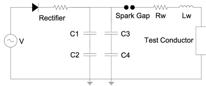
Fig. 1. Schematic of an 8/20 \mu s impulse generator utilized to simulate lightning currents. The capacitor bank (C1, C2, C3, C4) are charged, when the spark gap fires, the charge then flows through R_w and L_w which shape the rise and fall-time. This high-current impulse is then delivered to the Test Conductor or Object as if it were ‘struck by lightning’.
