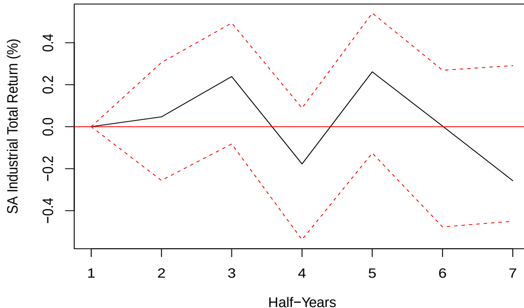
Figure 22: Orthogonal impulse response of the industrial property sector total return from a shock to stock market returns
