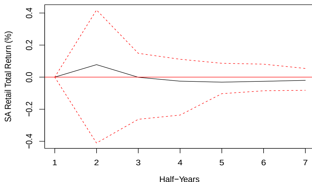
Figure 12: Orthogonal impulse response of the retail property sector total return from a shock to stock market returns
