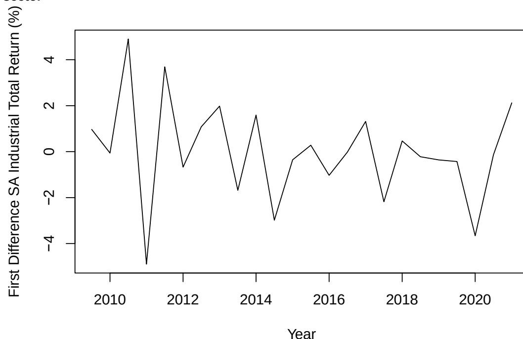
Figure 36: First difference of the semi-annual total return of the South African industrial property sector
