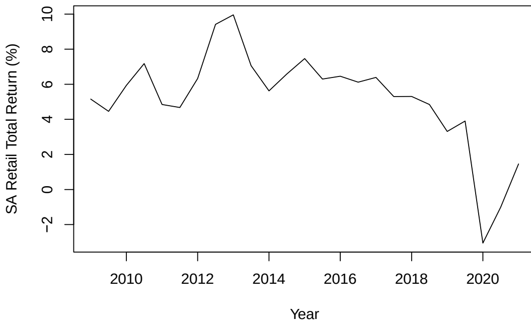
Figure 31: Semi-annual total return of the South African retail property sector
