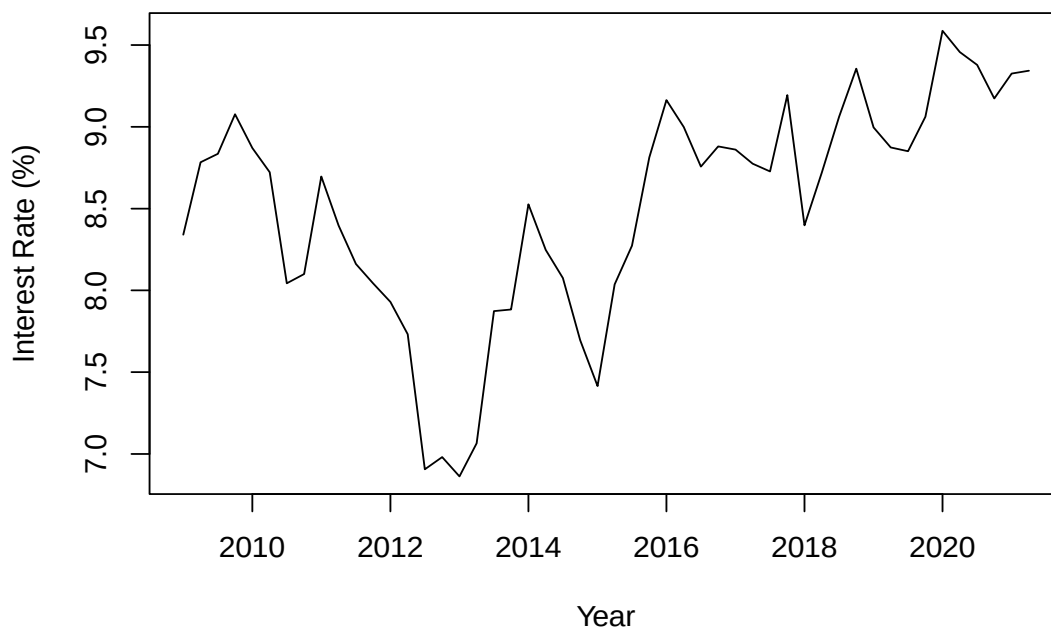
Figure 27: Quarterly South African interest rate
