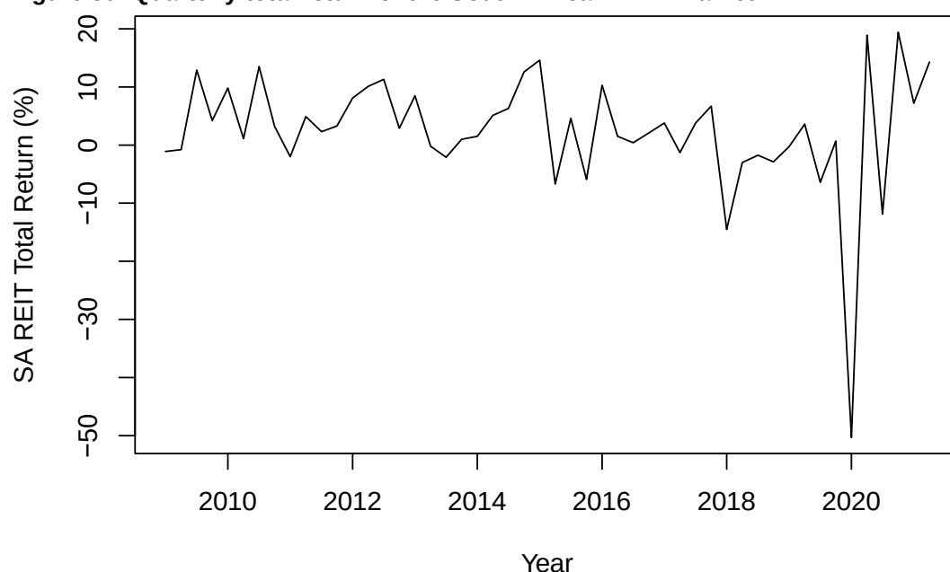
Figure 30: Quarterly total return of the South African REIT market
