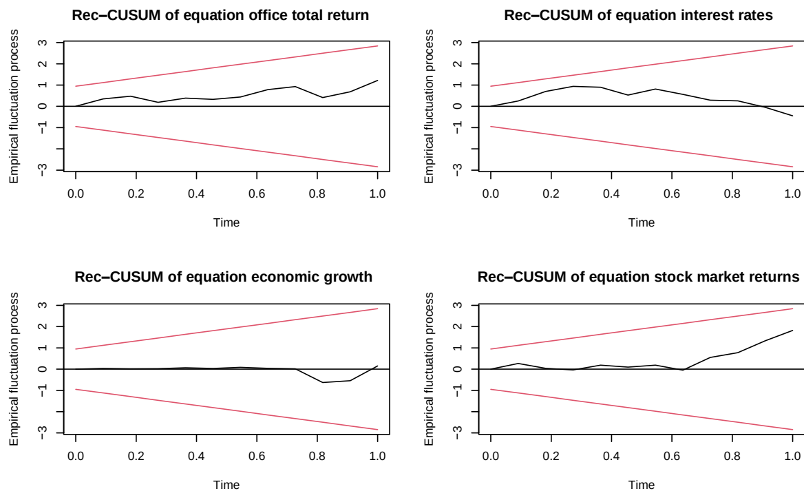
Figure 13: CUSUM tests of the individual equations of the VAR(2) model for the office property sector
