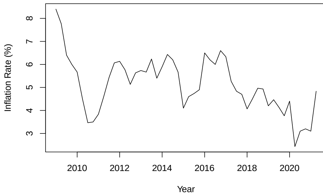
Figure 25: Quarterly South African inflation rate
