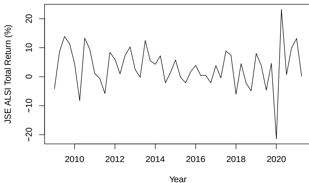
Figure 29: Quarterly total return of the South African stock market
