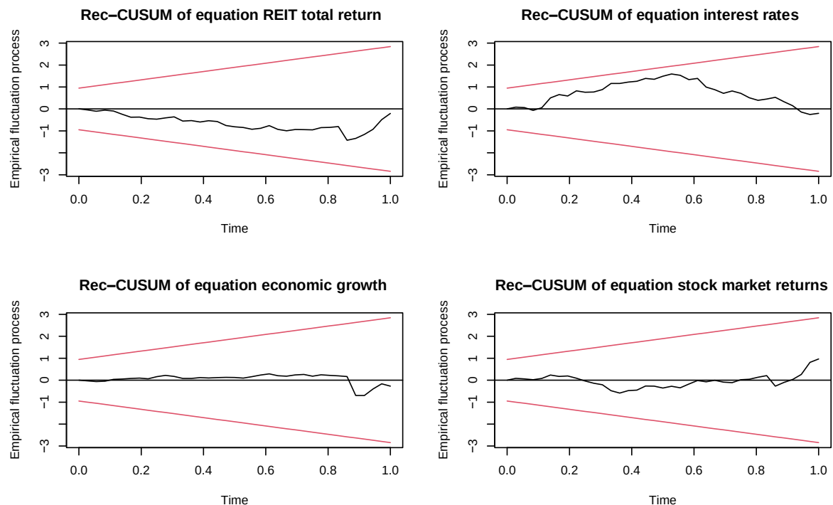
Figure 3: CUSUM tests of the individual equations of the VAR(2) model for the REIT market
