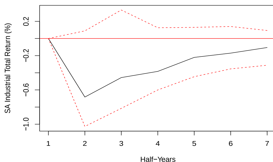
Figure 21: Orthogonal impulse response of the industrial property sector total return from a shock to interest rates
