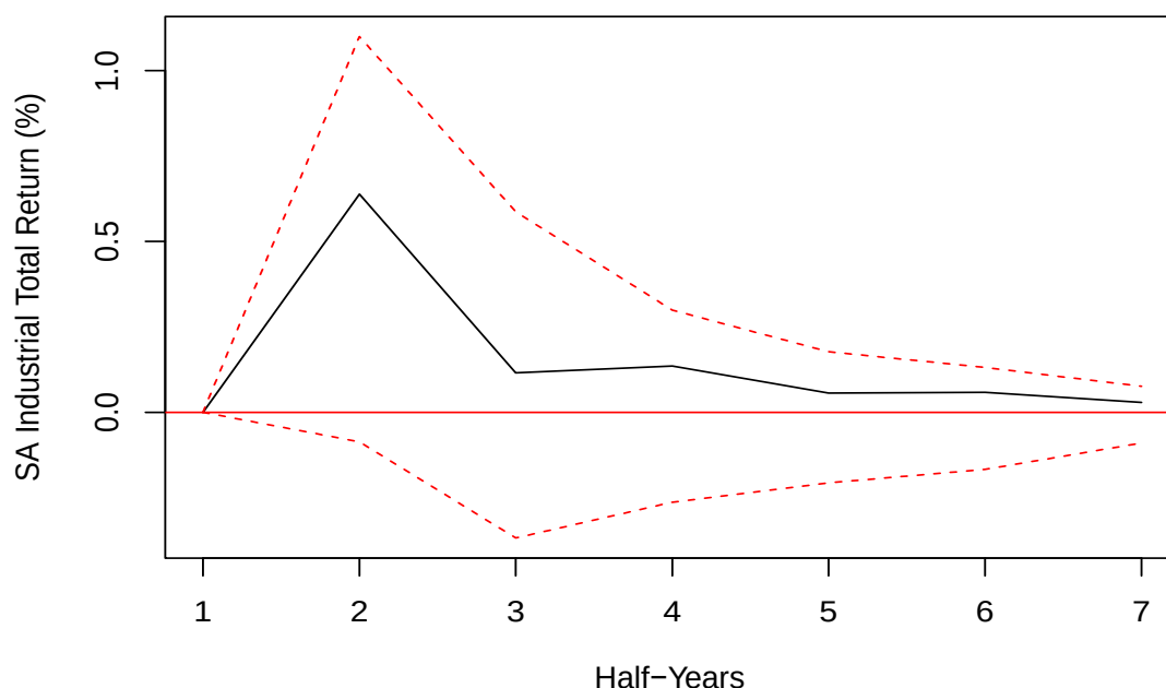
Figure 19: Orthogonal impulse response of the industrial property sector total return from a shock to economic growth
