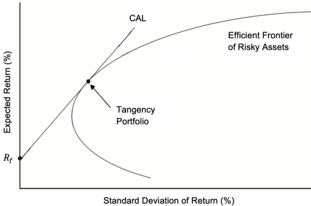
Figure 2: The tangency portfolio
