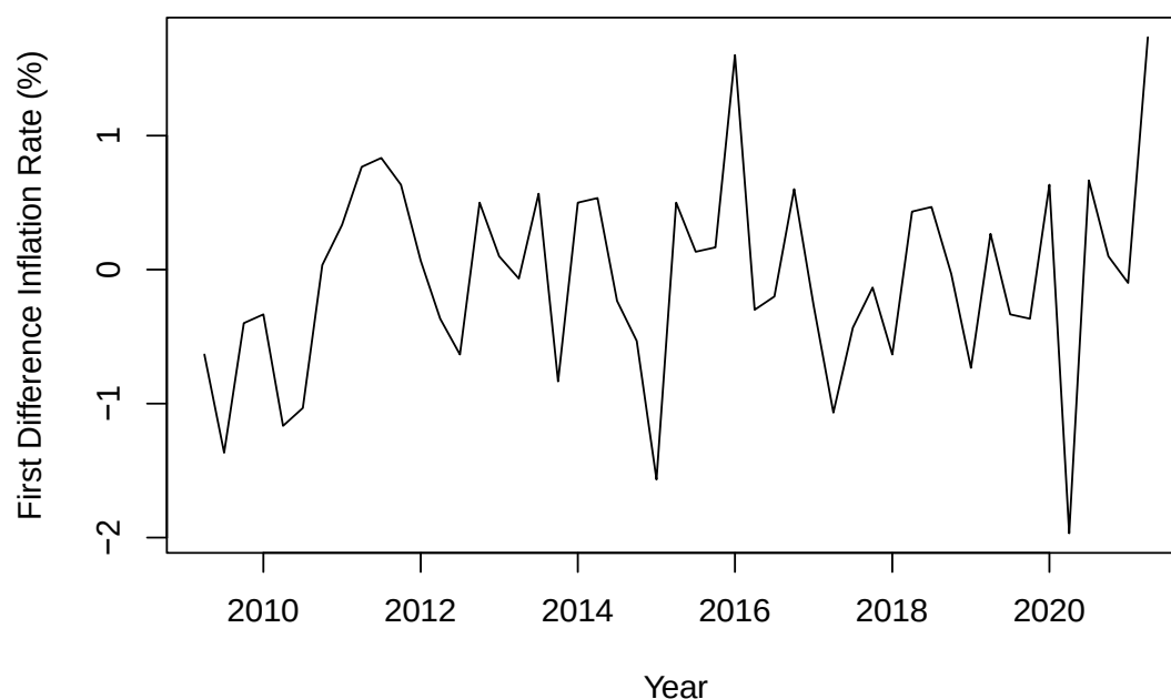
Figure 26: First difference of the quarterly South African inflation rate
