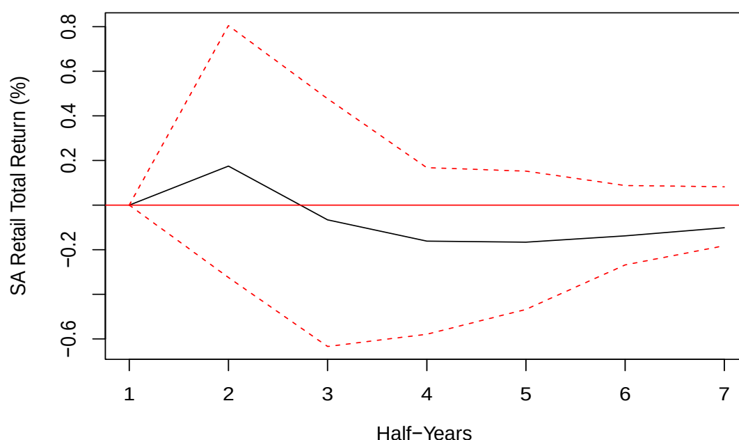
Figure 9: Orthogonal impulse response of the retail property sector total return from a shock to economic growth
