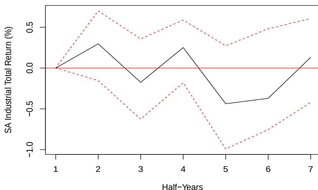
Figure 20: Orthogonal impulse response of the industrial property sector total return from a shock to inflation
