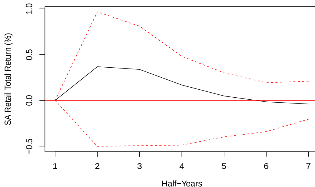
Figure 10: Orthogonal impulse response of the retail property sector total return from a shock to inflation
