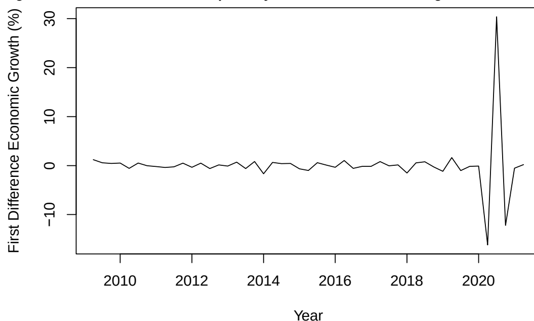
Figure 24: First difference of the quarterly South African economic growth rate
