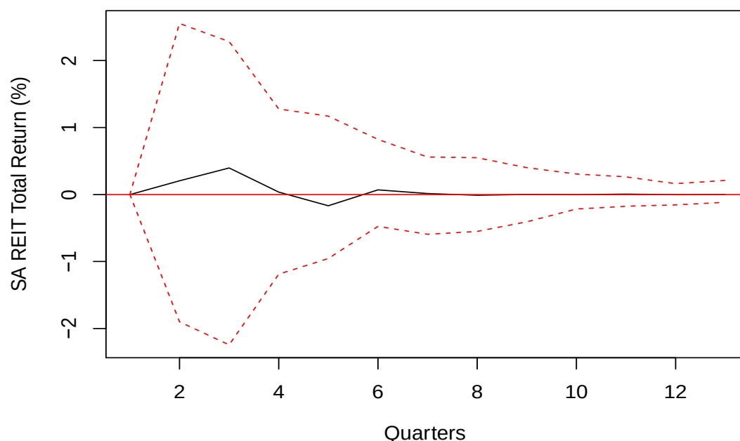
Figure 7: Orthogonal impulse response of the REIT market total return from a shock to stock market returns
