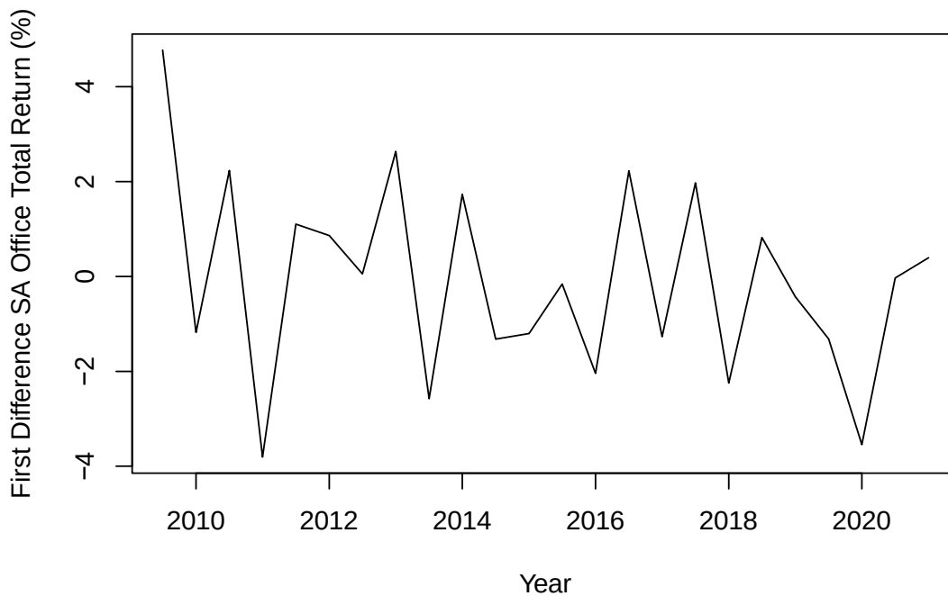
Figure 34: First difference of the semi-annual total return of the South African office property sector
