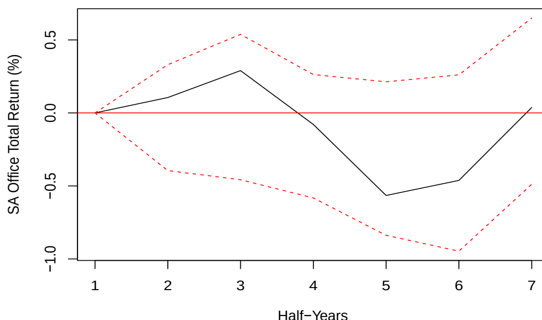
Figure 15: Orthogonal impulse response of the office property sector total return from a shock to inflation
