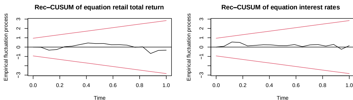
Figure 8: CUSUM tests of the individual equations of the VAR(1) model for the retail property sector
