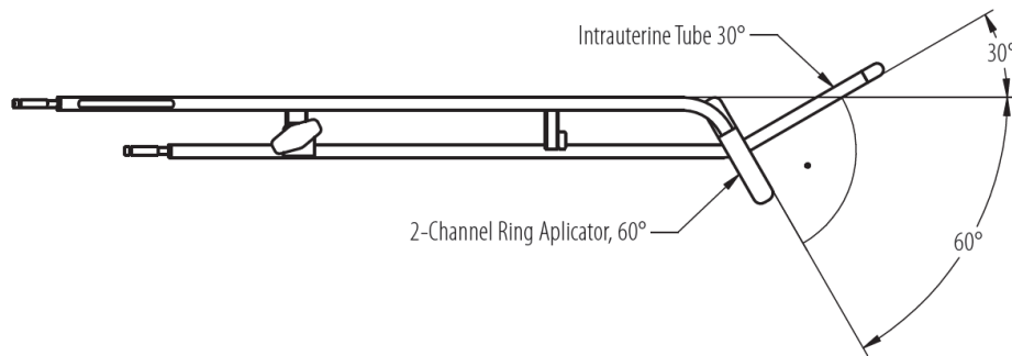
FIGURE 6.1: Diagram of a tandem and ring applicator as simulated in this report [20].
