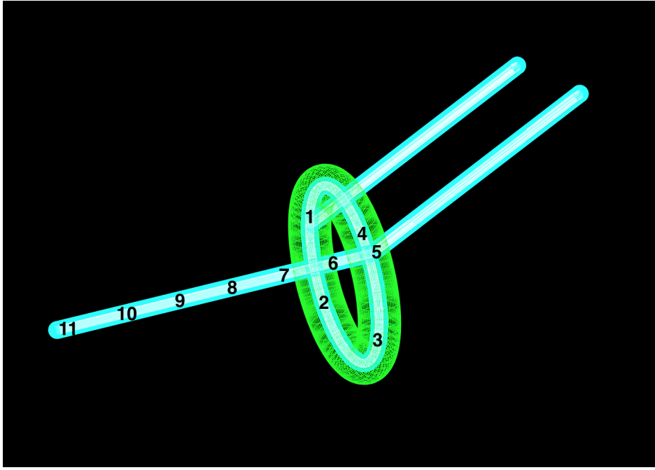
FIGURE 6.2: Tandem and ring applicator as simulated using Geant4. The dwell points for the optimisation are numbered 1-11.
