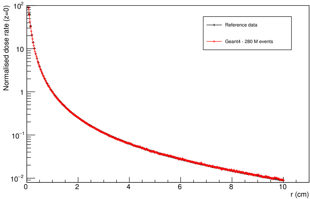
FIGURE 5.5: Normalised radial dose comparison between simulation using Geant4 and published reference data.
