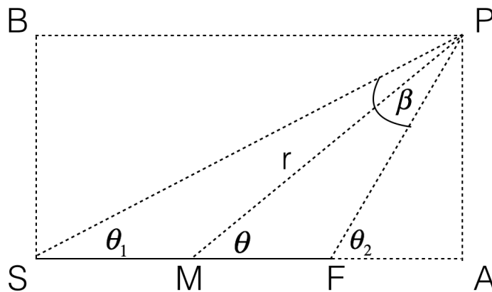
FIGURE 5.8: The geometry relevant to the determination of \beta , where the source length is |SF| , the measurement point is P , and the line |MP| joining the source centre to the measurement point has length r .
