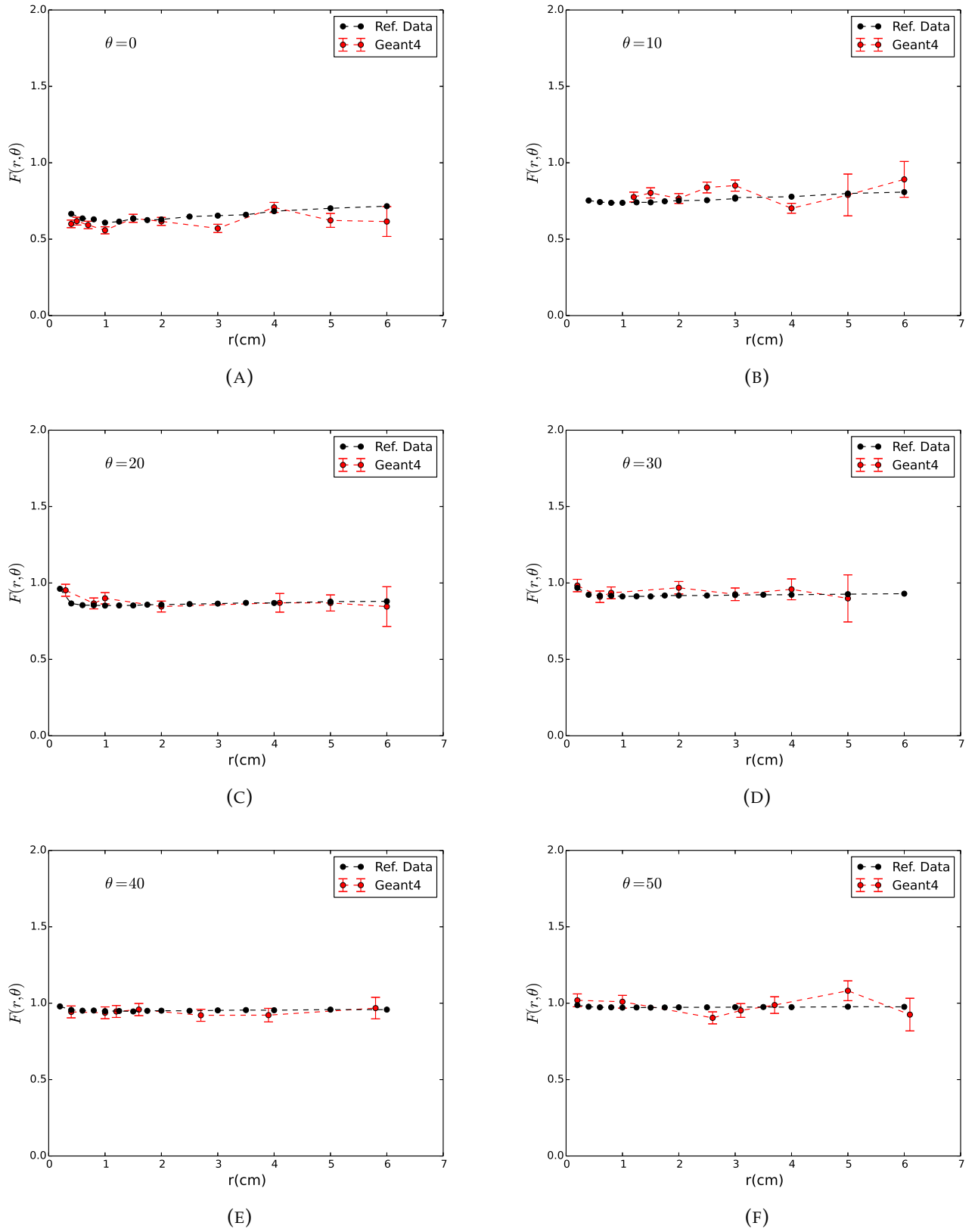
FIGURE 5.11: Values of F_L(r, \theta) for \theta = 0^\circ, 10^\circ, 20^\circ, 30^\circ, 40^\circ , and 50^\circ .
