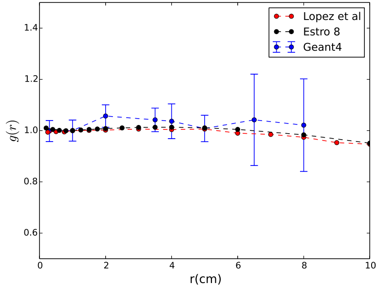
FIGURE 5.13: The radial dose function g_L(r) plotted against reference data.
