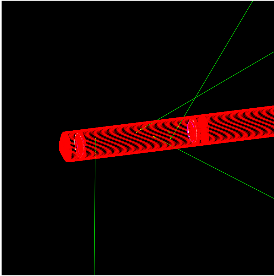
FIGURE 5.2: Simulation of the GammaMed ^{192}\text{Ir} source in air where the iridium core and capsule details are visible.
