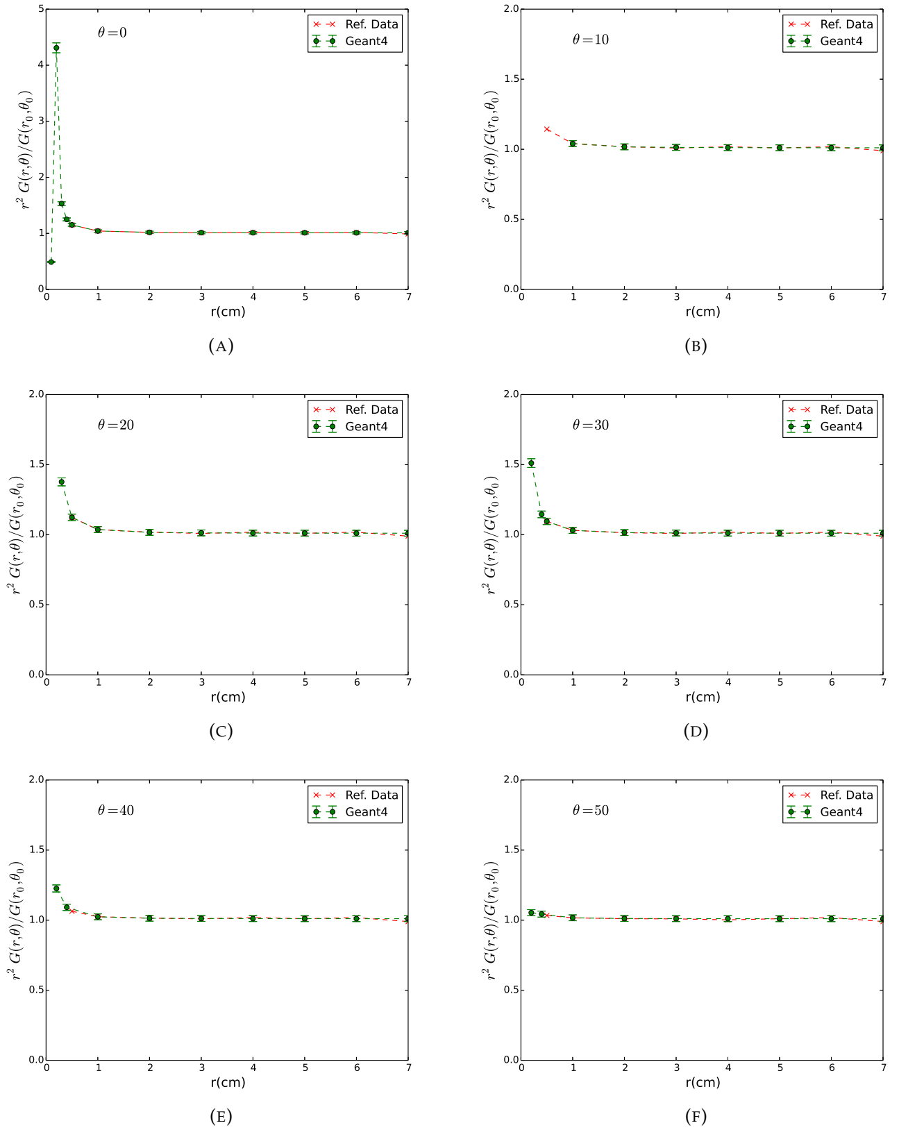
FIGURE 5.9: Values of r^2 G_L(r, \theta) / G_L(r_0, \theta_0) for \theta = 0^\circ, 10^\circ, 20^\circ, 30^\circ, 40^\circ , and 50^\circ .
