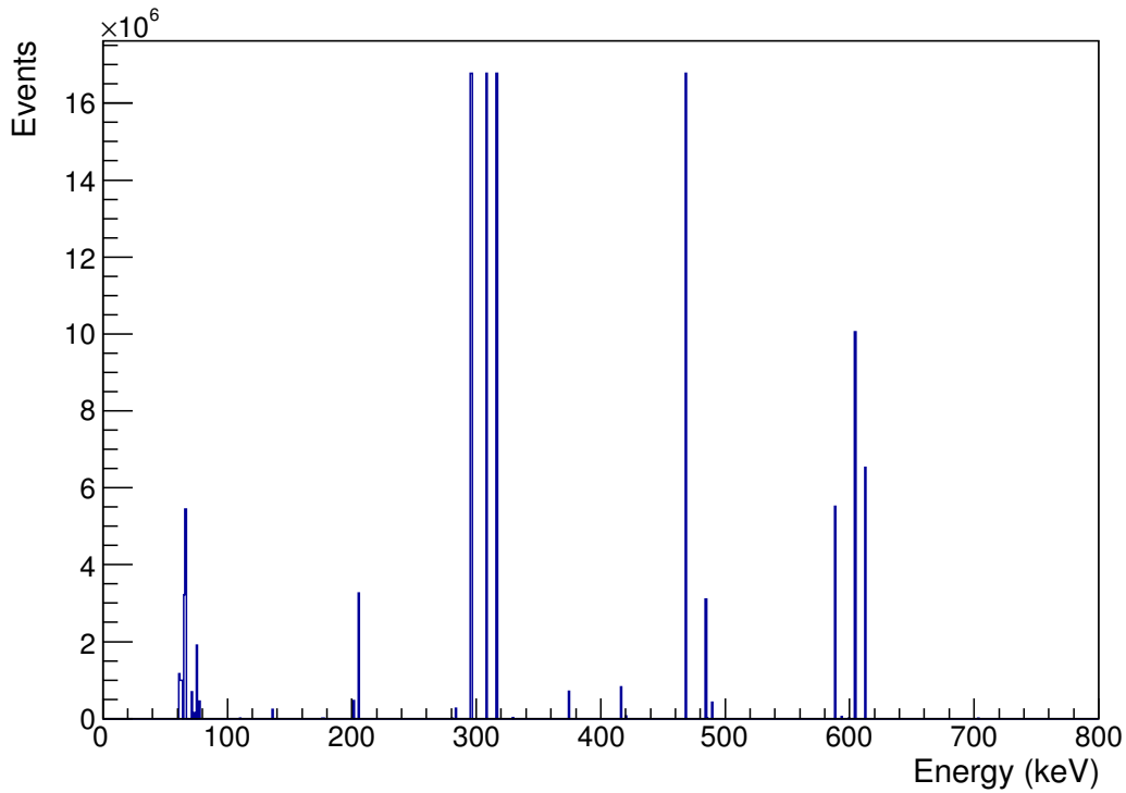
FIGURE 5.3: Energy spectrum of primary particles from the GammaMed source simulated in this report.
