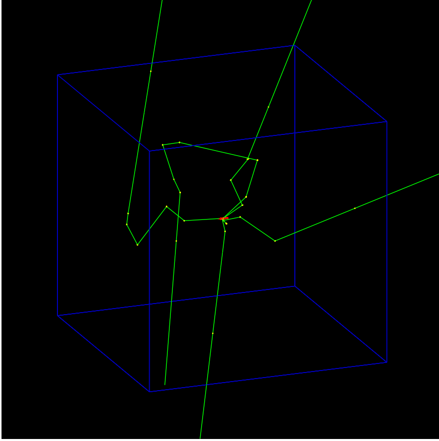
FIGURE 5.4: A depiction of the source undergoing decay events within the water phantom, denoted as a blue cube, used for the dose rate comparison to reference data.
