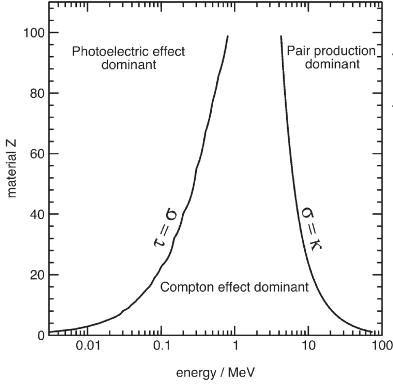
FIGURE 2.2: The dependence of the dominant photon interaction mechanisms on energy, E and atomic number, Z [9].
