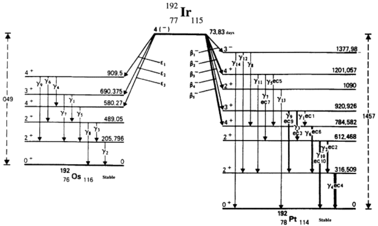
FIGURE 2.1: The decay scheme of ^{192}\text{Ir} , showing both electron capture and \beta decay modes [13].
