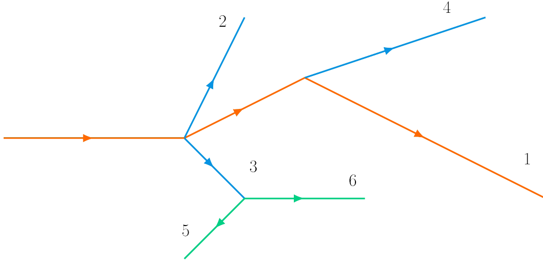
FIGURE 5.7: An example of the assignment of tracks moving through a volume.
