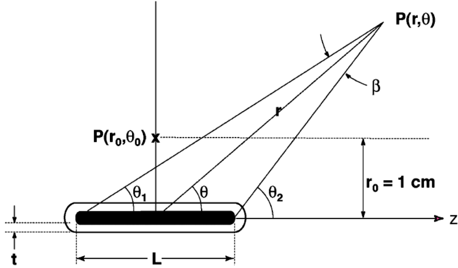
FIGURE 4.1: The two-dimensional coordinate system used by AAPM TG-43 in order to calculate the dose at point P(r, \theta) [4].
