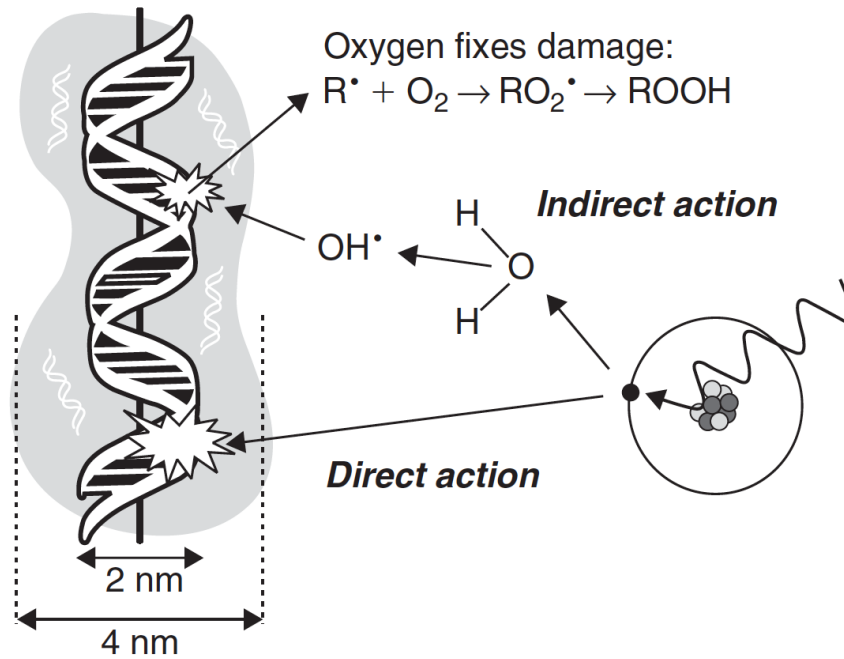
FIGURE 3.2: Creation of free radicals, R^{\bullet} , in nearby water molecules, termed indirect action, or within the DNA molecule, termed direct action [14].
