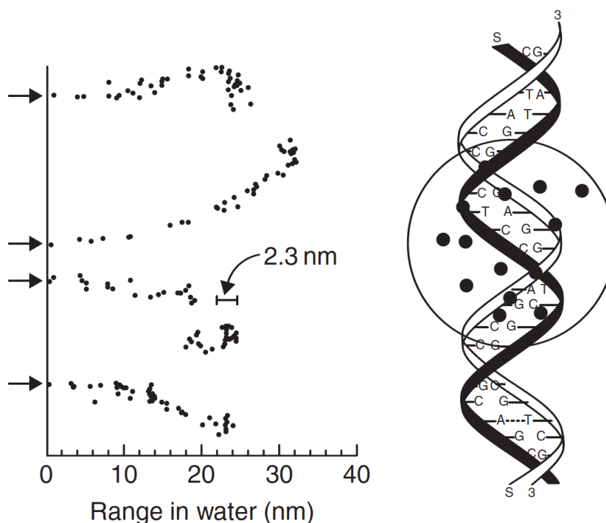
FIGURE 3.1: Computer-simulated tracks of 1 keV electrons showing the size of the clusters in relation to the size of the DNA [14].
