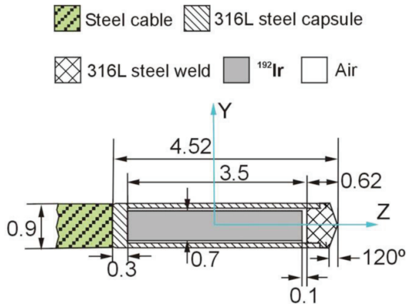
FIGURE 5.1: Materials and dimensions (mm) of the GammaMed source [32].
