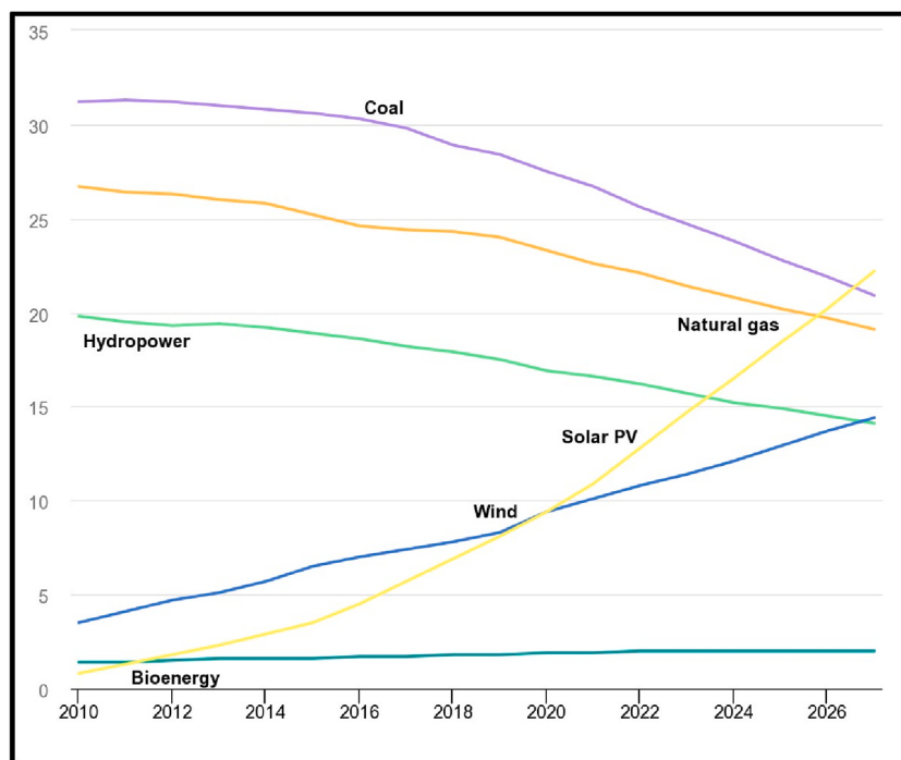
Fig. 7. Cumulative power capacity by technology, 2010–2027 (IEA, 2022).
