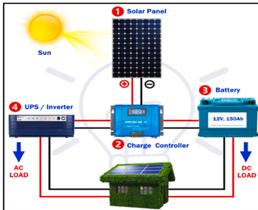
Fig. 4. The main components of a solar panel system.
