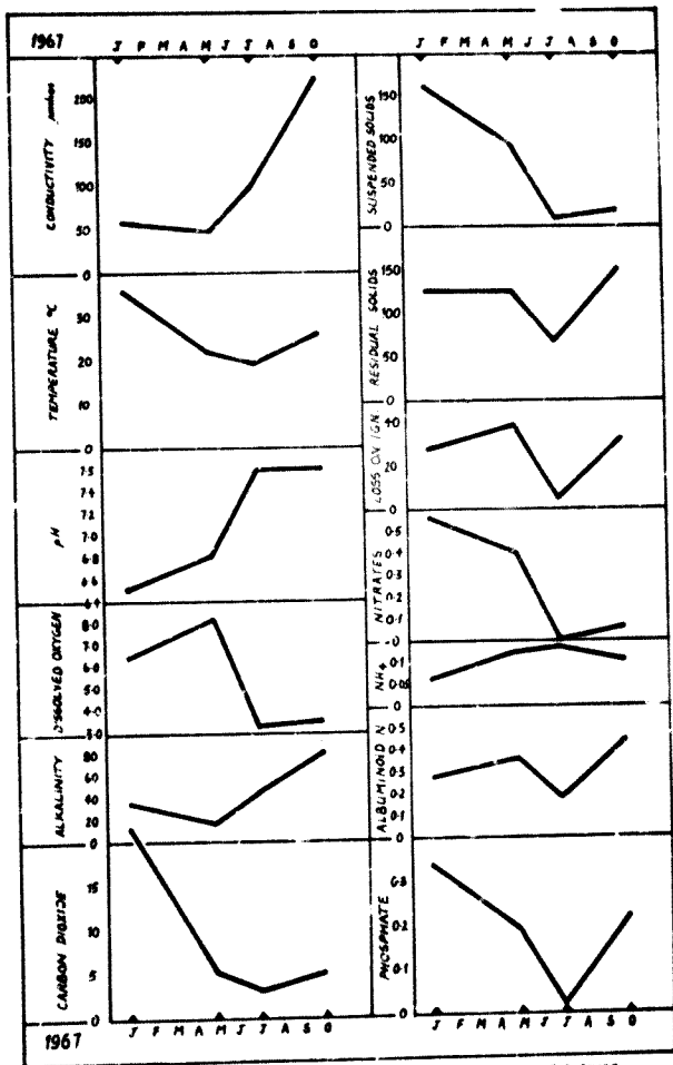
Fig. 5.10 THE SEASONAL CHANGES IN WATER QUALITY OF THE JATIC RIVER. Readings in mg/l unless otherwise stated.
