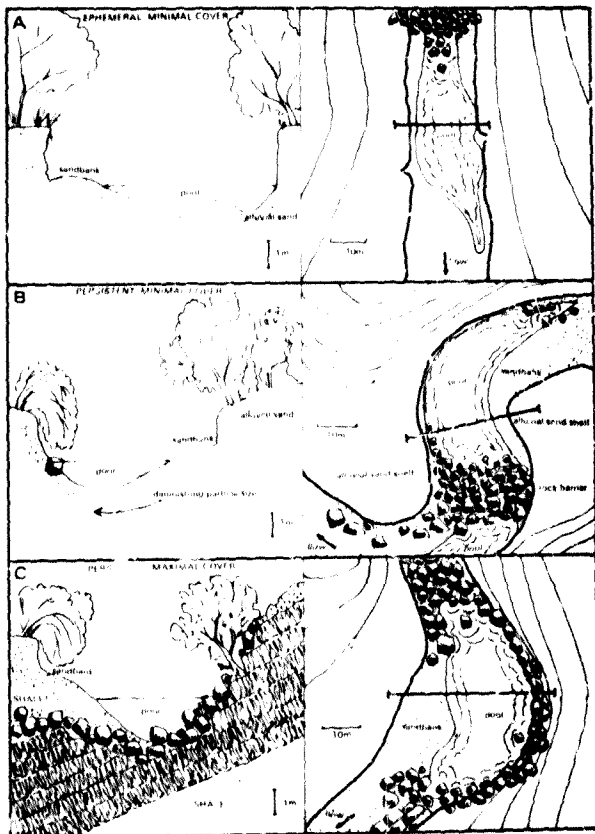
Fig. 3.10. DIAGRAMMATIC PLANS AND SECTIONS OF THREE POOLS: (A) EPHEMERAL CHAMPS POOL; (B) SURPRISE POOL; (C) DEEP POOL AS INTERPRETED FROM SURFACE INDICATIONS.
