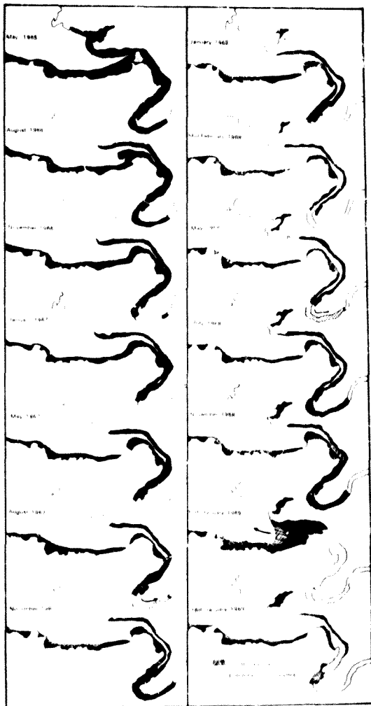
Fig. 4.7. VARIATION IN AREA COVERED BY SALINITY MAY 1965 TO JANUARY 1969
