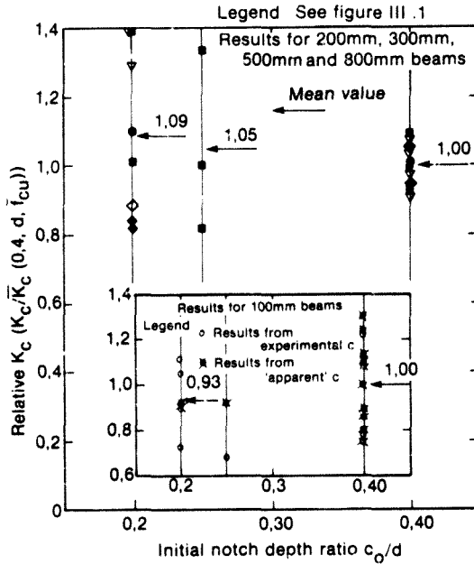
Figure 9.7 Effect of initial notch depth ratio on K_c
