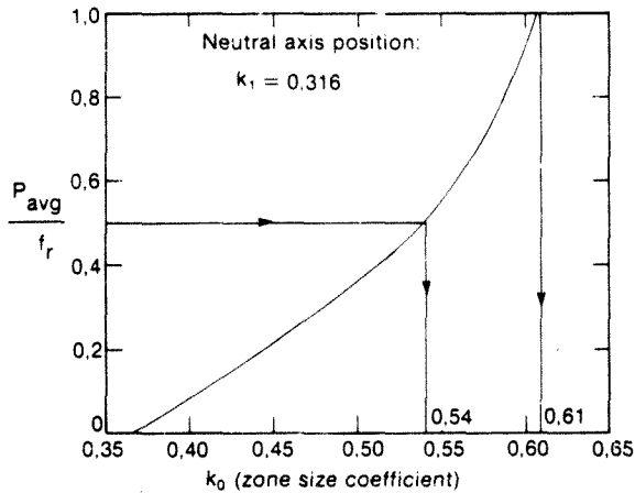
Figure 9.13 Dependence of average stress in microcracked zone on zone size
