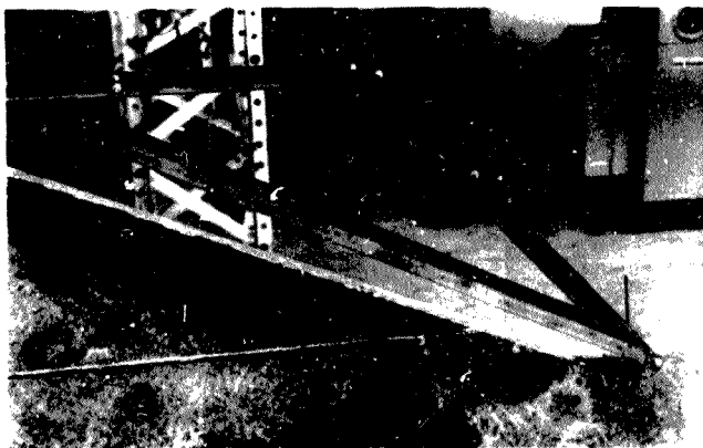
Figure B2(c) One side of modified deflection rig in position on a 800mm deep variable section beam (series F2)
