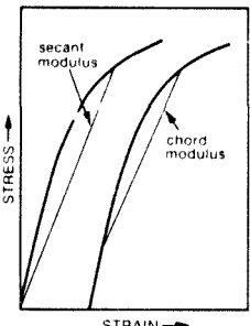
Figure 1 Typical stress-strain curve for concrete
