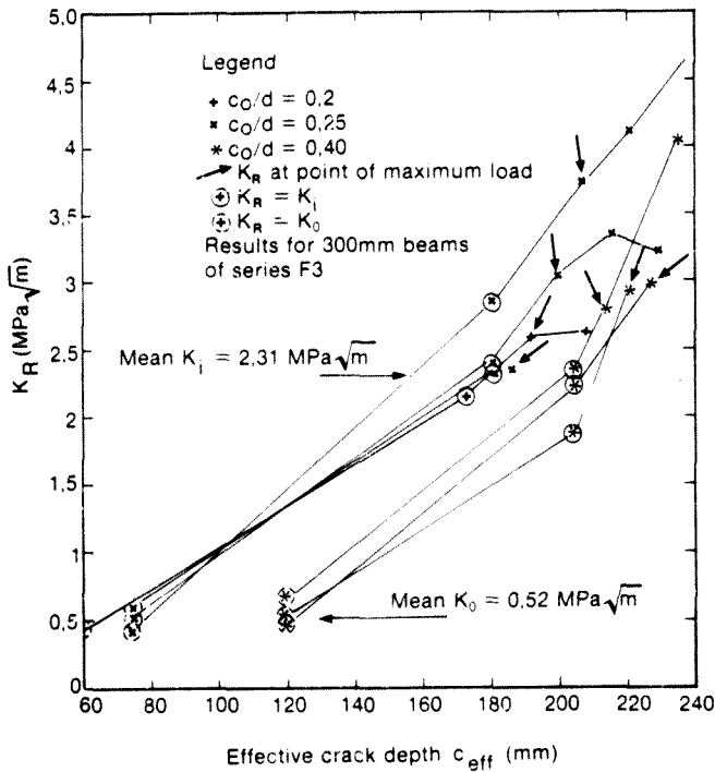
Figure 9.15 K_R -curves for 300mm beams of series F3
