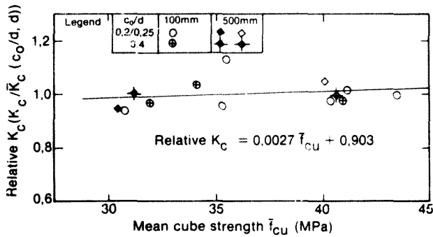
Figure 9.6 Effect of compressive strength on K_c
