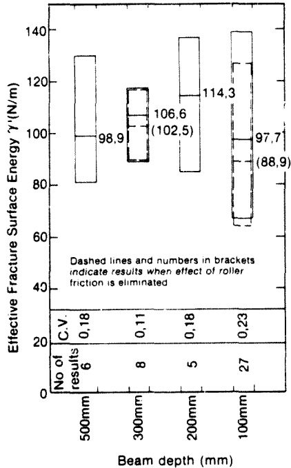
Figure 9.21 Combined results for effective fracture surface energy from all series
