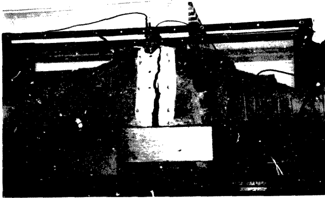
Figure B2(d) Modified deflection rig in position on a 300mm deep variable section beam (series F3) (Note different modification to that of figure B2(c))
