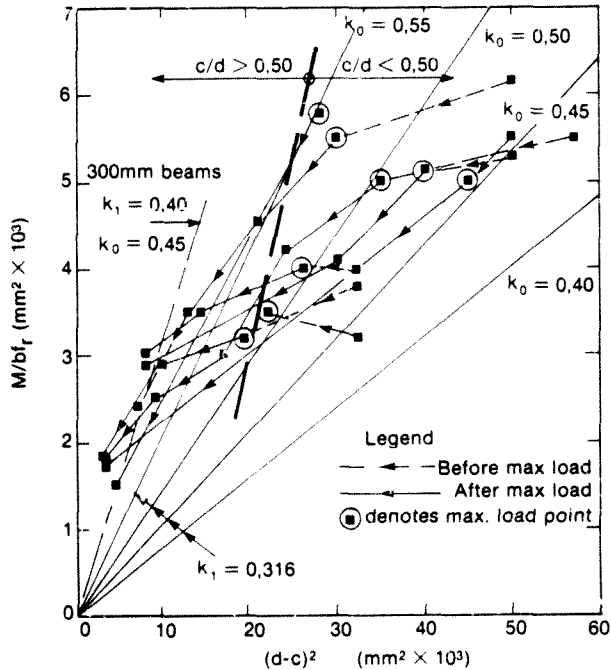
Figure 9.14 Moment of resistance relationships for 300mm fracture beams
