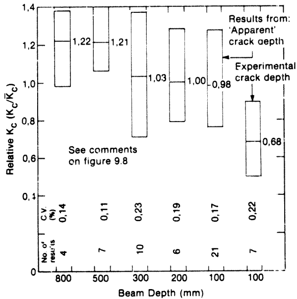
Figure 9.9 Effect of beam depth on K_c , combined results
