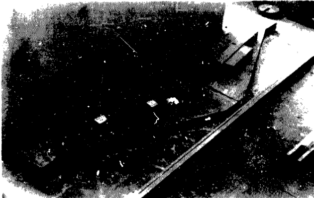
Figure A5 Demoulded beams on laboratory floor, prior to commencement of curing (series F2)
