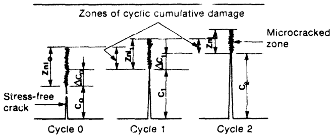
Figure 9.22 Schematic illustration of cyclic crack extension resulting in cumulative damage in the microcracked zone
