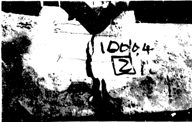
Figure 9.18 Cracking pattern at failure for beam F3/26(100/0,4)
