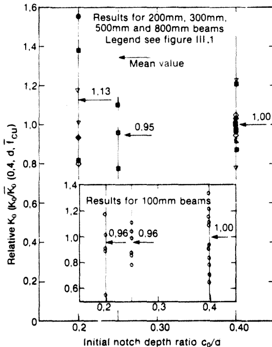
Figure 9.5 Effect of initial notch depth ratio on K_0
