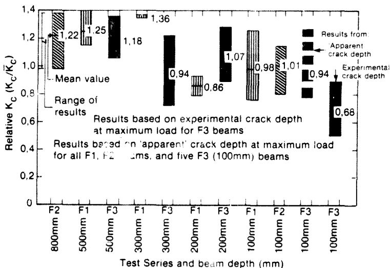
Figure 9.8 Effect of beam depth on K_c for various series
