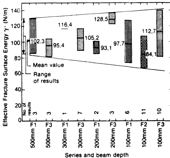
Figure 9.20 Effect of beam depth on effective fracture surface energy
