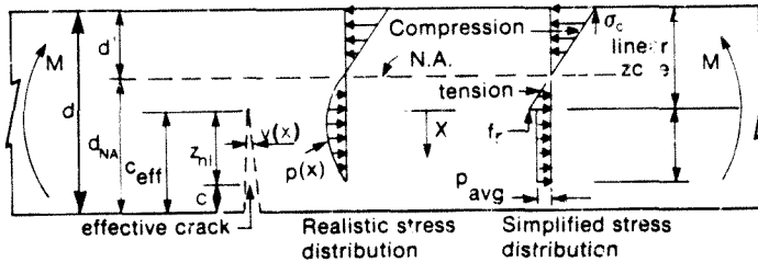
Figure 9.12 Effective crack and assumed stress distributions in concrete fracture beams
