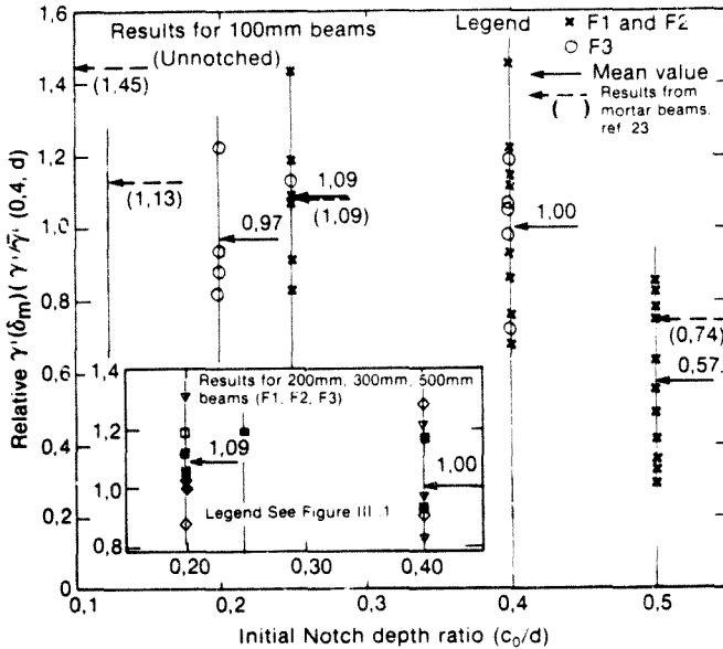
Figure 9.19 Effect of initial notch depth ratio on \gamma'
