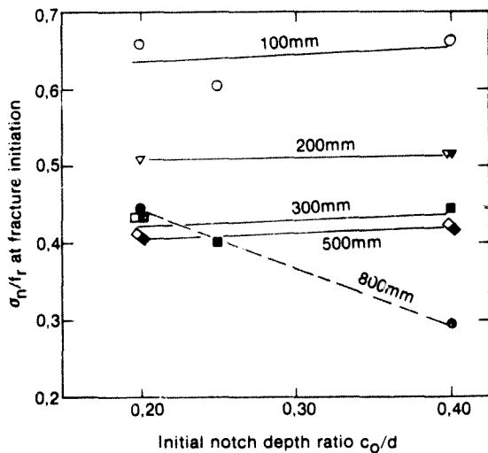
Figure 9.3 Relative net stress at fracture initiation (series F1, F2, F3)
