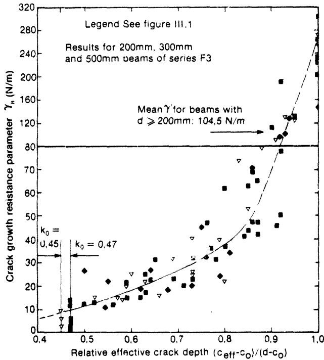
Figure 9.23 \gamma_R -curve for beams of series F3 expressed as a function of relative effective crack depth
