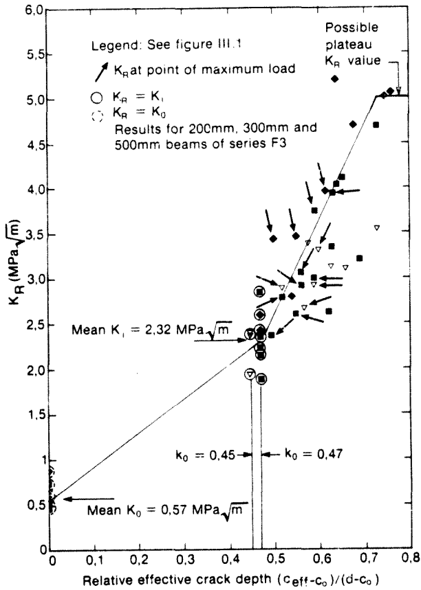
Figure 9.16 K_R -curve for beams of series F3 expressed as a function of relative effective crack depth
