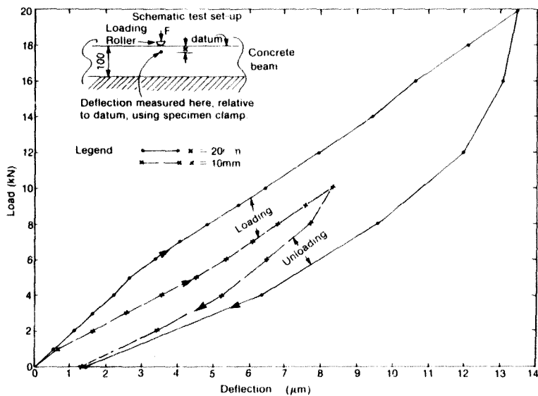
Figure B3 Load-deflection curves showing effect of loading roller on measured deflections
