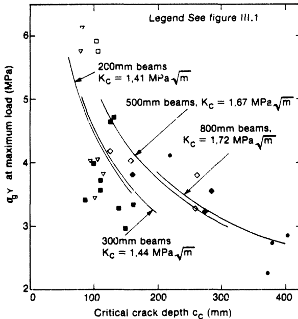
Figure 9.11 Mean K values for beams of all three series taken together (unmodified)
