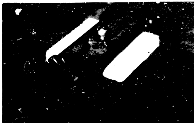
Figure B1 Detail of deflection clamp and loading roller
