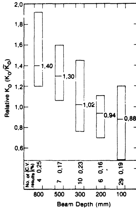
Figure 9.10 Effect of beam depth on K_0 , combined results
