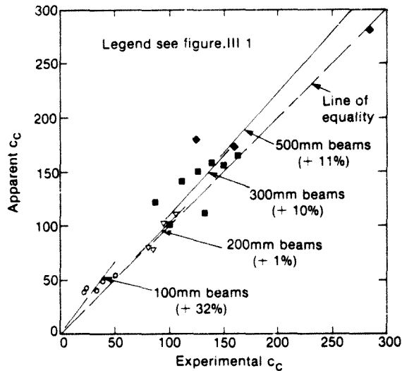
Figure 9.2 Comparison of apparent and experimental c_c values for beams of series F3
