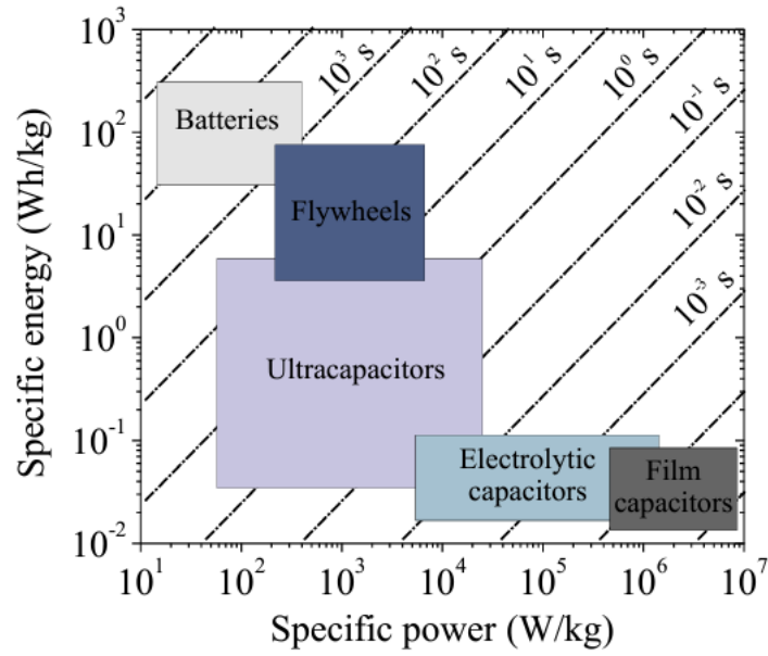
Figure 6.6: Ragone Plot showing the ESS power and energy densities [53]
