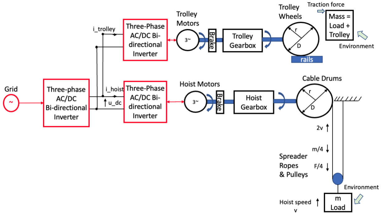
Figure 4.1: Studied port crane system
