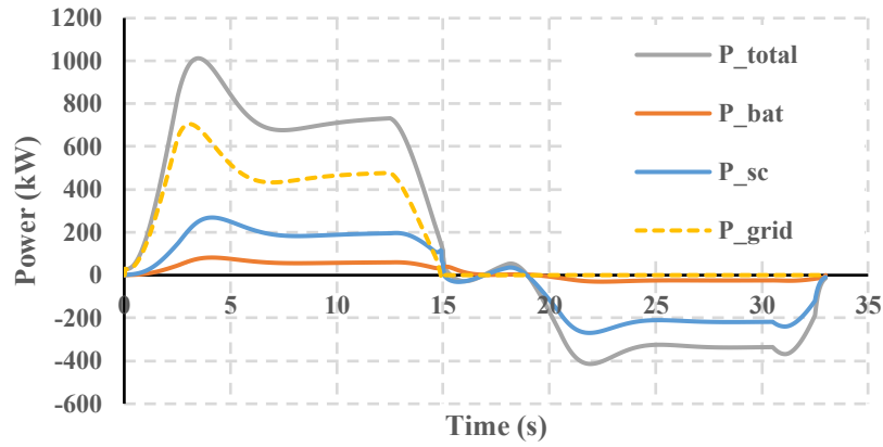
Figure 6.11: Port crane simulated power consumption
