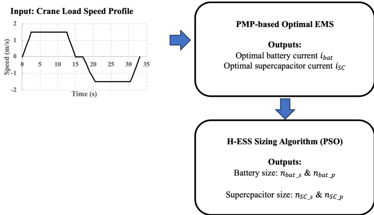
Figure 7.4: Generalised port crane H-ESS sizing framework
