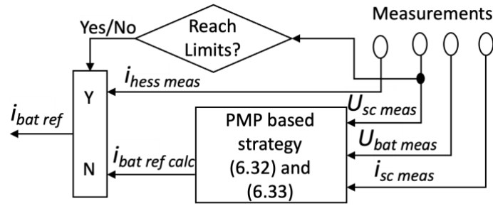
Figure 6.4: PMP-based EMS for power split management in the batt-SC H-ESS
