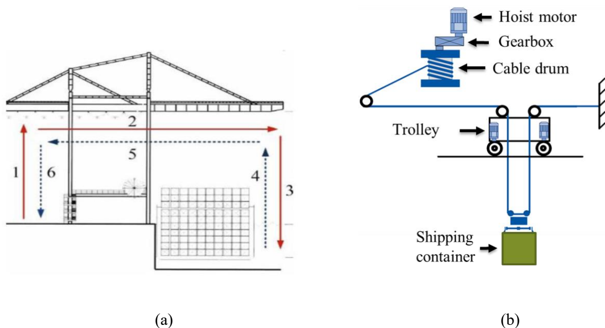
Figure 3.1: Port crane motions (a), port crane drivetrain (b)
