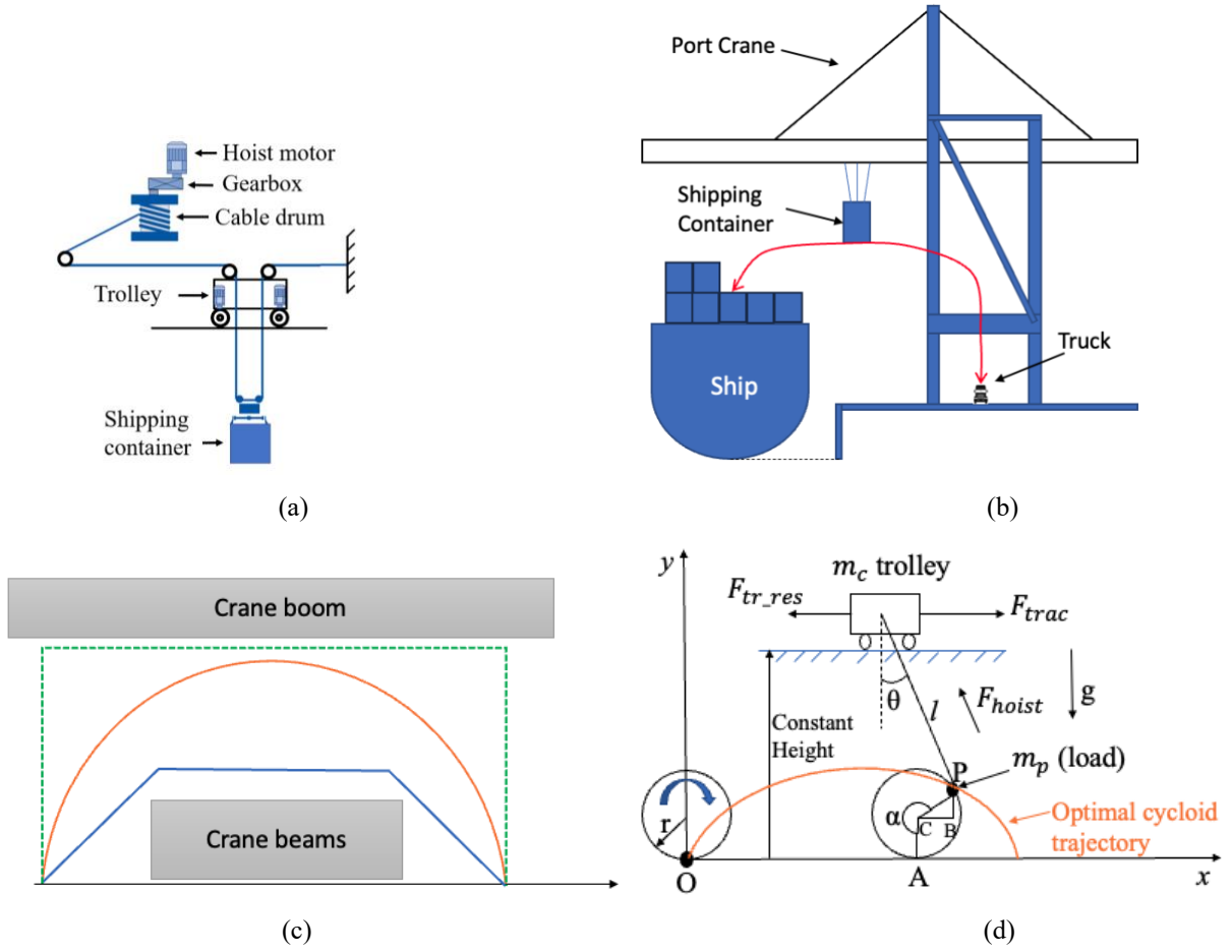
Figure 5.1: Port crane hoist and trolley mechanisms layout, (a) port crane motions, hoisting (1&4), lowering (6&3) and trolley (2&5) (b), port crane trajectories and constraints (c), and optimal port crane trajectory (d)
