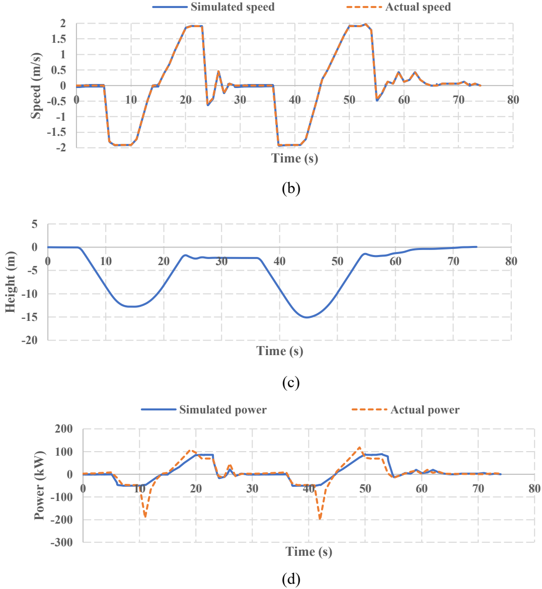
Figure 4.5: Port crane (a) hoist motor reference speed profile (b) simulated vs. actual speed (c) non-optimal trajectory (d) simulated vs. actual power consumption
