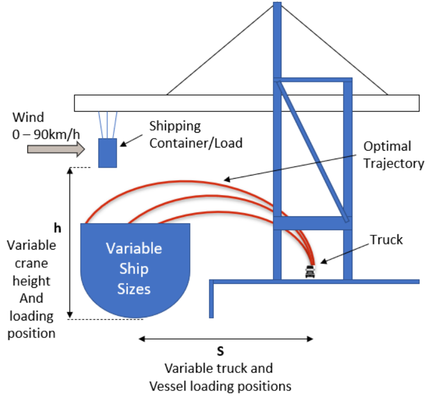
Figure 5.2: Port crane multiple optimal cycloid load trajectories
