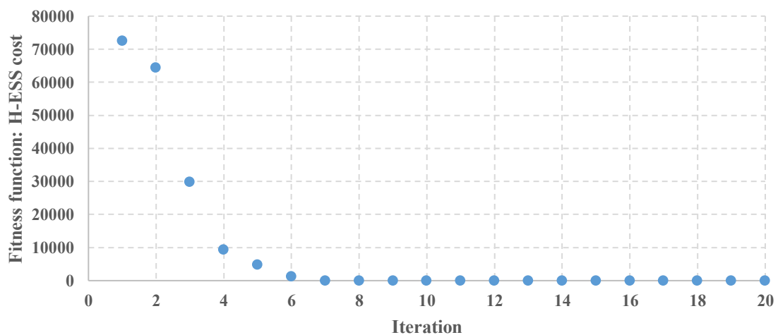
Figure 7.8: PSO H-ESS cost convergence plot
