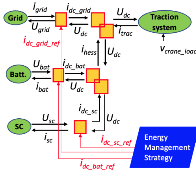
Figure 7.1: Reduced port crane EMR model
