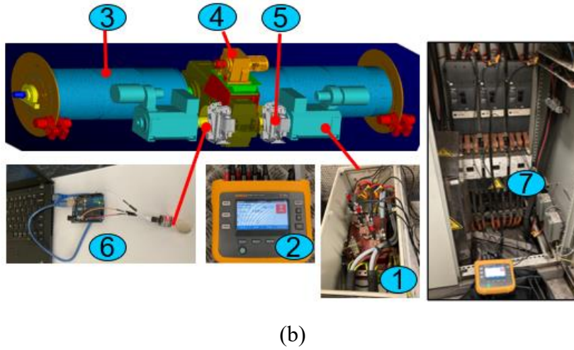
Figure 4.4: Experimental setup (a) and (b): (1) Hoist motor (2) Fluke 1736 power logger (3) Cable drum (4) Gearbox (5) Mechanical brakes (6) PC, Arduino UNO board, and hall effect sensor (7) Low voltage panel
