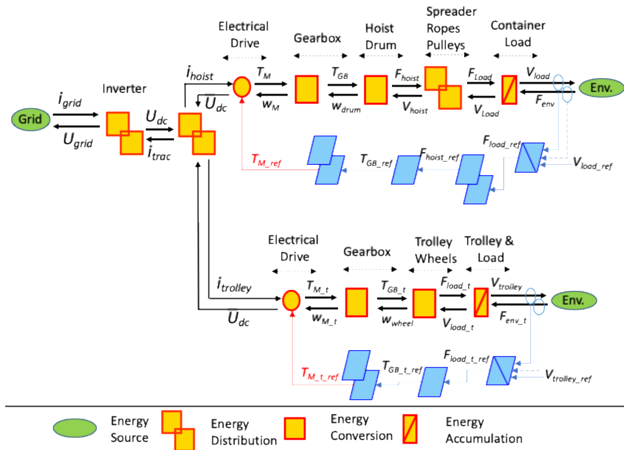
Figure 4.2: Port crane EMR and inversion-based local control
