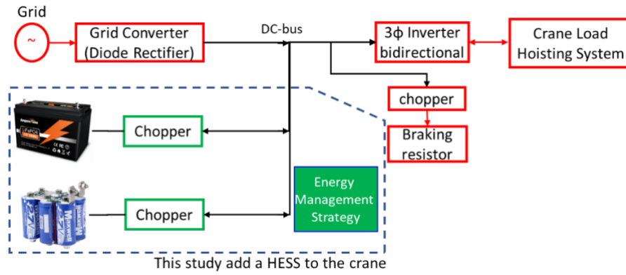
Figure 3.2: Port crane powertrain
