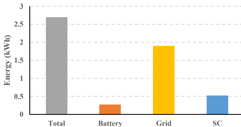
Figure 6.10: Port crane energy consumption for one load cycle
