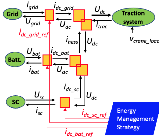
Figure 6.2: Reduced port crane EMR model used for EMS development
