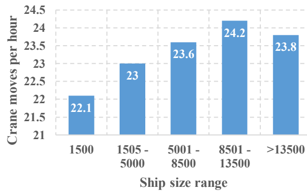
Figure 5.3: Real-world crane loading frequency per ship size [52]
