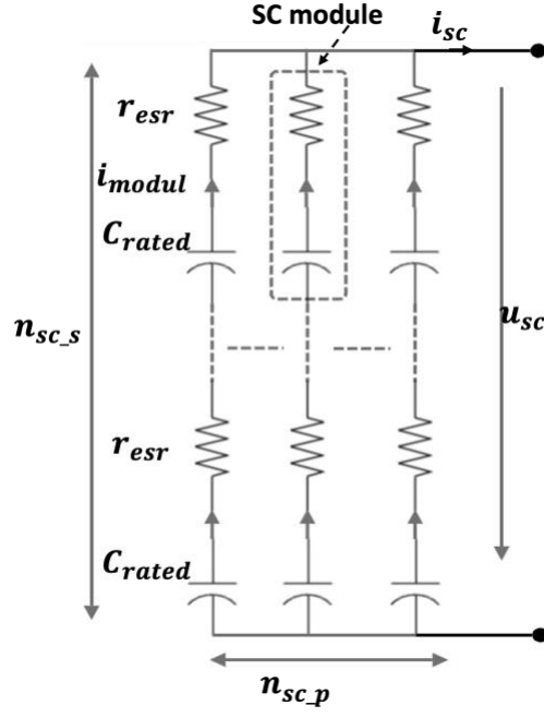
Figure 7.2: Supercapacitor pack equivalent circuit [62]
