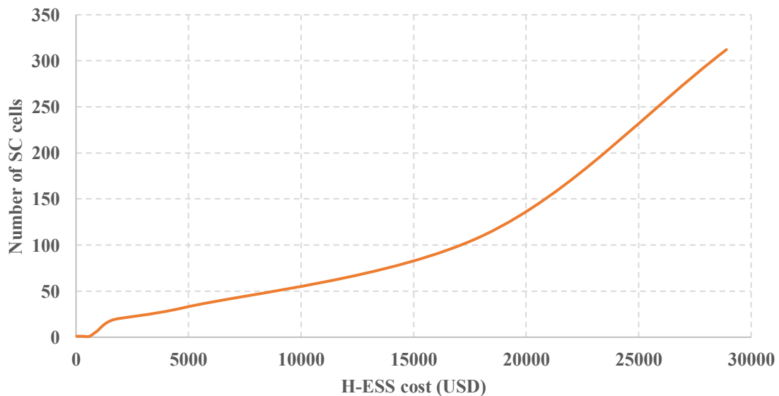
Figure 7.6: Supercapacitor size vs. H-ESS cost
