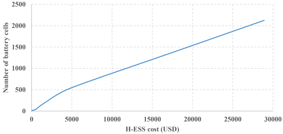
Figure 7.7: Battery size vs. H-ESS cost
