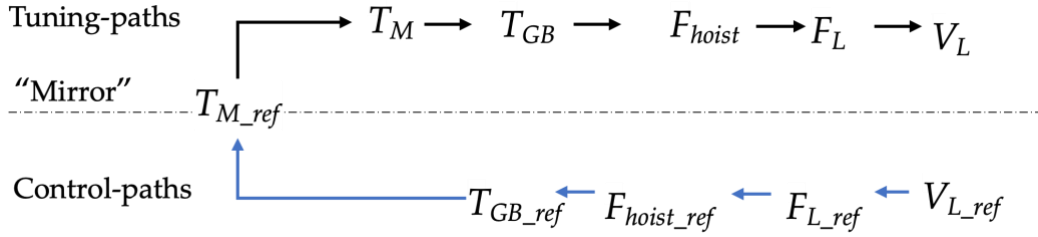
Figure 4.3: Port crane local control system
