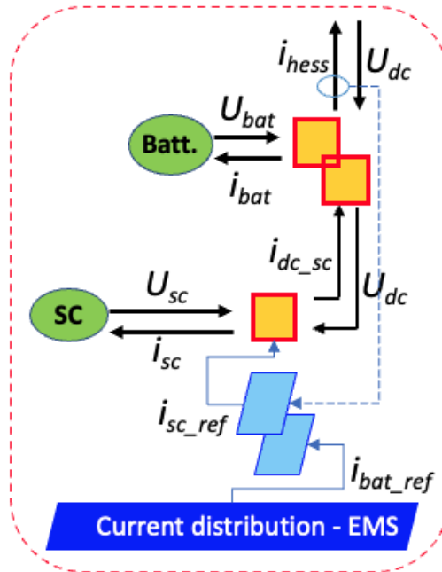
Figure 6.3: Port crane EMR model used for PMP strategy development
