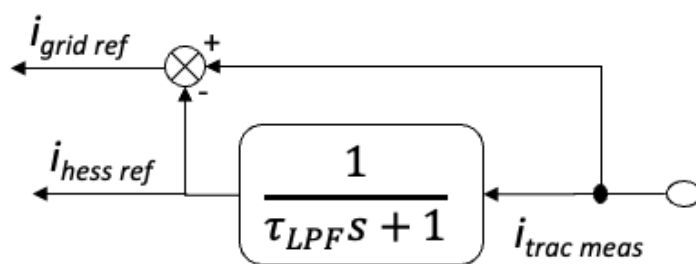
Figure 6.8: Implementation of the filtering strategy to manage the power split between the grid and the H-ESS
