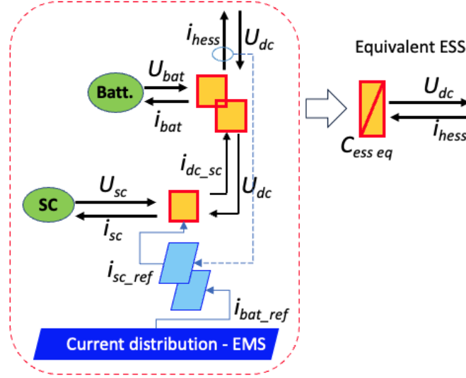
Figure 6.5: H-ESS reduction to an equivalent ESS given the battery's dominant capacitance
