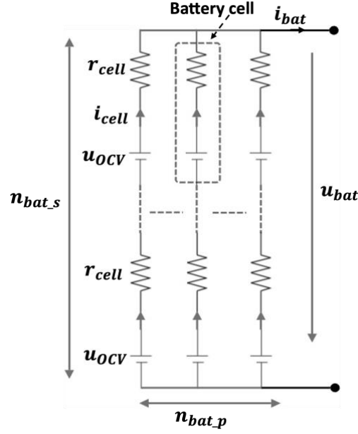
Figure 7.3: Battery pack equivalent circuit [62]
