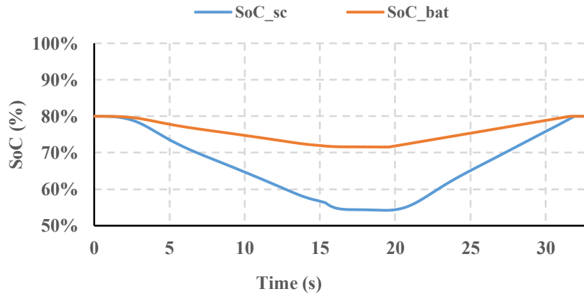
Figure 6.12: One load cycle battery and supercapacitor SOC
