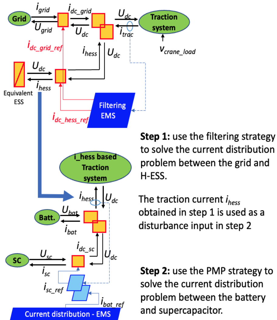
Figure 6.9: Step-by-step implementation of the combined EMS comprising of the filtering and the PMP-based sub-EMSs
