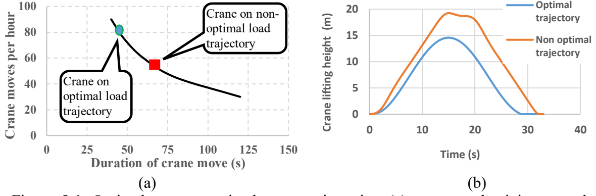
Figure 5.4: Optimal vs. non-optimal crane trajectories, (a) crane productivity curve-based comparison (b) trajectory-based comparison
