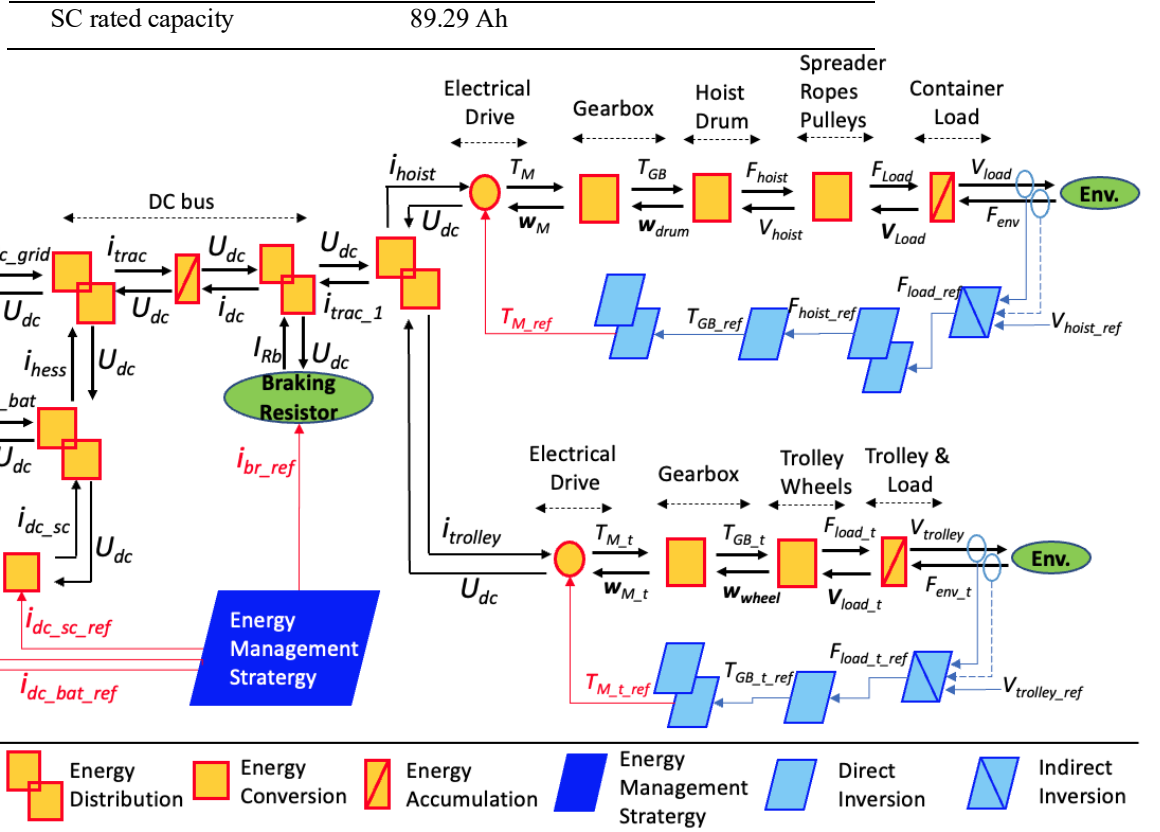
Figure 6.1: EMR model of the port crane and its inversion-based local control system
