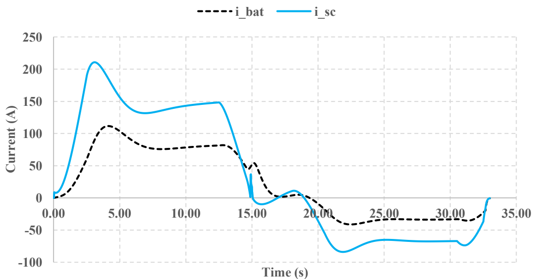
Figure 7.5: Optimal battery and supercapacitor currents
