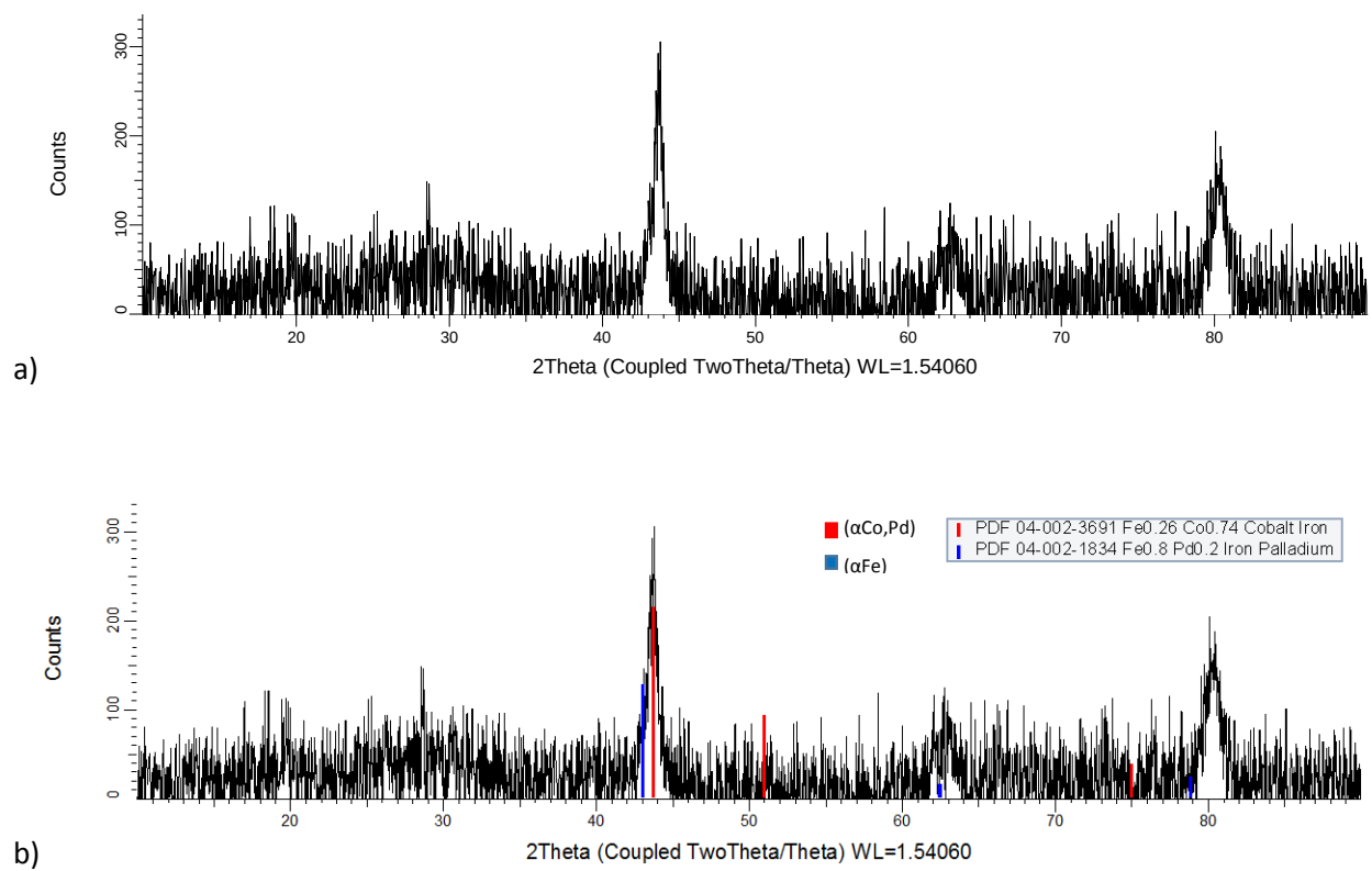
Figure 4.33. XRD patterns for nominal \text{Co}_{20}\text{:Fe}_{60}\text{:Pd}_{20} (at.%), Alloy 11 as-cast condition: a) raw, and b) labelled.
