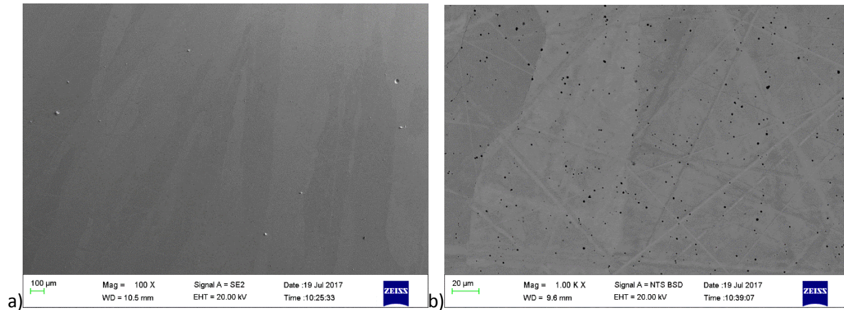
Figure 4.4. SEM images of as-cast \text{Co}_6\text{Fe}_{44}\text{Pd}_{50} (at.%), Alloy 2 showing: a) SE grains, and b) BSE higher magnification.
