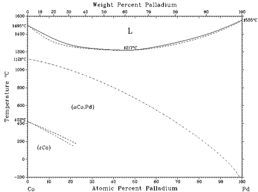
Figure 2.5. Binary diagram for Pd-Co system [1990Mas].
