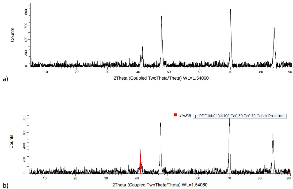
Figure 4.78. XRD patterns for nominal \text{Co}_6\text{:Fe}_{44}\text{:Pd}_{50} (at.%), Alloy 2 650°C annealed condition: a) raw, and b) labelled.
