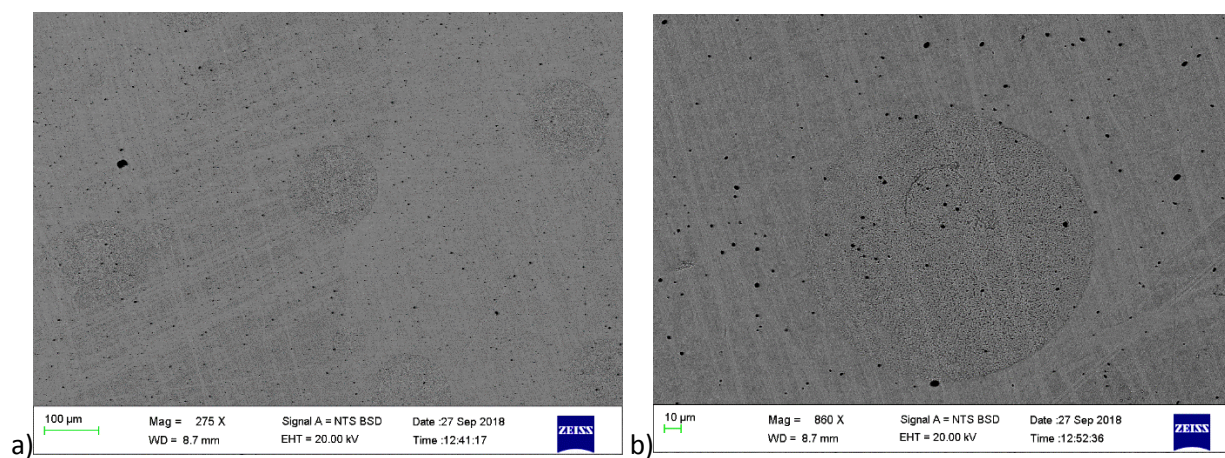
Figure 4.55. SEM-BSE images of \text{Co}_{10}\text{:Fe}_{30}\text{:Pd}_{60} (at.%), Alloy 7 annealed at 1000^{\circ}\text{C} for 1000 h showing: a) etched-out patches, and b) patch at higher magnification.
