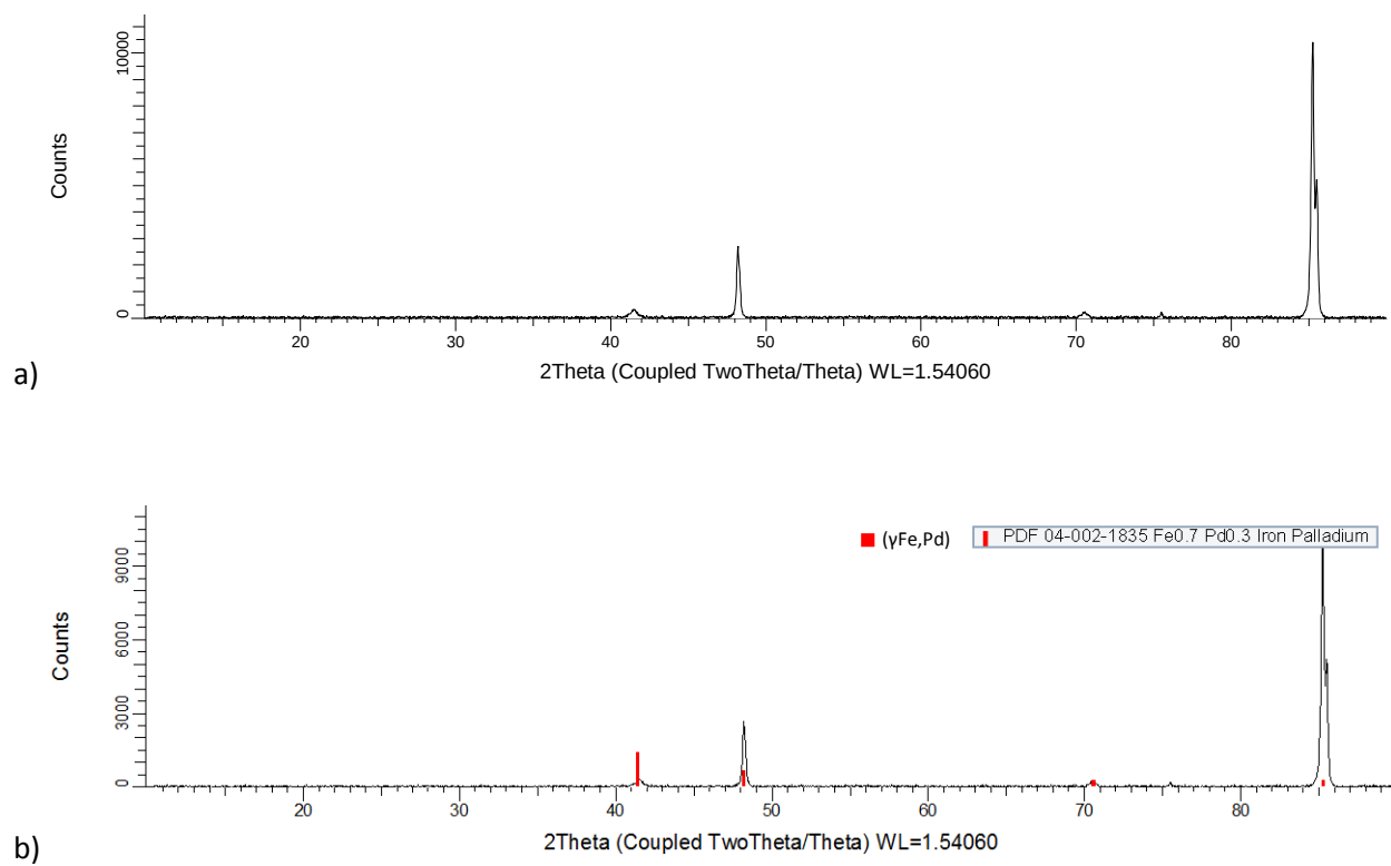
Figure 4.27. XRD patterns for nominal \text{Co}_{10}\text{:Fe}_{50}\text{:Pd}_{40} (at.%), Alloy 9 as-cast condition: a) raw, and b) labelled.
