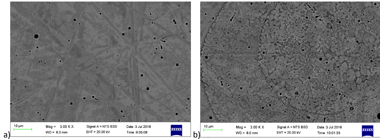
Figure 4.19. SEM-BSE images of as-cast \text{Co}_{10}\text{:Fe}_{30}\text{:Pd}_{60} (at.%), Alloy 7 showing: a) the formation of needles surrounded by a lighter phase, and b) a local area of inhomogeneity.
