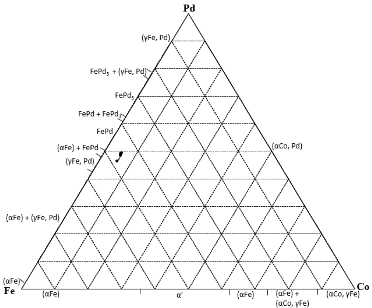
Figure 4.98. EDX analyses of nominal \text{Co}_{10}\text{:Fe}_{50}\text{:Pd}_{40} (at.%), Alloy 9 650°C annealed condition. (■ Overall composition; ● phases)
