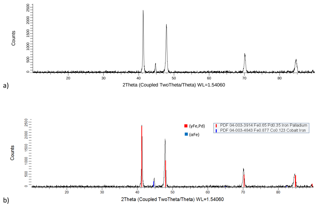
Figure 4.99. XRD patterns for nominal \text{Co}_{10}\text{:Fe}_{50}\text{:Pd}_{40} (at.%), Alloy 9 650°C annealed condition: a) raw, and b) labelled.
