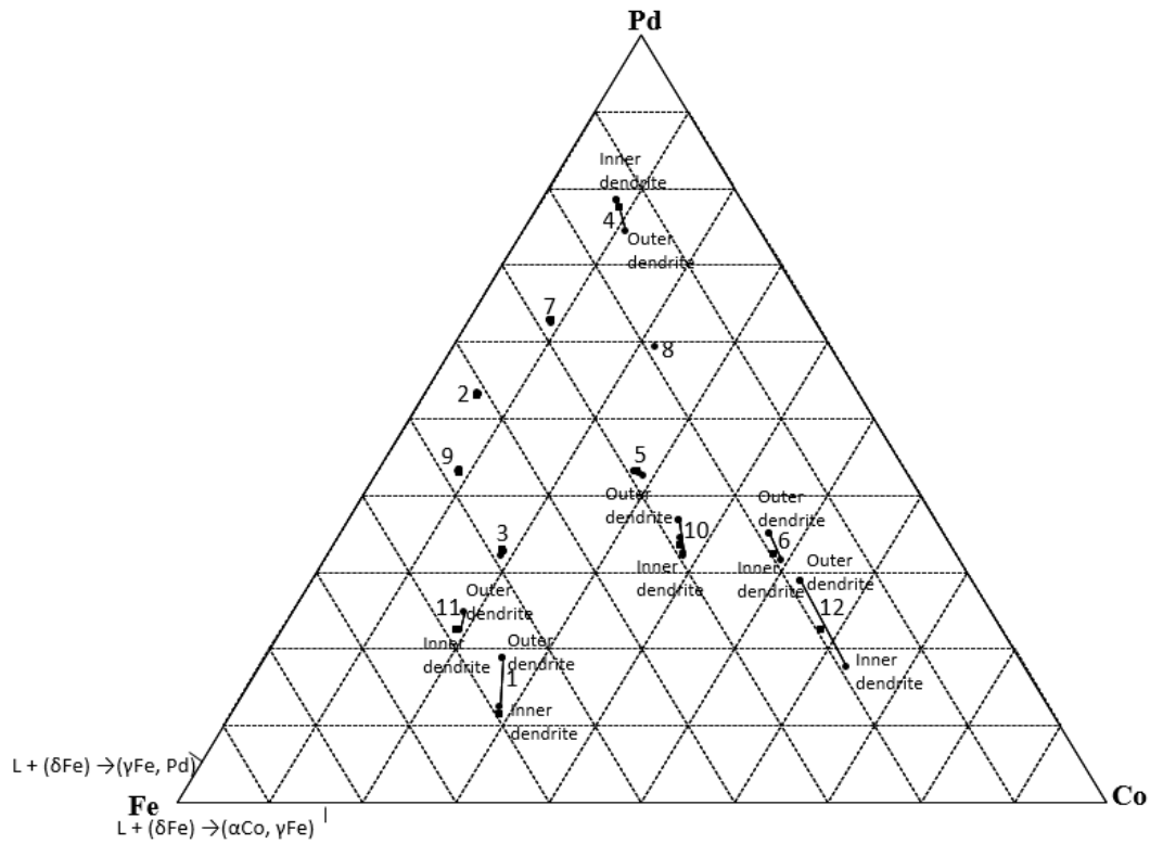
Figure 6.1 Solidification projection for the as-cast Co-Fe-Pd system. (■ Overall composition; ● phases)
