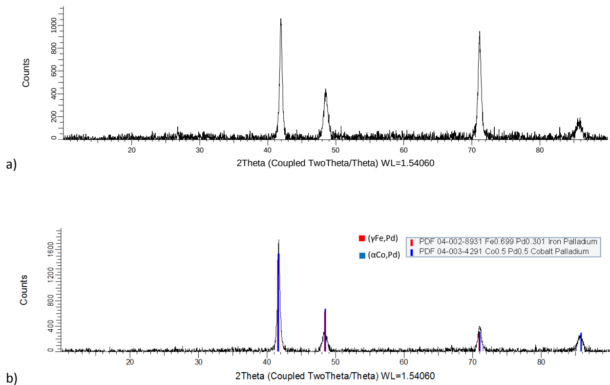
Figure 4.51. XRD patterns for nominal \text{Co}_{30}\text{:Fe}_{30}\text{:Pd}_{40} (at.%), Alloy 5 1000°C annealed condition: a) raw, and b) labelled.
