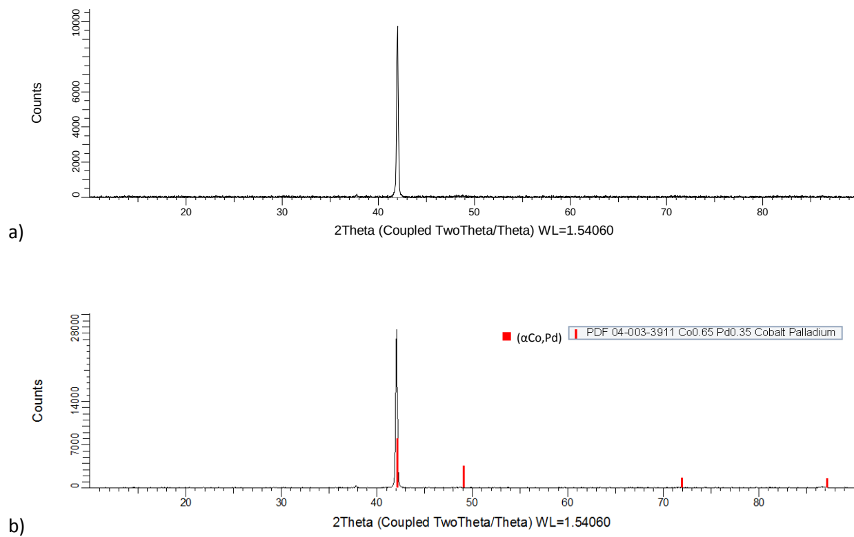
Figure 4.30. XRD patterns for nominal \text{Co}_{40}\text{:Fe}_{30}\text{:Pd}_{30} (at.%), Alloy 10 as-cast condition: a) raw, and b) labelled.
