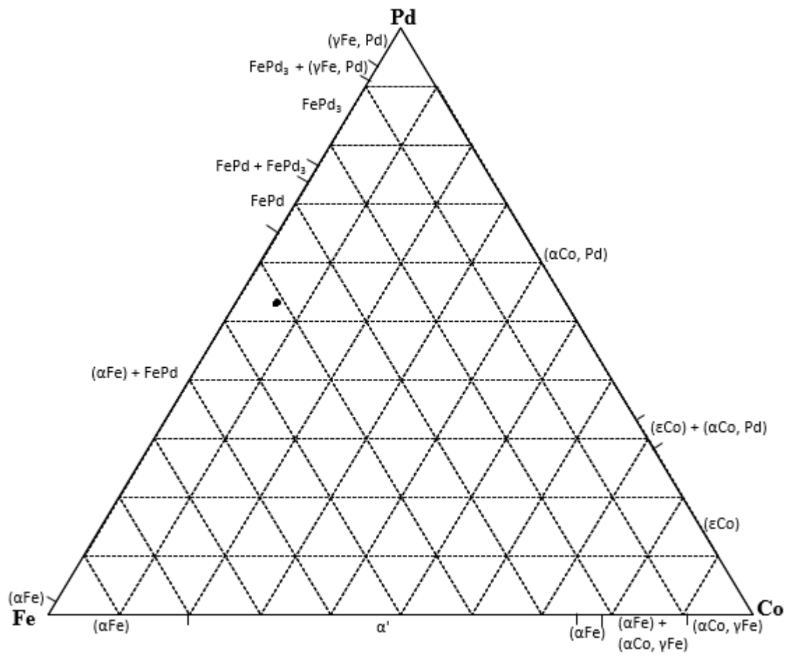
Figure 4.5. EDX analyses of nominal \text{Co}_6\text{:Fe}_{44}\text{:Pd}_{50} (at.%), Alloy 2 as-cast condition. (■ Overall composition; ● phases)
