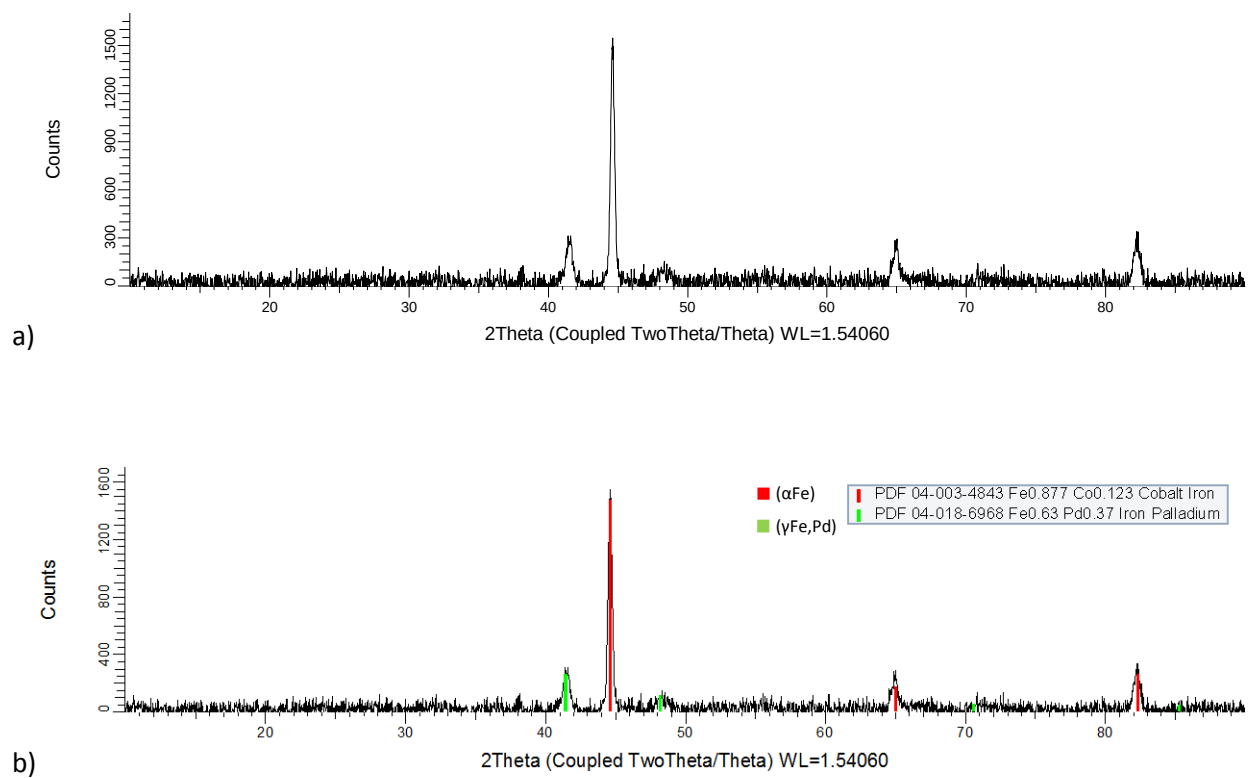
Figure 4.3. XRD patterns for nominal \text{Co}_{30}\text{:Fe}_{60}\text{:Pd}_{10} (at.%), Alloy 1 as-cast condition: a) raw, and b) labelled.
