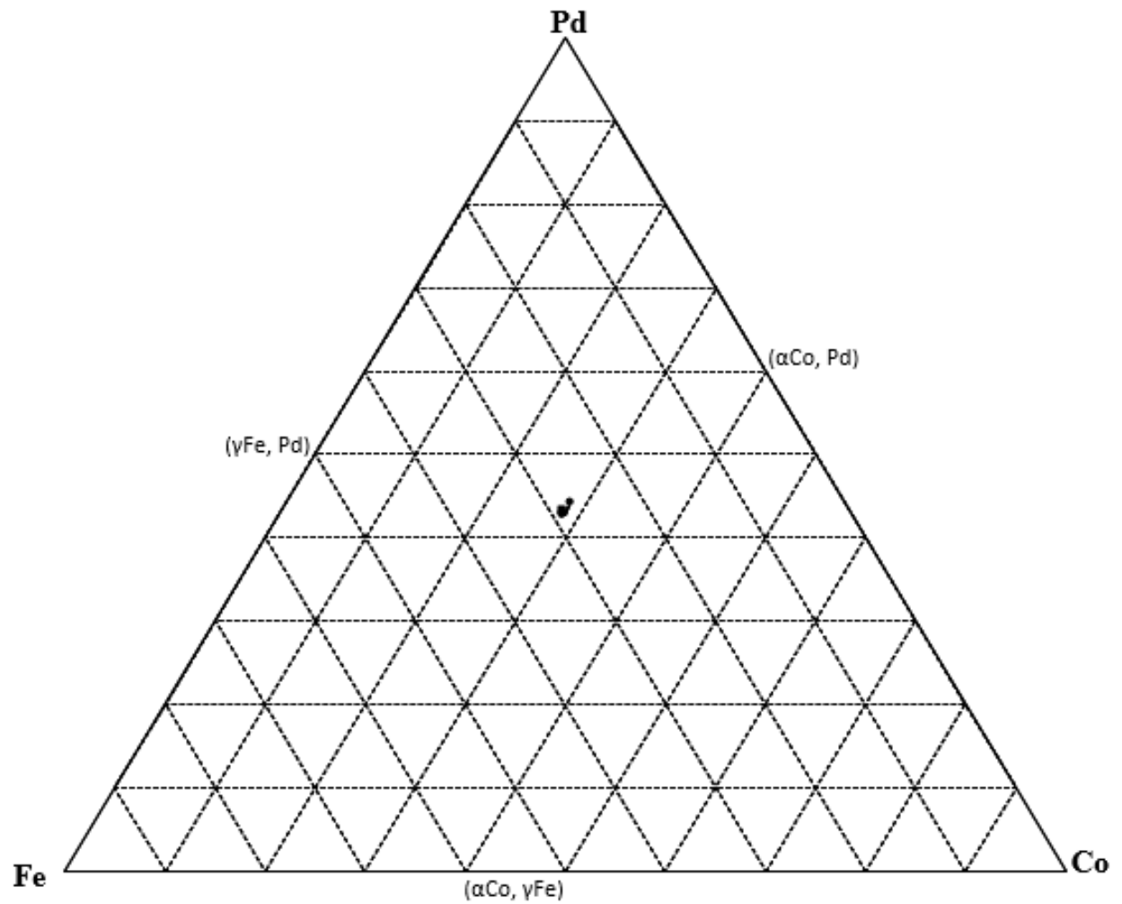
Figure 4.50. EDX analyses of nominal \text{Co}_{30}\text{Fe}_{30}\text{Pd}_{40} (at.%), Alloy 5 1000°C annealed condition. (■ Overall composition; ● phases)
