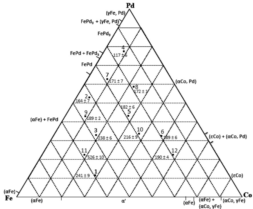
Figure 5.1. Ternary plot with microhardness values and errors for as-cast alloys. (■ Overall composition)
