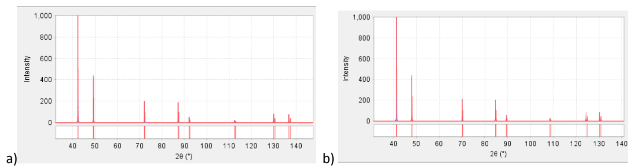
Figure 2. XRD peaks used to identify a) (γFe, Pd) and b) (αCo, Pd) [2018Dif].
