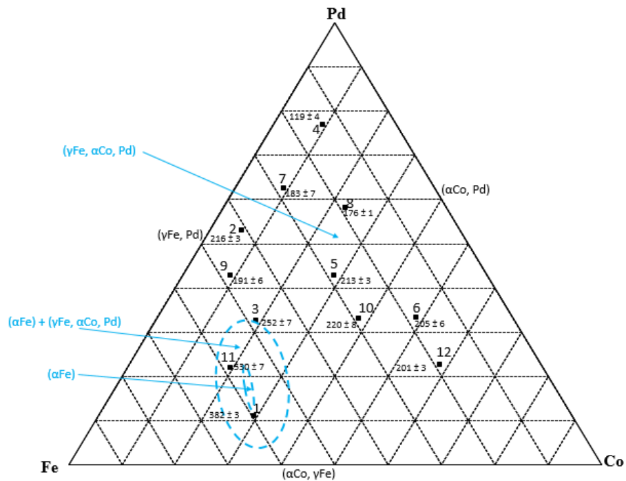
Figure 6.7. Isothermal section at 1000°C for the Co-Fe-Pd system with hardnesses. (■ Overall composition)
