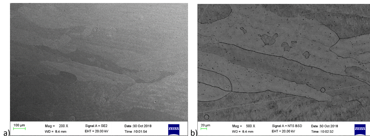
Figure 4.82. SEM-SE and SEM-BSE images of \text{Co}_{10}\text{Fe}_{15}\text{Pd}_{75} (at.%), Alloy 4 annealed at 650^\circ\text{C} for 1000 h: a) showing contrasting areas, and b) showing contrasting areas and grain boundaries.
