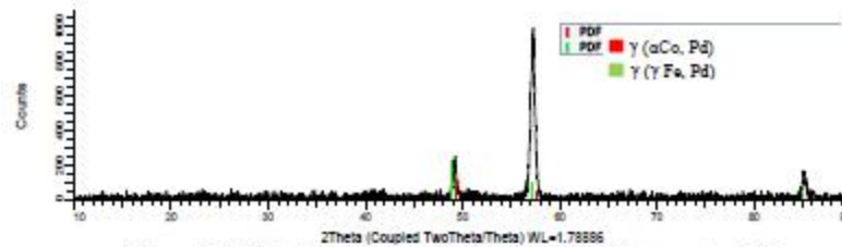
Figure 6. XRD pattern for nominal \text{Fe}_{30}\text{Co}_{30}\text{Pd}_{40} (at.%), as-cast condition.
