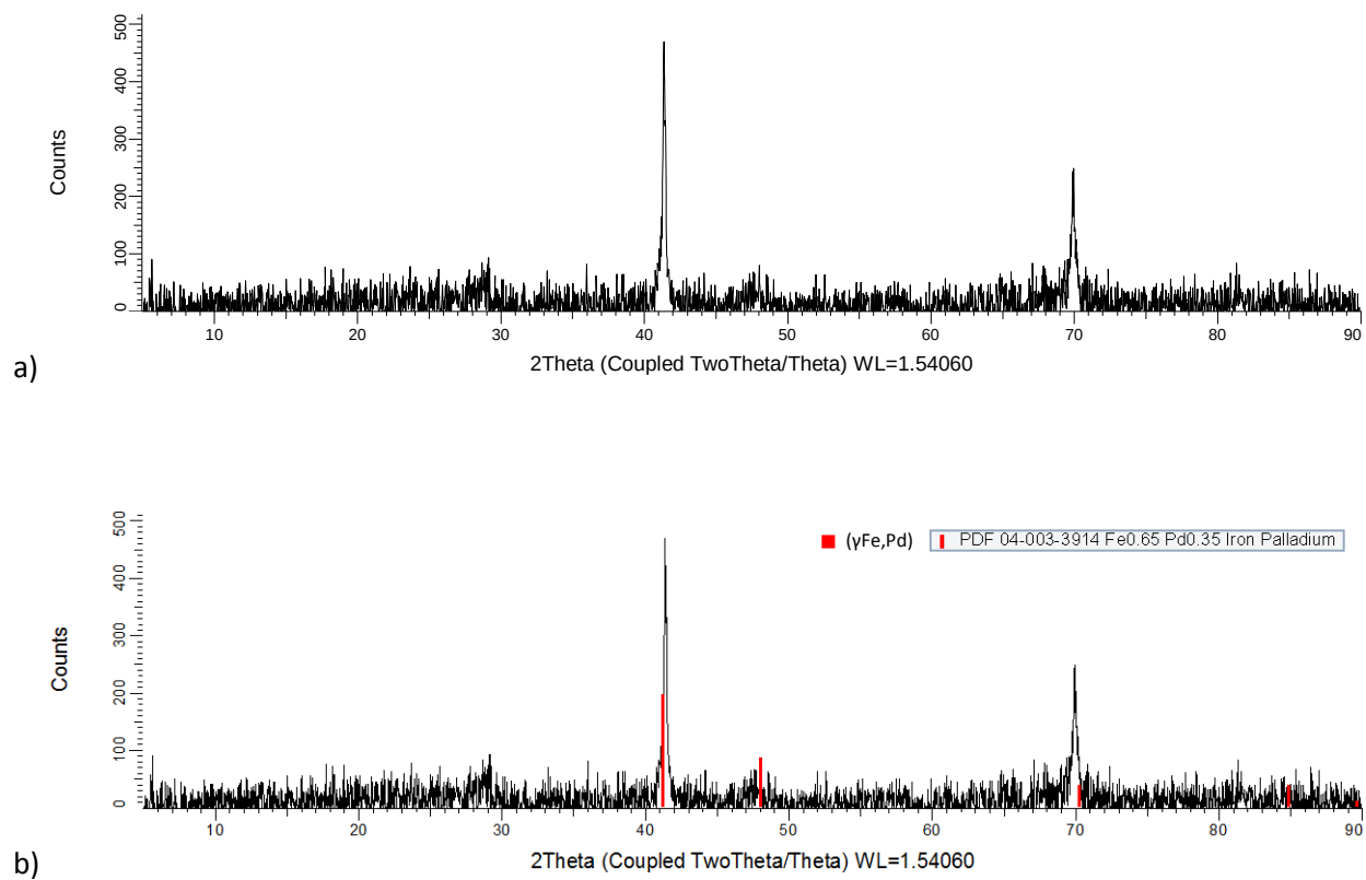
Figure 4.57. XRD patterns for nominal \text{Co}_{10}\text{:Fe}_{30}\text{:Pd}_{60} (at.%), Alloy 7 1000°C annealed condition: a) raw, and b) labelled.
