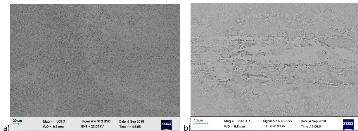
Figure 4.52. SEM-BSE images of \text{Co}_{50}\text{Fe}_{20}\text{Pd}_{30} (at.%), Alloy 6 annealed at 1000^{\circ}\text{C} for 1000 h showing: a) at low magnification the overall area, and b) a better etched area.
