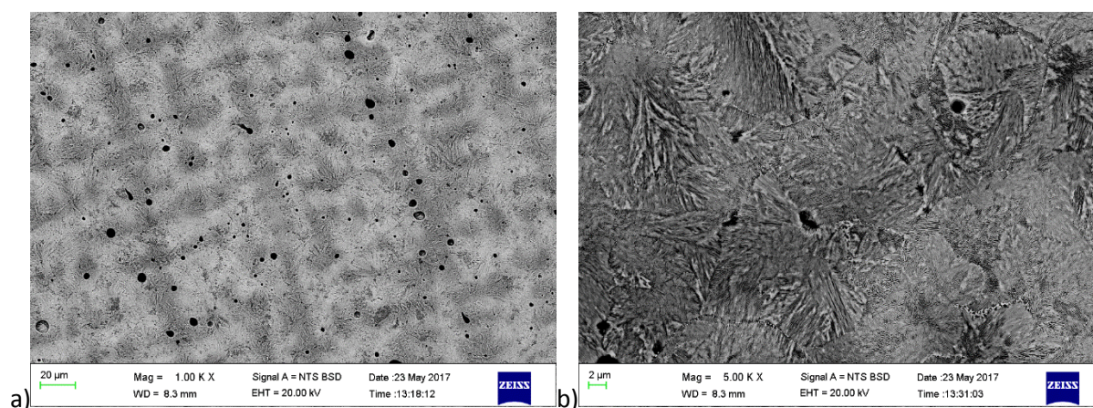
Figure 4.1. SEM-BSE images of as-cast \text{Co}_{30}\text{Fe}_{60}\text{Pd}_{10} (at.%), Alloy 1 showing: a) dendrites (darker), and b) showing decomposition at higher magnification.
