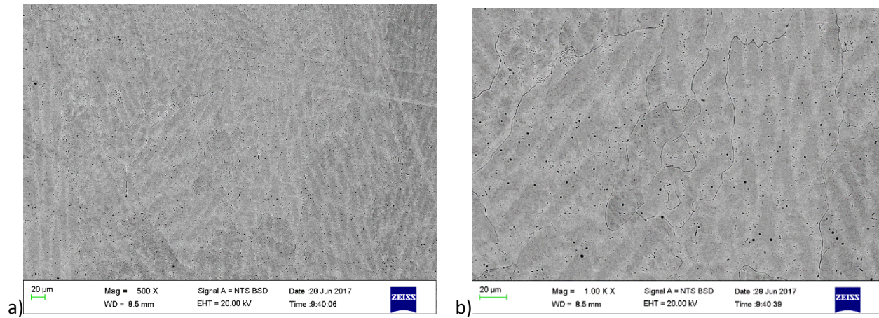
Figure 4.16. SEM-BSE images of as-cast \text{Co}_{50}\text{Fe}_{20}\text{Pd}_{30} (at.%), Alloy 6 showing a) coring and dark grain boundaries at low magnification and b) high magnification.
