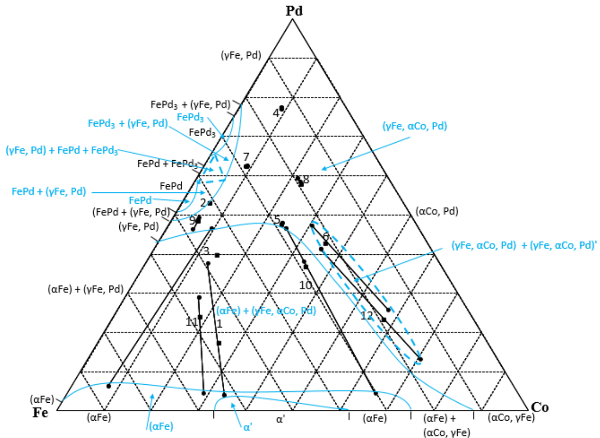
Figure 6.5. Isothermal section at 650°C annealed for the Co-Fe-Pd system (at.%). (■ Overall composition; ● phases)
