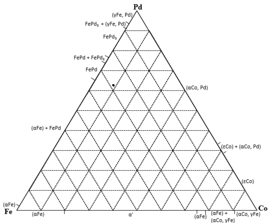
Figure 4.20. EDX analyses of nominal \text{Co}_{10}\text{Fe}_{30}\text{Pd}_{60} (at.%), Alloy 7 as-cast condition. (■ Overall composition; ● phases)
