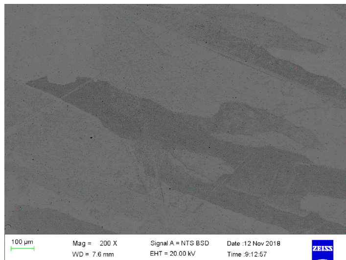
Figure 4.91. SEM-BSE image of \text{Co}_{10}\text{Fe}_{30}\text{Pd}_{60} (at.%), Alloy 7 annealed at 650^\circ\text{C} for 1000 h showing different grains.
