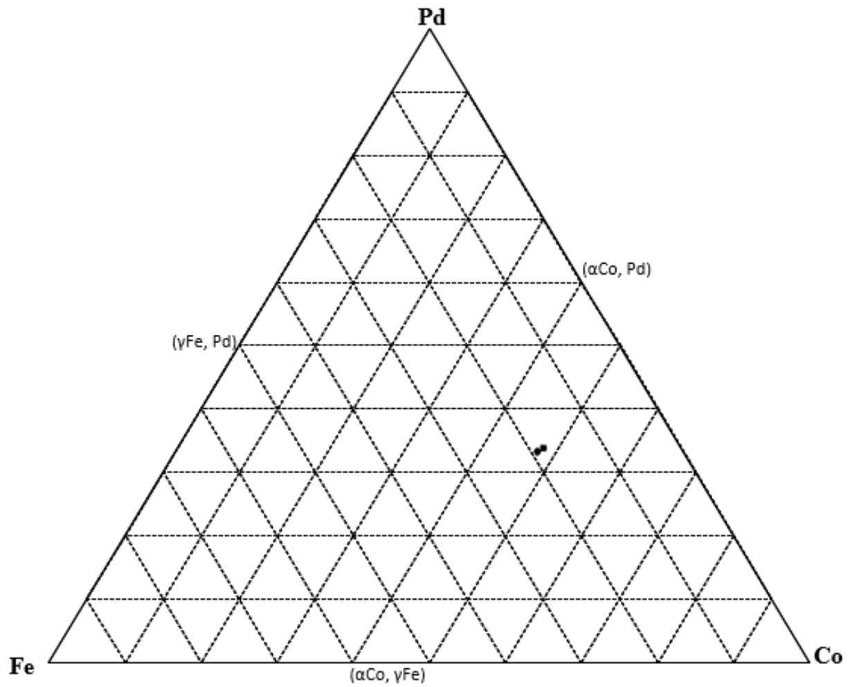
Figure 4.53. EDX analyses of nominal \text{Co}_{50}\text{Fe}_{20}\text{Pd}_{30} (at.%), Alloy 6 1000°C annealed condition. (■ Overall composition; ● phases)
