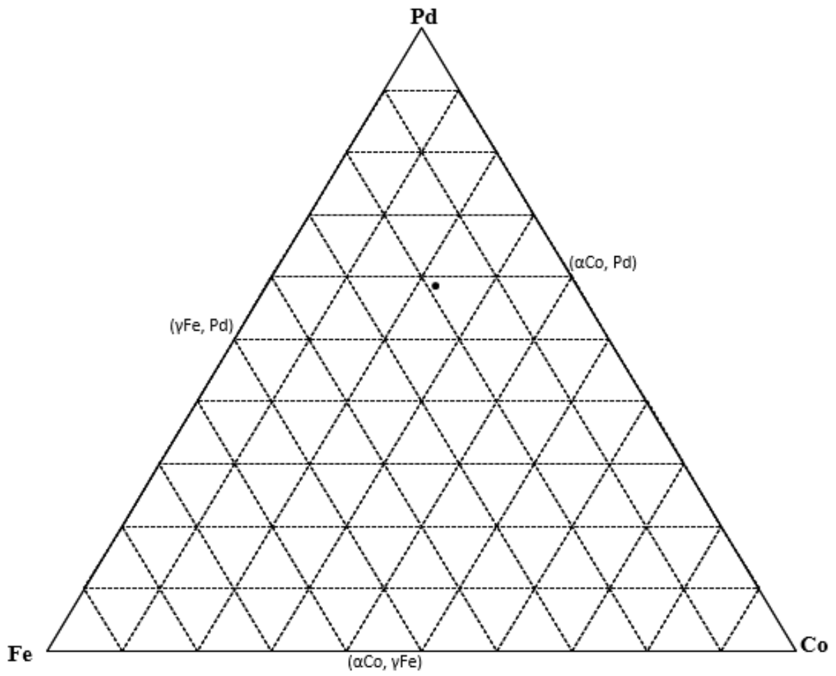
Figure 4.59. EDX analyses of nominal \text{Co}_{25}\text{Fe}_{20}\text{Pd}_{55} (at.%), Alloy 8 1000°C annealed condition. (■ Overall composition; ● phases)
