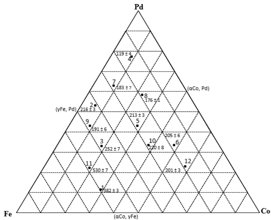
Figure 5.2. Ternary plot with microhardness values and errors for alloys annealed at 1000°C. (■ Overall composition)
