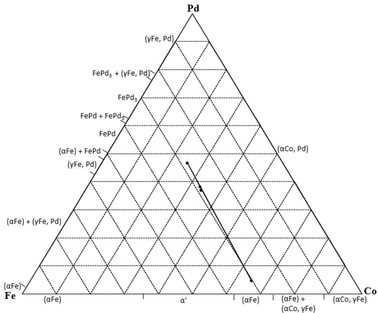
Figure 4.101. EDX analyses of nominal \text{Co}_{40}\text{:Fe}_{30}\text{:Pd}_{30} (at.%), Alloy 10 650°C annealed condition. (■ Overall composition; ● phases)
