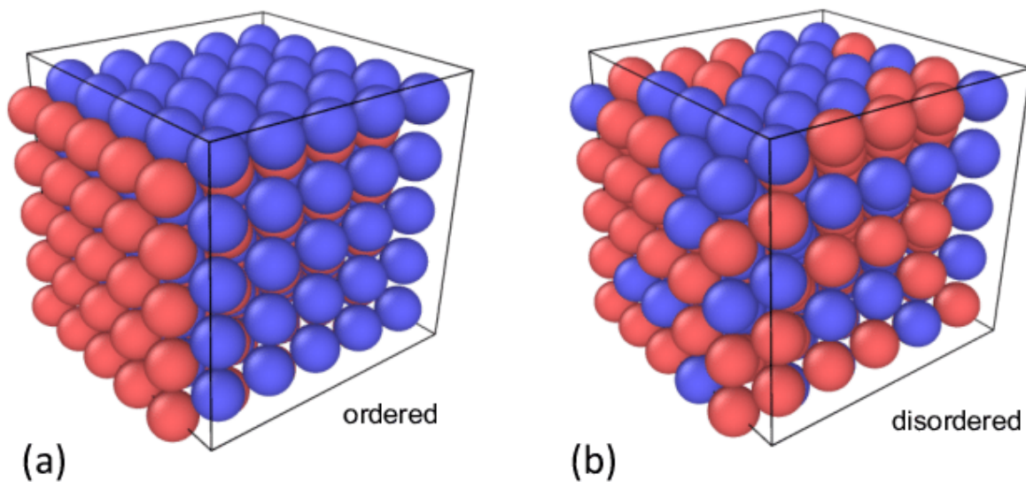
Figure 2.2. Schematic representation of the ordered and disordered \alpha' phase [2018Pei].
