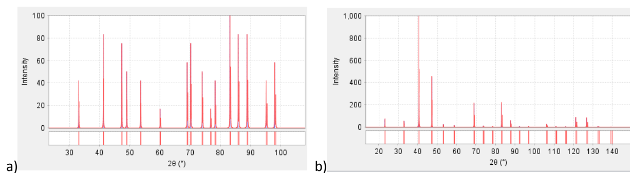
Figure 1. XRD peaks used to identify a) FePd and b) FePd 3 [2018Dif].
