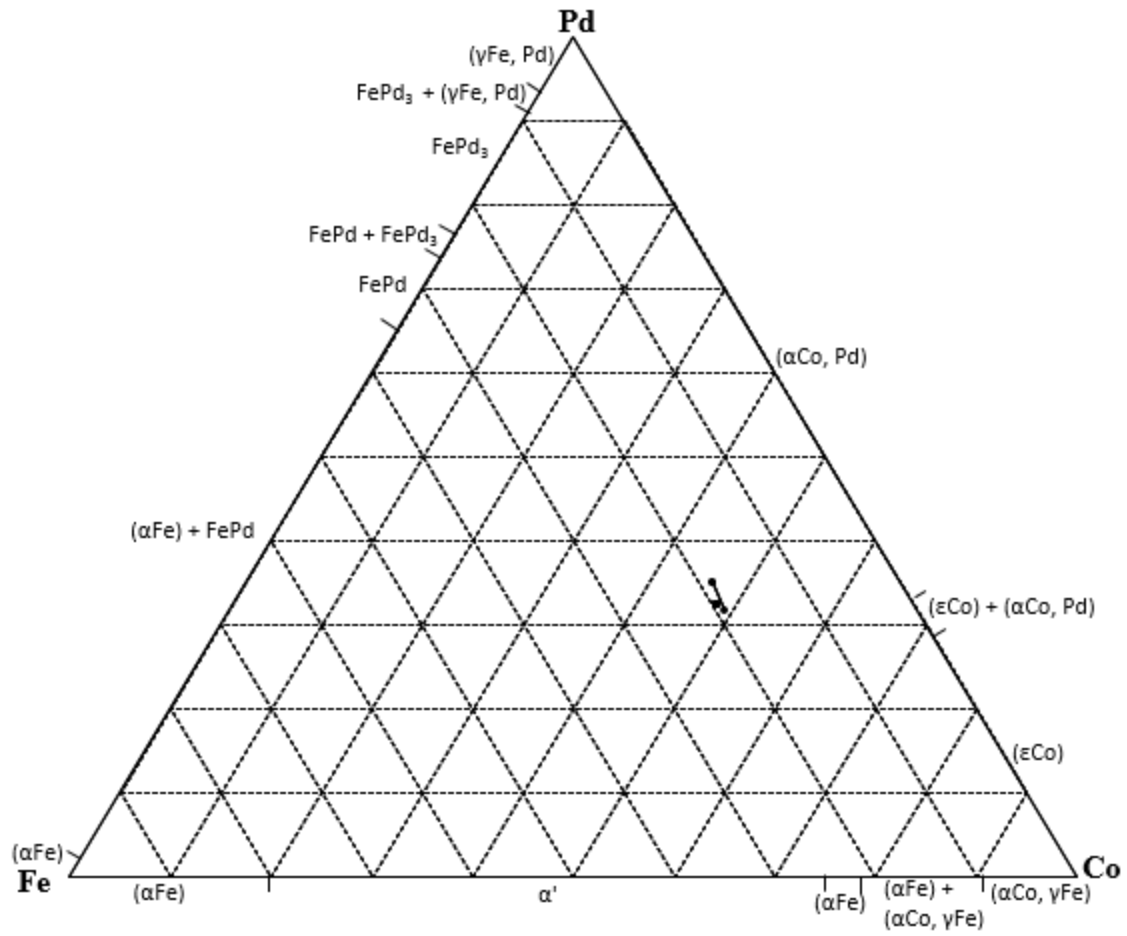
Figure 4.17. EDX analyses of nominal \text{Co}_{50}\text{Fe}_{20}\text{Pd}_{30} (at.%), Alloy 6 as-cast condition. (■ Overall composition; ● phases)
