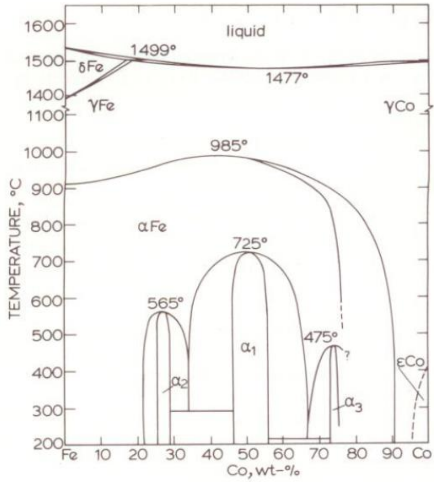
Figure 2.8. Co-Fe binary system previously accepted [1988Ray].
