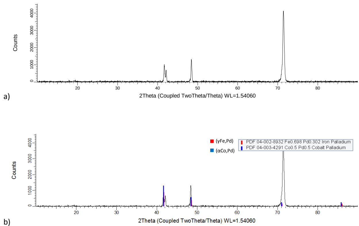
Figure 4.9. XRD patterns for nominal \text{Co}_{20}\text{:Fe}_{50}\text{:Pd}_{30} (at.%), Alloy 3 as-cast condition: a) raw, and b) labelled.
