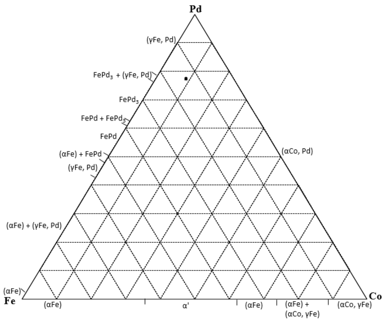
Figure 4.83. EDX analyses of nominal \text{Co}_{10}\text{:Fe}_{15}\text{:Pd}_{75} (at.%), Alloy 4 650°C annealed condition. (■ Overall composition; ● phases).
