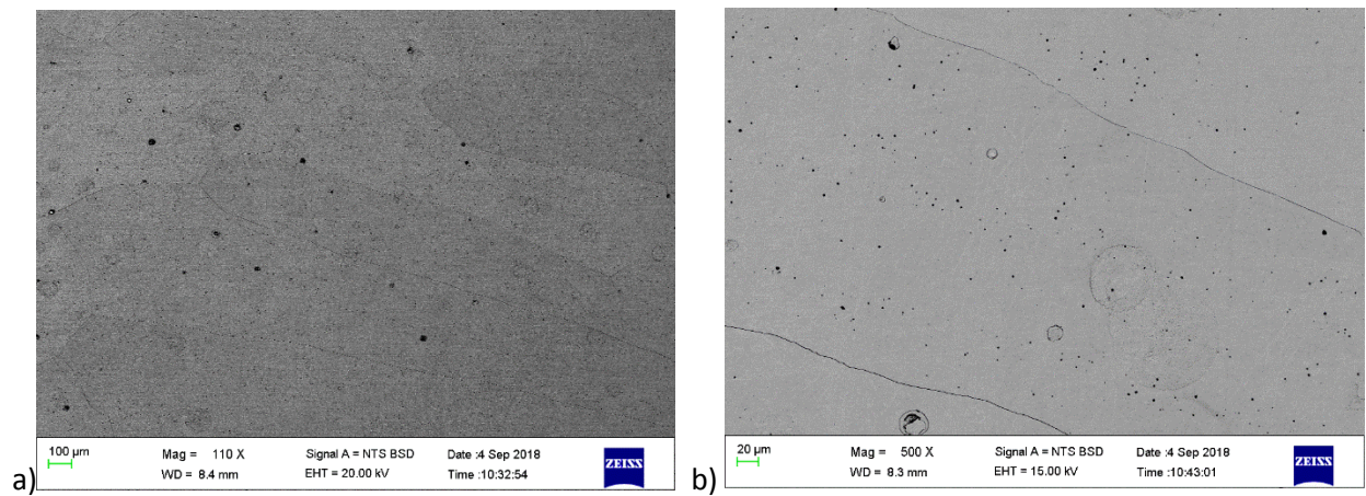
Figure 4.46. SEM-BSE images of \text{Co}_{10}\text{:Fe}_{15}\text{:Pd}_{75} (at.%), Alloy 4 annealed at 1000^{\circ}\text{C} for 1000 h showing: a) grains of different contrast, and b) grain boundaries, \sim\text{FePd}_3 precipitates and a region of different composition.
