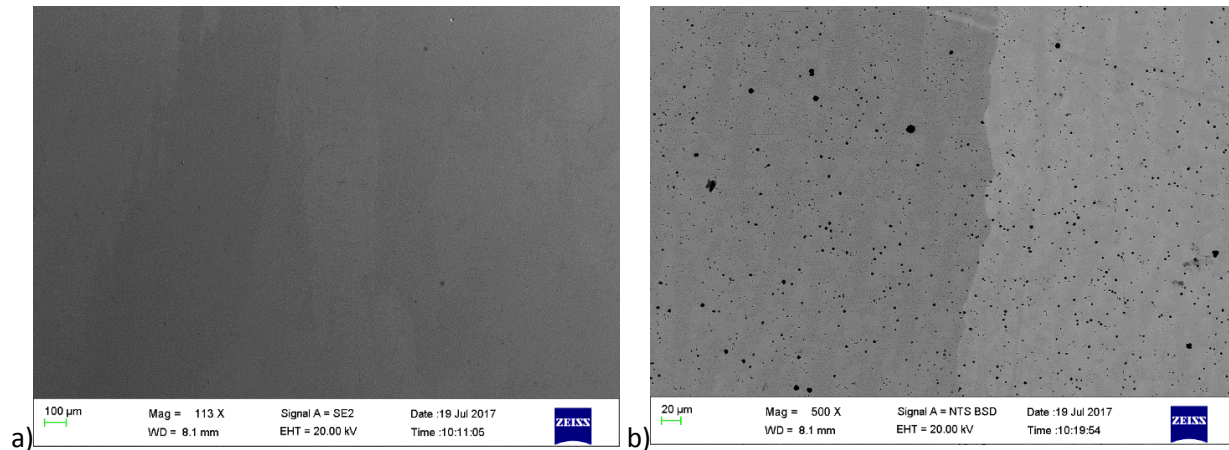
Figure 4.7. a) SEM-SE, and b) SEM-BSE images of as-cast \text{Co}_{20}\text{Fe}_{50}\text{Pd}_{30} (at.%), Alloy 3 showing grains and different contrasts.
