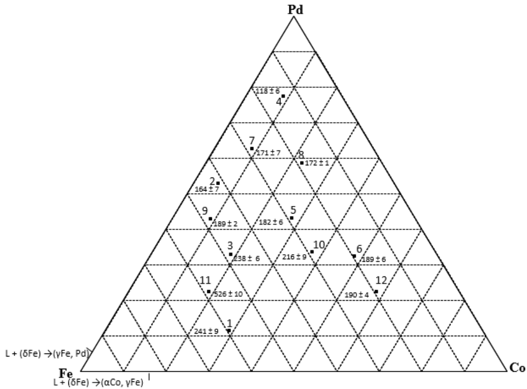
Figure 6.6. Solidification projection with hardnesses for as-cast Co-Fe-Pd alloys. (■ Overall composition)
