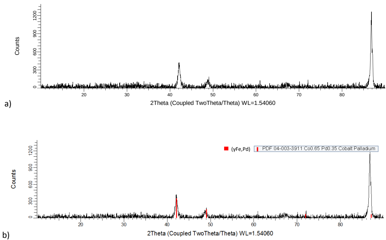
Figure 4.66. XRD patterns for nominal \text{Co}_{40}\text{:Fe}_{30}\text{:Pd}_{30} (at.%), Alloy 10 1000°C annealed condition: a) raw, and b) labelled.
