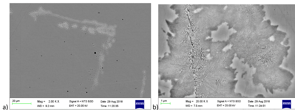
Figure 4.43. SEM-BSE images of \text{Co}_{20}\text{Fe}_{50}\text{Pd}_{30} (at.%), Alloy 3 annealed at 1000^{\circ}\text{C} for 1000 h showing: a) an etched area, and b) two-phase area at higher magnification.
