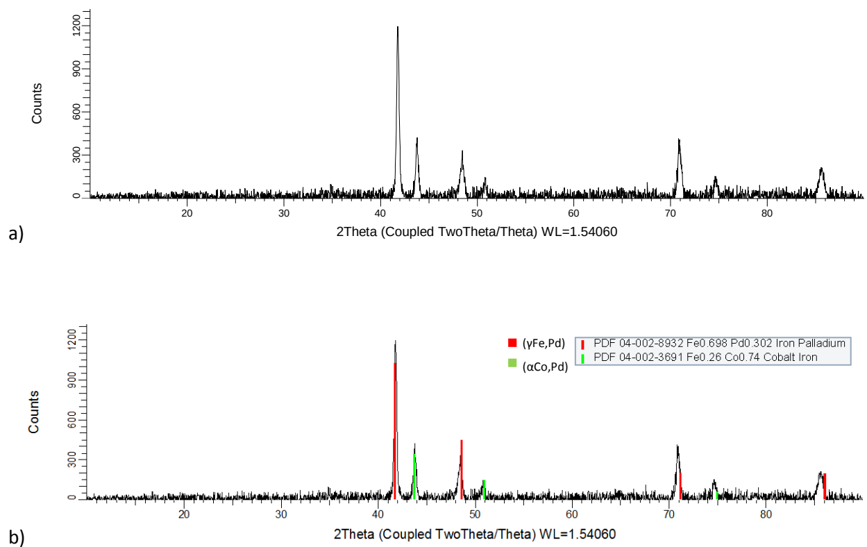
Figure 4.90. XRD patterns for nominal \text{Co}_{50}\text{:Fe}_{20}\text{:Pd}_{30} (at.%), Alloy 6 650°C annealed condition: a) raw, and b) labelled.
