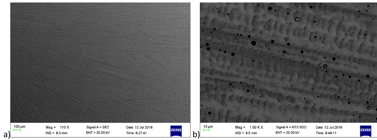
Figure 4.34. SEM-BSE images of as-cast \text{Co}_{60}\text{Fe}_{20}\text{Pd}_{20} (at.%), Alloy 12 showing dendrites surrounded by a lighter grey phase and porosity.
