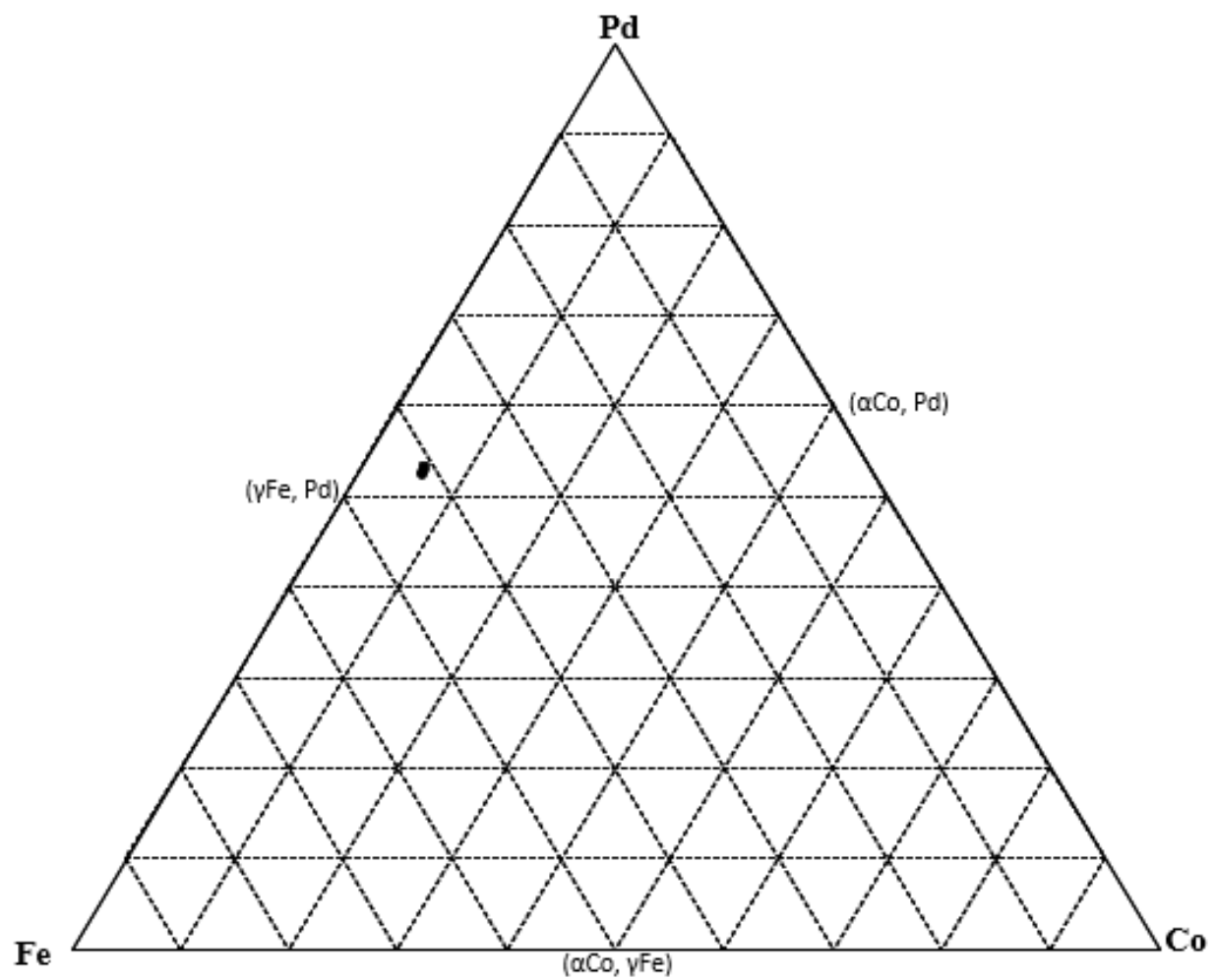
Figure 4.41. EDX analyses of nominal \text{Co}_6\text{:Fe}_{44}\text{:Pd}_{50} (at.%), Alloy 2 1000°C annealed condition. (■ Overall composition; ● phases)
