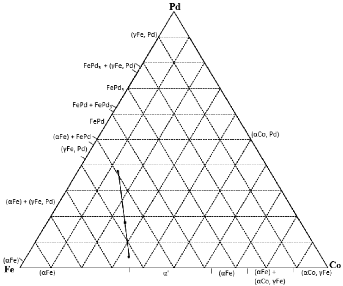
Figure 4.74. EDX analyses of nominal \text{Co}_{30}\text{Fe}_{60}\text{Pd}_{10} (at.%), Alloy 1 650°C annealed condition. (■ Overall composition; ● phases)
