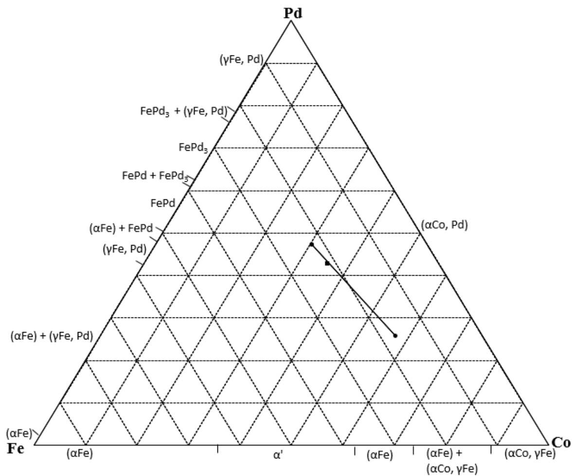
Figure 4.89. EDX analyses of nominal \text{Co}_{50}\text{:Fe}_{20}\text{:Pd}_{30} (at.%), Alloy 6 650°C annealed condition. (■ Overall composition; ● phases)
