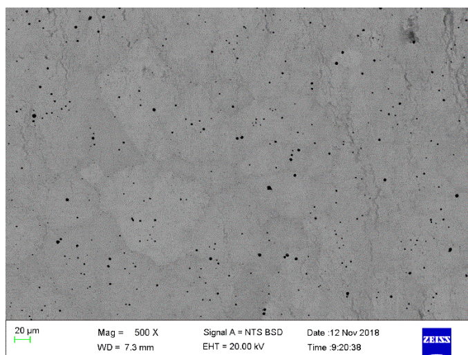
Figure 4.94. SEM-BSE image of \text{Co}_{25}\text{Fe}_{20}\text{Pd}_{55} (at.%), Alloy 8 annealed at 650^{\circ}\text{C} for 1000 h showing coring.
