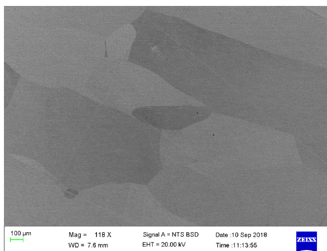
Figure 4.64. SEM-BSE image of \text{Co}_{40}\text{Fe}_{30}\text{Pd}_{30} (at.%), Alloy 10 annealed at 1000^\circ\text{C} for 1000 h showing contrasting grains.
