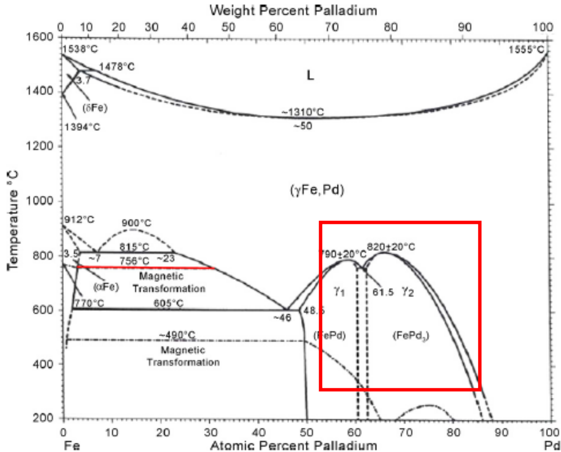
Figure 2.6. Binary diagram for Fe-Pd system [1990Mas].
