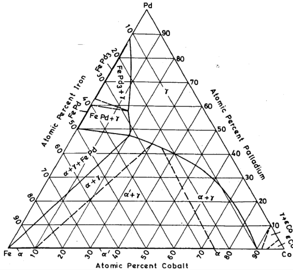
Figure 2.9. Co-Fe-Pd Isothermal section at ~25°C (at.%) [1992Rag].
