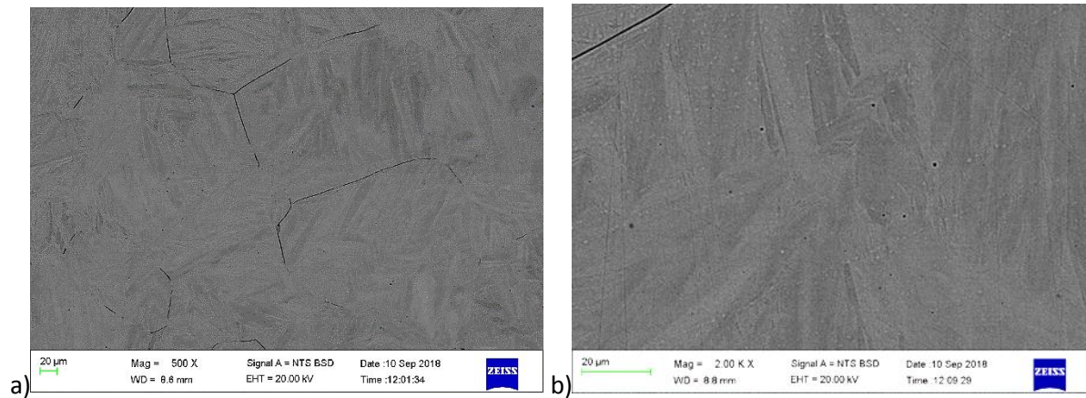
Figure 4.67. SEM-BSE images of \text{Co}_{20}\text{Fe}_{60}\text{Pd}_{20} (at.%), Alloy 11 annealed at 1000^\circ\text{C} for 1000 h showing: a) contrasting regions with grain boundaries) and b) fine precipitates.
