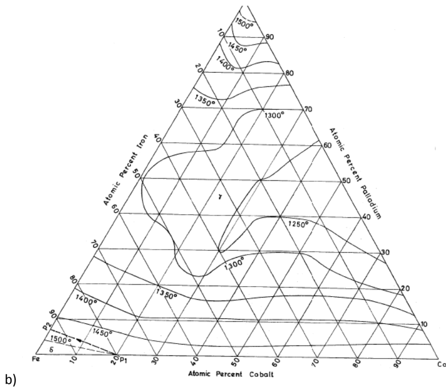
Figure 2.10. Liquidus surfaces of Co-Fe-Pd: a) Kuprina and Grigorev [1958Kup], and b) Raghavan [1992Rag].
