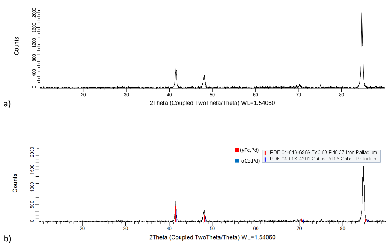
Figure 4.42. XRD patterns for nominal \text{Co}_6\text{:Fe}_{44}\text{:Pd}_{50} (at.%), Alloy 2 1000°C annealed condition: a) raw, and b) labelled.
