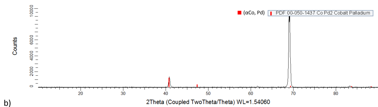
Figure 4.84. XRD patterns for nominal \text{Co}_{10}\text{:Fe}_{15}\text{:Pd}_{75} (at.%), Alloy 4 650^\circ\text{C} annealed condition: a) raw, and b) labelled.
