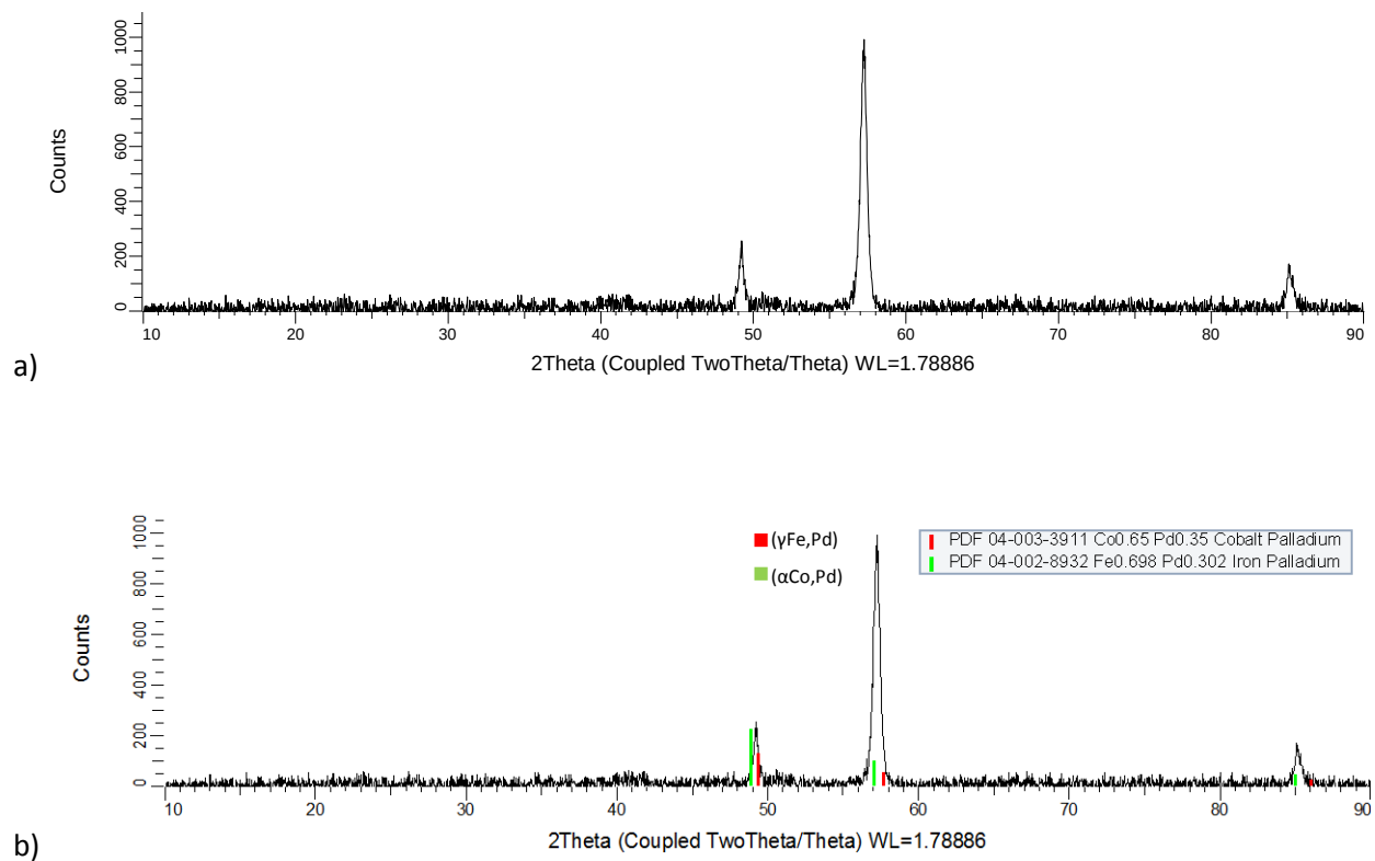
Figure 4.15. XRD patterns for nominal \text{Co}_{30}\text{:Fe}_{30}\text{:Pd}_{40} (at.%), Alloy 5 as-cast condition: a) raw, and b) labelled.
