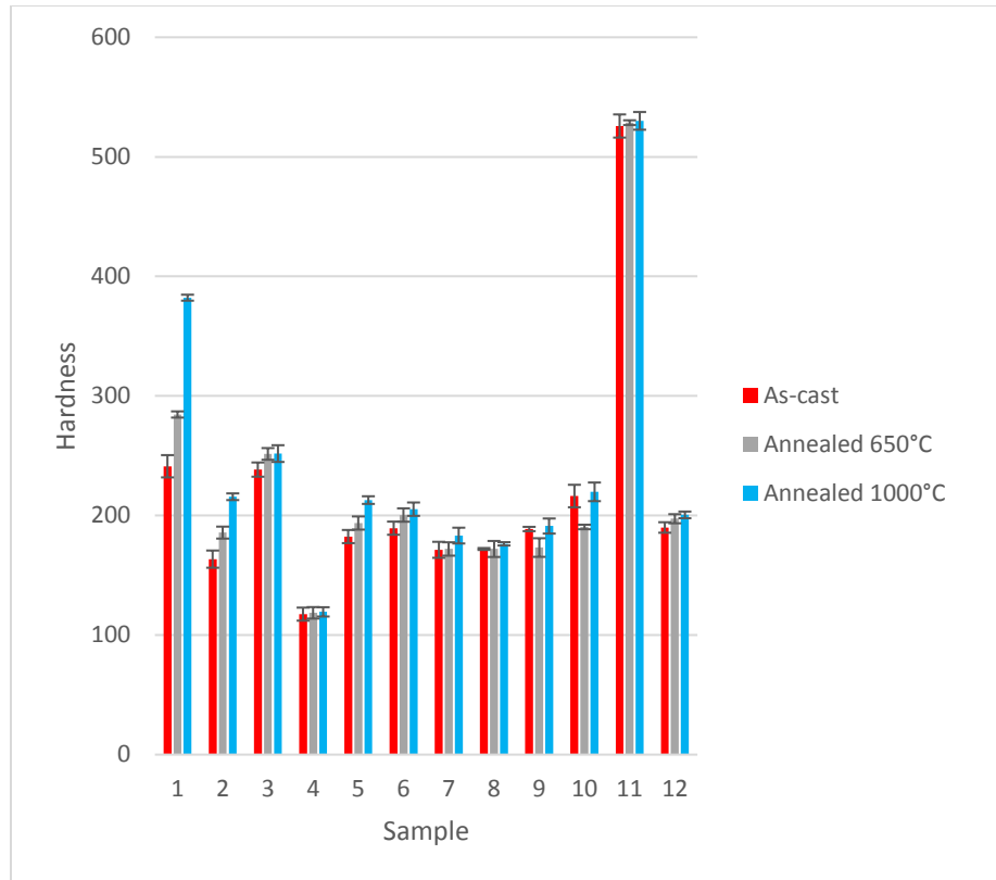
Figure 6.9. Comparison of hardnesses for all of the alloys in the different conditions.
