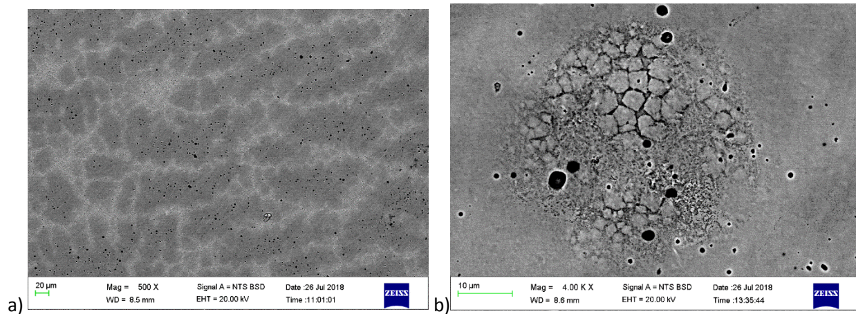
Figure 4.28. SEM-BSE images of as-cast \text{Co}_{40}\text{Fe}_{30}\text{Pd}_{30} (at.%), Alloy 10 showing: a) coring, and b) etched patch with particles surrounded by a matrix.
