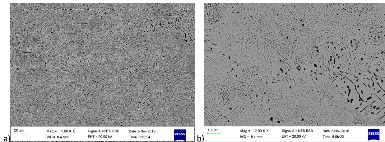
Figure 4.97. SEM-BSE images of \text{Co}_{10}\text{Fe}_{50}\text{Pd}_{40} (at.%), Alloy 9 annealed at 650^\circ\text{C} for 1000 h showing: a) fine microstructure and b) fine and coarse two-phase regions.
