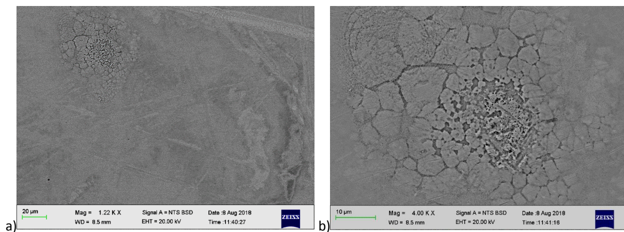
Figure 4.49. SEM-BSE images of Co 30 :Fe 30 :Pd 40 (at.%), Alloy 5 annealed at 1000°C for 1000 h showing: a) light and dark areas, and b) a magnified patch that was etched.
