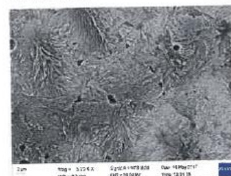
Figure 2. SEM-BSE image of as-cast Fe 50 Co 30 Pd 20 at.% showing decomposition of the dendrites.
