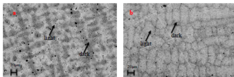
Figure 2. SEM-BSE images of as-cast a) Alloy1 \text{Fe}_{80}\text{Co}_{10}\text{Pd}_{10} (at.%) showing dendrites (darker) and b) Alloy 2 \text{Fe}_{15}\text{Co}_{10}\text{Pd}_{75} (at.%) showing gamma dendrites (lighter) and two phase interdendritic area (dark).
