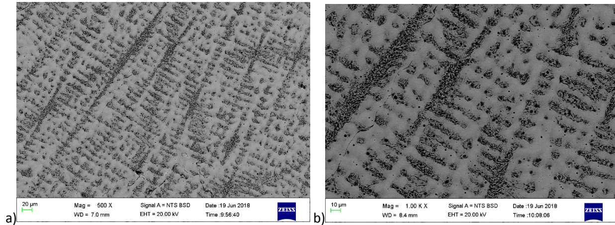
Figure 4.31. SEM-BSE images of as-cast \text{Co}_{20}\text{Fe}_{60}\text{Pd}_{20} (at.%), Alloy 11 showing the formation of dendrites surrounded by a matrix a) low magnification and b) higher magnification.
