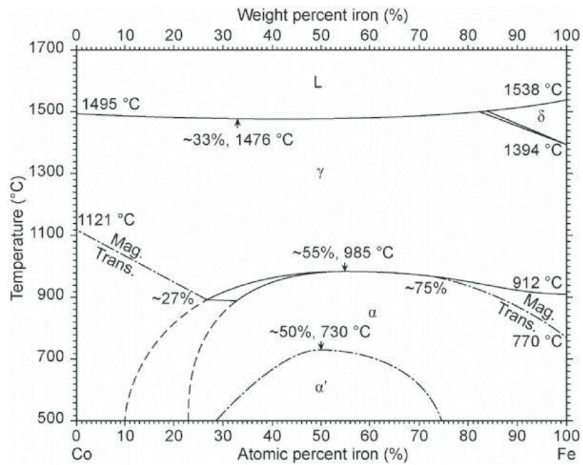
Figure 2. 4. Previously accepted Co-Fe phase diagram [1984Nis].
