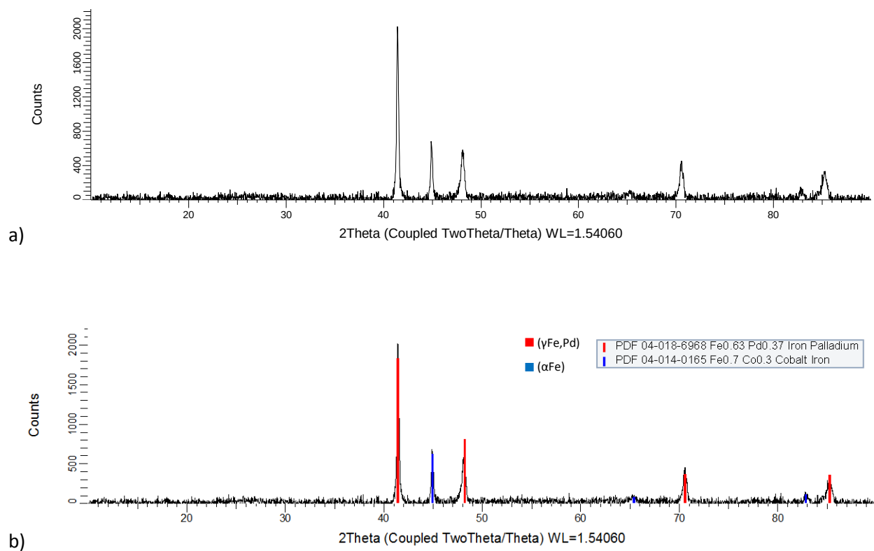
Figure 4.102. XRD patterns for nominal \text{Co}_{40}\text{:Fe}_{30}\text{:Pd}_{30} (at.%), Alloy 10 650°C annealed condition: a) raw, and b) labelled.
