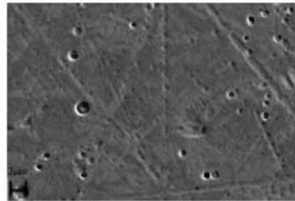
Figure 5. SEM-BSE image of as-cast Alloy 3 \text{Fe}_{30}\text{Co}_{30}\text{Pd}_{40} (at.%) showing a single phase with pores.
