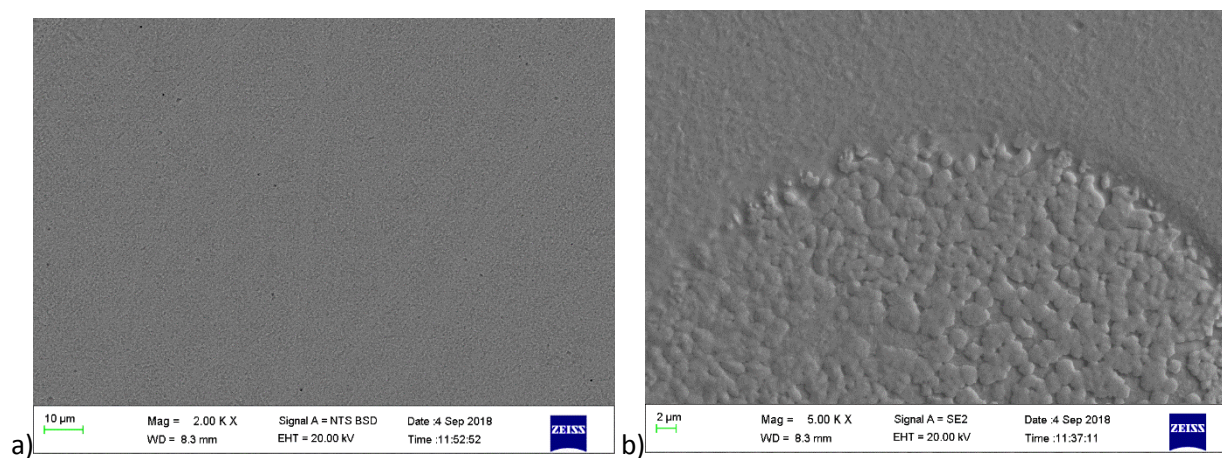
Figure 4. 58. SEM images of \text{Co}_{25}\text{Fe}_{20}\text{Pd}_{55} (at.%), Alloy 8 annealed at 1000^{\circ}\text{C} for 1000 h showing: a) BSE image at low magnification and b) SE image of a region at higher magnification.
