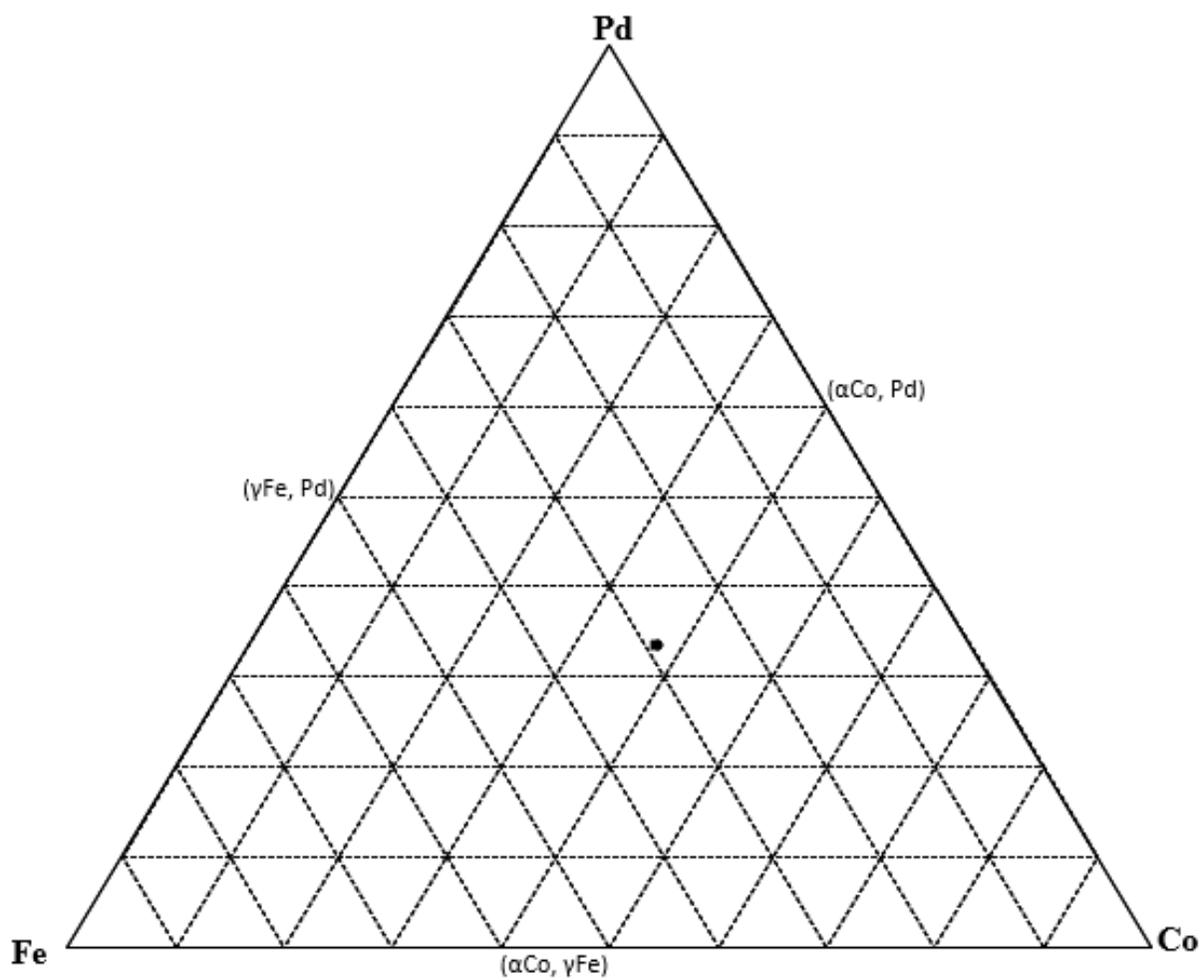
Figure 4.65. EDX analyses of nominal \text{Co}_{40}\text{Fe}_{30}\text{Pd}_{30} (at.%), Alloy 10 1000°C annealed condition. (■ Overall composition; ● phases)
