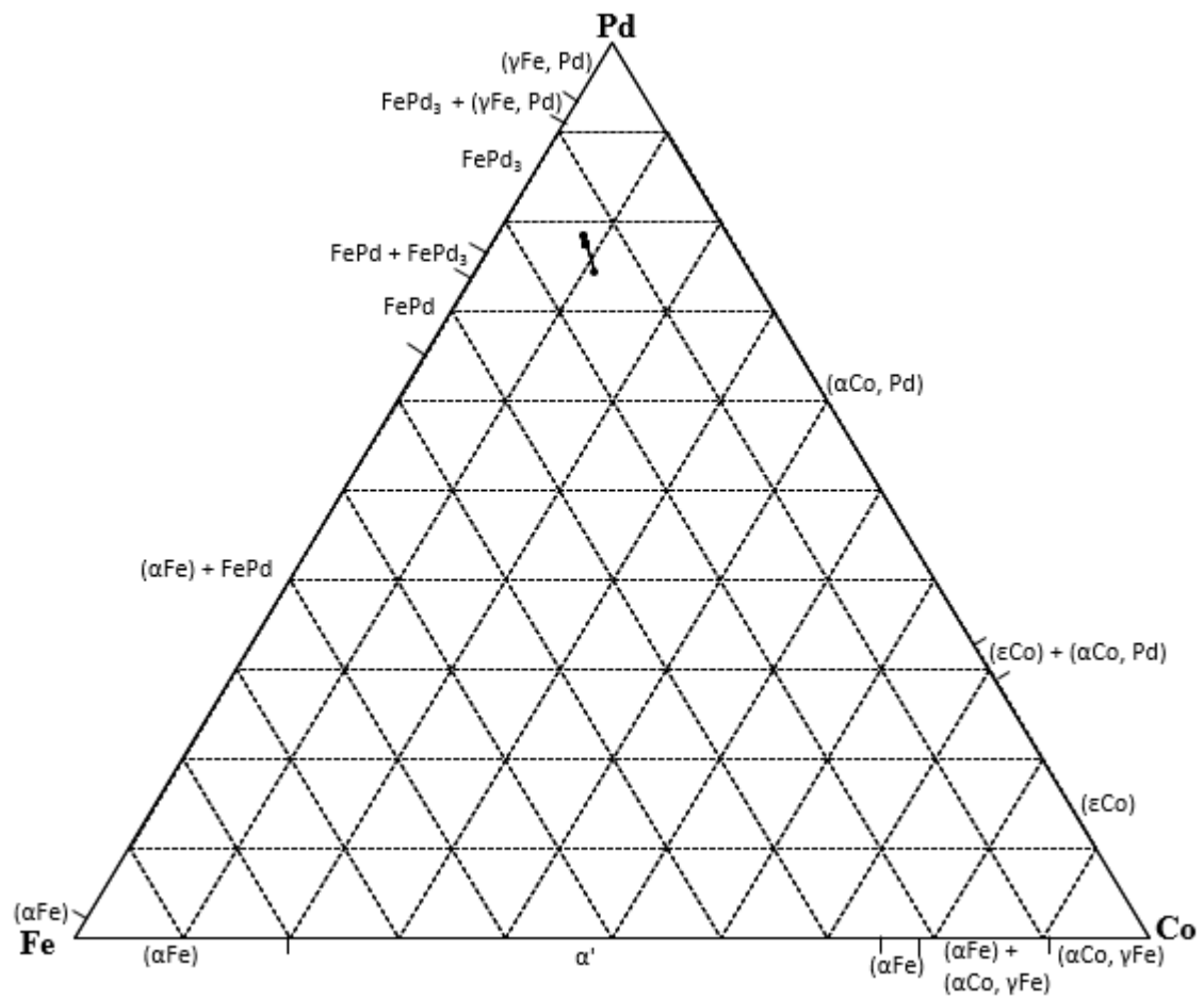
Figure 4.11. EDX analyses of nominal \text{Co}_{10}\text{Fe}_{15}\text{Pd}_{75} (at.%), Alloy 4 as-cast condition. (■ Overall composition; ● phases)
