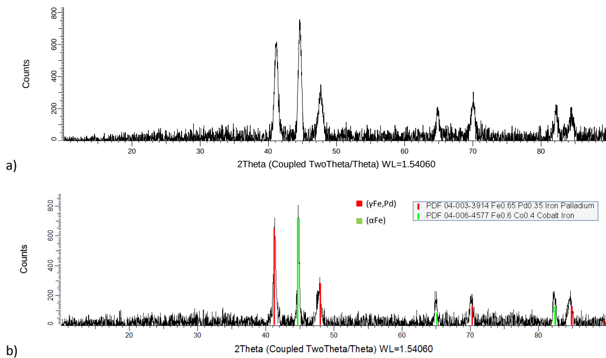
Figure 4.105. XRD patterns for nominal \text{Co}_{20}\text{:Fe}_{60}\text{:Pd}_{20} (at.%), Alloy 11 650°C annealed condition: a) raw, and b) labelled.
