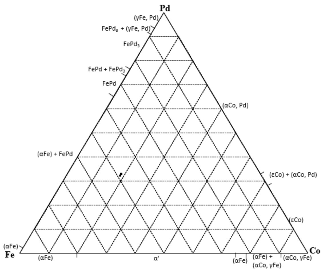
Figure 4.8. EDX analyses of nominal \text{Co}_{20}\text{:Fe}_{50}\text{:Pd}_{30} (at.%), Alloy 3 as-cast condition. (■ Overall composition; ● phases)
