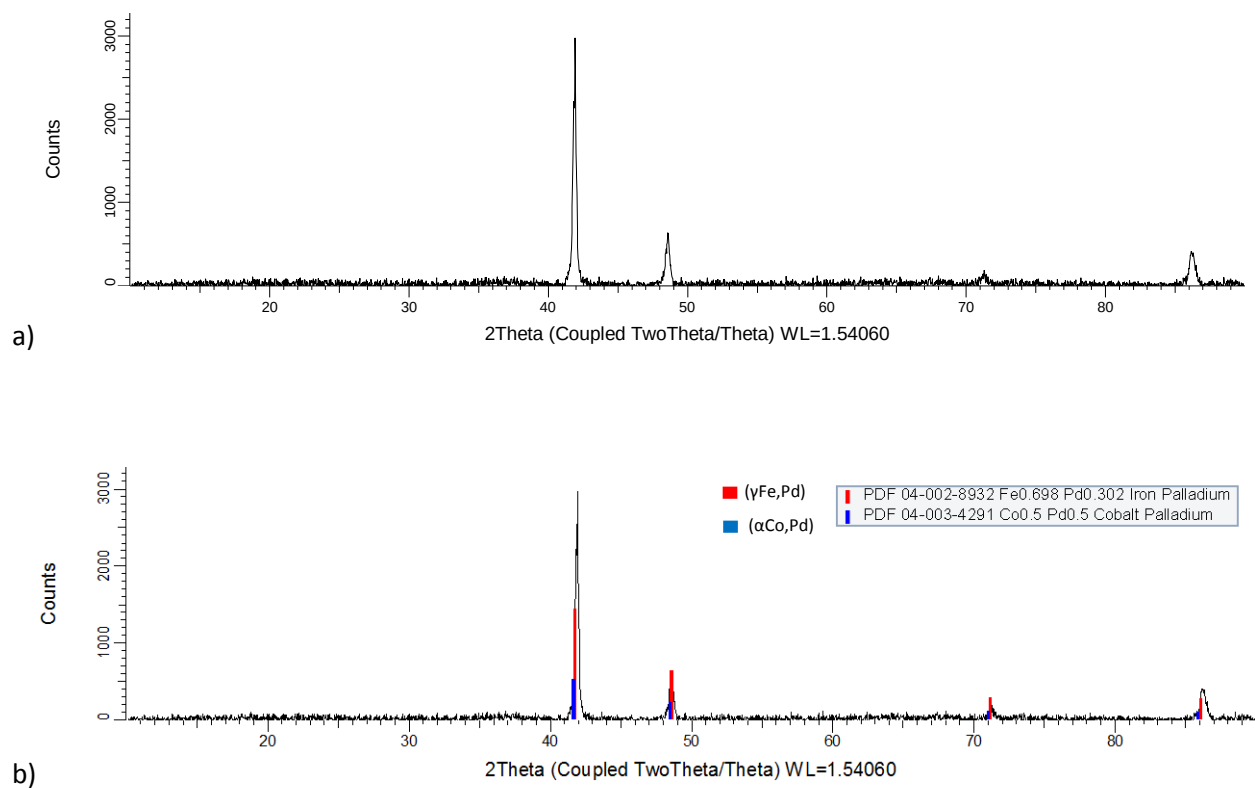
Figure 4.45. XRD patterns for nominal \text{Co}_{20}\text{:Fe}_{50}\text{:Pd}_{30} (at.%), Alloy 3 1000°C annealed condition: a) raw, and b) labelled.
