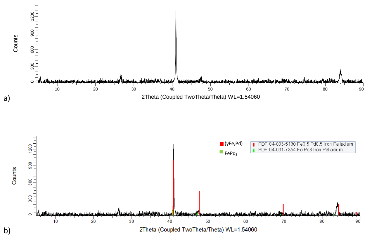
Figure 4.93. XRD patterns for nominal \text{Co}_{10}\text{:Fe}_{30}\text{:Pd}_{60} (at.%), Alloy 7 650°C annealed condition: a) raw, and b) labelled.
