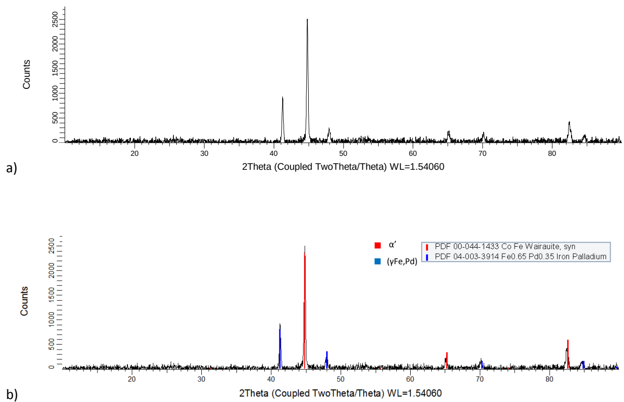
Figure 4.75. XRD patterns for nominal \text{Co}_{30}\text{:Fe}_{60}\text{:Pd}_{10} (at.%), Alloy 1 650°C annealed condition: a) raw, and b) labelled.
