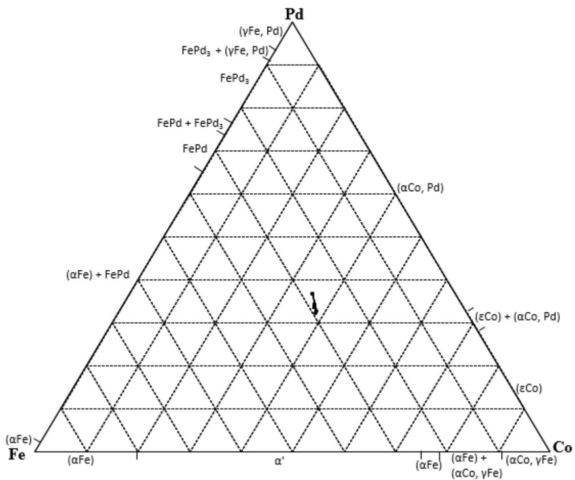
Figure 4.29. EDX analyses of nominal \text{Co}_{40}\text{Fe}_{30}\text{Pd}_{30} (at.%), Alloy 10 as-cast condition. (■ Overall composition; ● phases)
