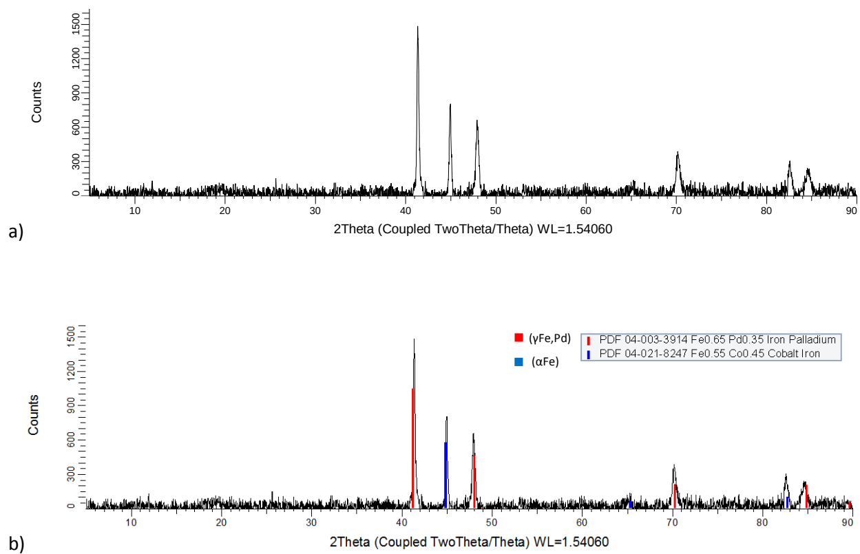
Figure 4.81. XRD patterns for nominal \text{Co}_{20}\text{:Fe}_{50}\text{:Pd}_{30} (at.%), Alloy 3 650°C annealed condition: a) raw, and b) labelled.
