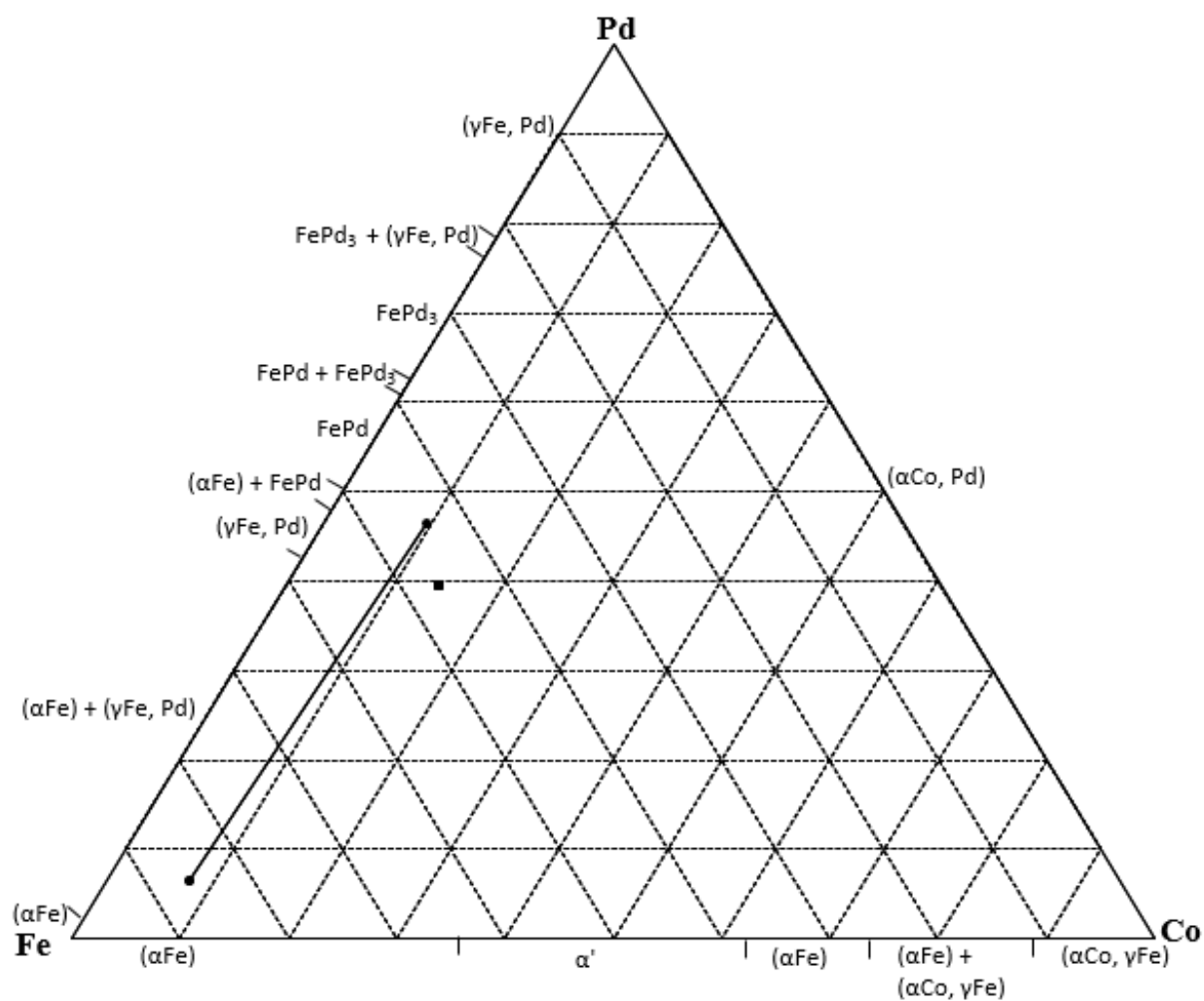
Figure 4.80. EDX analyses of nominal \text{Co}_{20}\text{Fe}_{50}\text{Pd}_{30} (at.%), Alloy 3 650°C annealed condition. (■ Overall composition; ● phases).
