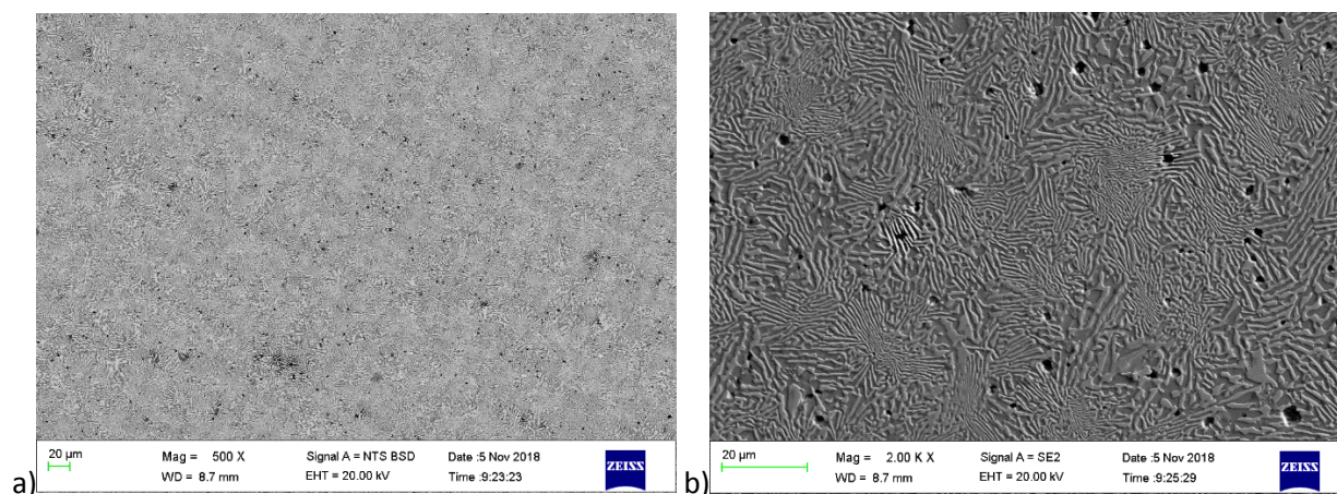
Figure 4.103. SEM images of \text{Co}_{20}\text{Fe}_{60}\text{Pd}_{20} (at.%), Alloy 11 annealed at 650^{\circ}\text{C} for 1000 h showing: a) BSE apparent dendrites and b) SE higher magnification fine phase.
