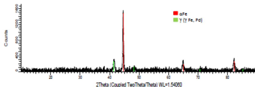
Figure 3. XRD pattern for Alloy 1 \text{Fe}_{80}\text{Co}_{10}\text{Pd}_{10} (at.%), as-cast condition.
