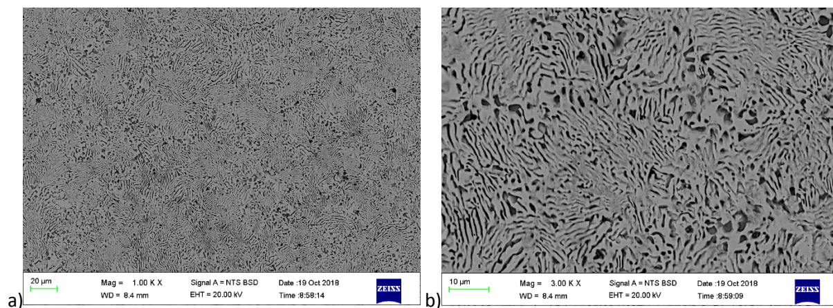
Figure 4.79. SEM-BSE images of \text{Co}_{20}\text{Fe}_{50}\text{Pd}_{30} (at.%), Alloy 3 annealed at 650^{\circ}\text{C} for 1000 h showing: a) the overall etched area, and b) higher magnification.
