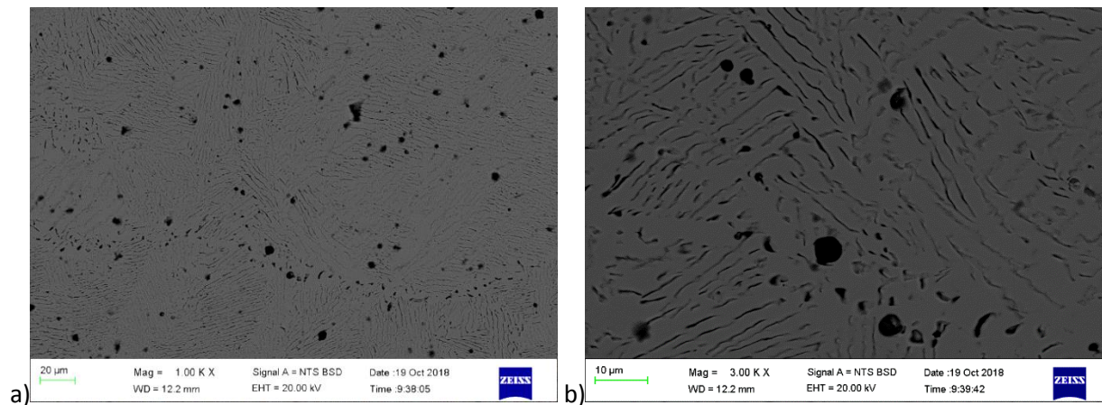
Figure 4.85. SEM-BSE images of \text{Co}_{30}\text{Fe}_{30}\text{Pd}_{40} (at.%), Alloy 5 annealed at 650^\circ\text{C} for 1000 h showing: a) representative area of the alloy, and b) magnified image.
