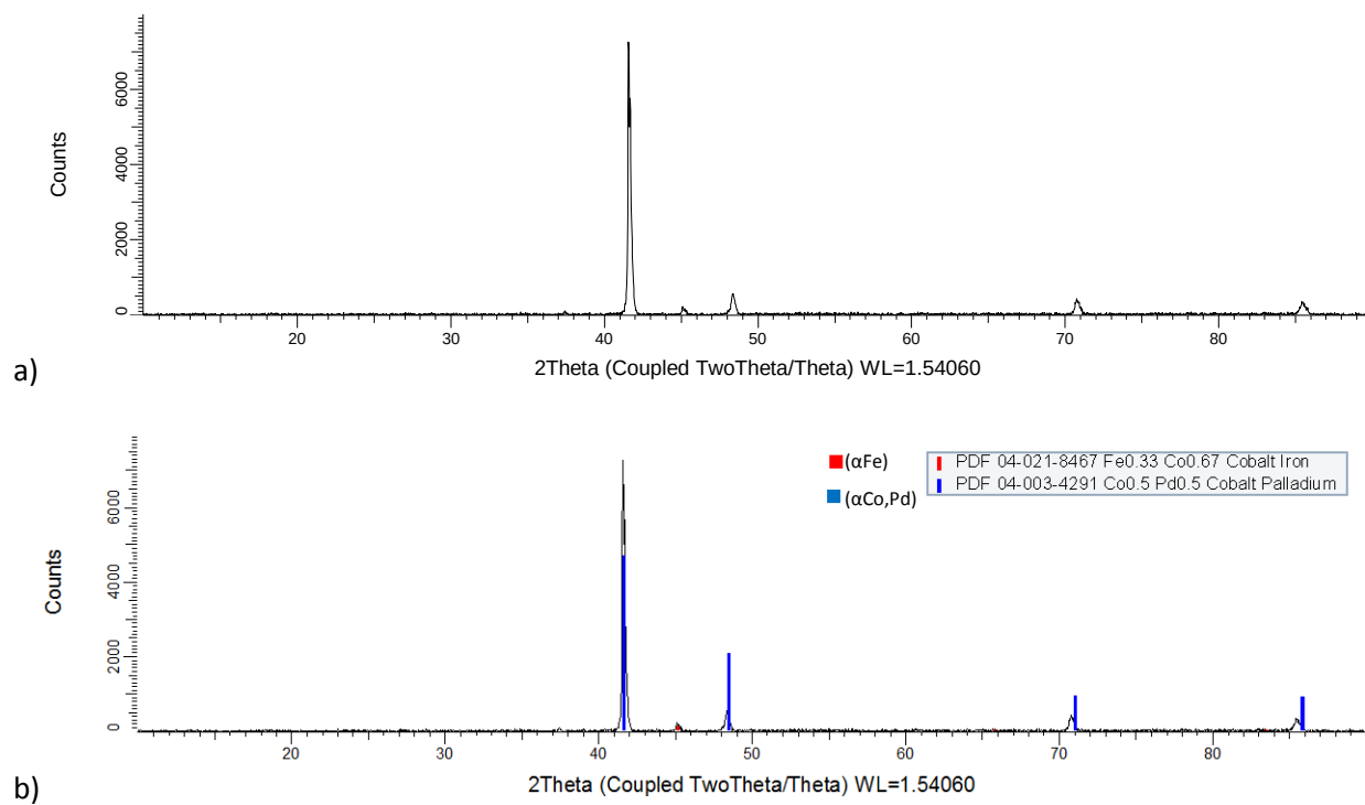
Figure 4.87. XRD patterns for nominal \text{Co}_{30}\text{:Fe}_{30}\text{:Pd}_{40} (at.%), Alloy 5 650°C annealed condition: a) raw, and b) labelled.
