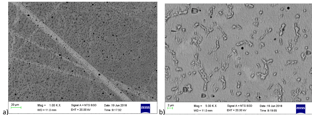
Figure 4.22. SEM-BSE images of as-cast \text{Co}_{25}\text{:Fe}_{20}\text{:Pd}_{55} (at.%), Alloy 8 showing: a) scratches surrounded by darker phase, and b) etched out particles surrounded by a light phase.
