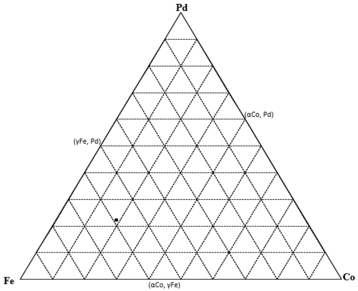
Figure 4.68. EDX analyses of nominal \text{Co}_{20}\text{Fe}_{60}\text{Pd}_{20} (at.%), Alloy 11 1000°C annealed condition. (■ Overall composition; ● phases)
