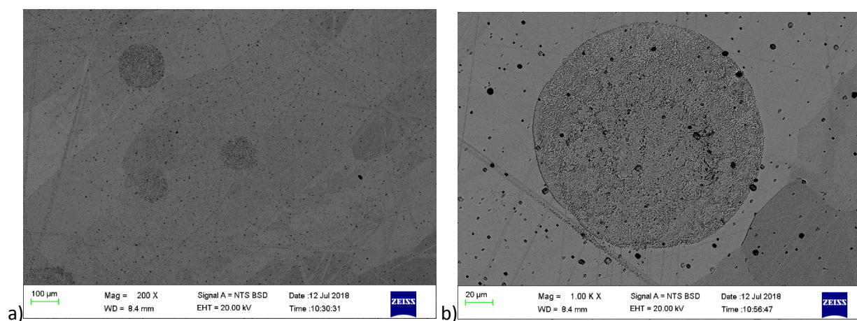
Figure 4.40. SEM-BSE images of \text{Co}_6\text{Fe}_{44}\text{Pd}_{50} (at.%), Alloy 2 annealed at 1000^\circ\text{C} for 1000 h showing: a) differently etched areas, and b) a better etched area at higher magnification.
