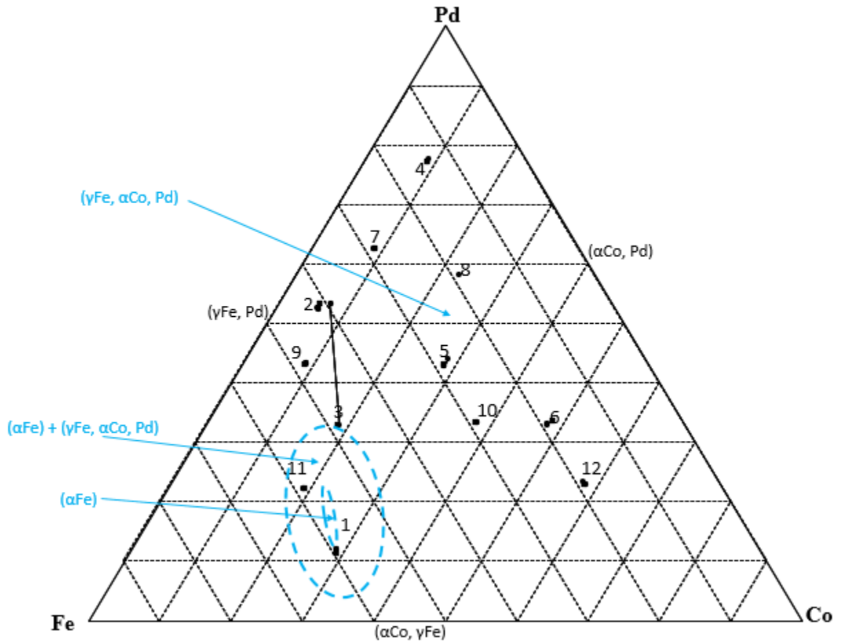
Figure 6.3. Isothermal section at 1000°C for the Co-Fe-Pd system (at.%). (■ Overall composition; ● phases)
