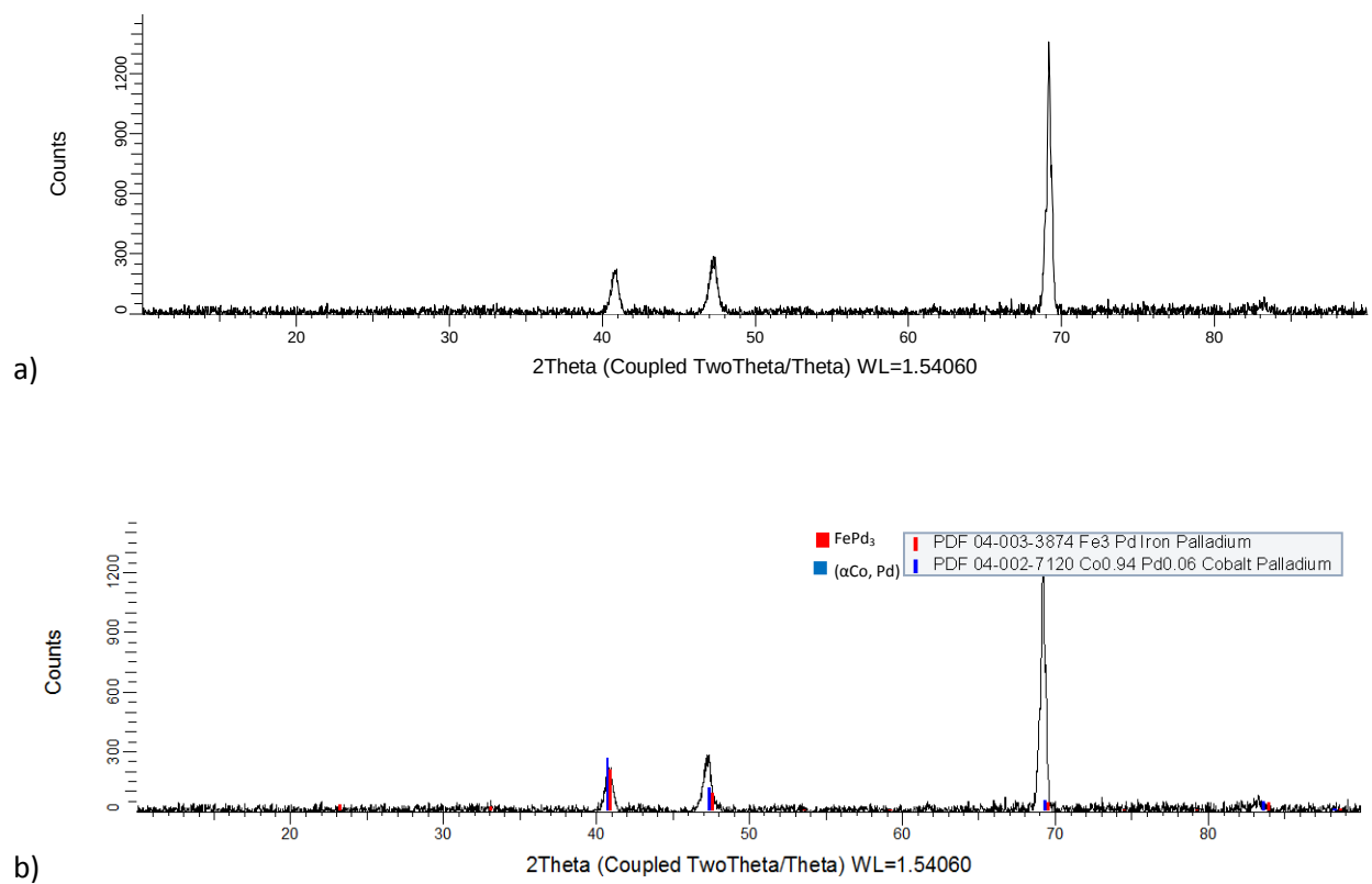
Figure 4.12. XRD patterns for nominal \text{Co}_{10}\text{:Fe}_{15}\text{:Pd}_{75} (at.%), Alloy 4 as-cast condition: a) raw, and b) labelled.
