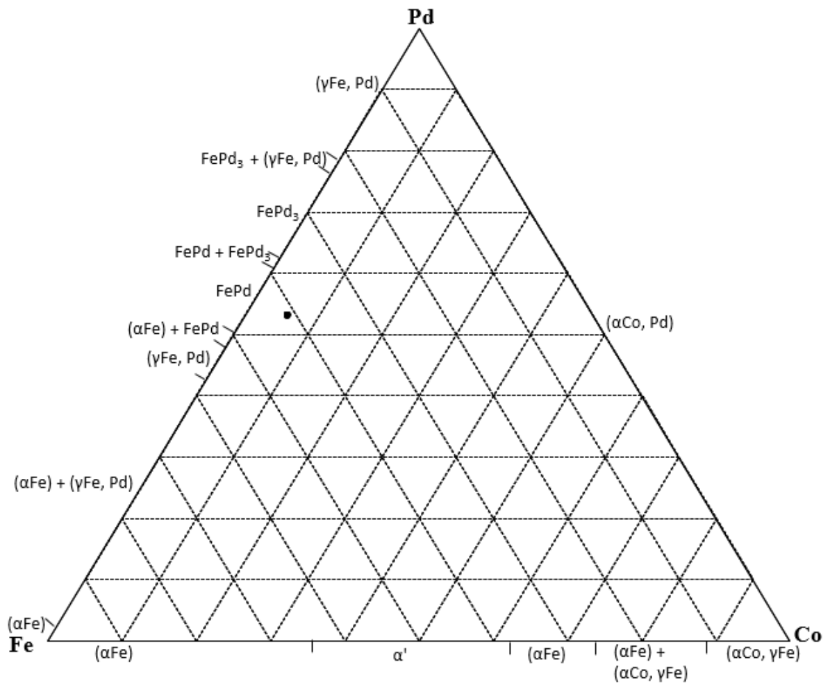
Figure 4.77. EDX analyses of nominal \text{Co}_{64}\text{Fe}_{44}\text{Pd}_{50} (at.%), Alloy 2 650°C annealed condition. (■ Overall composition; ● phases)
