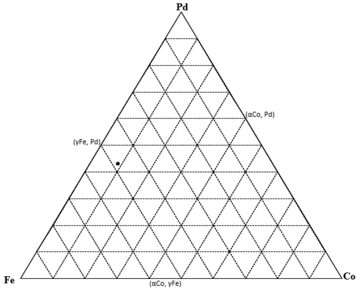
Figure 4.62. EDX analyses of nominal \text{Co}_{10}\text{Fe}_{50}\text{Pd}_{40} (at.%), Alloy 9 1000°C annealed condition. (■ Overall composition; ● phases)
