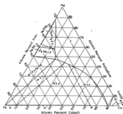
Figure 1. Co-Fe-Pd Isothermal section at ~25°C (at.%) [14].
