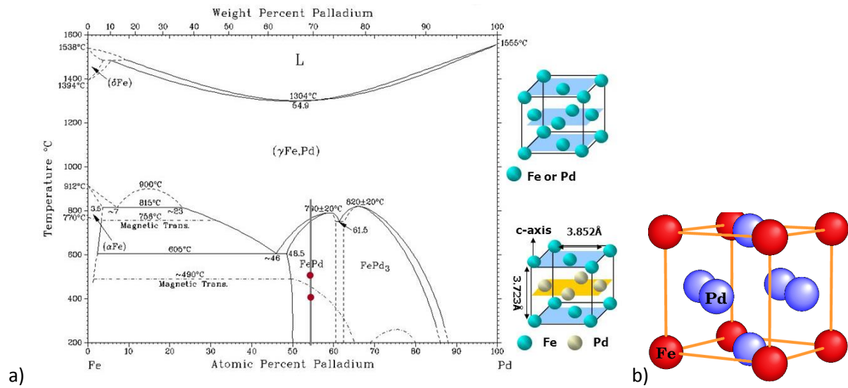
Figure 2.1. a) Fe-Pd binary diagram with disordered and ordered FePd phase structure [2018Lau] and b) schematic representation of ordered FePd 3 ordered alloy [2012Kva].
