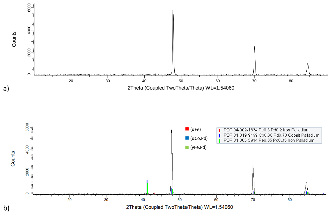
Figure 4.96. XRD patterns for nominal \text{Co}_{25}\text{:Fe}_{20}\text{:Pd}_{55} (at.%), Alloy 8 650°C annealed condition: a) raw, and b) labelled.
