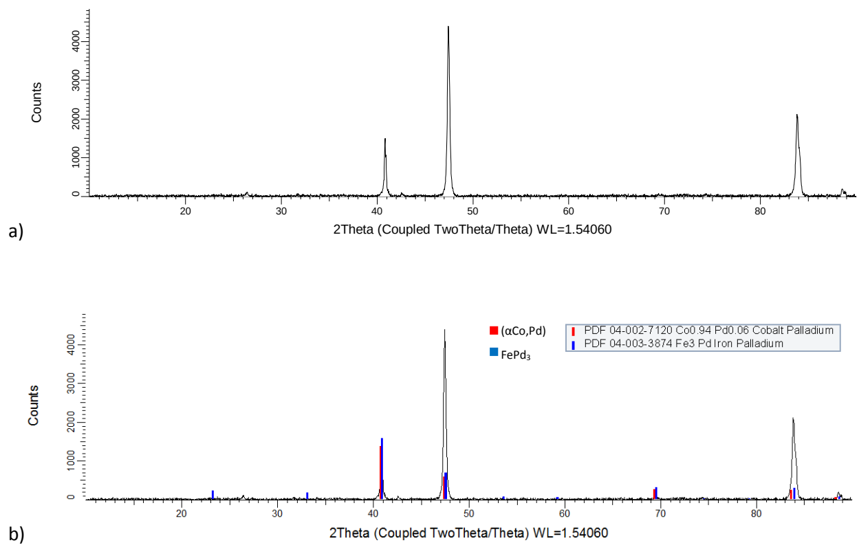
Figure 4.21. XRD patterns for nominal \text{Co}_{10}\text{:Fe}_{30}\text{:Pd}_{60} (at.%), Alloy 7 as-cast condition: a) raw, and b) labelled.
