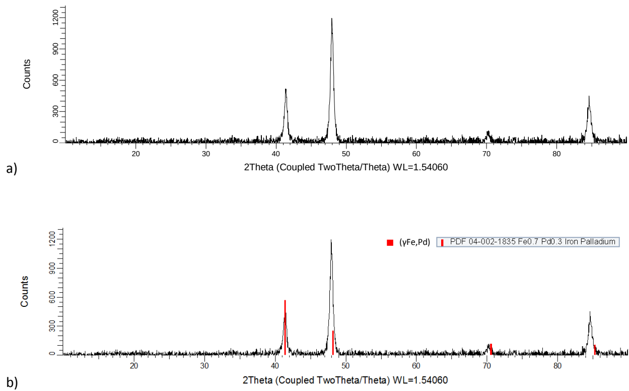
Figure 4.60. XRD patterns for nominal \text{Co}_{25}\text{:Fe}_{20}\text{:Pd}_{55} (at.%), Alloy 8 1000°C annealed condition: a) raw, and b) labelled.
