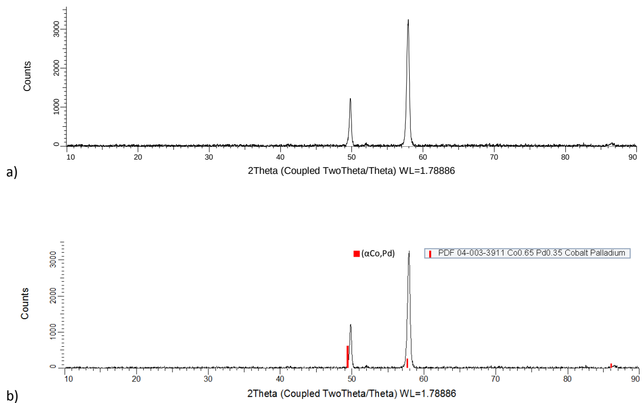
Figure 4.18. XRD patterns for nominal \text{Co}_{50}\text{:Fe}_{20}\text{:Pd}_{30} (at.%), Alloy 6 as-cast condition: a) raw, and b) labelled.
