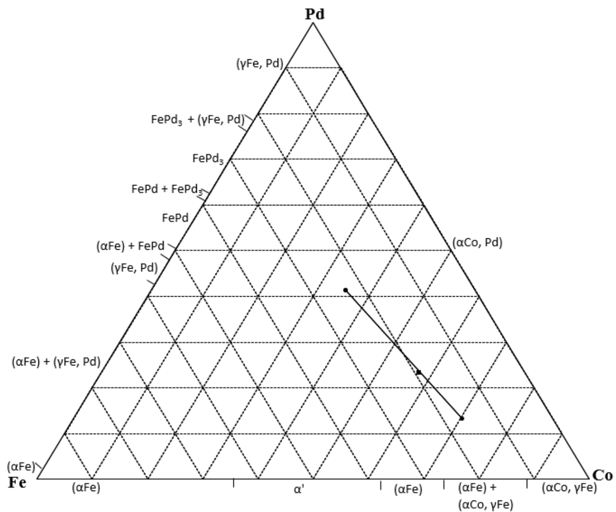
Figure 4.107. EDX analyses of nominal \text{Co}_{60}\text{:Fe}_{20}\text{:Pd}_{20} (at.%), Alloy 12 650°C annealed condition. (■ Overall composition; ● phases)
