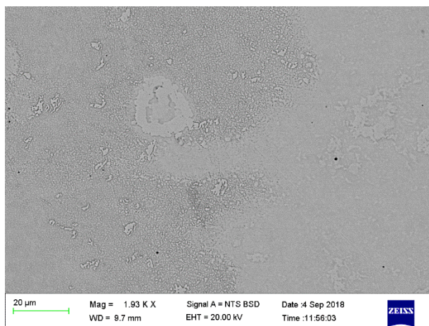
Figure 4.61. SEM-BSE image of \text{Co}_{10}\text{Fe}_{50}\text{Pd}_{40} (at.%), Alloy 9 annealed at 1000^{\circ}\text{C} for 1000 h showing differently etched lighter grey particles.
