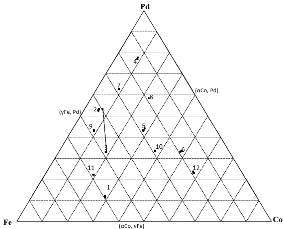
Figure 6.2. Results of the alloys annealed at 1000°C for the Co-Fe-Pd system (at.%). (■ Overall composition; ● phases)
