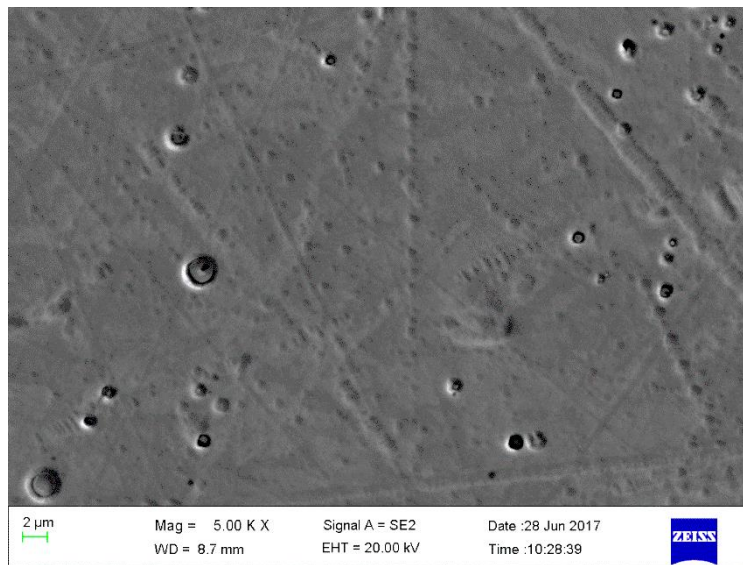
Figure 4.13. SEM-SE image of as-cast \text{Co}_{30}\text{Fe}_{30}\text{Pd}_{40} (at.%), Alloy 5 showing a single phase with pores.
