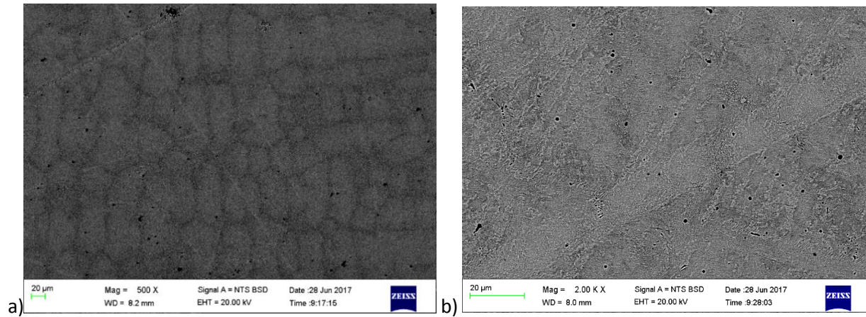
Figure 4.10. SEM-BSE images of as-cast Co 10 :Fe 15 :Pd 75 (at.%), Alloy 4 showing: a) dendrites (lighter), and interdendritic areas (dark) and b) higher magnification.
