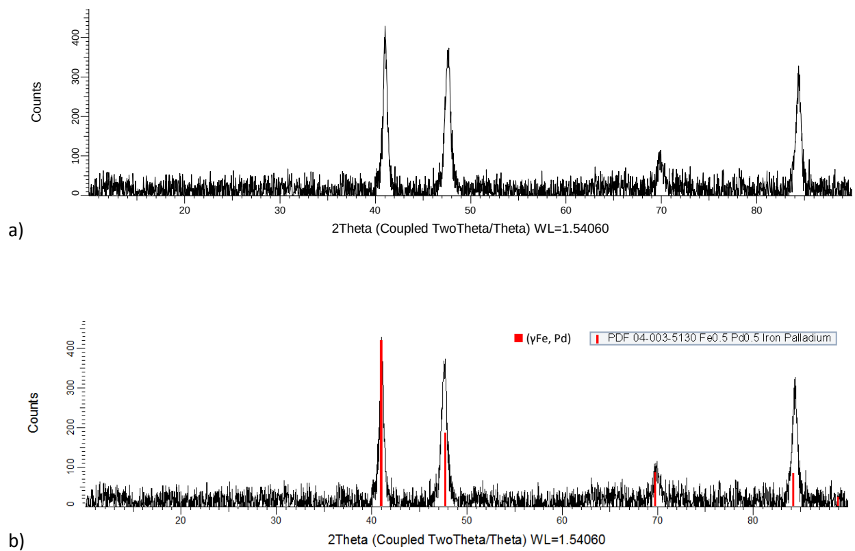
Figure 4.72. XRD patterns for nominal \text{Co}_{60}\text{:Fe}_{20}\text{:Pd}_{20} (at.%), Alloy 12 1000°C annealed condition: a) raw, and b) labelled.
