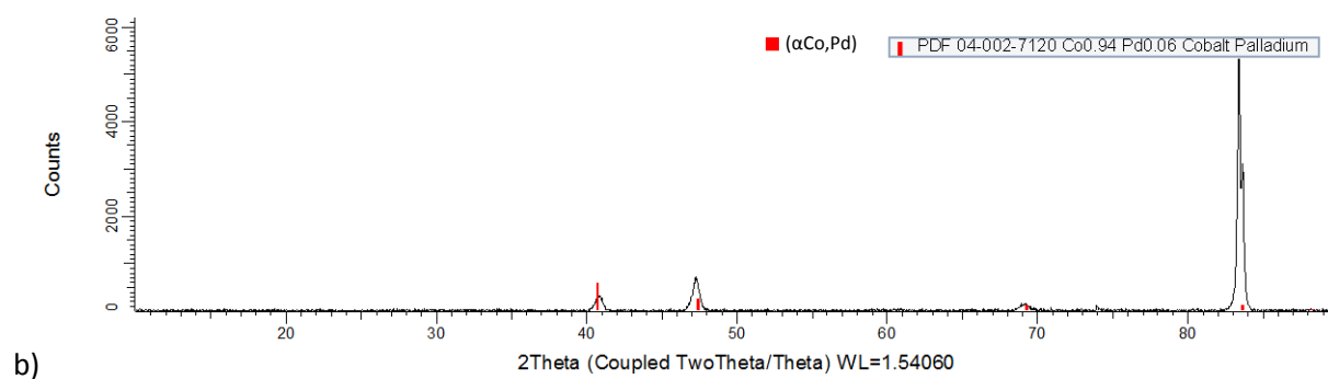
Figure 4.48. XRD patterns for nominal \text{Co}_{10}\text{:Fe}_{15}\text{:Pd}_{75} (at.%), Alloy 4 1000°C annealed condition: a) raw, and b) labelled.
