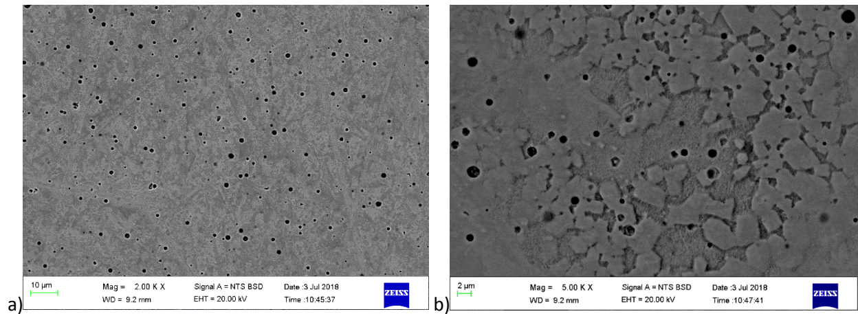
Figure 4.25. SEM-BSE images of as-cast Co 10 :Fe 50 :Pd 40 (at.%), Alloy 9 showing: a) the formation of a light phase surrounded by a dark phase, and b) a differently etched area with particles surrounded by a matrix.
