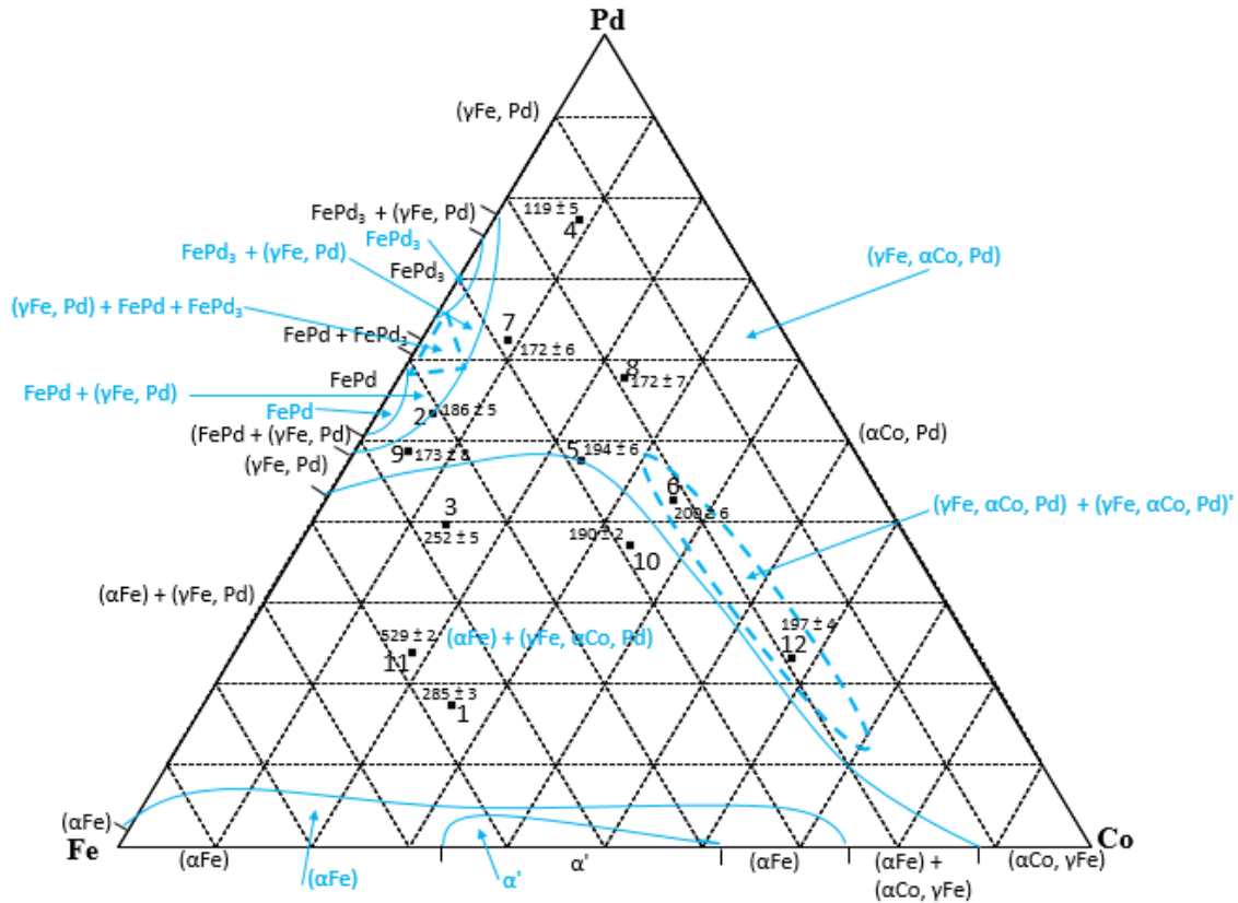
Figure 6.8. Isothermal section at 650°C for the Co-Fe-Pd system with hardnesses. (■ Overall composition)
