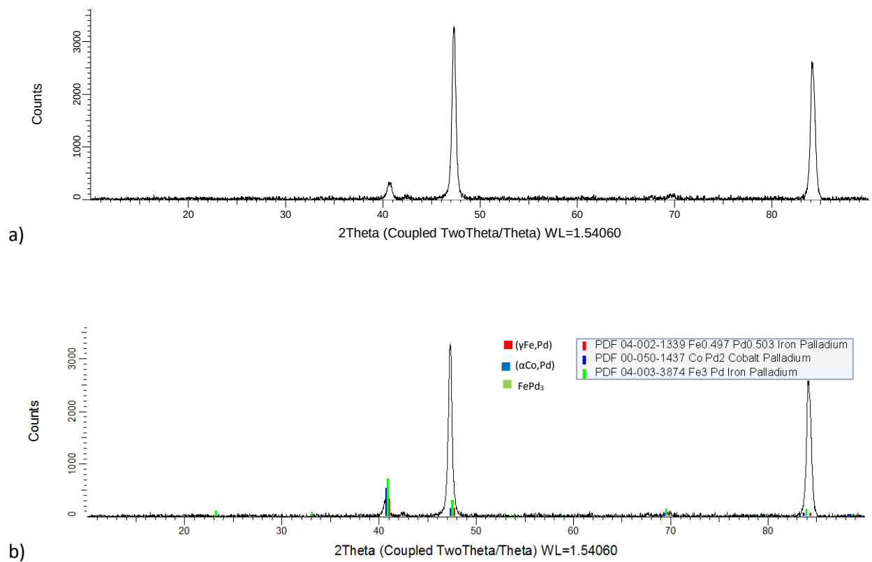
Figure 4.24. XRD patterns for nominal \text{Co}_{25}\text{:Fe}_{20}\text{:Pd}_{55} (at.%), Alloy 8 as-cast condition: a) raw, and b) labelled.
