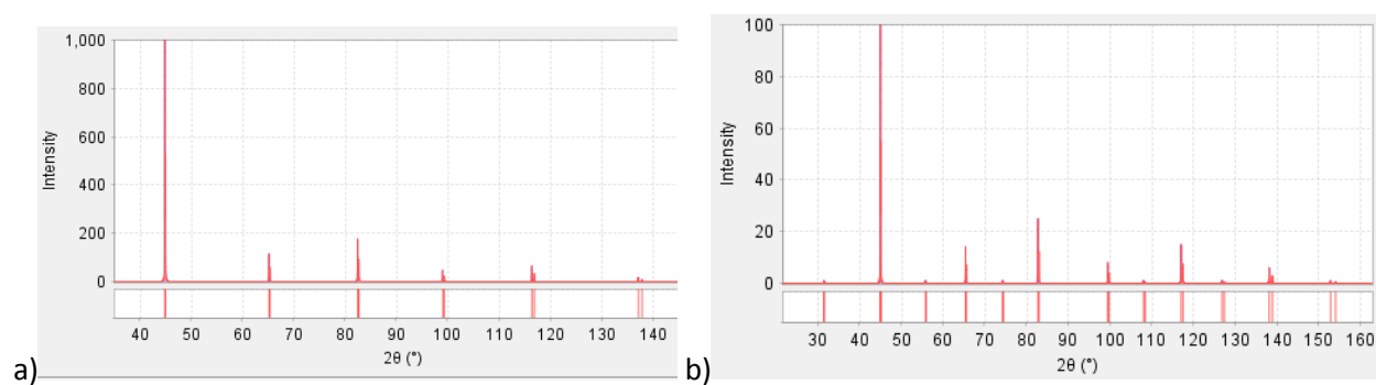
Figure 3. XRD peaks used to identify a) (αFe) and b) α' [2018Dif].
