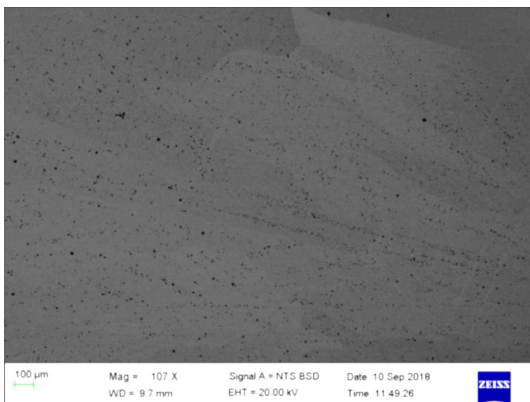
Figure 4.70. SEM-BSE image of \text{Co}_{60}\text{Fe}_{20}\text{Pd}_{20} (at.%), Alloy 12 annealed at 1000°C for 1000 h showing light and dark grains.
