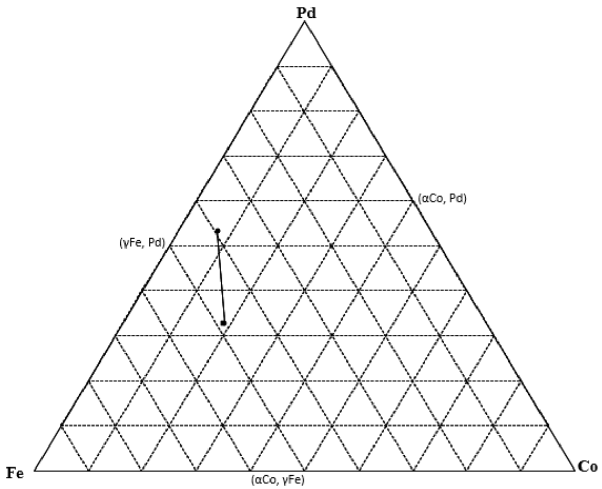
Figure 4.44. EDX analyses of nominal \text{Co}_{20}\text{Fe}_{50}\text{Pd}_{30} (at.%), Alloy 3 1000°C annealed condition. (■ Overall composition; ● phases)
