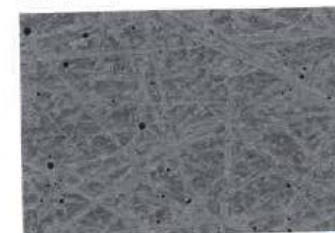
Figure 3. SEM-BSE image of as-cast Fe 50 Co 30 Pd 20 at.% showing needles (dark), peritectically-formed phase (light), with dark matrix.
