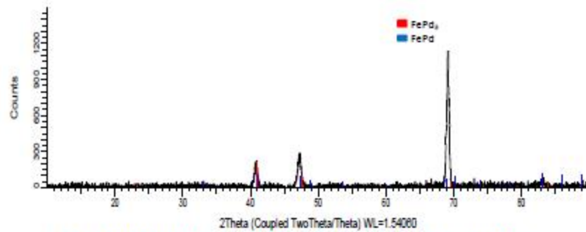
Figure 4. XRD pattern for nominal Alloy 2 \text{Fe}_{15}\text{Co}_{30}\text{Pd}_{75} (at.%), as-cast condition.
