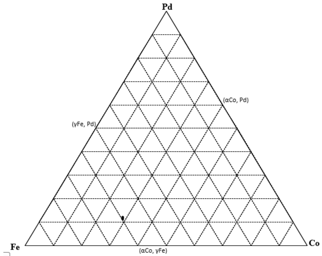
Figure 4.38. EDX analyses of nominal \text{Co}_{30}\text{Fe}_{60}\text{Pd}_{10} (at.%), Alloy 1 1000°C annealed condition. (■ Overall composition; ● phases).
