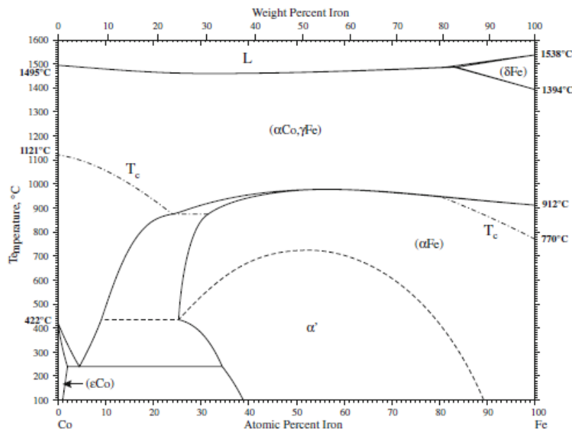
Figure 2.3. Binary diagram for Co-Fe system [2002Ohn].
