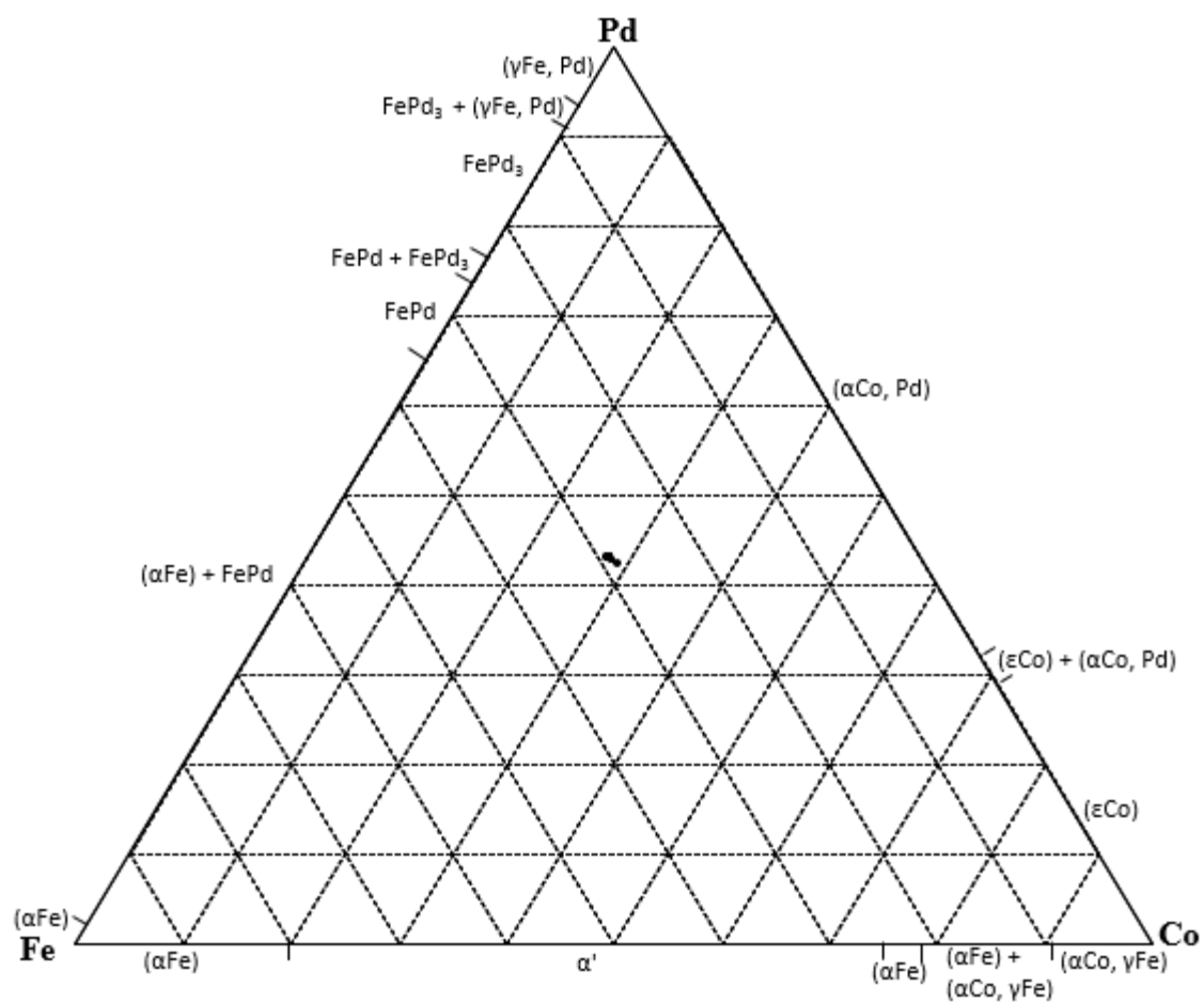
Figure 4.14. EDX analyses of nominal \text{Co}_{30}\text{Fe}_{30}\text{Pd}_{40} (at.%), Alloy 5 as-cast condition. (■ Overall composition; ● phases)
