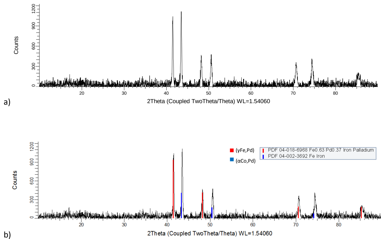
Figure 4.108. XRD patterns for nominal \text{Co}_{60}\text{:Fe}_{20}\text{:Pd}_{20} (at.%), Alloy 12 650°C annealed condition: a) raw, and b) labelled.
