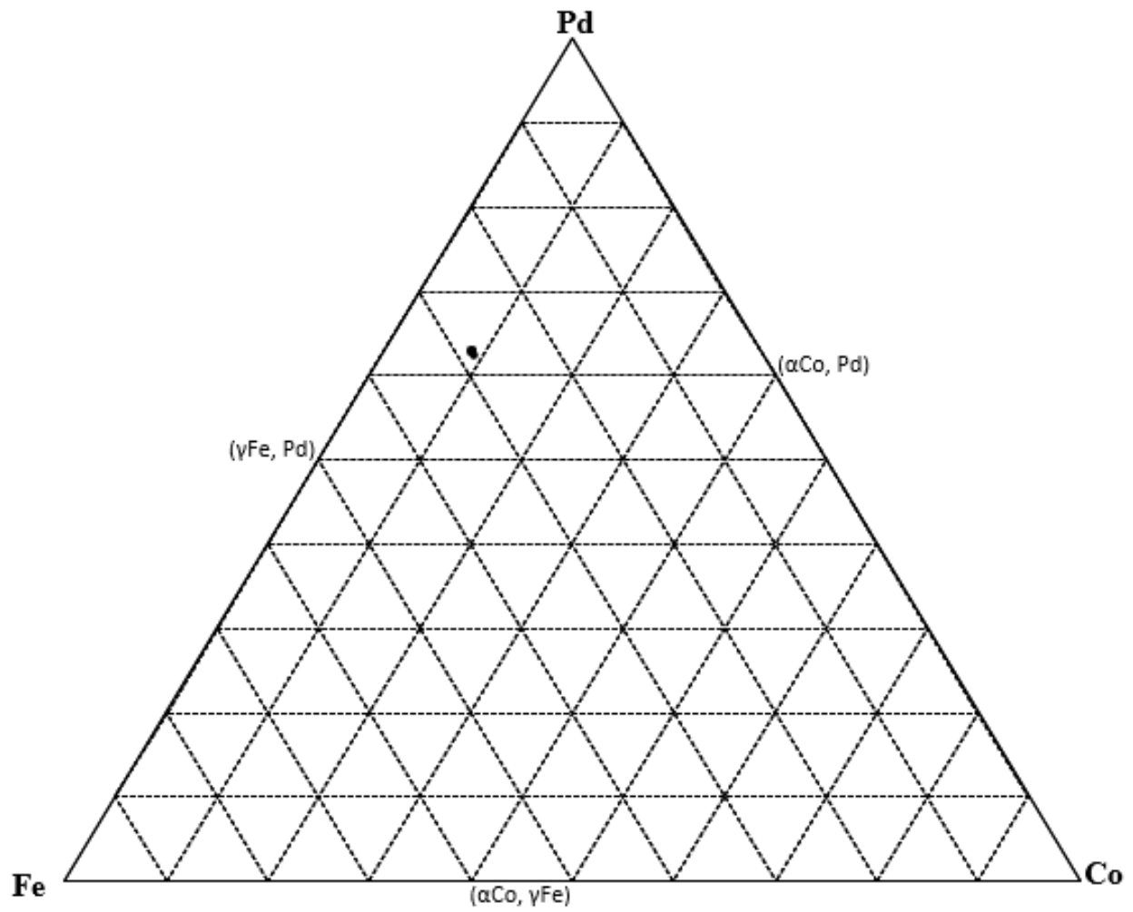
Figure 4.56. EDX analyses of nominal \text{Co}_{10}\text{Fe}_{30}\text{Pd}_{60} (at.%), Alloy 7 1000°C annealed condition. (■ Overall composition; ● phases)
