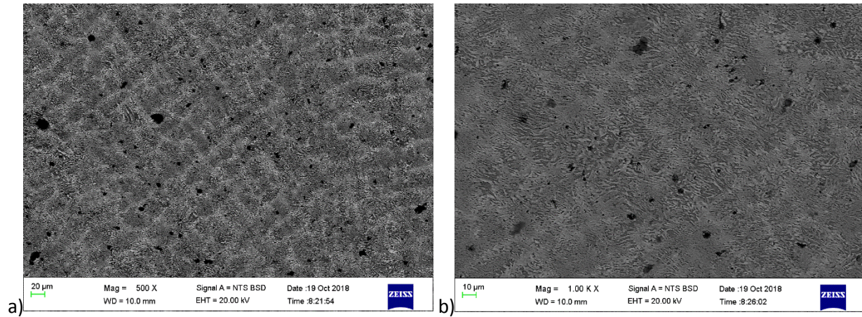
Figure 4.73. SEM-BSE images of \text{Co}_{30}\text{Fe}_{60}\text{Pd}_{10} (at.%), Alloy 1 annealed at 650°C for 1000 h showing: a) apparent dendrites, and b) higher magnification light and dark fine phases.
