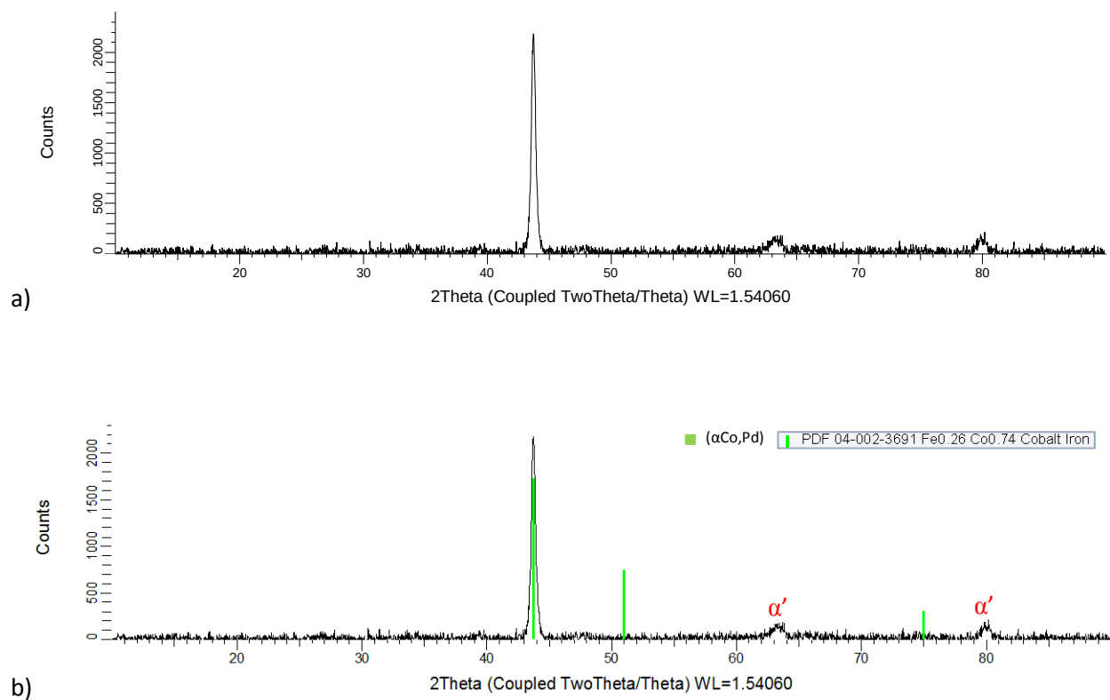
Figure 4.69. XRD patterns for nominal \text{Co}_{20}\text{:Fe}_{60}\text{:Pd}_{20} (at.%), Alloy 11 1000°C annealed condition: a) raw, and b) labelled.
