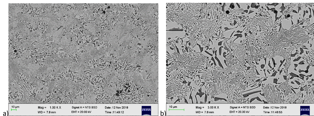
Figure 4.100. SEM-BSE images of \text{Co}_{40}\text{Fe}_{30}\text{Pd}_{30} (at.%), Alloy 10 annealed at 650^\circ\text{C} for 1000 h showing: a) an overall, and b) formation of fine phase, light and dark phases.
