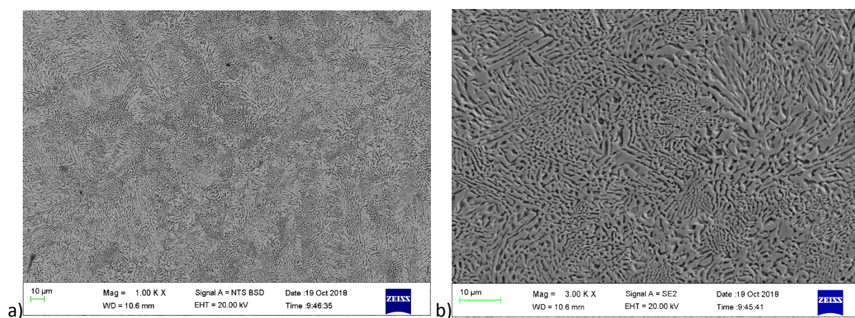
Figure 4.88. SEM images of \text{Co}_{50}\text{Fe}_{20}\text{Pd}_{30} (at.%), Alloy 6 annealed at 650^{\circ}\text{C} for 1000 h showing: a) BSE overall of the alloy and b) SE microstructure at higher magnification.
