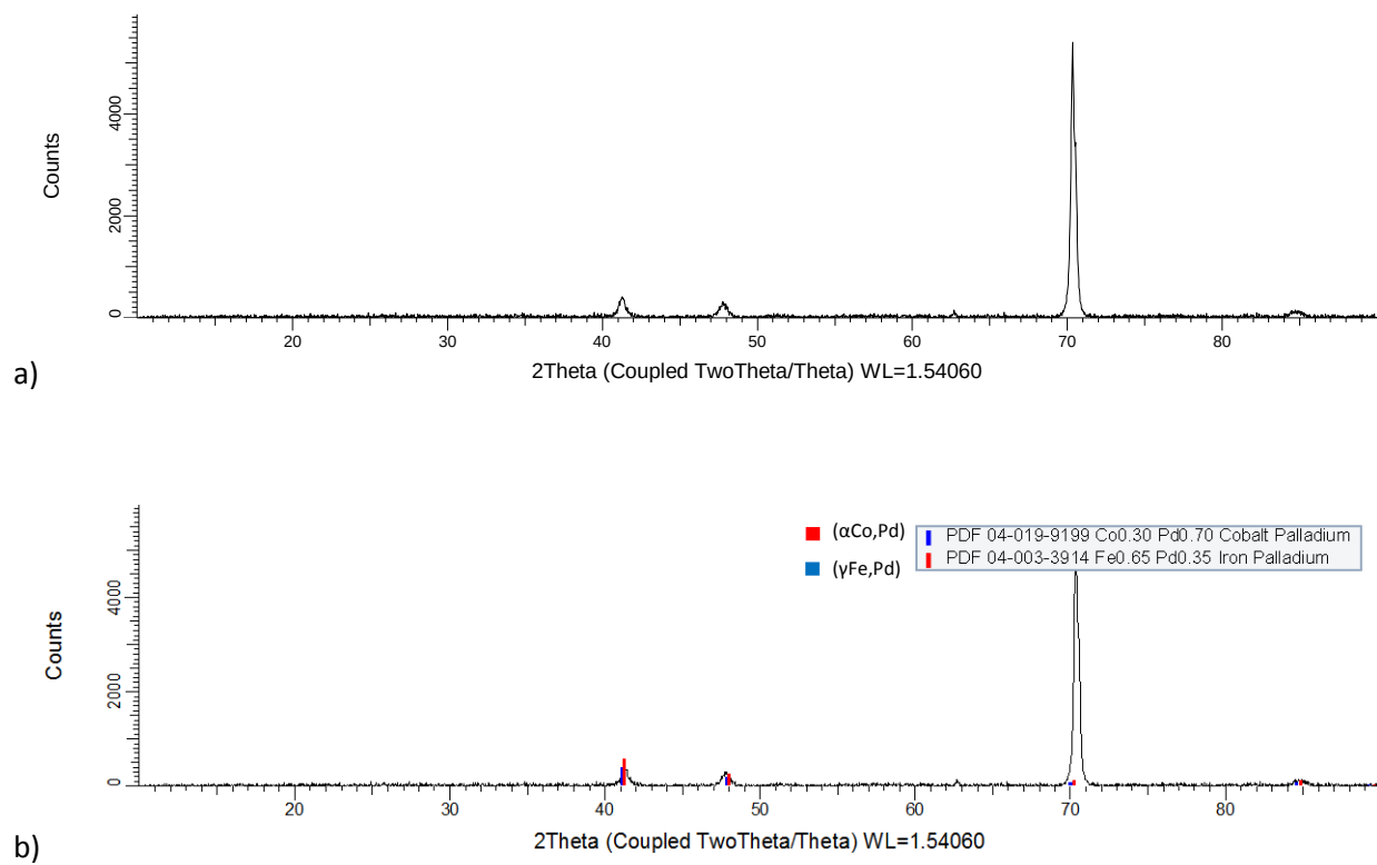
Figure 4.63. XRD patterns for nominal \text{Co}_{10}\text{:Fe}_{50}\text{:Pd}_{40} (at.%), Alloy 9 1000°C annealed condition: a) raw, and b) labelled.
