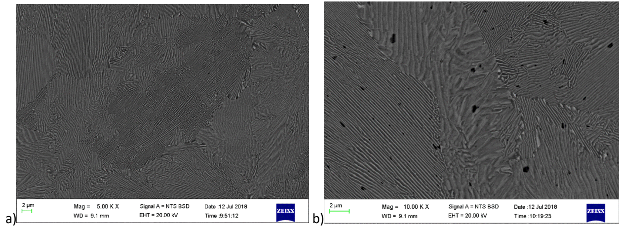
Figure 4.37. SEM-BSE images of \text{Co}_{30}\text{Fe}_{60}\text{Pd}_{10} (at.%), Alloy 1 annealed at 1000°C for 1000 h showing: a) the lamellar microstructure and b) at higher magnification.
