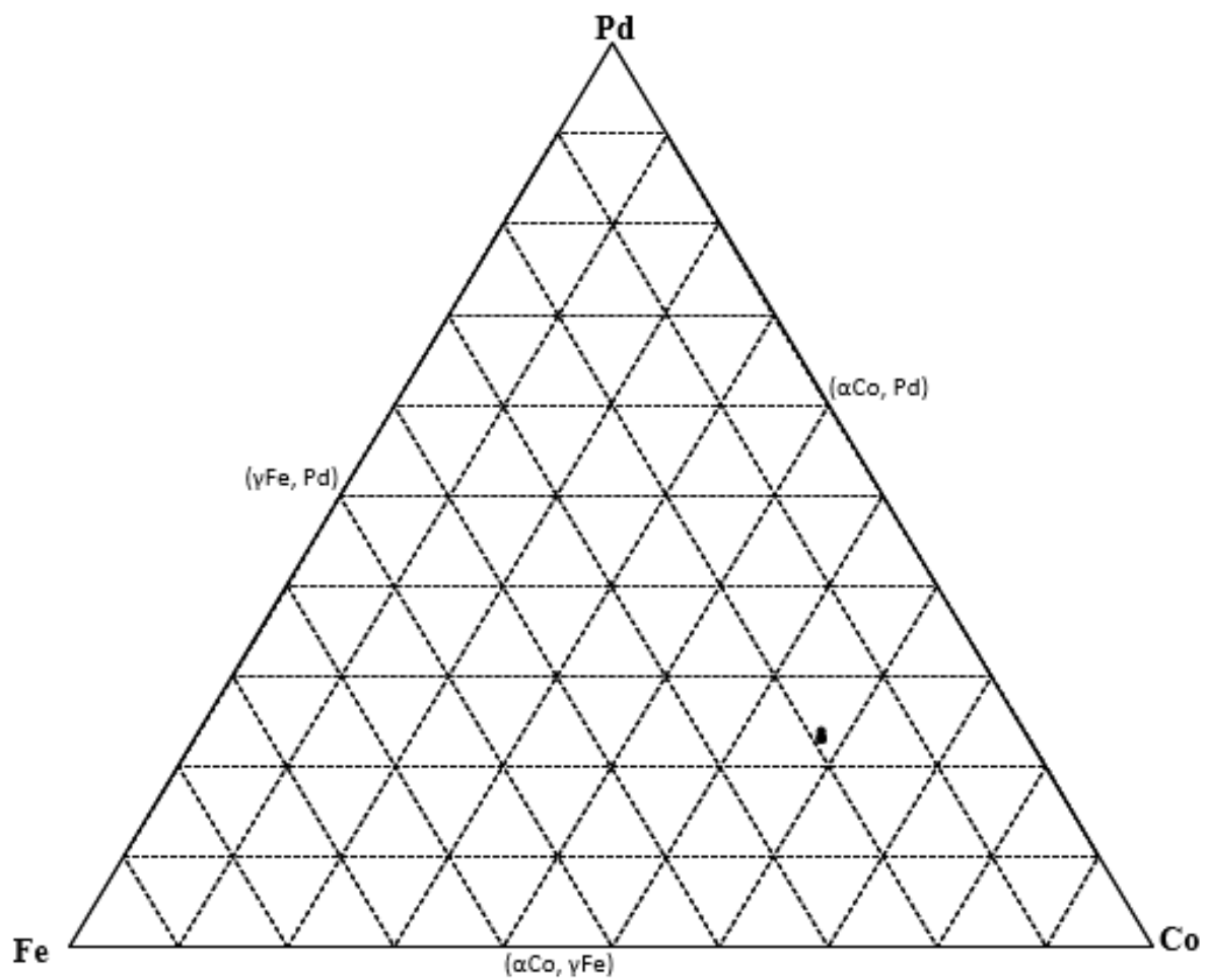
Figure 4.71. EDX analyses of nominal \text{Co}_{60}\text{:Fe}_{20}\text{:Pd}_{20} (at.%), Alloy 12 1000°C annealed condition. (■ Overall composition; ● phases)
