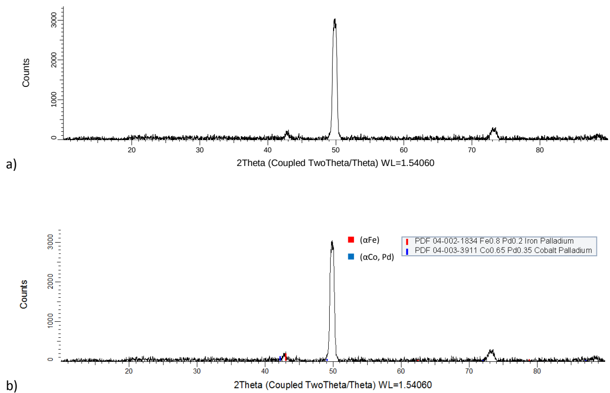
Figure 4.36. XRD patterns for nominal \text{Co}_{60}\text{:Fe}_{20}\text{:Pd}_{20} (at.%), Alloy 12 as-cast condition: a) raw, and b) labelled.
