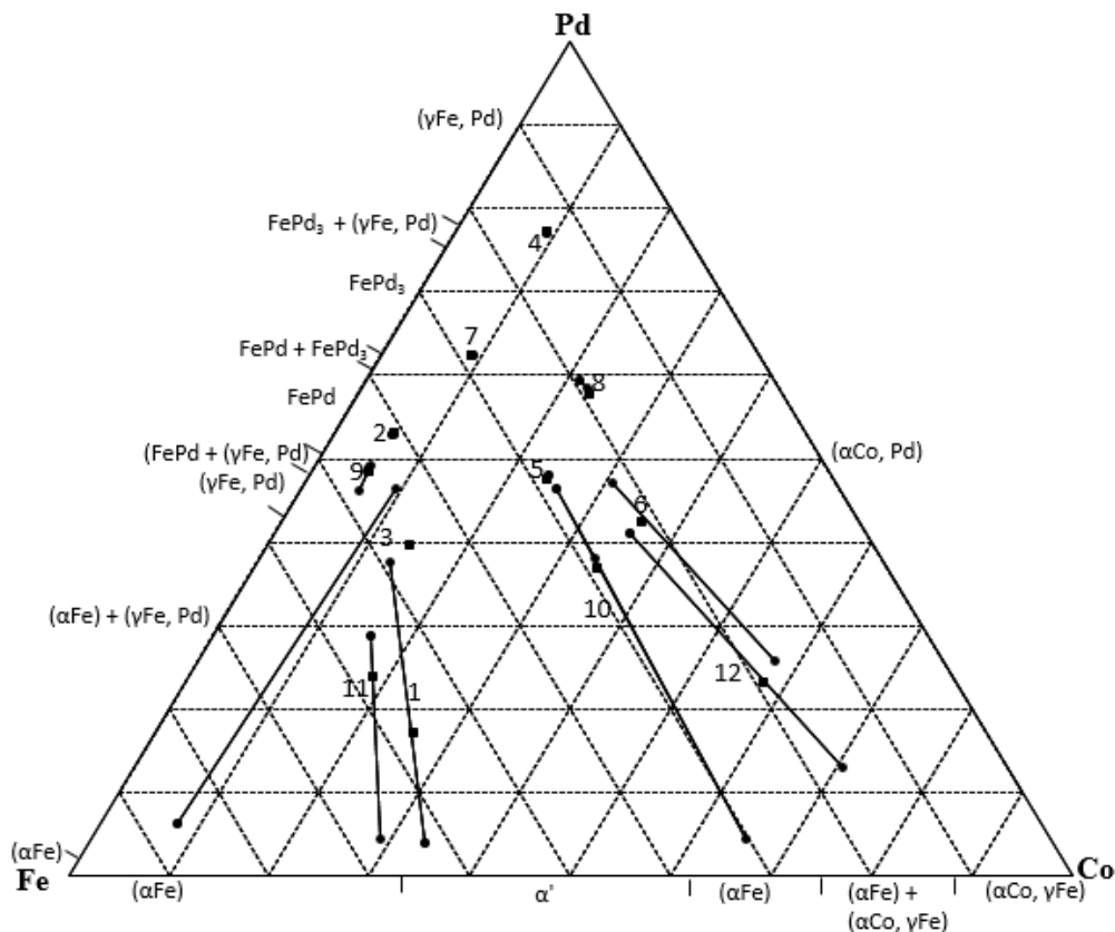
Figure 6.4. Results for the alloys annealed at 650°C for the Co-Fe-Pd system (at.%). (■ Overall composition; ● phases)
