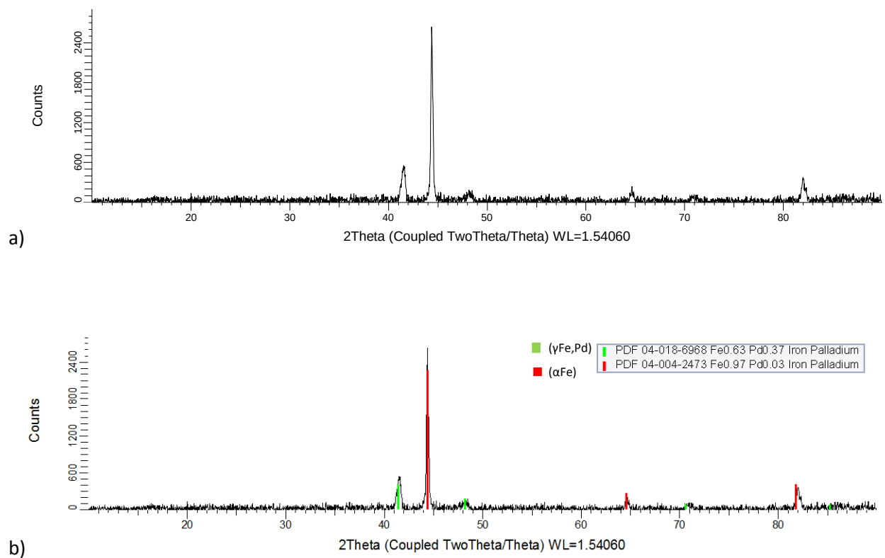
Figure 4.39. XRD patterns for nominal \text{Co}_{30}\text{:Fe}_{60}\text{:Pd}_{10} (at.%), Alloy 1 1000°C annealed condition: a) raw, and b) labelled.
