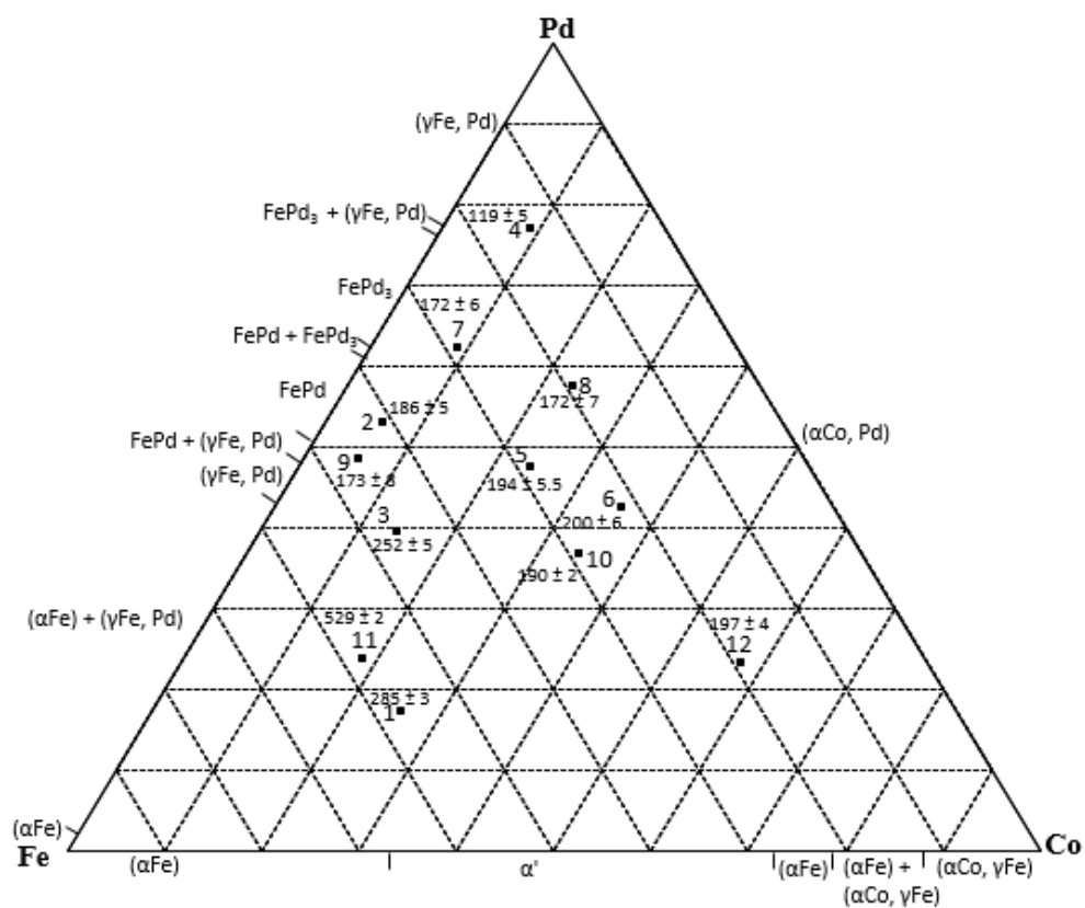
Figure 5.3. Ternary plot with hardness values and errors for alloys annealed at 650°C. (■ Overall composition)
