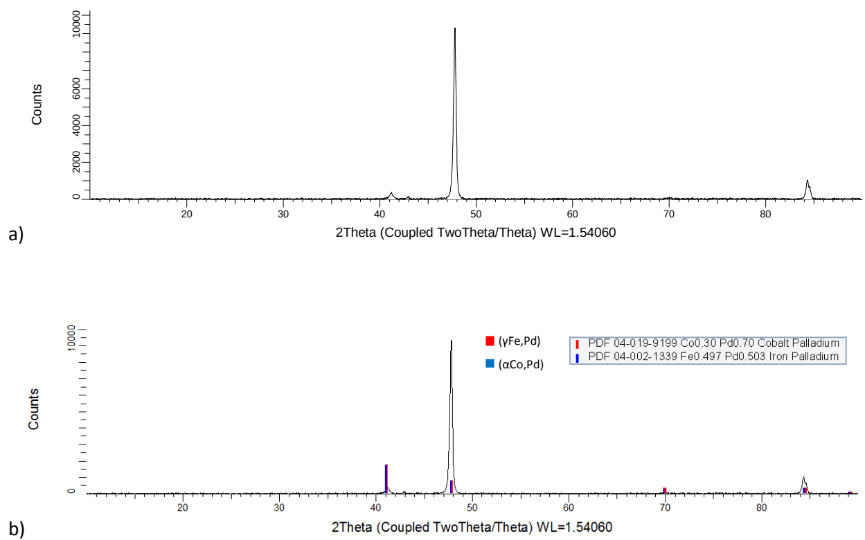
Figure 4.6. XRD patterns for nominal \text{Co}_6\text{:Fe}_{44}\text{:Pd}_{50} (at.%), Alloy 2 as-cast condition: a) raw, and b) labelled.
