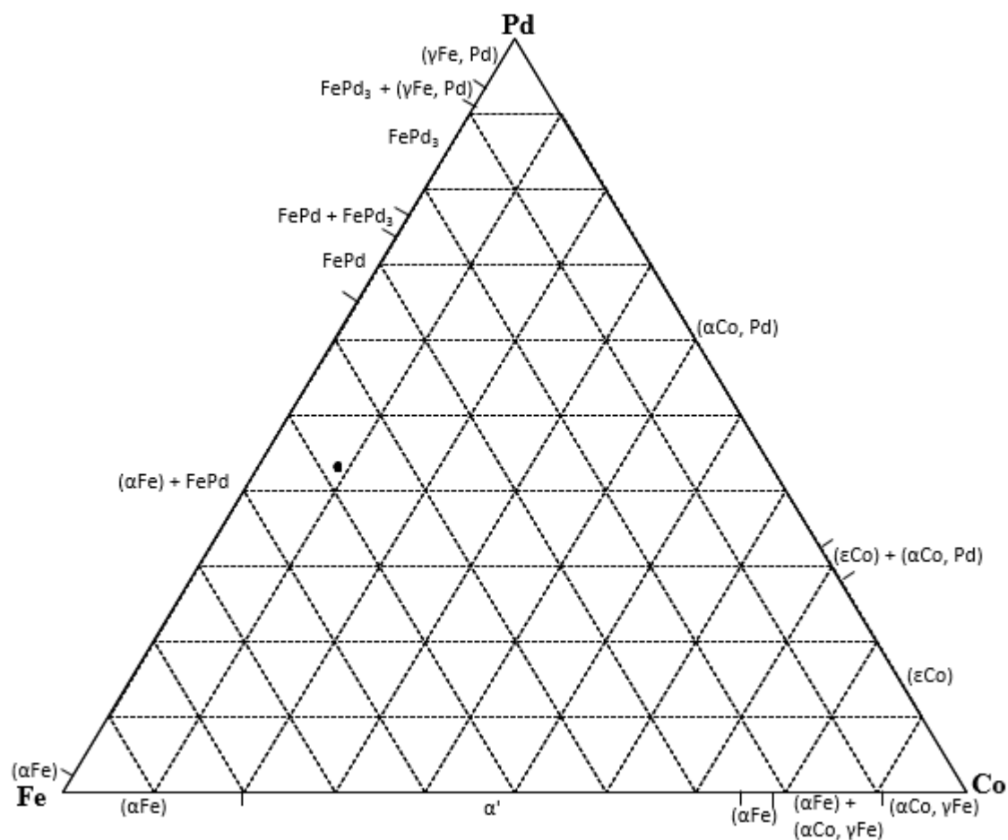
Figure 4.26. EDX analyses of nominal \text{Co}_{10}\text{Fe}_{50}\text{Pd}_{40} (at.%), Alloy 9 as-cast condition. (■ Overall composition; ● phases)
