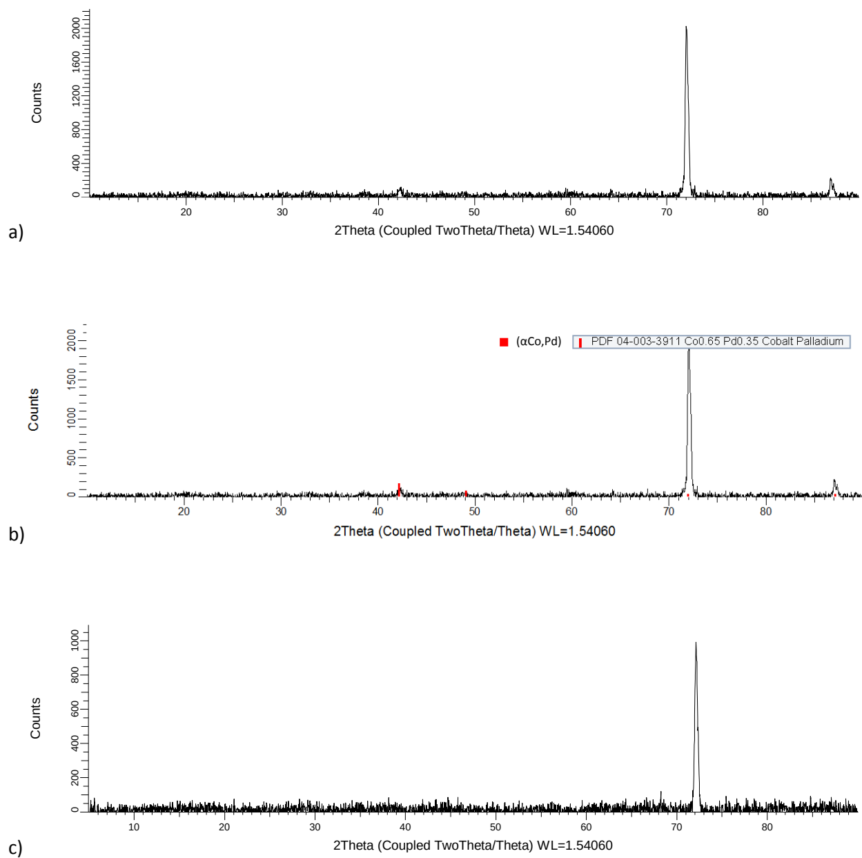
Figure 4.54. XRD patterns for nominal \text{Co}_{50}\text{:Fe}_{20}\text{:Pd}_{30} (at.%), Alloy 6 1000^{\circ}\text{C} annealed condition: a) raw 10 minutes scan, b) labelled, and c) raw 20 minutes scan.
