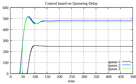
Figure A.105: Queue size, case 1 with 3 links and 4 sources (C Q D)
