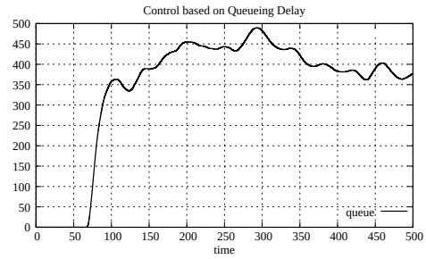
Figure A.96: Queue size, case 4 with 1 link and 3 sources (C Q D)
