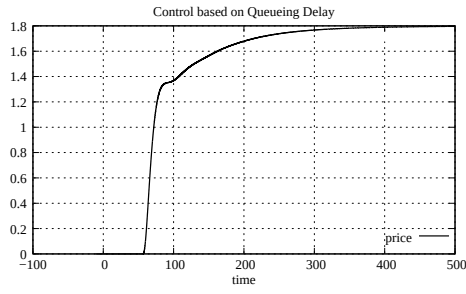
Figure A.87: Link price, case 3 with 1 link and 3 sources (C Q D)
