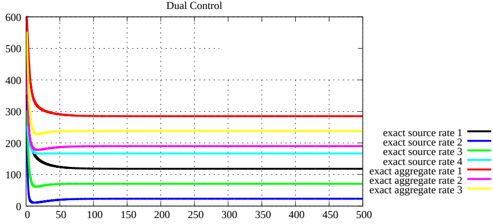
Figure 5.25: Source rates with 3 links and 4 sources (Dual)
