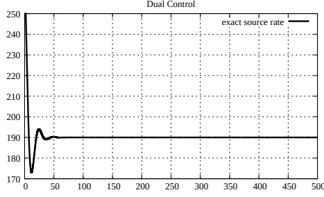
Figure 5.4: Source rate, case 1 with 1 link and 1 source (Dual)
