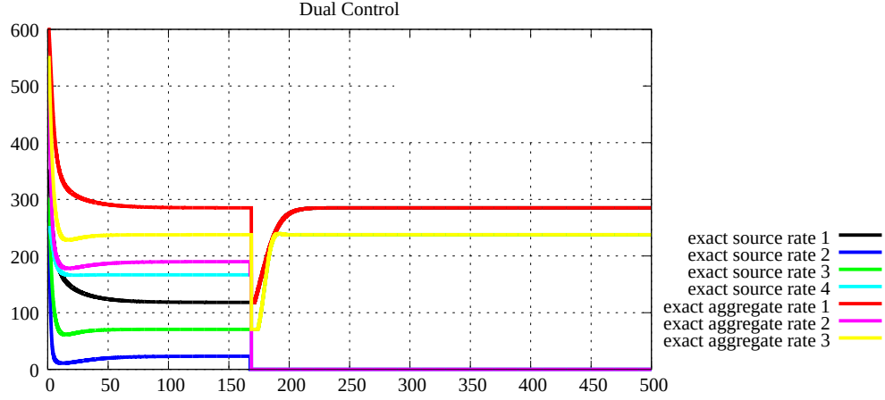
Figure 6.2: Source rates with 3 links and 4 sources (Dual)
