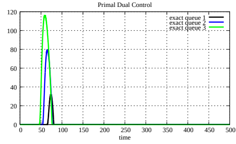
Figure 5.46: Queue sizes with 3 links (same capacity) and 4 sources (P D C)
