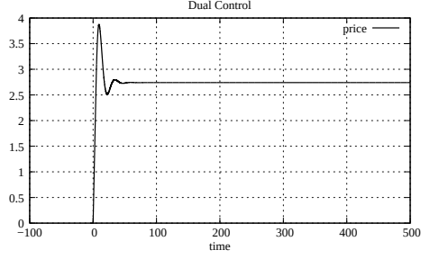
Figure A.3: Link price, case 3 with 1 link and 1 source (Dual)
