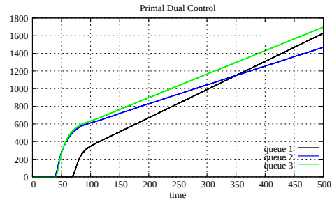
Figure A.70: Queue size, case 2 with 3 links and 4 sources (P D C)
