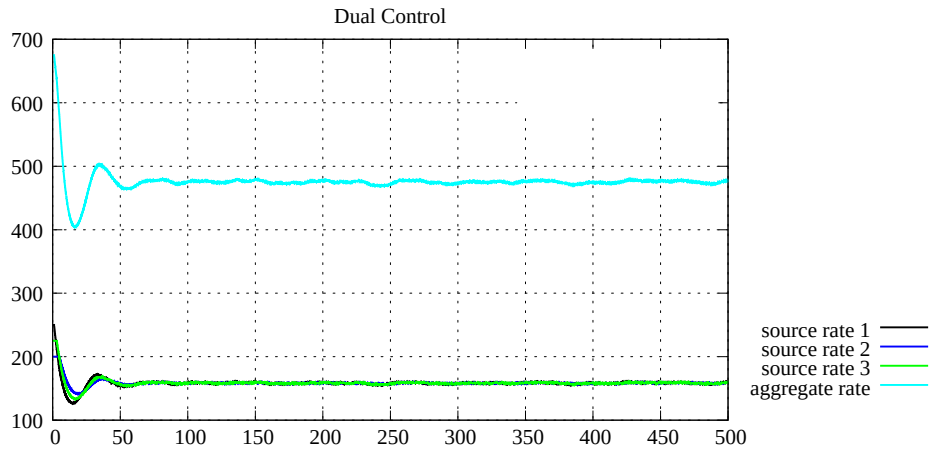
Figure A.20: Source rates, case 4 with 1 link and 3 sources (Dual)
