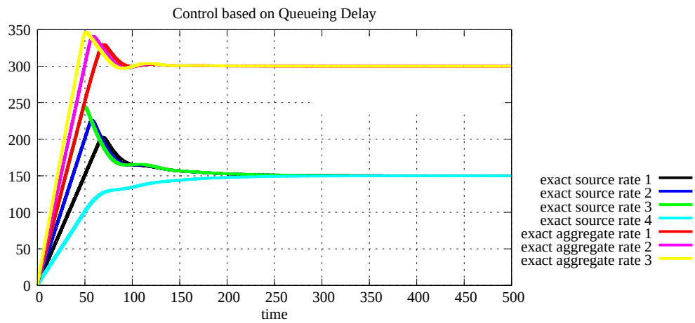
Figure 5.62: Source rates with 3 links (same capacity) and 4 sources (C Q D)
