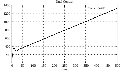
Figure A.10: Queue size, case 2 with 1 link and 1 source (Dual)
