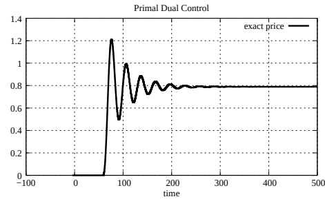
Figure 5.30: Link price, case 2 with 1 link and 1 source (P D C)
