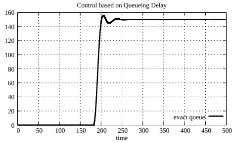
Figure 5.51: Queue size, case 1 with 1 link and 1 source (C Q D)
