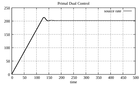
Figure A.42: Source rate, case 2 with 1 link and 1 source (P D C)
