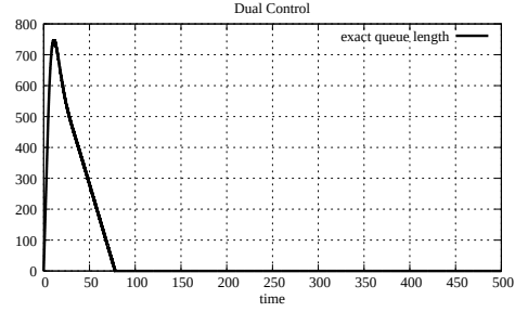
Figure 5.7: Queue size, case 2 with 1 link and 1 source (Dual)
