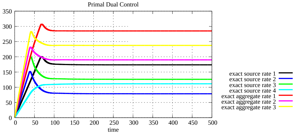
Figure 5.43: Source rates with 3 links and 4 sources (P D C)
