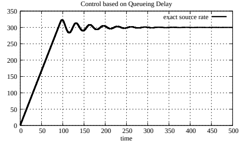
Figure 5.50: Source rate, case 2 with 1 link and 1 source (C Q D)
