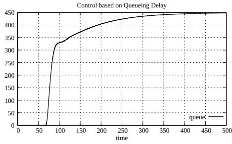
Figure A.93: Queue size, case 1 with 1 link and 3 sources (C Q D)
