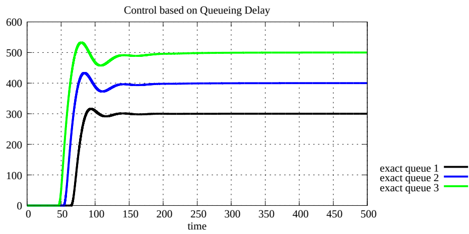
Figure 5.64: Queue sizes with 3 links (same capacity) and 4 sources (C Q D)
