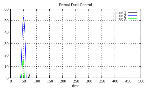
Figure A.72: Queue size, case 4 with 3 links and 4 sources (P D C)
