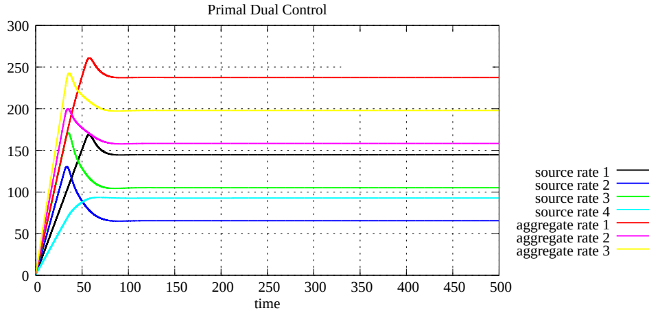
Figure A.67: Source rates, case 3 with 3 links and 4 sources (P D C)
