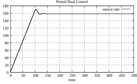
Figure A.43: Source rate, case 3 with 1 link and 1 source (P D C)
