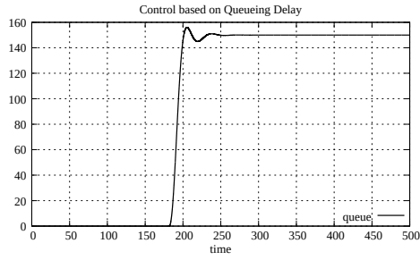
Figure A.81: Queue size, case 1 with 1 link and 1 source (C Q D)
