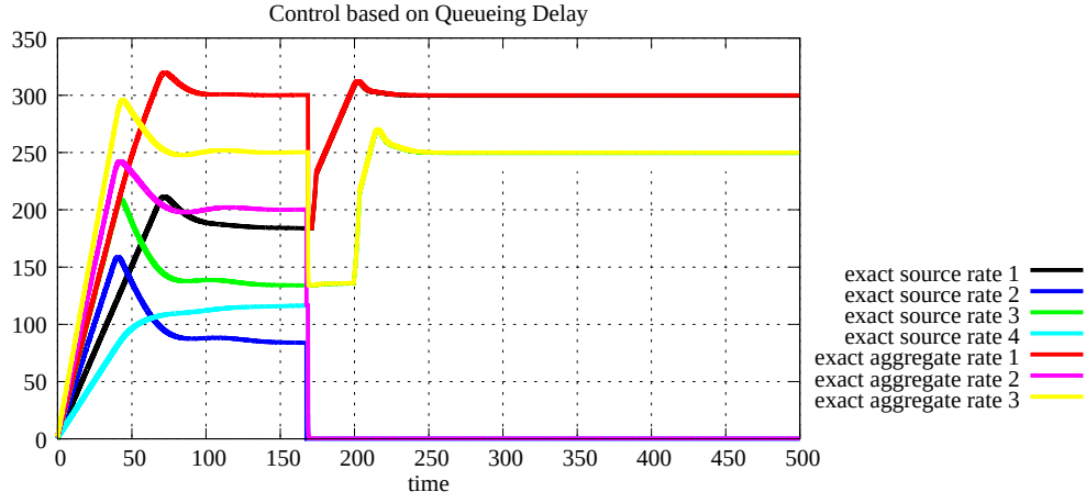
Figure 6.6: Source rates with 3 links and 4 sources (C Q D)
