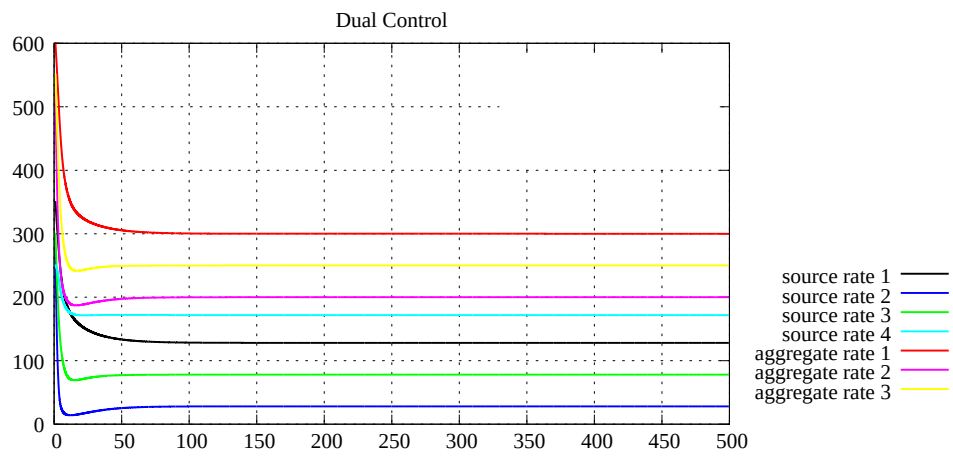
Figure A.29: Source rates, case 1 with 3 links and 4 sources (Dual)
