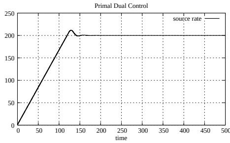
Figure A.41: Source rate, case 1 with 1 link and 1 source (P D C)
