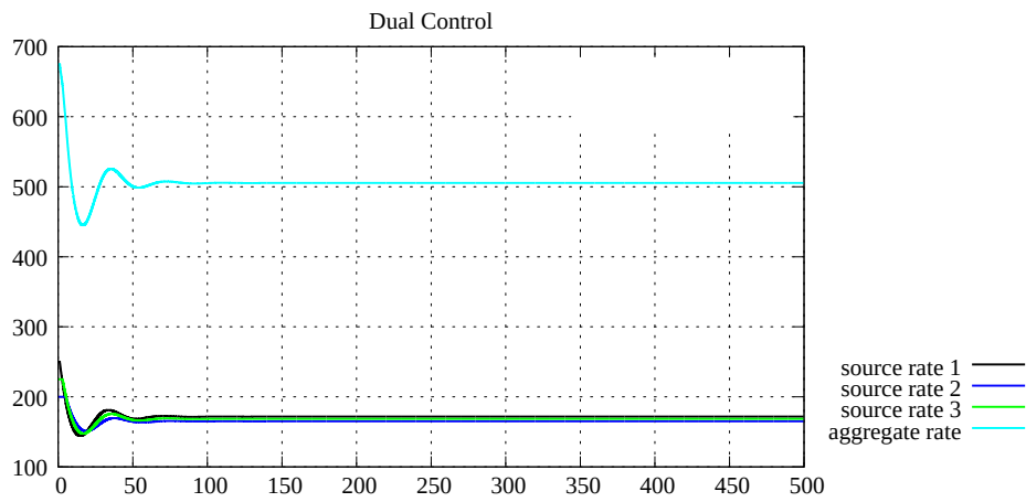
Figure A.18: Source rates, case 2 with 1 link and 3 sources (Dual)
