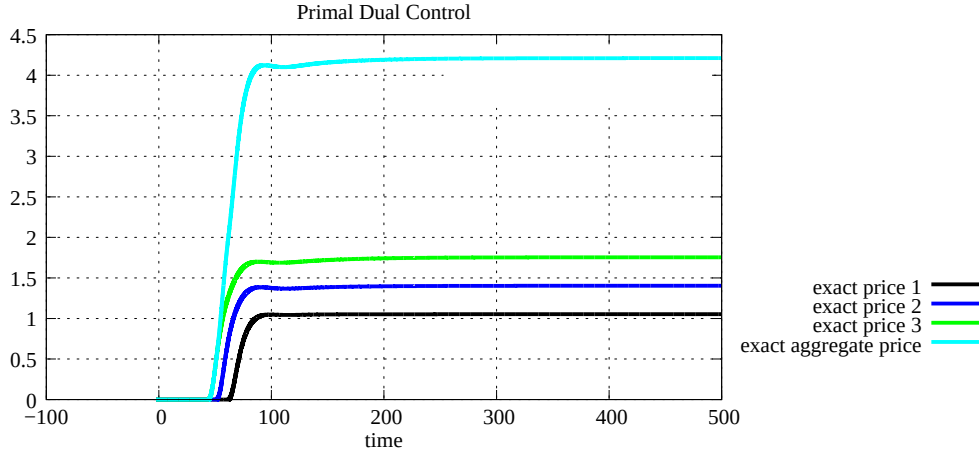
Figure 5.42: Link prices with 3 links (same capacity) and 4 sources (P D C)
