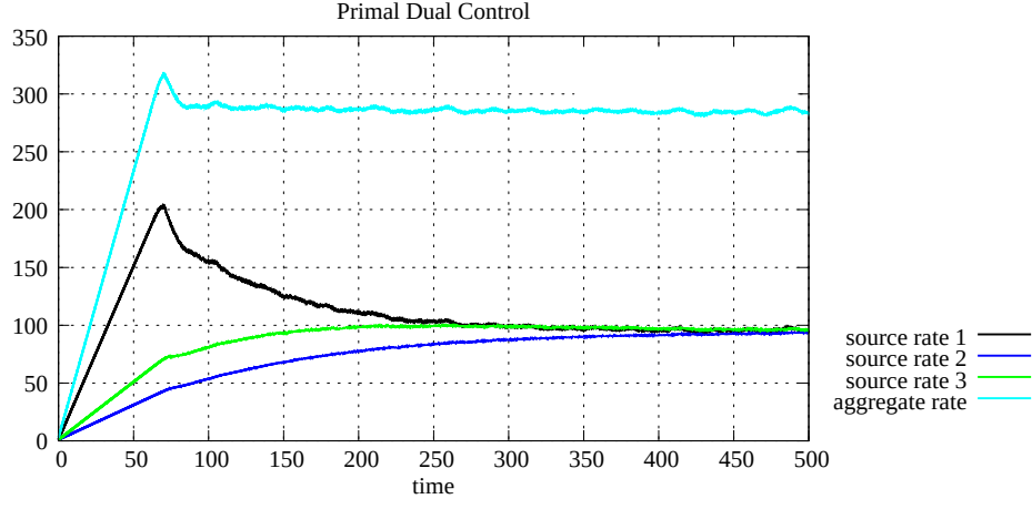
Figure A.56: Source rates, case 4 with 1 link and 3 sources (P D C)
