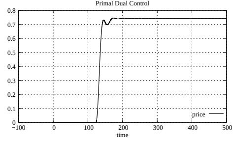
Figure A.38: Link price, case 2 with 1 link and 1 source (P D C)
