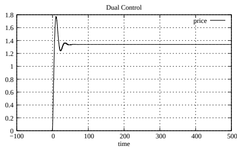
Figure A.1: Link price, case 1 with 1 link and 1 source (Dual)
