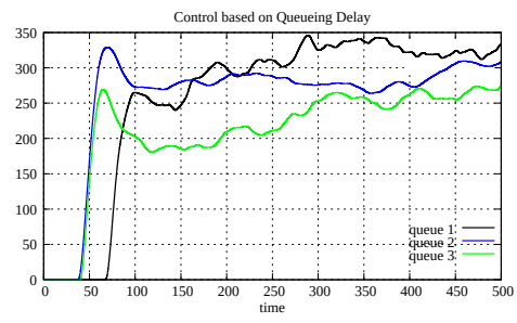
Figure A.108: Queue size, case 4 with 3 links and 4 sources (C Q D)
