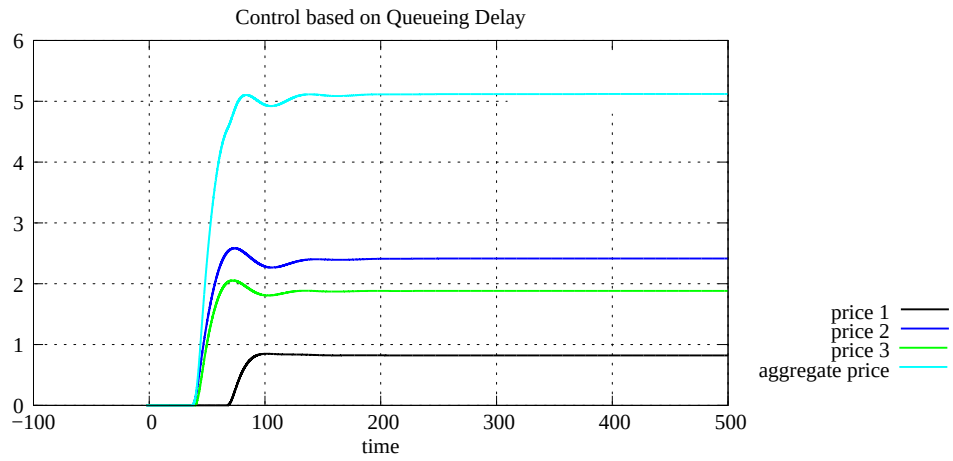
Figure A.97: Link price, case 1 with 3 links and 4 sources (C Q D)
