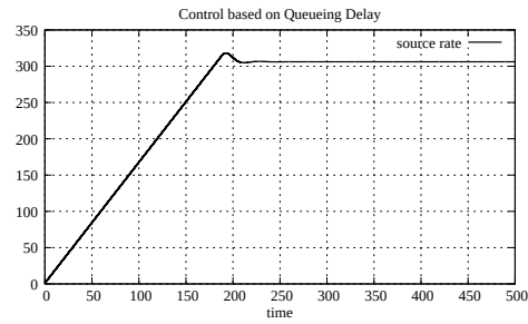
Figure A.78: Source rate, case 2 with 1 link and 1 source (C Q D)
