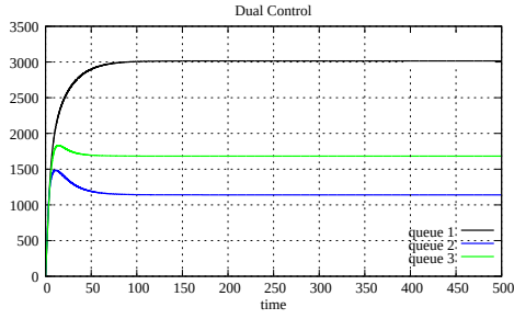
Figure A.33: Queue size, case 1 with 3 links and 4 sources (Dual)
