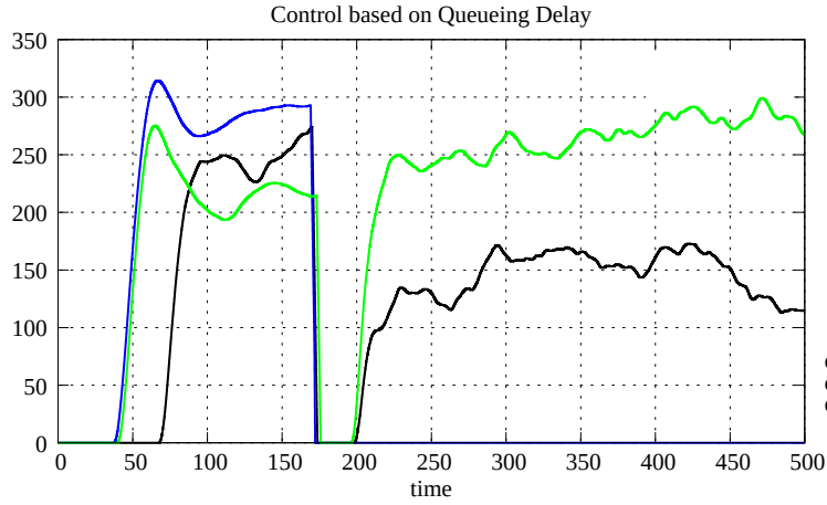
Figure 6.9: Queue size (with noise) with 3 links and 4 sources (C Q D)
