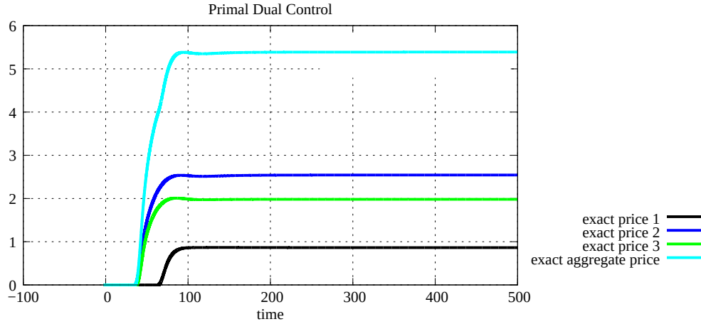
Figure 5.41: Link prices with 3 links and 4 sources (P D C)
