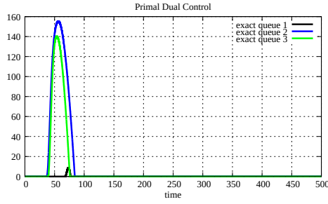
Figure 5.45: Queue sizes with 3 links and 4 sources (P D C)
