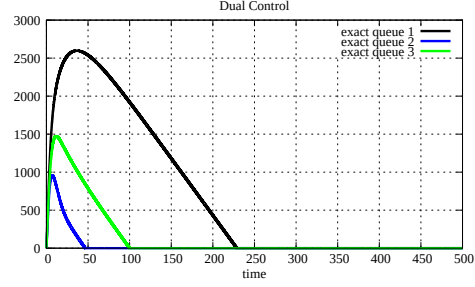
Figure 5.28: Queue sizes with 3 links (same capacity) and 4 sources (Dual)
