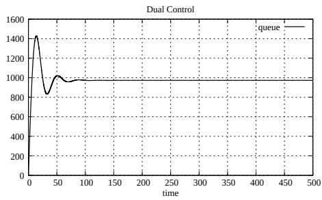
Figure A.21: Queue size, case 1 with 1 link and 3 sources (Dual)
