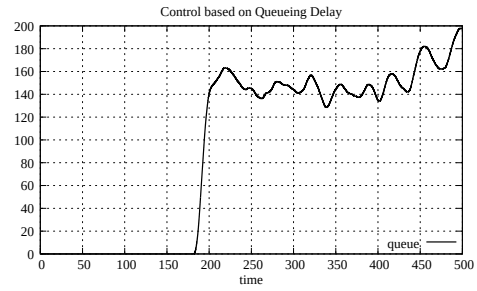
Figure A.84: Queue size, case 4 with 1 link and 1 source (C Q D)
