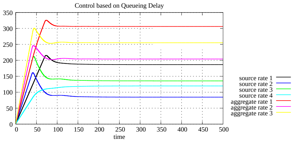
Figure A.102: Source rates, case 2 with 3 links and 4 sources (C Q D)
