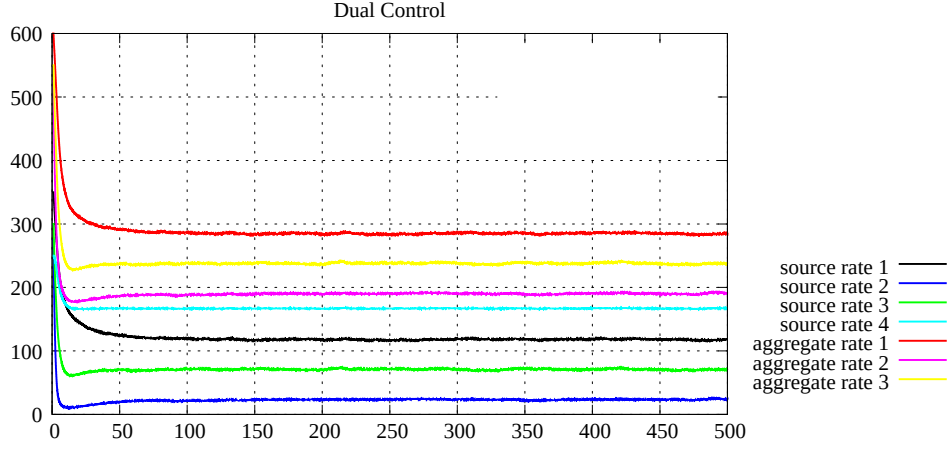
Figure A.32: Source rates, case 4 with 3 links and 4 sources (Dual)
