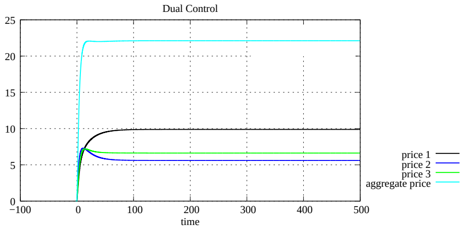
Figure A.26: Link price, case 2 with 3 links and 4 sources (Dual)
