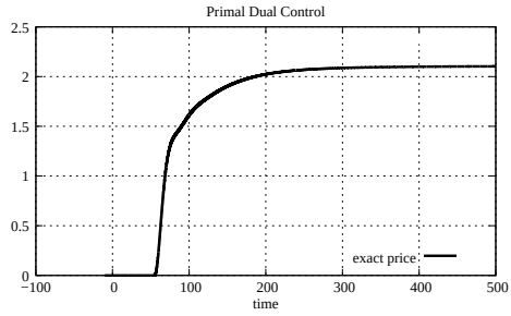
Figure 5.35: Link price, simple case with 1 link and 3 sources (P D C)
