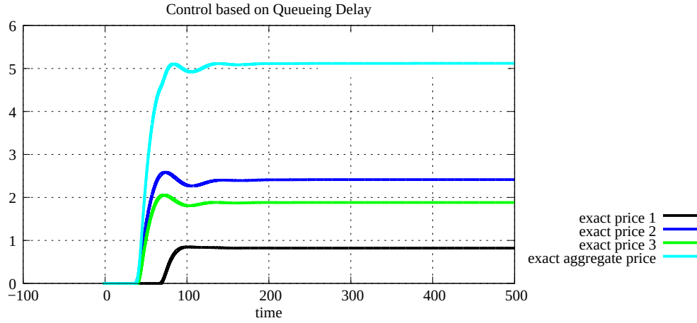
Figure 5.59: Link prices with 3 links and 4 sources (C Q D)
