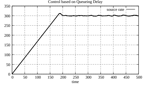
Figure A.80: Source rate, case 4 with 1 link and 1 source (C Q D)
