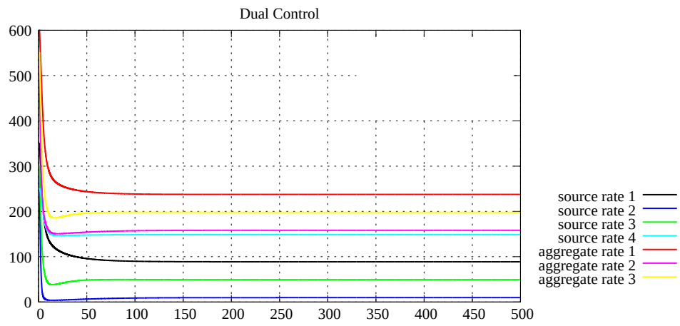
Figure A.31: Source rates, case 3 with 3 links and 4 sources (Dual)
