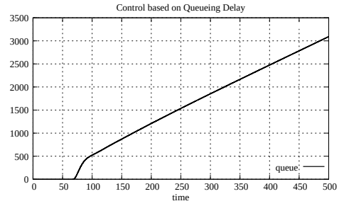
Figure A.94: Queue size, case 2 with 1 link and 3 sources (C Q D)
