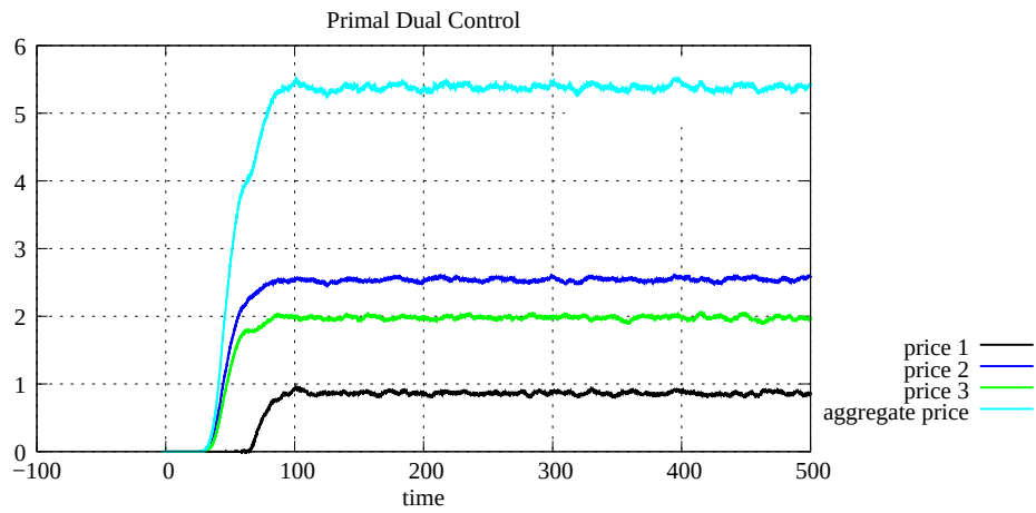
Figure A.64: Link price, case 4 with 3 links and 4 sources (P D C)
