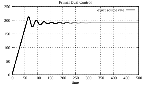
Figure 5.32: Source rate, case 2 with 1 link and 1 source (P D C)
