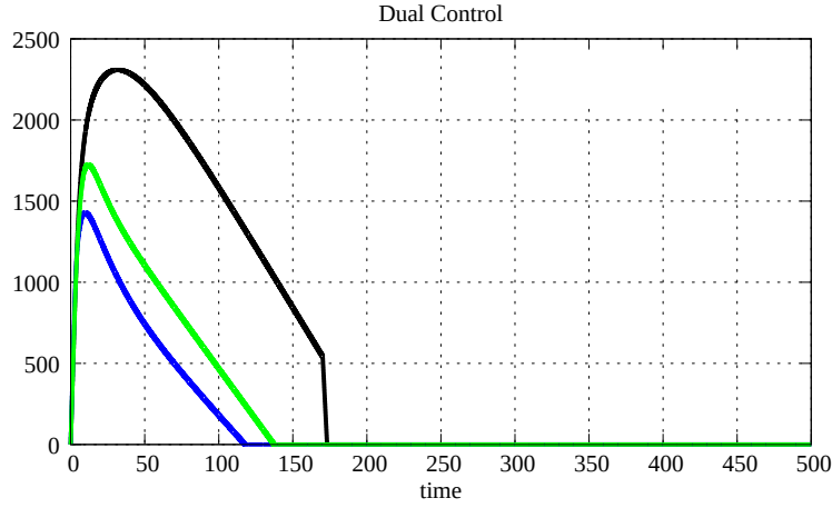
Figure 6.3: Queue size with 3 links and 4 sources (Dual)
