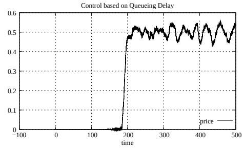
Figure A.76: Link price, case 4 with 1 link and 1 source (C Q D)
