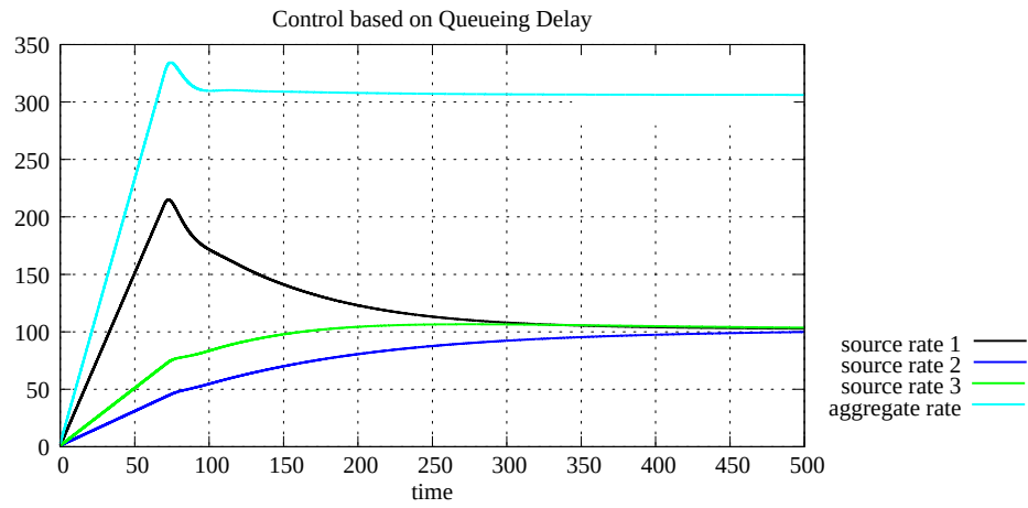
Figure A.90: Source rates, case 2 with 1 link and 3 sources (C Q D)
