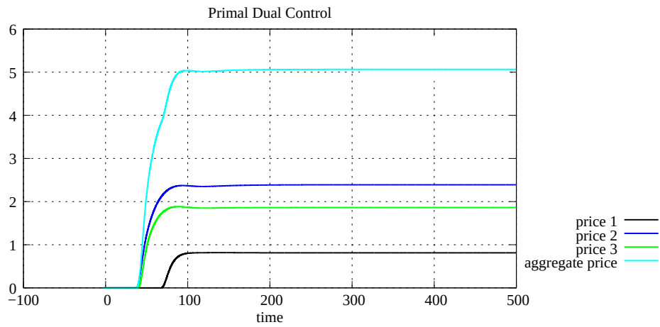
Figure A.62: Link price, case 2 with 3 links and 4 sources (P D C)
