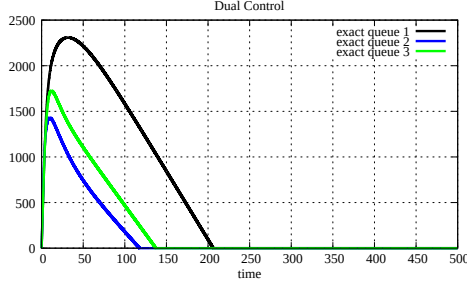
Figure 5.27: Queue sizes with 3 links and 4 sources (Dual)
