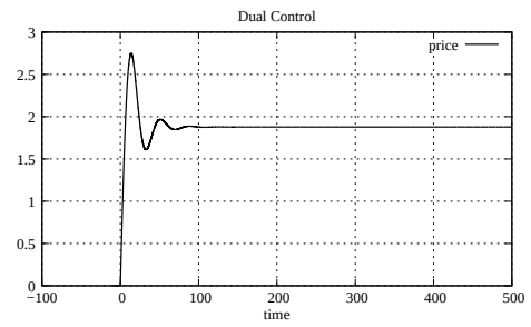
Figure A.14: Link price, case 2 with 1 link and 3 sources (Dual)
