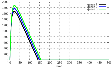
Figure 5.20: Queue sizes, case 1 with 3 links and 1 source (Dual)
