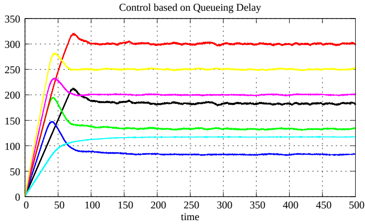
Figure A.104: Source rates, case 4 with 3 links and 4 sources (C Q D)
