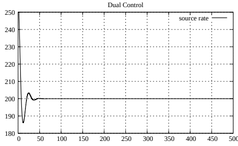
Figure A.5: Source rate, case 1 with 1 link and 1 source (Dual)
