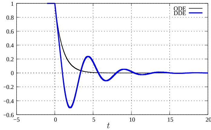
Figure 3.2: Ordinary and delay differential equations 1
