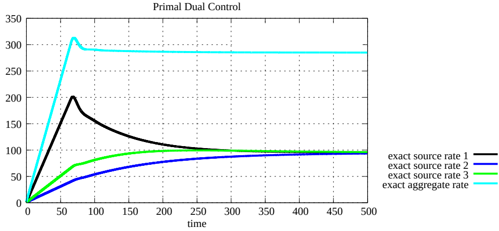
Figure 5.38: Source rates, fairness case with 1 links and 3 sources (P D C)
