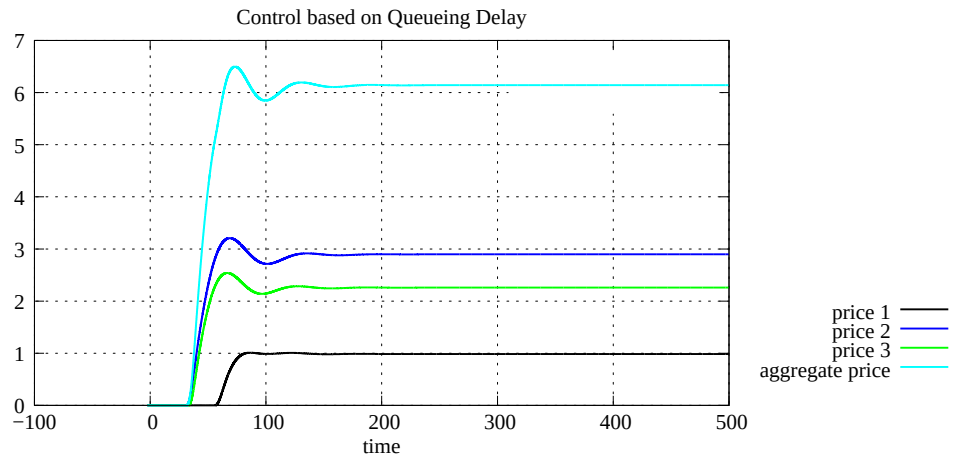
Figure A.99: Link price, case 3 with 3 links and 4 sources (C Q D)
