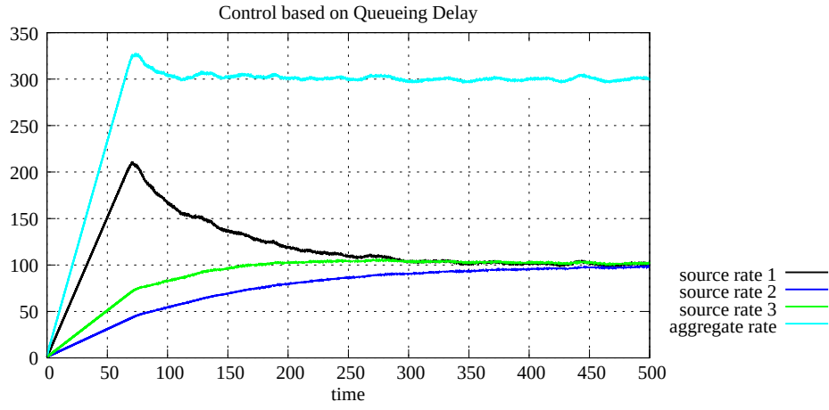
Figure A.92: Source rates, case 4 with 1 link and 3 sources (C Q D)
