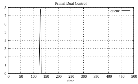
Figure A.48: Queue size, case 4 with 1 link and 1 source (P D C)
