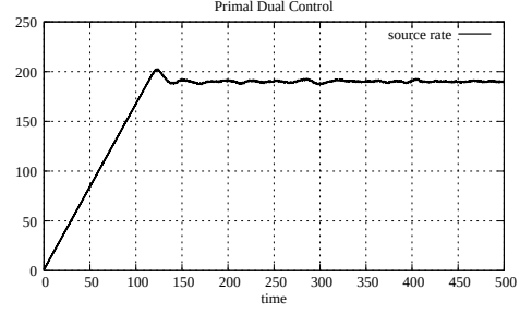
Figure A.44: Source rate, case 4 with 1 link and 1 source (P D C)
