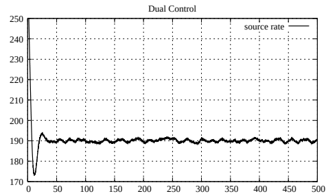
Figure A.8: Source rate, case 4 with 1 link and 1 source (Dual)
