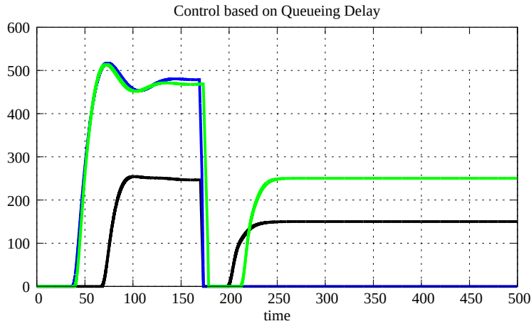
Figure 6.7: Queue size with 3 links and 4 sources (C Q D)
