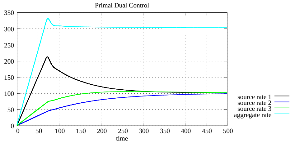
Figure A.54: Source rates, case 2 with 1 link and 3 sources (P D C)
