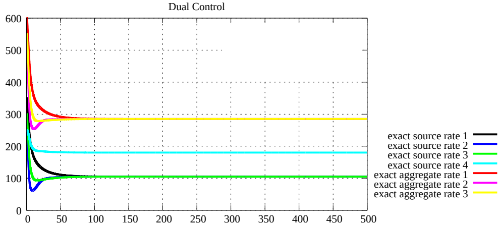
Figure 5.26: Source rates with 3 links (same capacity) and 4 sources (Dual)
