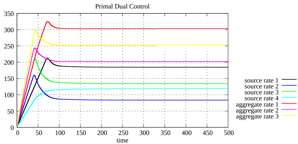
Figure A.66: Source rates, case 2 with 3 links and 4 sources (P D C)
