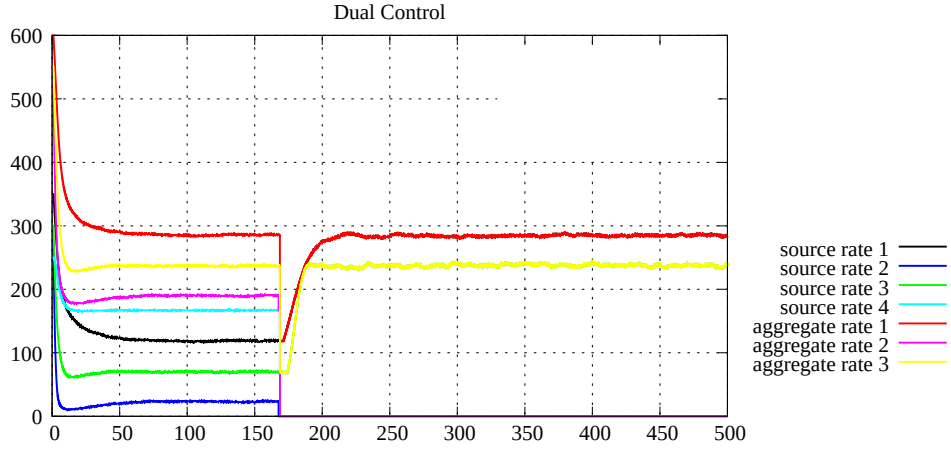
Figure 6.4: Source rates (with noise) with 3 links and 4 sources (Dual)
