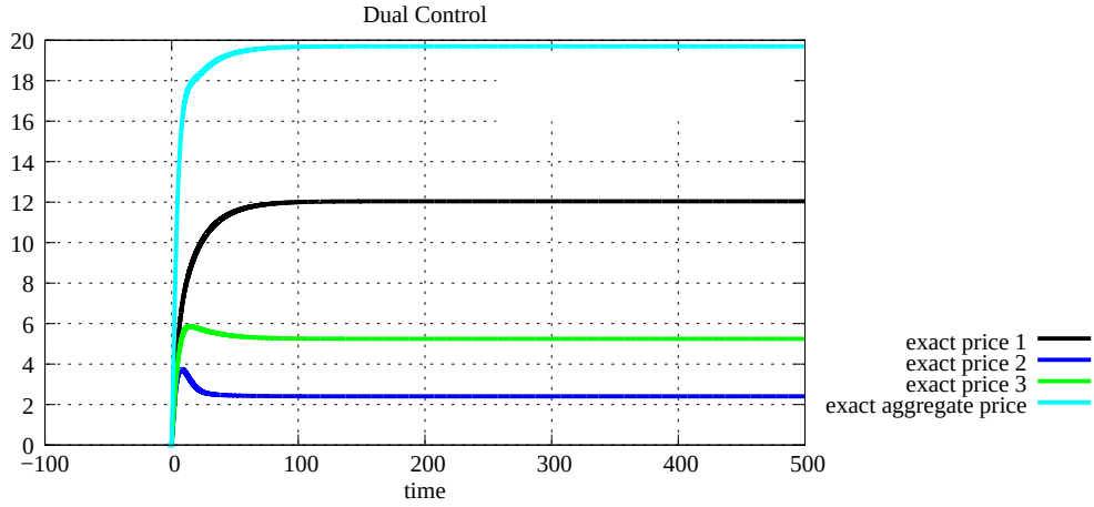
Figure 5.24: Link prices with 3 links (same capacity) and 4 sources (Dual)
