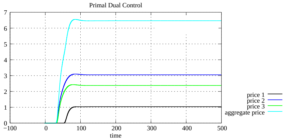
Figure A.63: Link price, case 3 with 3 links and 4 sources (P D C)
