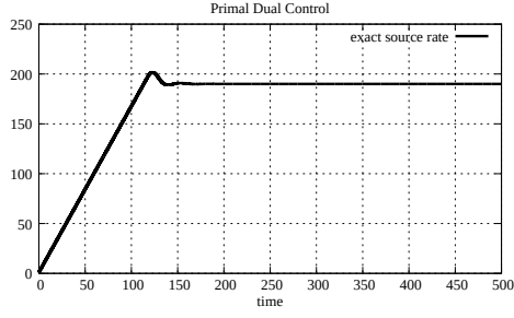
Figure 5.31: Source rate, case 1 with 1 link and 1 source (P D C)
