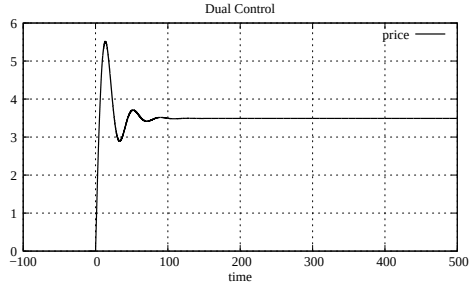
Figure A.15: Link price, case 3 with 1 link and 3 sources (Dual)
