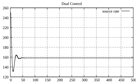
Figure A.7: Source rate, case 3 with 1 link and 1 source (Dual)
