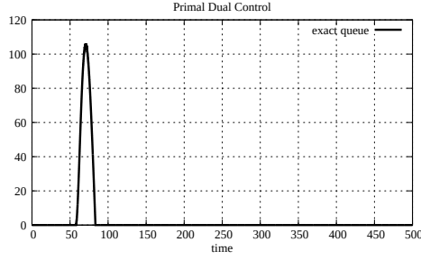
Figure 5.39: Queue size, simple case with 1 link and 3 sources (P D C)
