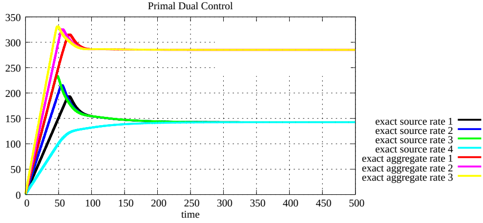
Figure 5.44: Source rates with 3 links (same capacity) and 4 sources (P D C)
