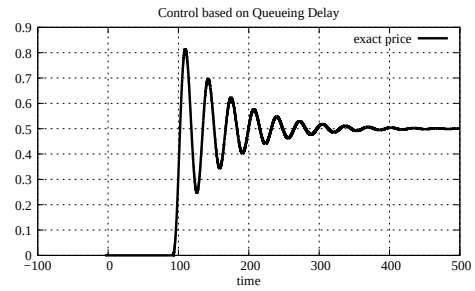
Figure 5.48: Link price, case 2 with 1 link and 1 source (C Q D)
