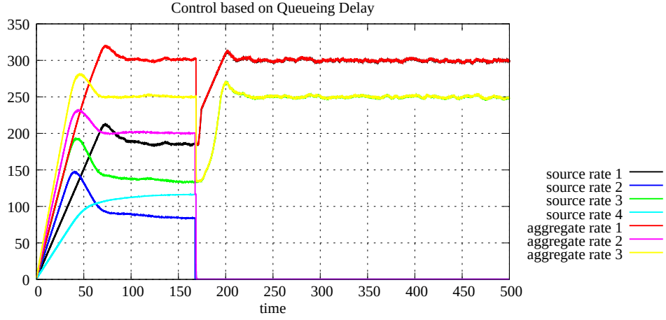
Figure 6.8: Source rates (with noise) with 3 links and 4 sources (C Q D)
