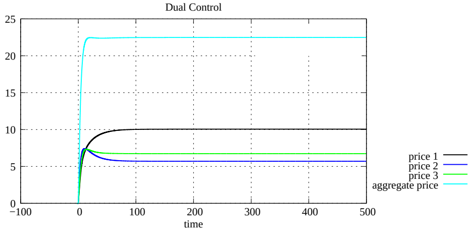
Figure A.25: Link price, case 1 with 3 links and 4 sources (Dual)
