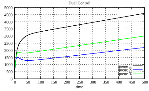
Figure A.34: Queue size, case 2 with 3 links and 4 sources (Dual)
