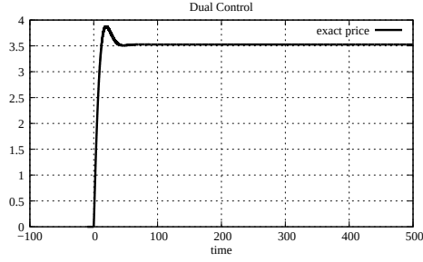
Figure 5.9: Link price, simple case with 1 link and 3 sources (Dual)
