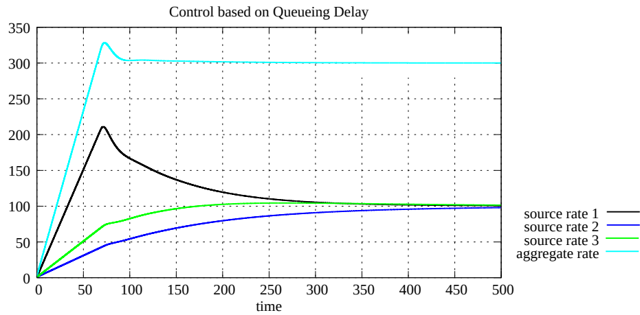
Figure A.89: Source rates, case 1 with 1 link and 3 sources (C Q D)
