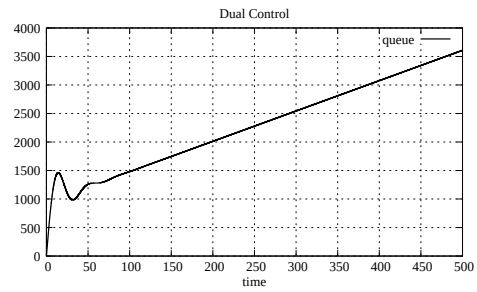
Figure A.22: Queue size, case 2 with 1 link and 3 sources (Dual)
