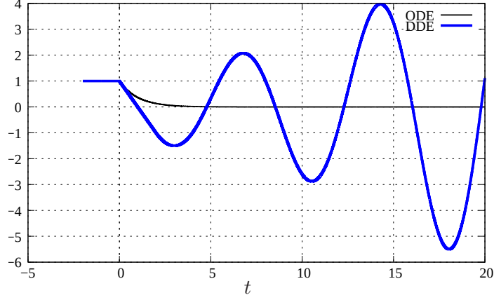
Figure 3.3: Ordinary and delay differential equations 2
