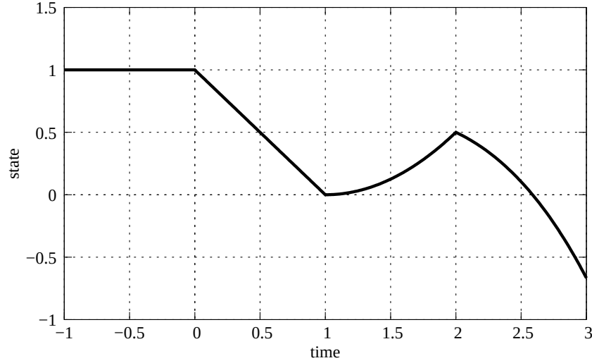
Figure 3.1: Poor approximation to the solution of a DDE.
