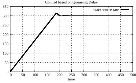
Figure 5.49: Source rate, case 1 with 1 link and 1 source (C Q D)
