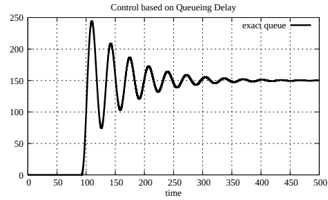
Figure 5.52: Queue size, case 2 with 1 link and 1 source (C Q D)
