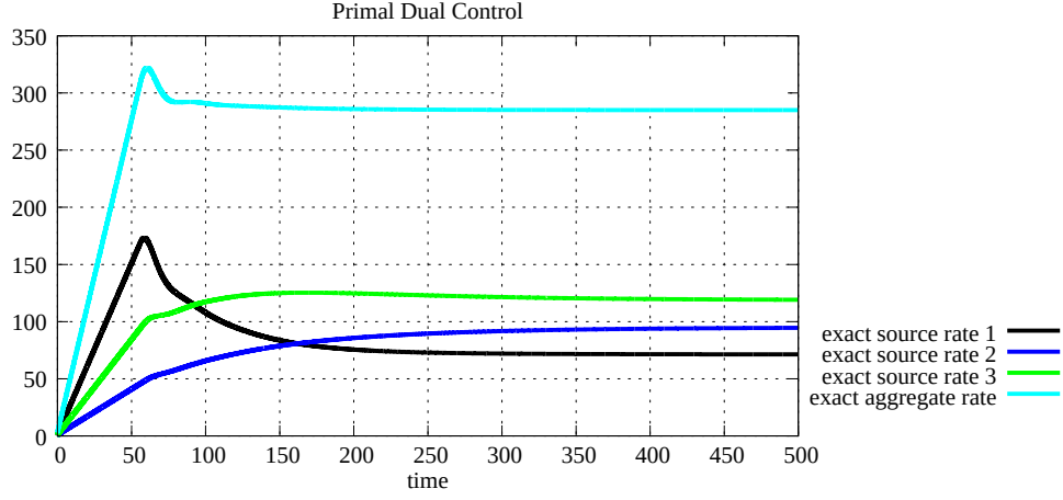
Figure 5.37: Source rates, simple case with 1 link and 3 sources (P D C)
