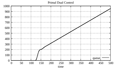
Figure A.46: Queue size, case 2 with 1 link and 1 source (P D C)
