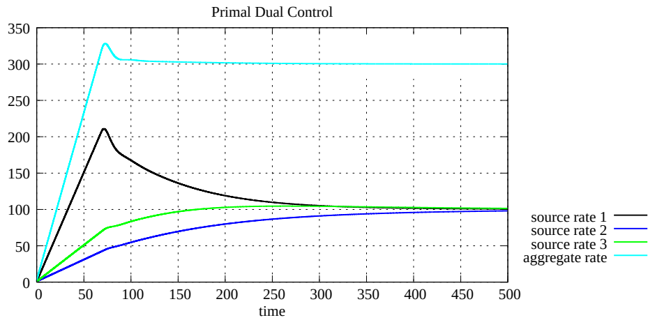
Figure A.53: Source rates, case 1 with 1 link and 3 sources (P D C)
