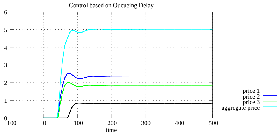
Figure A.98: Link price, case 2 with 3 links and 4 sources (C Q D)
