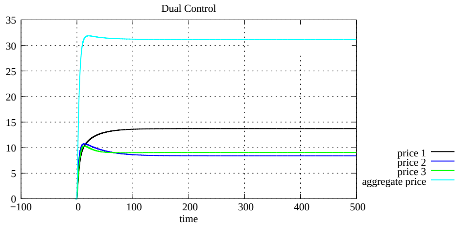
Figure A.27: Link price, case 3 with 3 links and 4 sources (Dual)
