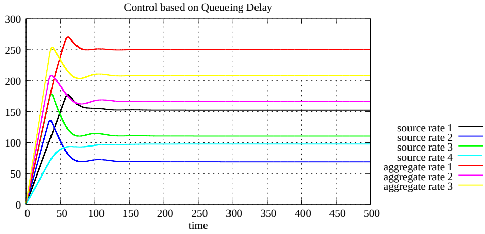
Figure A.103: Source rates, case 3 with 3 links and 4 sources (C Q D)
