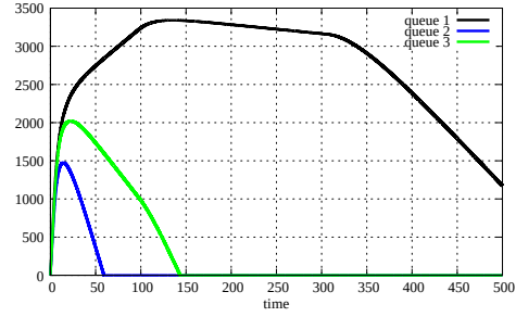
Figure 5.21: Queue sizes, case 2 with 3 links and 1 source (Dual)
