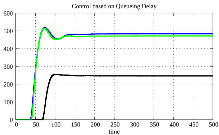
Figure 5.63: Queue sizes with 3 links and 4 sources (C Q D)
