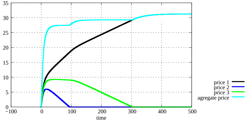
Figure 5.17: Link prices, case 2 with 3 links and 1 source (Dual)
