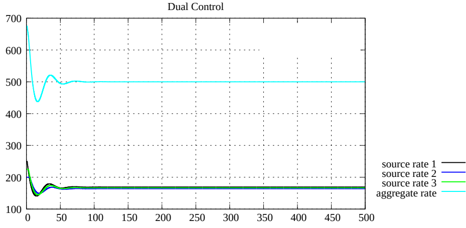
Figure A.17: Source rates, case 1 with 1 link and 3 sources (Dual)
