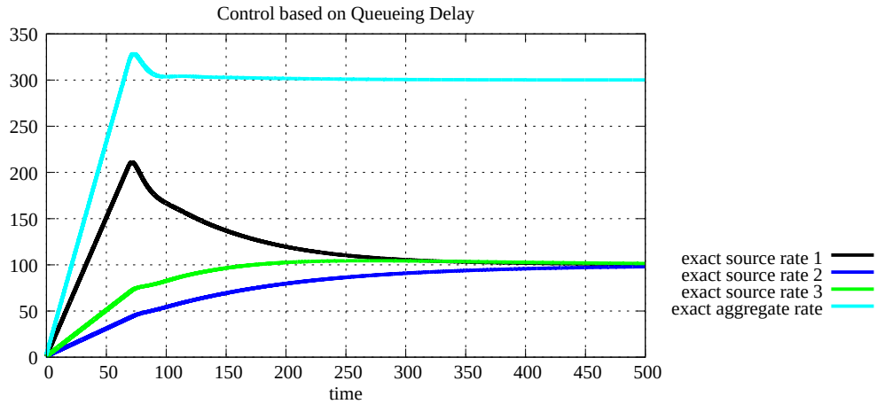
Figure 5.56: Source rates, fairness case with 1 links and 3 sources (C Q D)
