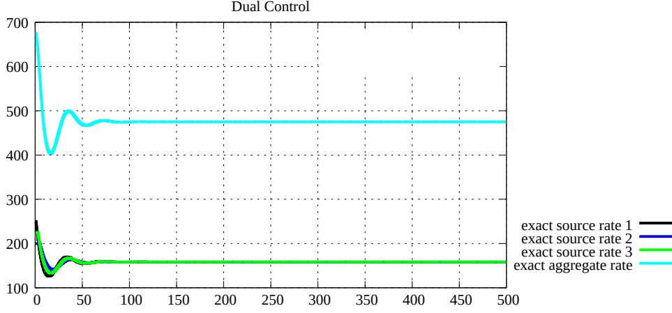
Figure 5.12: Source rates, fairness case with 1 links and 3 sources (Dual)
