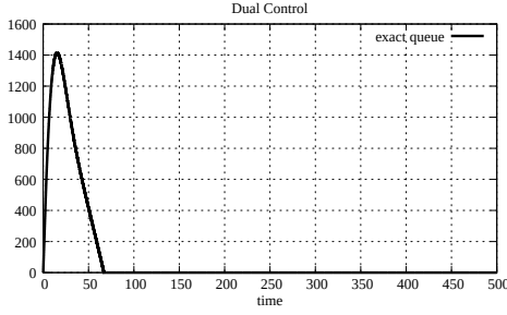
Figure 5.13: Queue size, simple case with 1 link and 3 sources (Dual)
