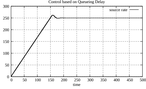
Figure A.79: Source rate, case 3 with 1 link and 1 source (C Q D)
