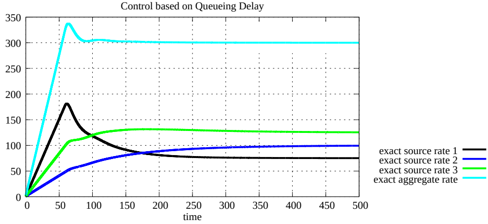
Figure 5.55: Source rates, simple case with 1 link and 3 sources (C Q D)
