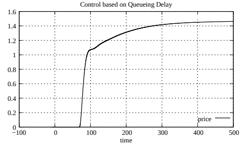
Figure A.86: Link price, case 2 with 1 link and 3 sources (C Q D)
