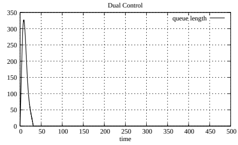
Figure A.12: Queue size, case 4 with 1 link and 1 source (Dual)
