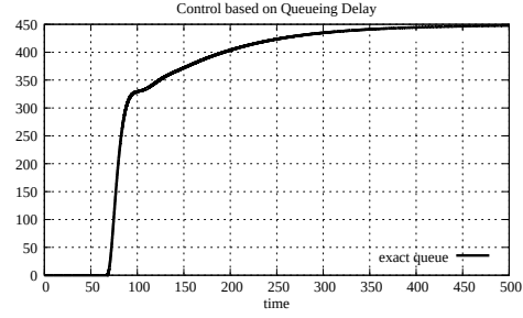
Figure 5.58: Queue size, fairness case with 1 link and 3 sources (C Q D)
