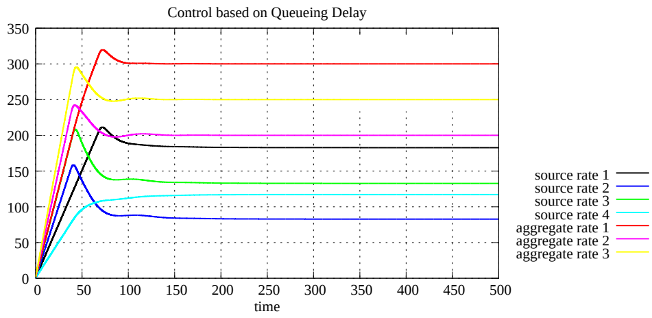
Figure A.101: Source rates, case 1 with 3 links and 4 sources (C Q D)
