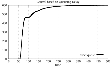
Figure 5.57: Queue size, simple case with 1 link and 3 sources (C Q D)
