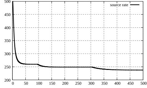
Figure 5.19: Source rate, case 2 with 3 links and 1 source (Dual)
