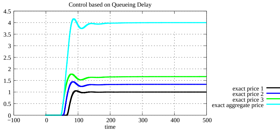
Figure 5.60: Link prices with 3 links (same capacity) and 4 sources (C Q D)
