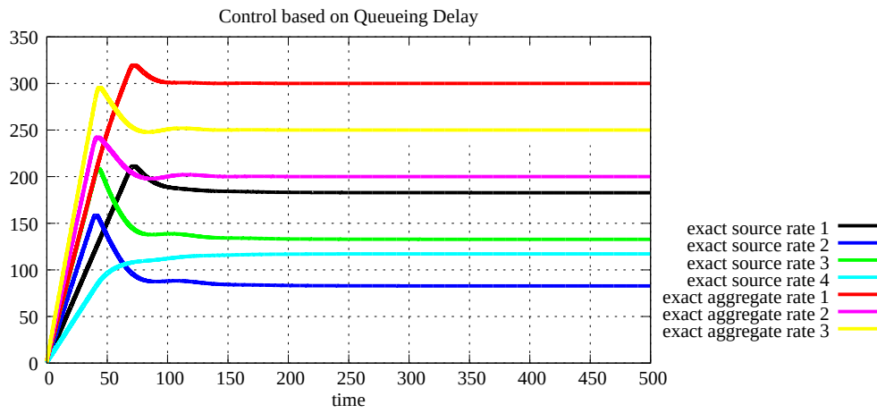
Figure 5.61: Source rates with 3 links and 4 sources (C Q D)
