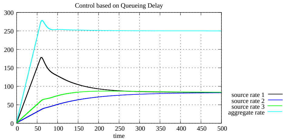
Figure A.91: Source rates, case 3 with 1 link and 3 sources (C Q D)
