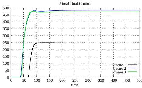
Figure A.69: Queue size, case 1 with 3 links and 4 sources (P D C)
