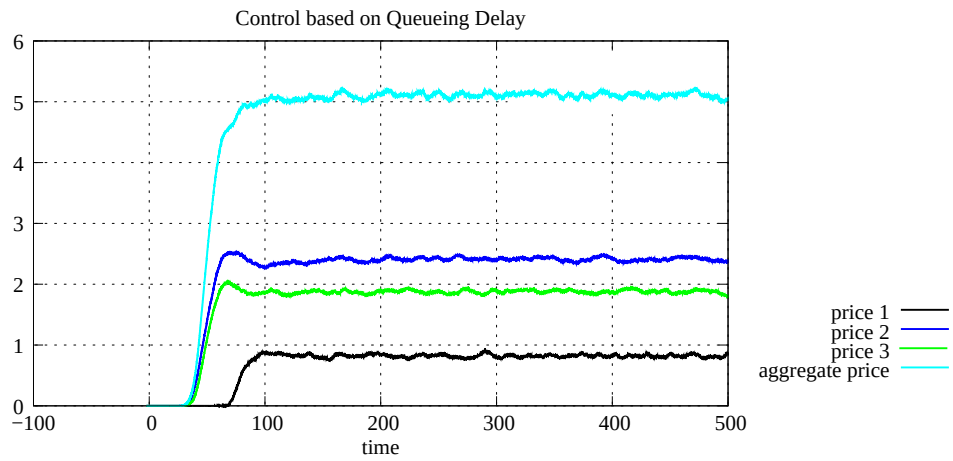
Figure A.100: Link price, case 4 with 3 links and 4 sources (C Q D)
