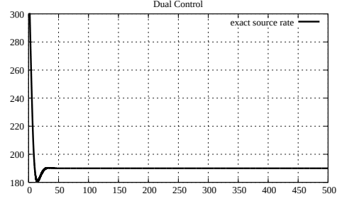
Figure 5.5: Source rate, case 2 with 1 link and 1 source (Dual)
