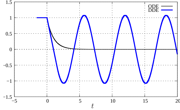
Figure 3.4: Ordinary and delay differential equations 3
