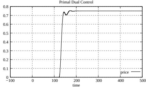
Figure A.37: Link price, case 1 with 1 link and 1 source (P D C)
