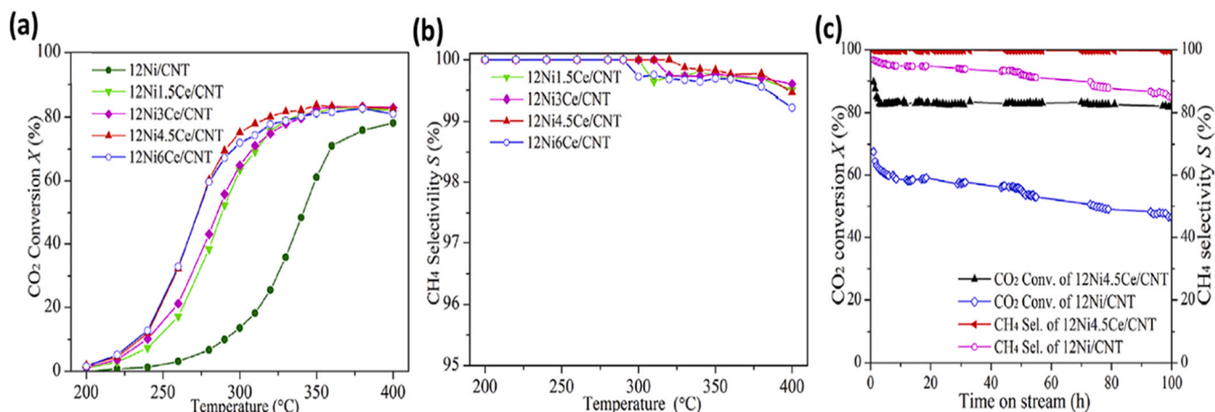
Fig. 2. (a) CO 2 conversion, (b) CH 4 selectivity as a function of temperature for different catalysts, and (c) The stability and CH 4 selectivity of 12Ni/CNT compared to 12Ni4.5Ce/CNT. Reproduced from [26] with permission of Elsevier.
