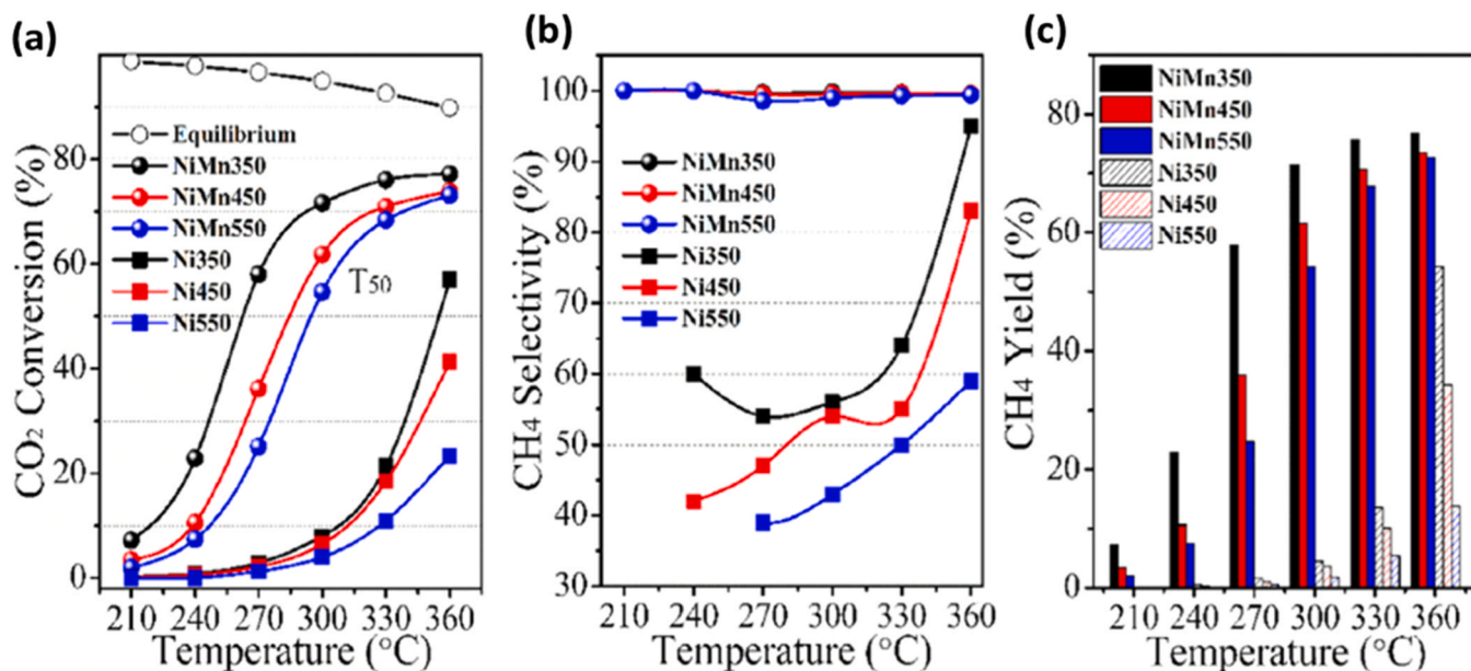
Fig. 4. CO 2 conversion (a), CH 4 selectivity (b), and CH 4 yield (c) for Ni and Mn-promoted Ni catalysts at atmospheric pressure, 100 mg catalysts, H 2 /CO 2 molar ratio = 4:1. Reproduced from [31] with permission of ACS.
