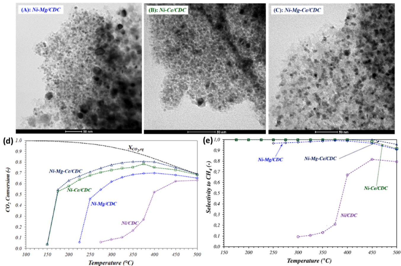
Fig. 9. TEM images of (a) Ni-Mg/CDC, (b) Ni-Ce/CDC, and (c) Ni-Mg-Ce/CDC. (d) CO 2 conversion and (e) CH 4 selectivity of all catalysts. Reproduced from [48] with permission of ACS.
