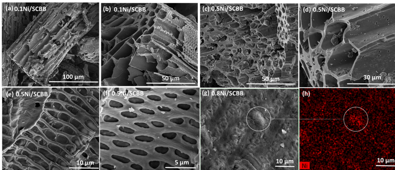
Fig. 7. (a–g) SEM images of different catalysts, and (h) nickel elemental mapping of 0.8Ni/SCBB. Reproduced from [50] with permission of Elsevier.
