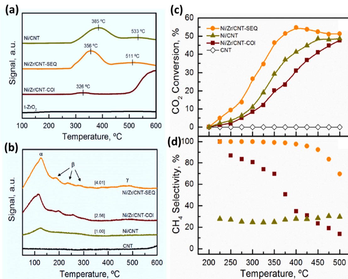
Fig. 3. (a) H 2 -TPR profiles, (b) CO 2 -TPD profiles, (c) CO 2 conversion, and (d) Selectivity to CH 4 , of Ni/Zr/CNT-SEQ. Reproduced from [27] with permission of Elsevier.
