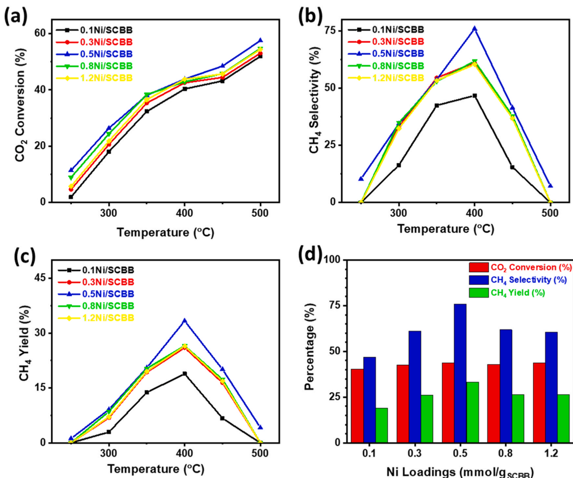
Fig. 8. (a) CO 2 conversion, (b) CH 4 selectivity, CH 4 yield of all Ni/SCB catalysts. Reproduced from [50] with permission of Elsevier.
