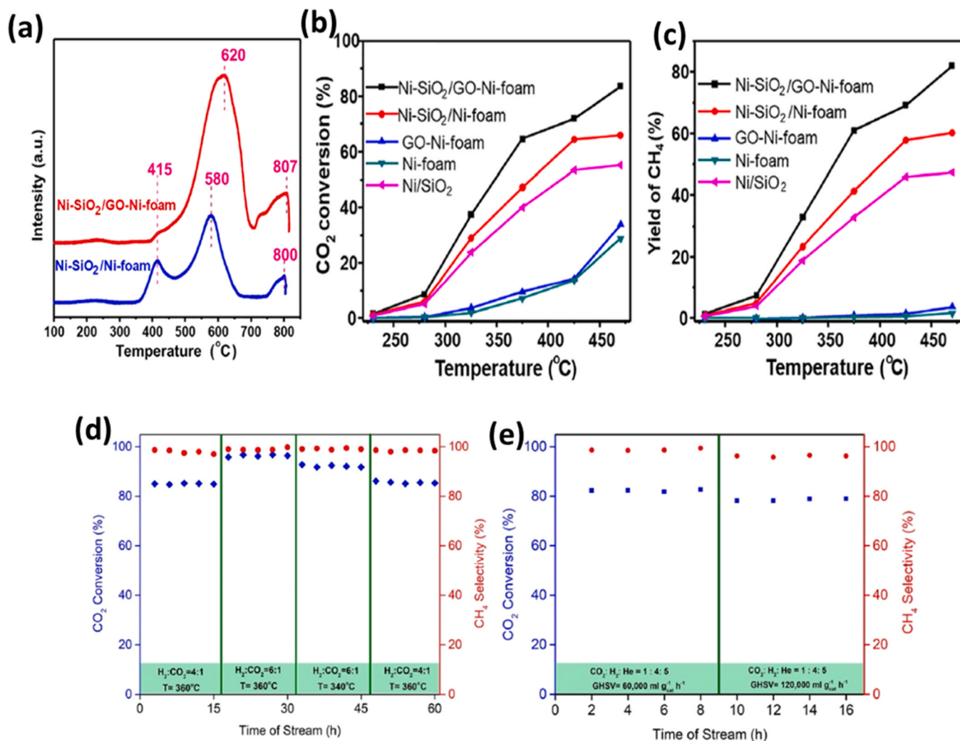
Fig. 6. (a) TPR profiles of Ni-SiO 2 /GO-Ni-foam, Ni-SiO 2 /Ni-foam catalysts, (b) CO 2 conversion and (c) CH 4 yield of different catalysts at 1.0 g cat., 0.1 MPa. GHSV = 500. Reproduced from [36] with permission of Elsevier.
