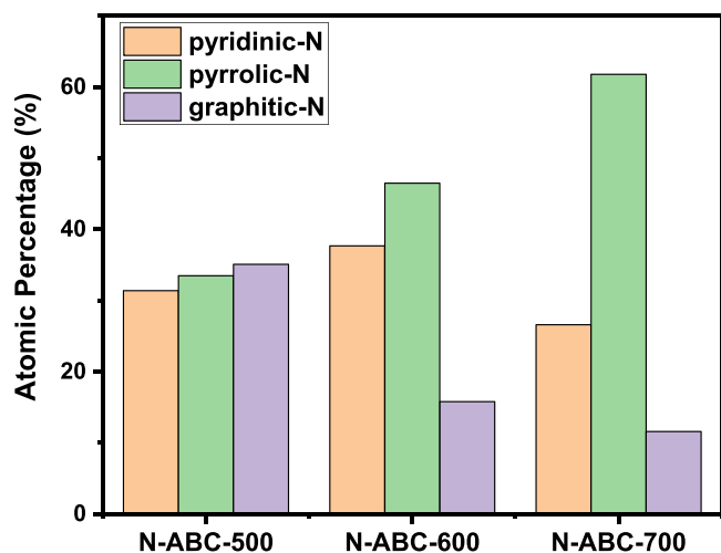
Fig. 10. Relative atomic percentages of the N-ABC supports, determined by XPS. Adapted from the surface analysis reported in reference [9].
