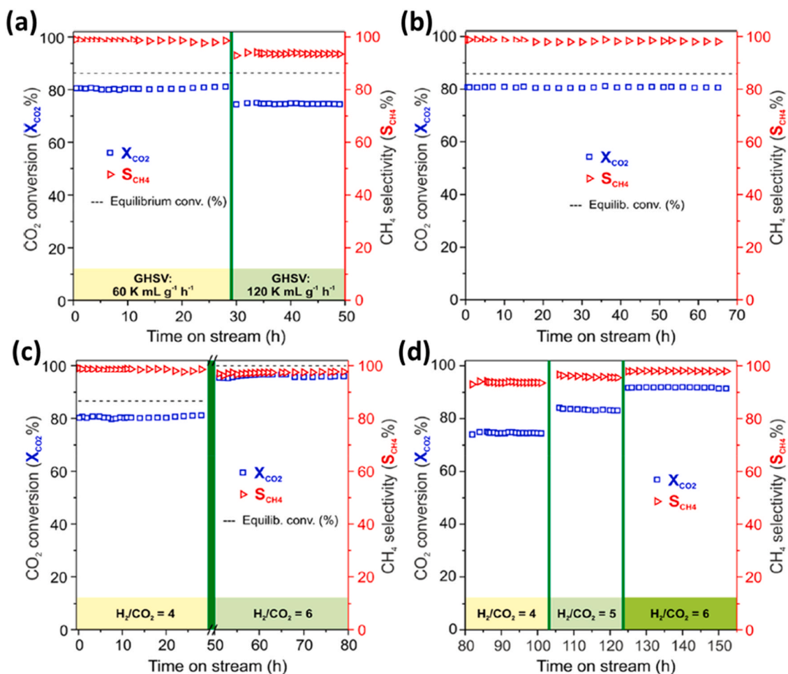
Fig. 5. (a) Effect of GHSV on the catalytic activity, (b) Long-term stability test at a GHSV of 60,000 mL g -1 h -1 , (c) Effect of H 2 /CO 2 ratio on the catalytic performance at a GHSV of 60,000 mL g -1 h -1 and (d) Effect of H 2 /CO 2 ratio on the catalytic activity at a GHSV of 120,000 mL g -1 h -1 . Reproduced from [32] with permission of ACS.
