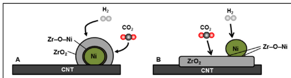
Scheme 1. The NiO, ZrO 2 and interface Ni-O-Zr in the surface of CNT for Ni-Zr-CNT-COI (A) and Ni-Zr-CNT-SEQ catalysts (B). Reproduced from [27] with permission of Elsevier.
