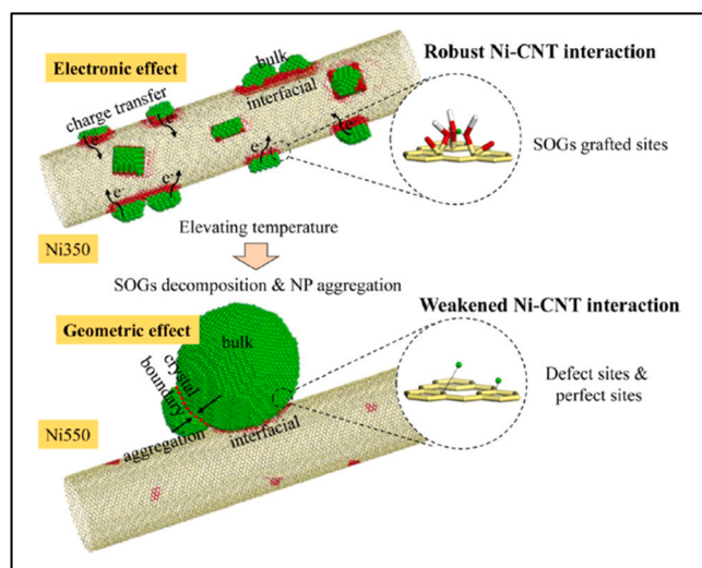
Scheme 2. The proposed mechanism accounting for the interaction between Ni and CNT. Reproduced from [31] with permission of ACS.
