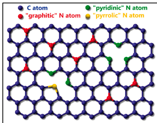
Scheme 3. Schematic representation of the N-doped graphene. Reproduced from [67] with the permission of ACS.
