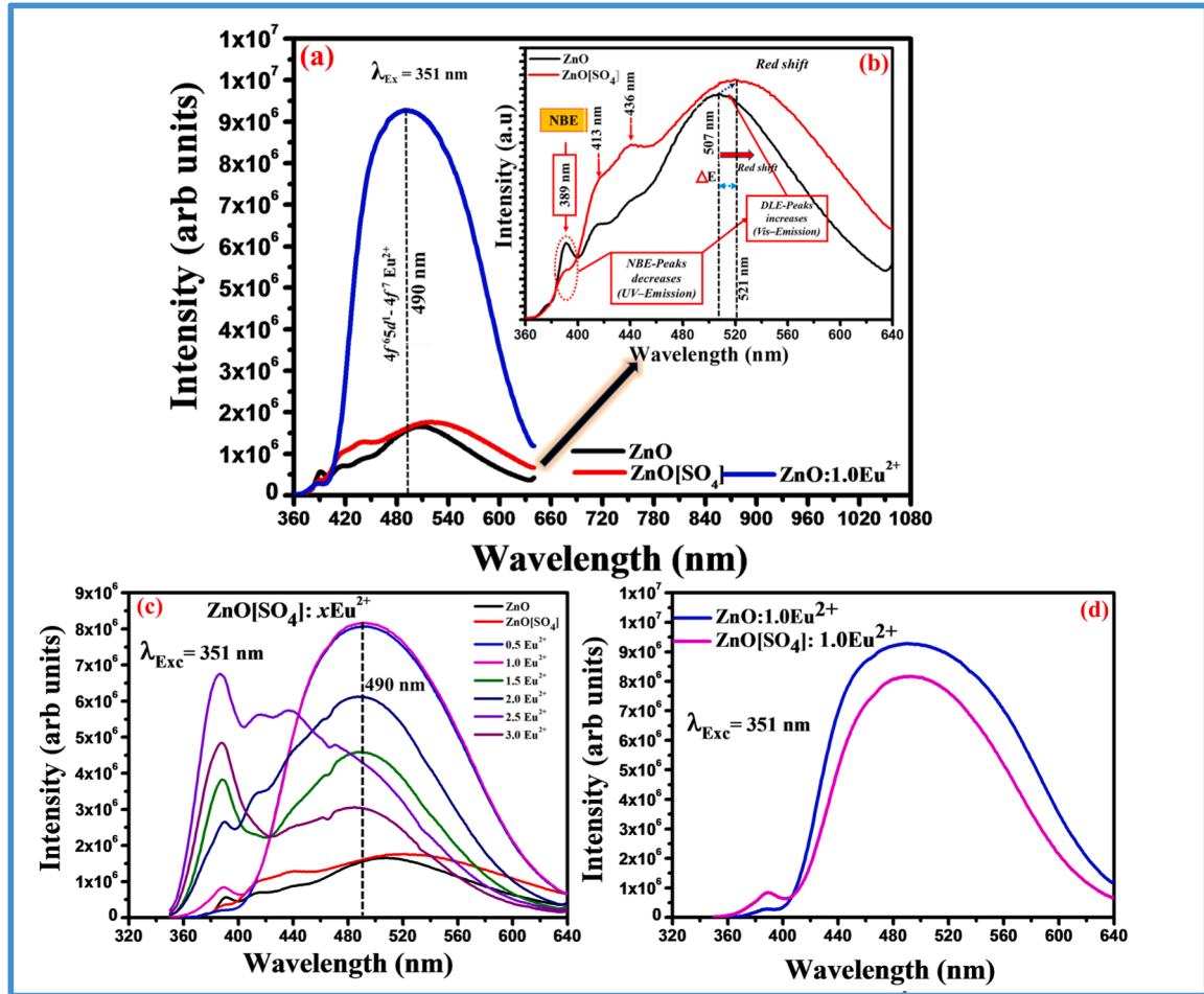
Fig. 8. PL spectra of (a) undoped, and SO 4 2- and 1 mol% Eu 2+ doped ZnO, (b) ZnO[SO 4 ] and ZnO (enlarged), (c) ZnO[SO 4 ]: Eu 2+ with varying content of Eu 2+ , and (d) ZnO:Eu 2+ (1 mol%) and ZnO[SO 4 ]:Eu 2+ (1 mol%).
