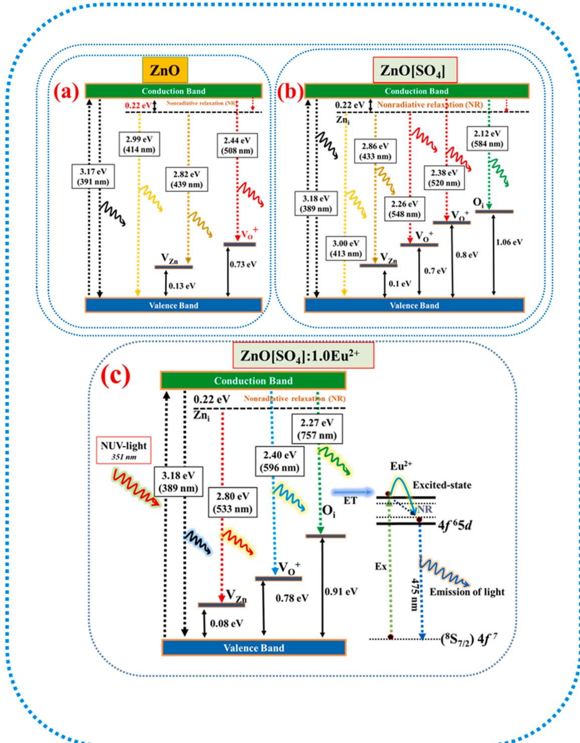
Fig. 11. Simplified energy level diagrams of light emission mechanisms based on deconvoluted PL emission spectrum of (a) ZnO, (b) ZnO[SO 4 ], and (c) ZnO[SO 4 ]:1.0Eu 2+ .
