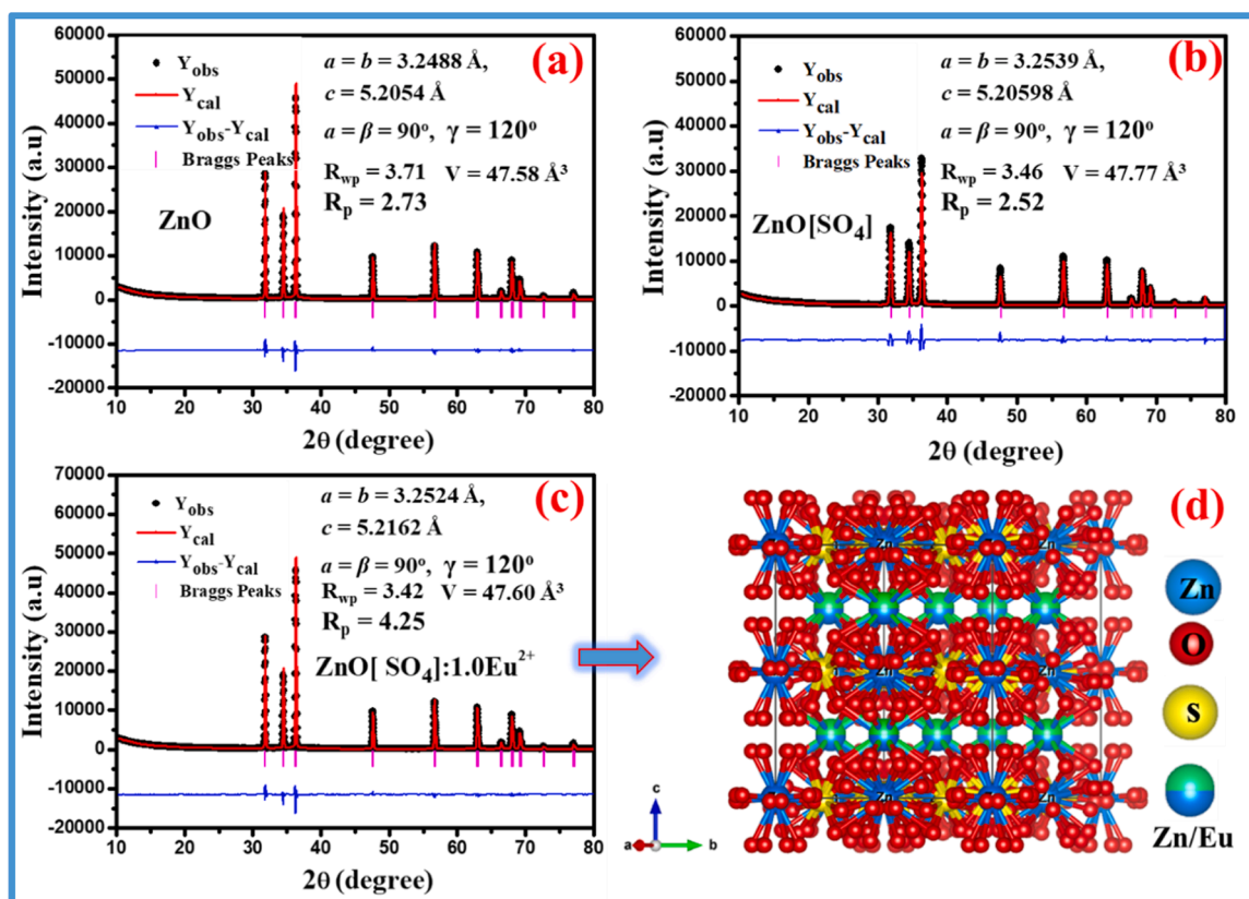
Fig. 2. (a) the Rietveld fits of (a) undoped, (b) \text{SO}_4^{2-} and (c) (1 mol%) \text{Eu}^{2+} doped ZnO crystal structures.
