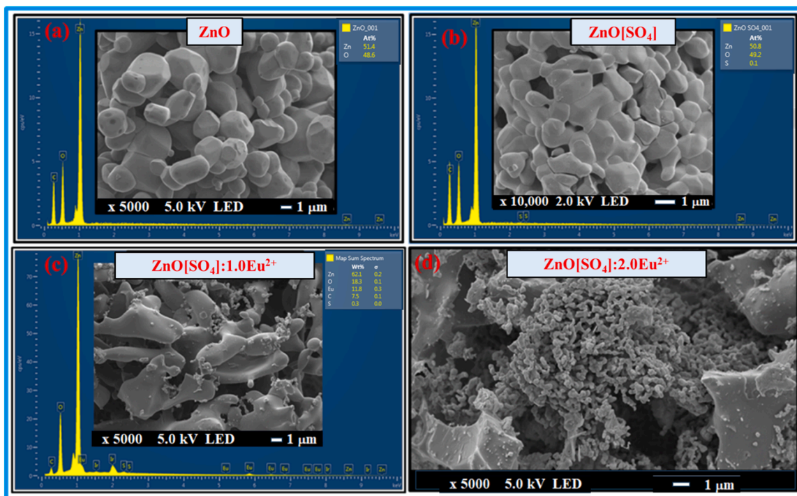
Fig. 3. (a–d) SEM images and (a–c) EDS spectra of ZnO, ZnO[SO 4 ], and Eu 2+ -doped ZnO[SO 4 ] phosphors sintered in argon/hydrogen atmosphere. The insets are weight percentages of the elements.
