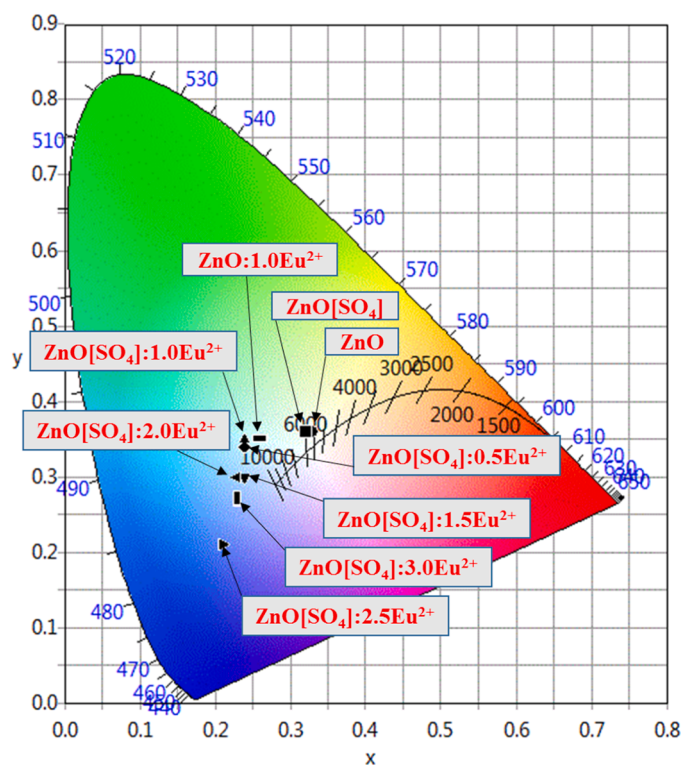
Fig. 13. (a) Schematic configuration coordinate diagram for \text{ZnO}[\text{SO}_4]:x\text{Eu}^{2+} and (b) ZnO, \text{ZnO}[\text{SO}_4] , \text{ZnO}:1.0\text{Eu}^{2+} and \text{ZnO}[\text{SO}_4]:x\text{Eu}^{2+} (where x = 0.5-3.0 ) phosphors CIE chromaticity diagram.
