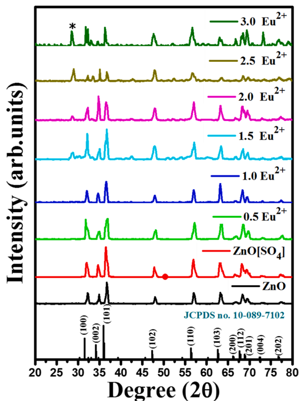
Fig. 1. X-ray diffraction spectra of undoped and \text{SO}_4^{2-} and (0.5 – 3 mol%) \text{Eu}^{2+} doped ZnO.
