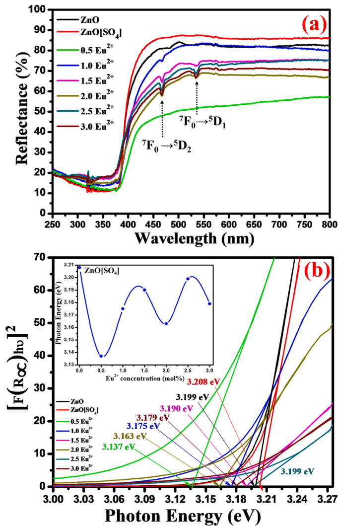
Fig. 7. (a) Diffuse reflectance spectra and the (b) Tauc plots from which the band gap energies were estimated.
