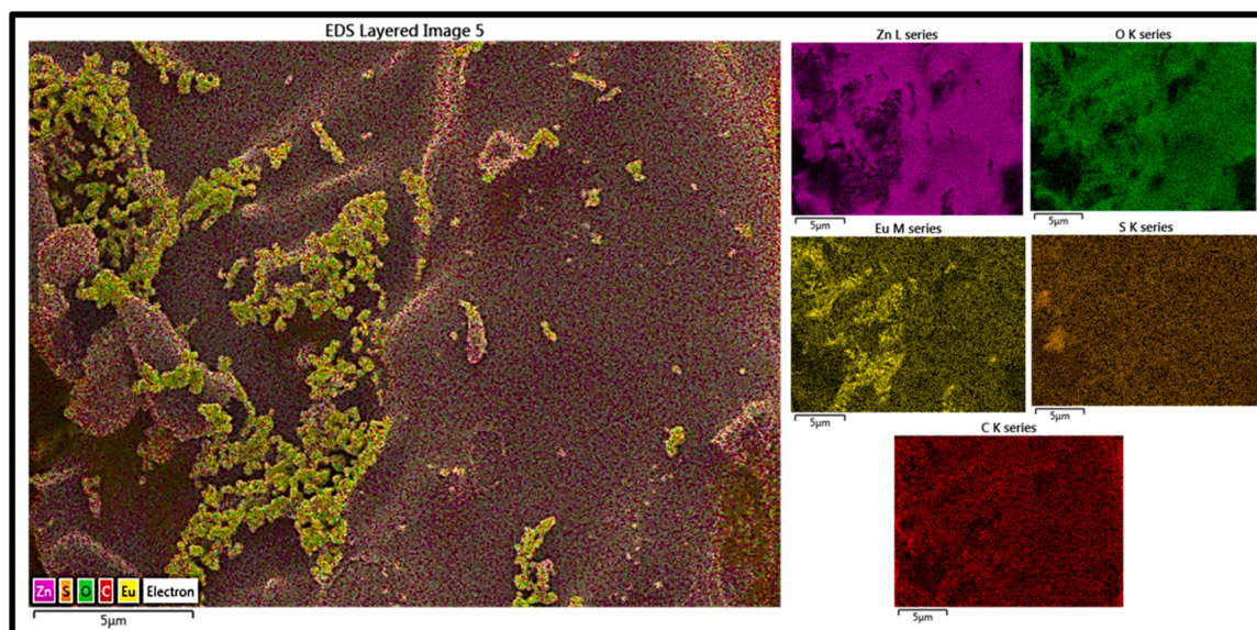
Fig. 4. EDS mapping of \text{ZnO}[\text{SO}_4]:1.0\text{Eu}^{2+} phosphor powder.
