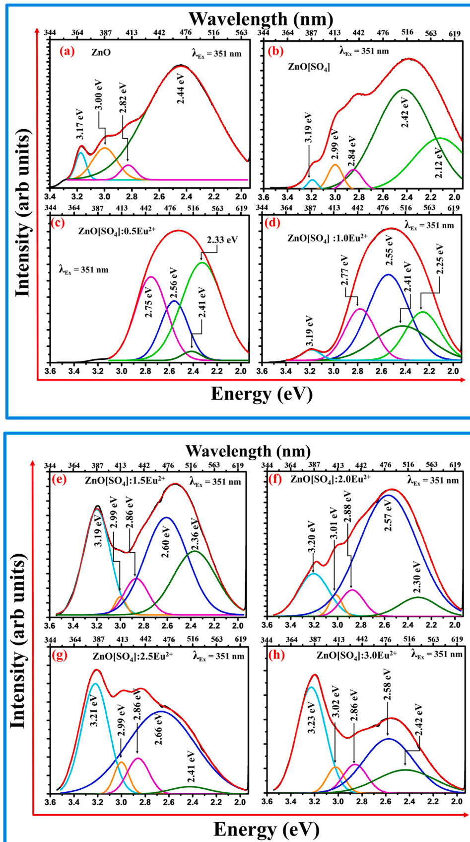
Fig. 9. (a)-(h): De-convoluted PL spectra of \text{SO}_4^{2-} and \text{Eu}^{2+} doped ZnO phosphors.
