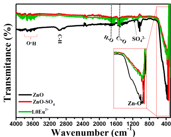
Fig. 5. FTIR spectra of undoped, \text{SO}_4^{2-} and (1 mol%) \text{Eu}^{2+} doped ZnO phosphors.
