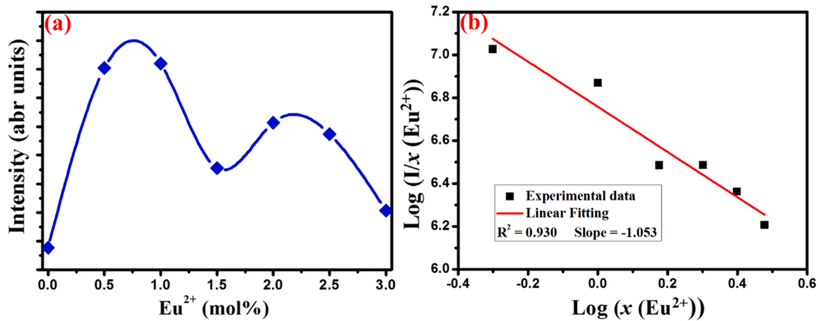
Fig. 10. (a) Intensity against \text{Eu}^{2+} concentration of \text{ZnO}[\text{SO}_4]:x\text{Eu}^{2+} (0–3.0 mol%) and (b) Linear fitting of \log(x(\text{Eu}^{2+})) against \log(I/x(\text{Eu}^{2+})) with different \text{Eu}^{2+} concentration for \text{ZnO}[\text{SO}_4]:\text{Eu}^{2+} phosphors.
