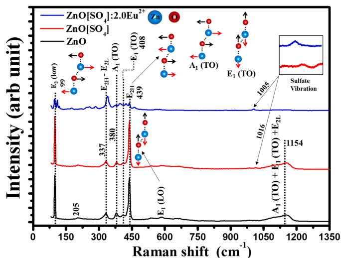
Fig. 6. Raman spectra of undoped, and \text{SO}_4^{2-} (2.0 mol%) and \text{Eu}^{2+} -doped ZnO phosphors.
