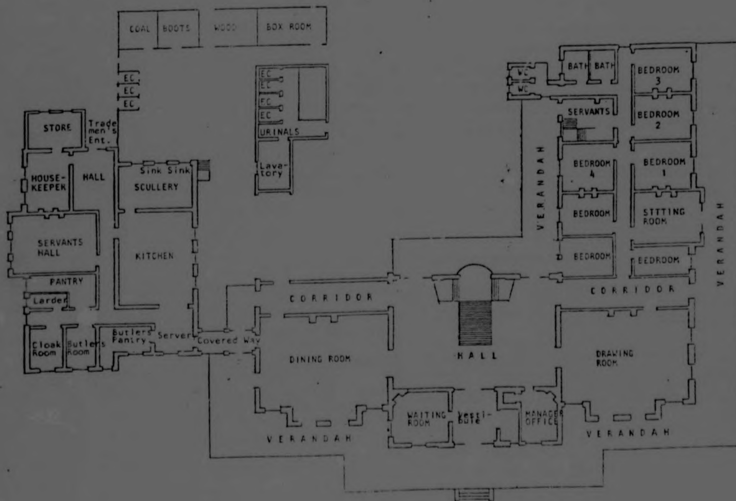
GROUND PLAN
