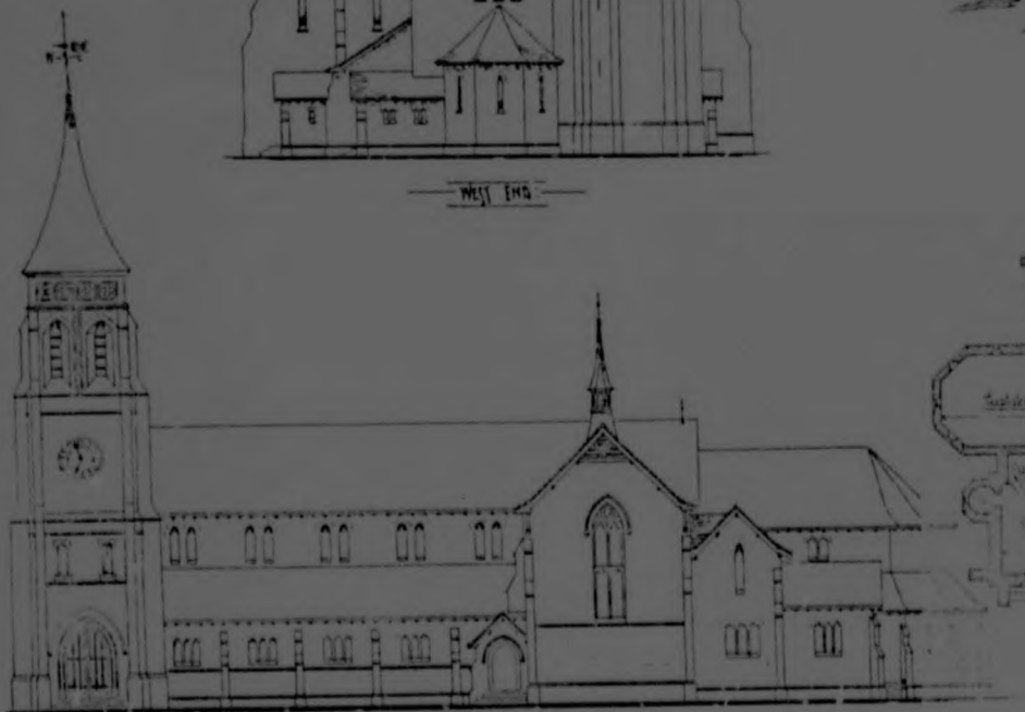
SOUTH ELEVATION
