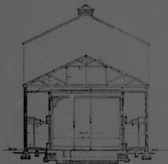
Section on line C.D.
