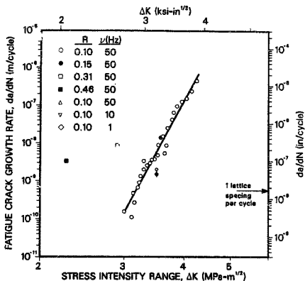
Figure 4.2 Variation of fatigue crack propagation rate, da/dN , with applied stress intensity range, \Delta K , for the low-toughened PSZ (MgO) ceramic, tested in room temperature air (45% relative humidity) at a load ratio R of 0.10 and a cyclic frequency of 50 Hz. Data for varying load ratio (0.10 - 0.46) and cyclic frequency (1 - 50 Hz) are included for comparison.
