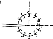
Figure 1.8 Crack tip dislocation configurations indicating (a) a screw dislocation off the symmetry plane of the crack, and (b) a circle of 2N - 1 dislocations around the crack tip.
