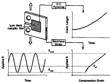
Figure 4.1 Schematic illustration of experimental techniques used to continuously monitor crack length and the stress intensity, K_{cl} , at fatigue crack closure.
