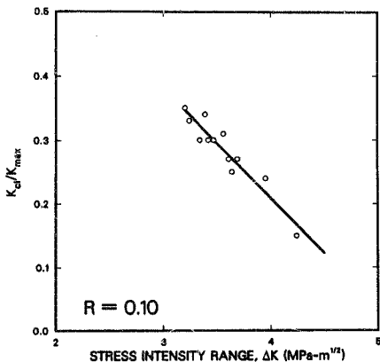
Figure 4.3 Experimentally measured variation of fatigue crack closure in PSZ (MgO), corresponding to cyclic crack growth rate data at R = 0.10 in Figure 4.2. Results, based on back-face strain compliance measurements, show the ratio of closure to maximum stress intensity, K_{cl}/K_{max} , as a function of the applied stress intensity range, \Delta K .
