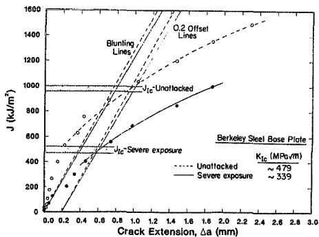
Figure 2.7 J_R(\Delta a) resistance curves for the 3Cr-1.5Mo steel indicating the effect of hydrogen attack on the crack initiation toughness J_{IC} .
