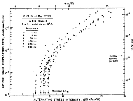
Figure 2.13 Influence of cyclic frequency (1 to 500 Hz) on fatigue crack propagation behavior in quenched and tempered fully bainitic 2.25Cr-1Mo steel (A542-3), tested at R = 0.1 in moist air (22).
