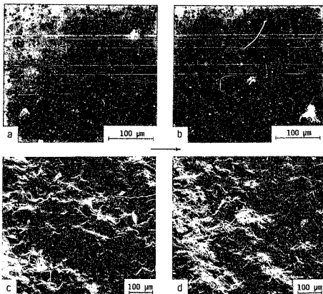
Figure 4.4 Fractography of crack growth in PSZ (MgO): optical micrographs of the fatigue crack path, showing (a) crack deflection and (b) crack bridging immediately behind the crack tip; scanning electron micrographs showing predominantly transgranular fracture surfaces associated with both (c) cyclically and (d) monotonically loaded cracks. Arrow indicates general direction of crack growth.
