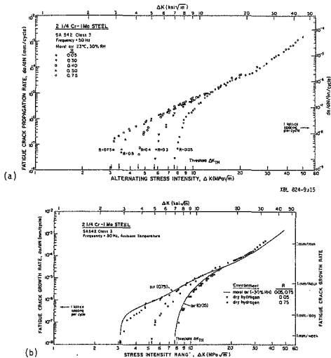
Figure 7.12 Fatigue crack propagation behavior of quenched and tempered 2.25Cr-1Mo A542-3 steel tested in (a) moist air and (b) dry gaseous hydrogen (138 kPa) at high frequencies (50 Hz), showing the influence of load ratio for R varying between 0.05 and 0.75 (7,10).
