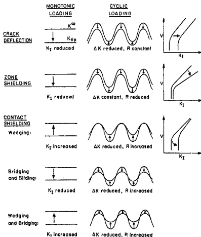
Figure 1.3 Effect of specific crack tip shielding mechanism of the "crack driving force", e.g., the stress intensity K_I , and crack velocity, v , under monotonic and cyclic loading.
