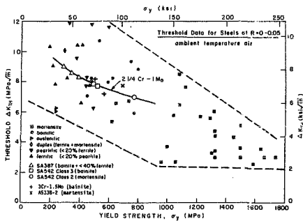
Figure 2.1 Variation of fatigue threshold stress intensity range, \Delta K_{TH} (at low load ratios), as a function of yield strength for a wide range of steels (8), showing results for the 2.25Cr-1Mo, 3Cr-Mo, and Mn-Mo-Ni steels in the present study.
