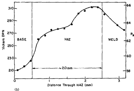
Figure 2.16 Microstructural and hardness characterization of the HAZ in the 3Cr-1.5Mo steel weldment, showing (a) a representative optical micrograph indicating the finer bainitic microstructure of the HAZ, and (b) the Vickers microhardness variation through the same region.
