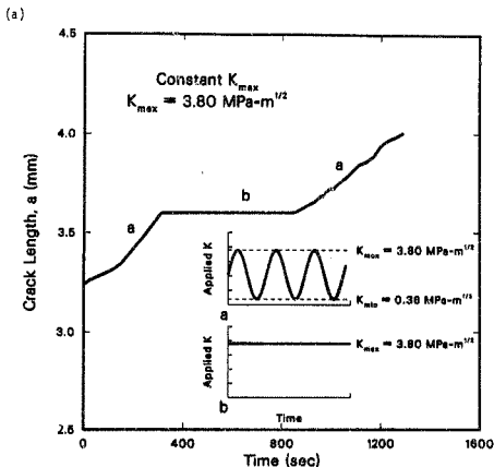
Figure 4.5 Effect in PSZ (MgO) of (a) sustained and cyclic loading conditions on crack growth rate, da/dN , at constant K_{max} ( = 3.8 \text{ MPa}/\sqrt{\text{m}} ), (b) varying cyclic frequency on crack growth rate, da/dN , and crack velocity, da/dt , at constant \Delta K ( = 3.5 \text{ MPa}/\sqrt{\text{m}} ), and (c) varying applied stress intensity range, \Delta K , on crack velocity, da/dt , at constant K_{max} ( = 4.2 \text{ MPa}/\sqrt{\text{m}} ).
