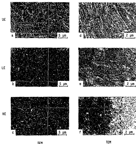
Figure 3.1 Microstructure of A533B steel in the unexposed (UE) and hydrogen pre-exposed (LE and NE) conditions. Micrographs on the left are from SEM of polished surfaces (etched in 2% nital); on the right from TEM of thin foils.
