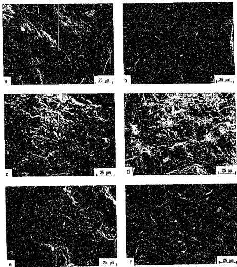
Figure 3.12 Scanning electron micrographs of fatigue fracture surfaces at near-threshold and higher growth rates in A533B steel, for varying degrees of grain boundary microvoid damage, showing UE structure at (a) \Delta K = 8 MPa \sqrt{m} and (b) \Delta K = 30 MPa \sqrt{m} ; NE structure at (c) \Delta K = 7 MPa \sqrt{m} and (d) \Delta K = 29 MPa \sqrt{m} ; and SE structure at (e) \Delta K = 7 MPa \sqrt{m} and (f) \Delta K = 26 MPa \sqrt{m} . Arrows indicate general direction of crack growth.
