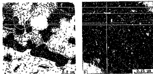
Figure 3.2 Typical carbide morphologies in the unexposed A533B steel showing the coarse interlath and grain boundary Fe-rich MgC and fine needle-shaped intralath (Mo rich + Fe) M_2C carbides. (TEM carbon extraction replica.)
