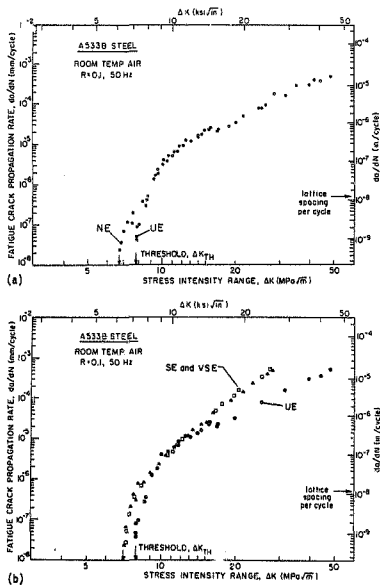
Figure 3.11 Fatigue crack propagation ( da/dN ) behavior as a function of the nominal stress intensity range ( \Delta K ) in A533B steel at R = 0.1 . Both (a) mild degrees (NE) and (b) severe degrees (SE and VSE) of pre-existing grain boundary microvoid formation have only a small influence on crack propagation rates, compared to behavior in the undamaged (UE) condition (after ref. 10).
