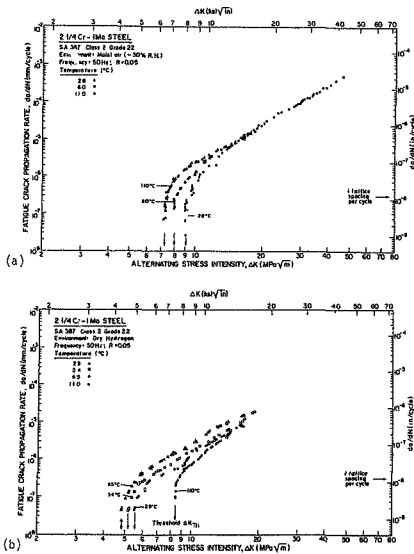
Figure 2.14 Influence of temperature (28-110°C) on fatigue crack propagation behavior in normalized ferritic-bainitic 2.25Cr-1Mo steel (A387-2-22), tested at R = 0.05 in (a) moist air and (b) dry gaseous hydrogen (138 kPa) (14).
