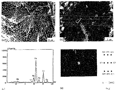
Figure 3.4 Severely cavitated intergranular fracture surface from fracture toughness test on A533B following NE. (a) SEM micrograph, (b) TEM of fracture surface extraction replica, and identification of particles using EDS and SAD in (c) and (d), respectively.
