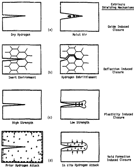
Figure 2.20 Schematic illustration of micro-mechanisms of crack tip shielding relevant to the present study, showing wedge shielding from (a) oxide-induced closure, and (b) deflection and roughness-induced closure, and zone shielding from (c) plasticity-induced closure and (d) from compressive zones around the crack due to the dilatant growth of methane bubbles (in situ hydrogen attack).
