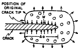
Figure 3.A1 Schematic illustration of a crack surrounded by a constrained dilatant zone: tractions give rise to an internal pressure resulting from the dilatant strain of void formation.
