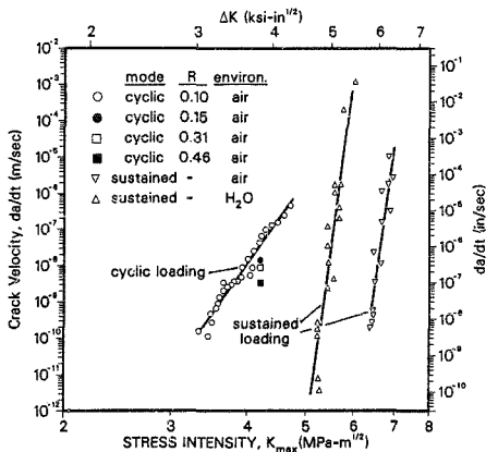
Figure 4.10 Subcritical crack growth behavior in PSZ (MgO) showing a comparison of cyclic crack velocities, da/dt , from the present study with sustained-load cracking data of Becher (6,7) for 55% relative humidity air and distilled water. Note how fatigue-induced crack growth is much faster than environmentally-assisted crack growth under monotonic loading conditions.
