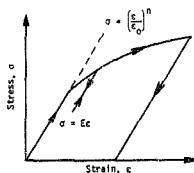
Figure 5.2 Schematic illustration of non-linear behavior of material in the process zone of transformation toughened ceramics compared to that of conventional monolithic ceramics.
