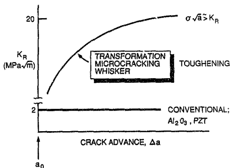
Figure 5.1 Resistance curve behavior illustrating the increase in fracture resistance with crack advance typically encountered in toughened ceramics.
