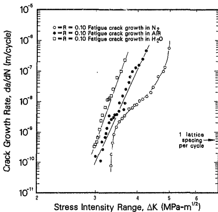
Figure 4.6 Fatigue crack propagation behavior of the low-toughened PSZ indicating the influence of an inert (dry nitrogen), (45% RH) air and corrosive (distilled water) environment at a frequency of 50 Hz and R = 0.10 .
