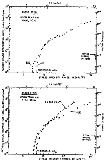
Figure 2.9 Fatigue crack propagation behavior of a bainitic Mn-Mo-Ni nuclear pressure vessel steel (A533B-2), tested at R = 0.10 , showing influence of prior damage from hydrogen attack. Results are given for the unexposed (UE) condition, and following 240 hr (NE), 1096 hr (SE), and 1480 hr (VSE) exposures to gaseous hydrogen at 13.8–17.2 MPa pressure (550–600°C) (13,20).
