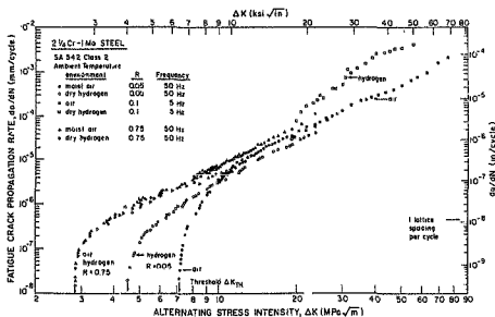
Figure 2.4 Fatigue crack propagation behavior of a quenched and tempered fully martensitic 2.25Cr-1Mo steel (A542-2), showing the influence of moist air and dry gaseous hydrogen (138 kPa) environments at low and high frequencies at R=0.05 and 0.75 (7,9,12).
