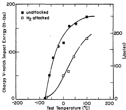
Figure 2.6 Charpy V-notch transition curves for the 3Cr-1.5Mo steel showing the effect of microstructural damage from exposure to high temperature/pressure hydrogen environments.
