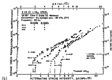
Figure 2.15 Fatigue crack propagation behavior in a thick-section weldment of normalized 2.25Cr-1Mo steel, (A387-2-22), showing comparison of growth rates in base plate, HAZ and weld metal microstructures in (a) moist air and (b) dry gaseous hydrogen (138 kPa) at R = 0.05 and 0.80 (*).
