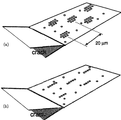
Figure 3.10 Extent of void clusters intersected by the crack plane in the (a) S-T, and (b) L-T orientations.
