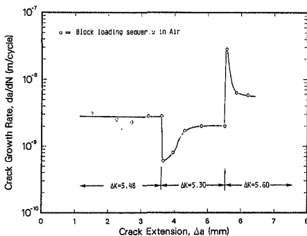
Figure 4.9 Variation of fatigue crack propagation rate ( da/dN ) showing the effect of constant \Delta K = 5.48 MPa \sqrt{m} , and following block loading sequences. Note the transient retardation following the high-low sequence, and the transient acceleration following the low-high sequence.
