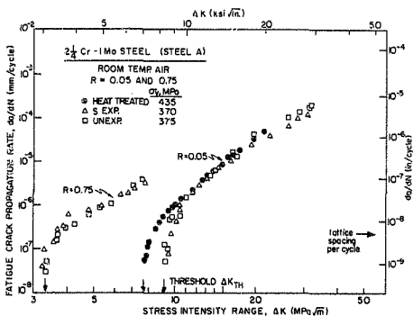
Figure 2.5 Fatigue crack propagation behavior for a normalized ferritic-bainitic 2.25Cr-1Mo steel (A387-2-22), at load ratios of R = 0.05 and 0.75 , showing influence of prior 1000 hr exposure to gaseous hydrogen at 13.8 MPa pressure (550°C). Results are for heat treated (HT), hydrogen attacked (SE), and unexposed (UE) conditions (13).
