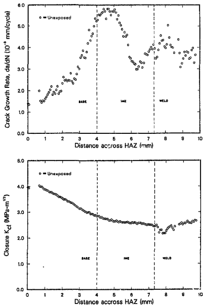
Figure 2.19 Fatigue crack propagation behavior of the JSW steel weldment showing (a) the variation of the crack growth rate ( da/dN ) as a function of the distance through the HAZ at a constant \Delta K = 12 \text{ MPa}\sqrt{\text{m}} , and (b) the level of crack closure.
