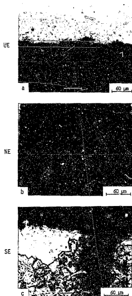
Figure 3.14 Near-threshold crack path morphologies, obtained in A533B steel from nickel-plated fracture surfaces, showing linear crack paths in (a) undamaged (UE) and (b) voided (NE) microstructures, and highly tortuous crack path in (c) extensively voided (SE) microstructure. Arrows indicate general direction of crack advance.
