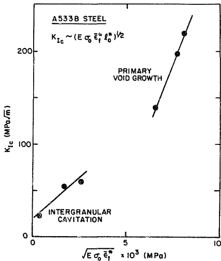
Figure 3.8 Plot of fracture toughness K_{Ic} as a function of (E \sigma_0 \bar{\epsilon}_f^*)^{0.5} , showing two discrete regimes of toughness behavior, namely primary void growth at high toughness levels and intergranular cavitation at low toughness levels.
