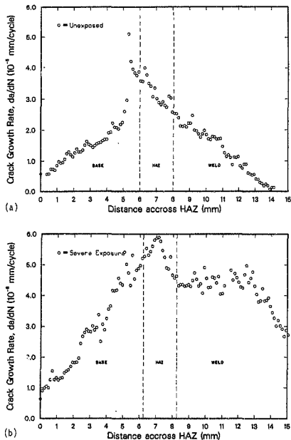
Figure 2.18 Fatigue crack propagation behavior of the 3Cr-1.5Mo steel weldment showing the variation of the crack growth rate ( da/dN ) as a function of the distance through the HAZ at a constant \Delta K = 12 \text{ MPa}\sqrt{\text{m}} , both (a) prior to, and (b) after the introduction of microstructural damage associated with hydrogen attack.
