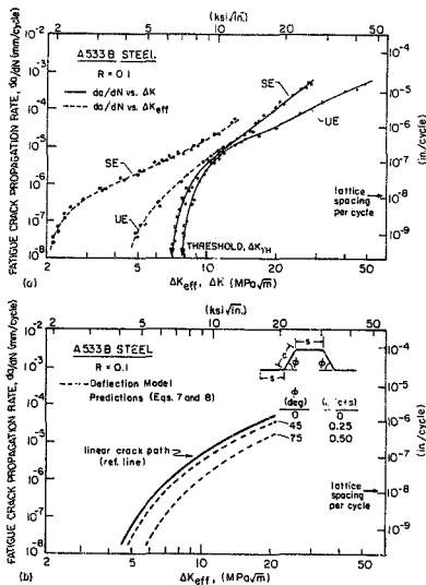
Figure 3.15 Respective roles of crack closure and crack deflection in influencing fatigue crack propagation in undamaged (UE) and extensively voided (SE) A533B steel, showing (a) experimental da/dN versus nominal \Delta K data (from Figure 3.11) corrected for closure for da/dN versus \Delta K_{eff} data, using experimental K_{CI} measurements; and (b) predictions of the effect of crack deflection using two-dimensional linear elastic deflection model (Eqns. 3.7 and 3.8) for \phi = 45 to 75 deg with c/(c+s) = 0.25 to 0.5 .
