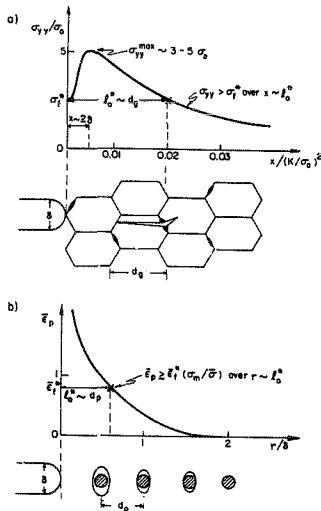
Figure 1.1 Schematic idealization of microscopic fracture criteria pertaining to (a) critical stress-controlled model for cleavage fracture (RKR), and (b) stress-modified critical strain-controlled model for microvoid coalescence. Such models provide a micro-mechanical description of intrinsic toughness. \sigma_I^* and \bar{\epsilon}_I^* are the critical fracture stress and critical equivalent plastic strain, respectively, and l_0 the characteristic distance.
