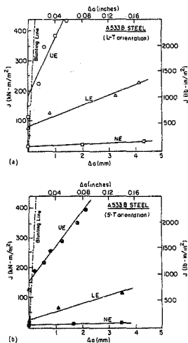
Figure 3.5 J_R(\Delta a) resistance curves for the undamaged (UE) and grain boundary voided (LE and NE) conditions in A533B steel tested in the (a) L-T and (b) S-T orientations. Tests on C(T) specimens are used to determine the crack initiation fracture toughness, K_{IC} and J_{IC} , and the tearing modulus, T_R .
