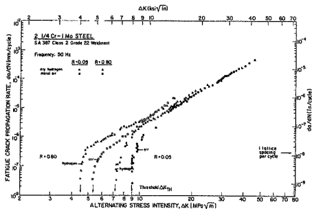
Figure 2.2 Fatigue crack propagation behavior of a normalized (thick-section) ferritic-bainitic 2.25Cr-1Mo steel (A387-2-22), showing the influence of moist air and dry gaseous hydrogen (138 kPa) environments at R=0.05 and 0.80 (6,14).
