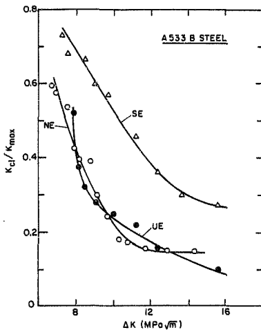
Figure 2.10 Experimentally measured variation in fatigue crack closure in A533B-2 steel corresponding to growth rate data in Figure 2.9. Results show the ratio of closure to maximum stress intensity, K_{cl}/K_{max} , as a function of \Delta K , and indicate higher levels of crack tip shielding in the severely hydrogen attack damage microstructure (SE) (13).
