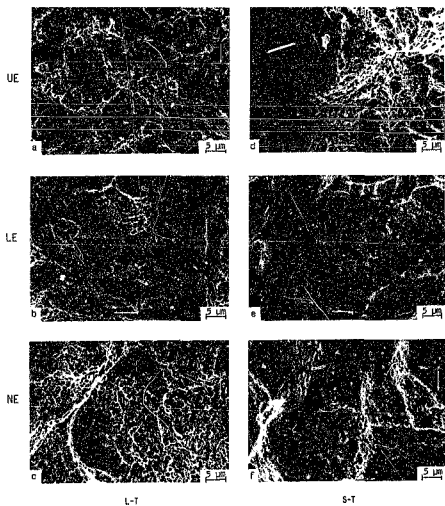
Figure 3.6 SEM fractographs of broken C(T) specimens in the unexposed UE and hydrogen exposed LE and NE conditions. Note the increasing incidence of methane bubble formation on grain boundaries with increasing hydrogen exposure. Arrows indicate general direction of crack growth.
