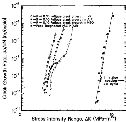
Figure 4.8 Variation of the fatigue crack propagation rate ( da/dN ) with applied stress intensity range \Delta K for the peak-toughened PSZ material. Results for the low-toughened material are included for comparison.
