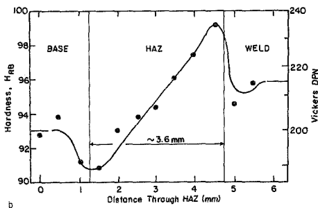
Figure 2.17 Microstructural and hardness characterization of the HAZ in the JSW steel weldment, showing (a) a representative optical micrograph indicating the finer bainitic microstructure of the HAZ, and (b) the Vickers microhardness variation through the same region.
