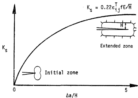
Figure 1.6 Variation of shielding with extension of the transformation zone into the wake of a stably advancing crack showing the initial frontal zone and the steady-state zone. R-curve behavior for intermediate zone sizes is predicted.
