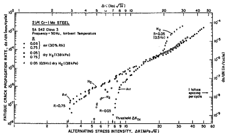
Figure 2.3 Fatigue crack propagation behavior of a quenched and tempered (thick-section) fully bainitic 2.25Cr-1Mo steel (A542-3), showing the influence of moist air and dry gaseous hydrogen (138 kPa) environments at low and high frequencies at R=0.05 and 0.75 (7,12).
