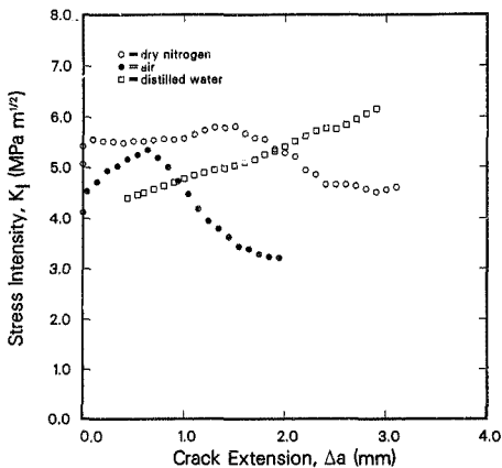
Figure 4.7 K_R(\Delta a) resistance curves from fracture toughness tests indicating the effect of environment on the maximum toughness achieved.
