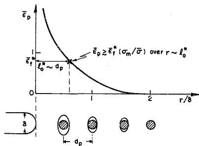
Figure 3.7 Schematic illustration of the stress-modified critical strain model for ductile fracture by microvoid coalescence.
