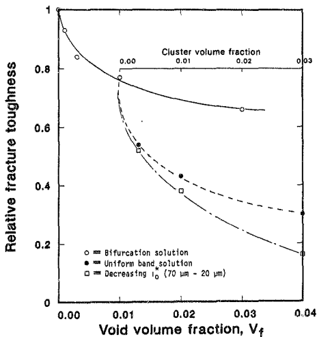
Figure 3.9 Predicted trends of the relative intrinsic toughness of an elastic-plastic solid with increasing background void volume fraction, V_f (solid line), microvoid cluster volume fraction above the background V_f of 0.01 (upper broken line), and the additional effect of decreasing the characteristic distance l_0 (lower broken line).
