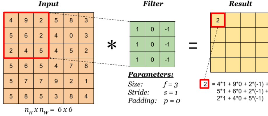
Figure 3.4: Structure of Convolutional Layer
