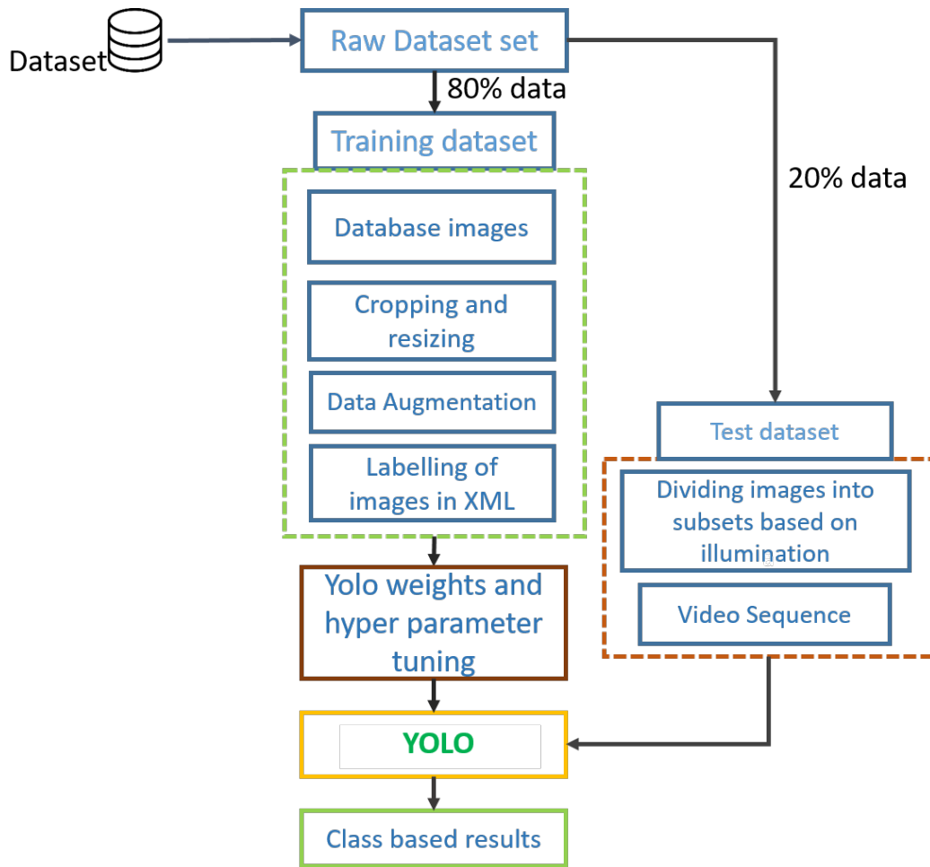
Figure 6.8: Framework of Yolo implementation
