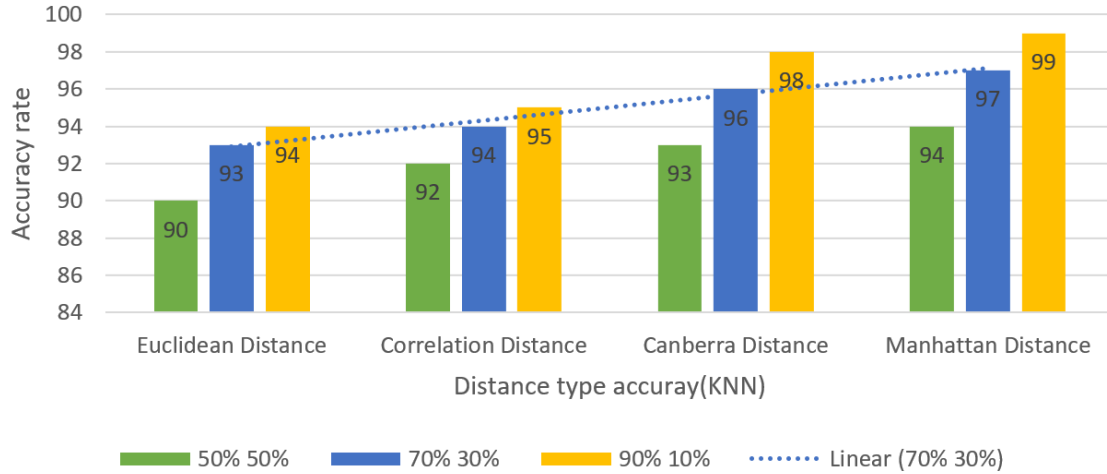
Figure 7.1: Accuracy with different distance method in KNN
