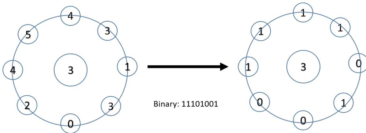
Figure 5.2: Local binary Pattern Histogram (LBPH) calculation for feature extraction
