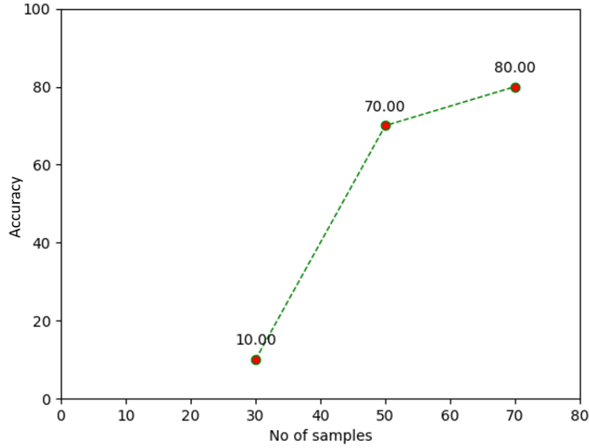
Figure 7.6: Accuracy results for subset 4 using LBPH with KNN
