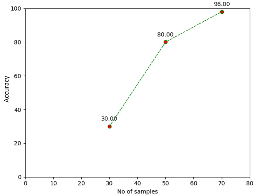
Figure 7.4: Recognition accuracy result of subset 2 using LBPH and KNN Image with 13^{\circ} to 25^{\circ} where the lighting angle is described as well illuminated image
