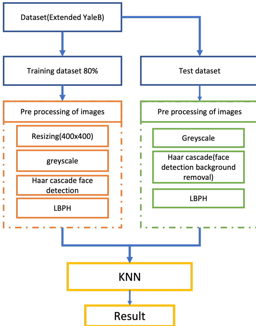
Figure 6.6: LBPH and KNN implementation
