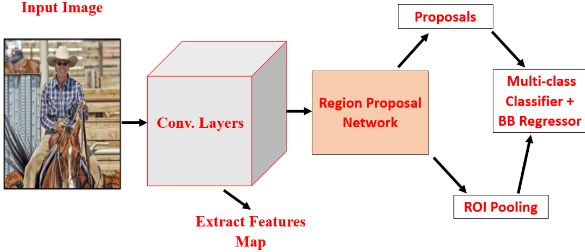
Figure 5.4: Region based Neural network Illustration
