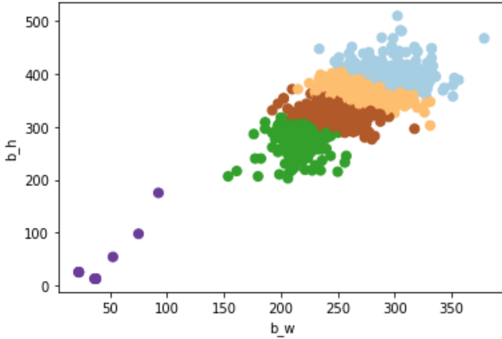
Figure 6.12: K mean clustering using k=5
