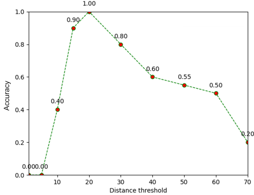
Figure 7.2: Recognition accuracy of LBPH with KNN with different K values
