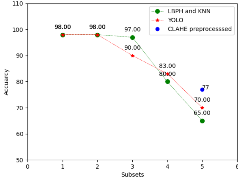
Figure 7.14: Combined results for a)LBPH with KNN 2)YOLO 3) YOLO using Clahe for preprocessing
