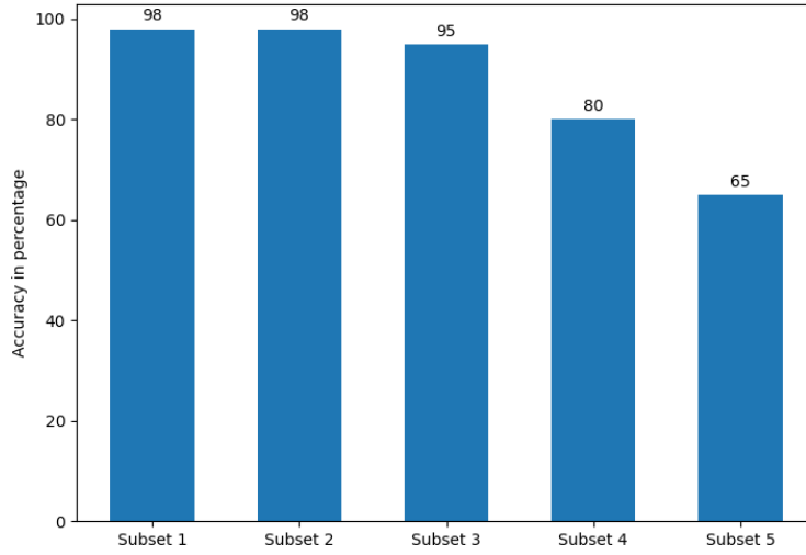
Figure 7.8: Results of LBPH with KNN considering all subsets Subset 1 is best illumination and subset 5 is represented as low illumination.
