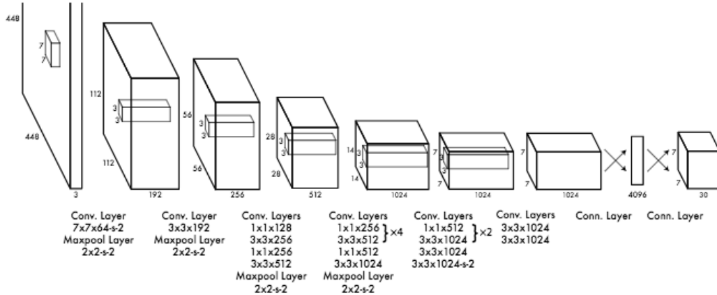
Figure 5.6: YOLO Architecture [7]
