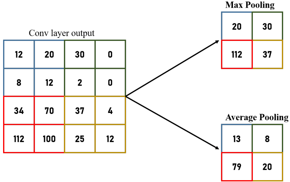
Figure 3.5: Schematic representation of max and average Pooling with filter 2 \times 2 with stride 2
