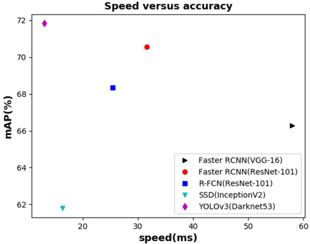
Figure 2.4: Speed (ms) versus accuracy (mAP) [5]
