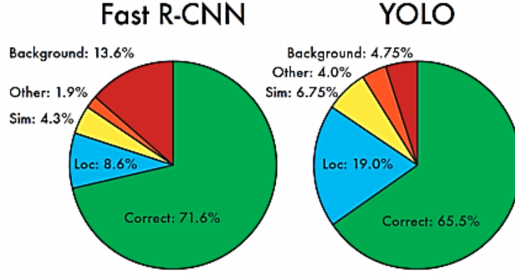
Figure 5.3: Ratio of samples and recognition[7][8][9]
