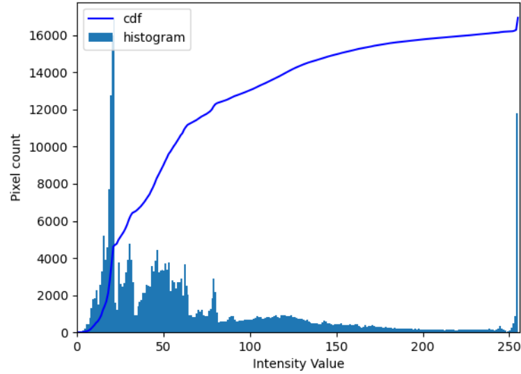
Figure 7.11: Histogram of subset 5, After applying CLAHE on subject 1
