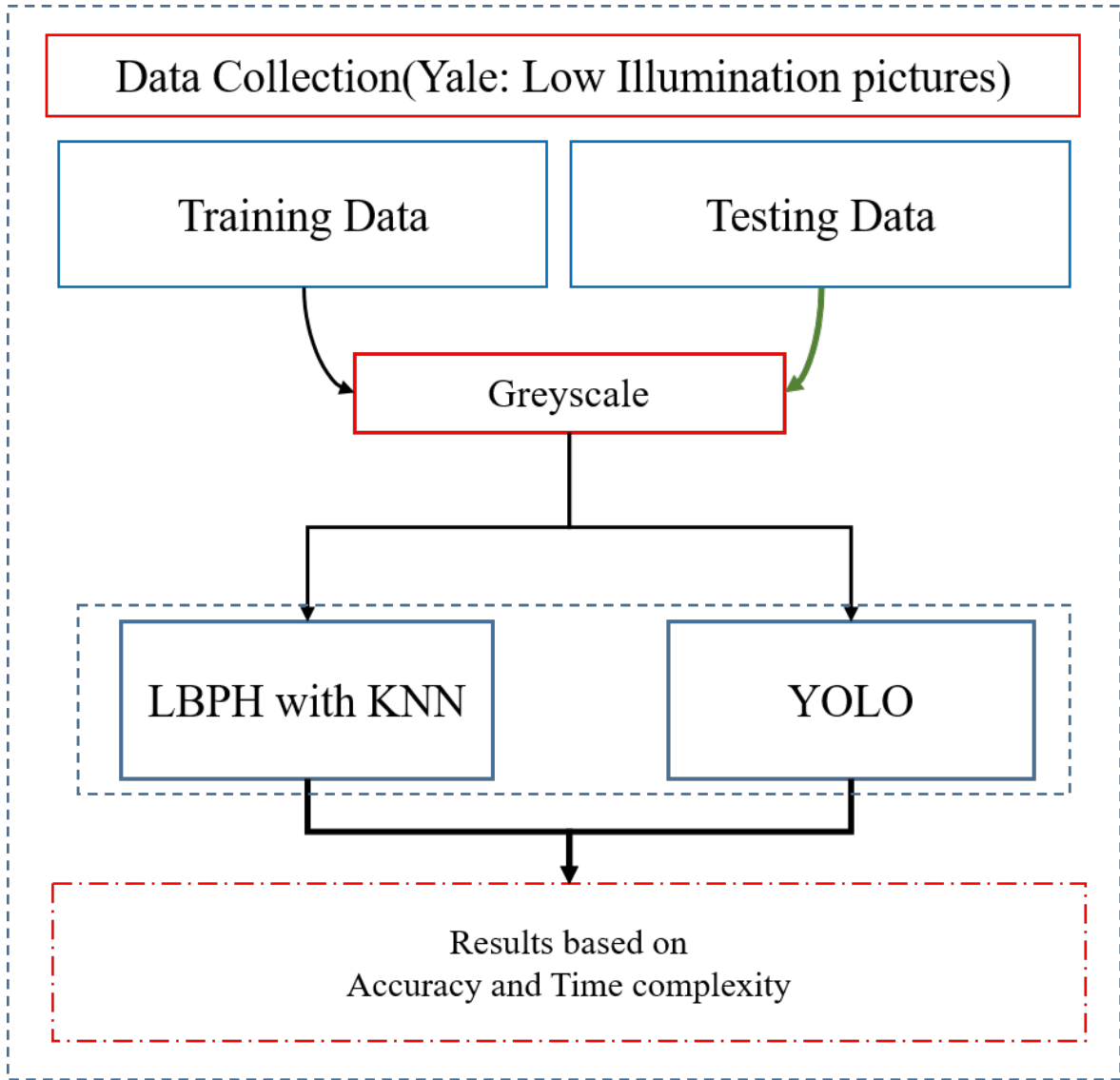
Figure 5.1: Research methodology
