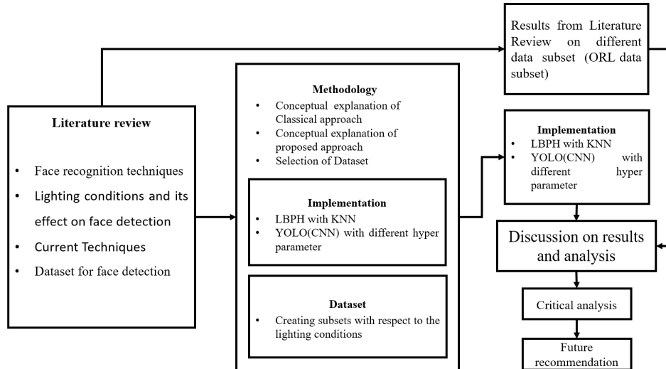
Figure 1.1: Research framework
