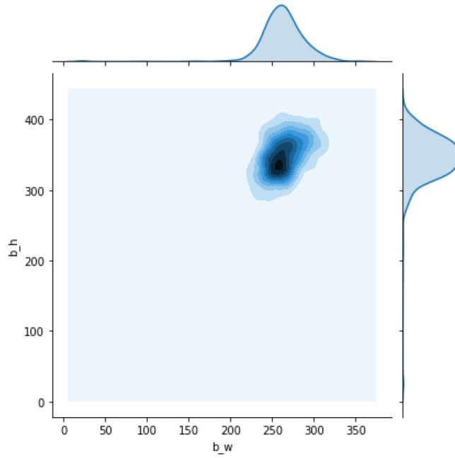
Figure 6.11: Kernel density estimation of data points
