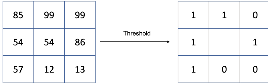
Figure 3.1: Basic LBP operator
