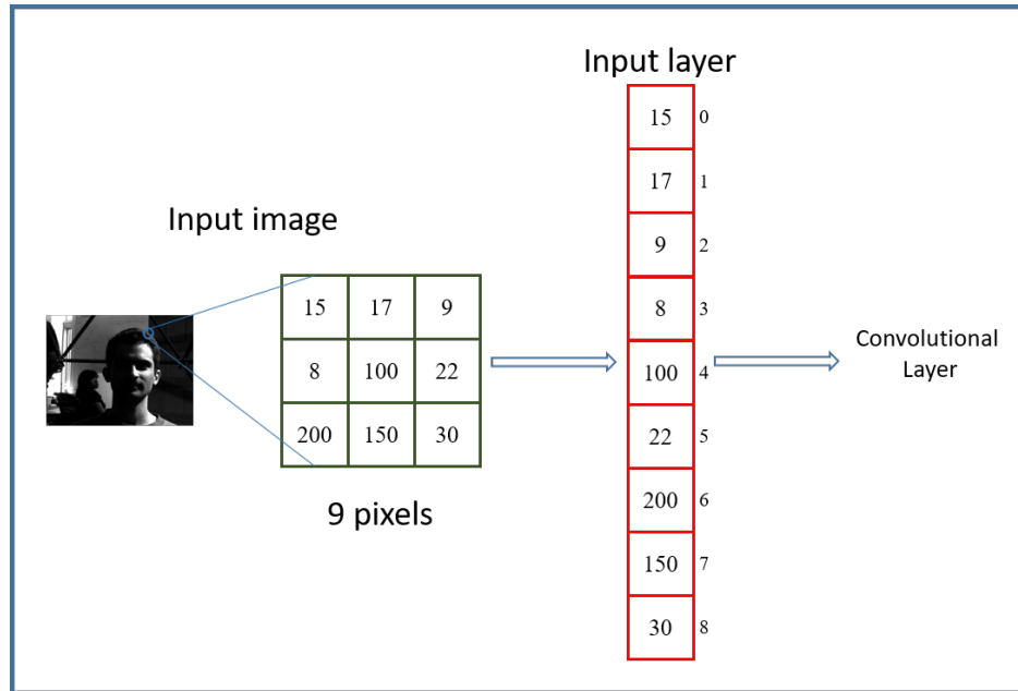
Figure 3.3: Workflow of Input layer in Convolutional Neural Network
