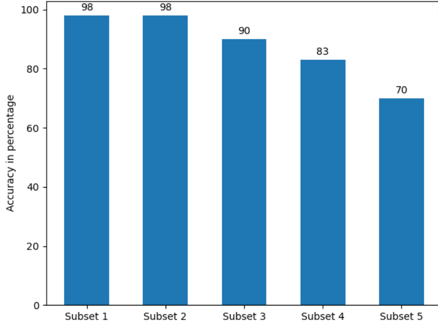
Figure 7.9: Results of YOLO on different subsets
