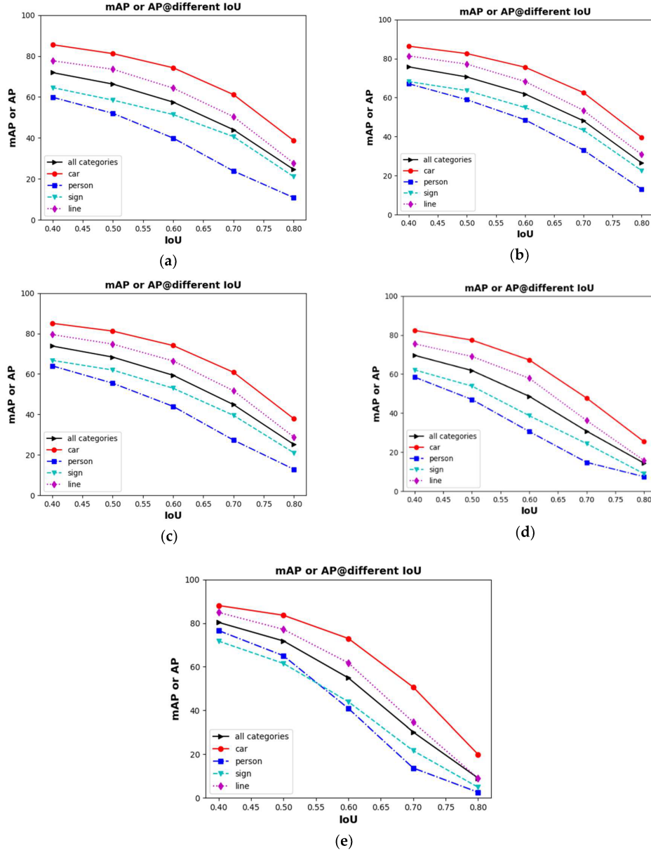
Figure 2.5: Detection performance under different IoU threshold for each detector when predicting. (a) Faster RCNN(VGG-16); (b) Faster RCNN(ResNet-101); (c) R-FCN(ResNet-101); (d) SSD(InceptionV2); (e) YOLOv3 (Darknet53) [5].
