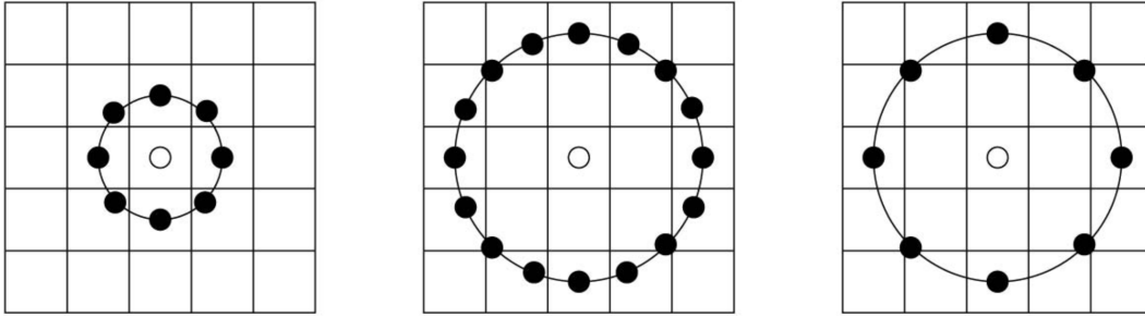
Figure 3.2: The circular (8,1) , (16,2) , and (8,2) neighborhoods. The pixel values are bilinearly interpolated whenever the sampling point is not in the center of a pixel[6]
